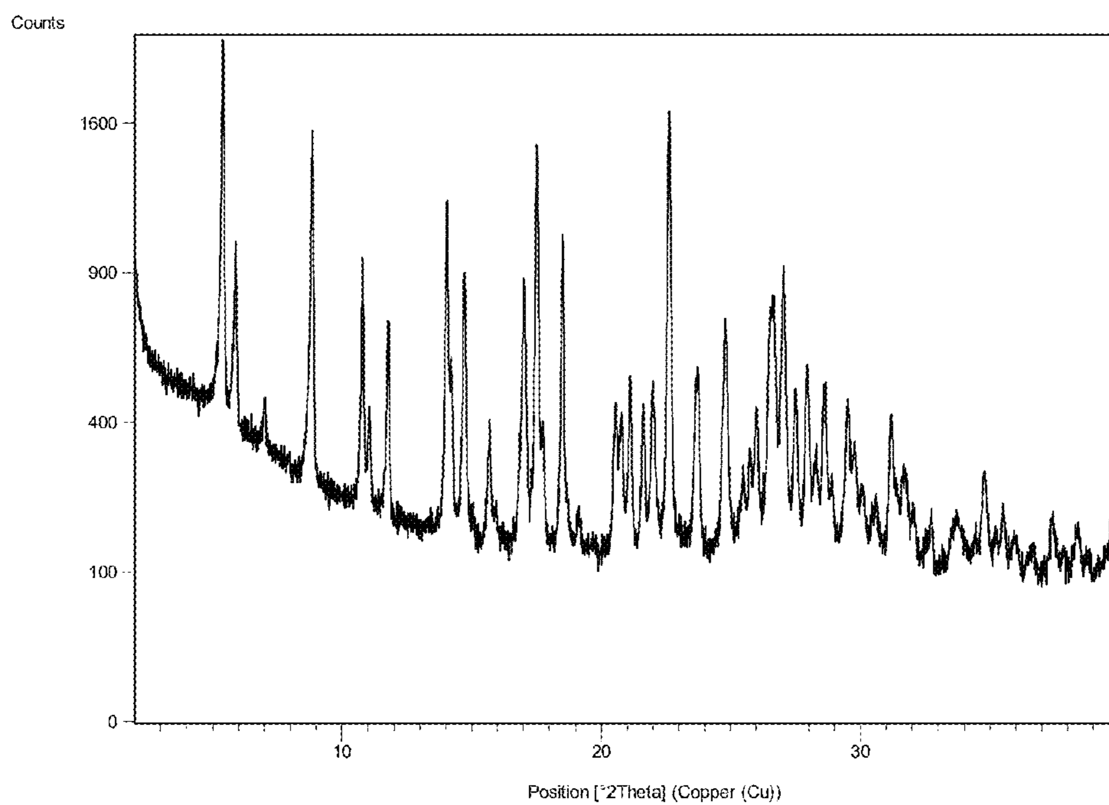
XRPD Pattern of the CEP-37440 trihydrochloride dihydrate salt
