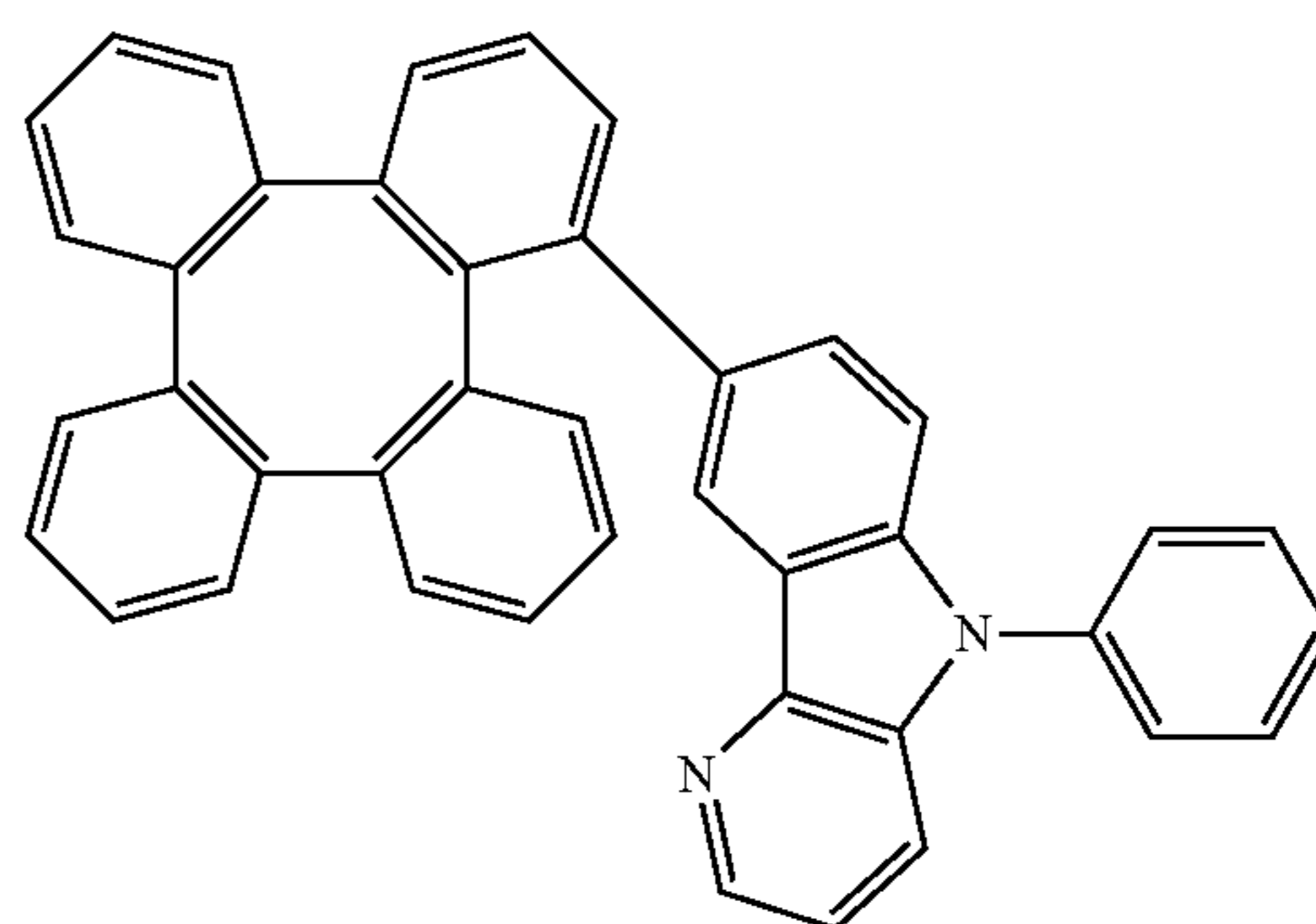
Compound 20
