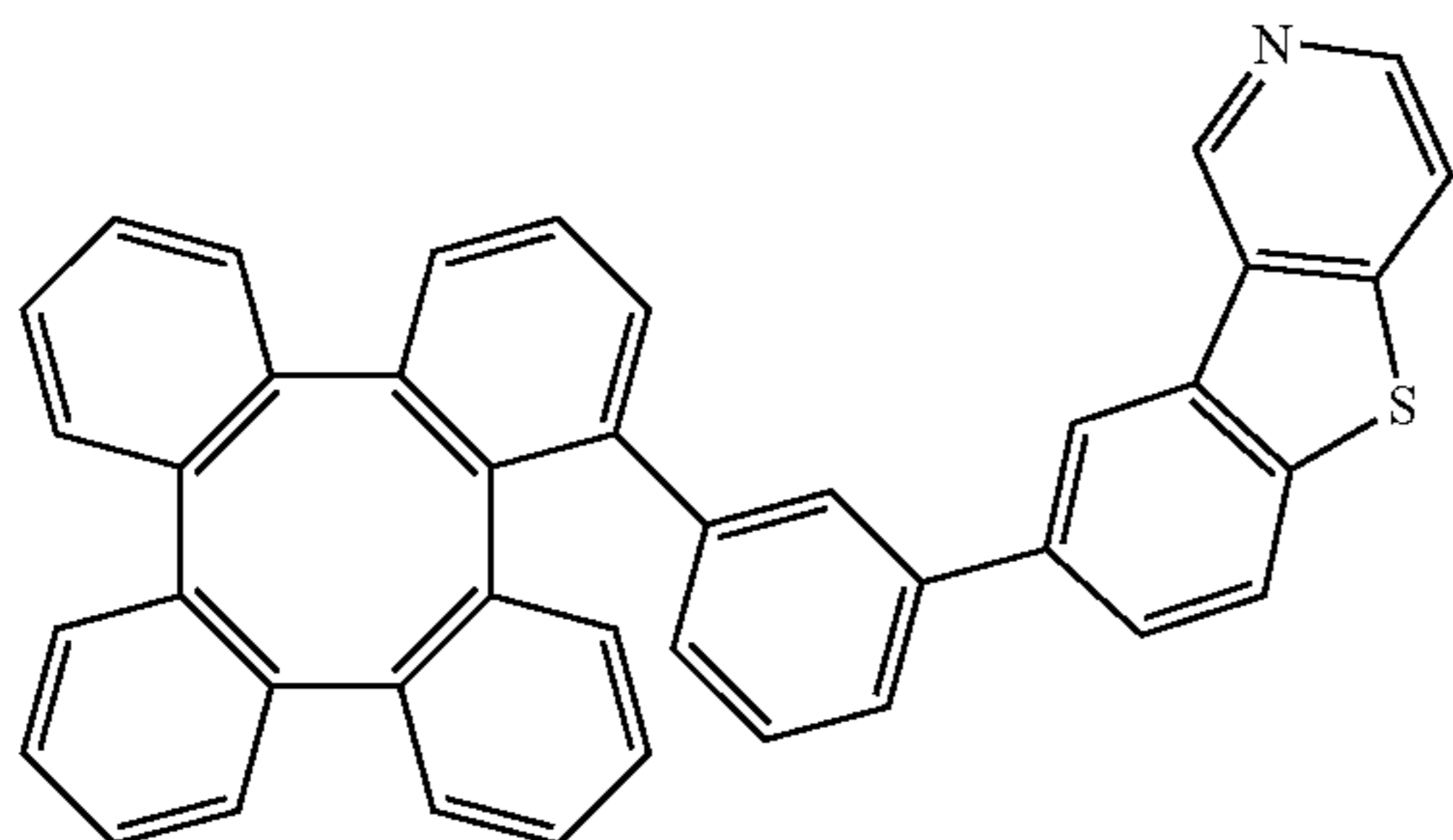
Compound 178
