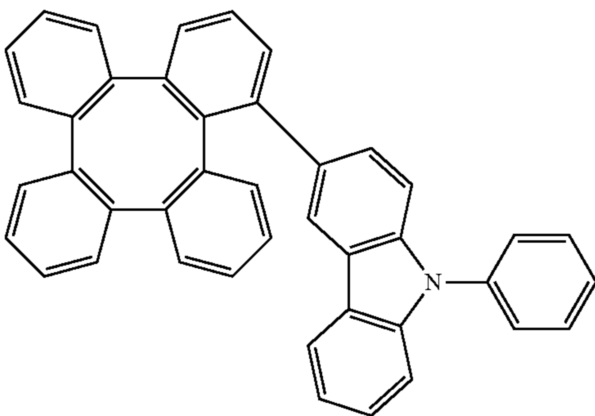
Compound 12
