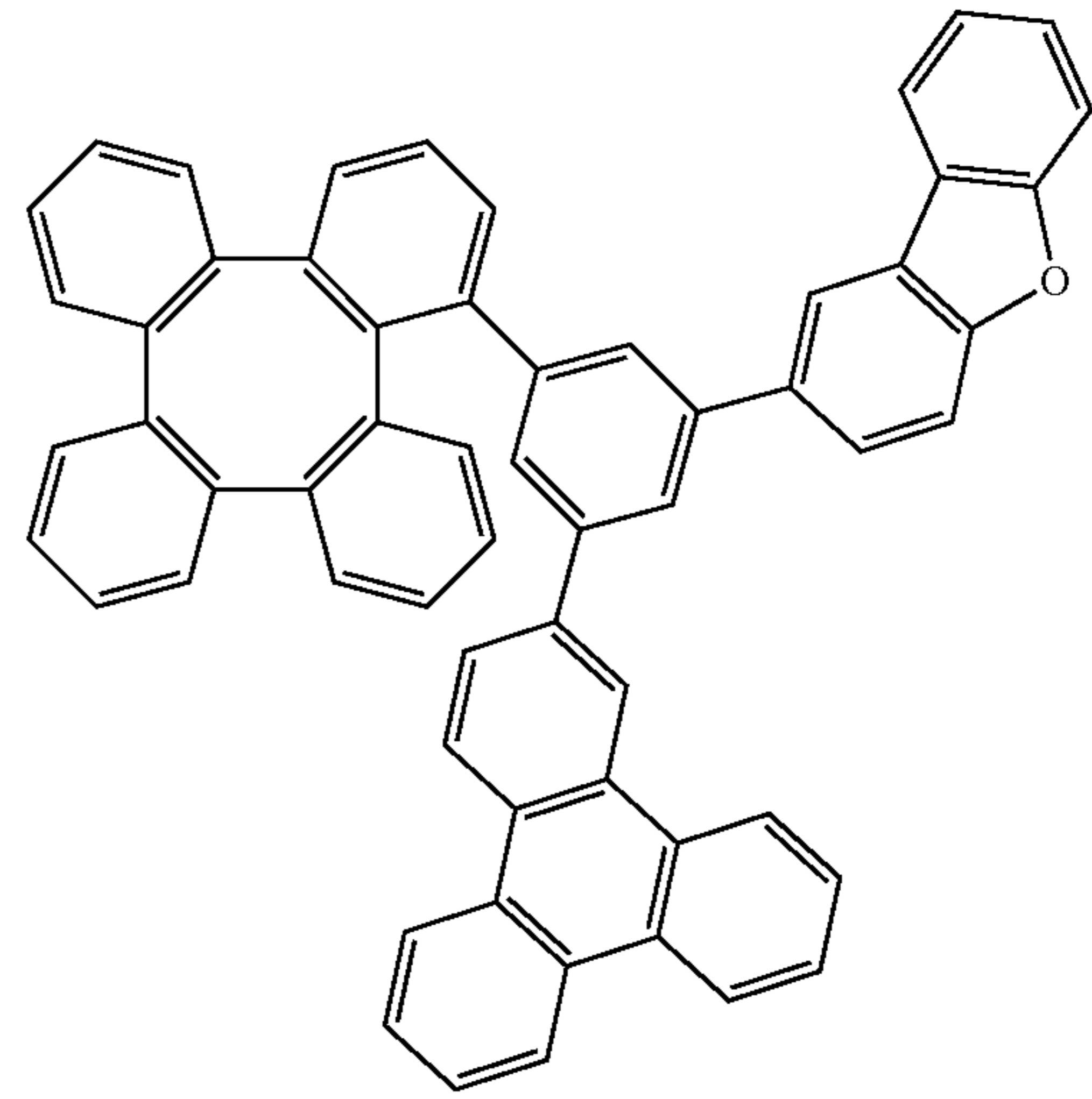
Compound 322
