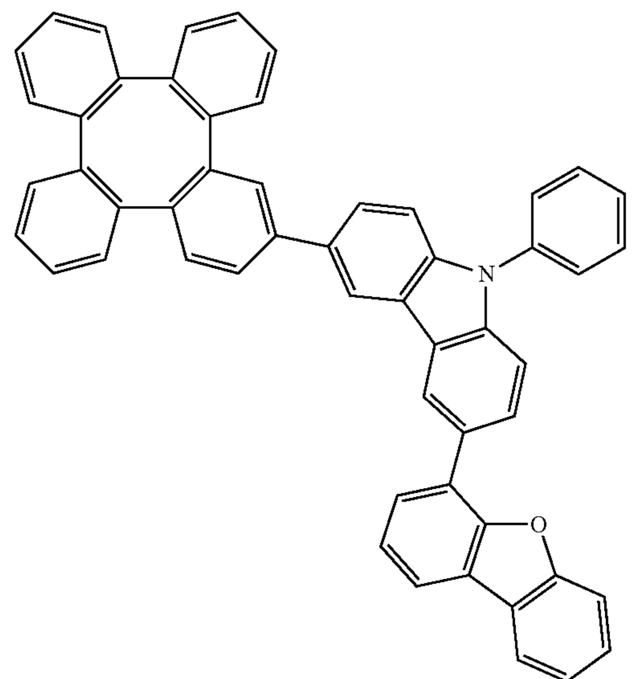
Compound 433
