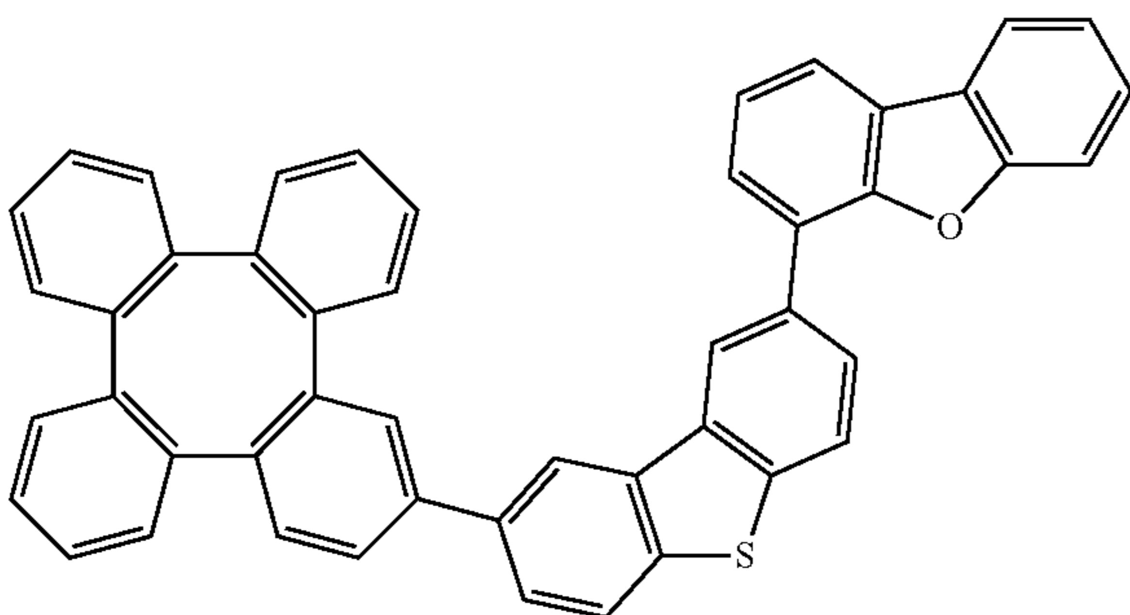
Compound 446
