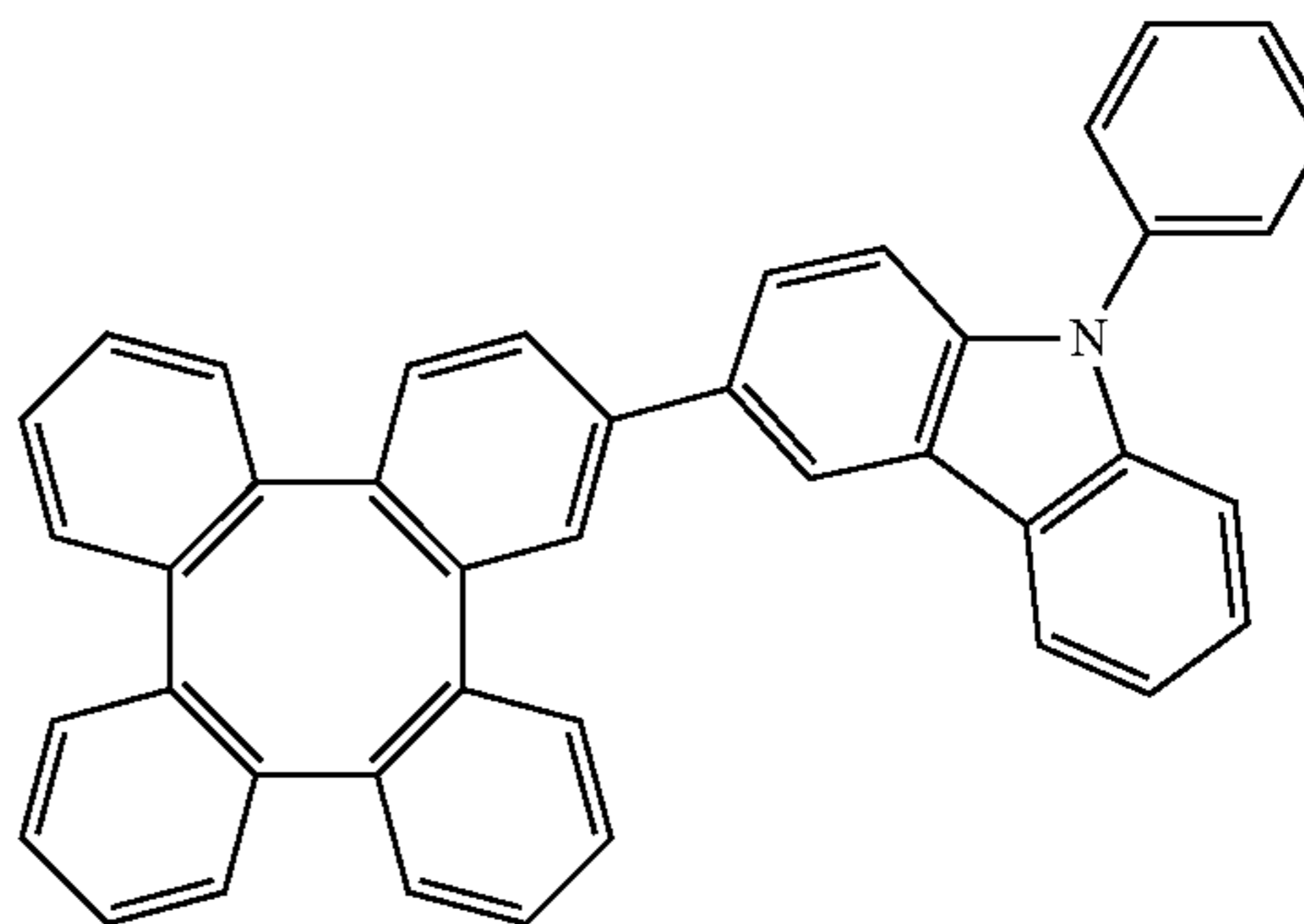
Compound 11
