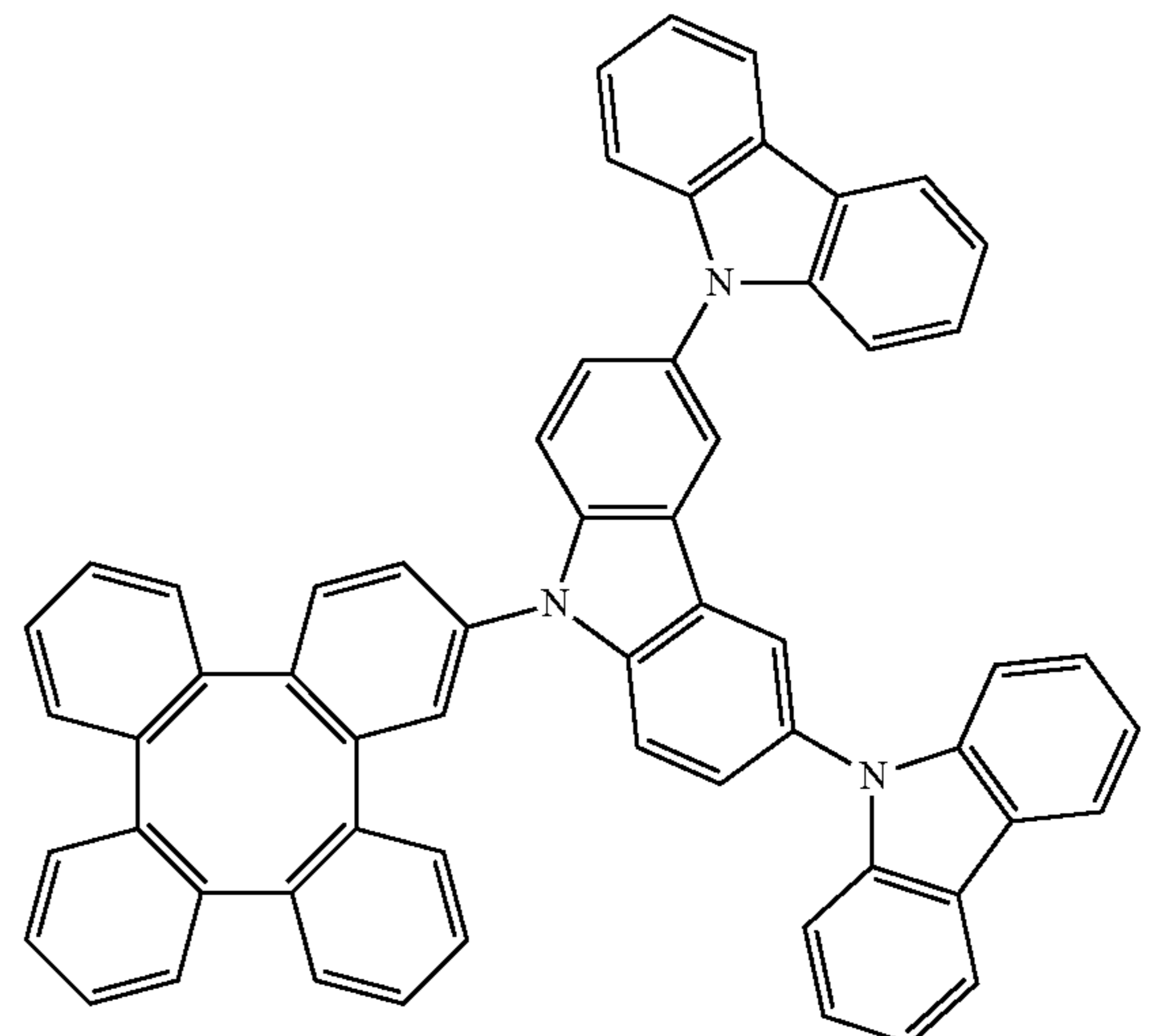
Compound 475
