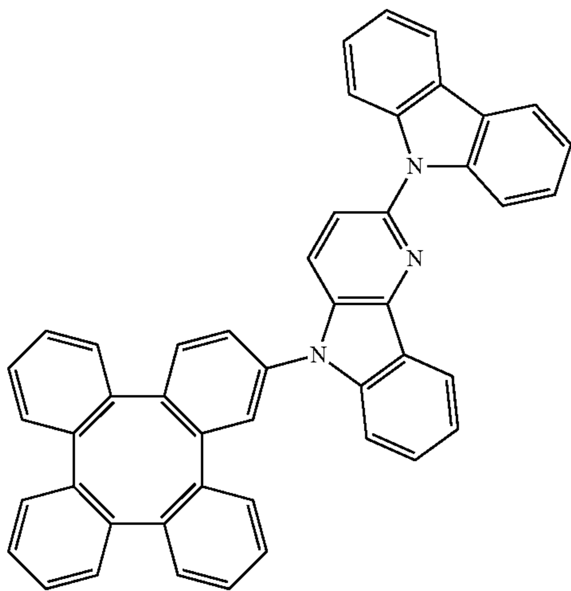
Compound 486
