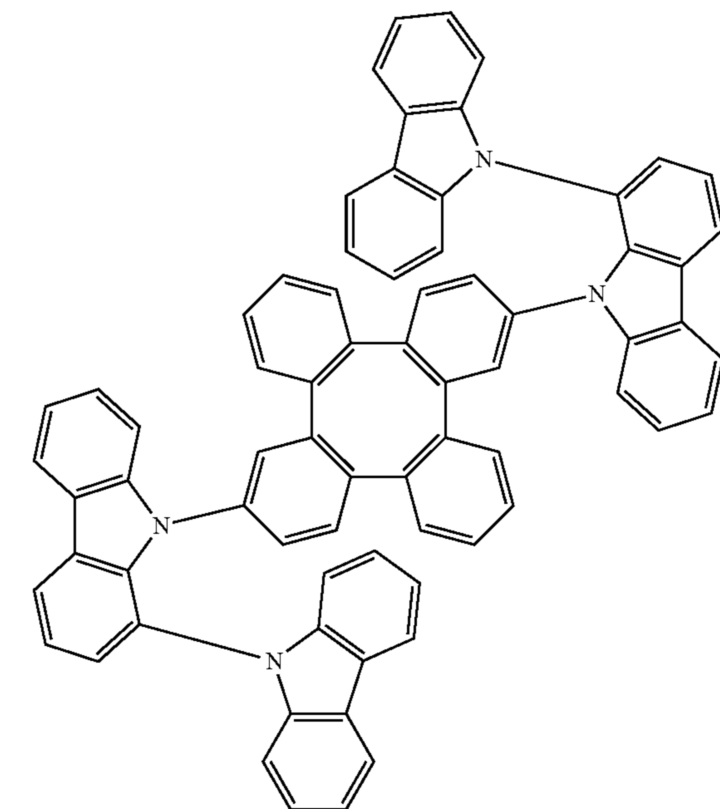
Compound 500
