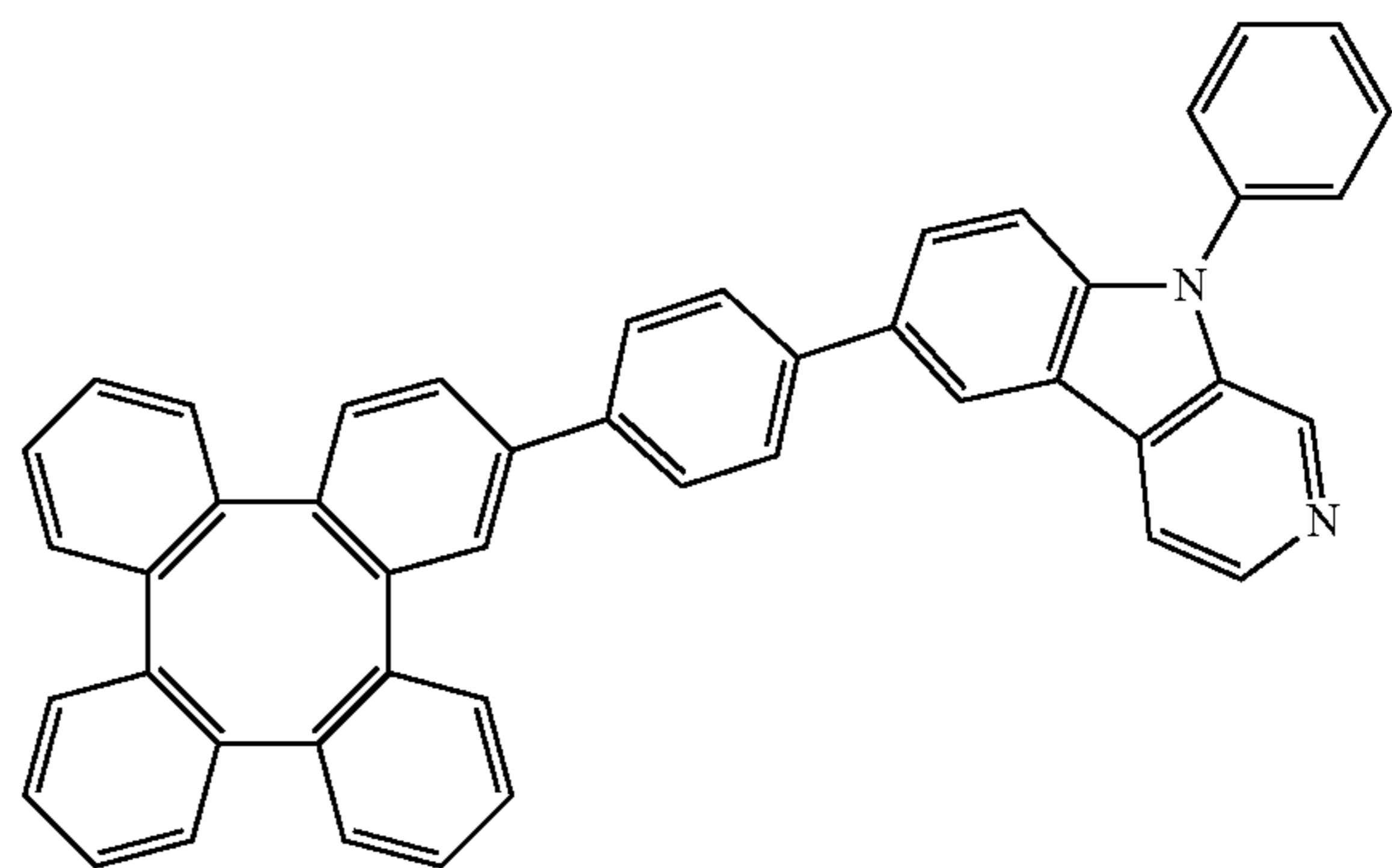
Compound 85
