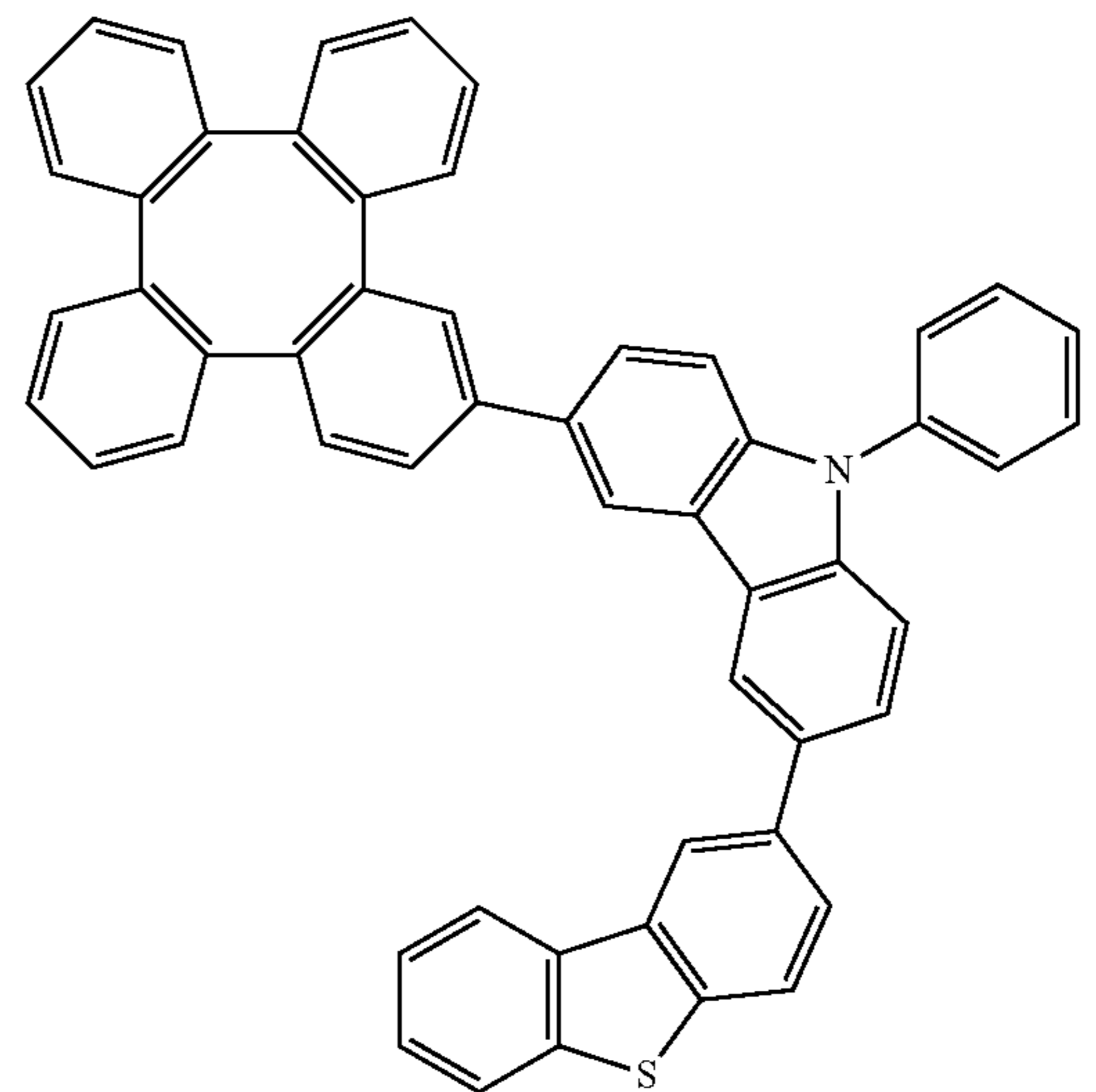
Compound 432
