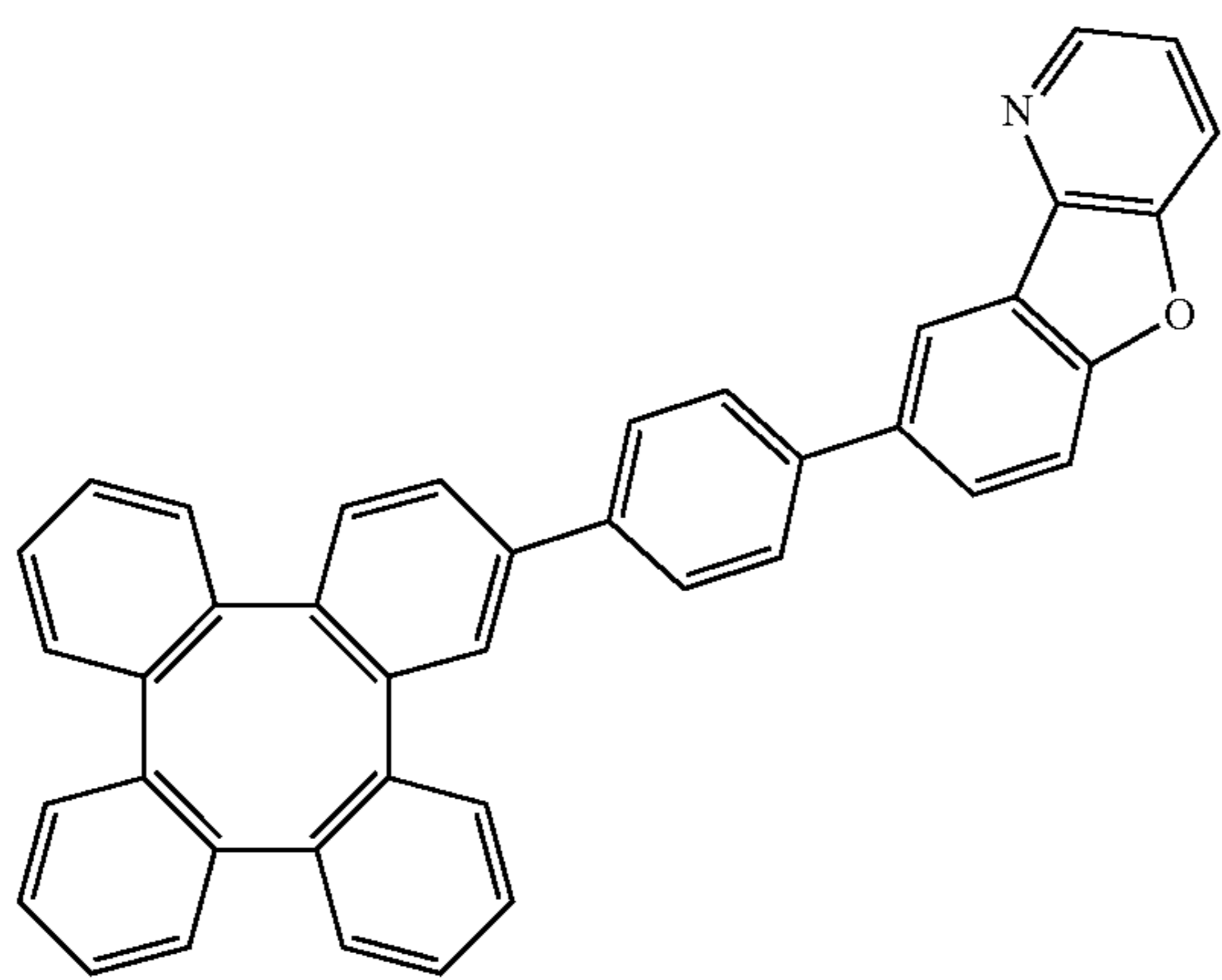
Compound 130
