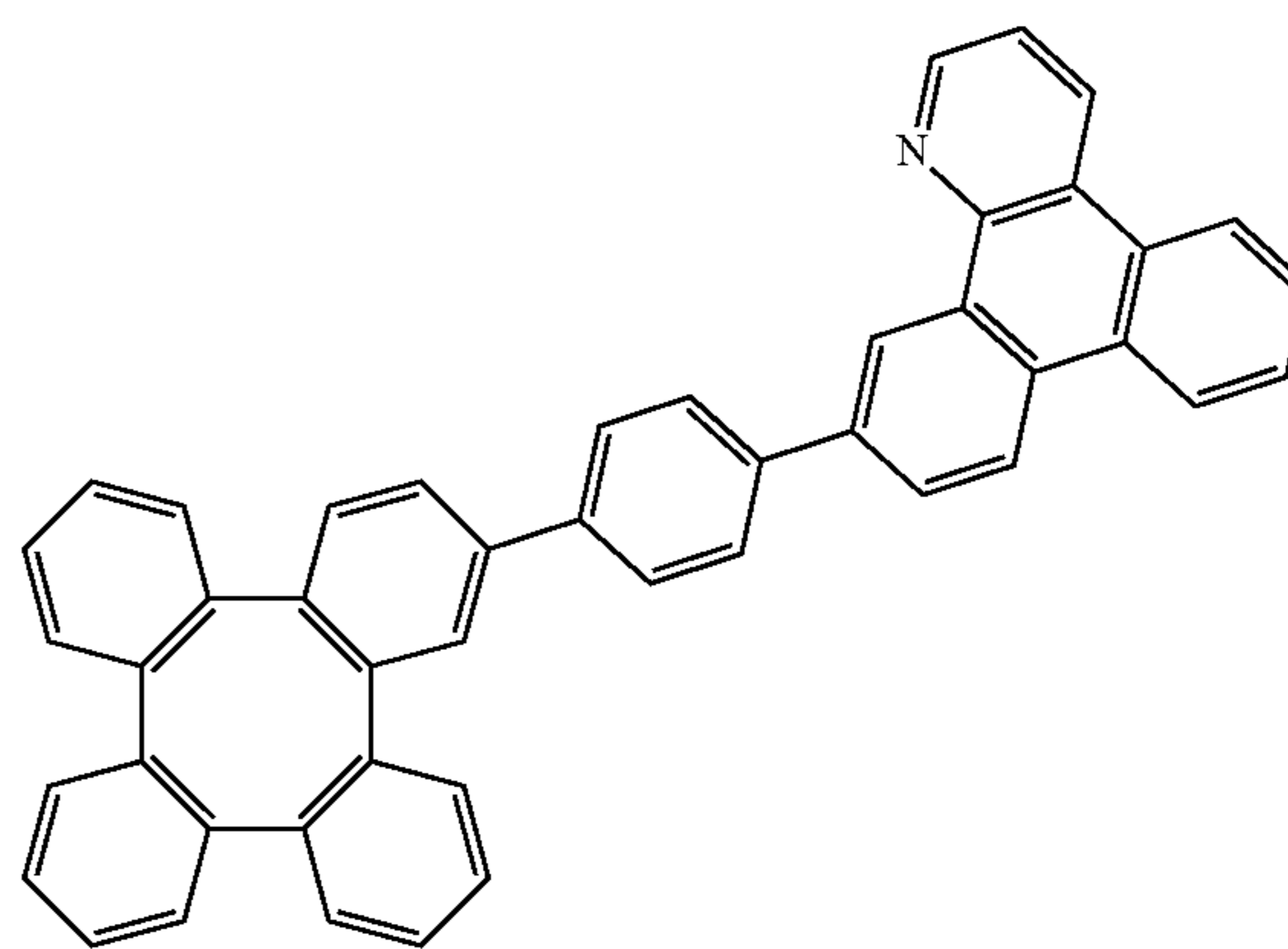
Compound 134
