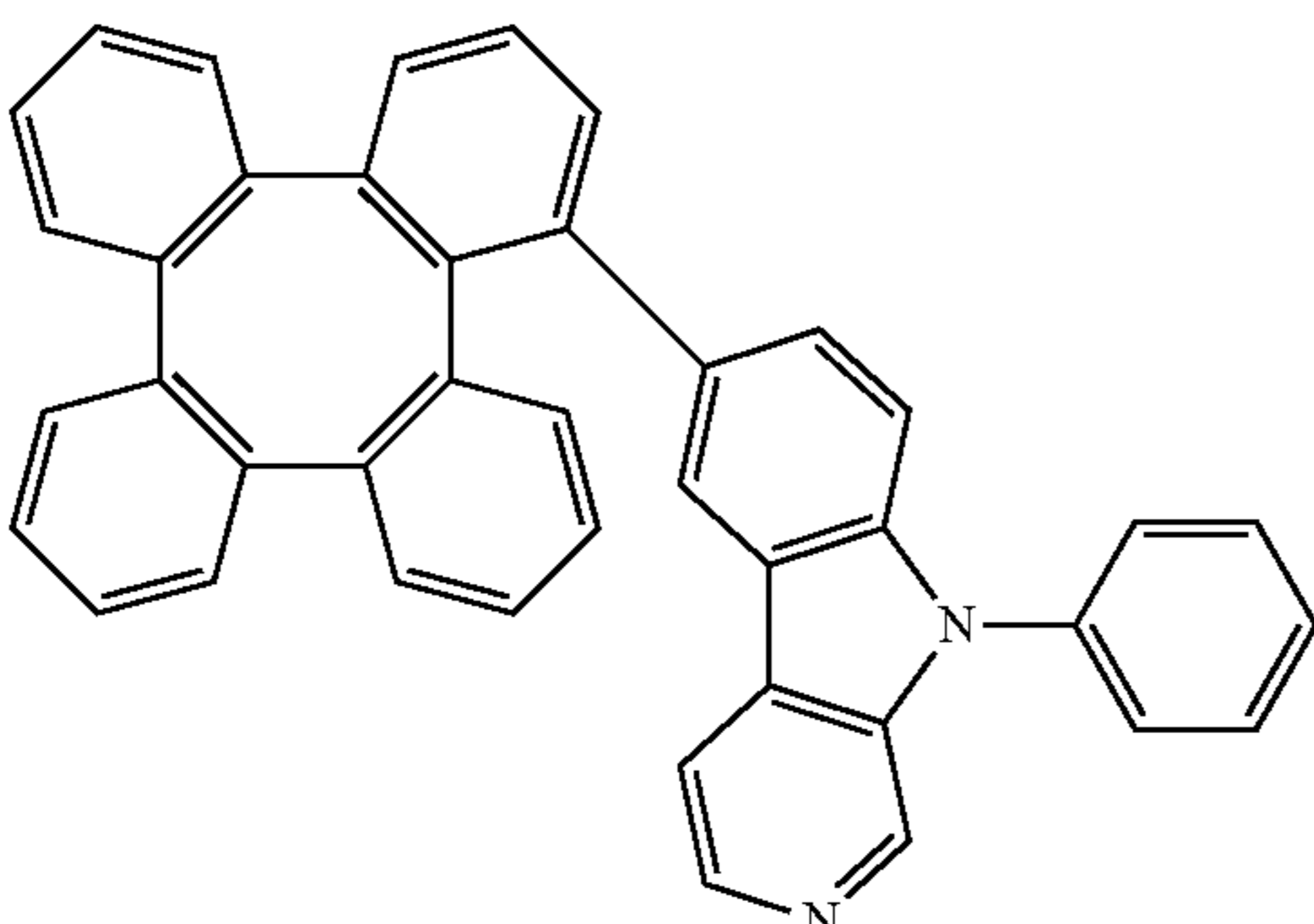
Compound 16
