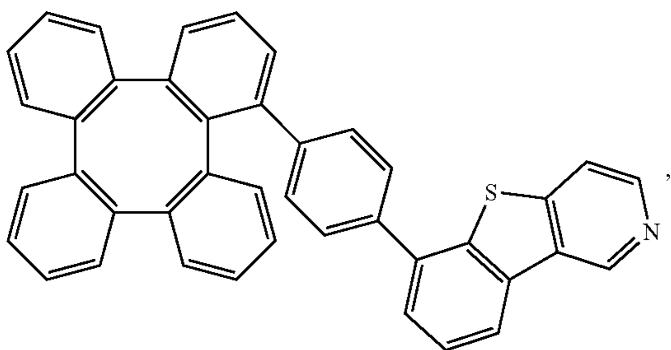
Compound 98
