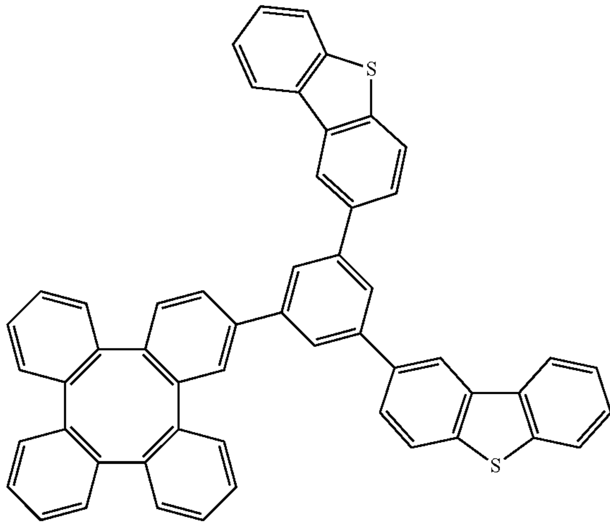
Compound 241
