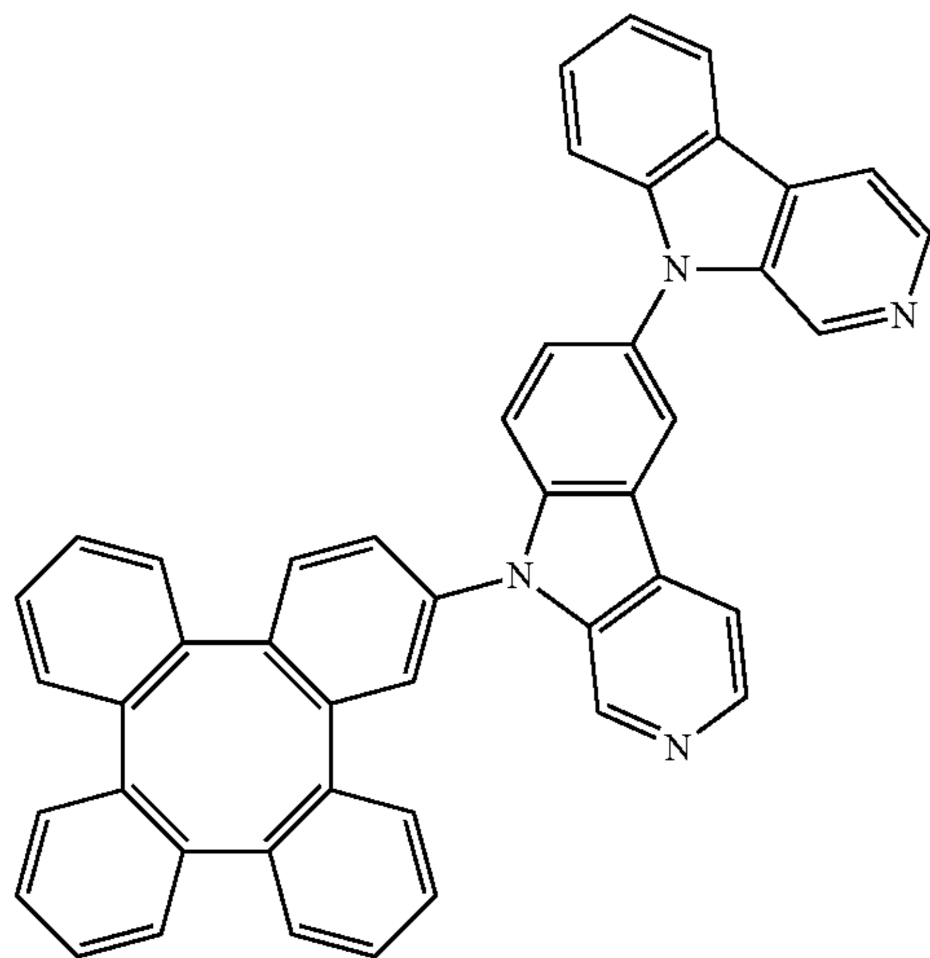
Compound 494
