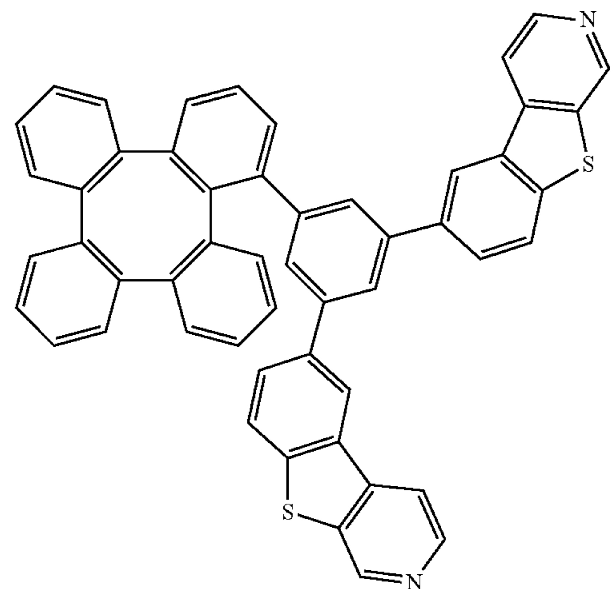
Compound 246
