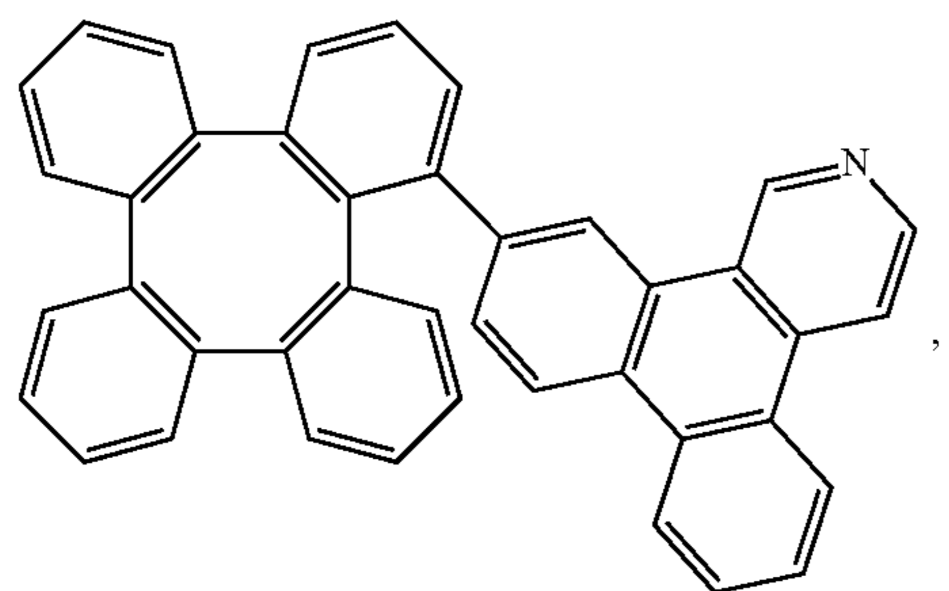
Compound 66
