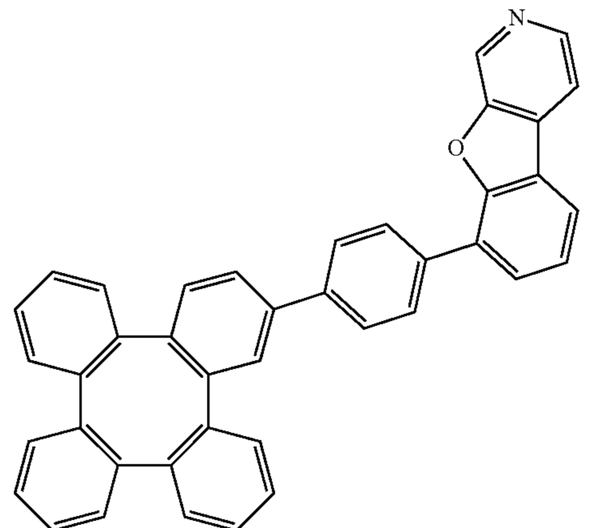
Compound 116
