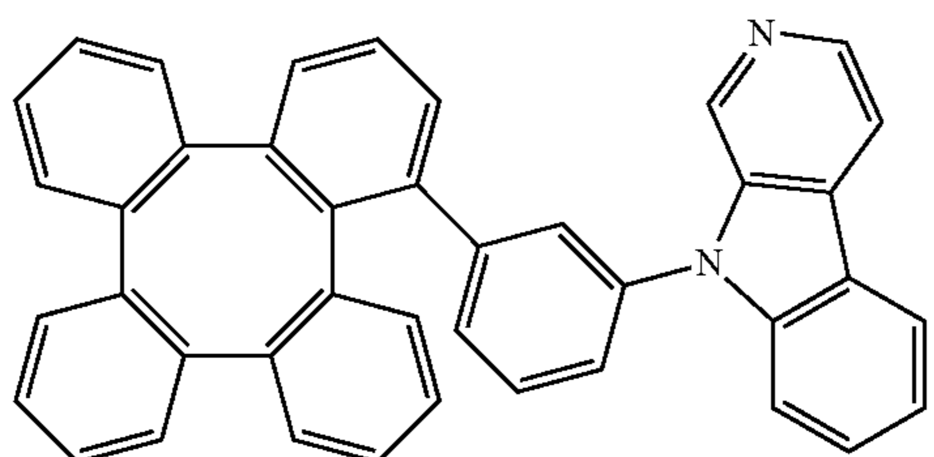
Compound 146
