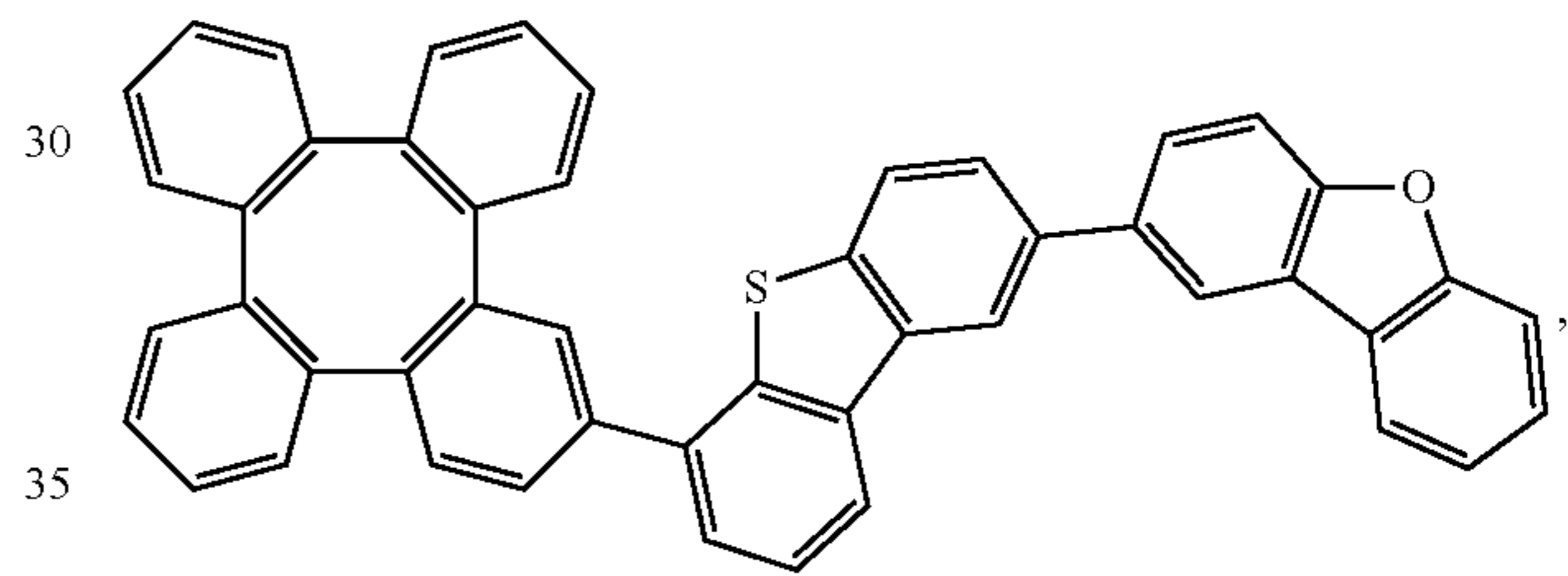
Compound 440
