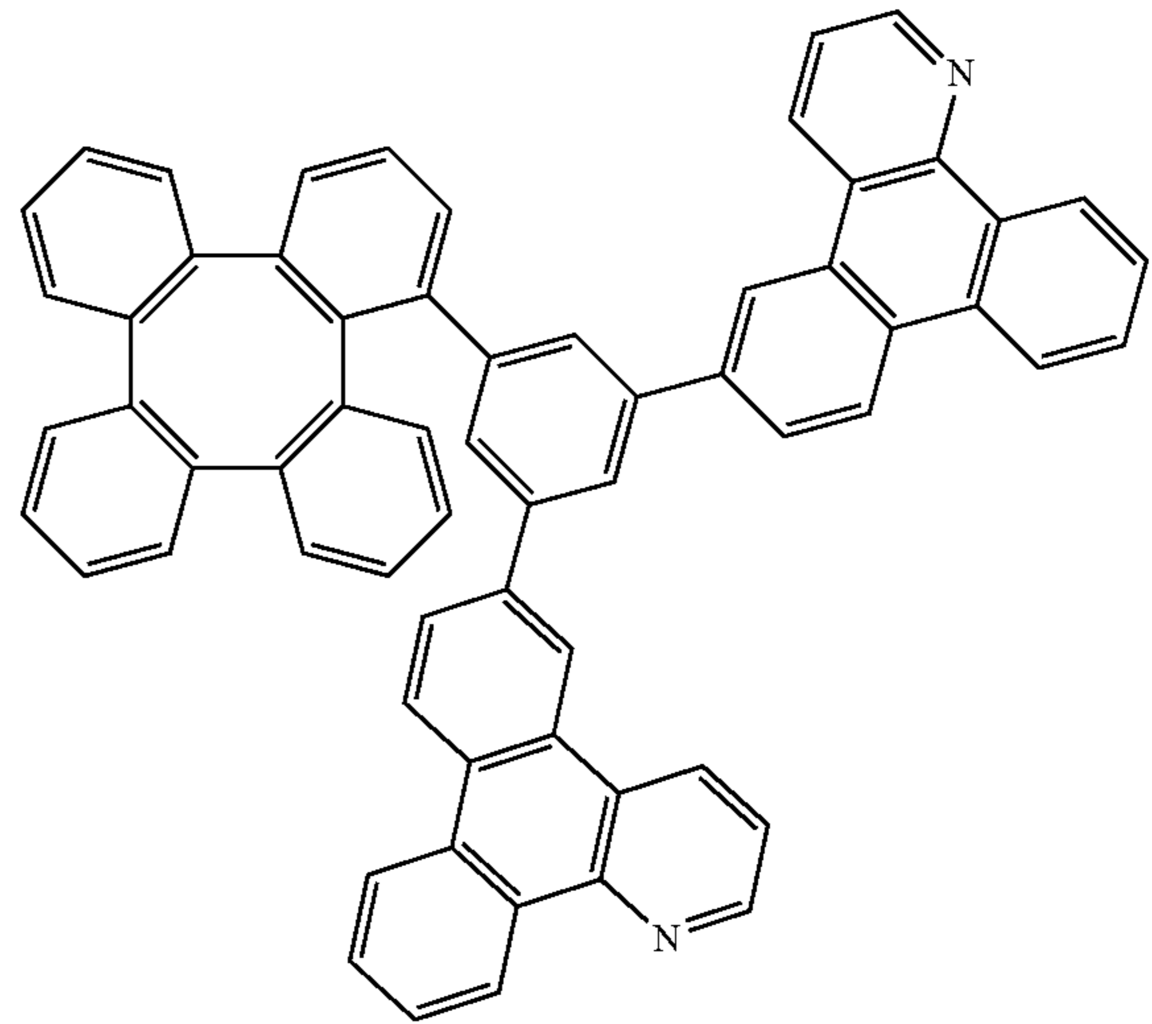
Compound 281
