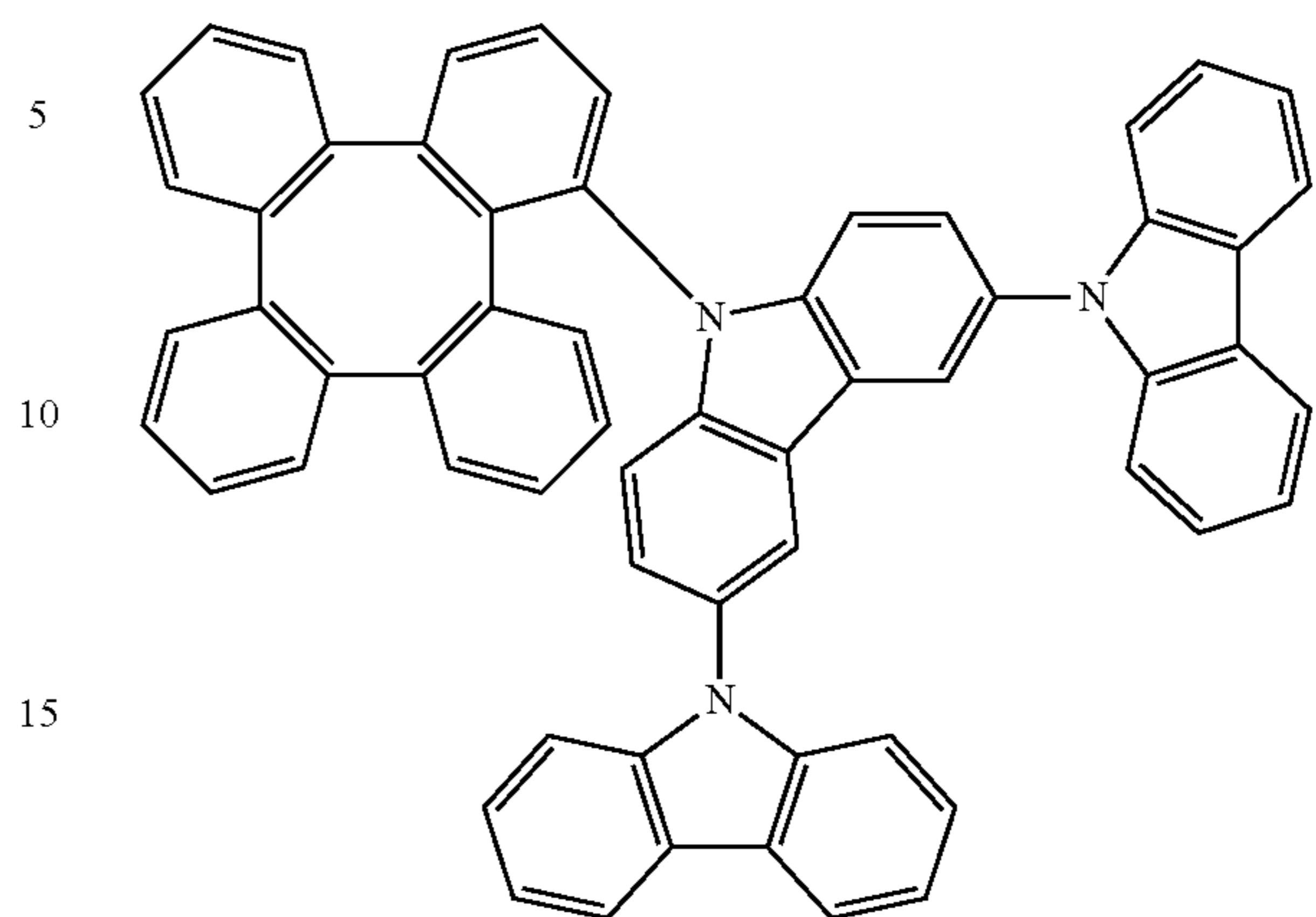
Compound 482
