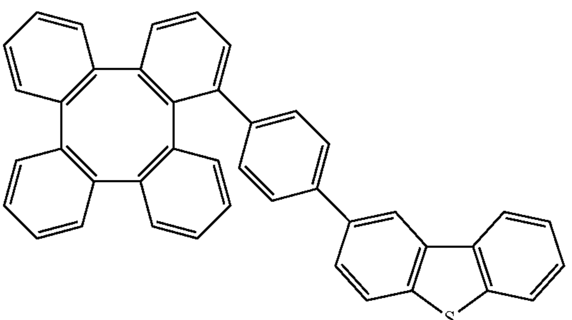
Compound 102
