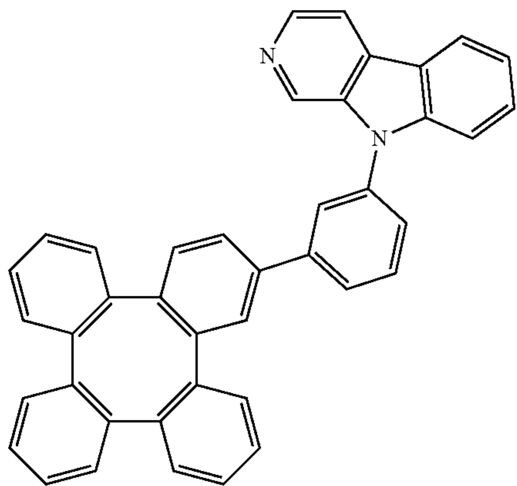
Compound 146
