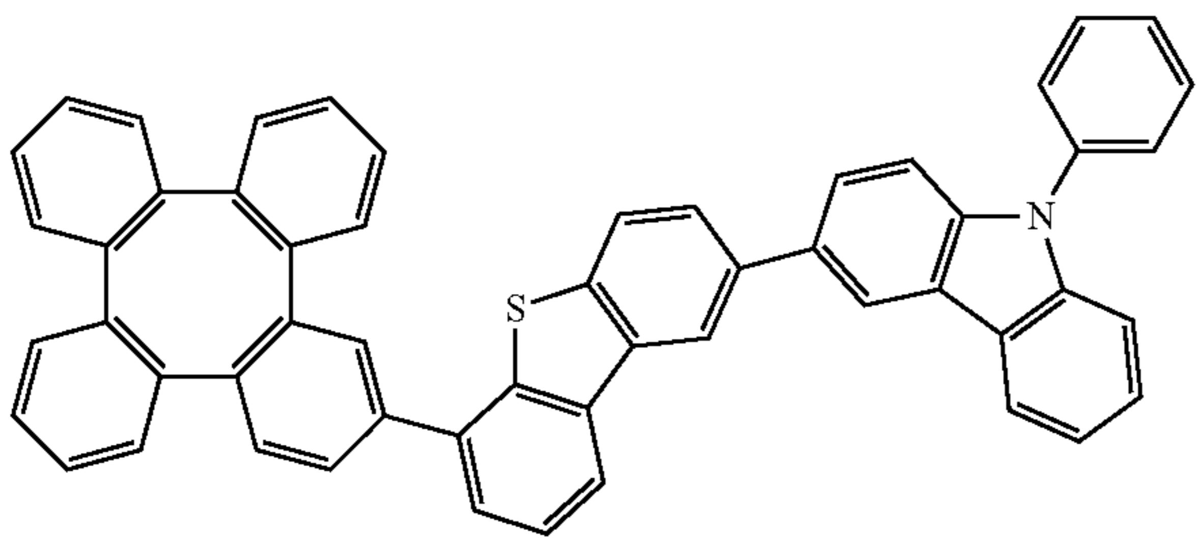
Compound 436
