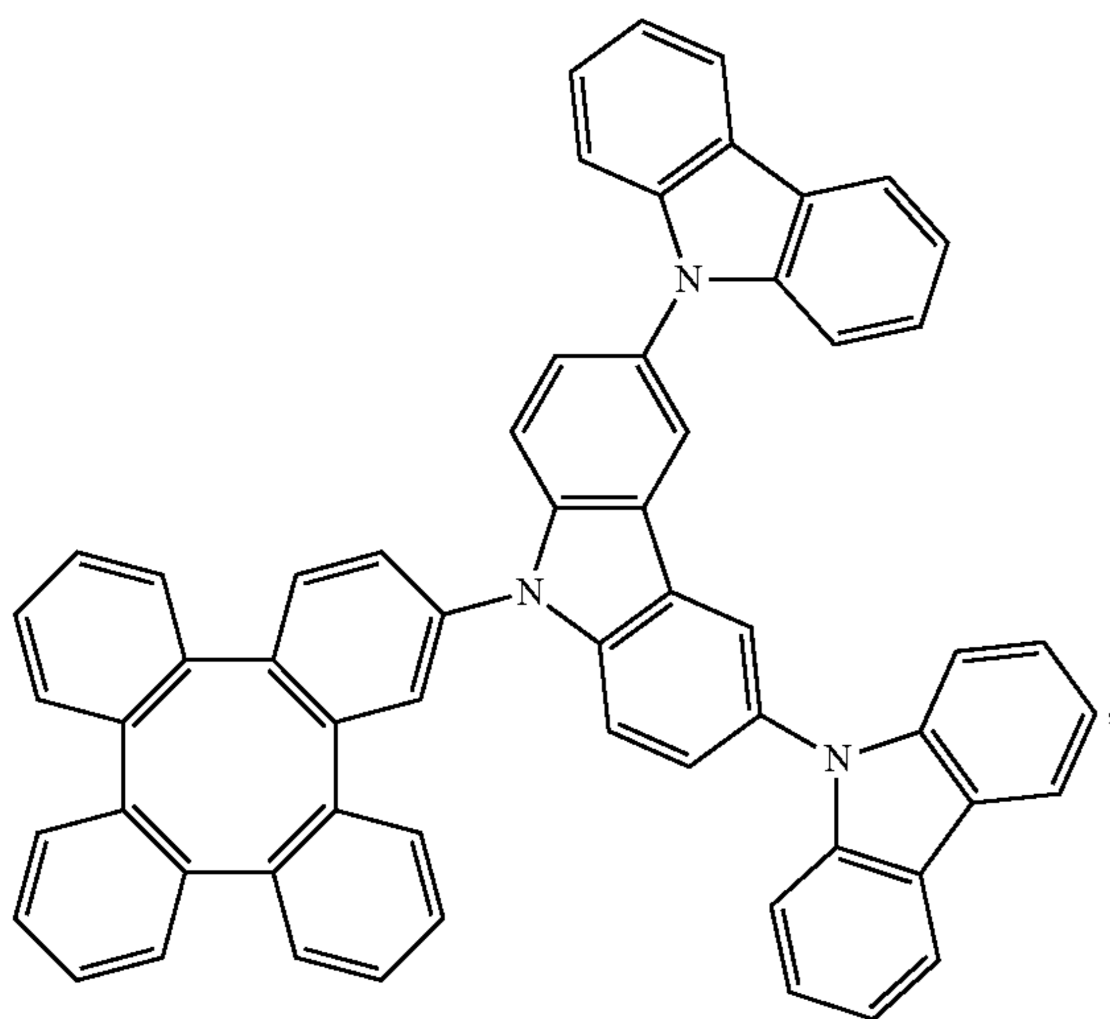
Compound 475
