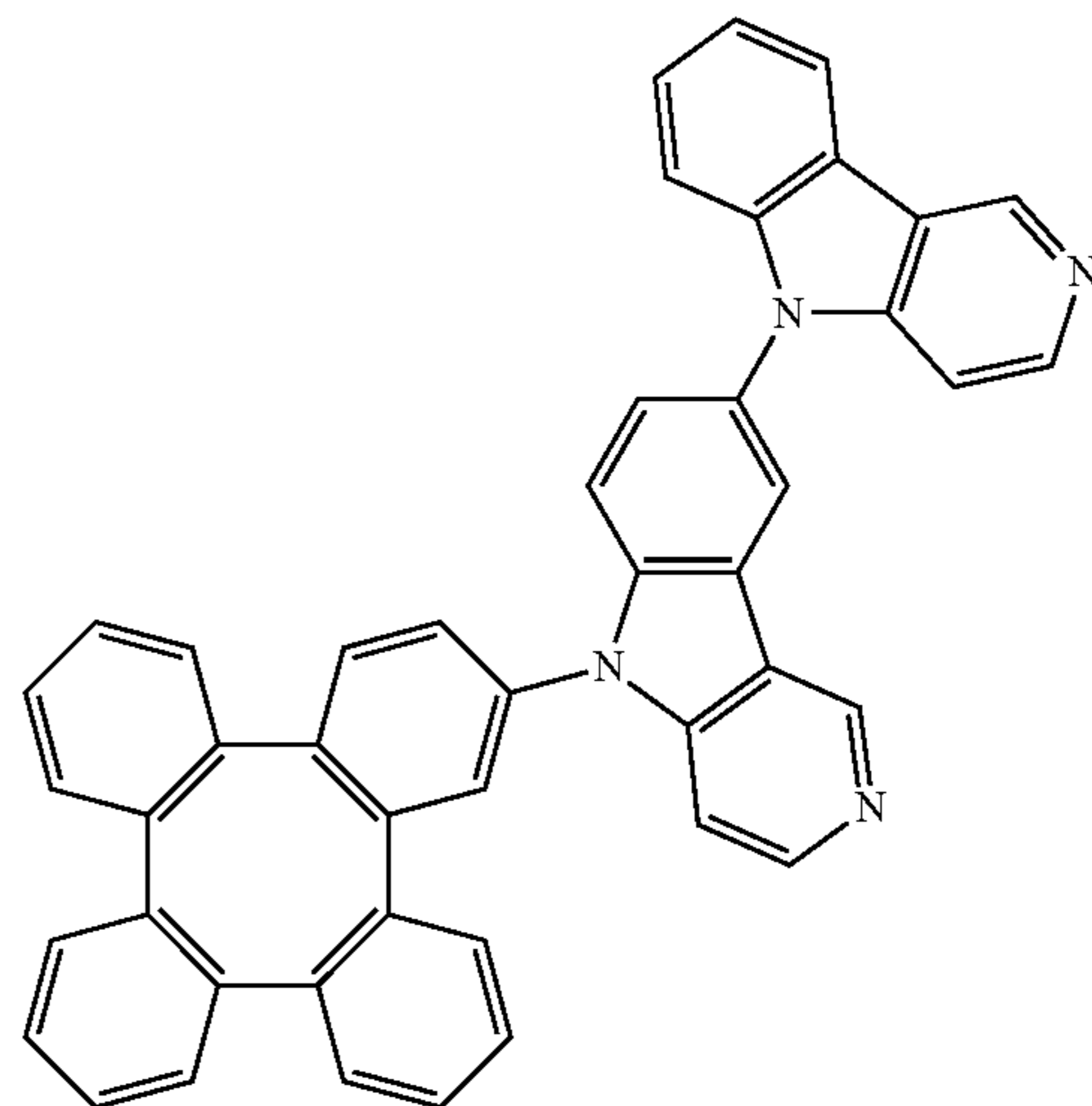
Compound 496
