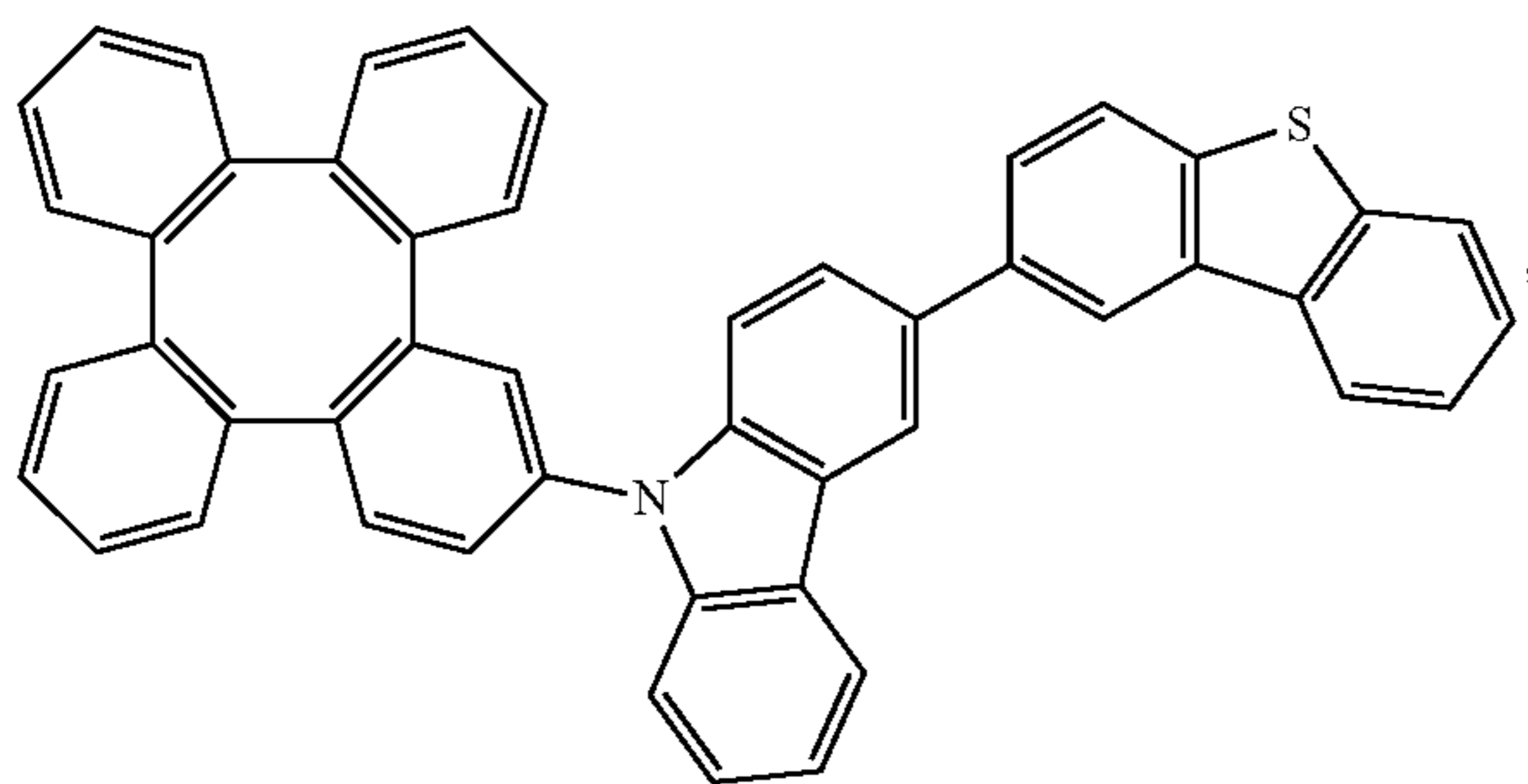
Compound 424
