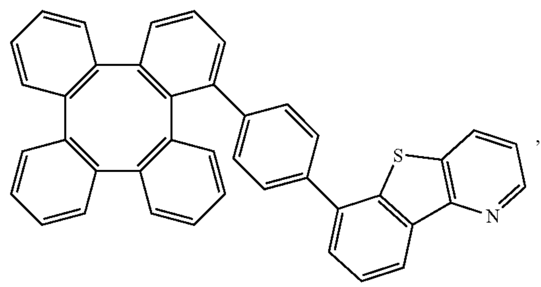
Compound 100
