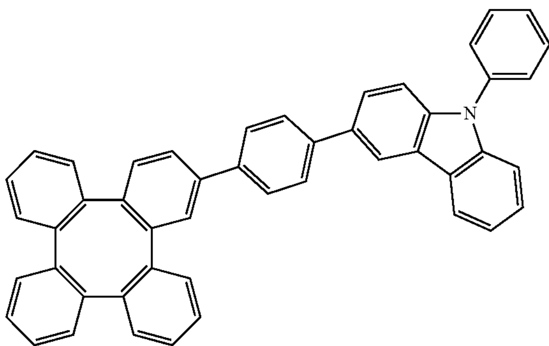
Compound 82
