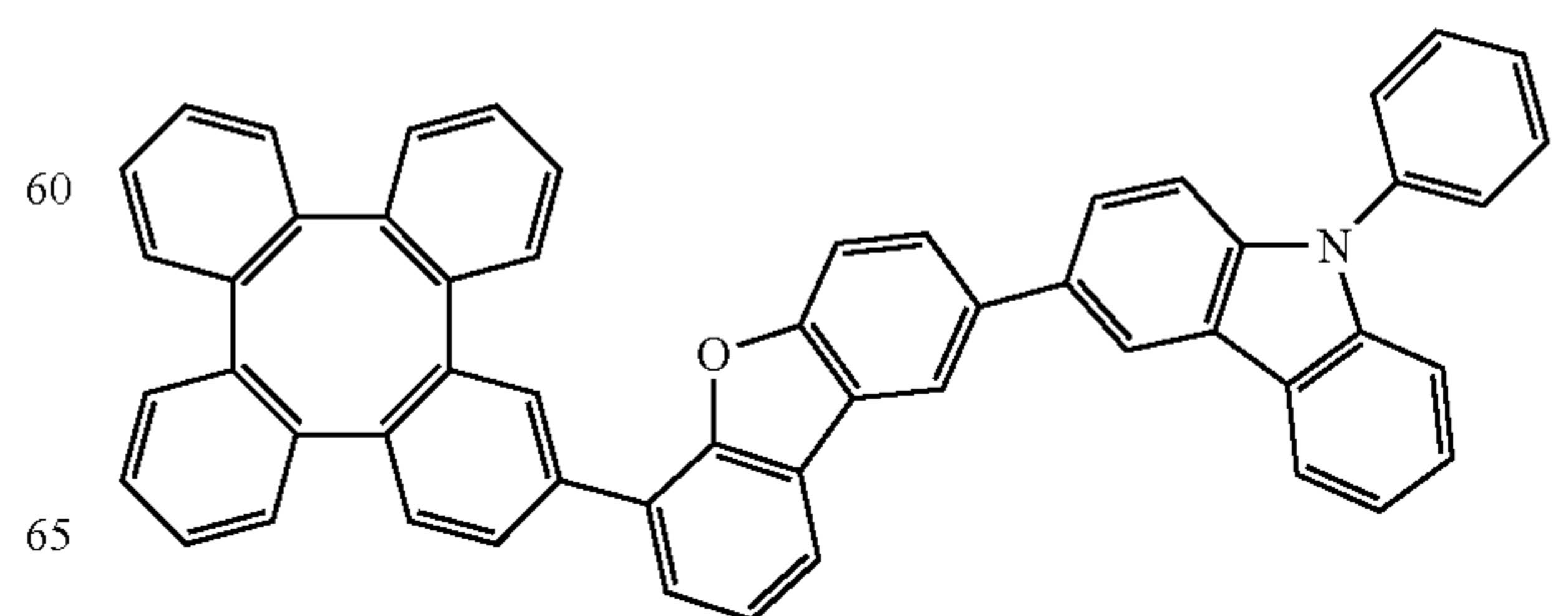
Compound 450
