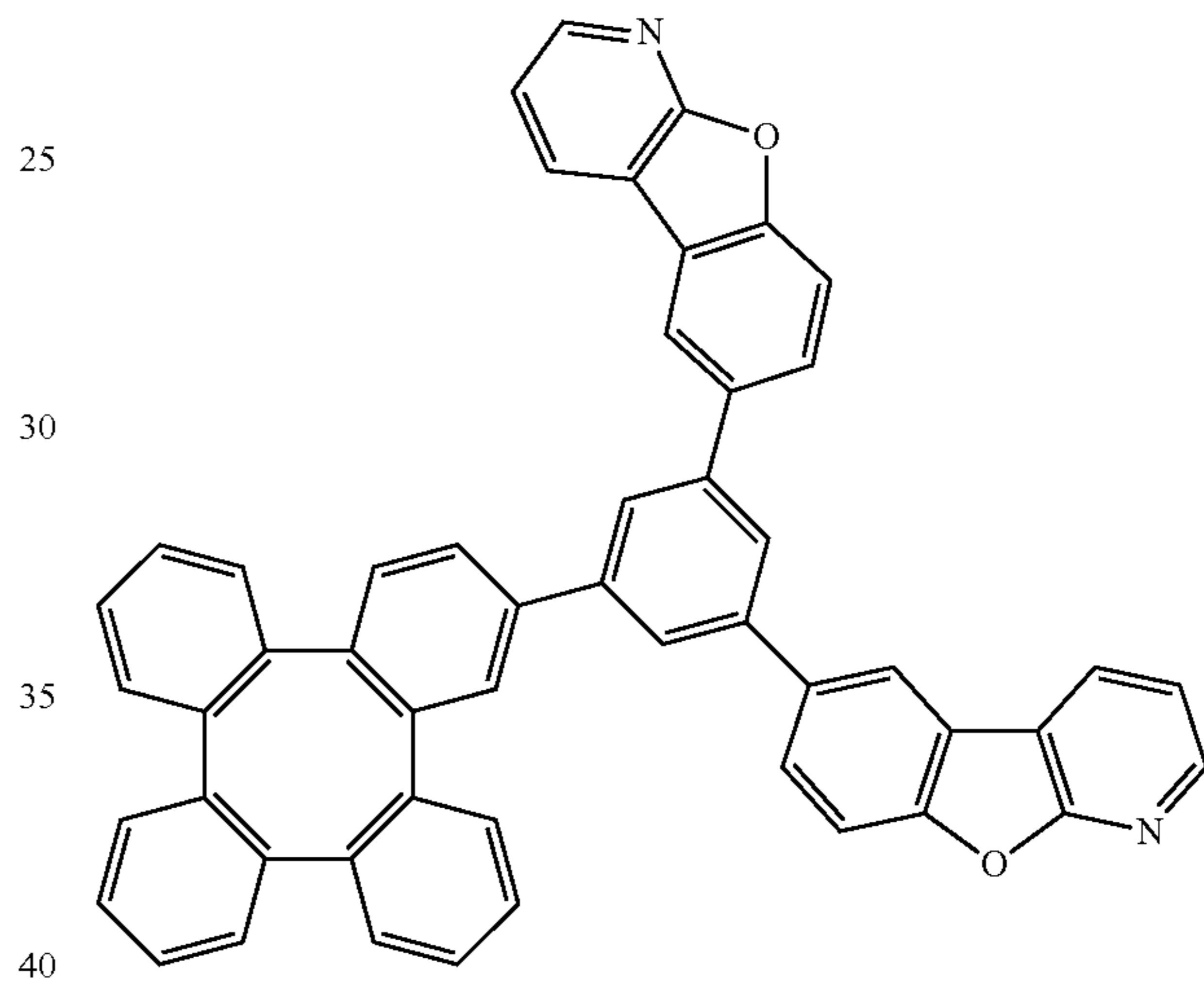
Compound 263
