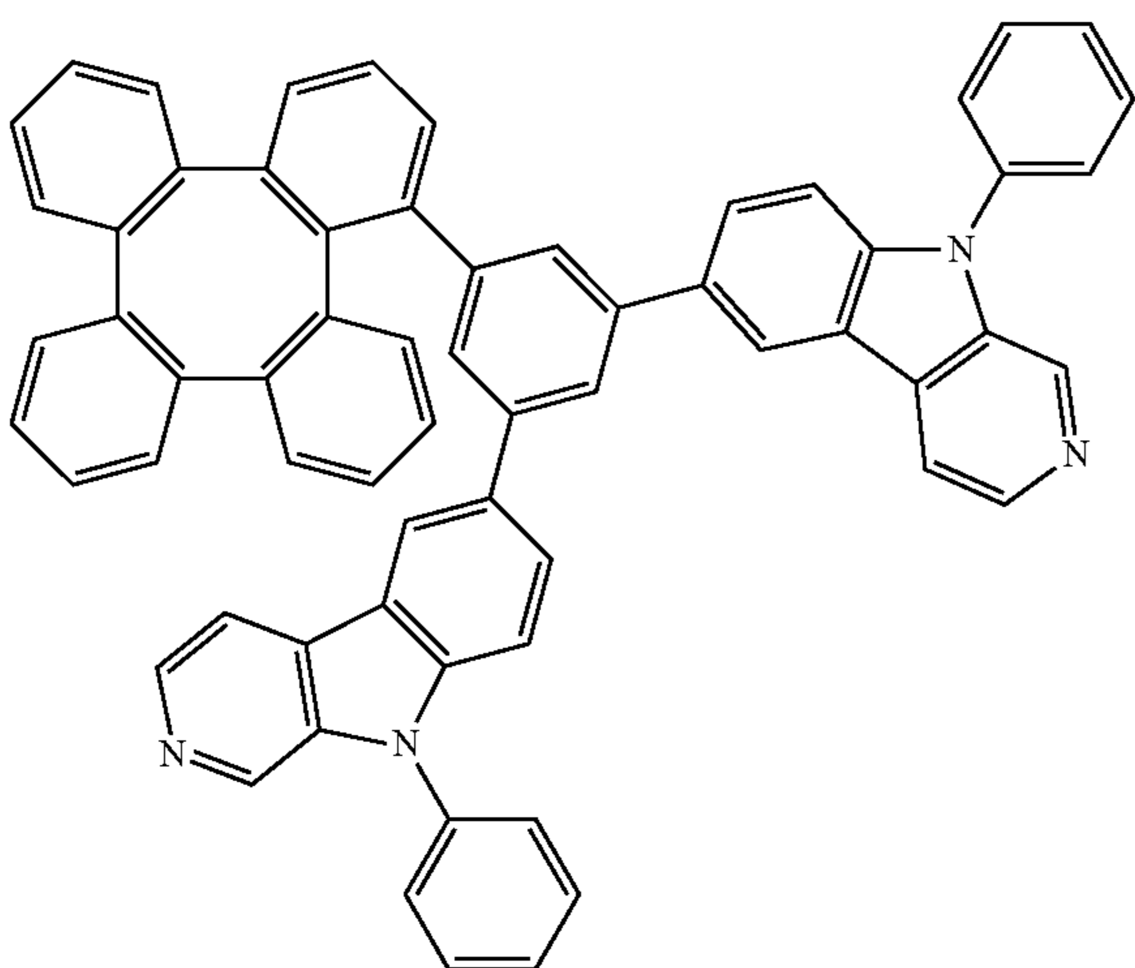
Compound 226
