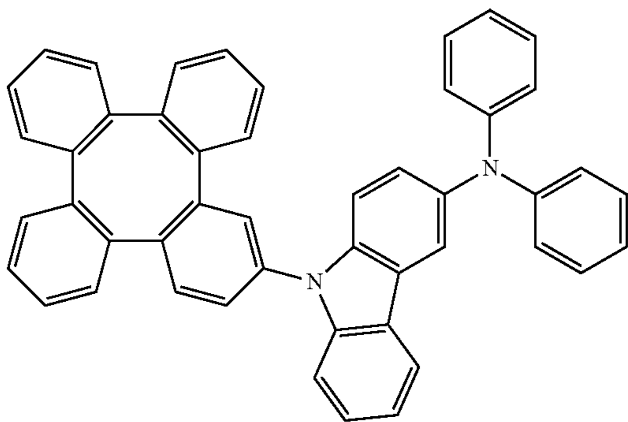
Compound 422
