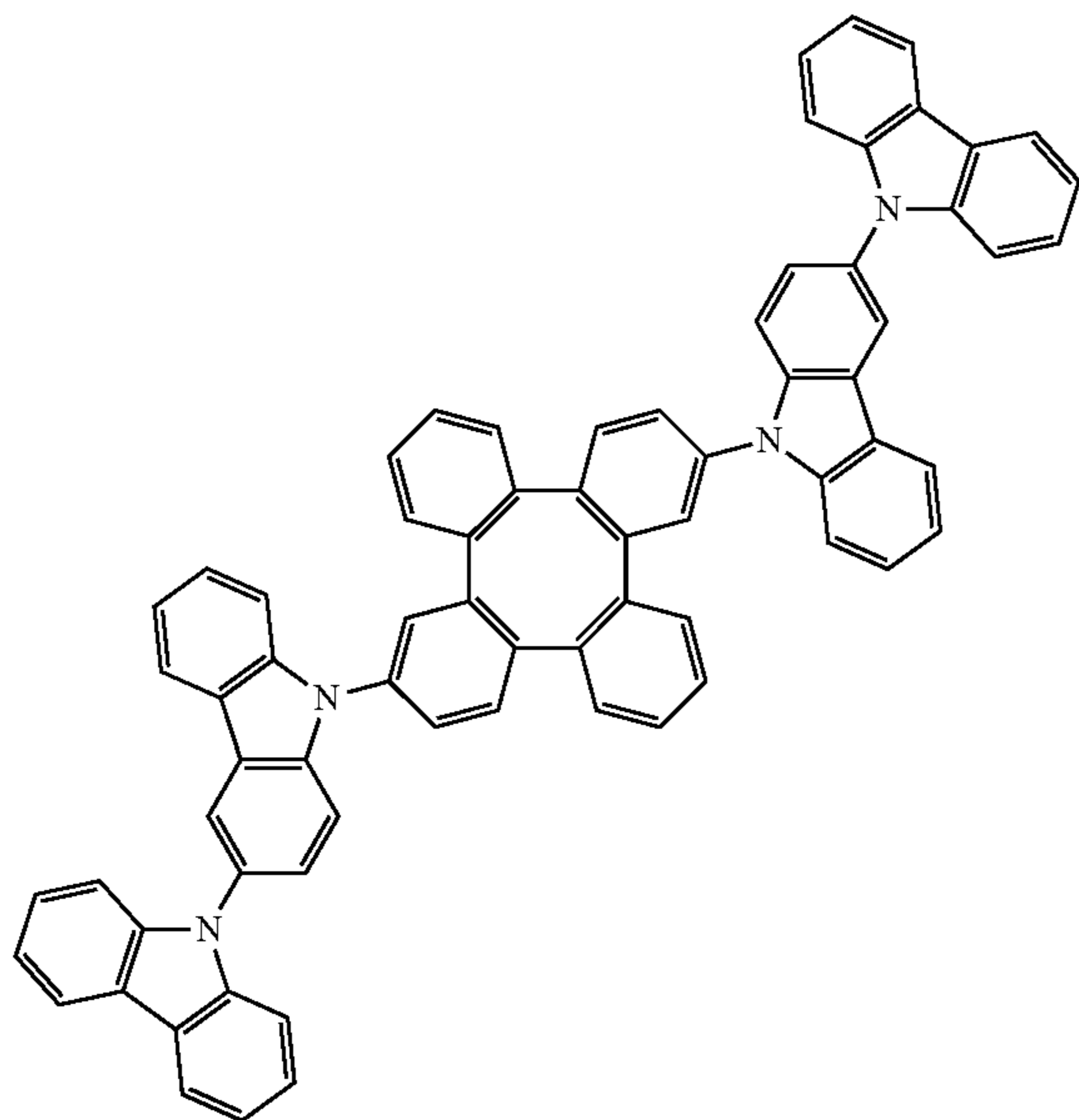
Compound 497
