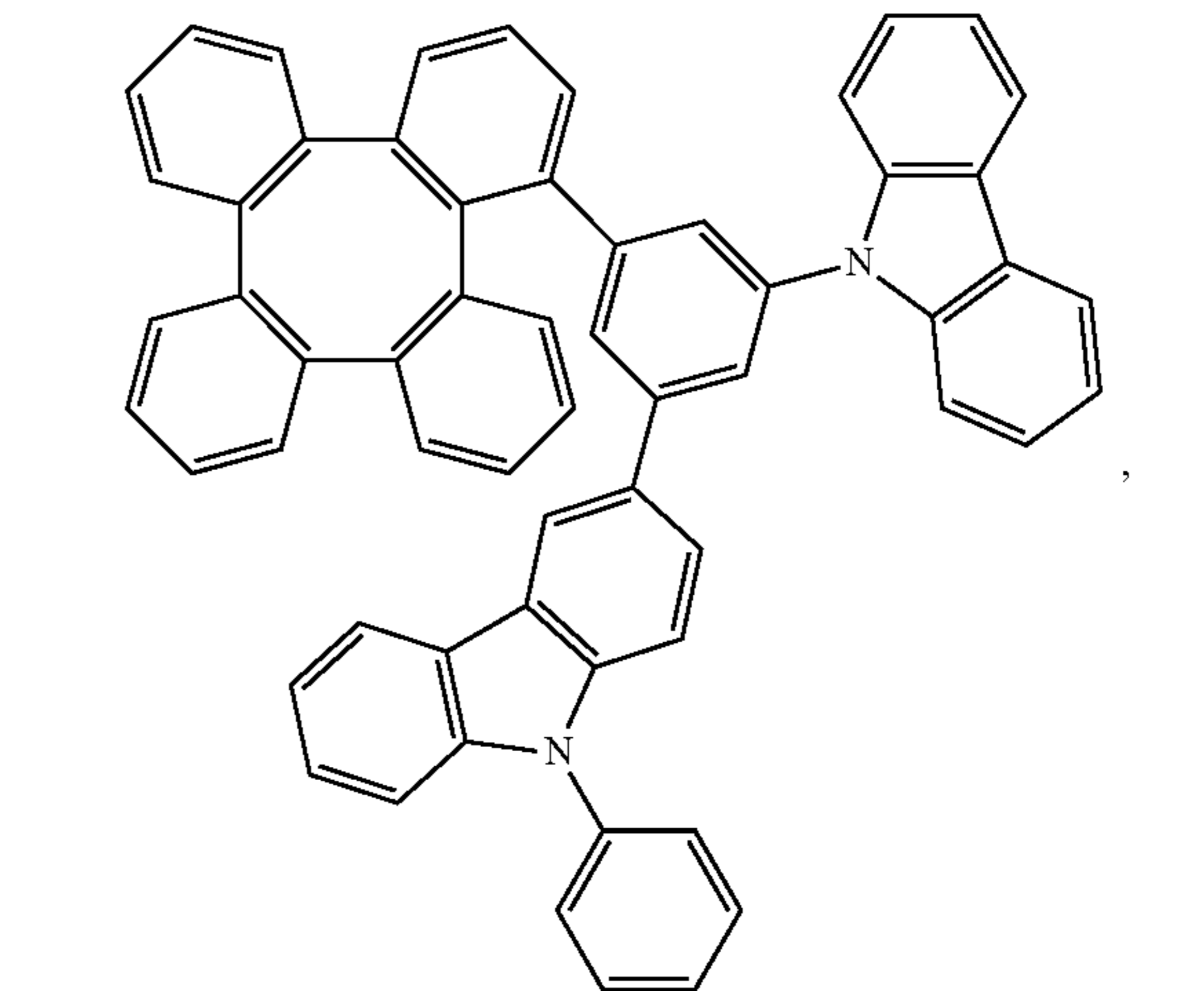
Compound 282
