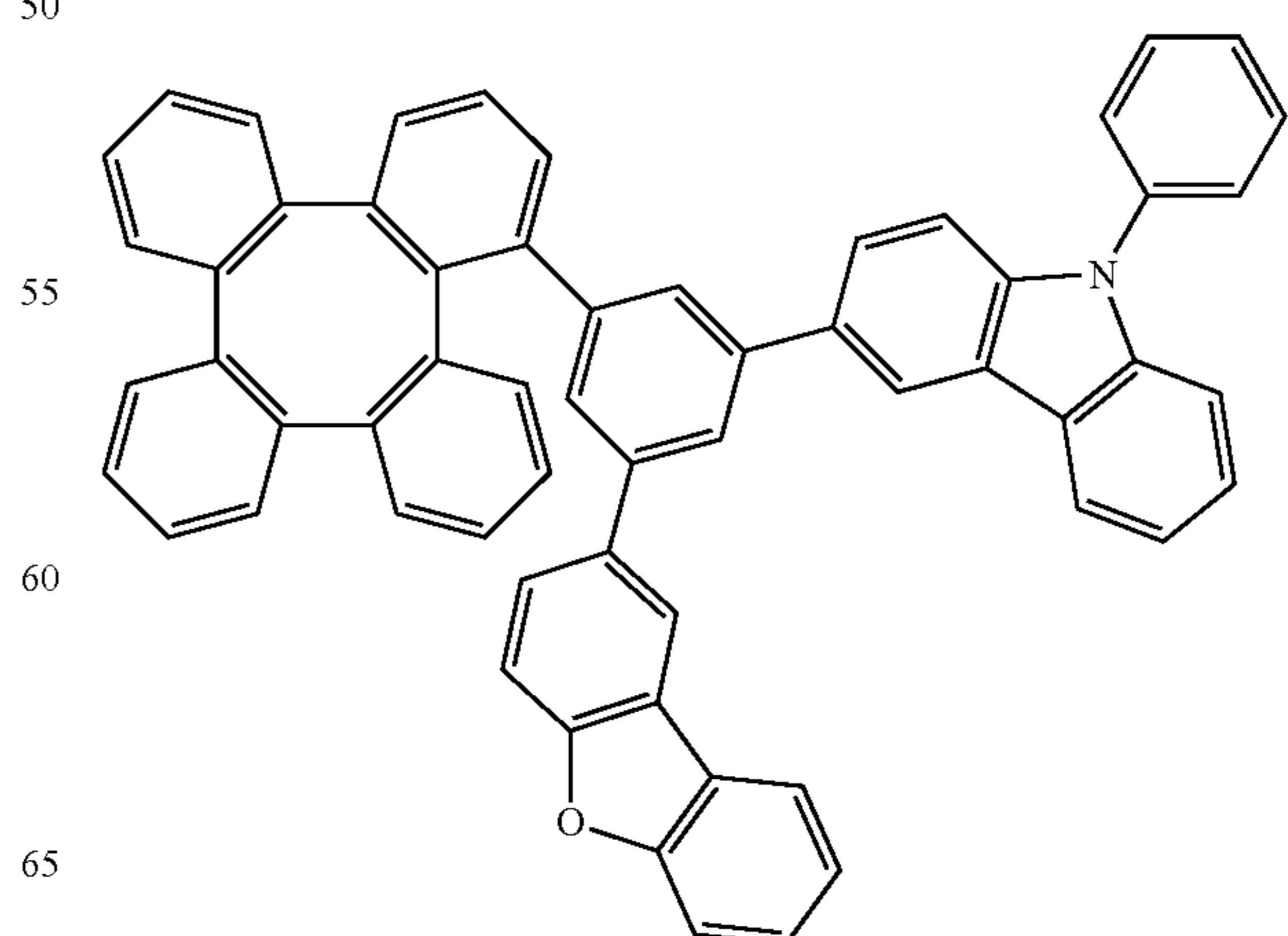
Compound 300
