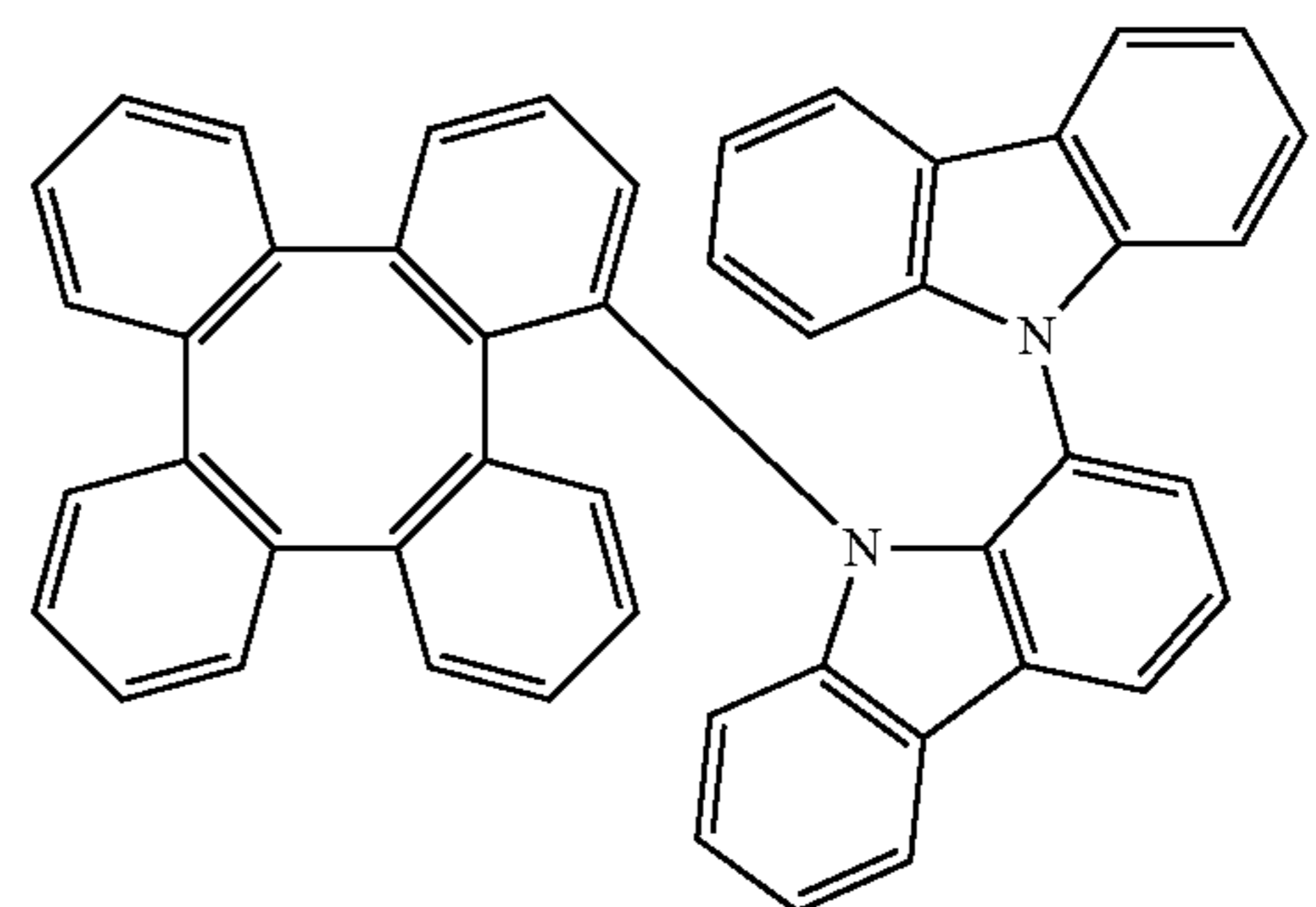
Compound 479
