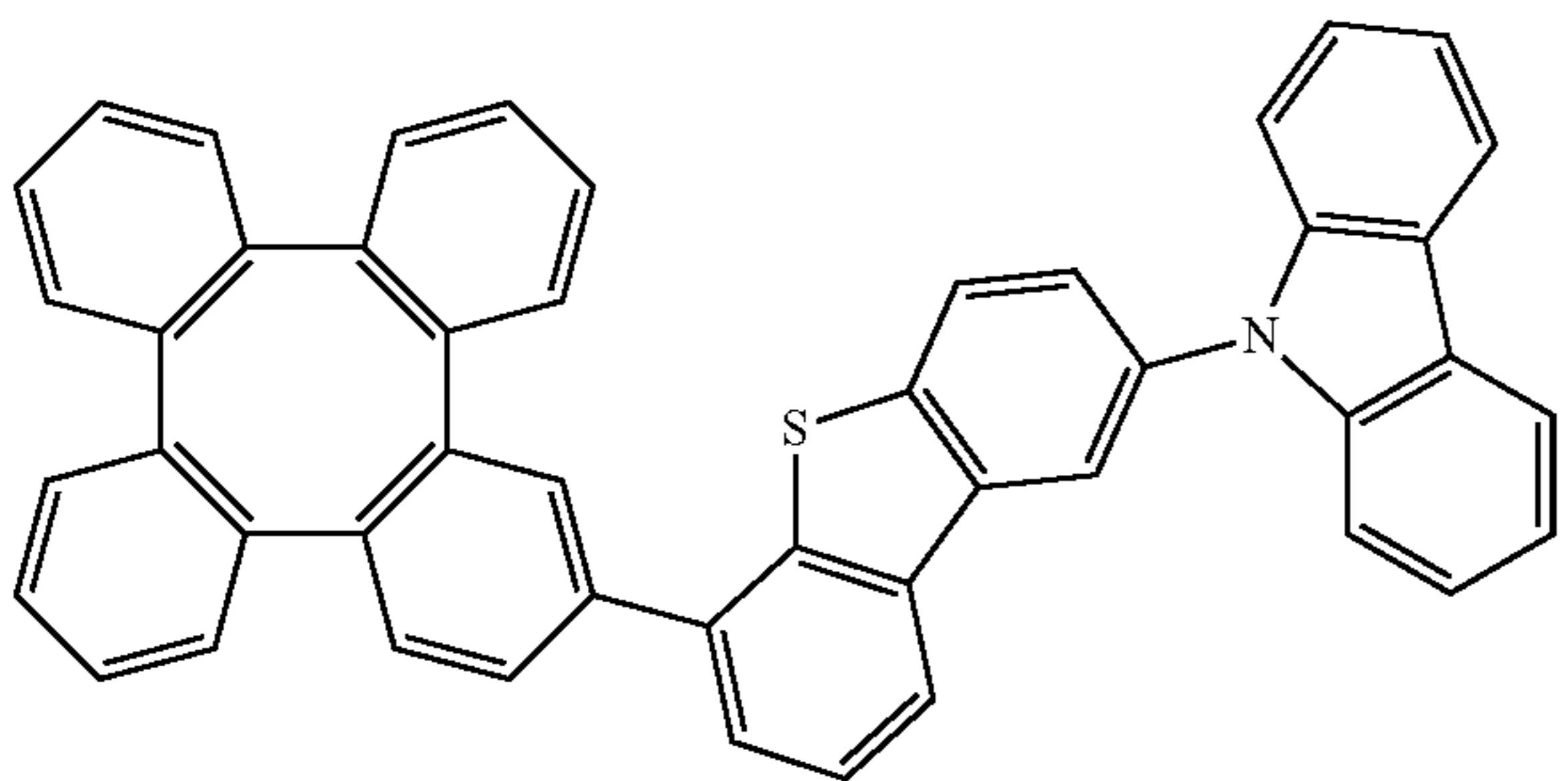
Compound 436
