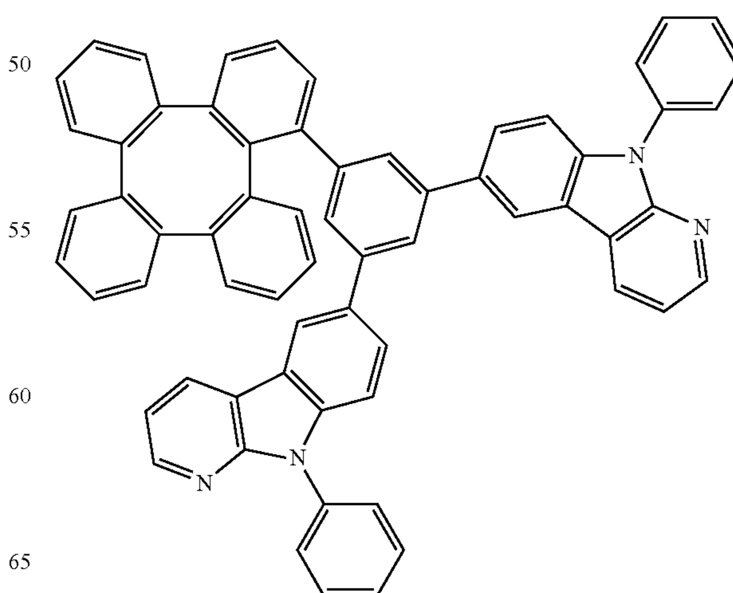
Compound 224
