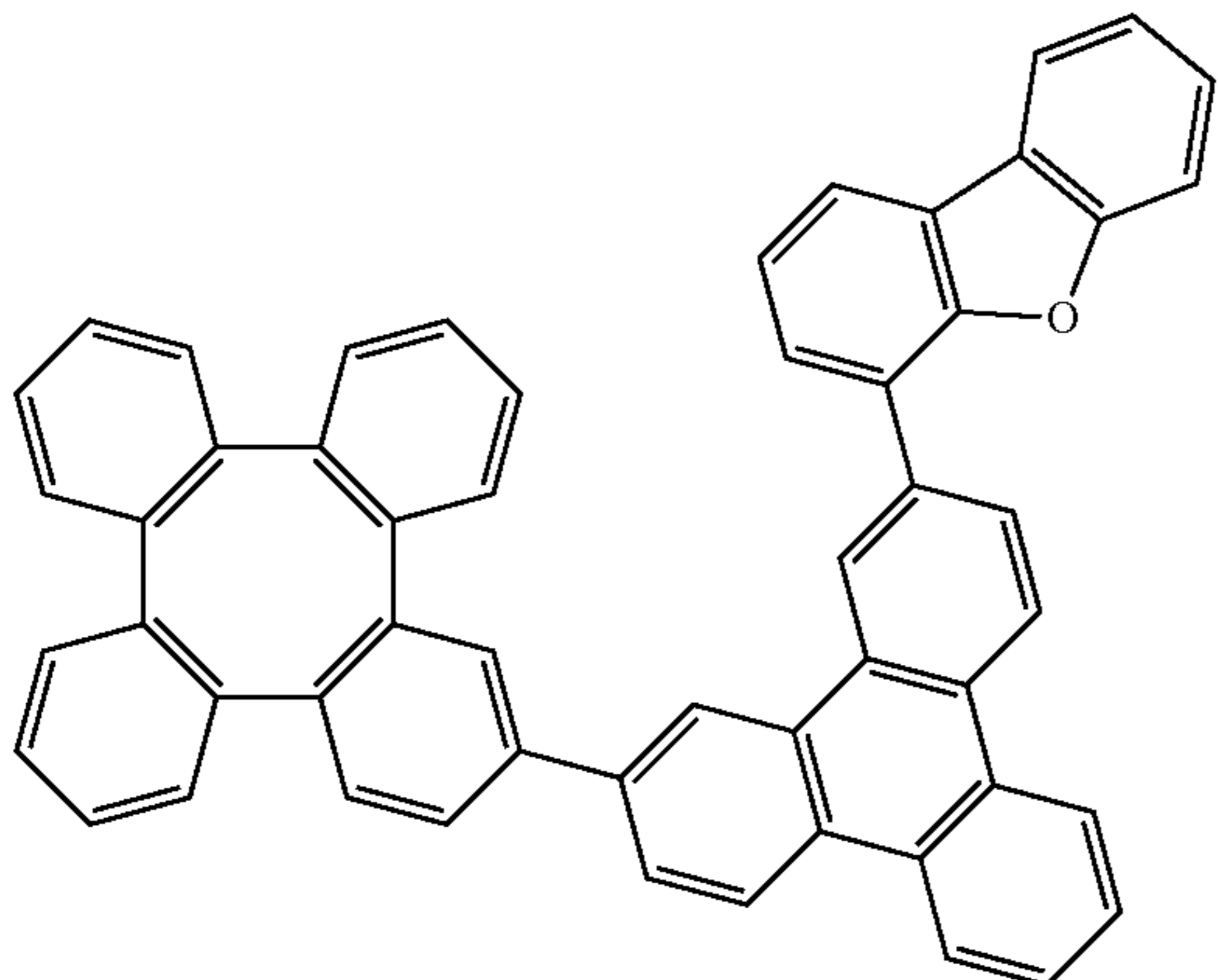
Compound 468
