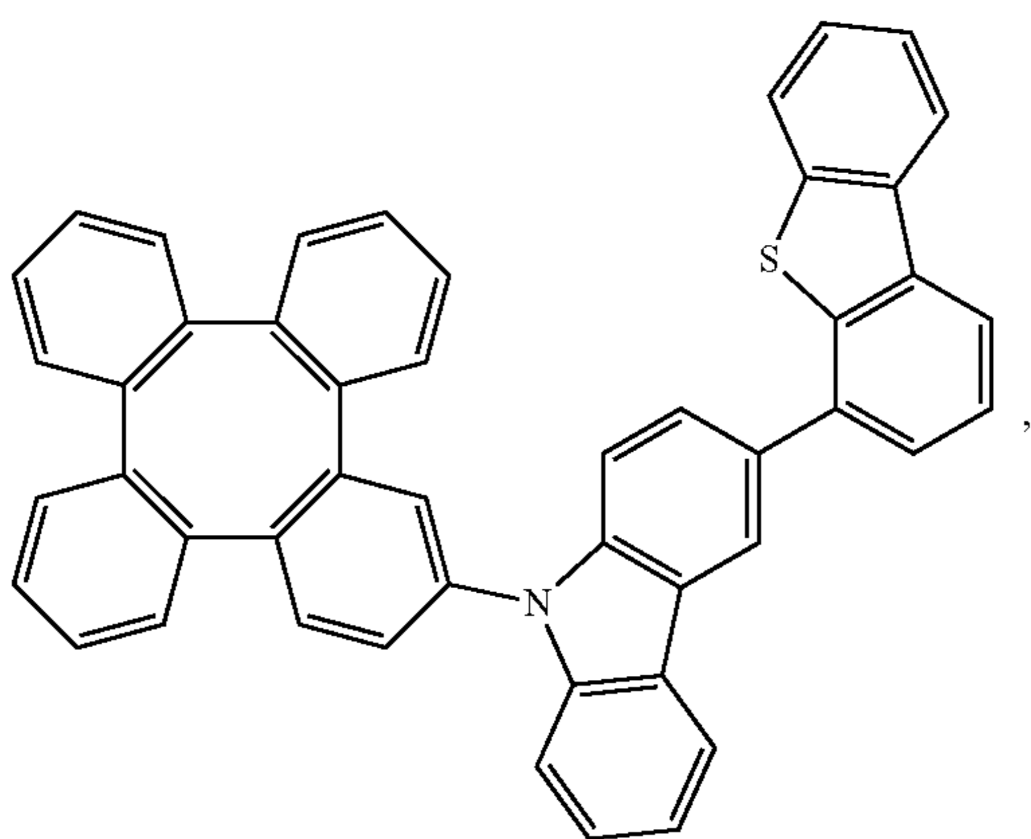
Compound 424
