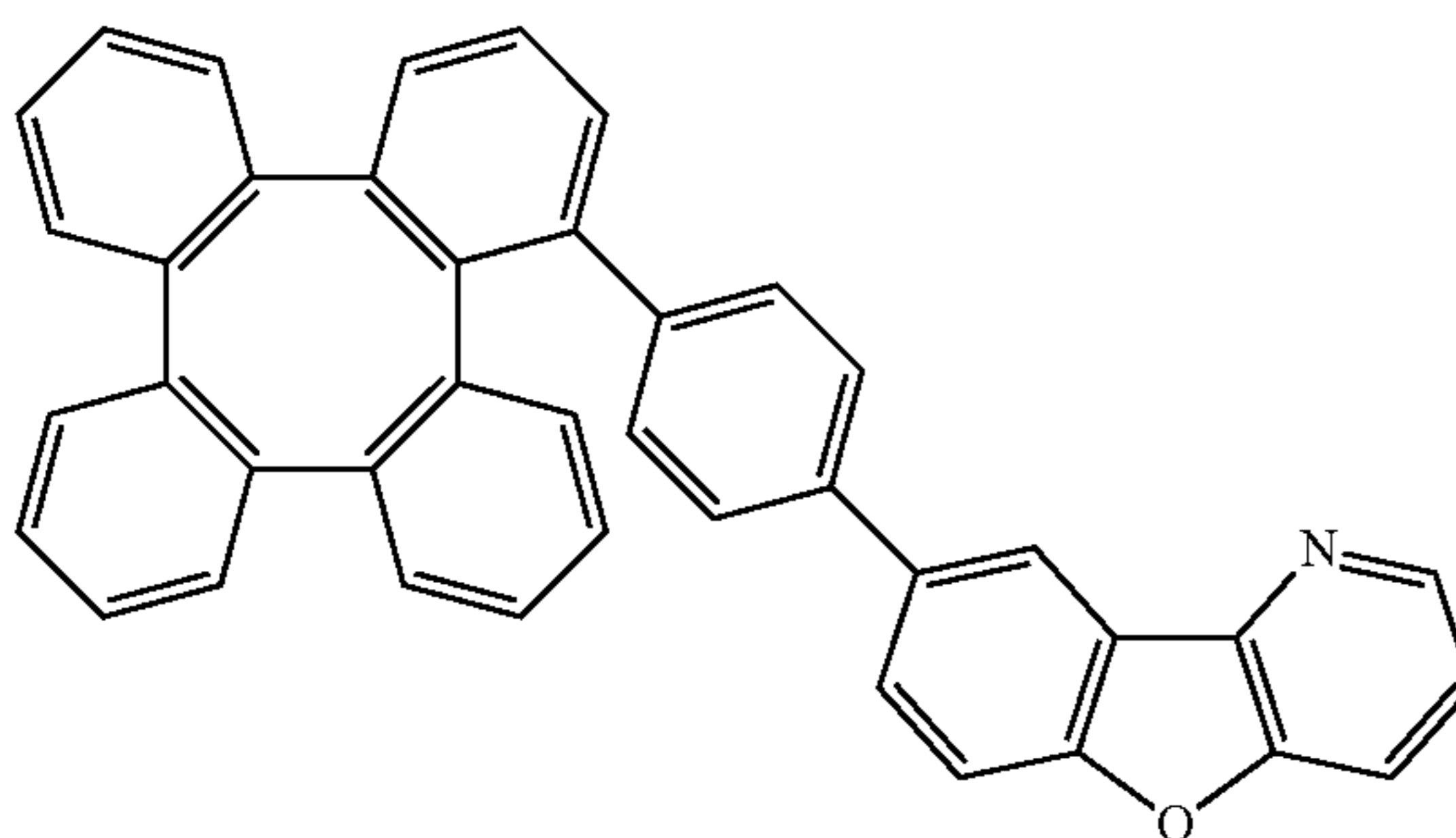
Compound 130
