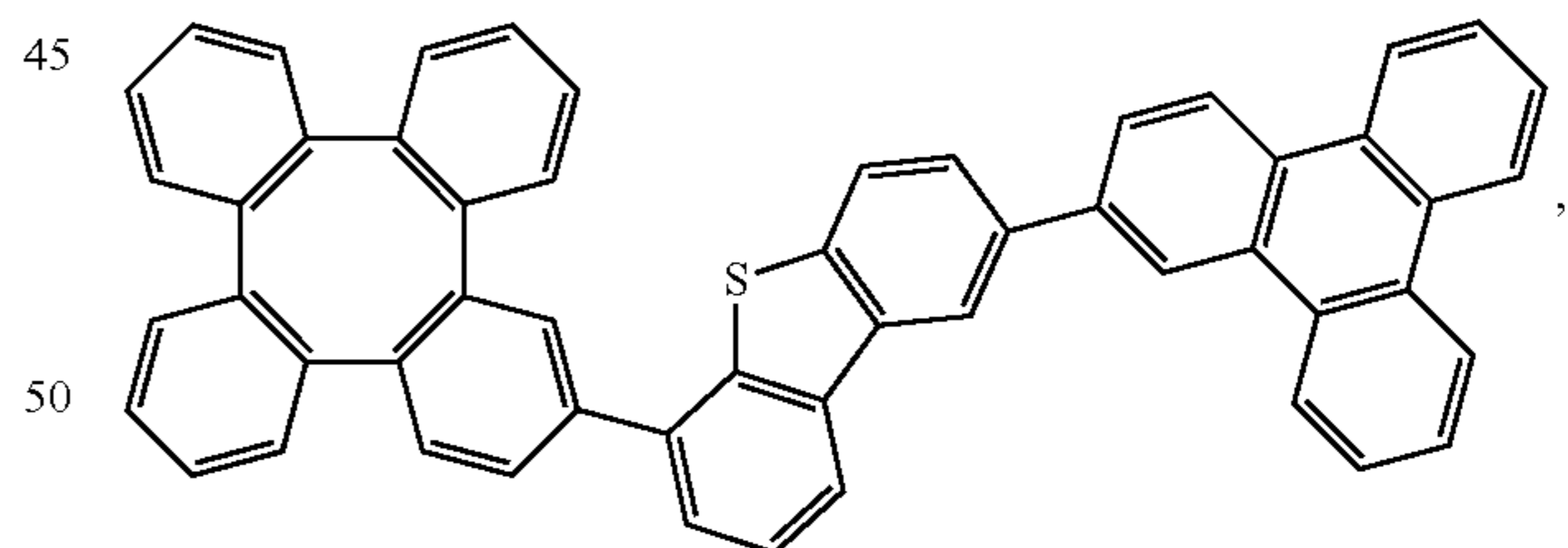
Compound 442
