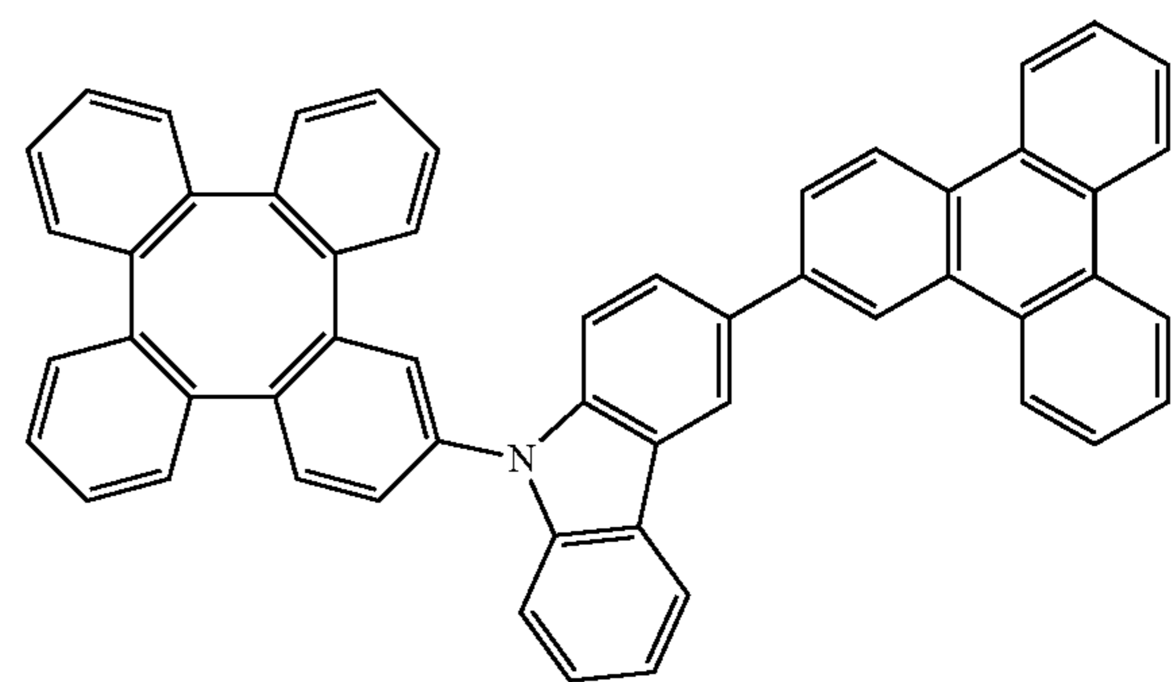
Compound 428
