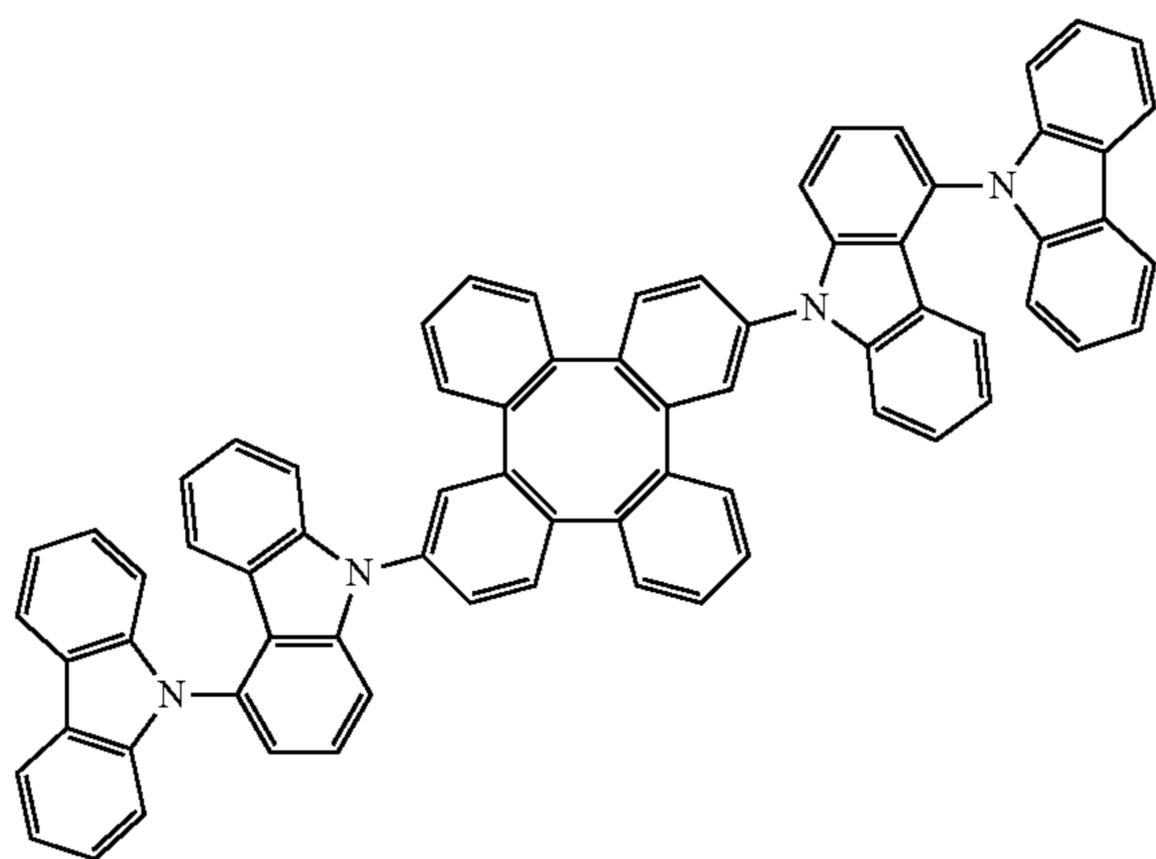
Compound 498
