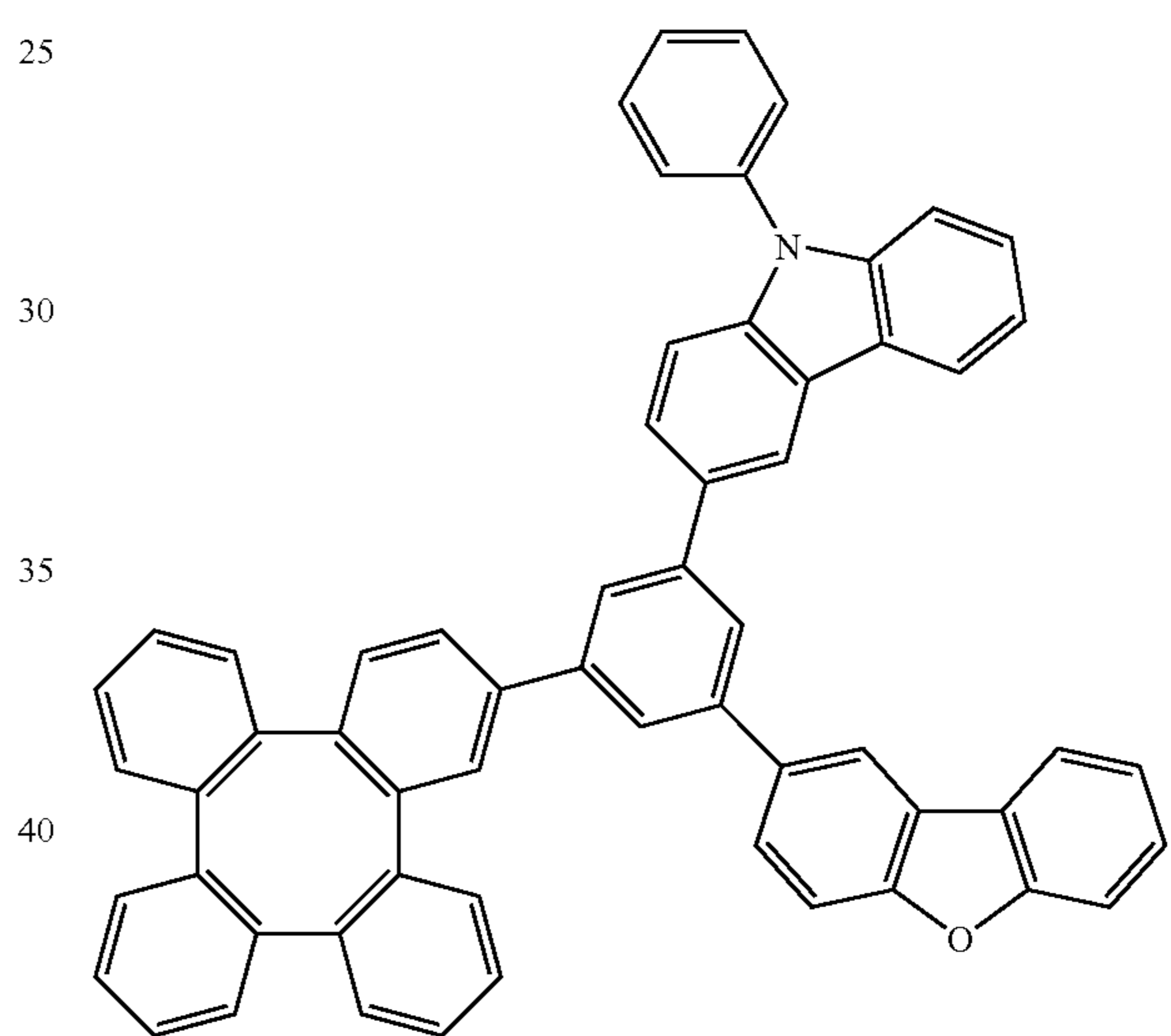
Compound 299
