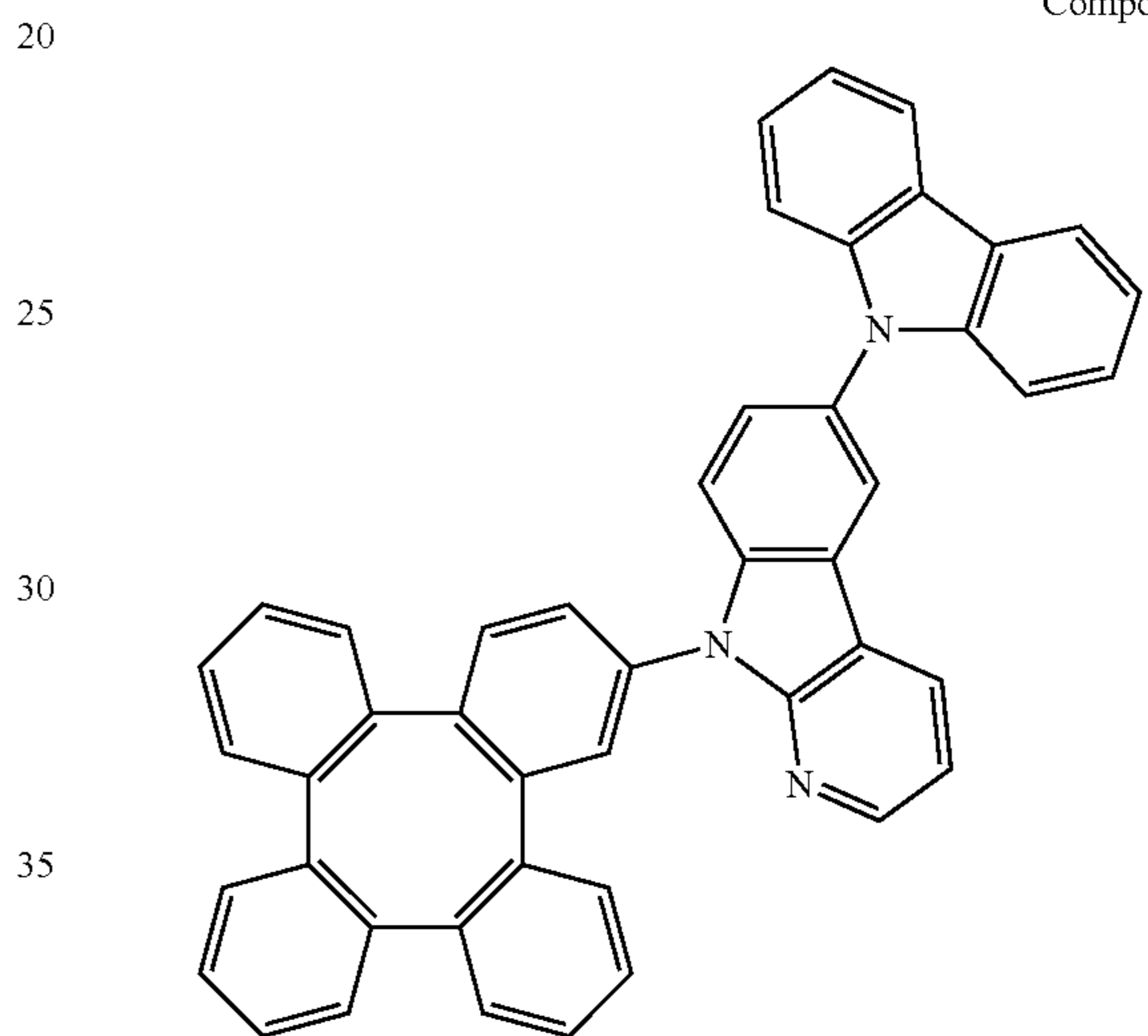
Compound 482
