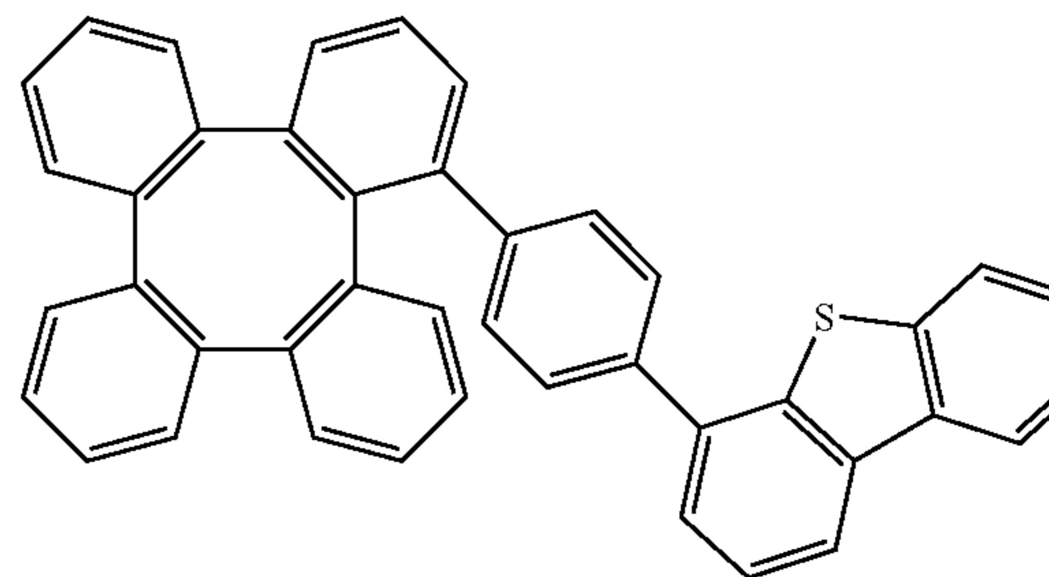
Compound 92
