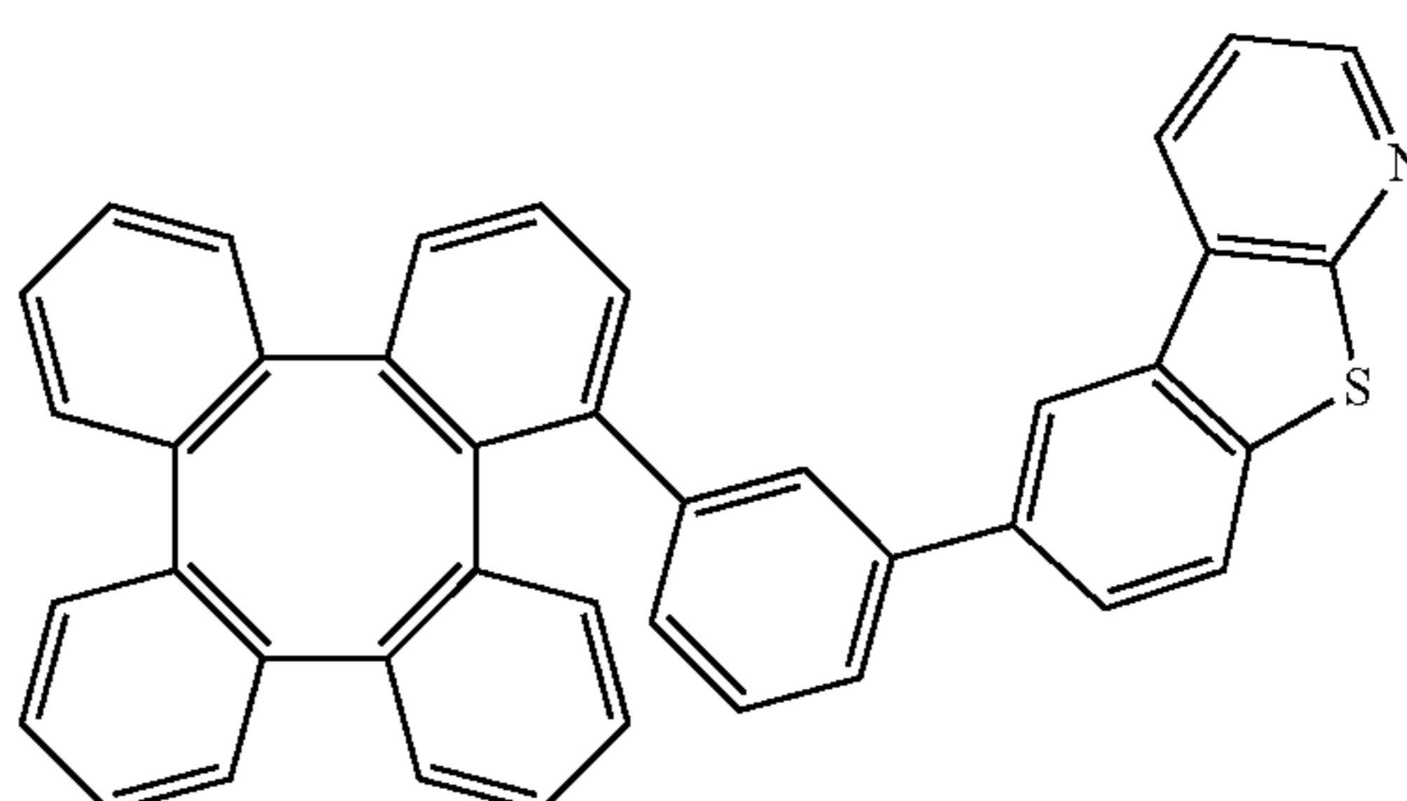
Compound 174
