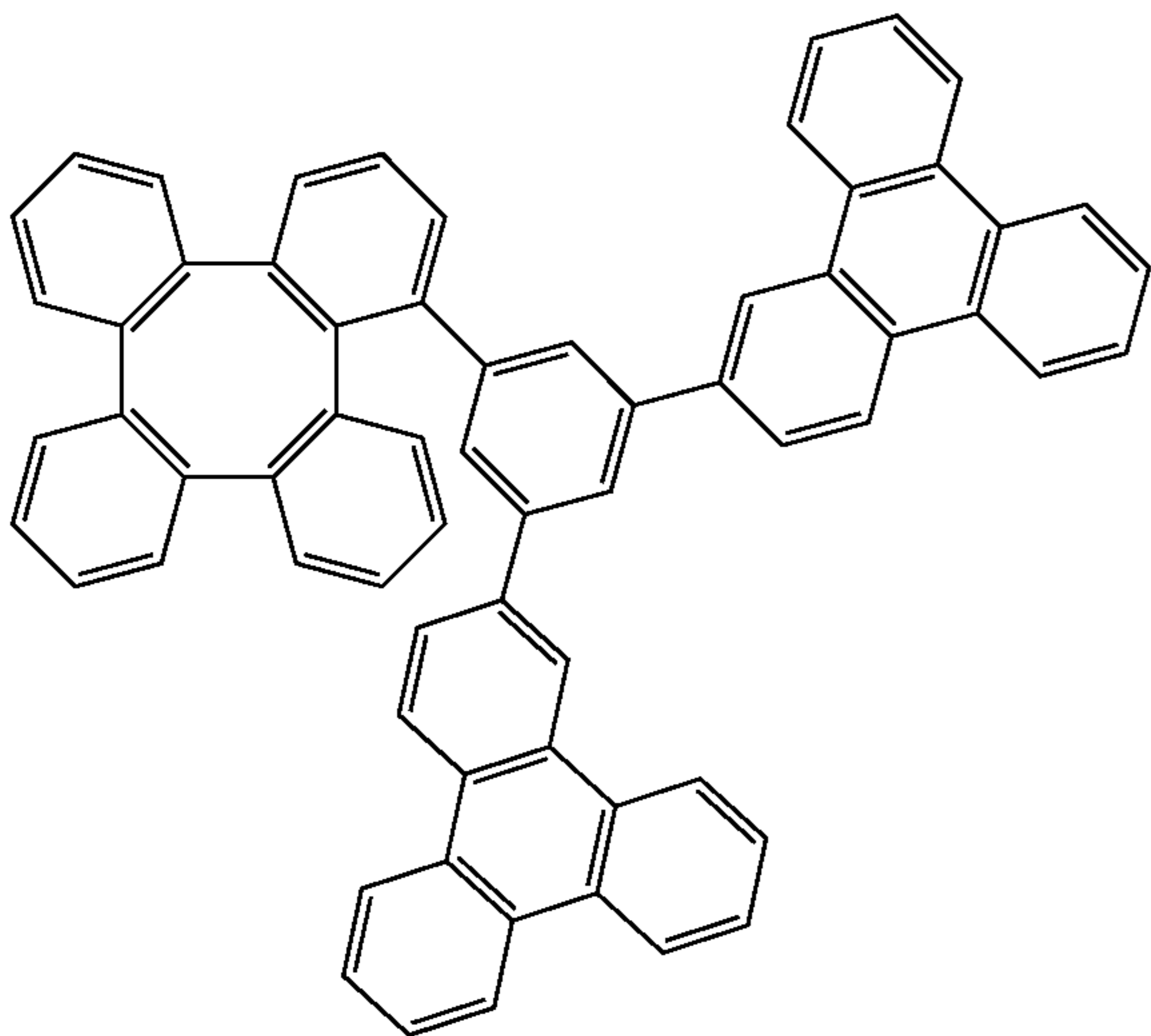
Compound 273
