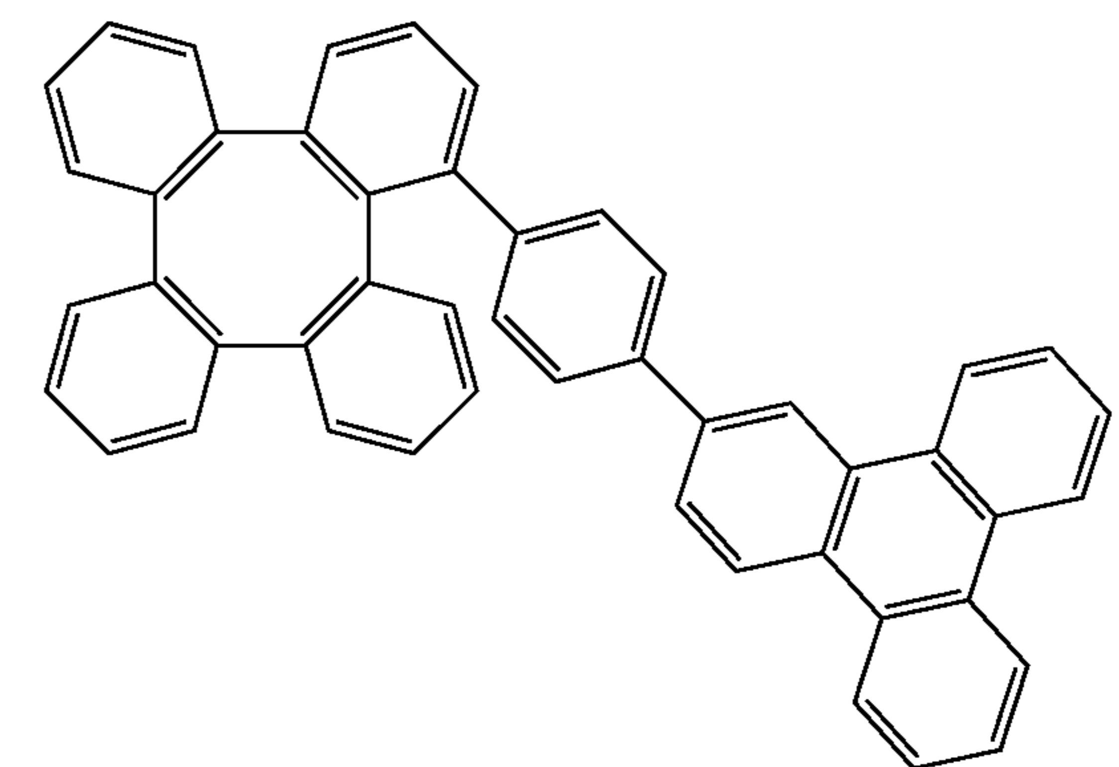
Compound 133
