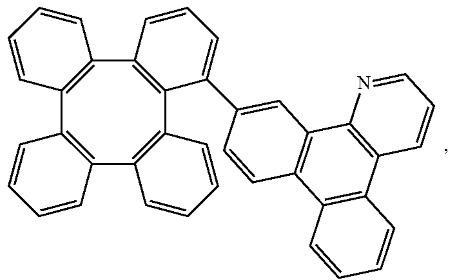
Compound 64
