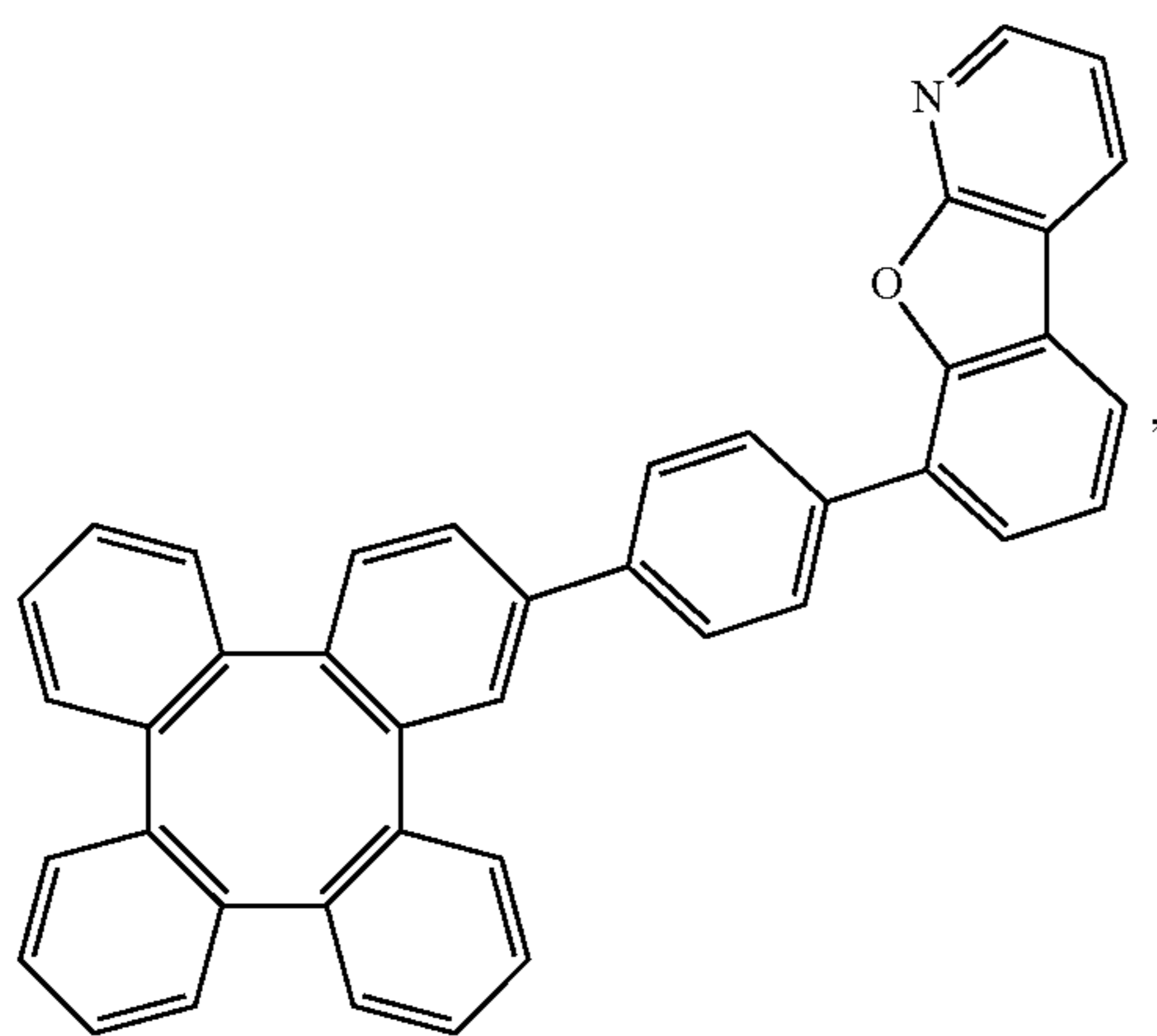
Compound 114
