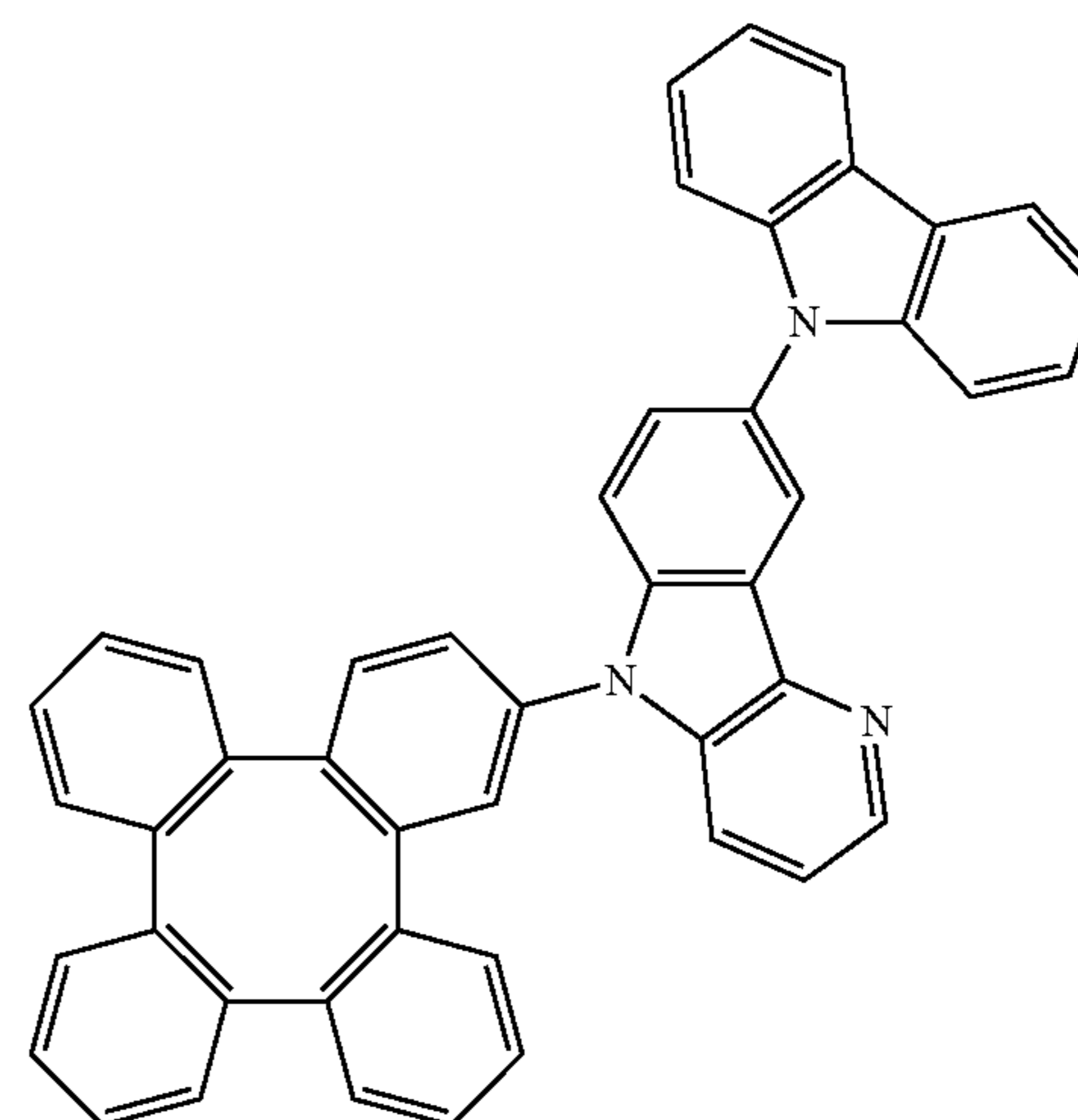
Compound 485
