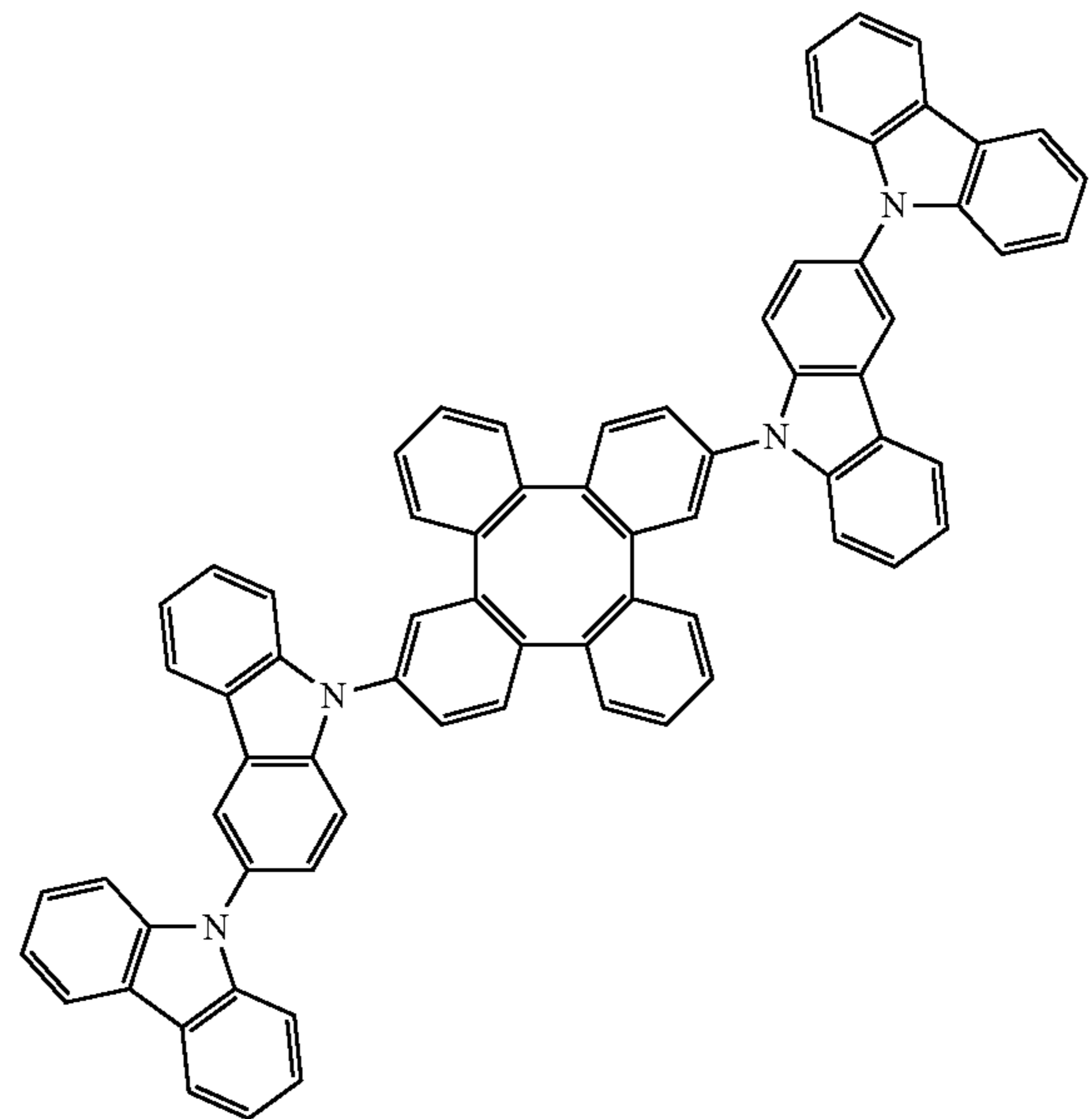
Compound 497
