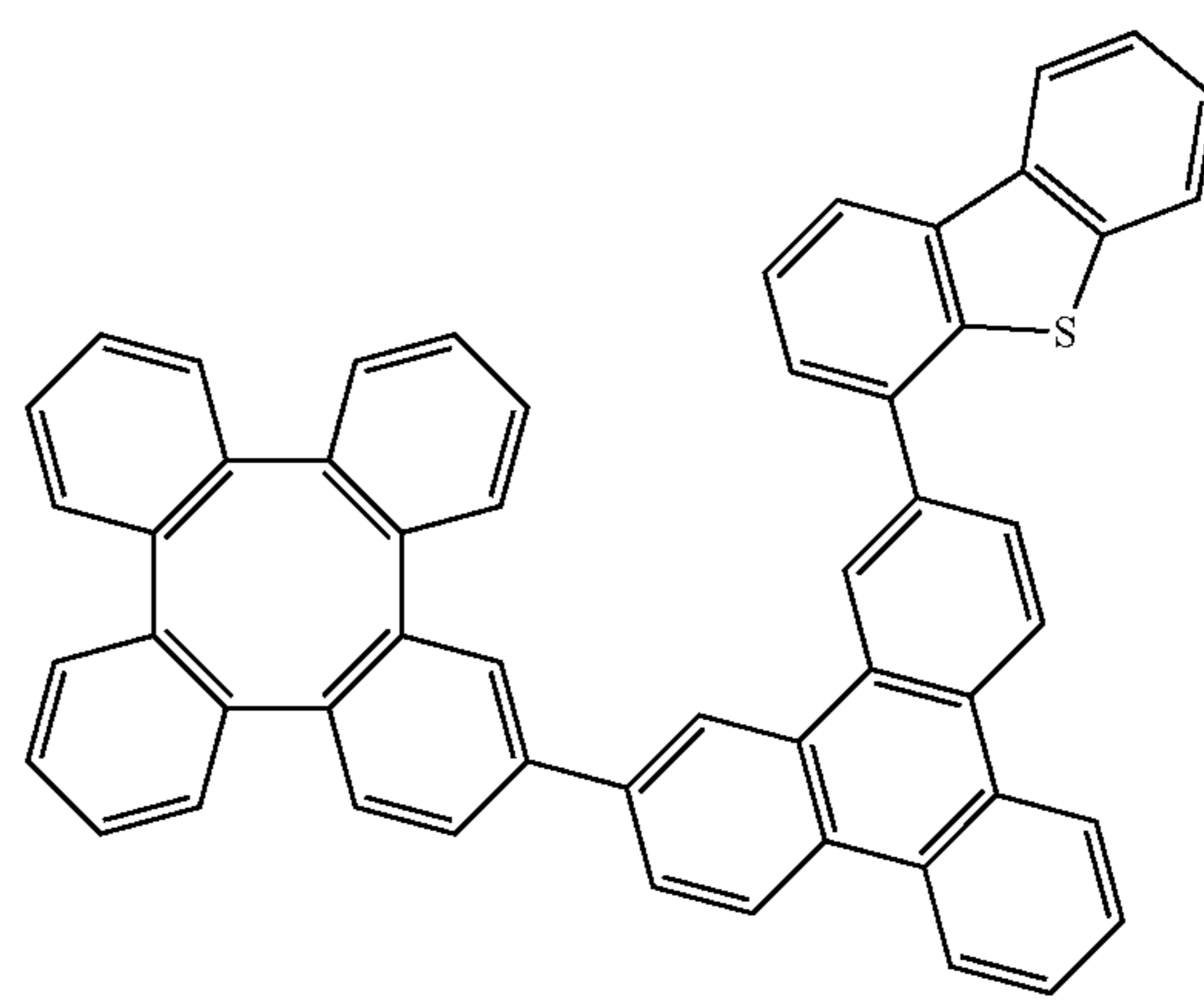
Compound 466
