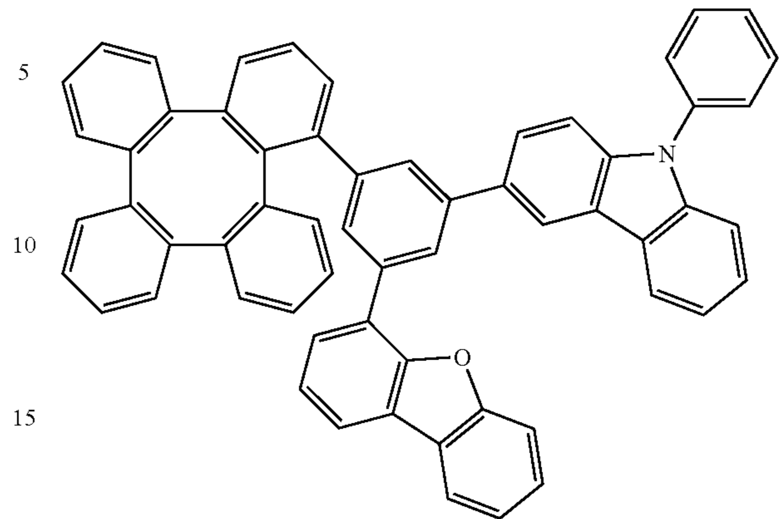
Compound 298
