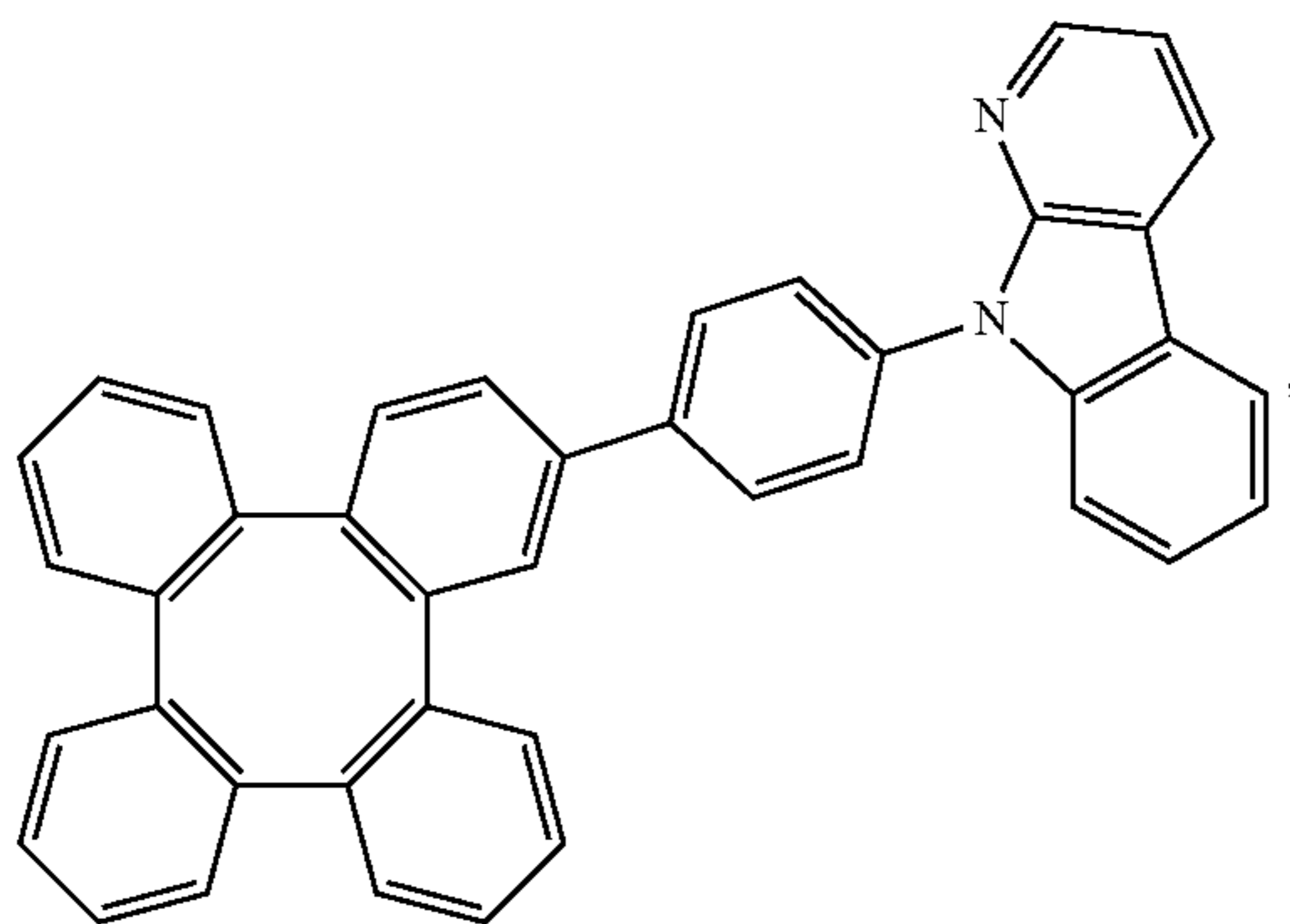
Compound 74
