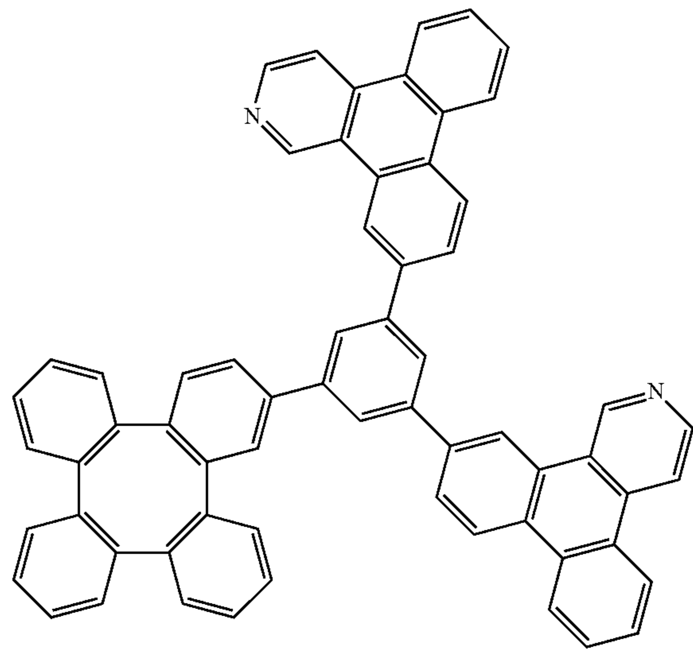
Compound 275
