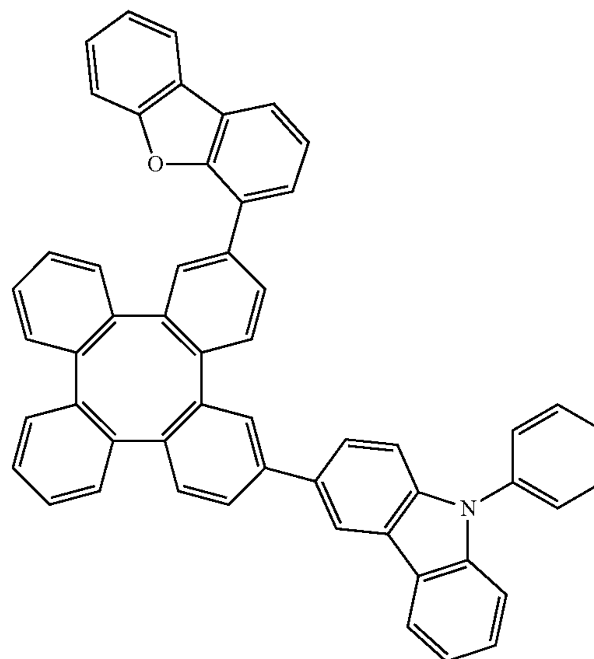
Compound 401
