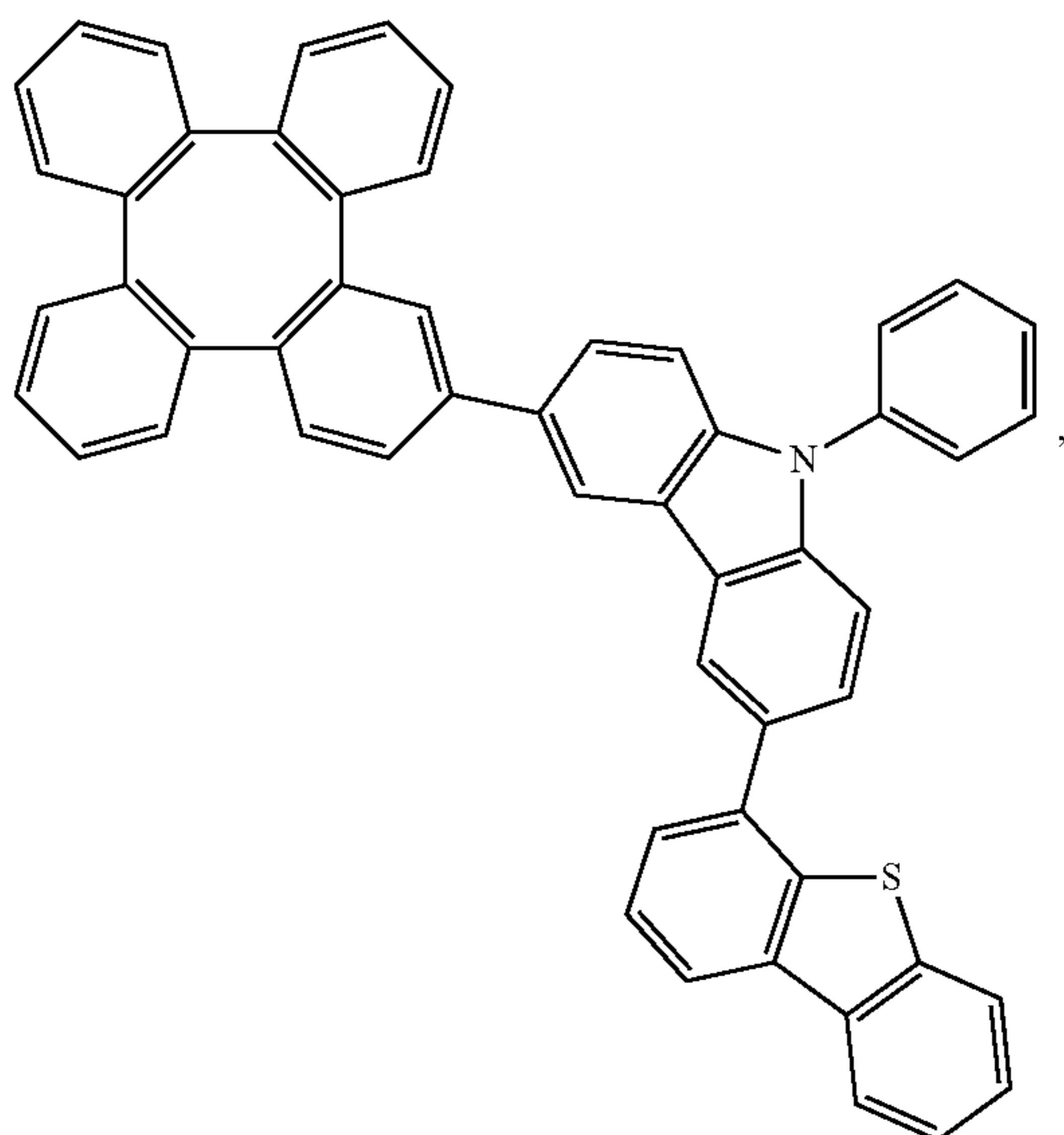
Compound 430
