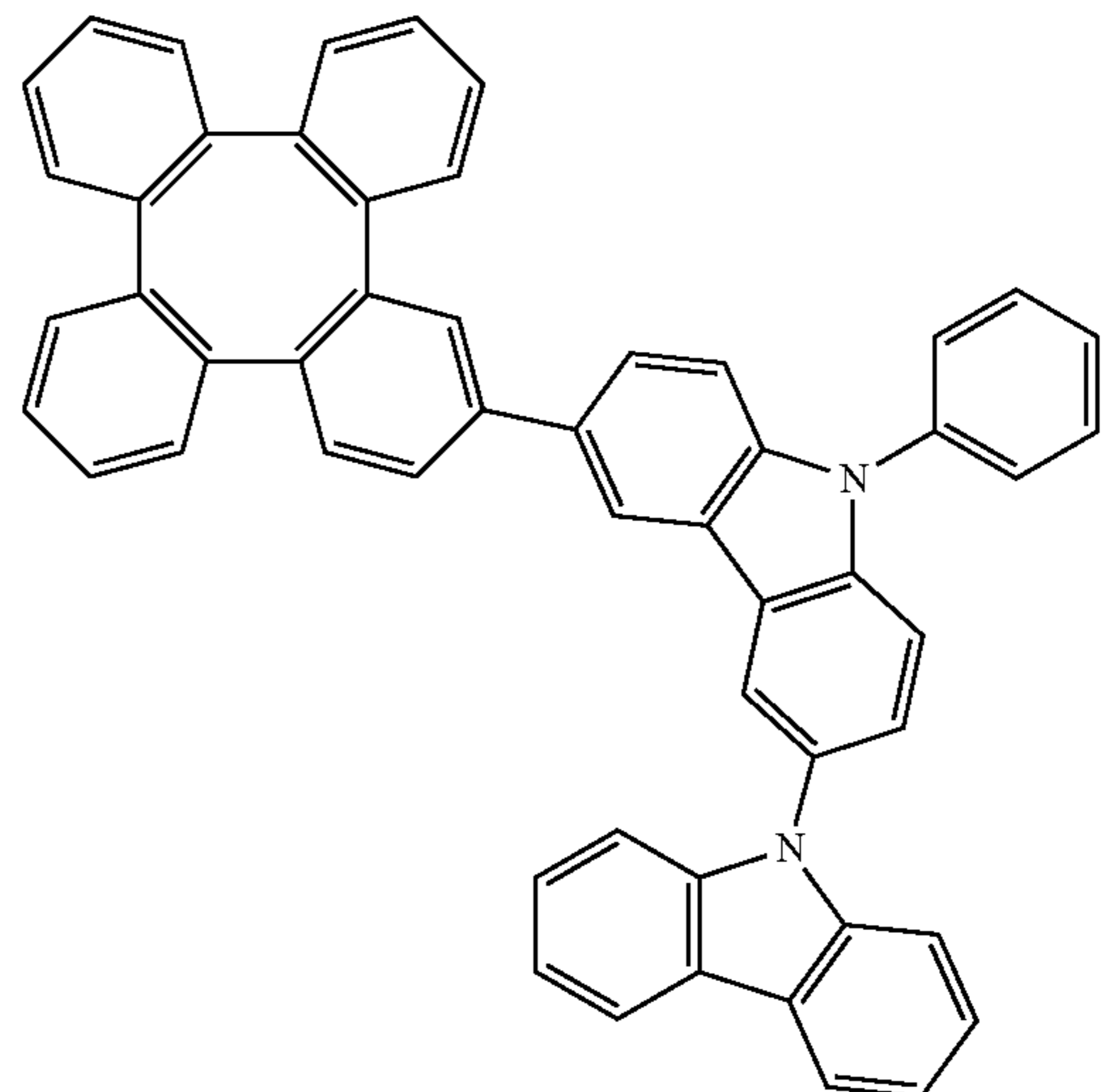
Compound 428
