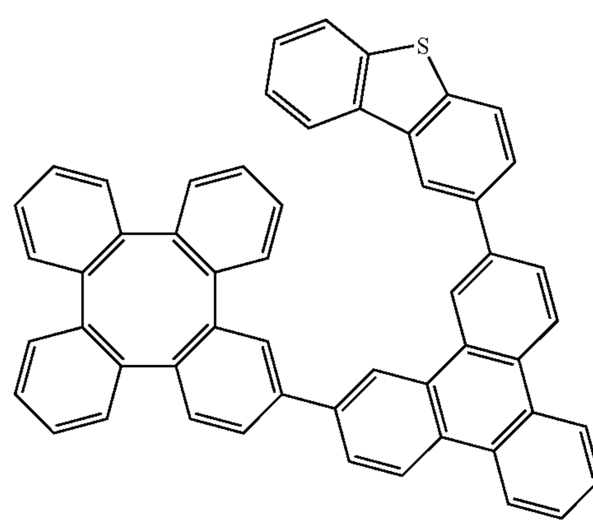
Compound 466
