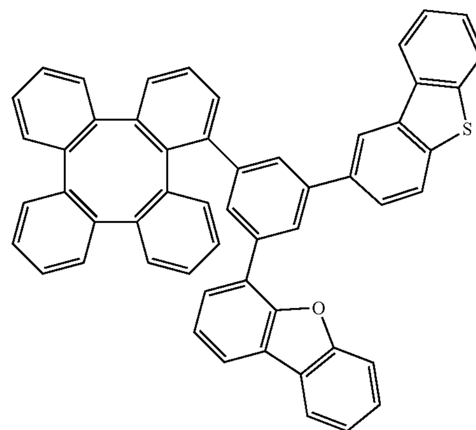
Compound 312
