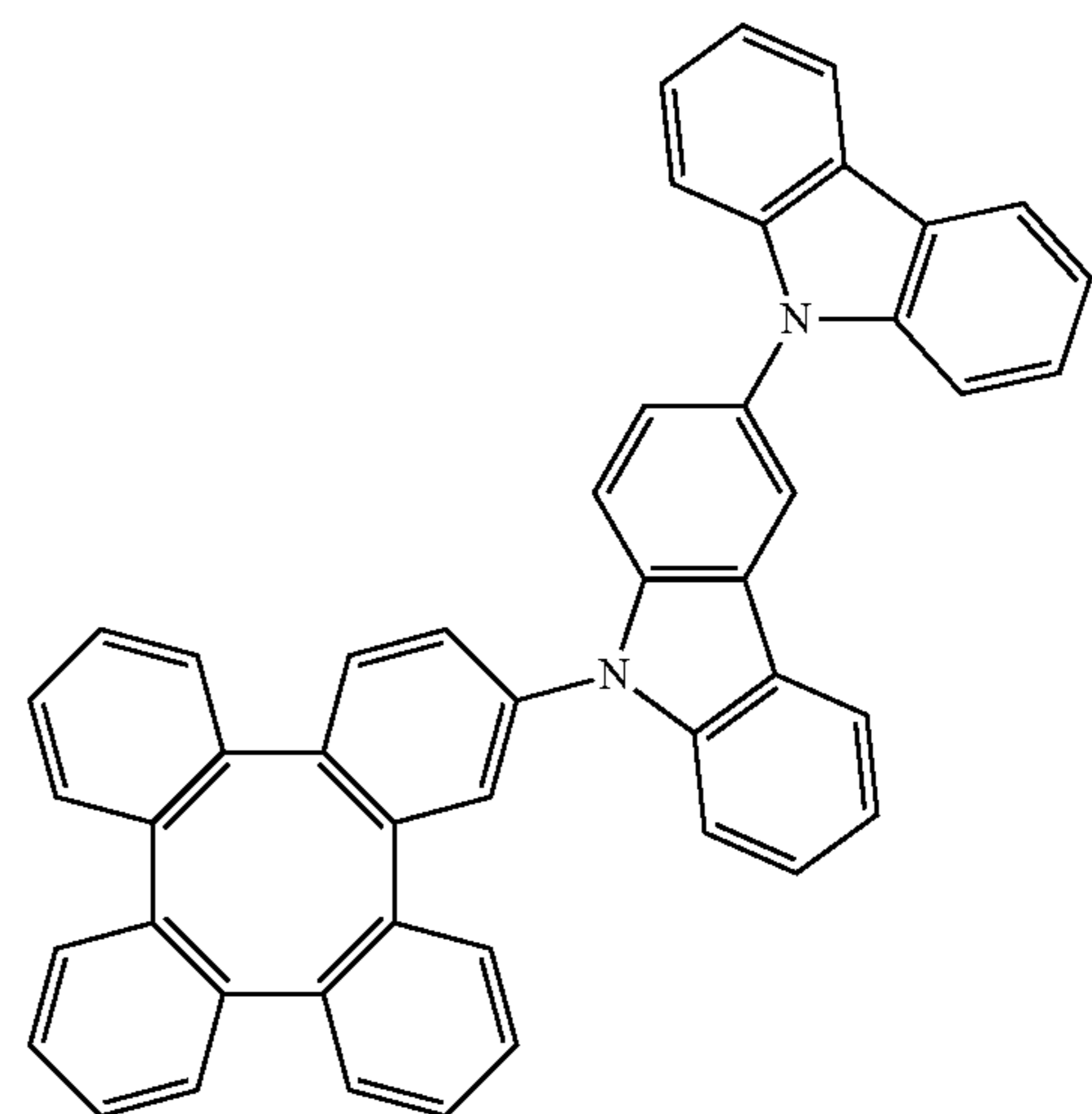
Compound 470
