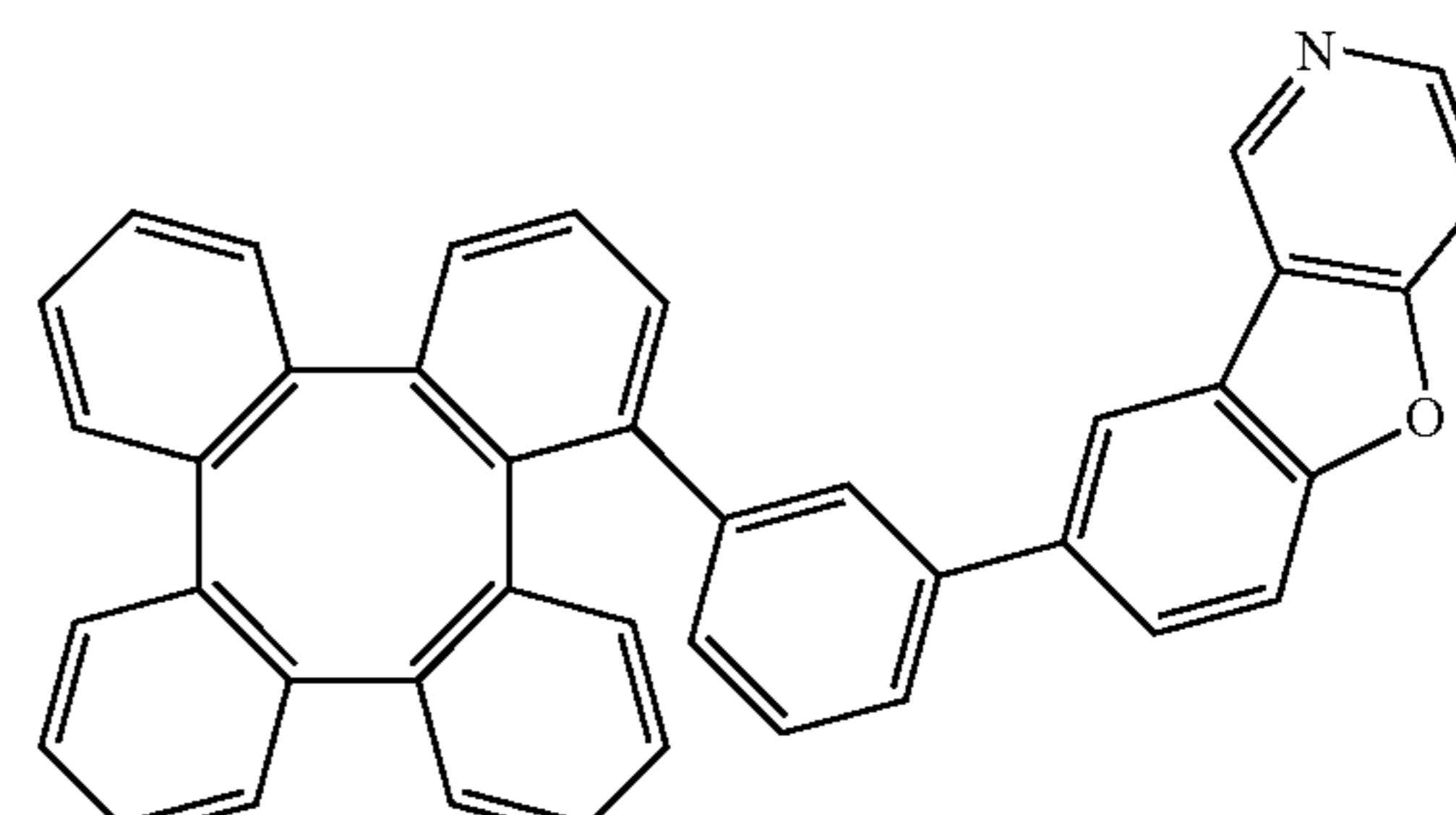
Compound 198
