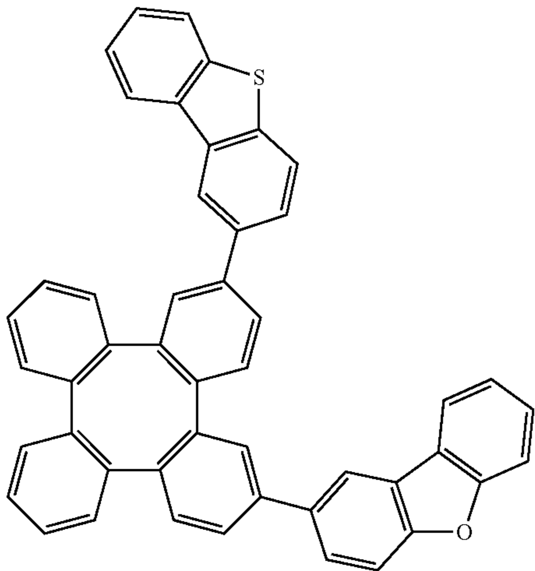
Compound 398
