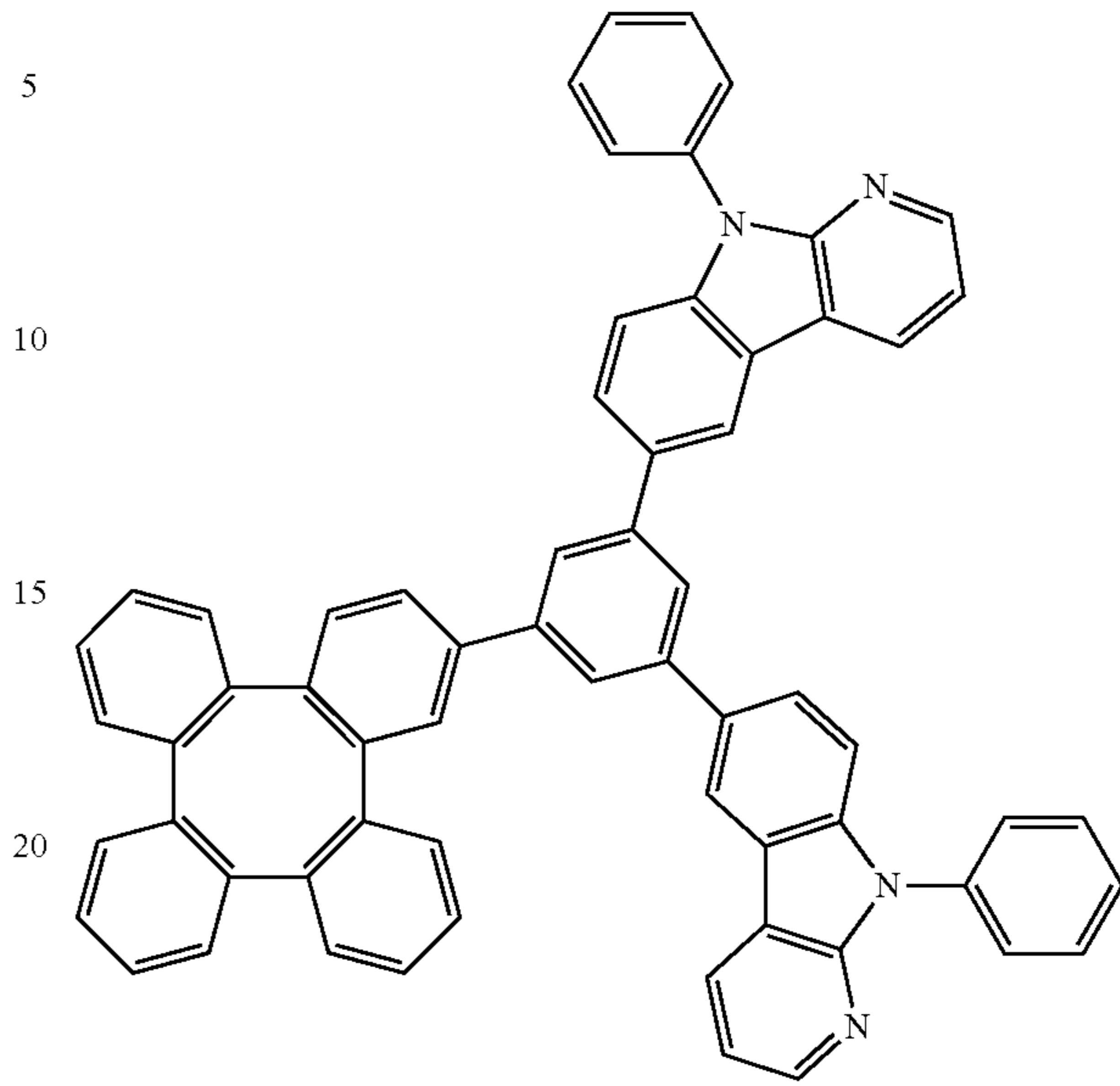
Compound 223
