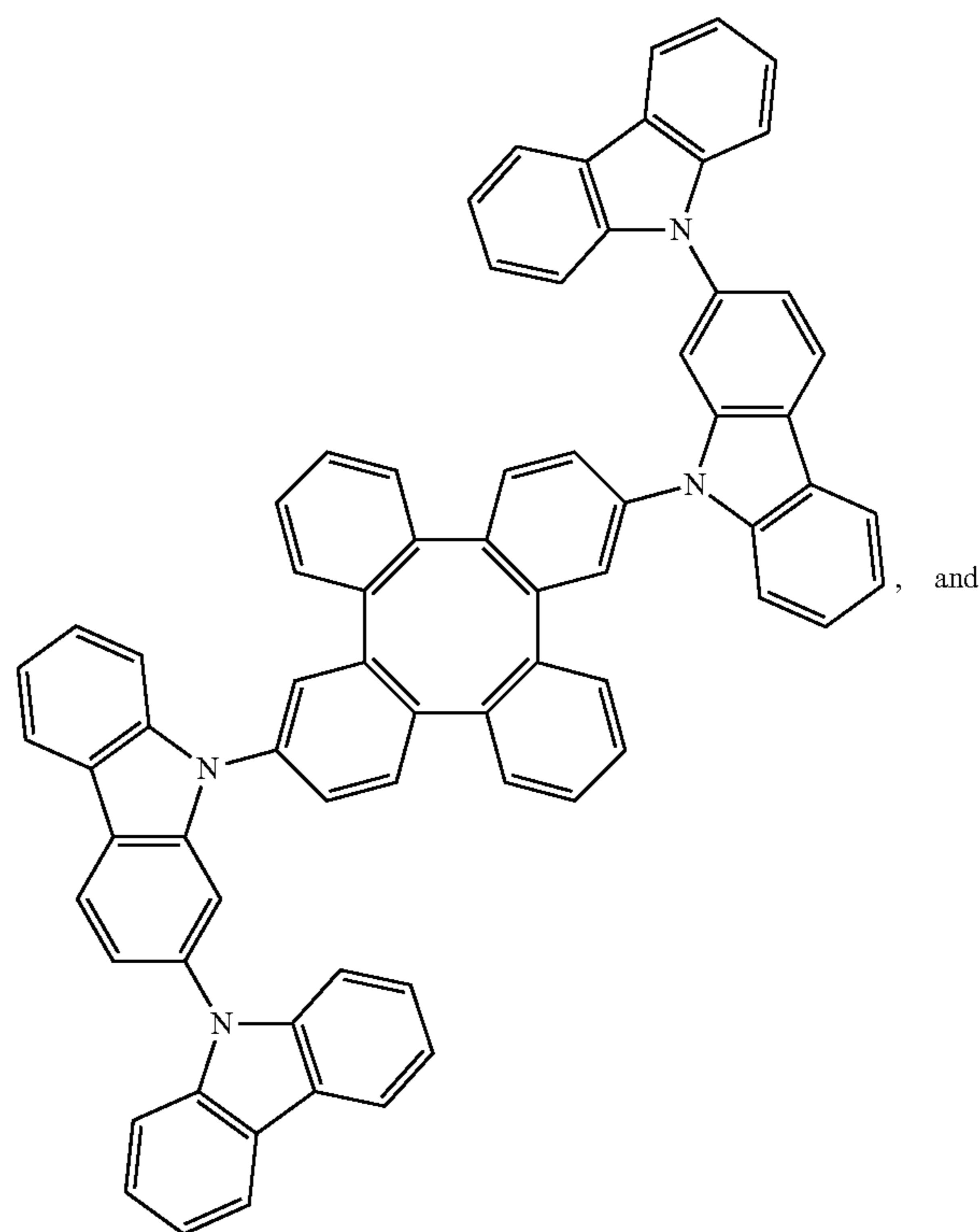
Compound 500
