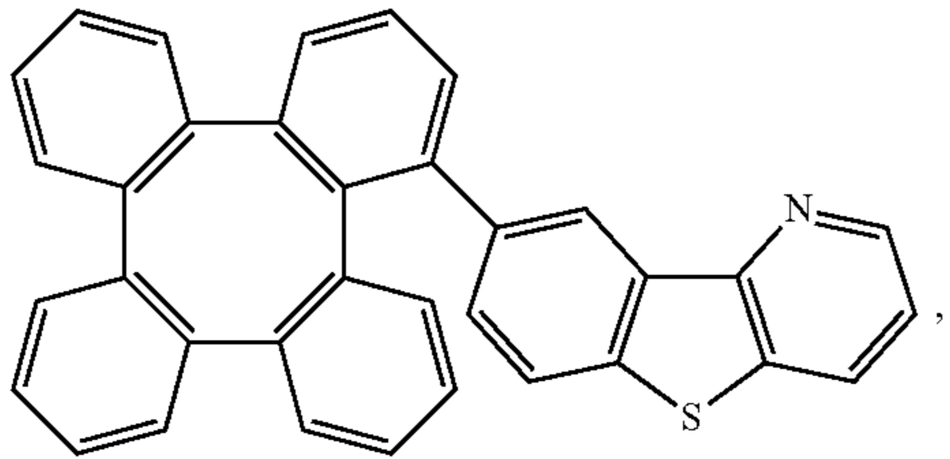
Compound 40
