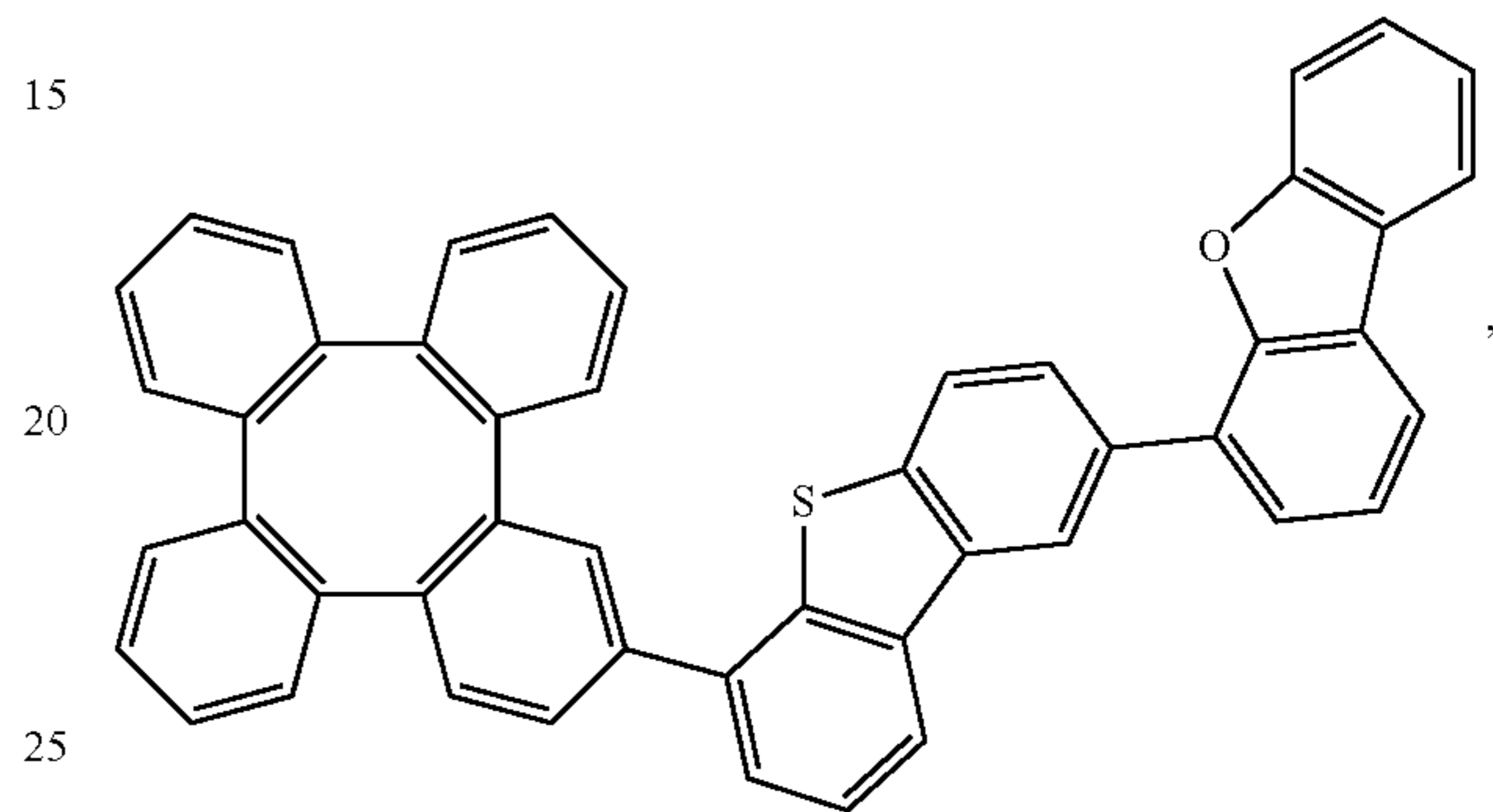
Compound 440
