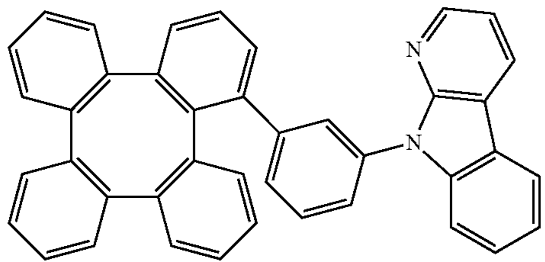
Compound 145
