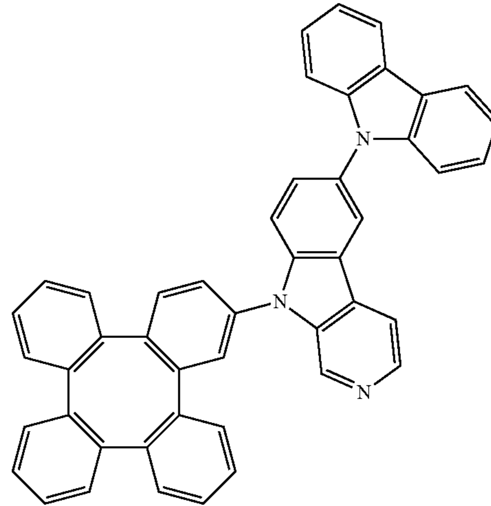
Compound 484
