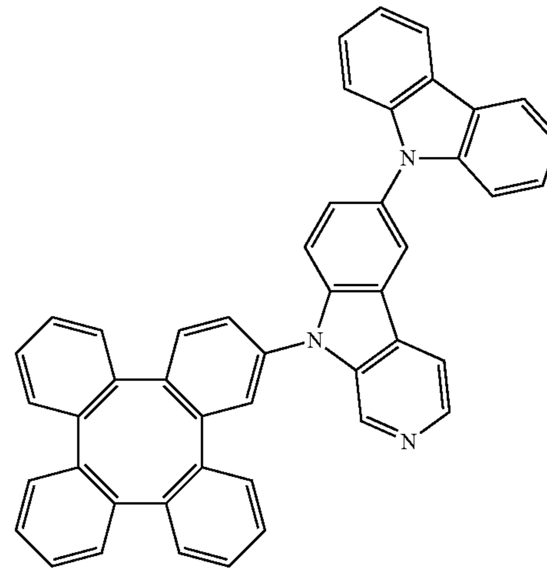
Compound 484
