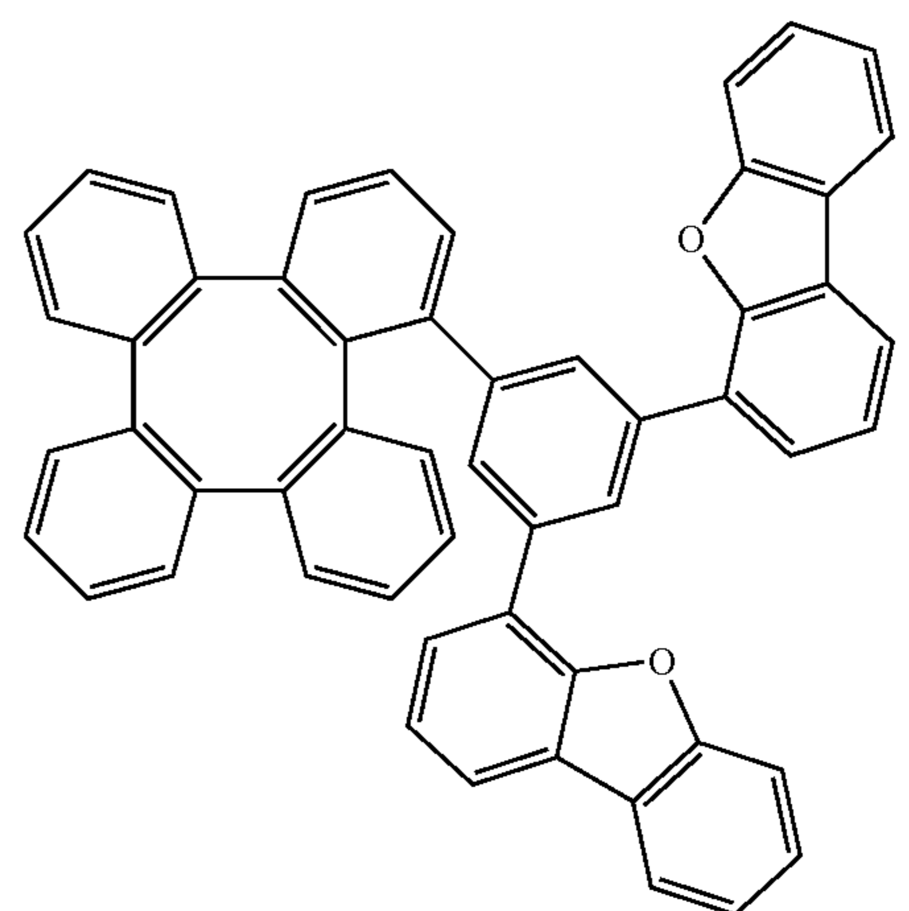
Compound 252
