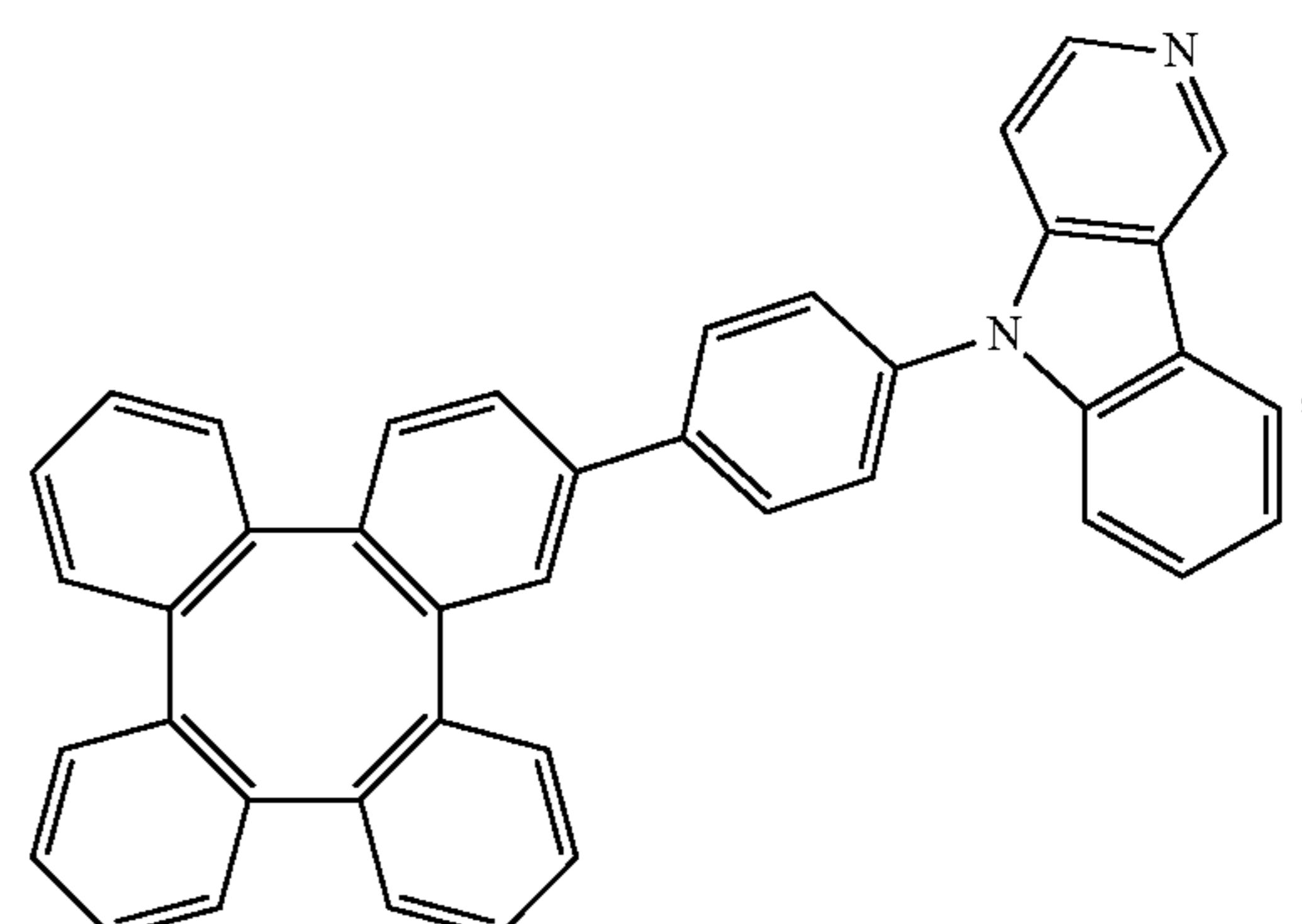
Compound 78
