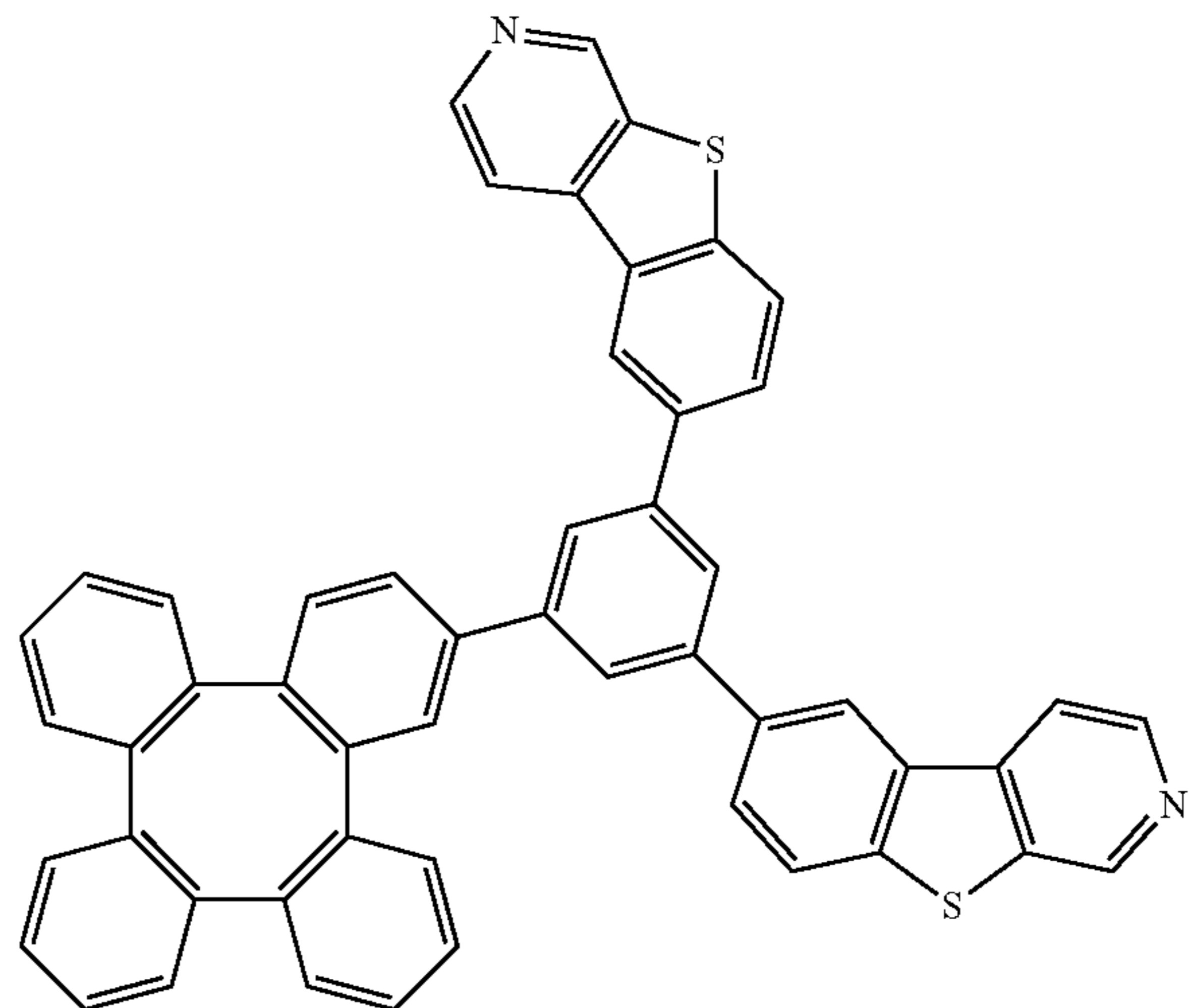
Compound 245
