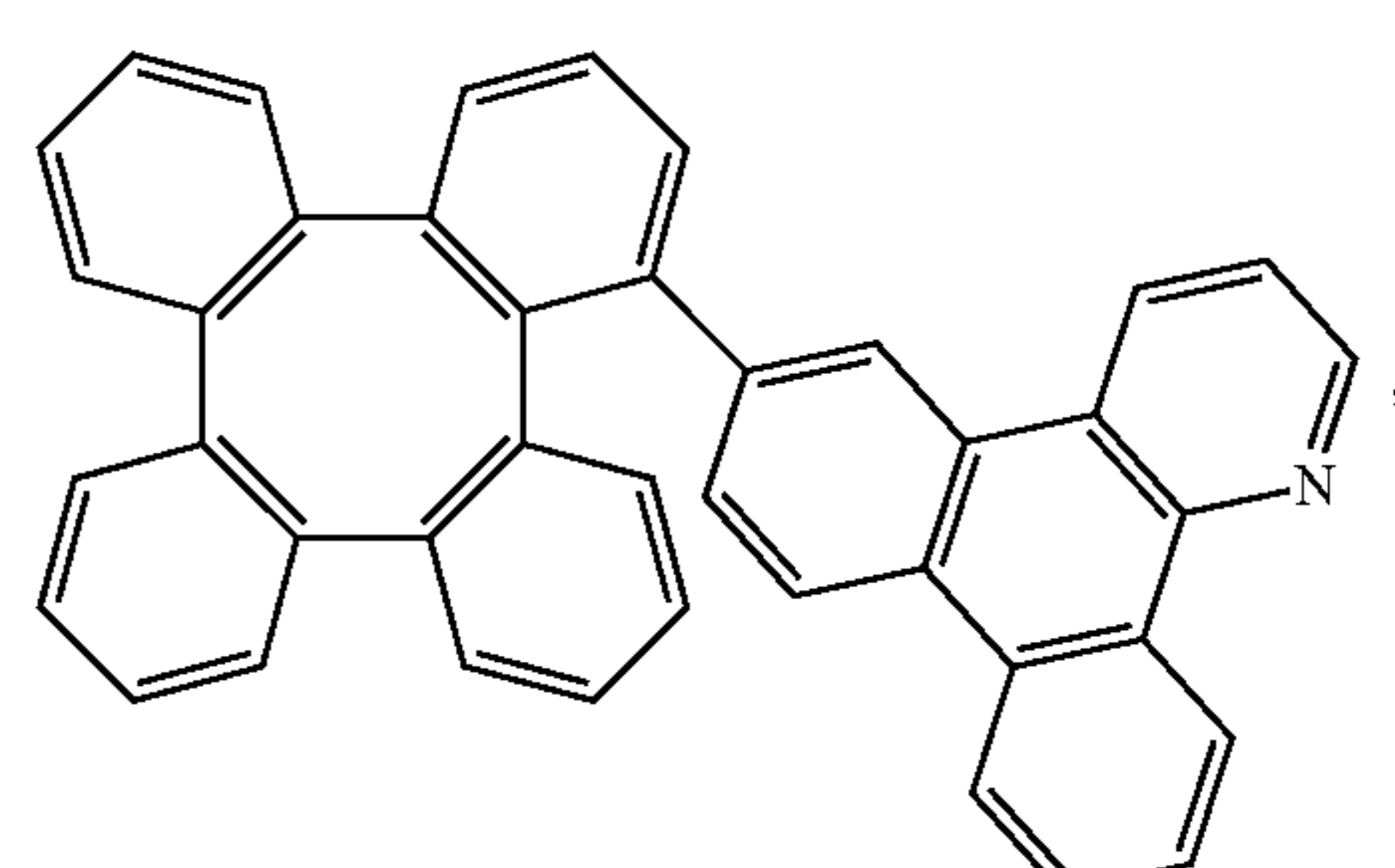
Compound 70
