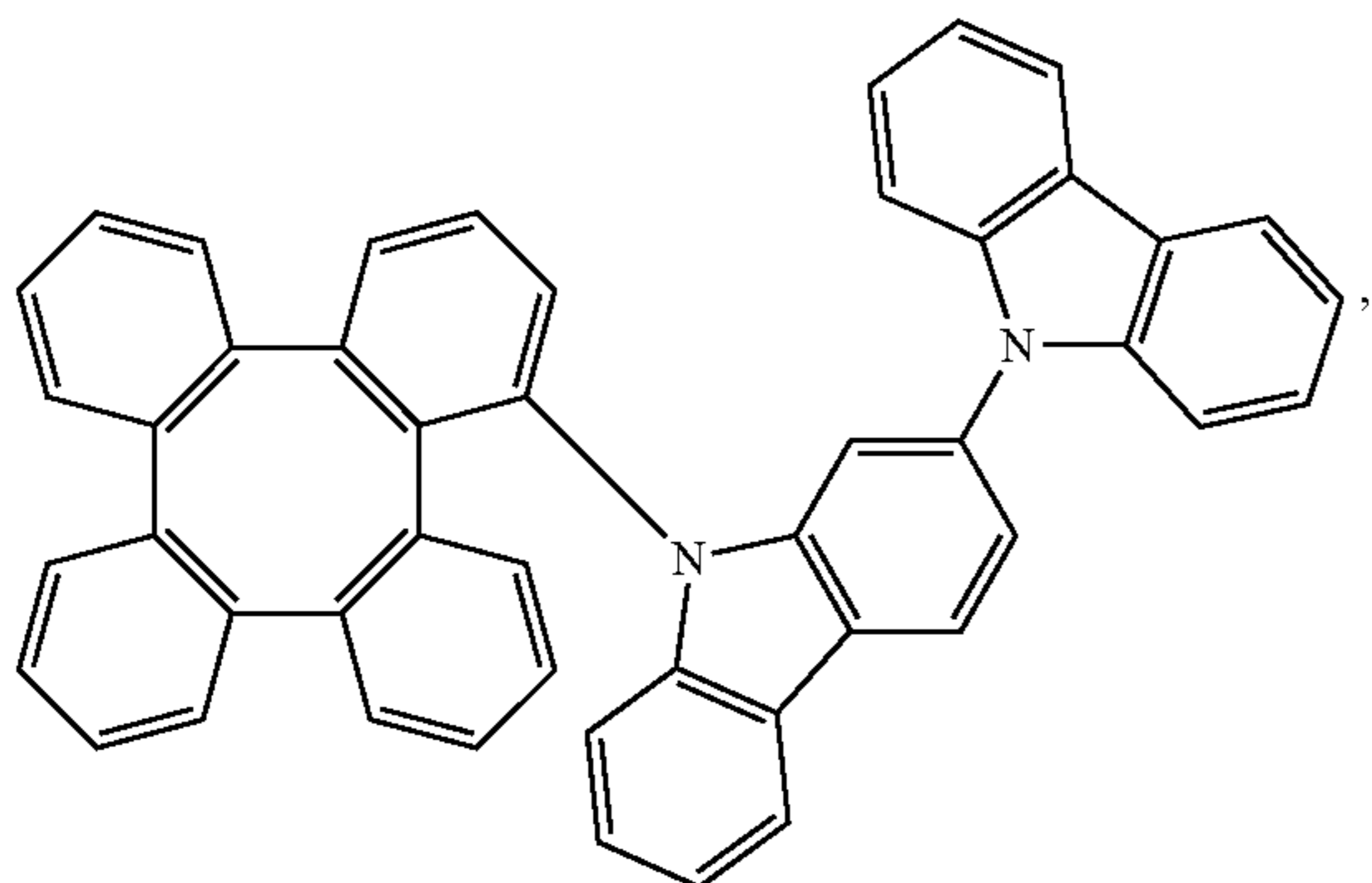
Compound 478
