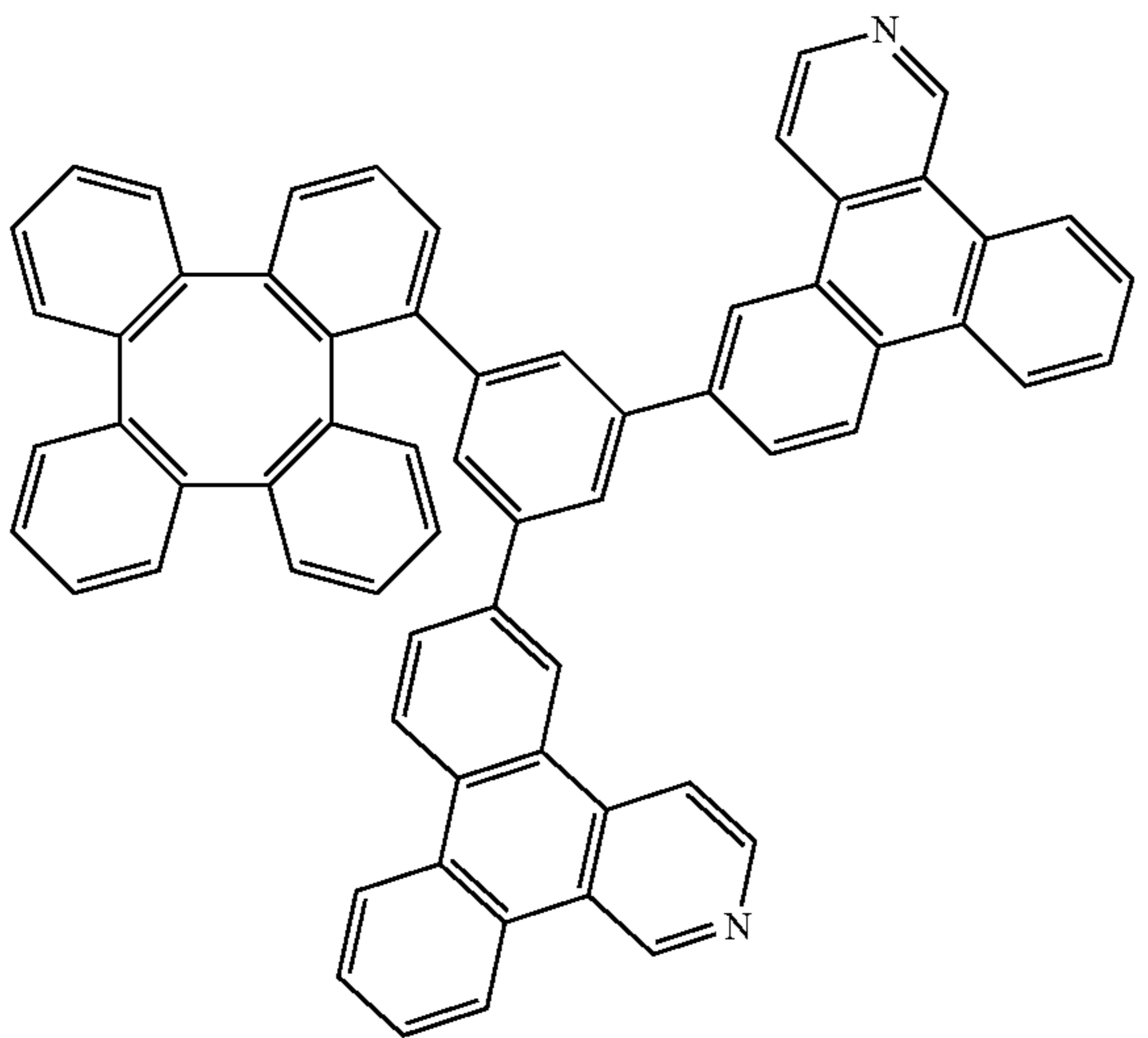
Compound 279
