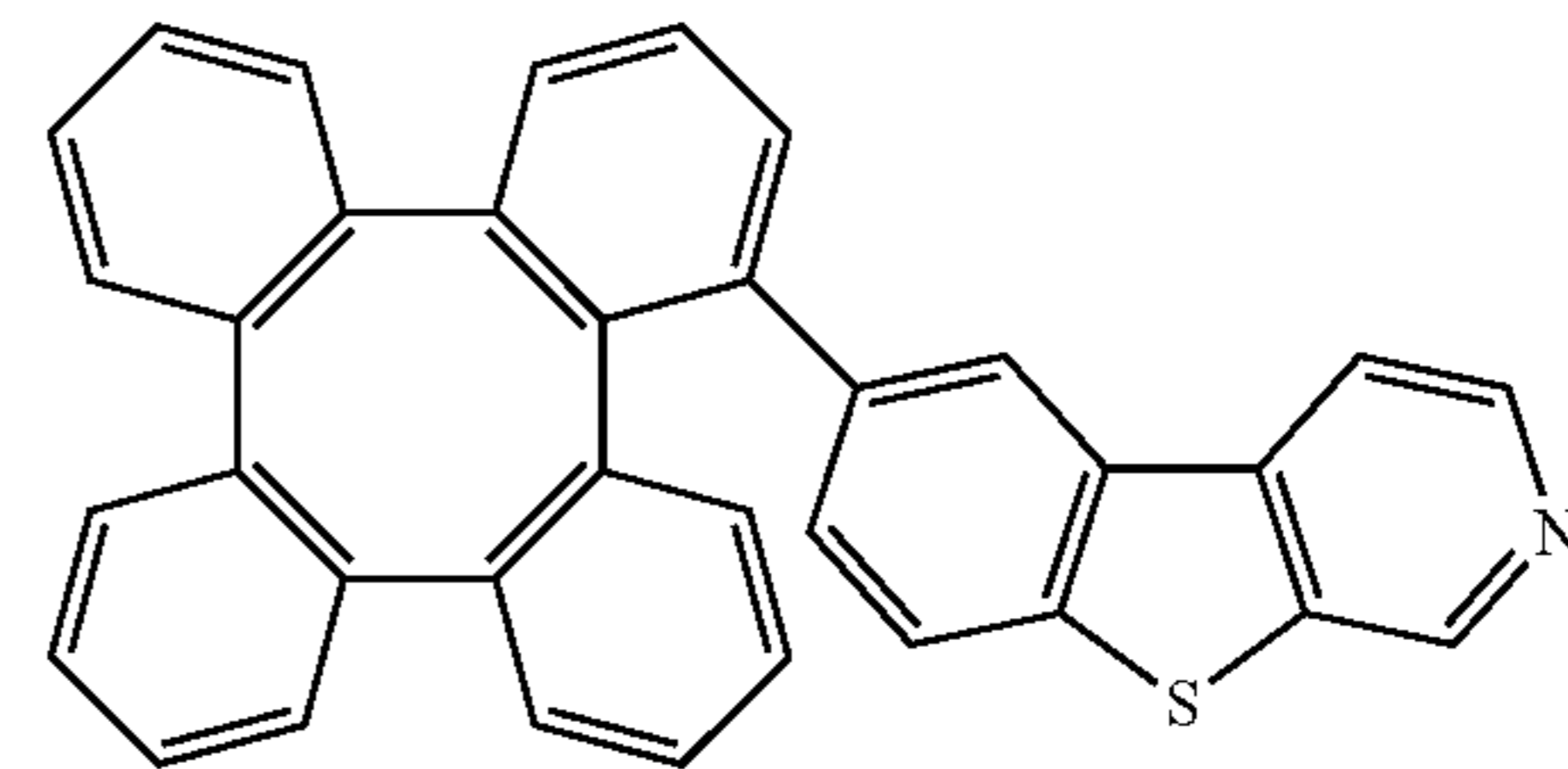
Compound 36
