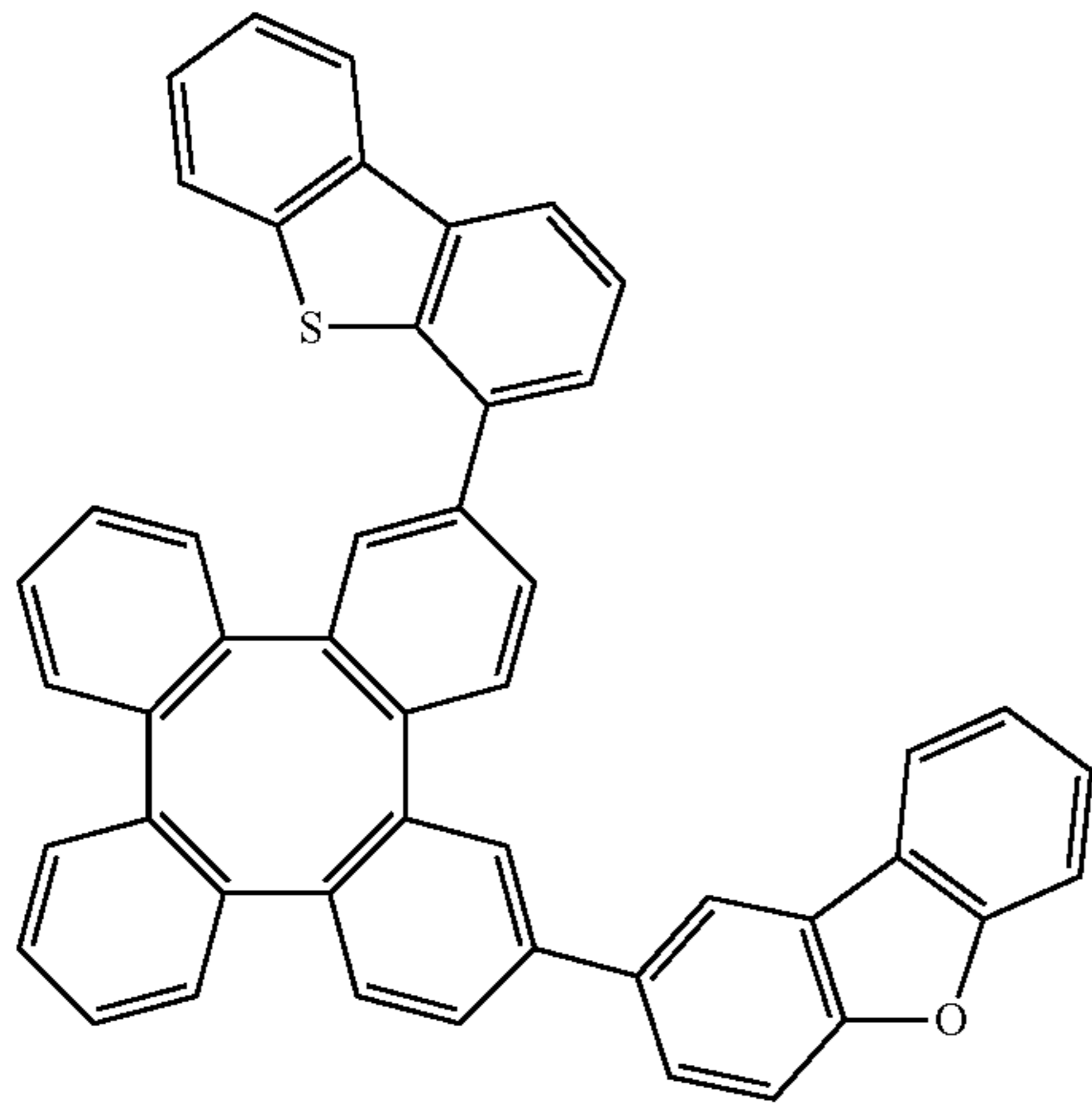
Compound 392
