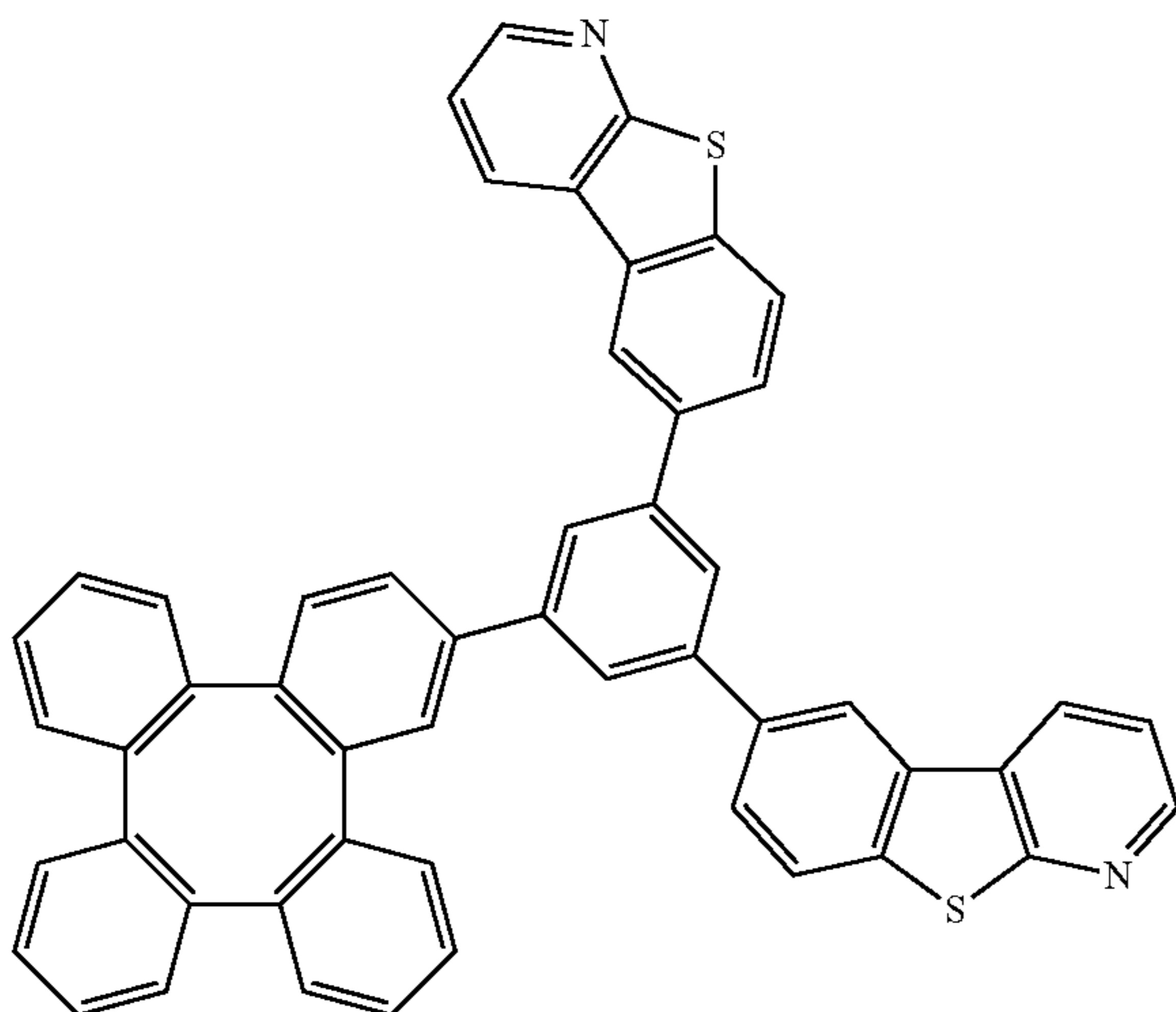
Compound 243
