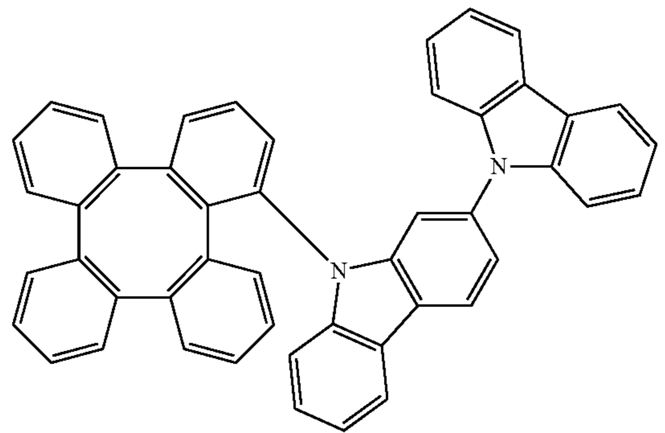
Compound 479
