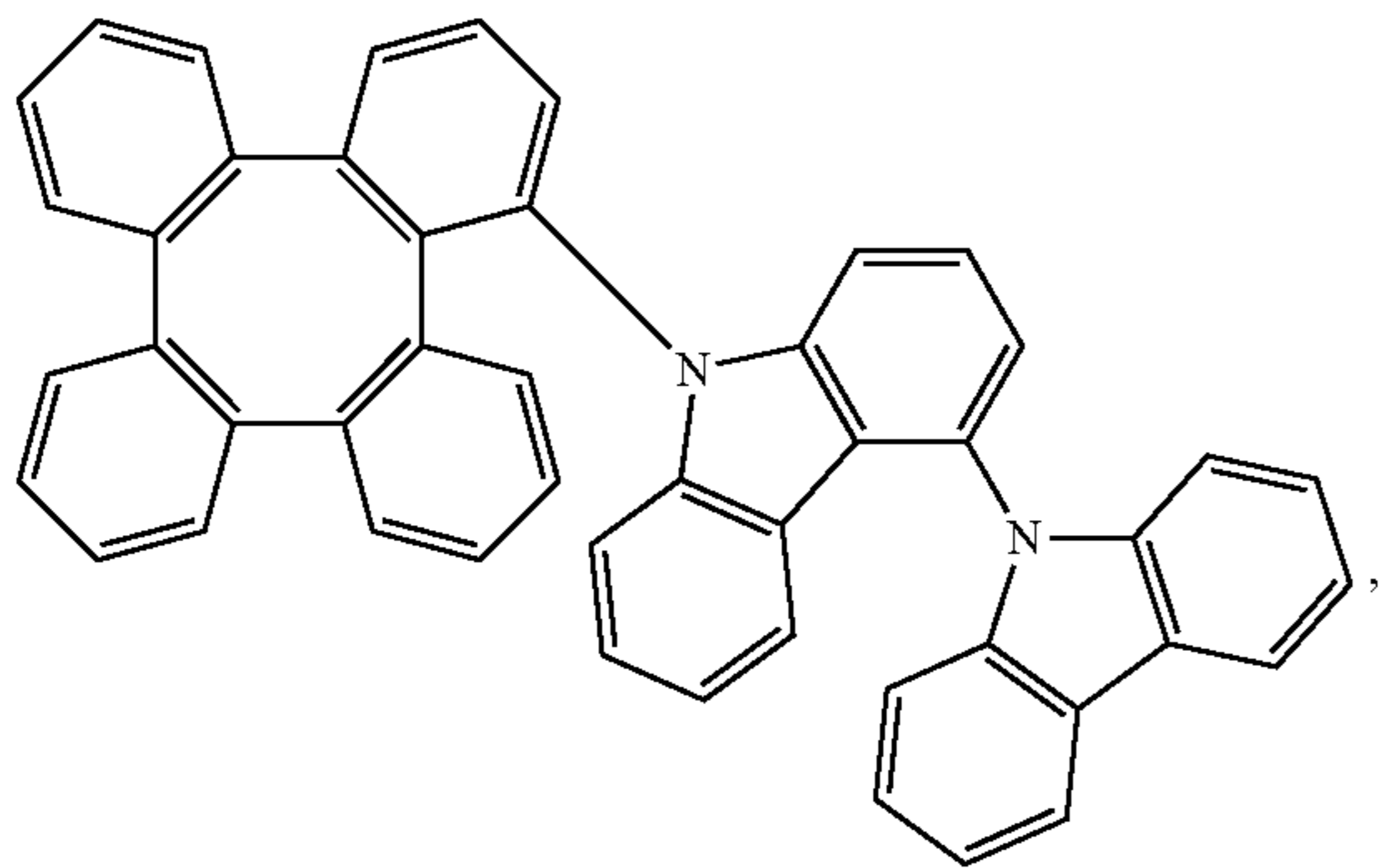
Compound 478
