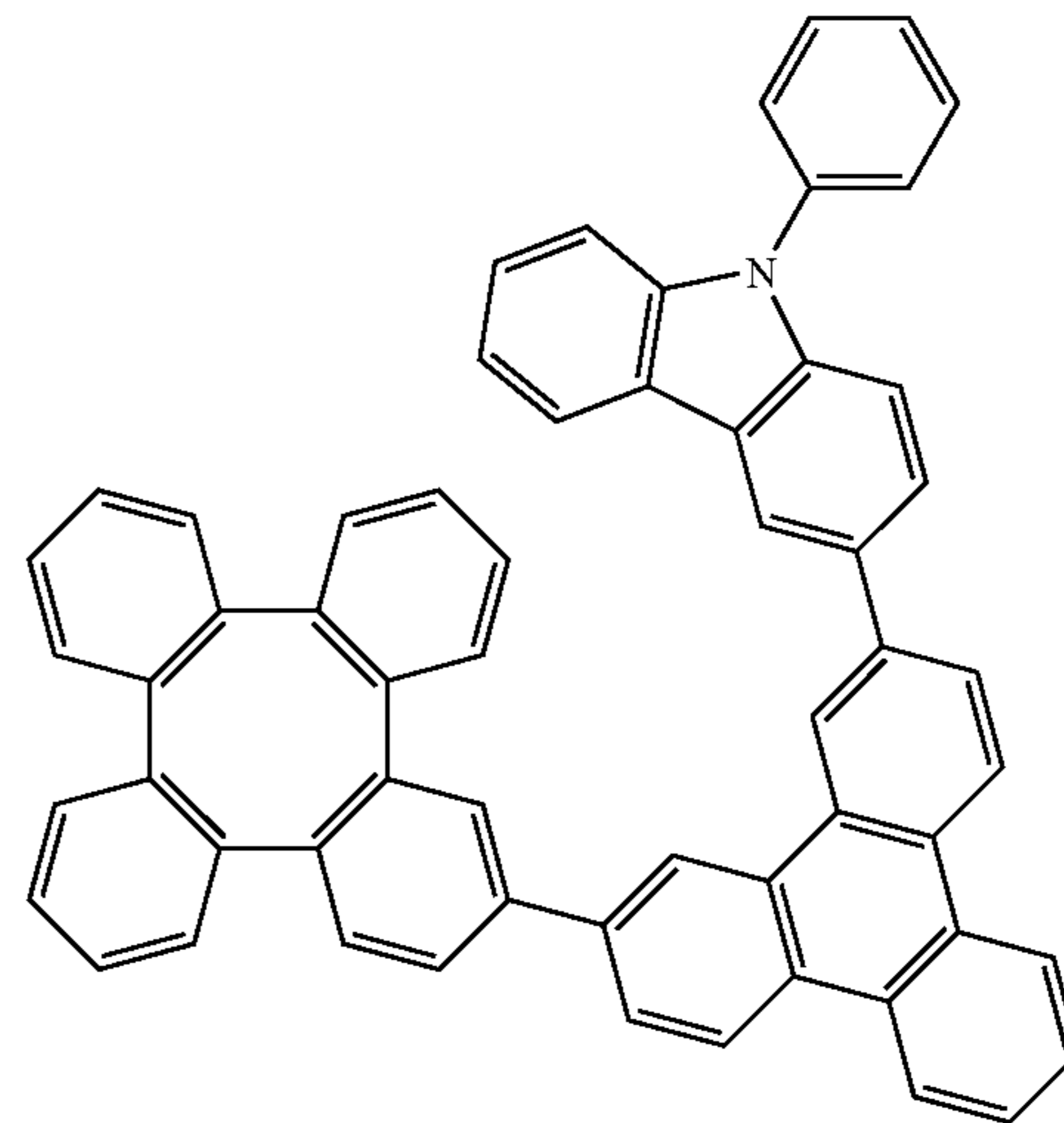
Compound 464
