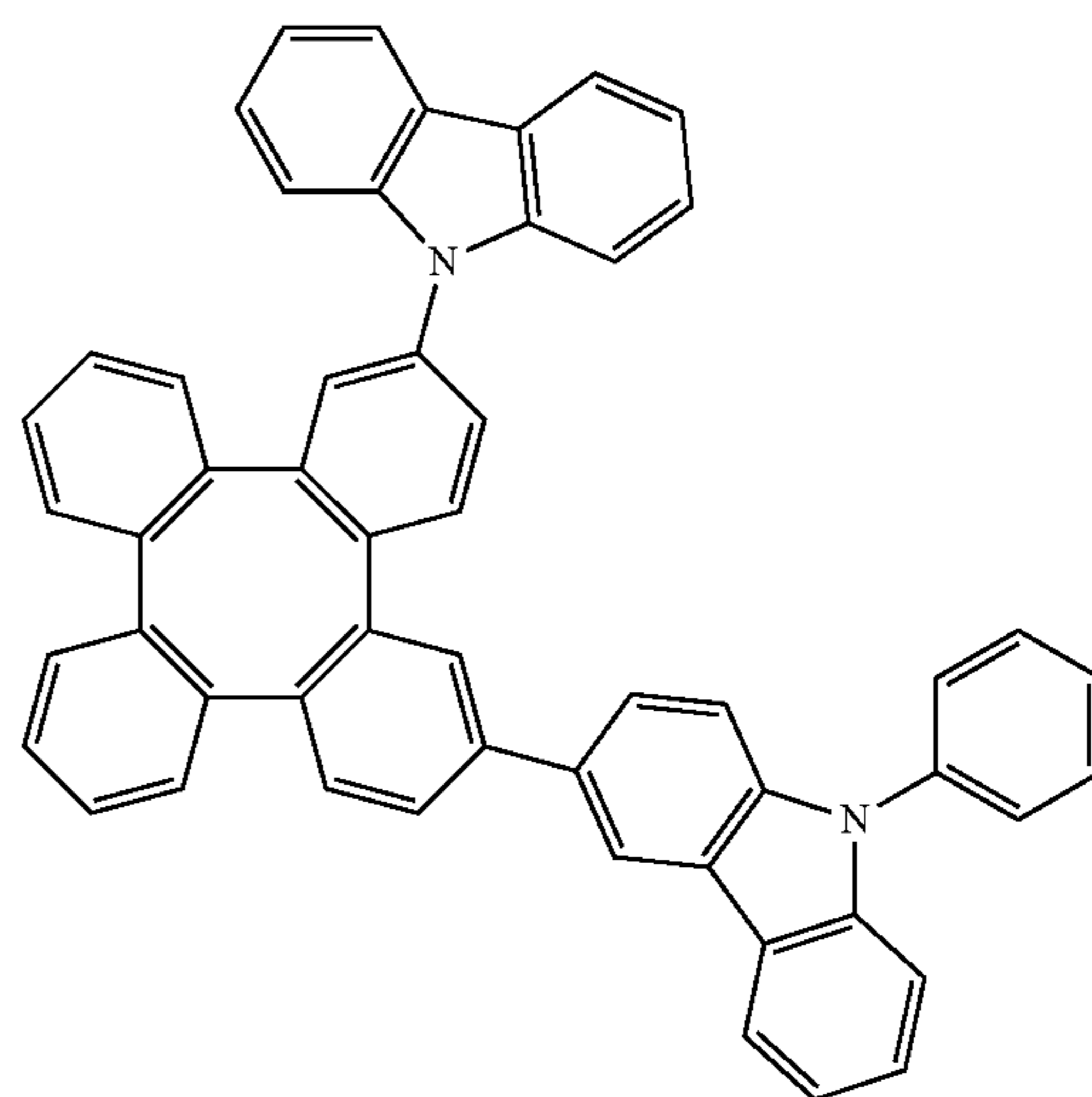
Compound 373
