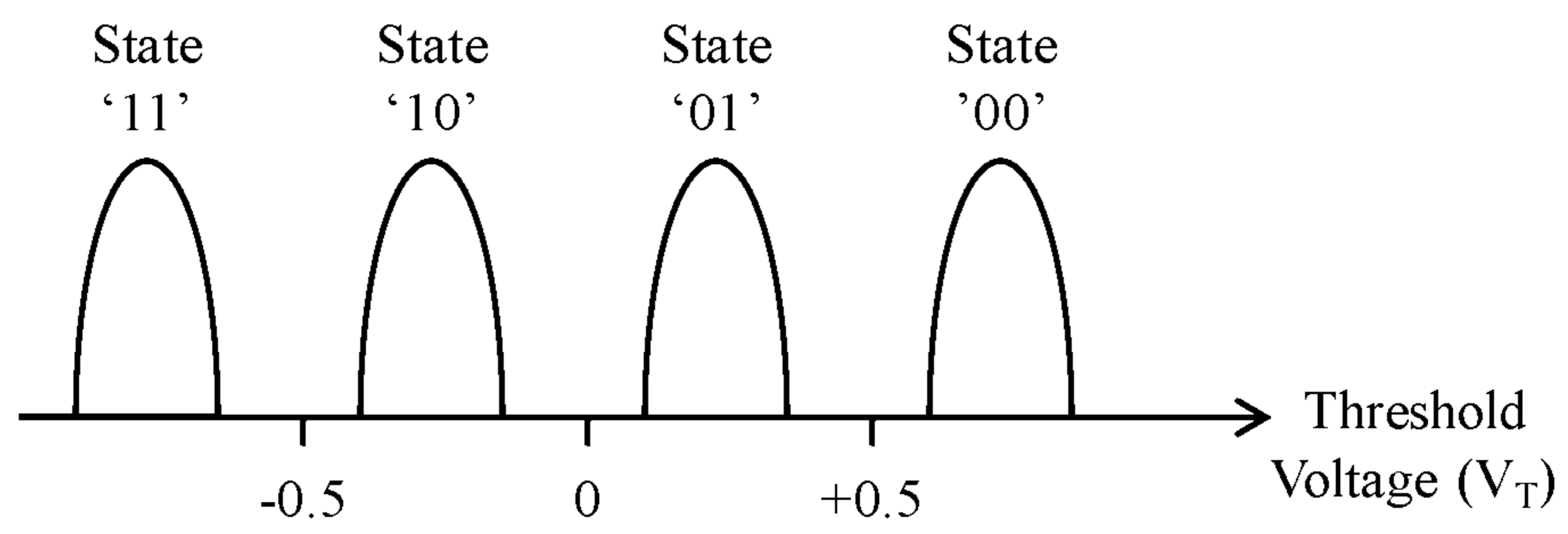
Multi-Level Cell
