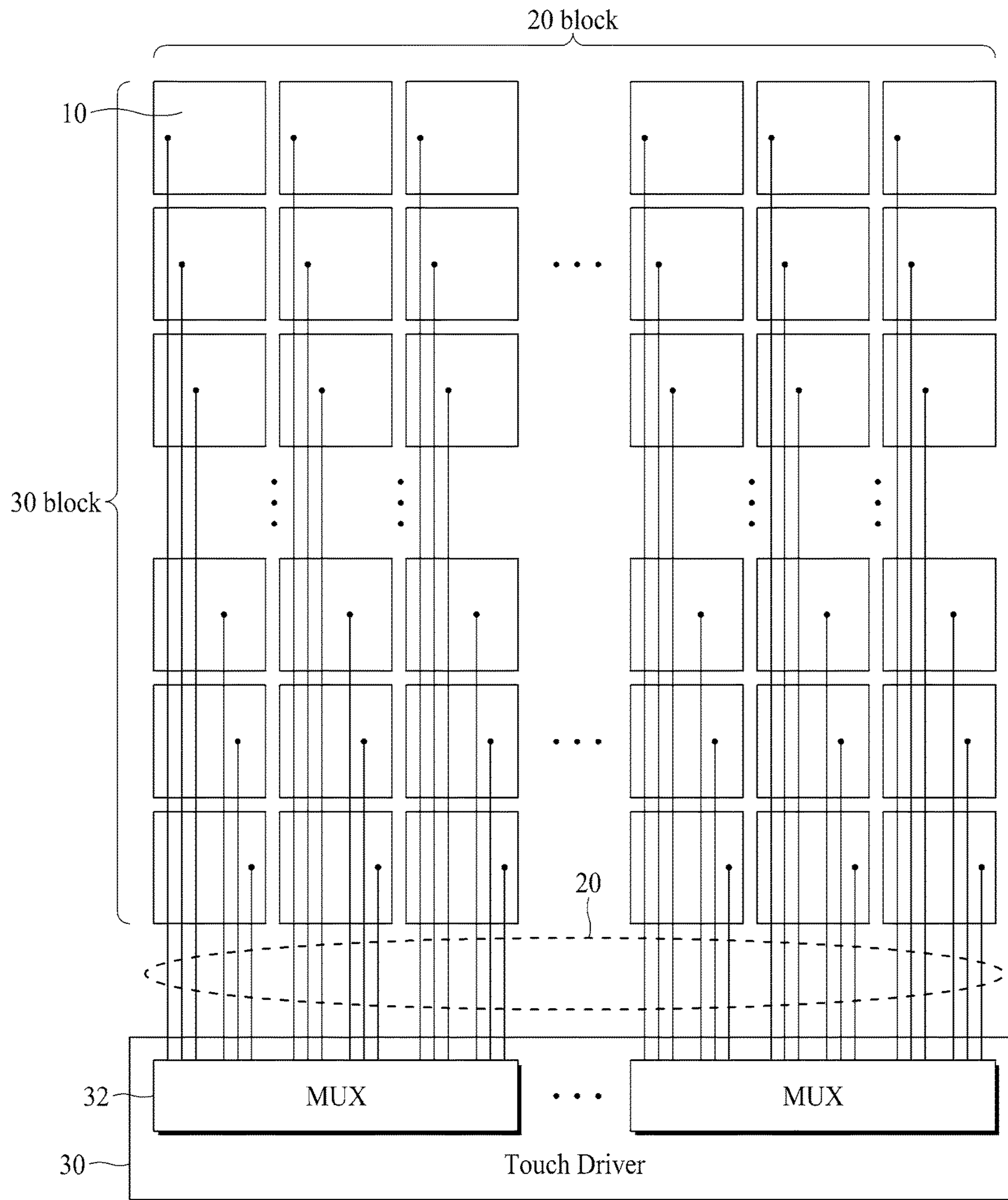
FIG. 1 (RELATED ART)
