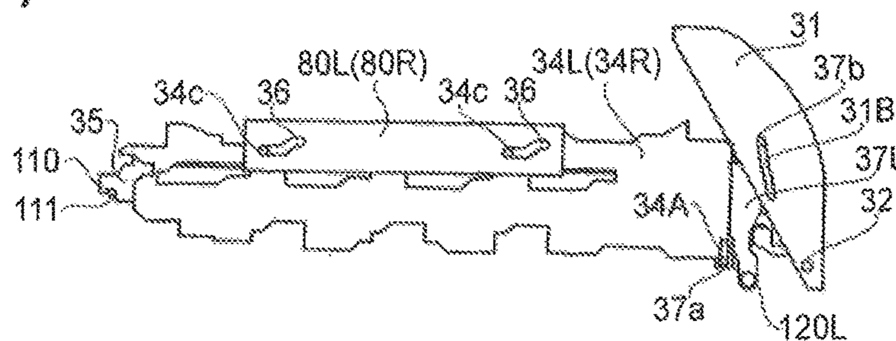
FIG. 5(a) CLOSED
