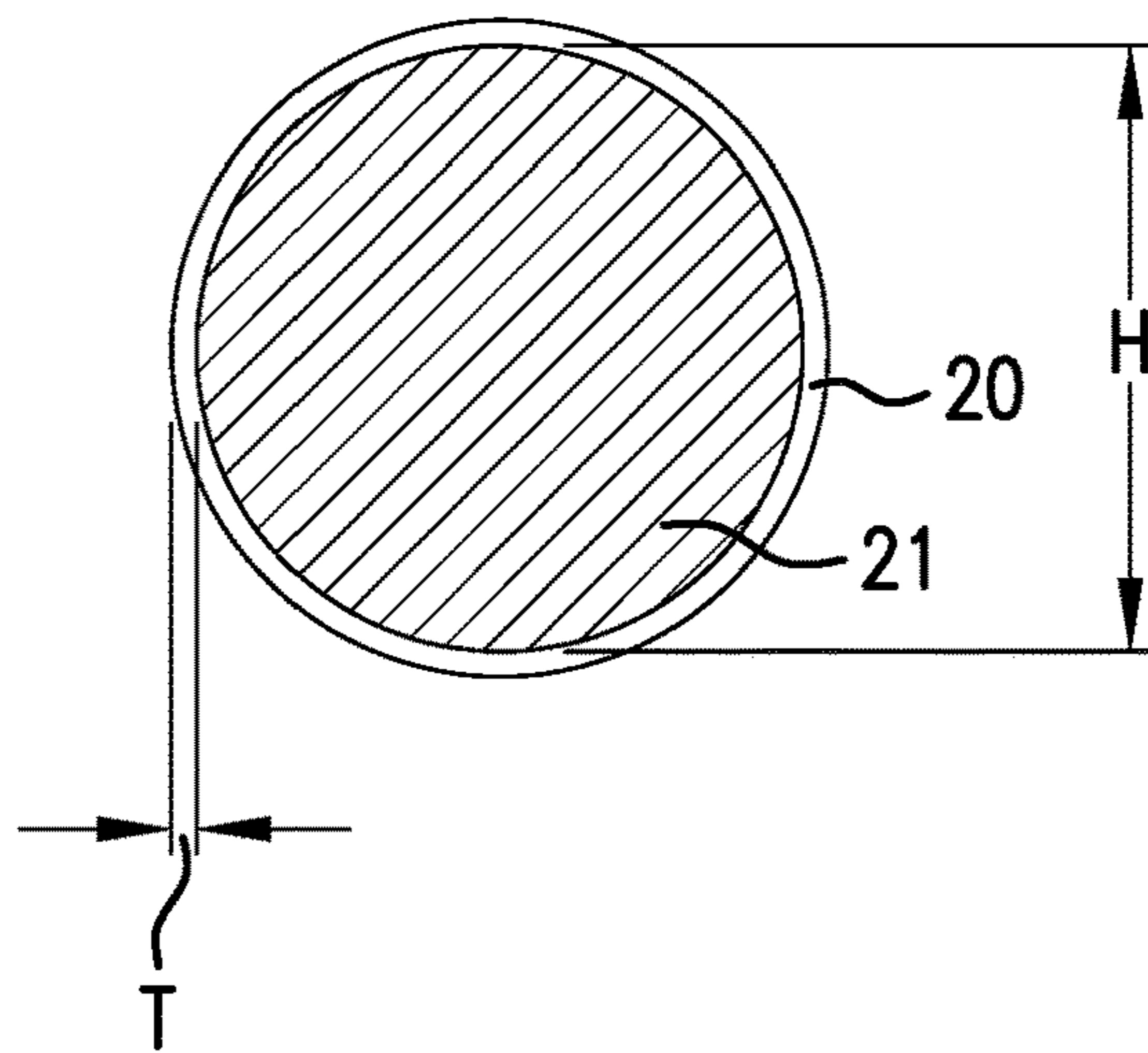
Section B-B'
