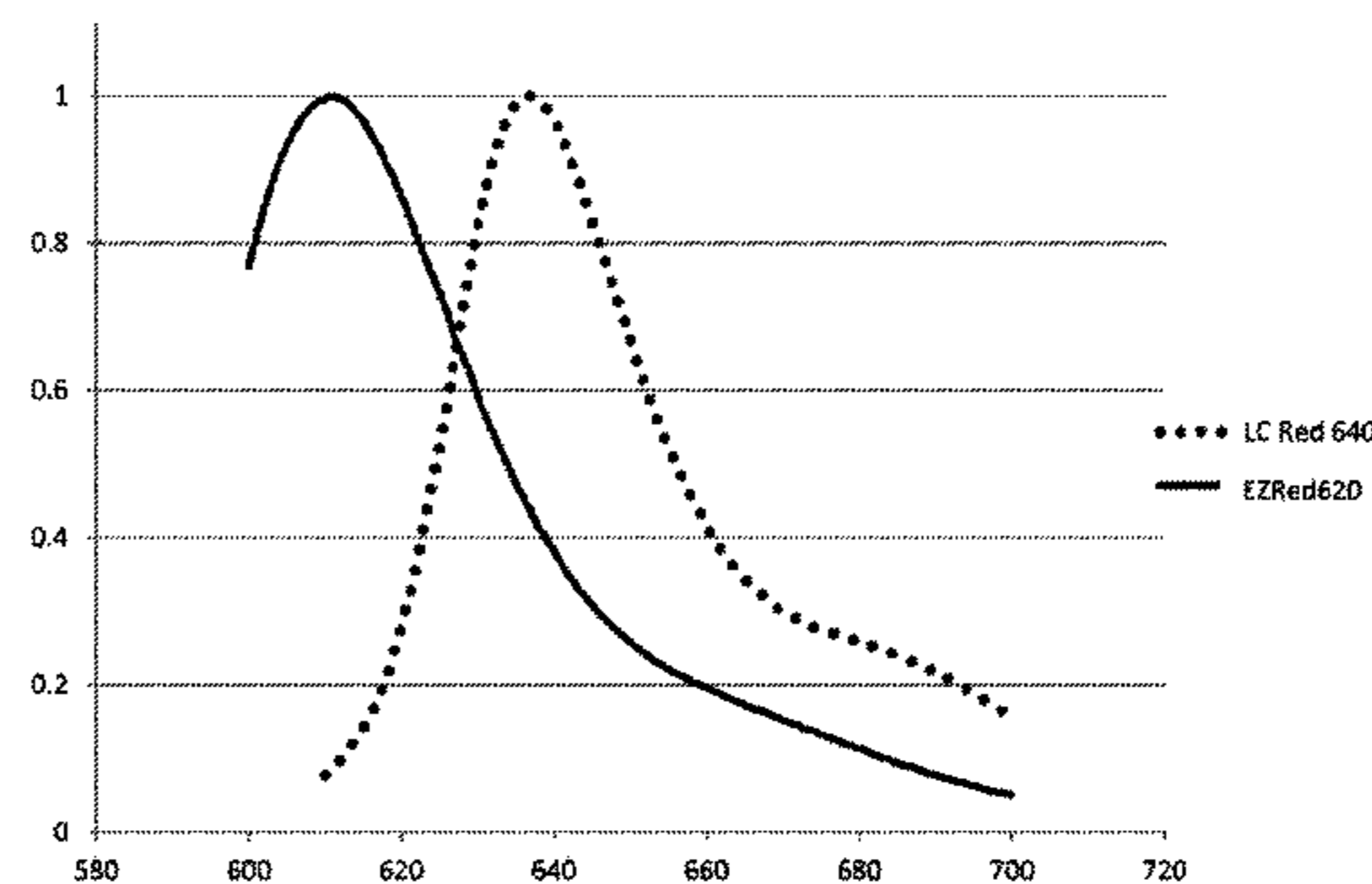
Emission spectra of LC Red 640 and EZRed620
