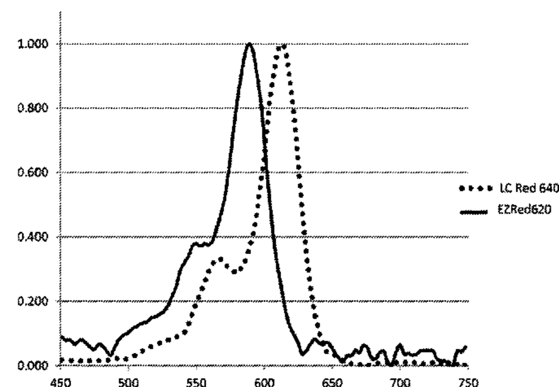
UV-Vis spectra of LC Red 640 and EZRed620
