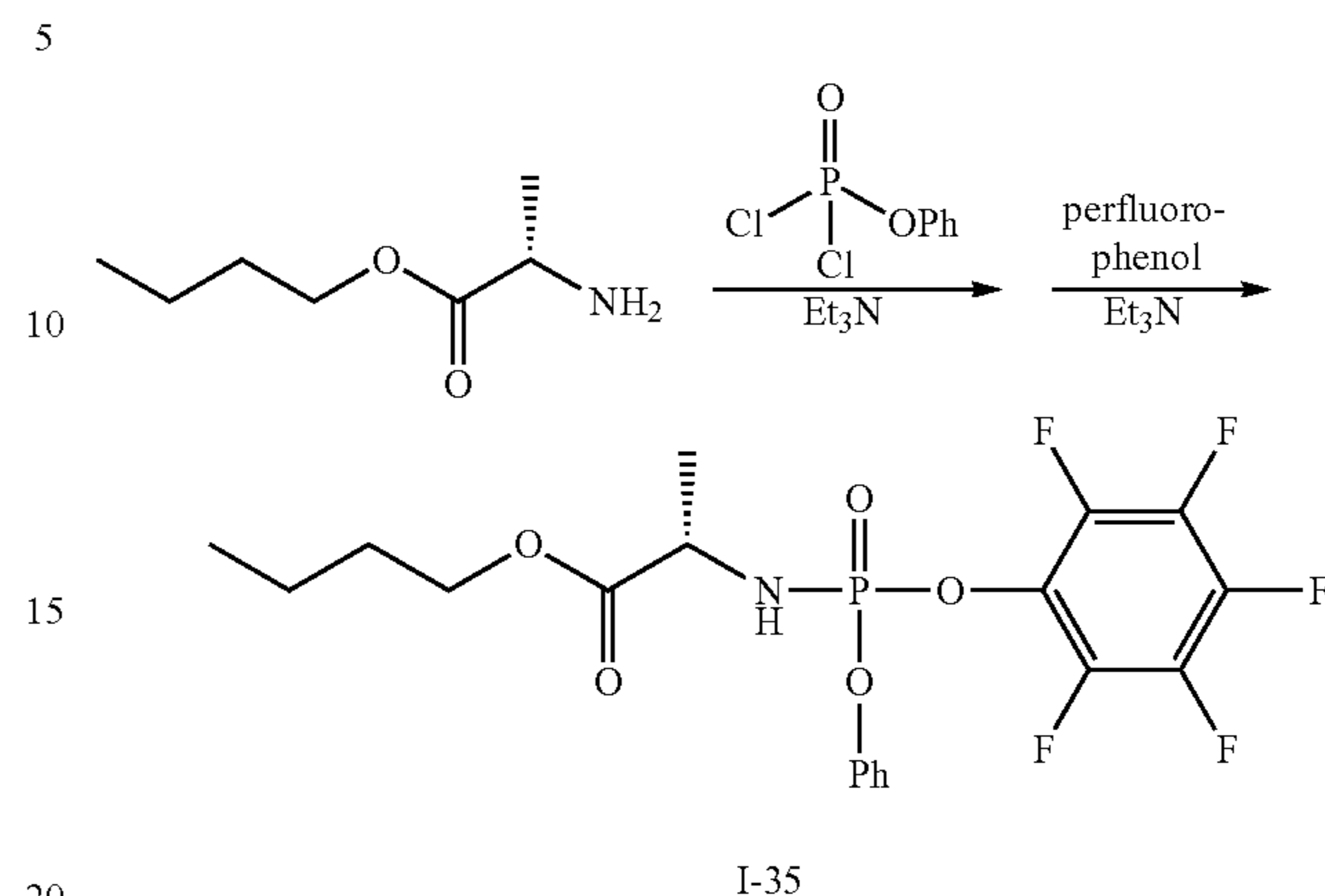
(2S)-butyl 2-(((perfluorophenoxy)(phenoxy)phosphoryl)amino)propanoate (I-35)
