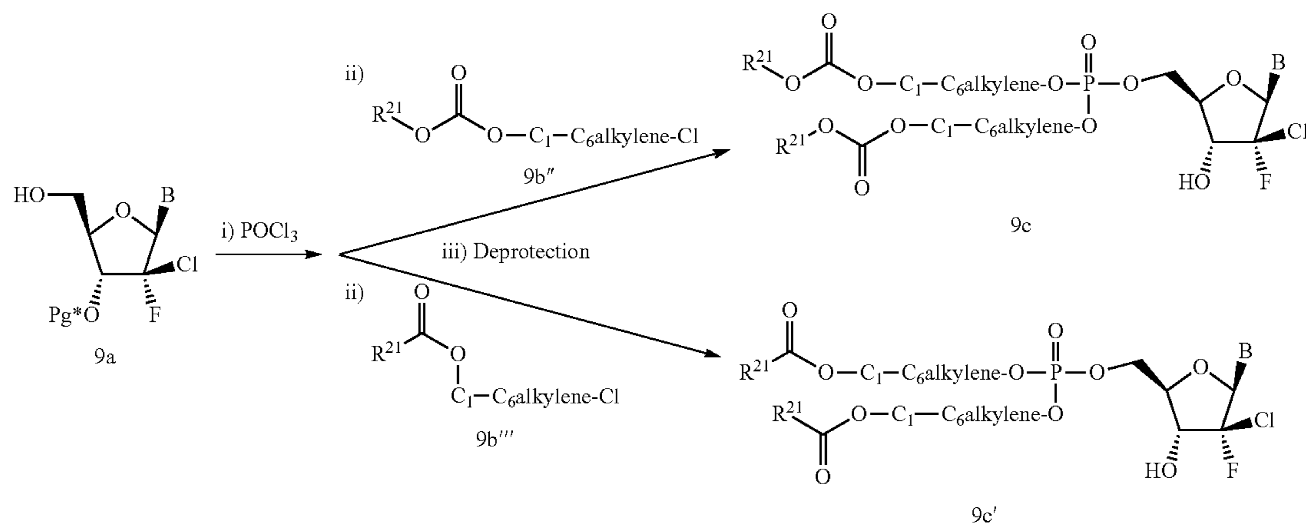
Scheme 9B
