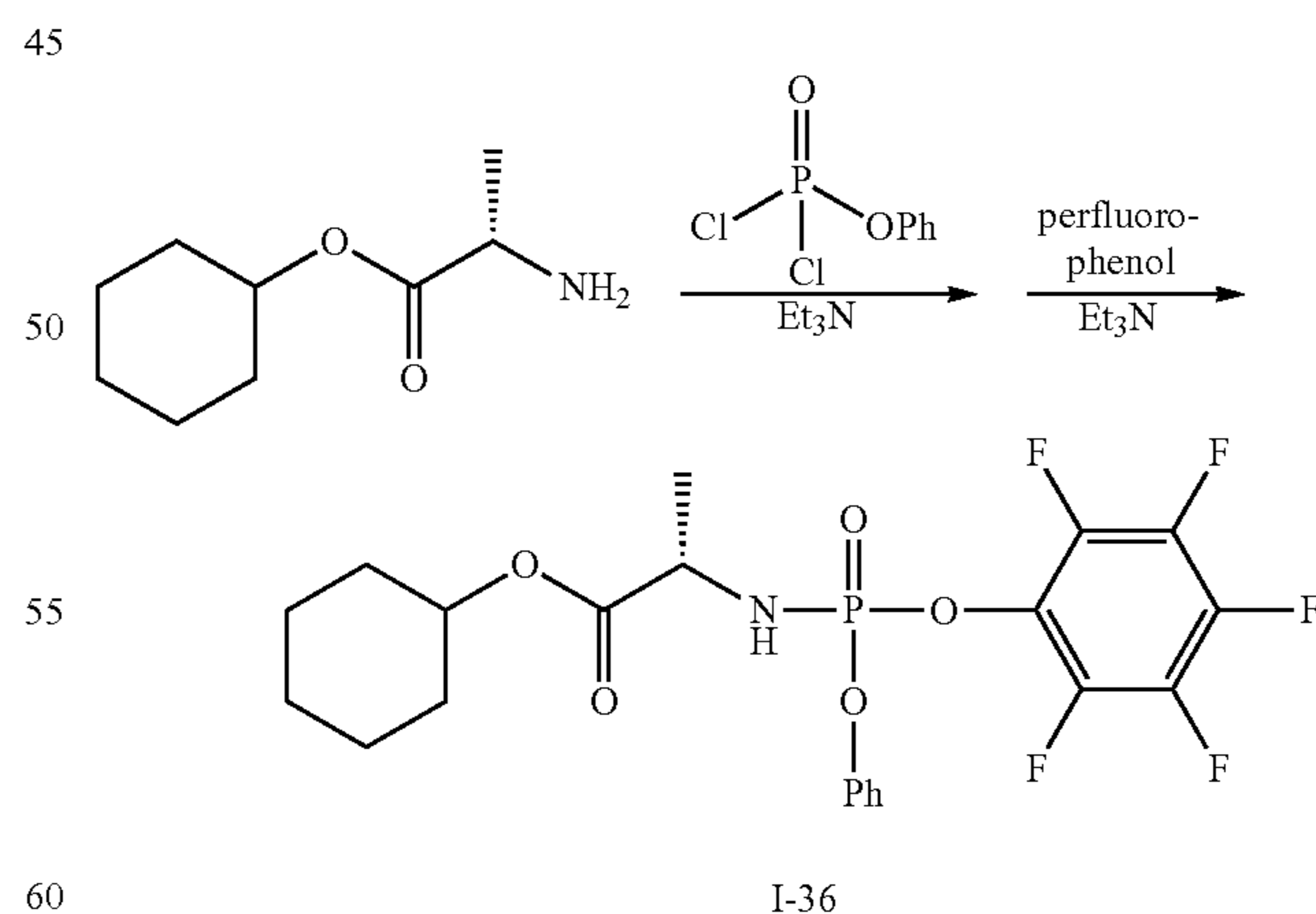
(2S)-Cyclohexyl 2-(((perfluorophenoxy)(phenoxy)phosphoryl)amino)propanoate (I-36)
