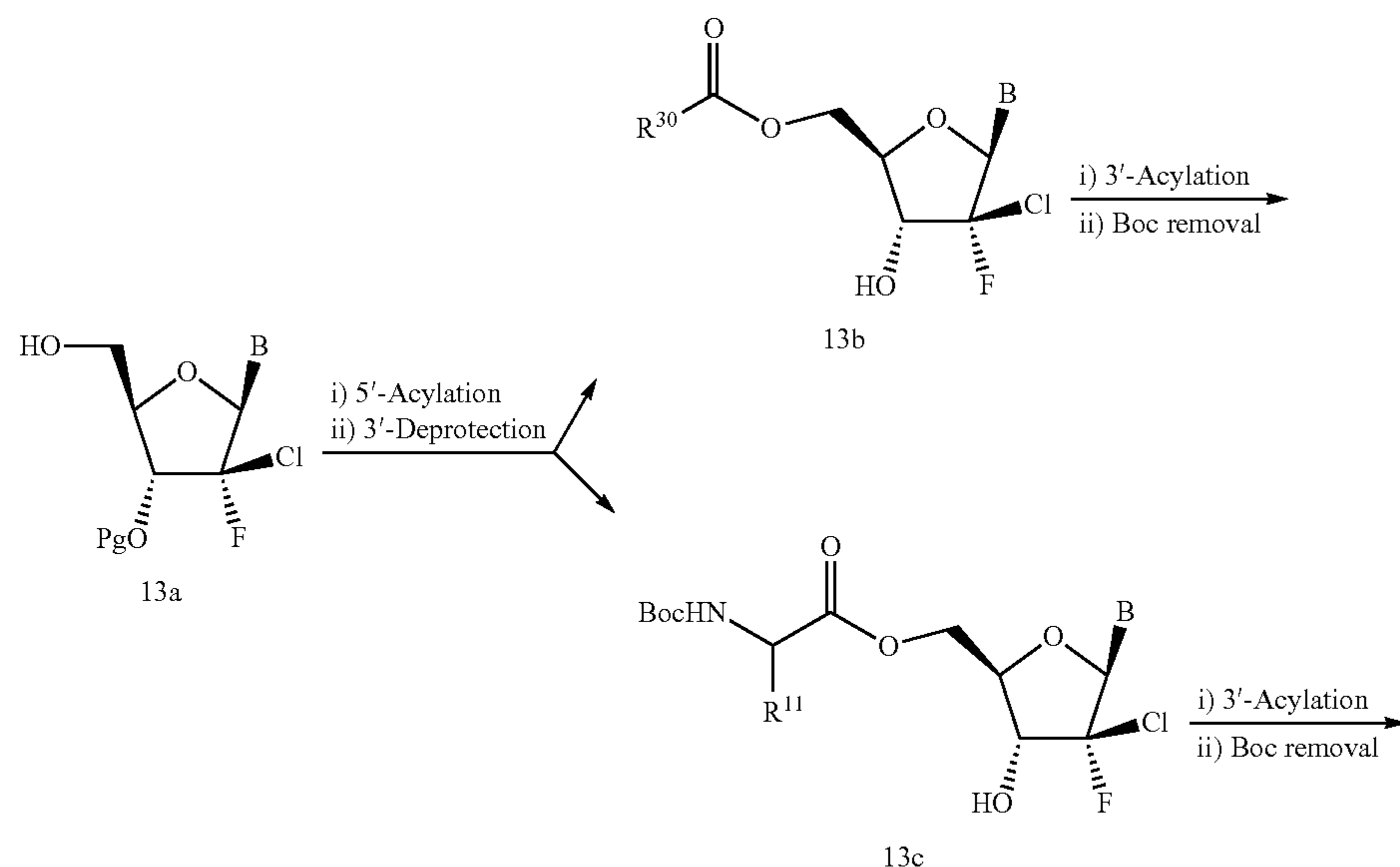
Scheme 13
