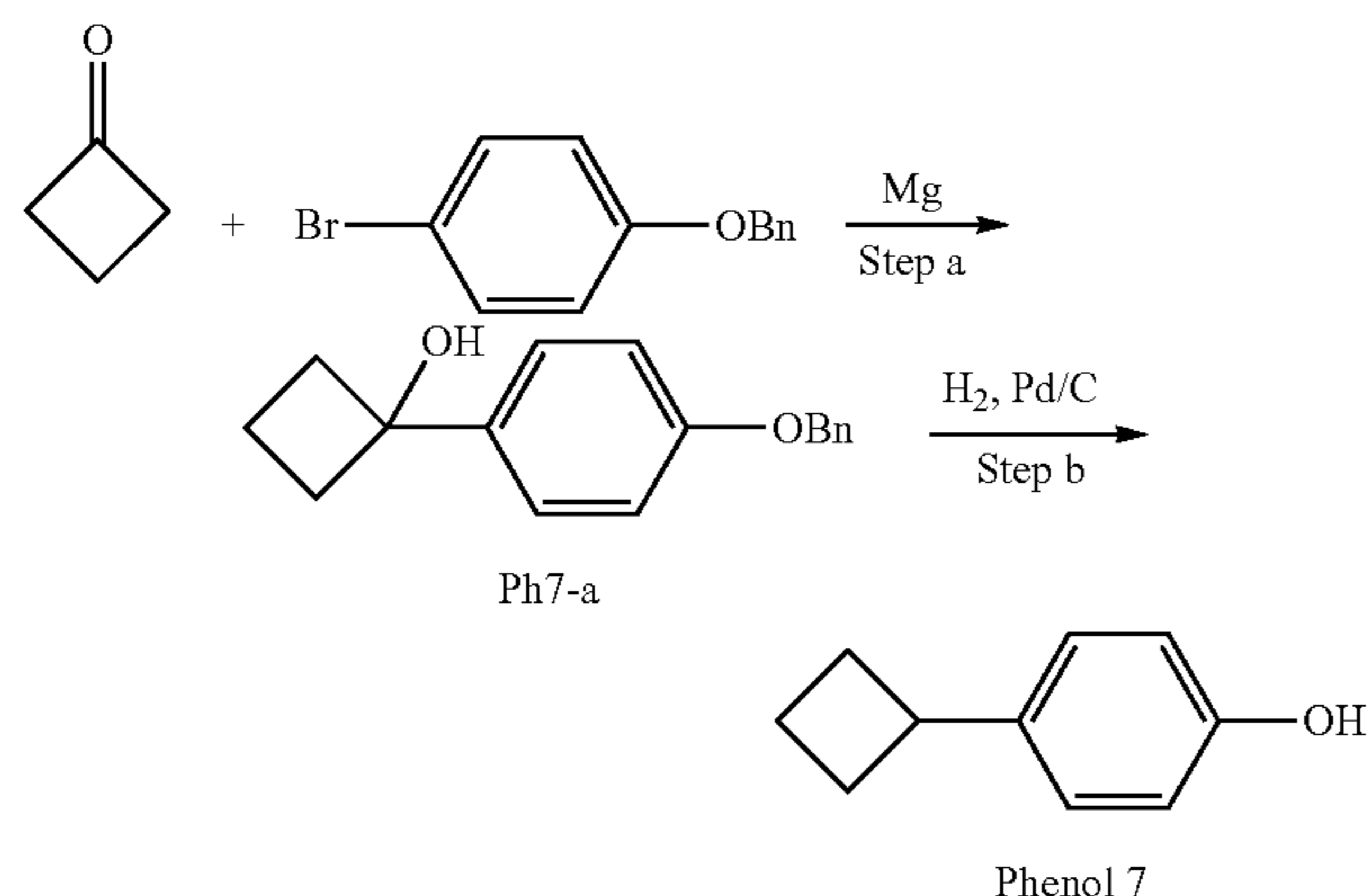
Step a) 1-(4-(benzyloxy)phenyl)cyclobutanol (Ph7-a)
