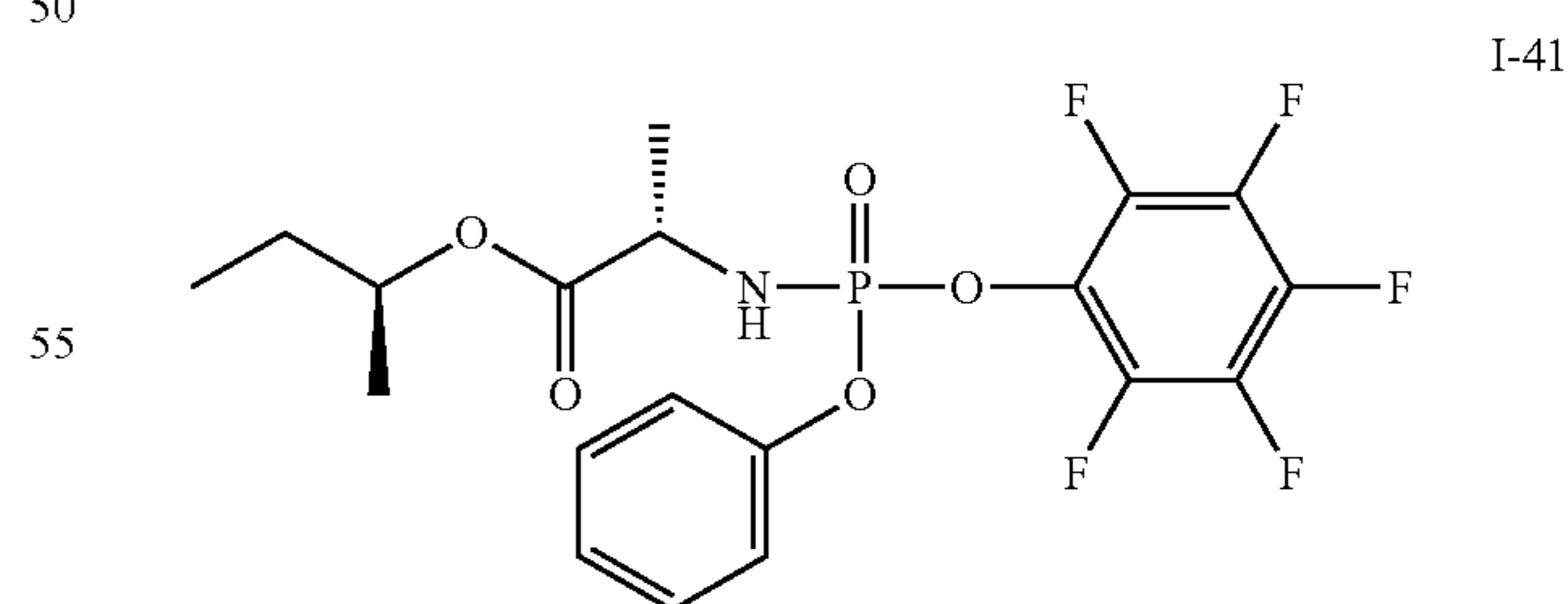
(2S)-(S)-Sec-butyl 2-(((perfluorophenoxy)(phenoxy)phosphoryl)amino)propanoate (I-41)
