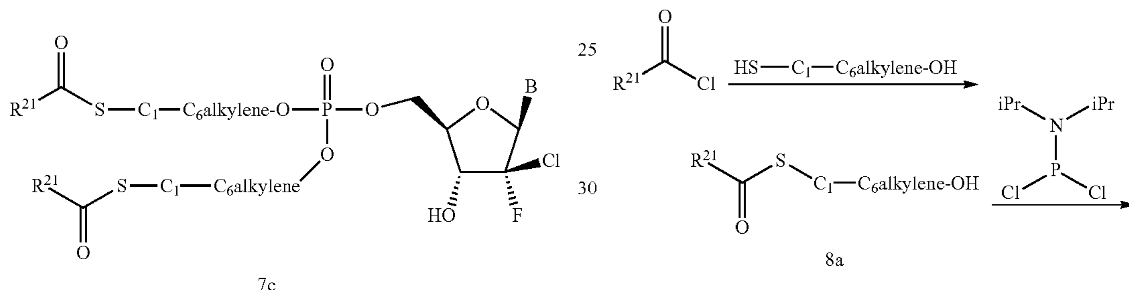
Scheme 8
