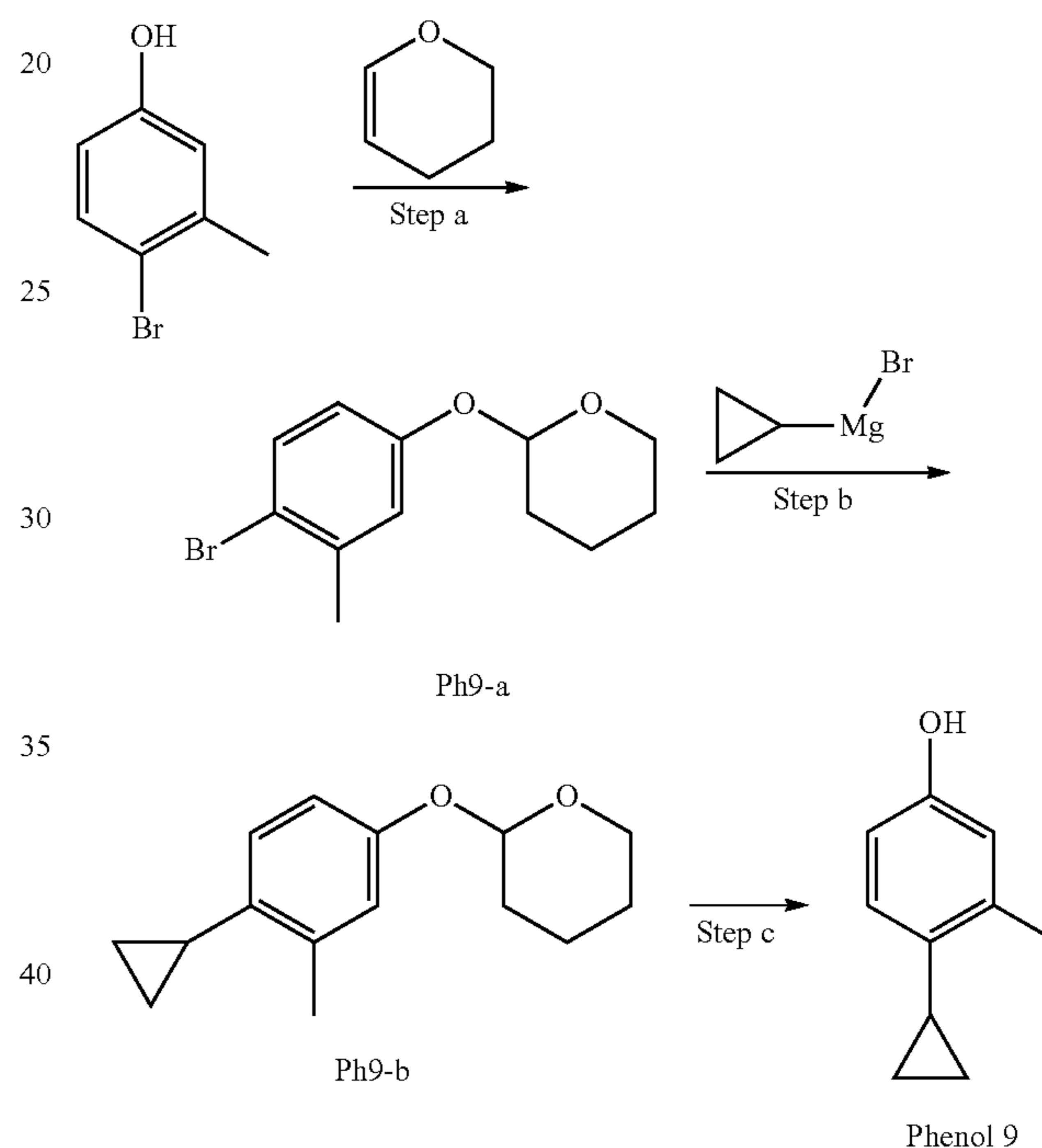
Step a) 2-(4-Bromo-3-methylphenoxy)tetrahydro-2H-pyran (Ph9-a)
