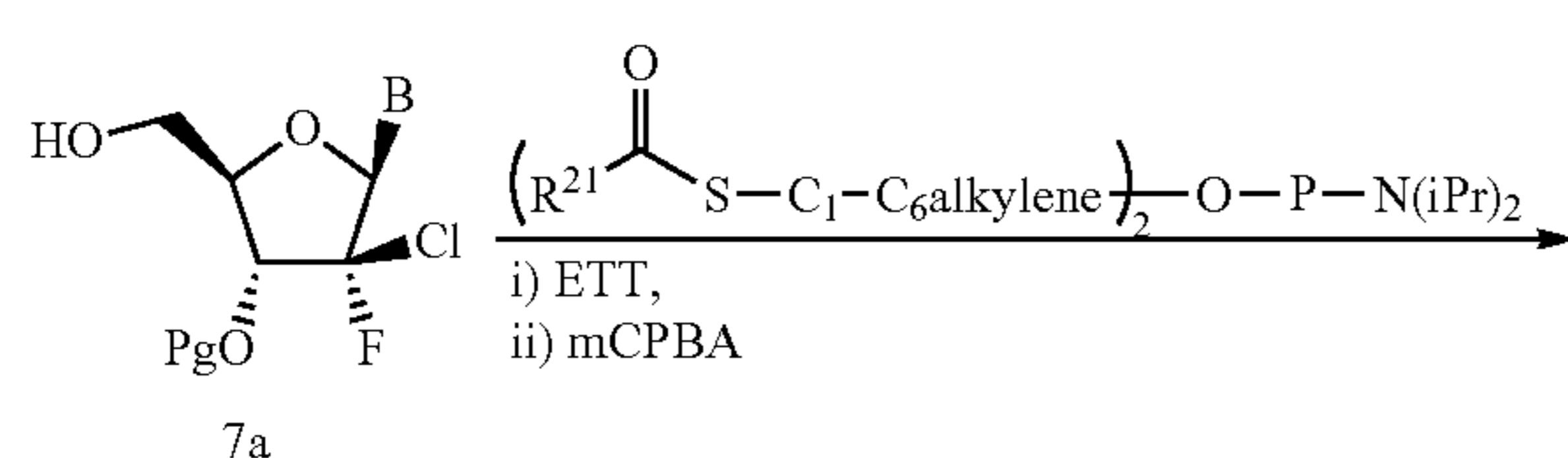
Scheme 7B
