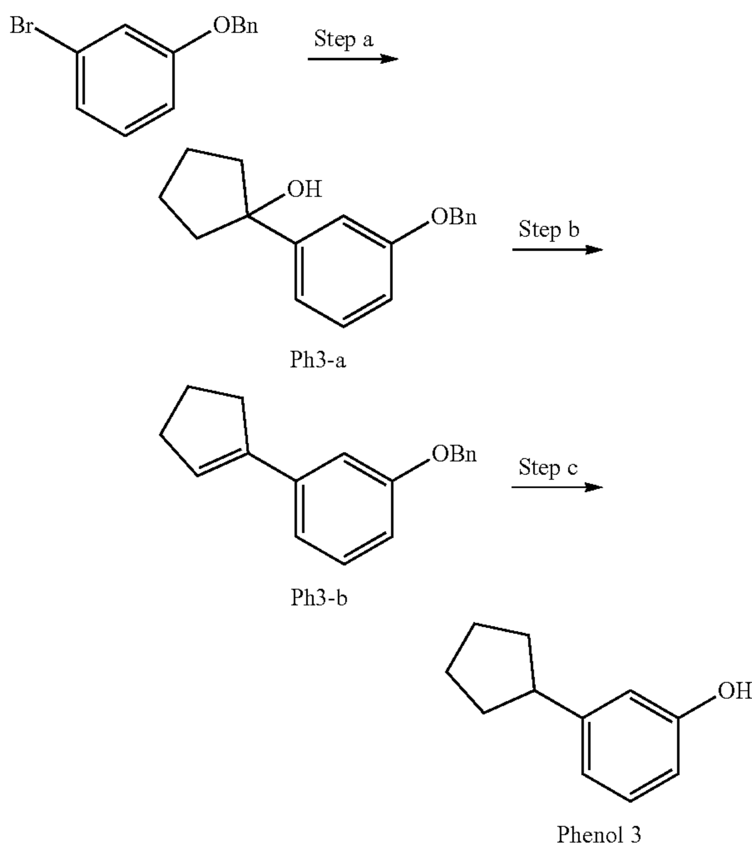
Step a) 1-(3-(benzyloxy)phenyl)cyclopentanol (Ph3-a)
