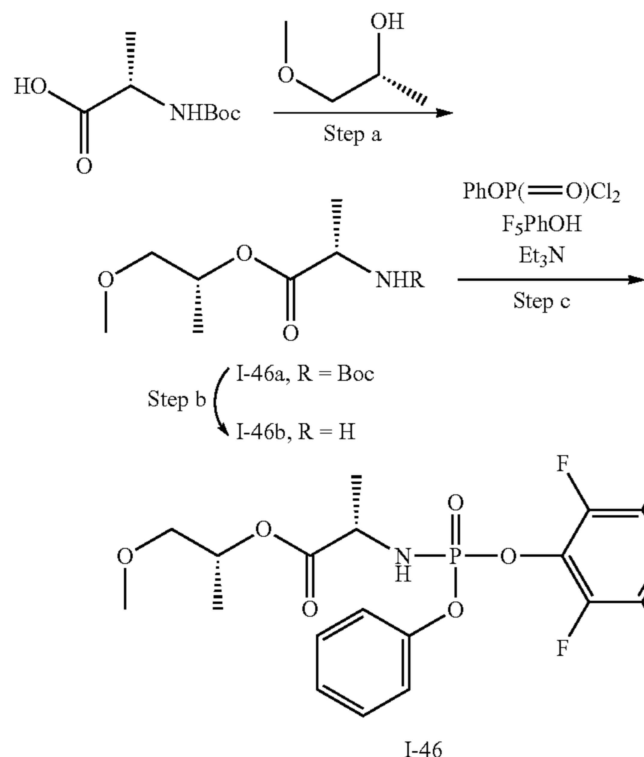
Step a) (S)—(R)-1-Methoxypropan-2-yl 2-((tert-butoxycarbonyl)amino)propanoate (I-46a)
