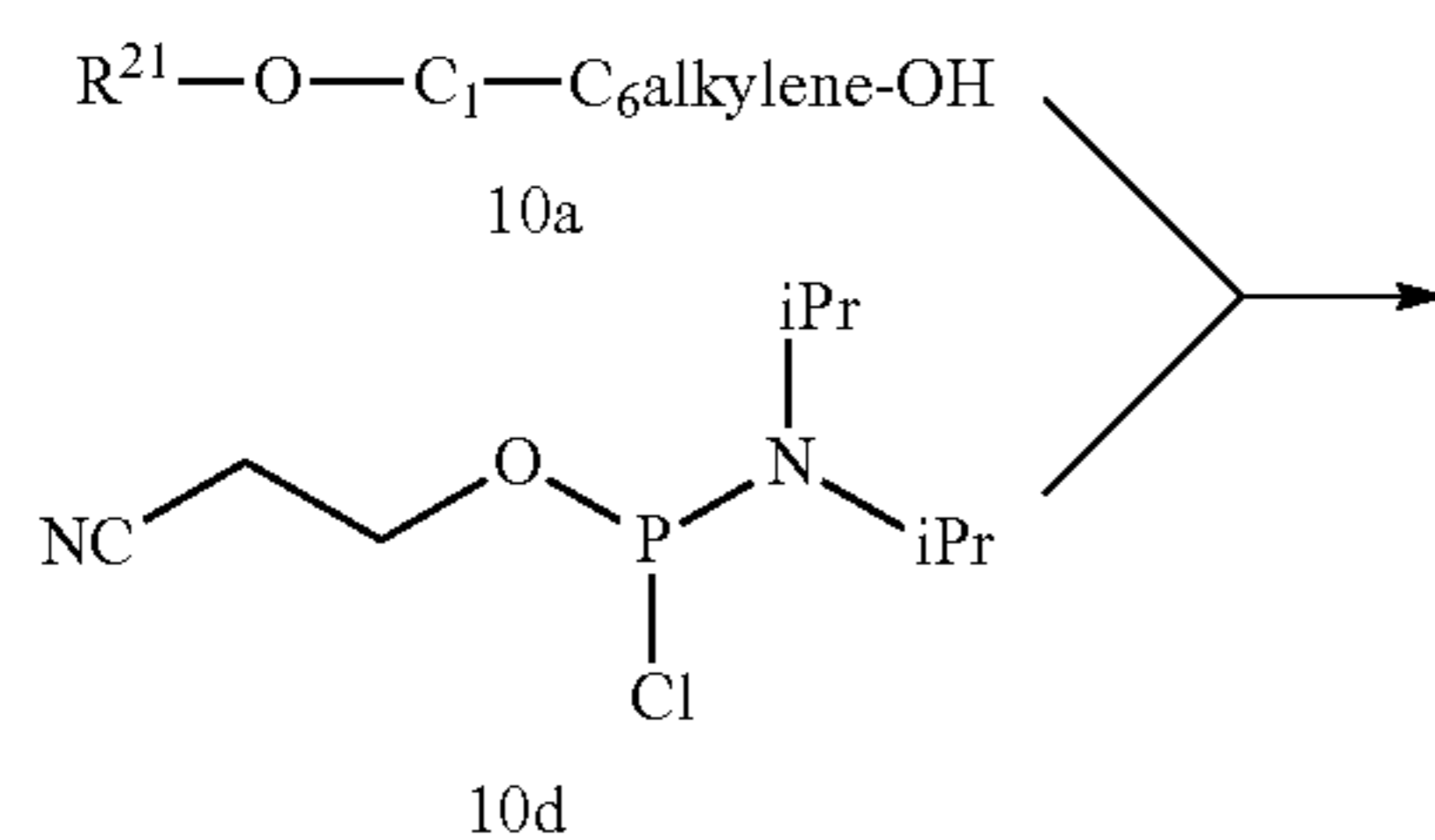
Scheme 10B
