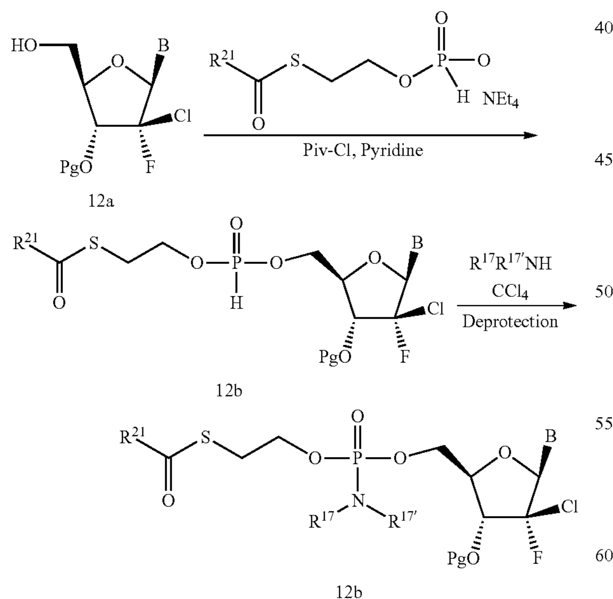
Scheme 12A
