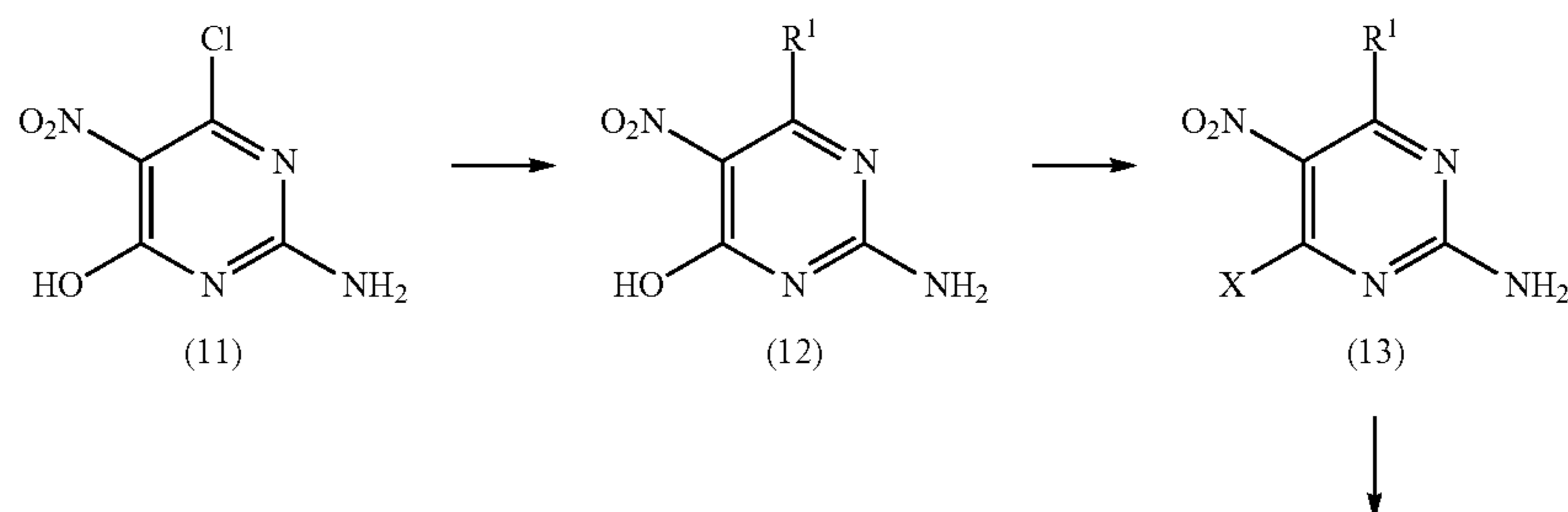
Reaction Scheme 3
