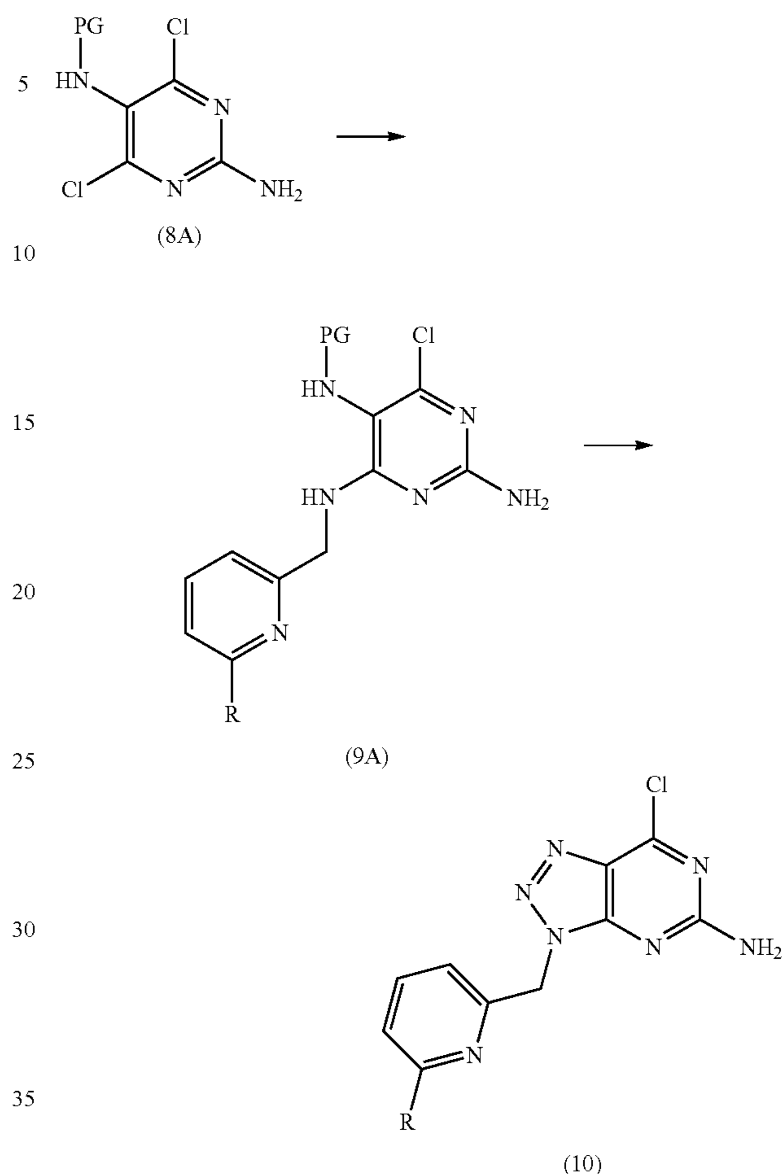
Reaction Scheme 2A:
