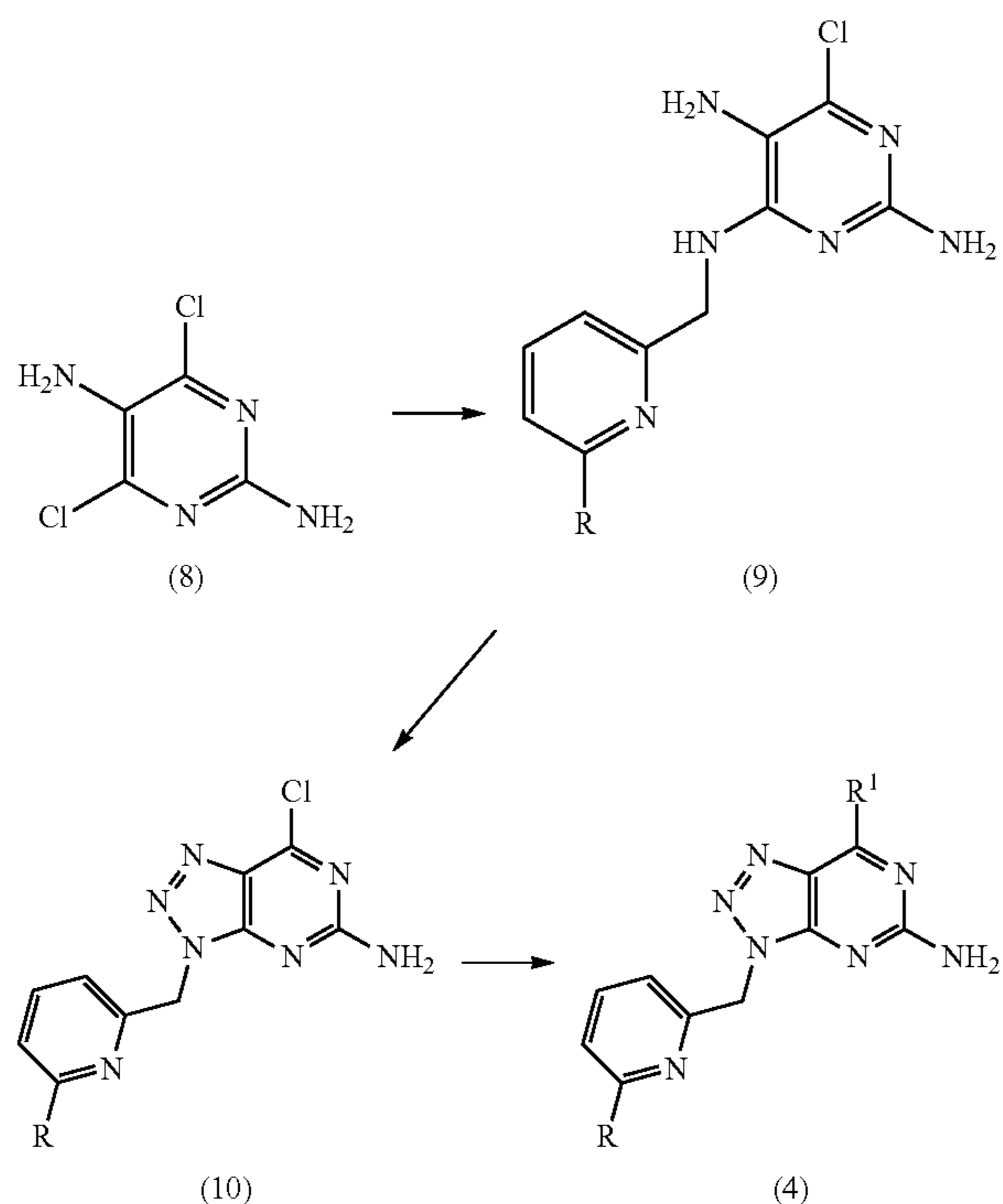
Reaction Scheme 2
