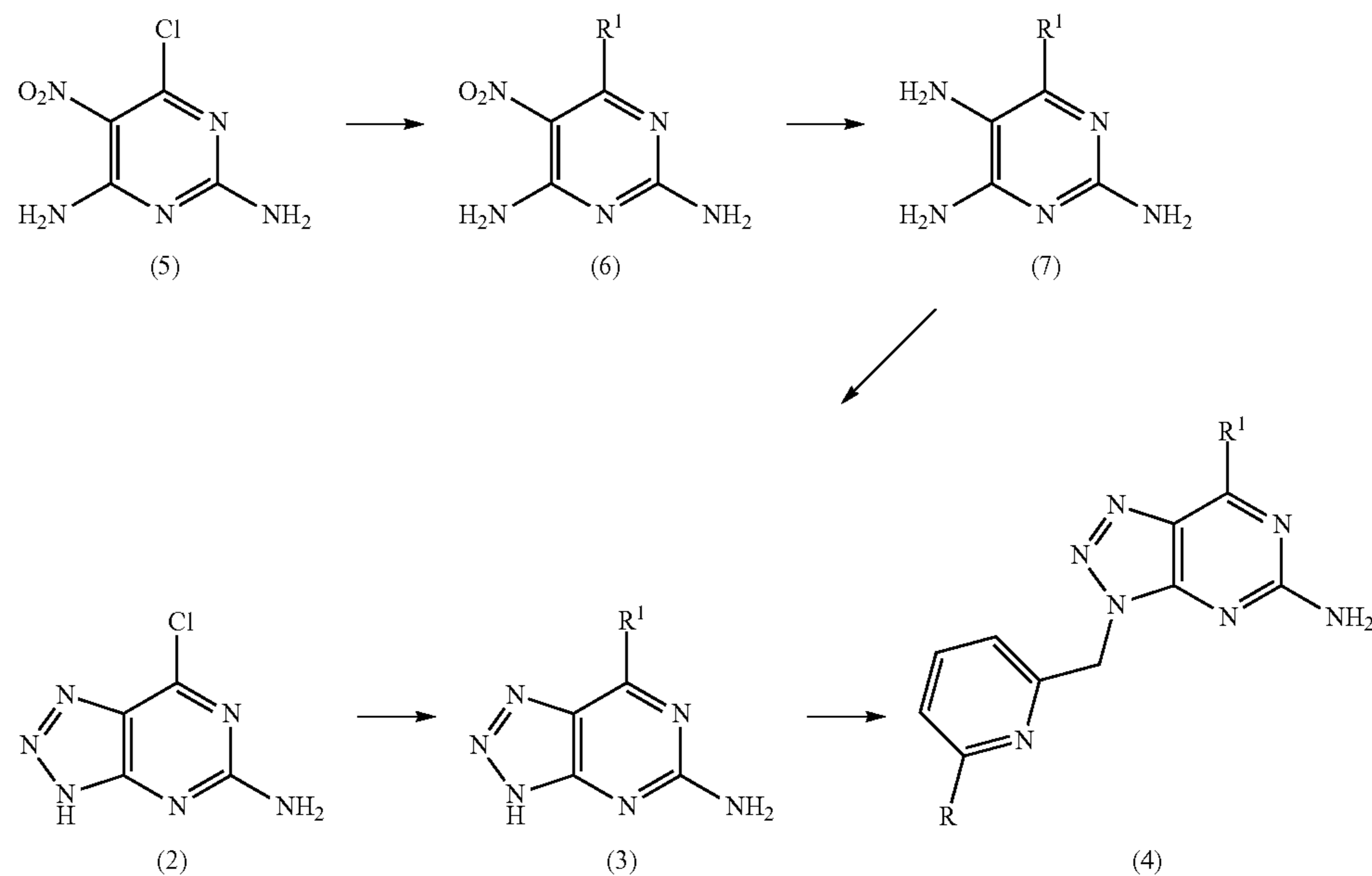
Reaction Scheme 1
