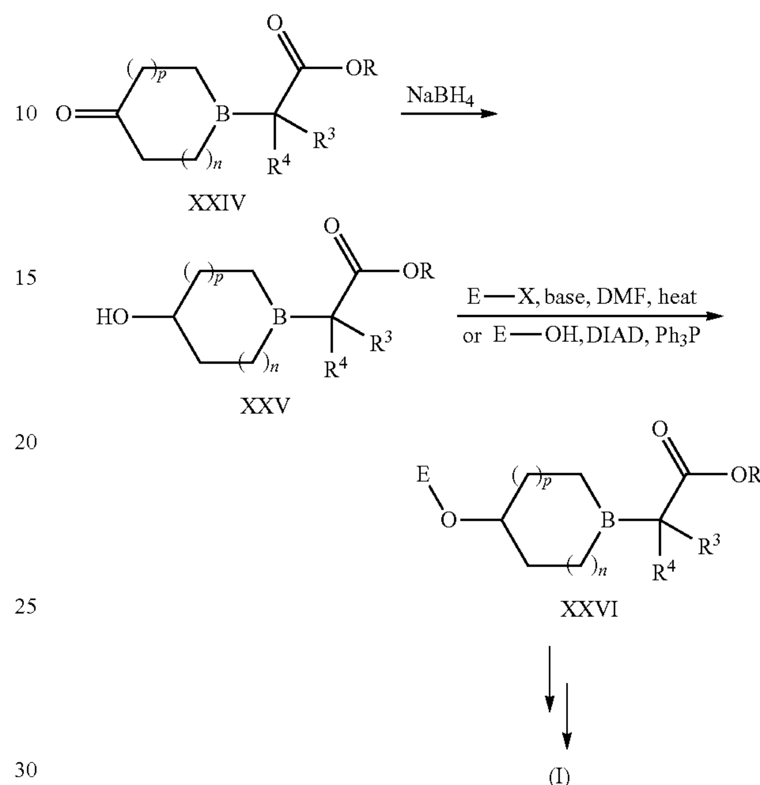
Scheme 6
