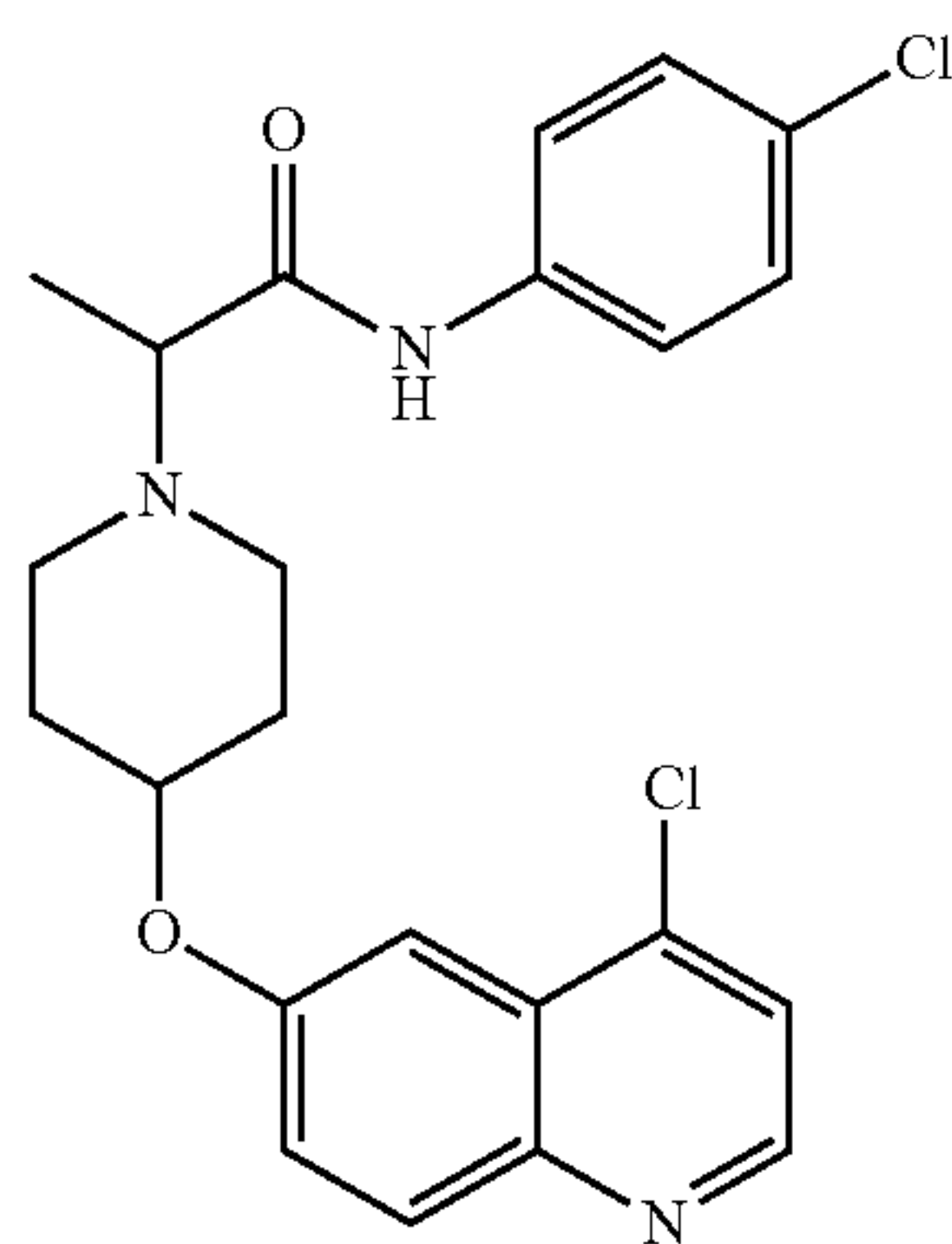
Intermediate 91A
