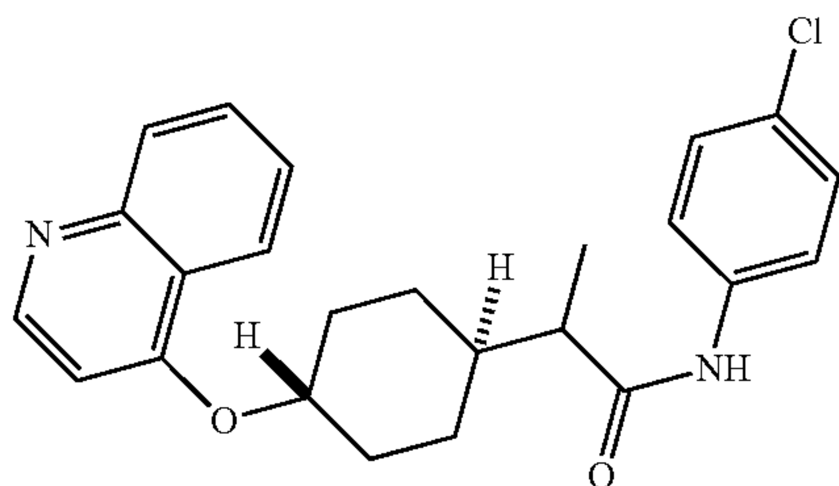
Intermediate 27A
