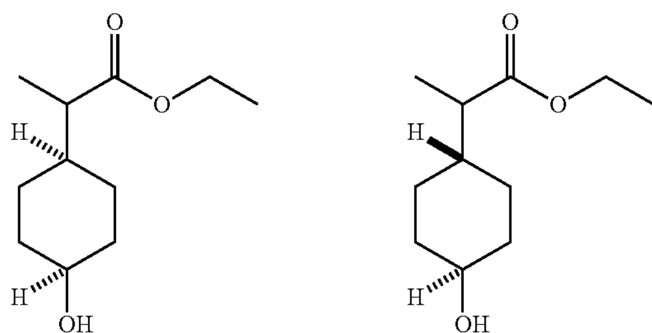
Intermediates 153A and 153B
