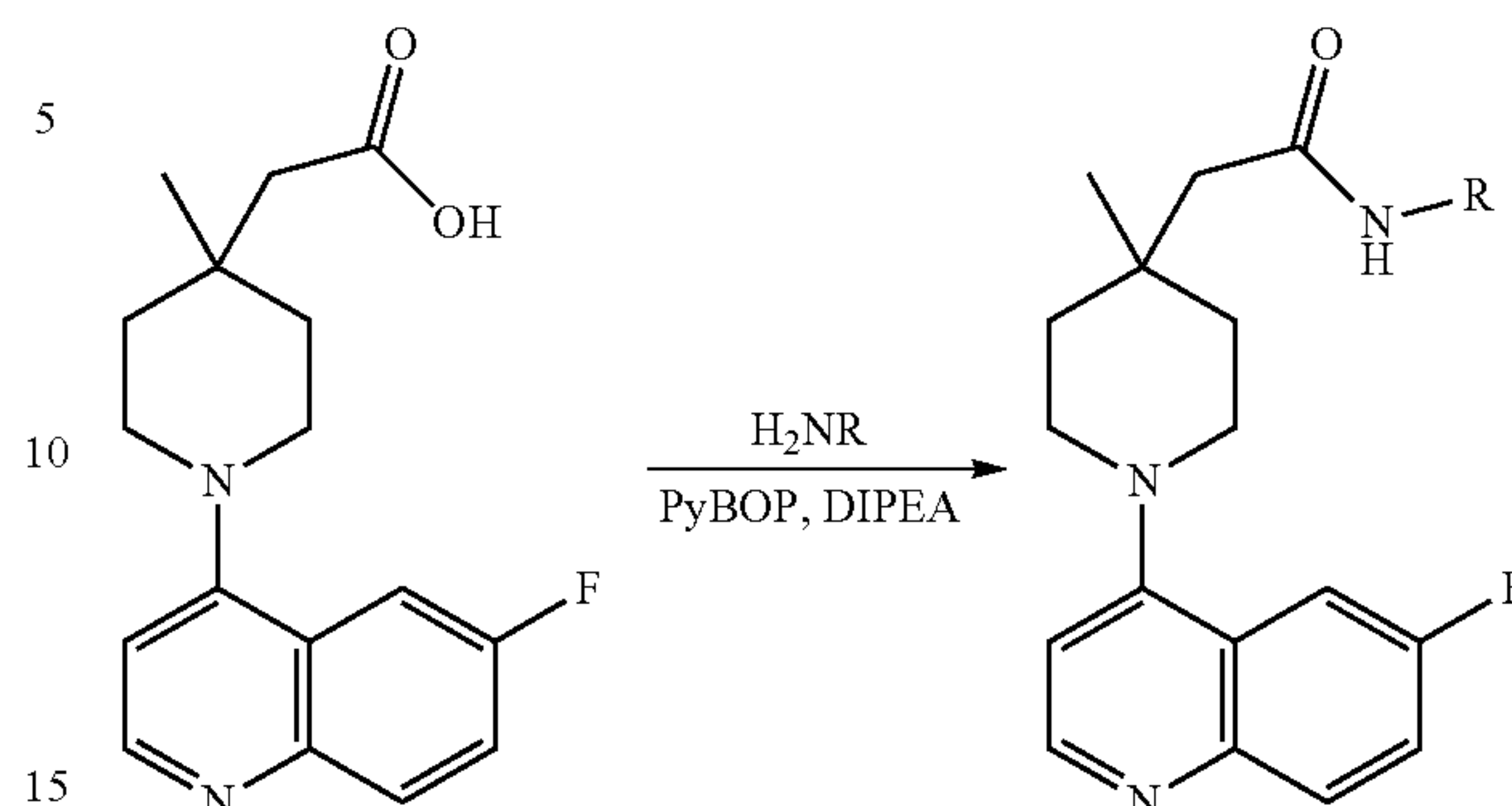
Scheme 4
