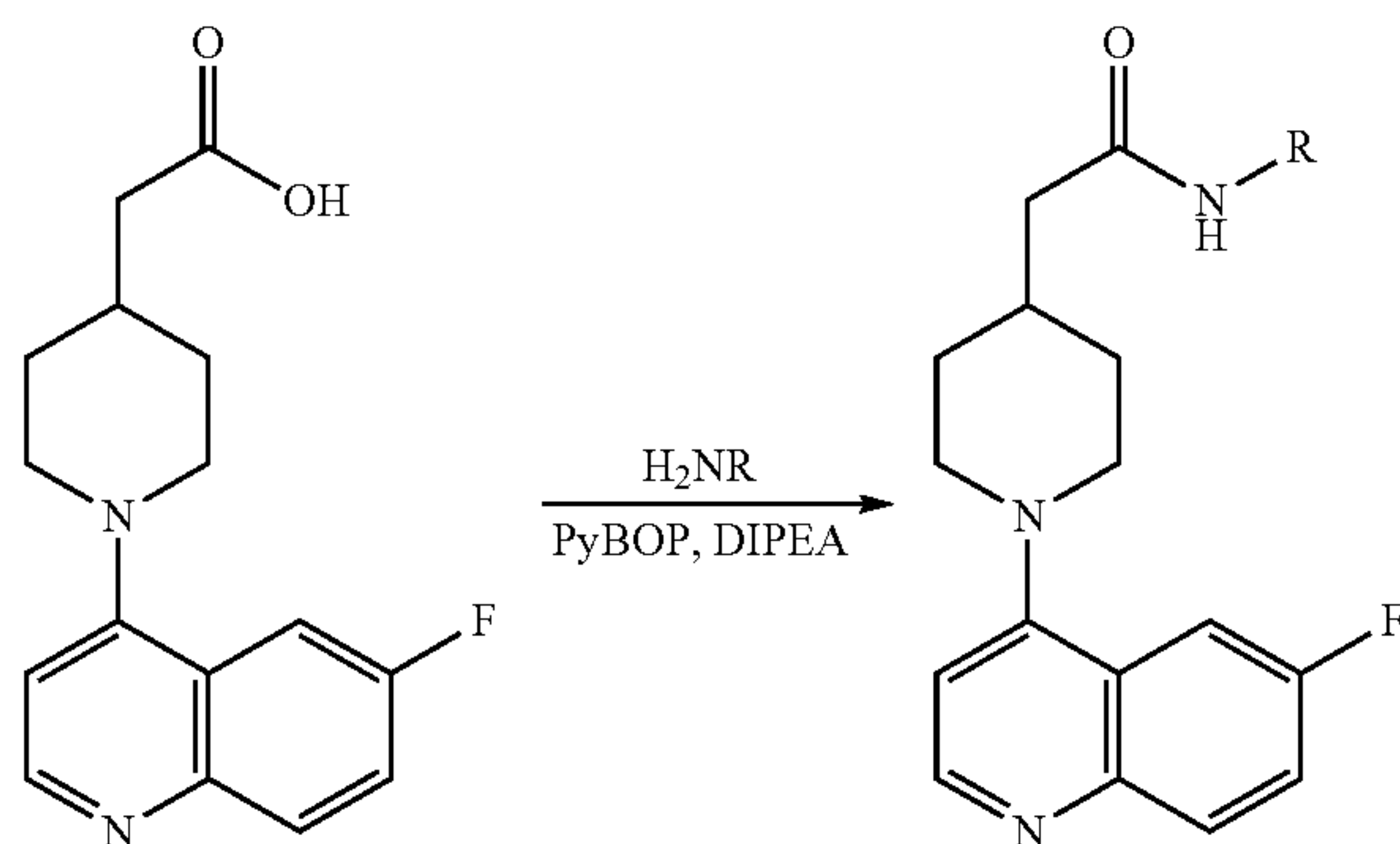
Scheme 3
