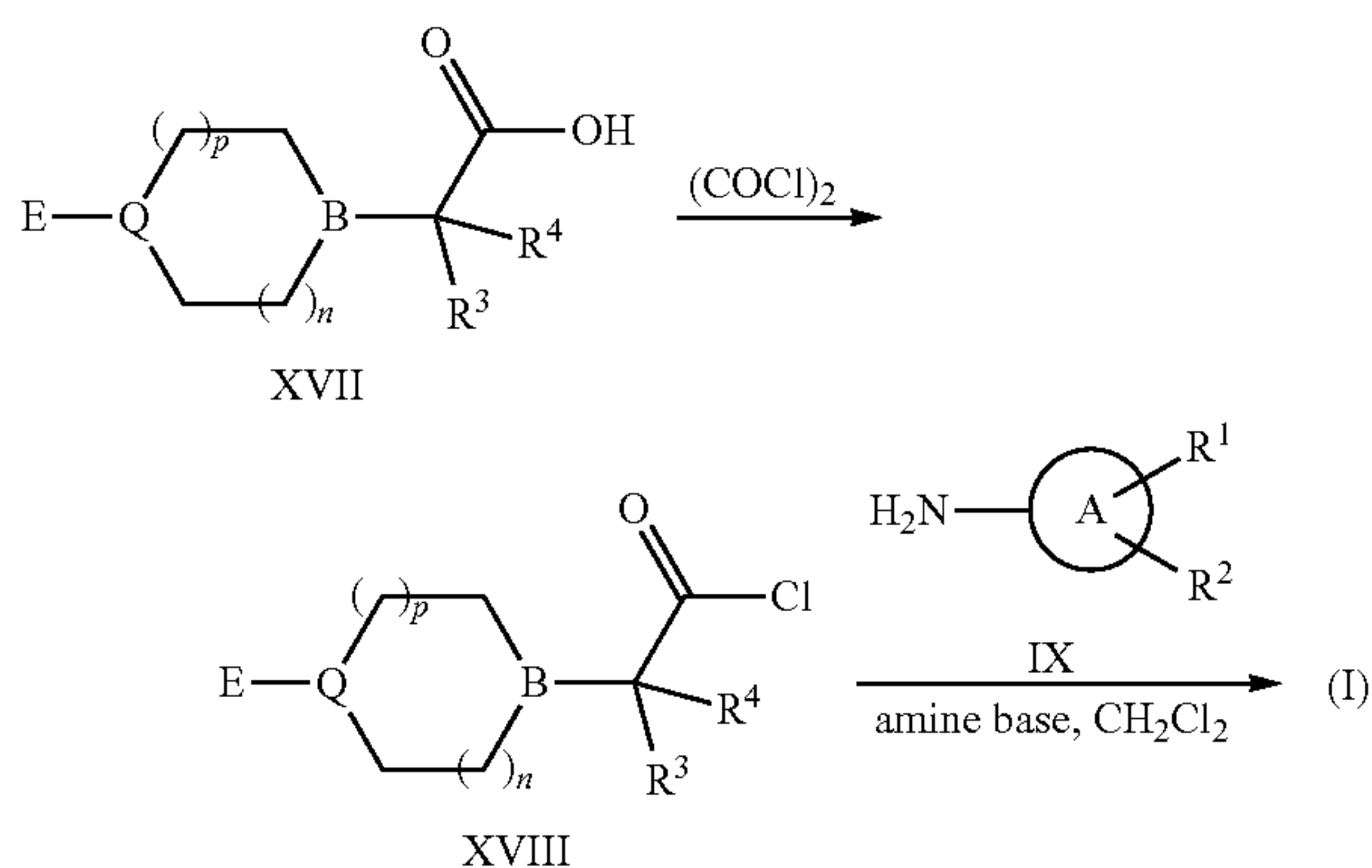
Scheme 4
