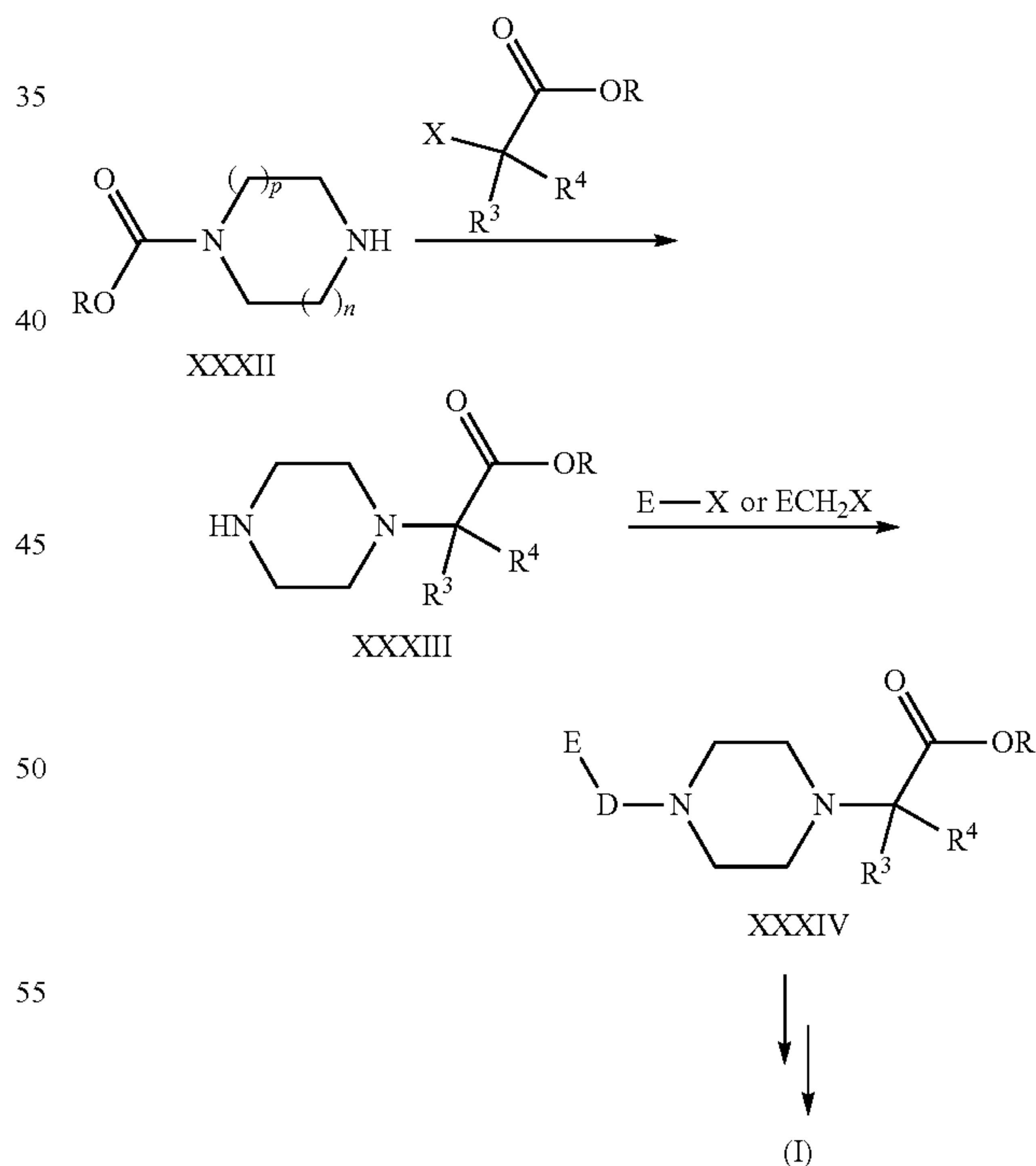
Scheme 10
