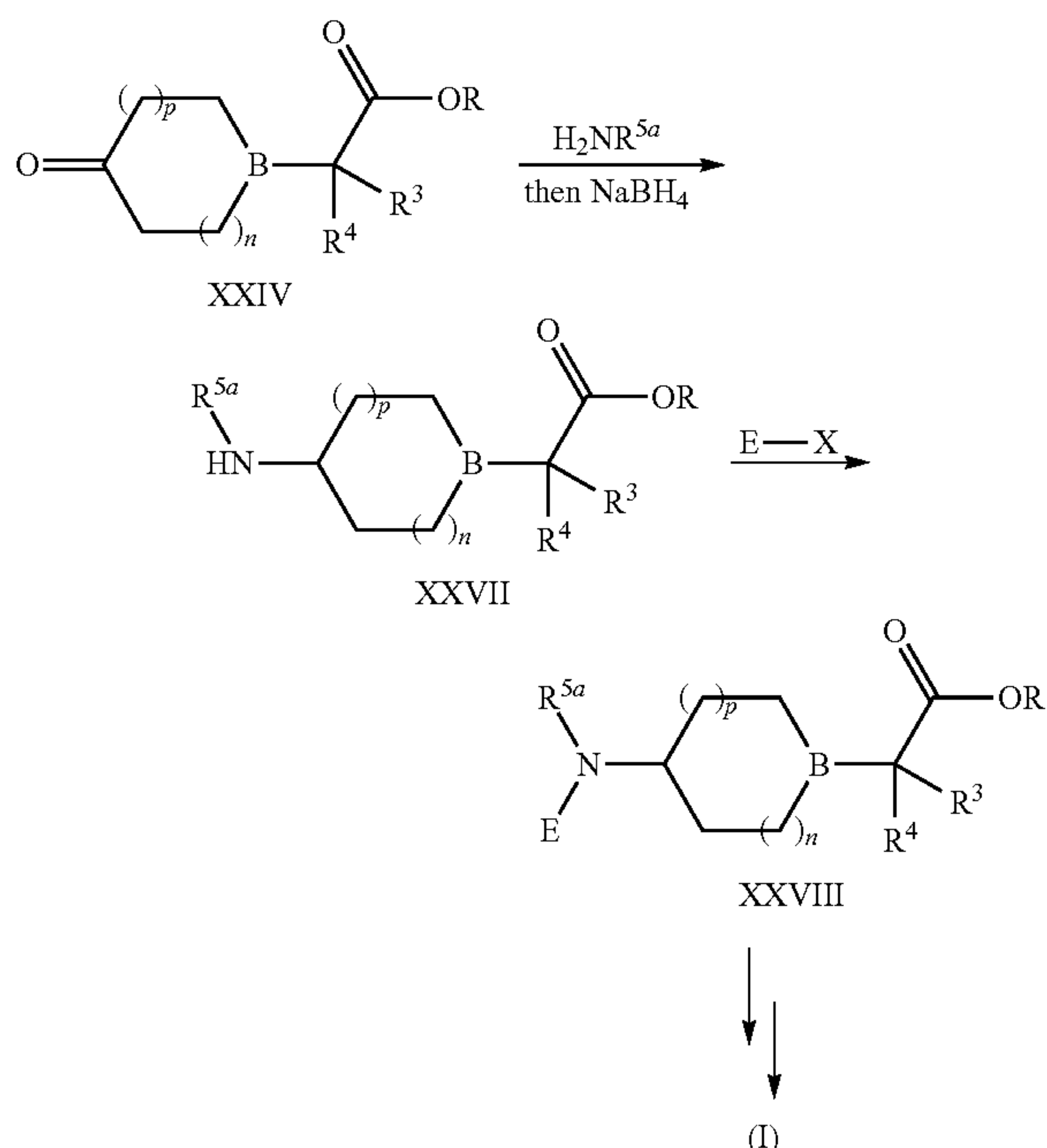
Scheme 7
