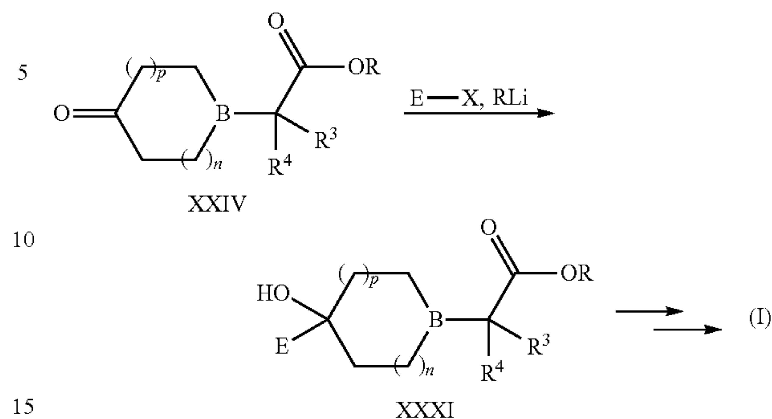
Scheme 9
