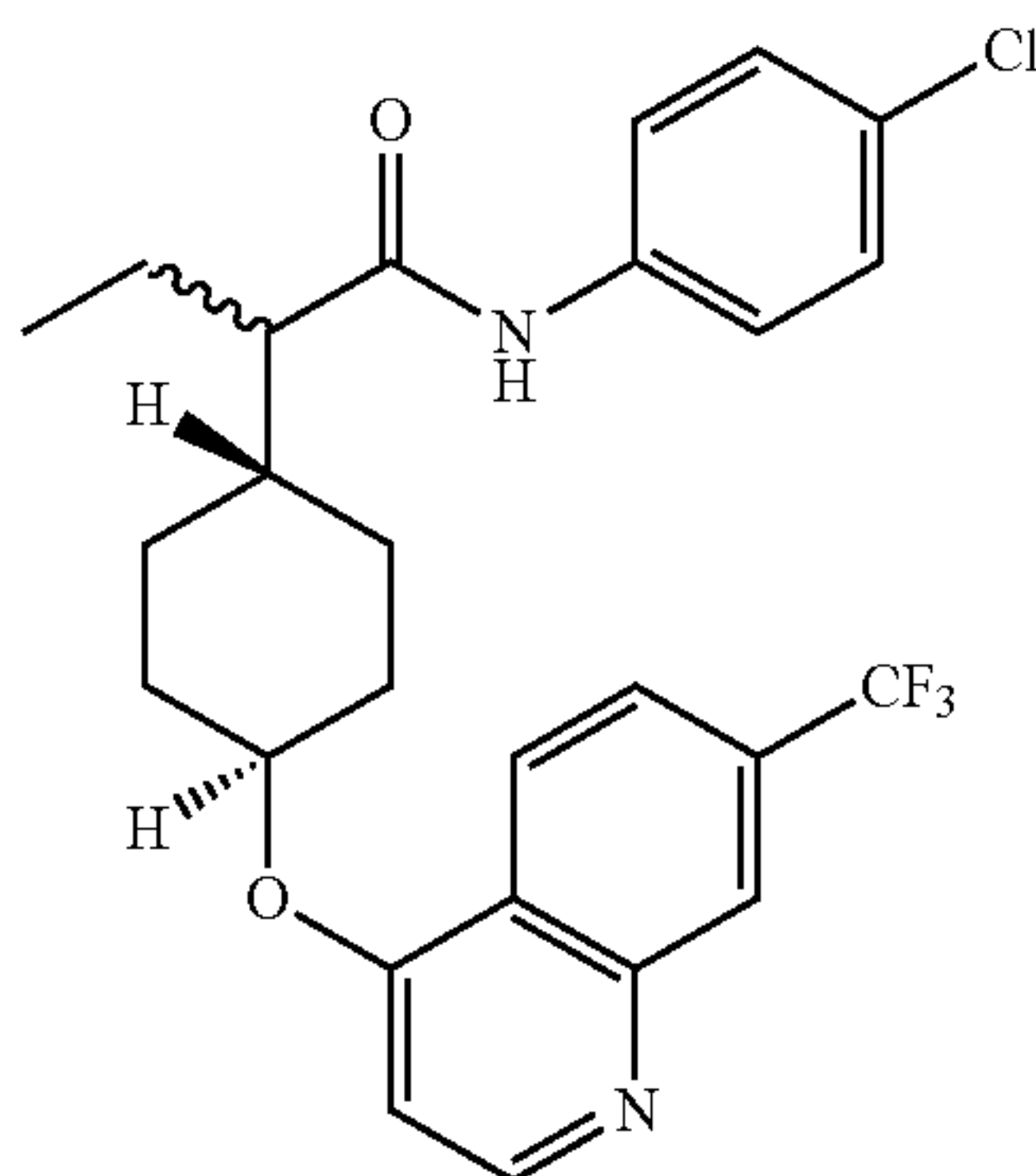
Intermediate 83A
