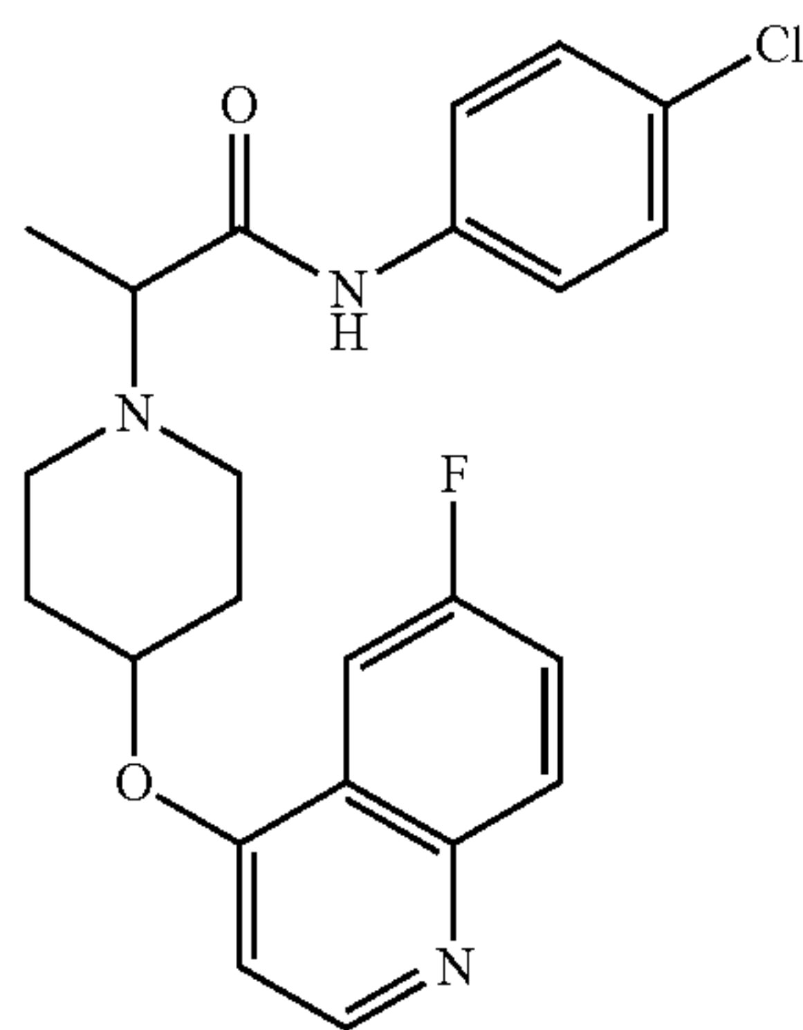
Intermediate 96A
