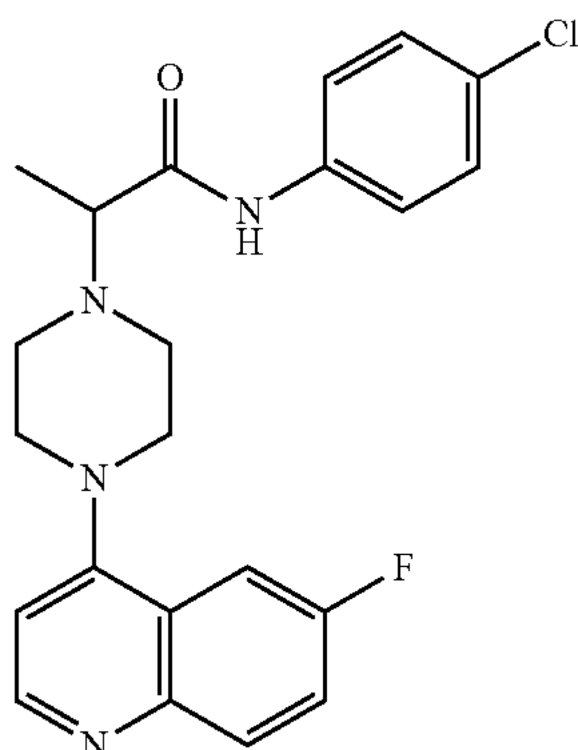
Intermediate 126A
