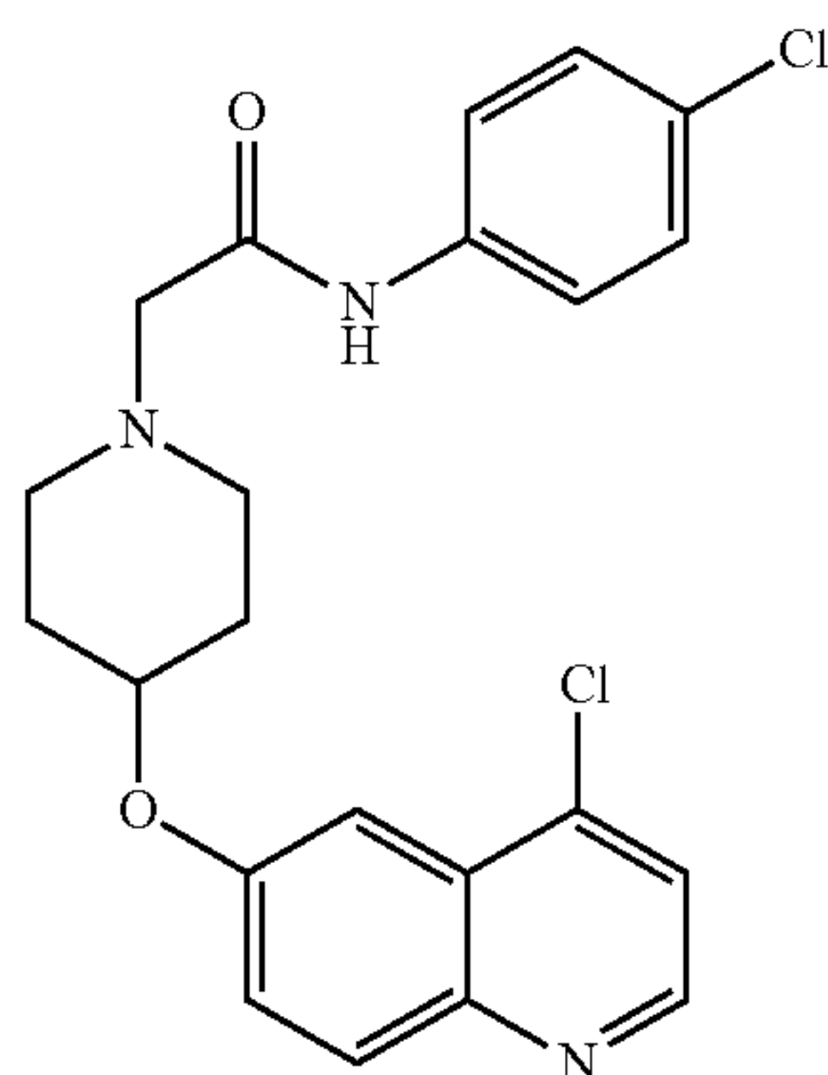
Intermediate 90A.
