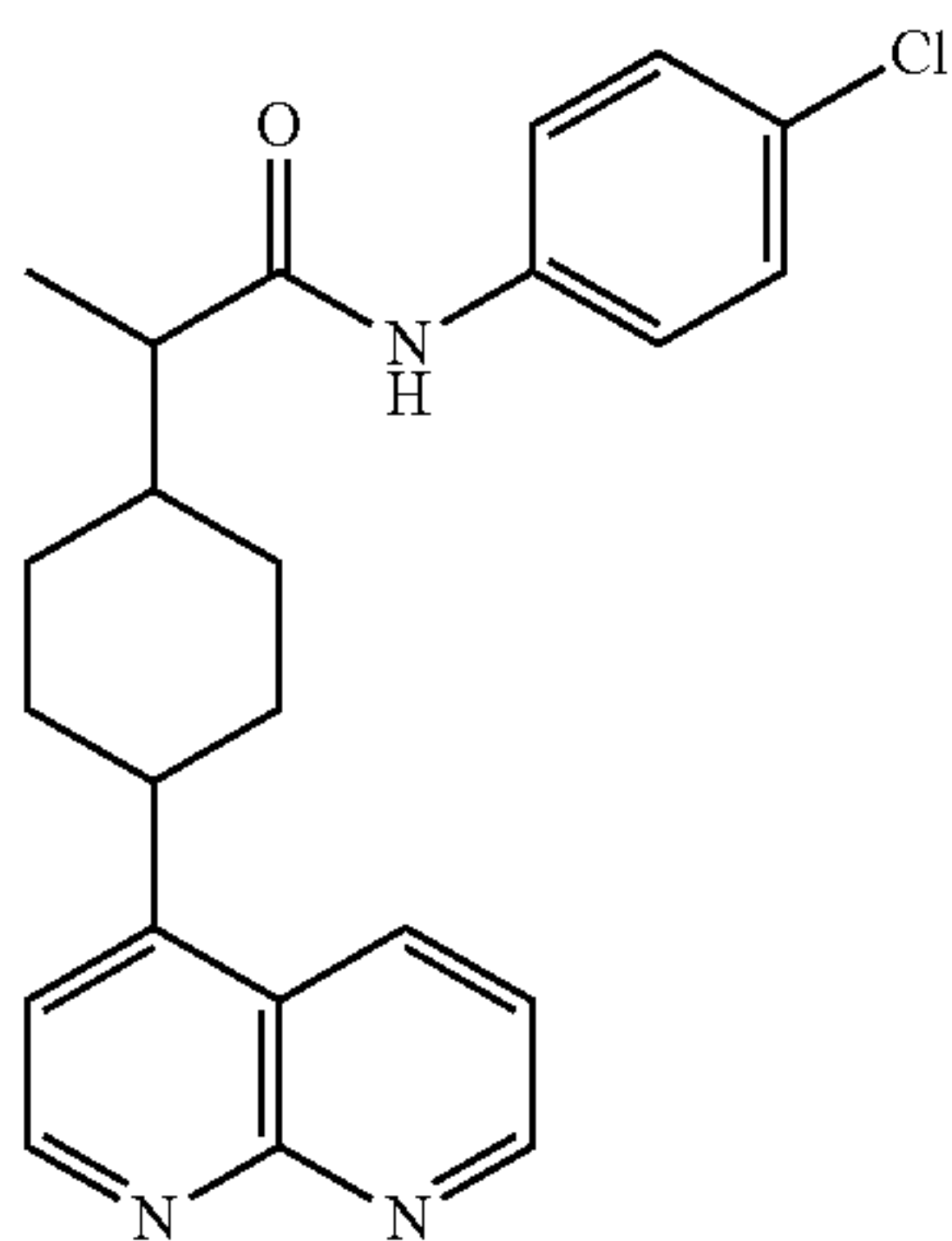
Intermediate 147A
