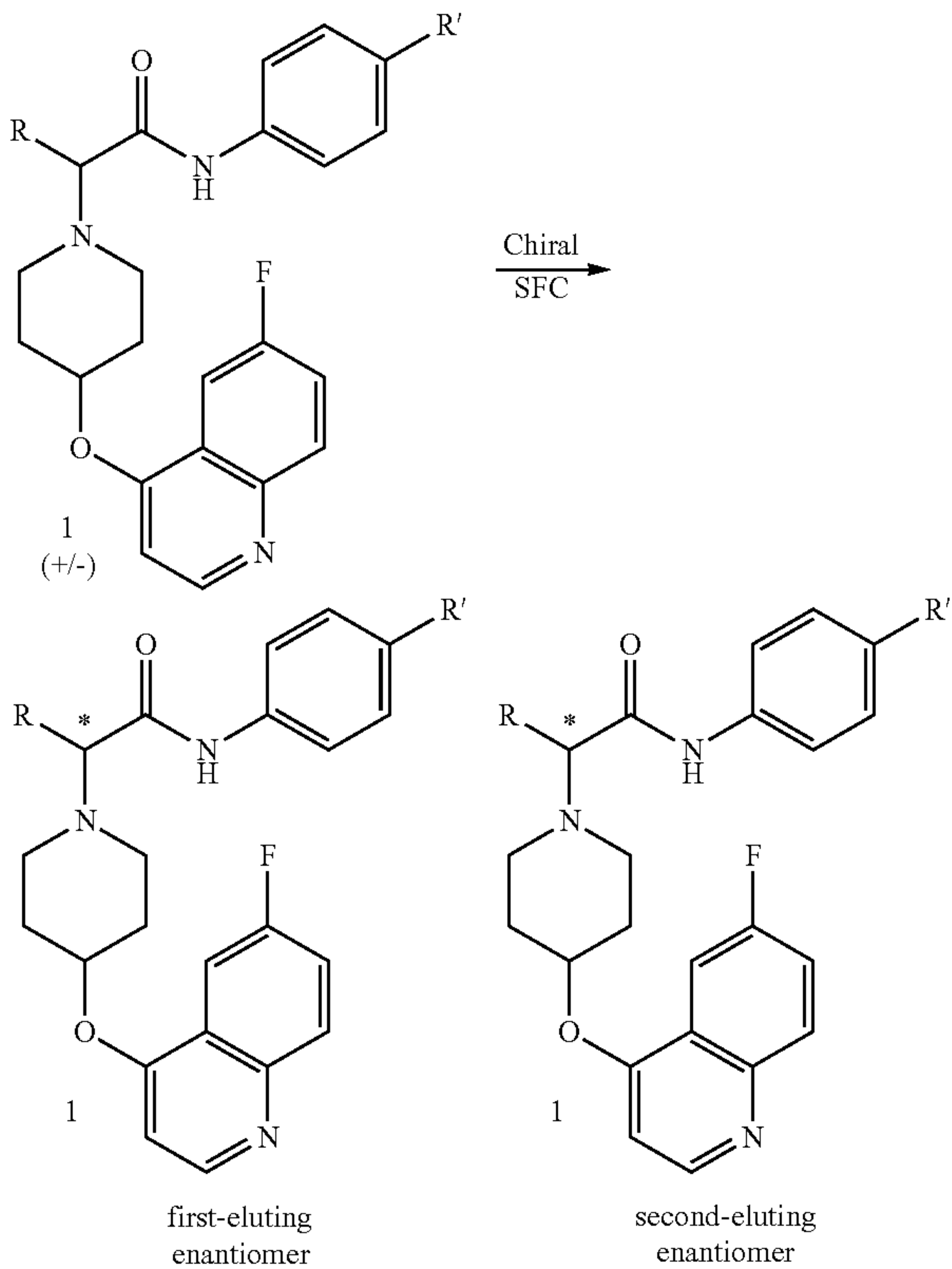
Scheme 2
