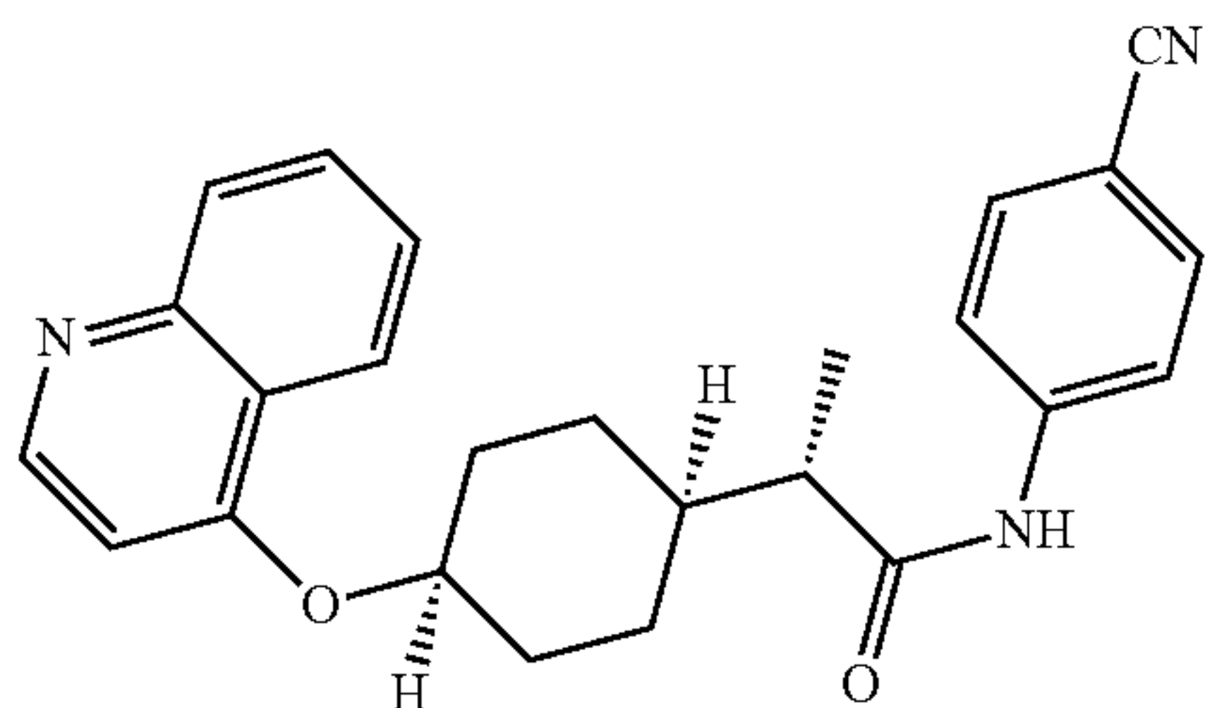
Intermediate 38A
