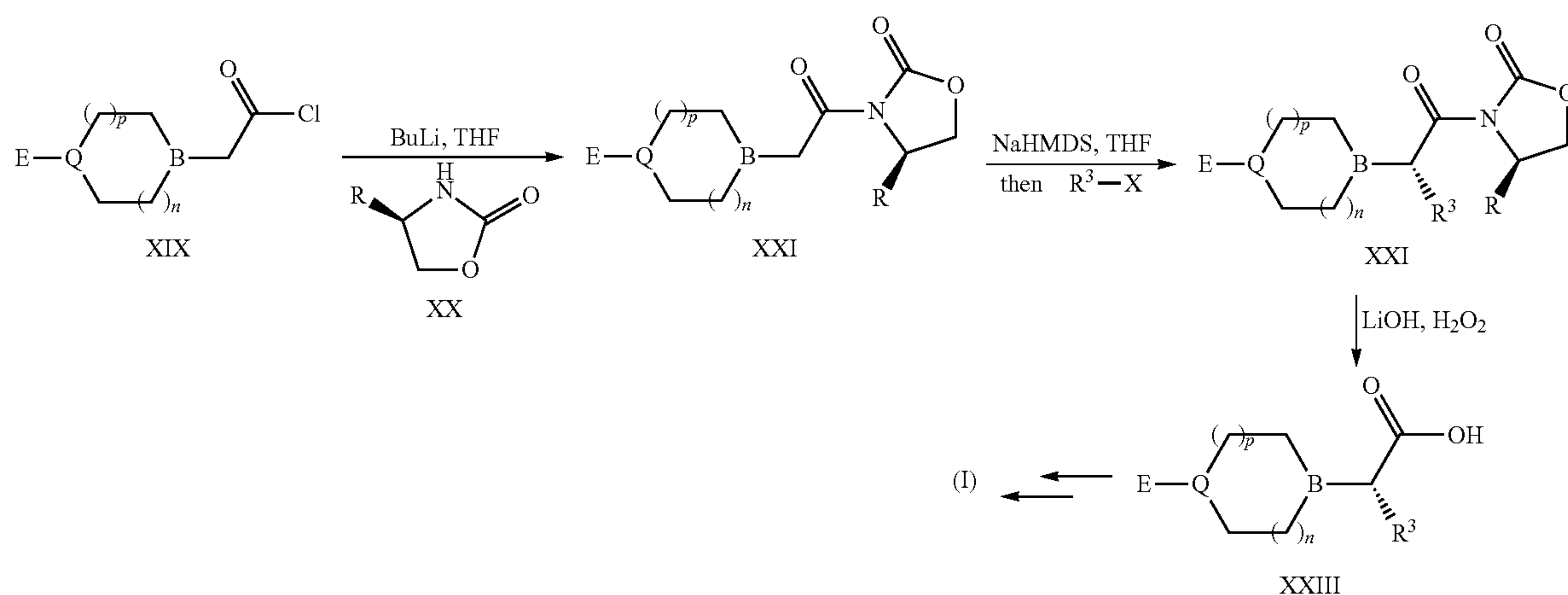
Scheme 5
