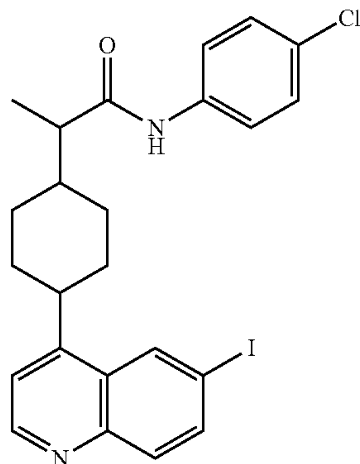
Intermediate 151A
