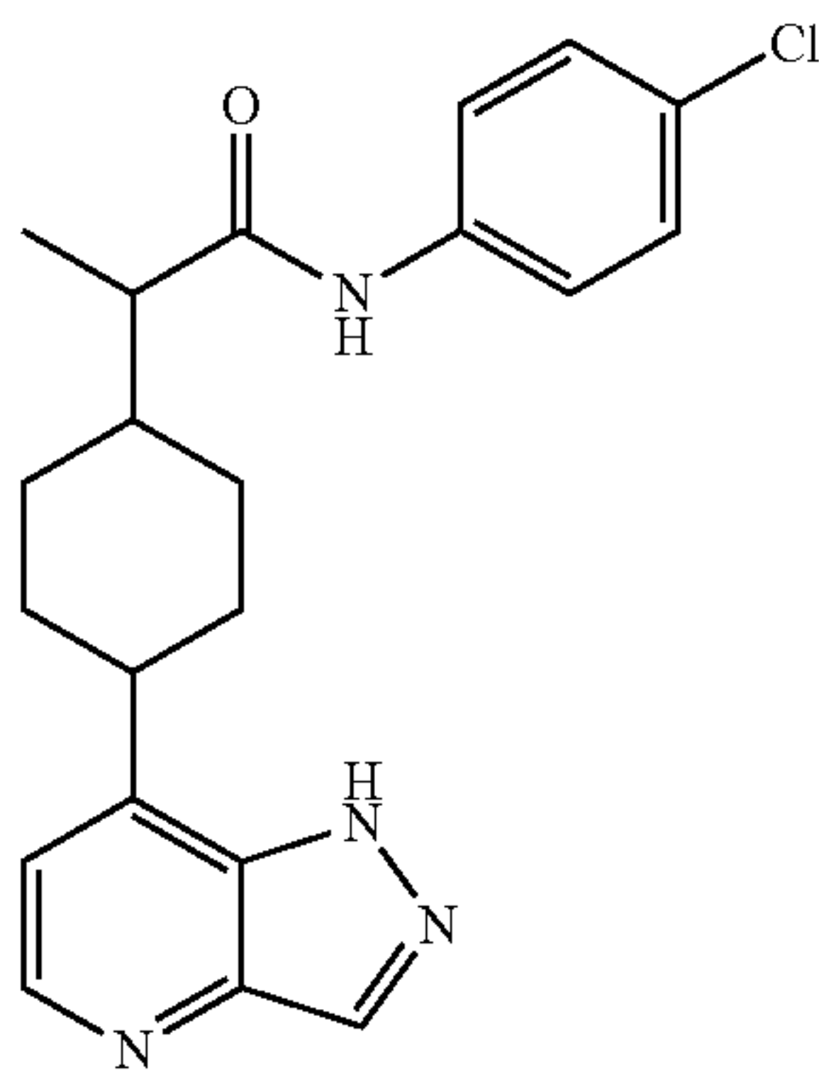
Intermediate 149A
