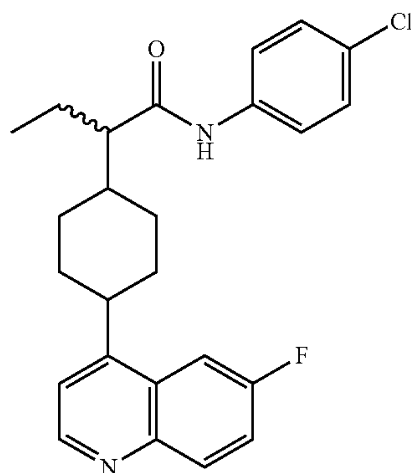
Intermediate 154A
