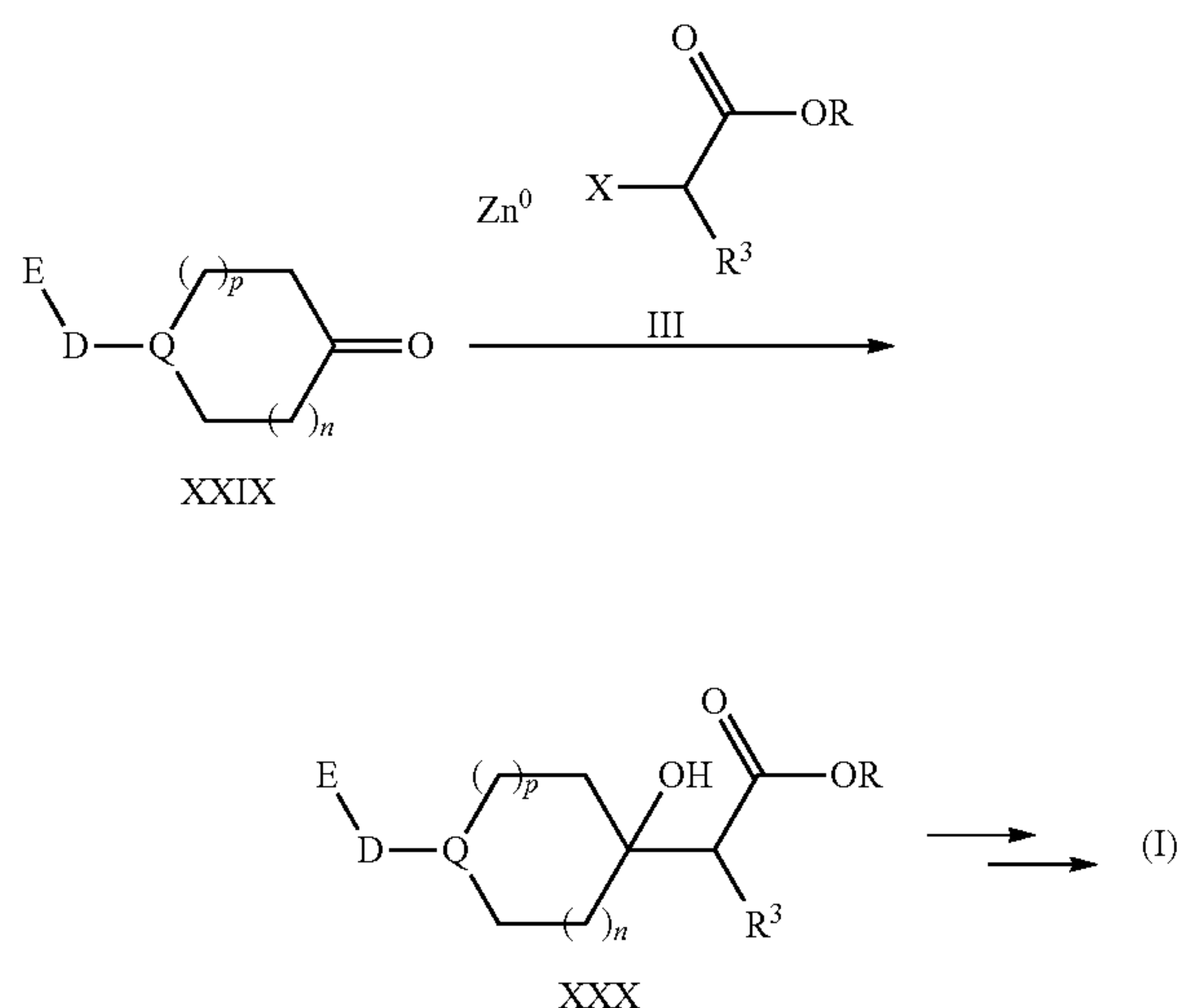
Scheme 8
