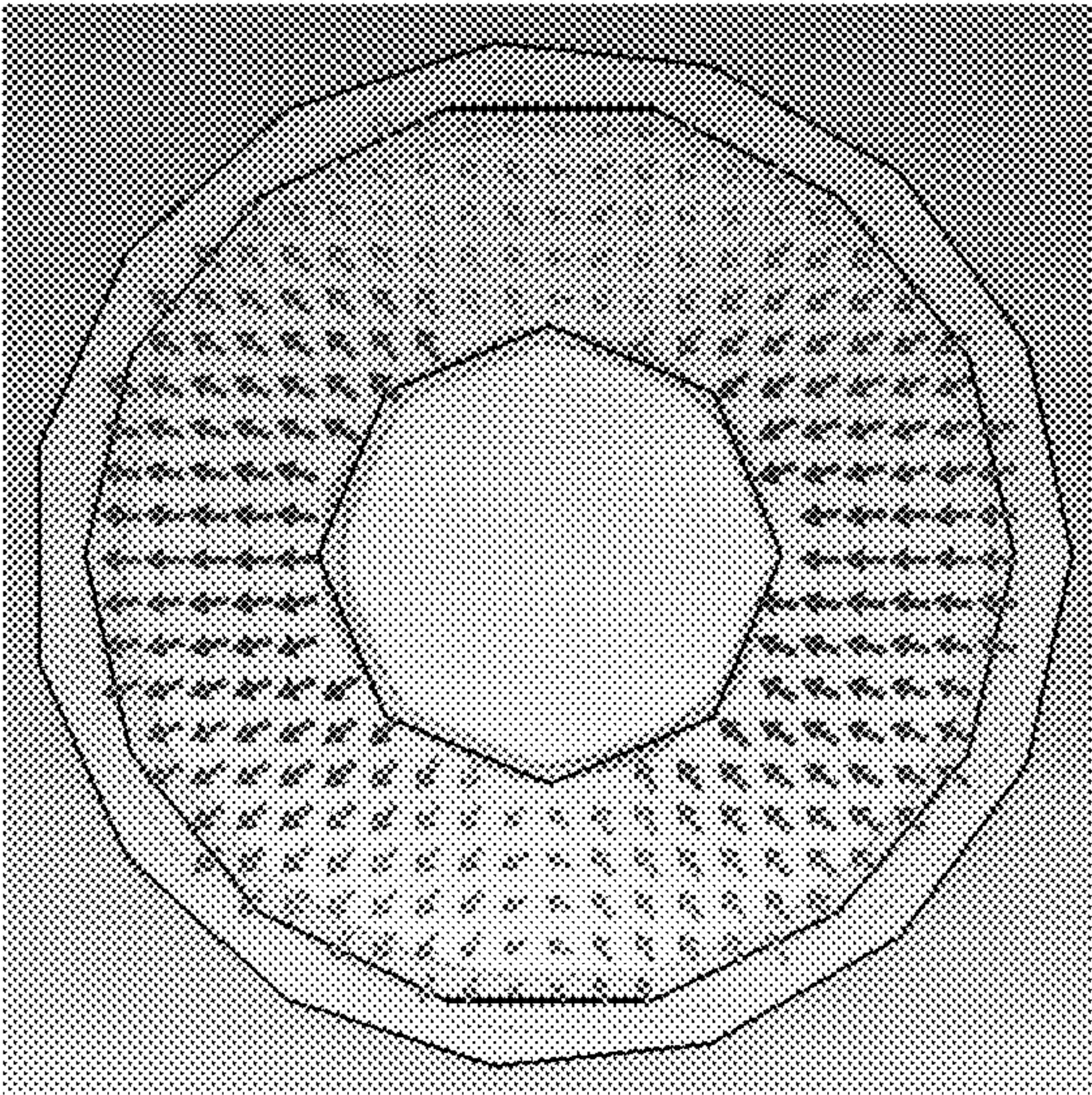
HE11, Vertical Polarization
