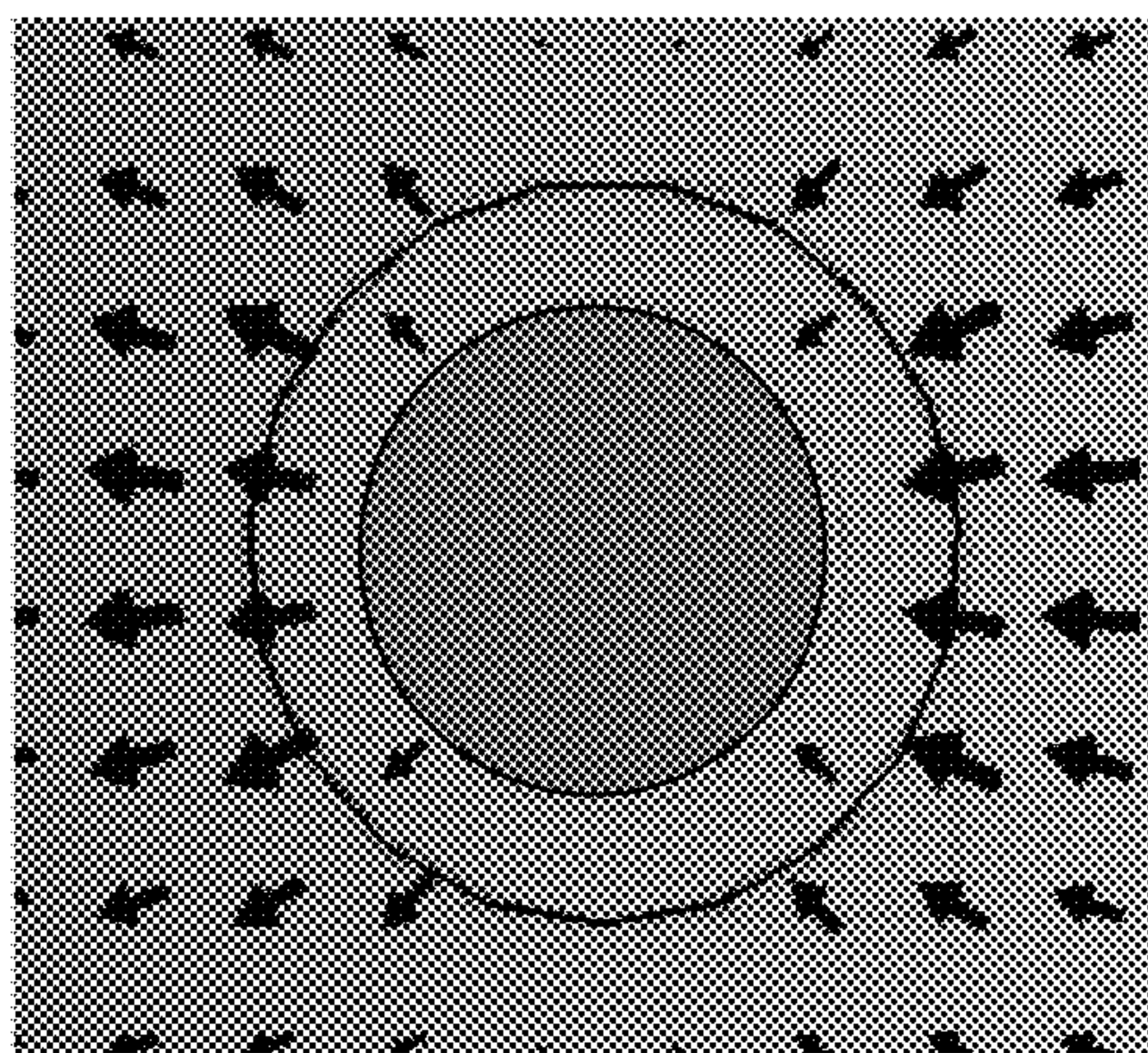
Hybrid mode (HE11) 2168
