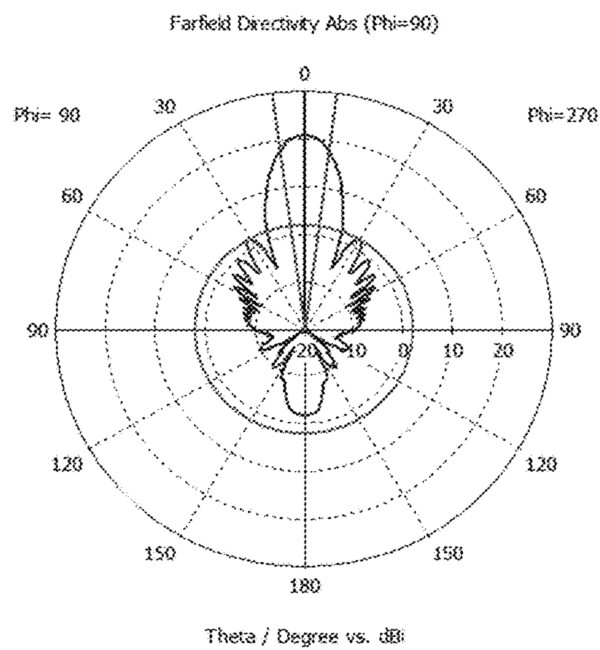
Antenna Gain Pattern
