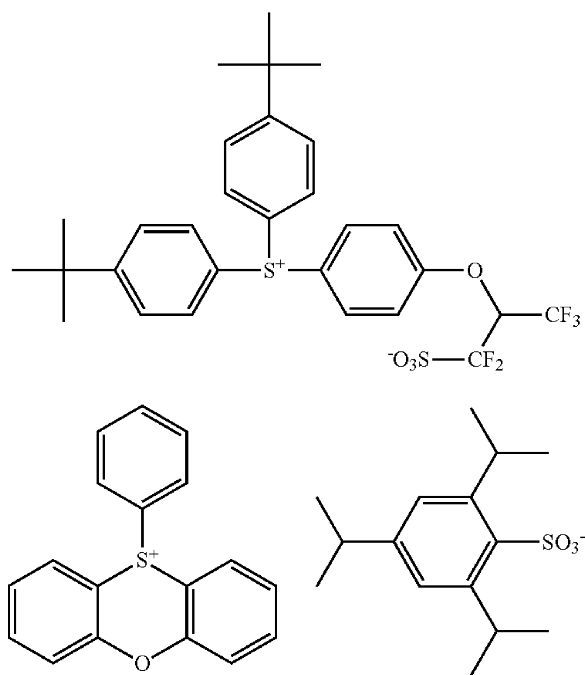
Comparative Quenchers 1 to 6:
