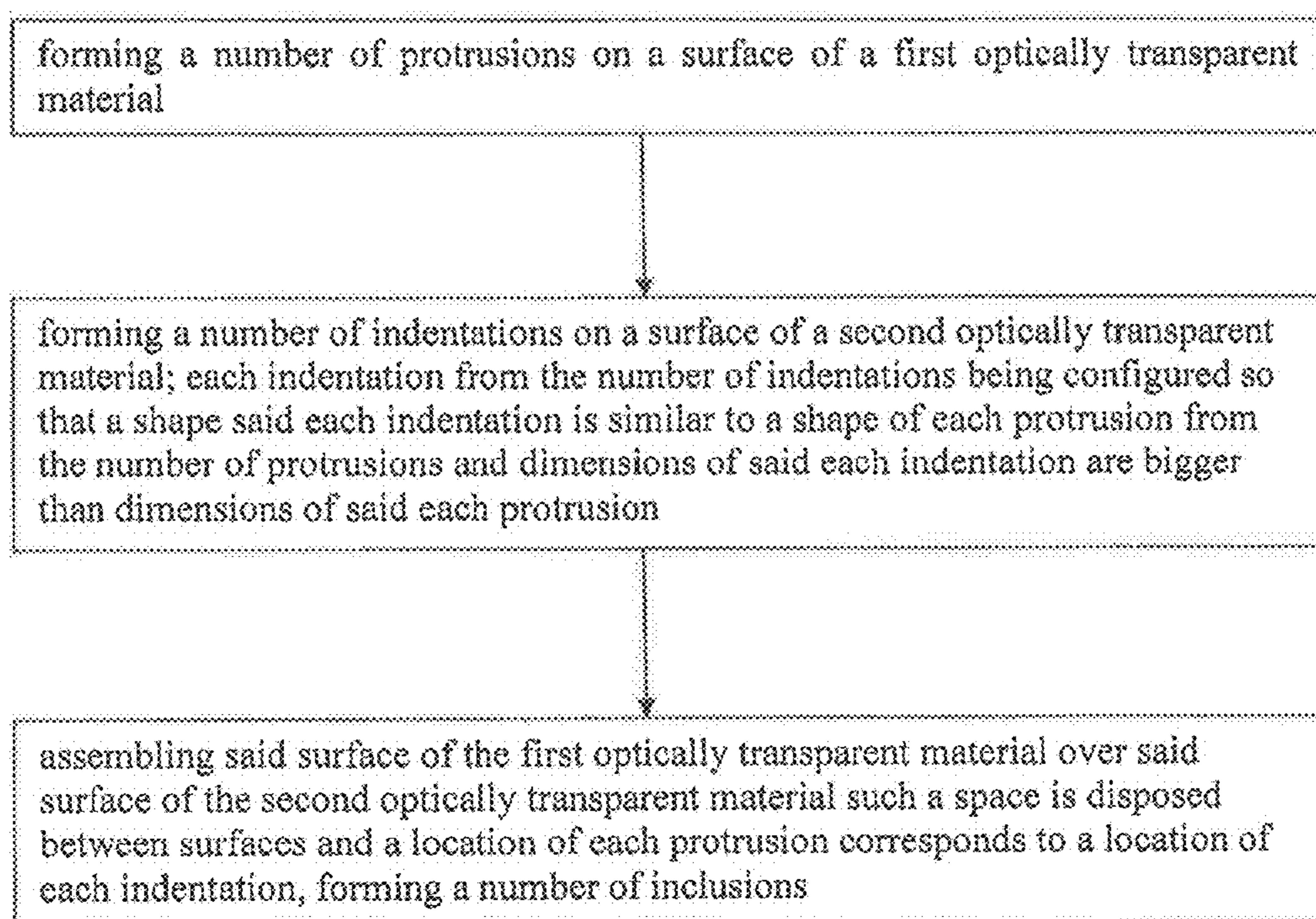
Figure 11(c). Fabrication method
