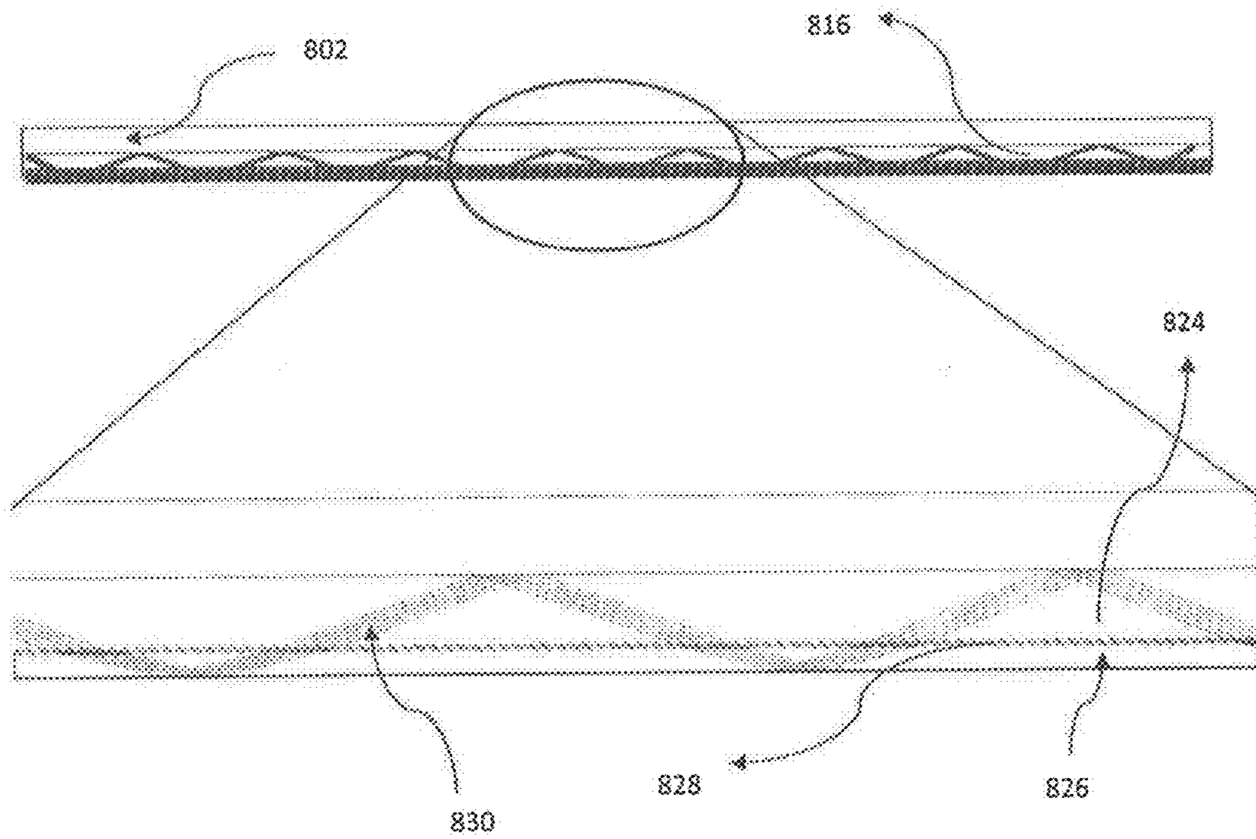
Figure 8(f) Ray traces of a prismatic planar core shown in Figure 8(e)
