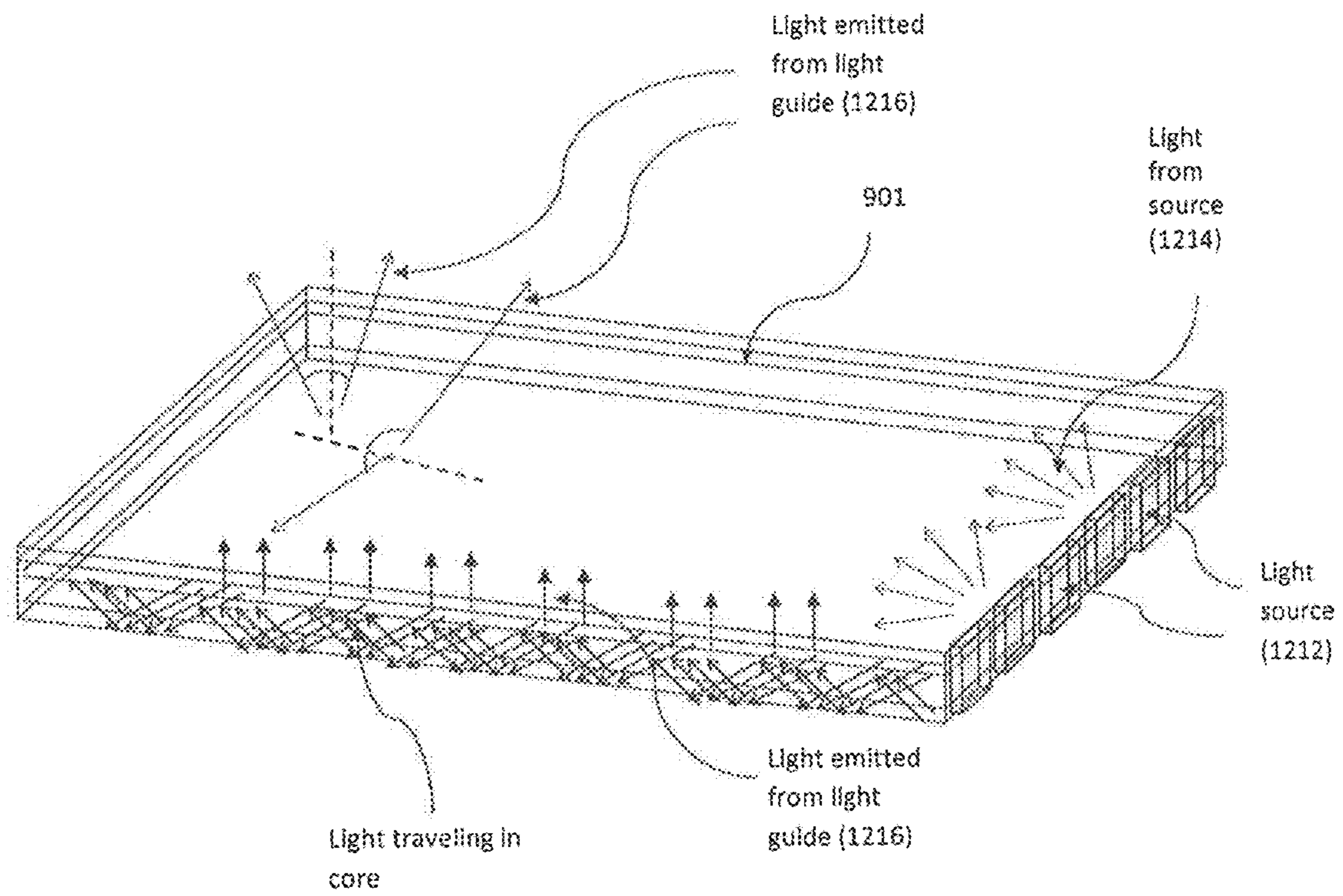
Figure 12(b). Use of light guide apparatus as described in this invention as a lighting device
