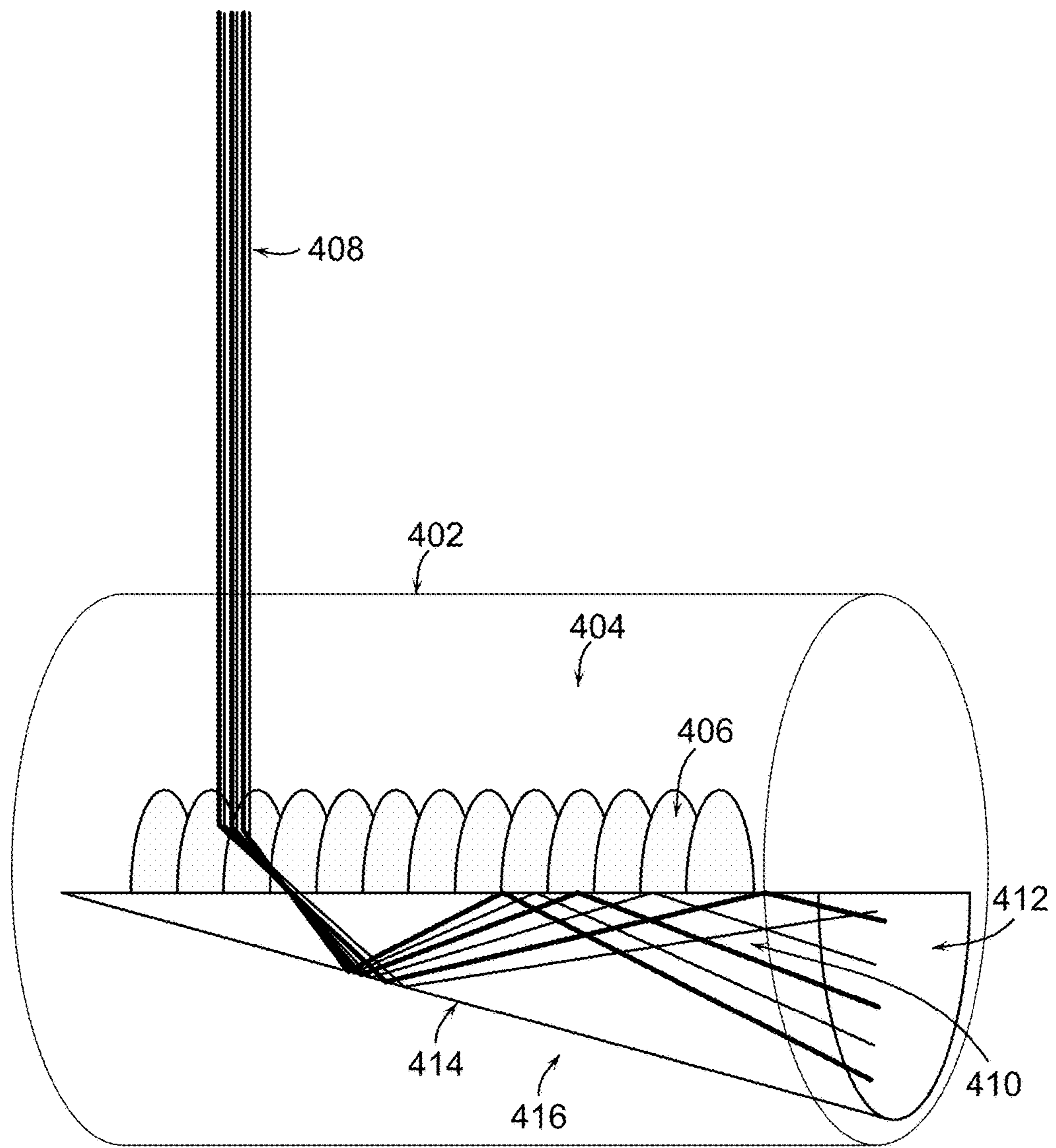
Figure 4(a) Ray traces of light in the cladding and core
