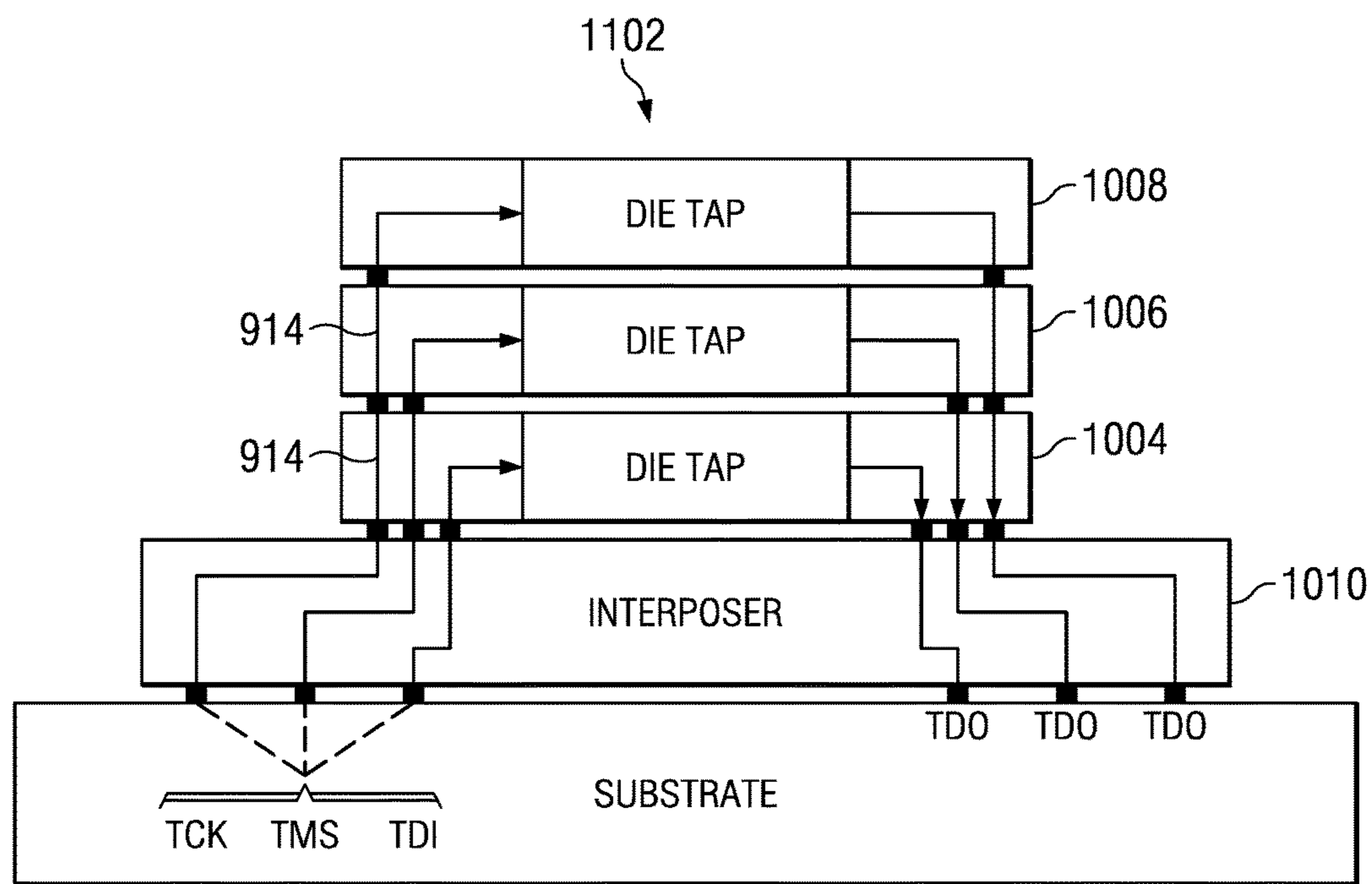
FIG. 11 (PRIOR ART)
