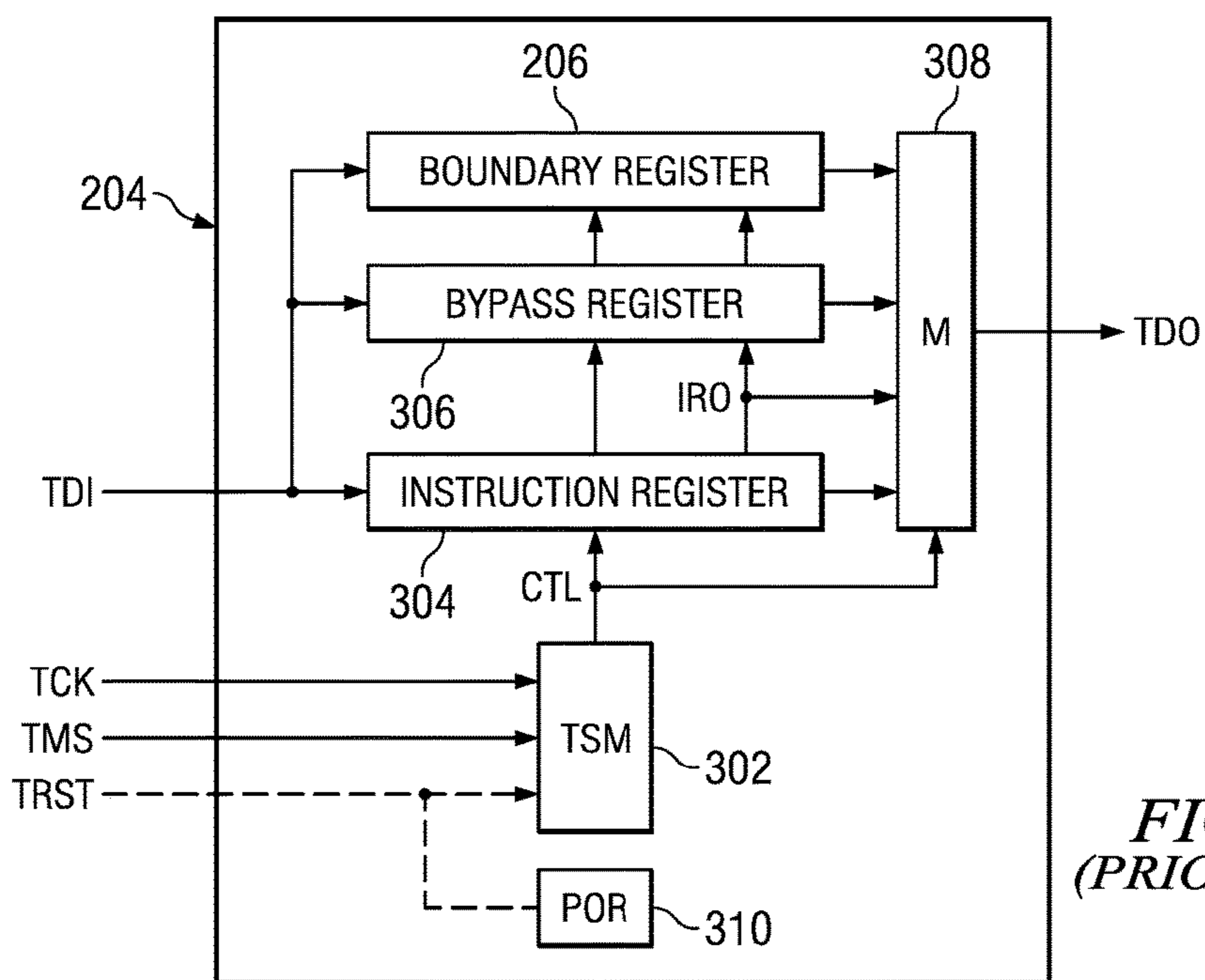
FIG. 4 (PRIOR ART)
