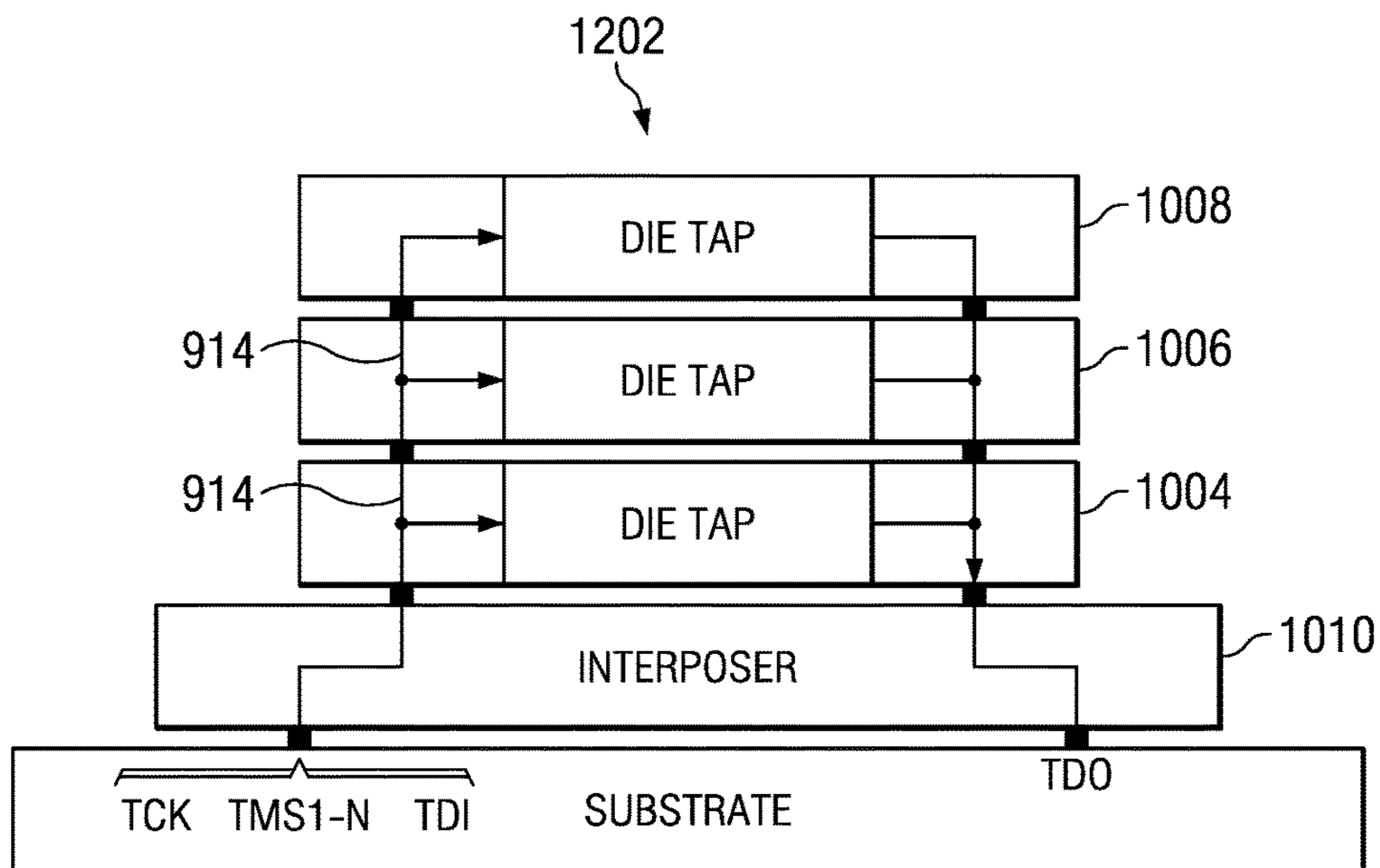
FIG. 12 (PRIOR ART)
