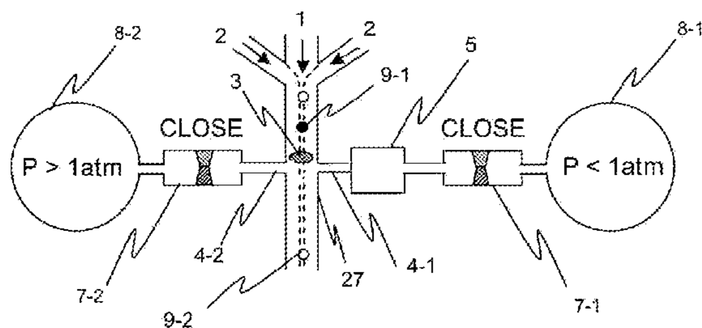
a) Electromagnetic valve off
