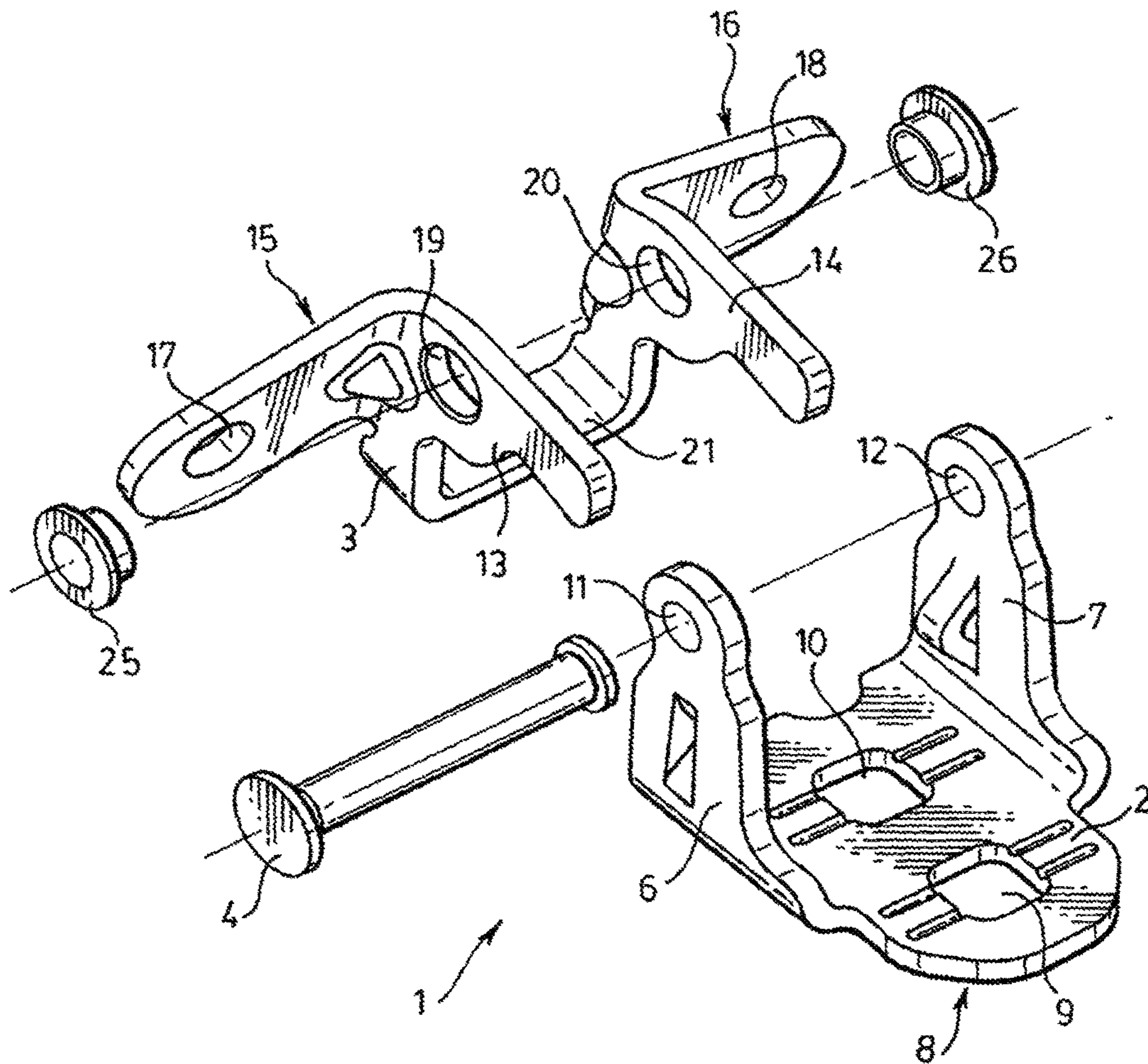
FIG. 1. (PRIOR ART)
