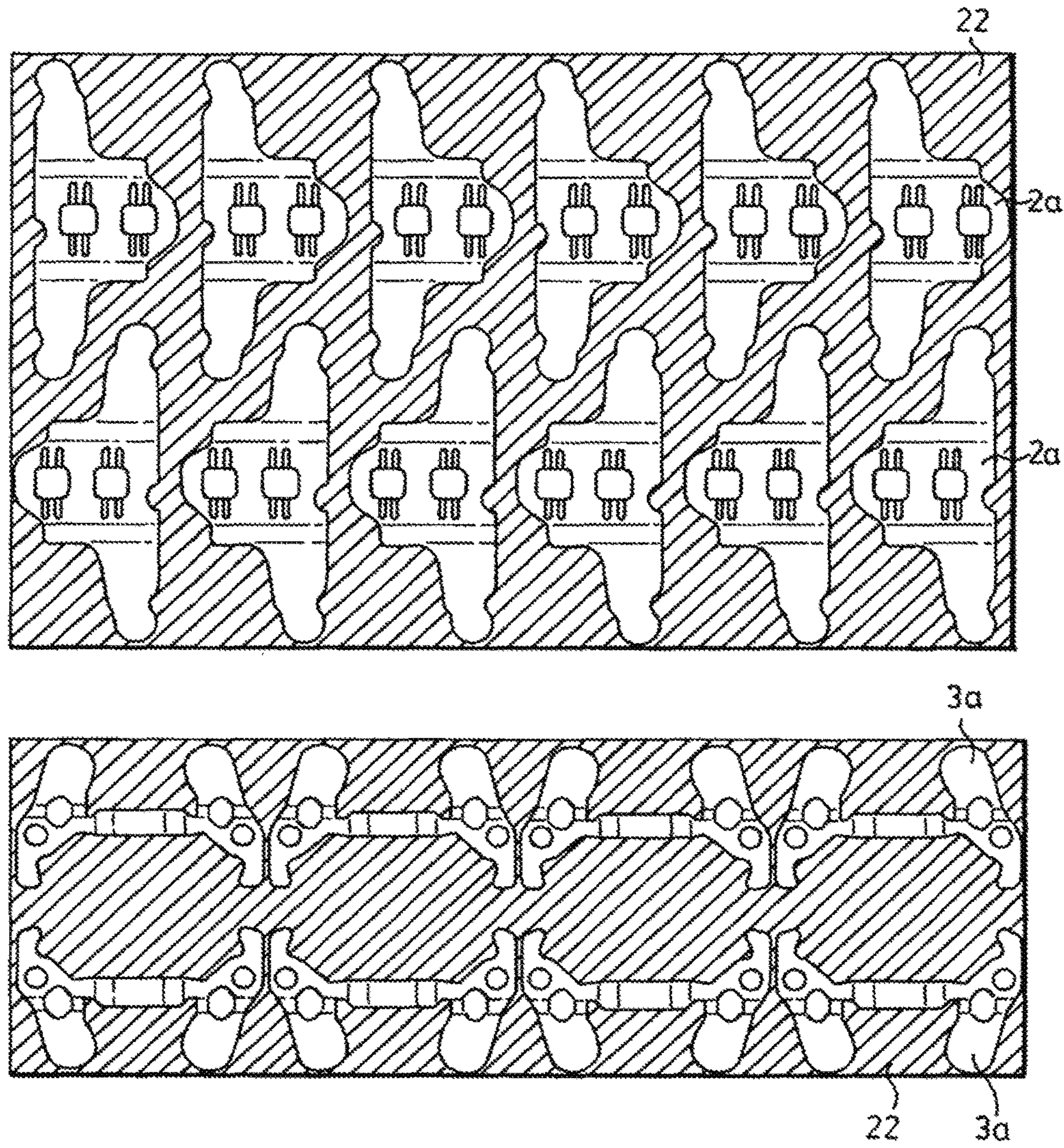
FIG. 2. (PRIOR ART)
