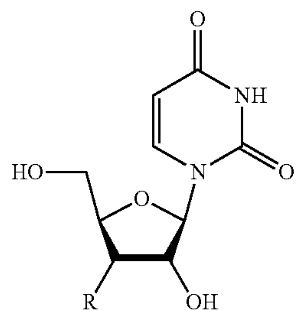
Scheme 9
