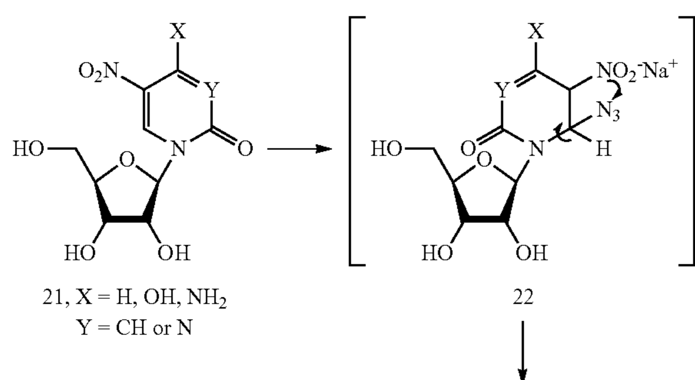
Scheme 4
