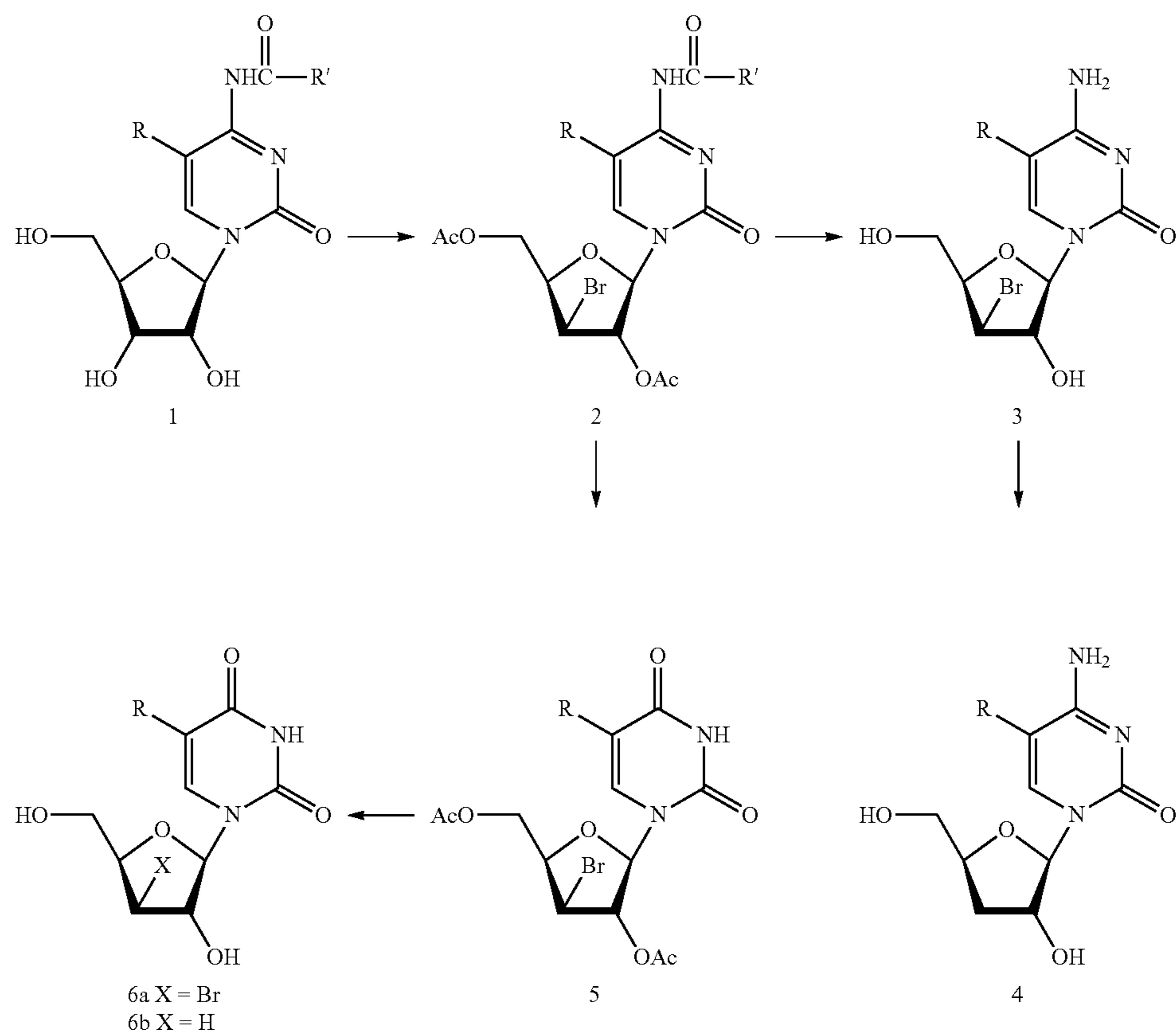
Scheme 1
