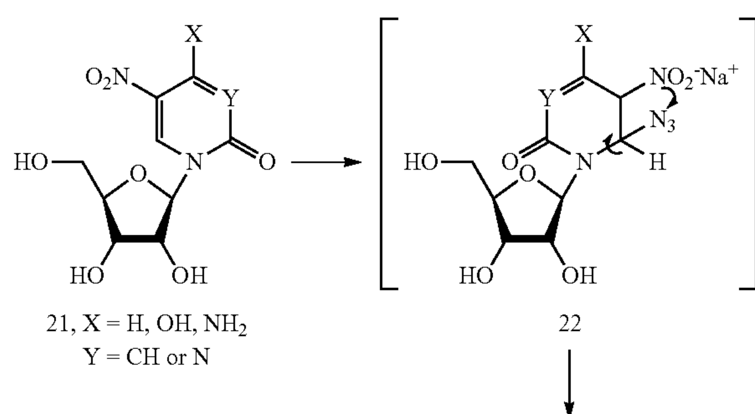
Scheme 4
