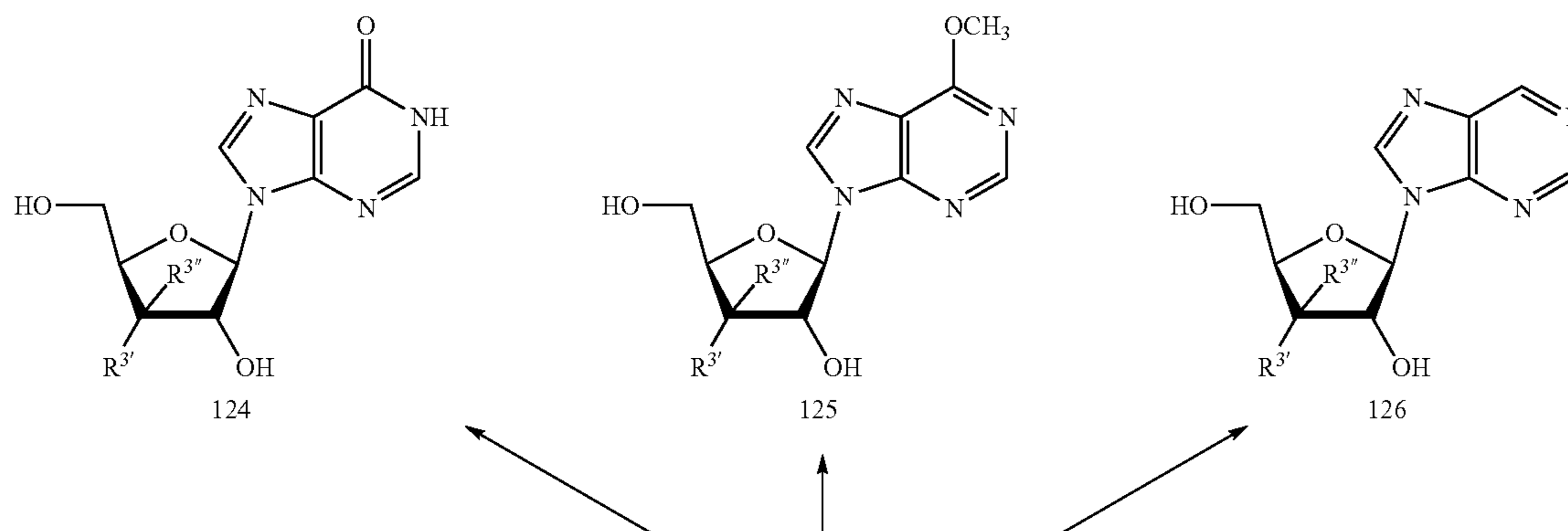
Scheme 18
