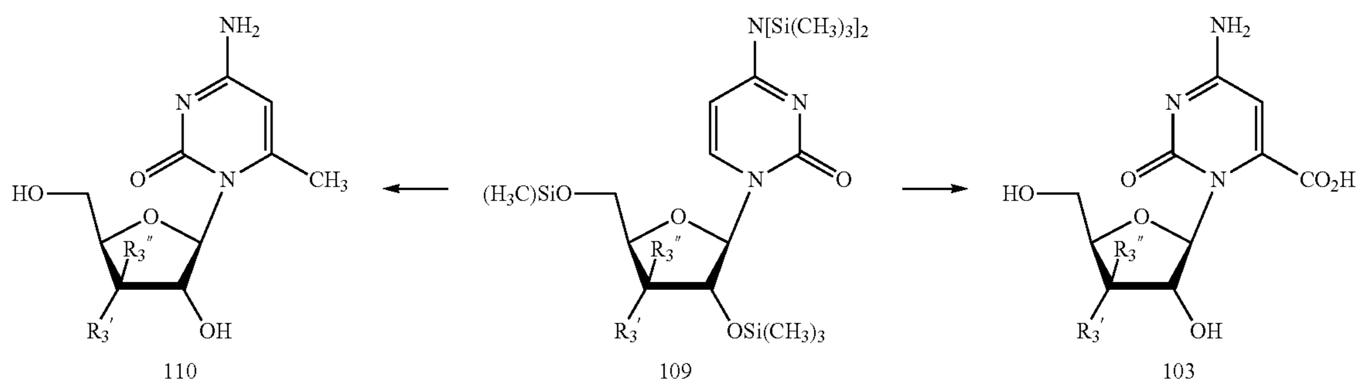
Scheme 16
