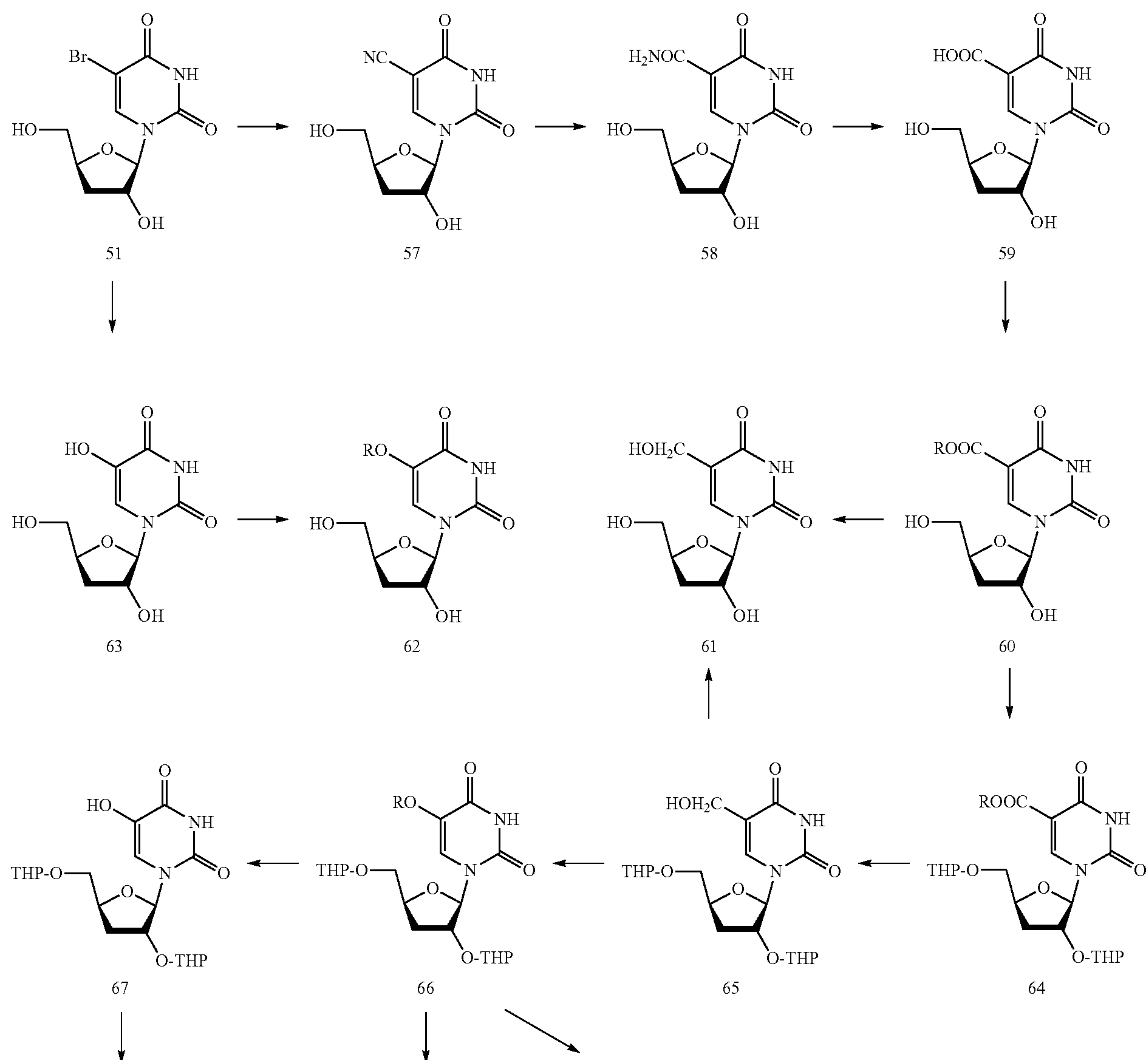
Scheme 10
