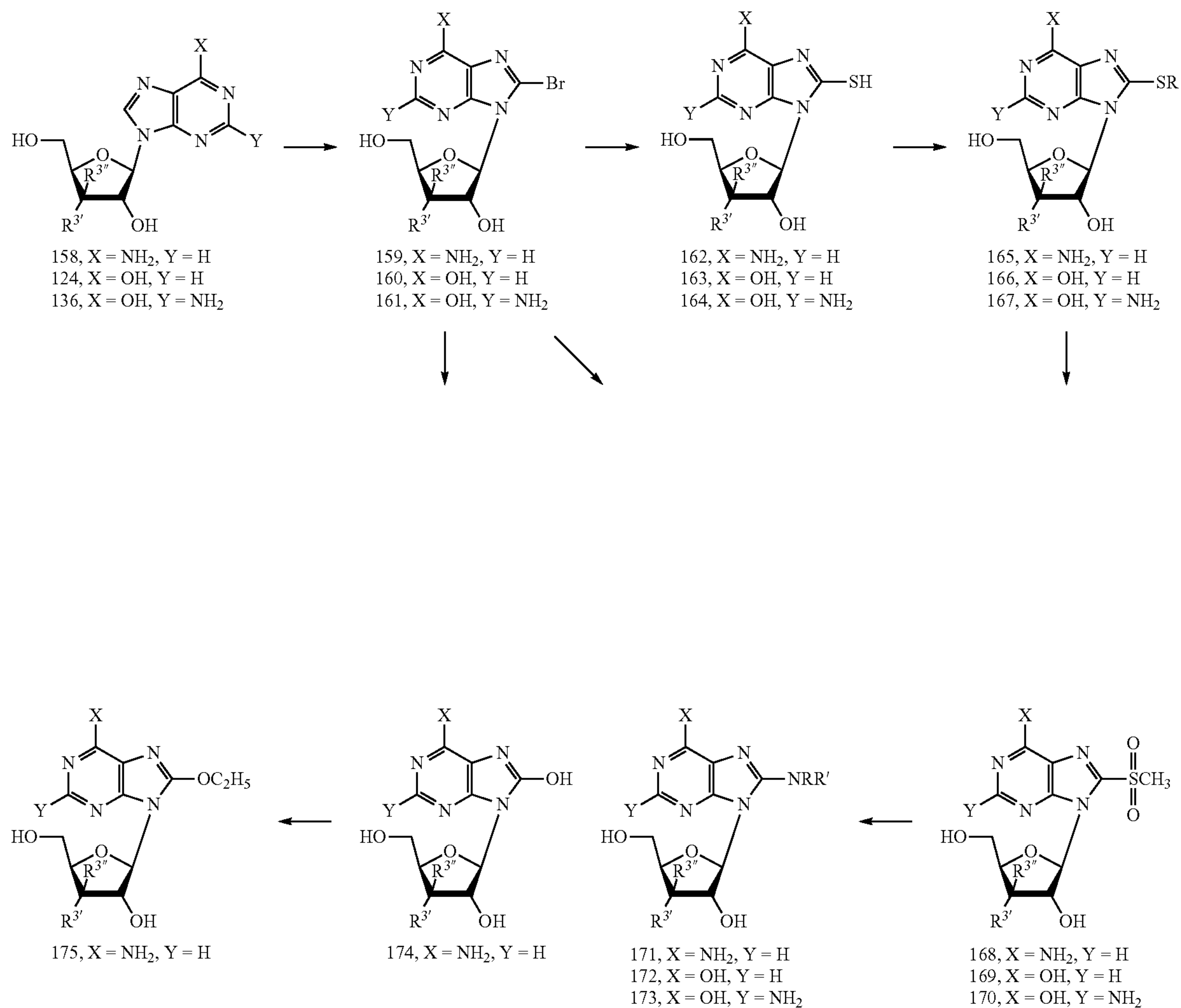
Scheme 22
