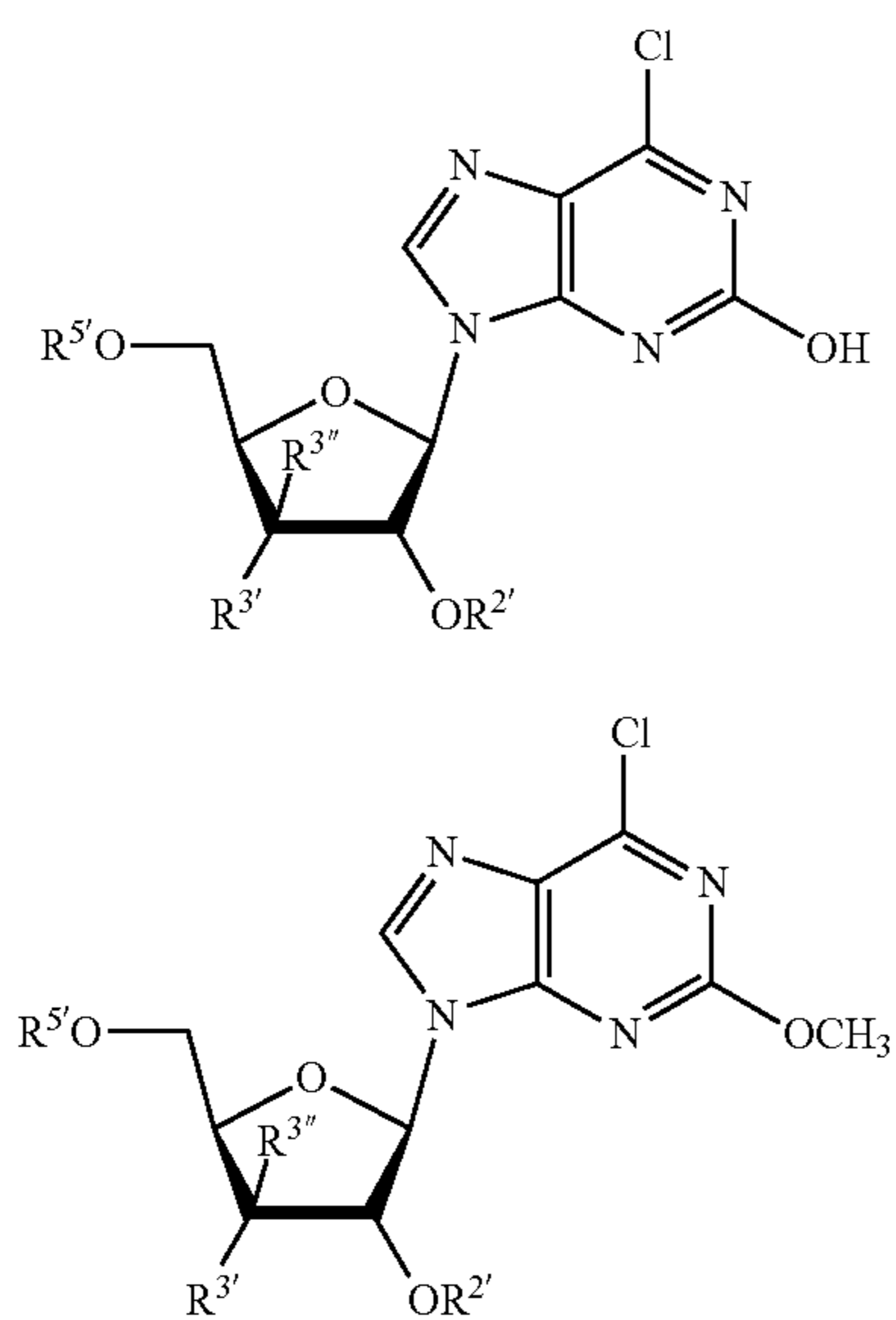
Scheme 20
