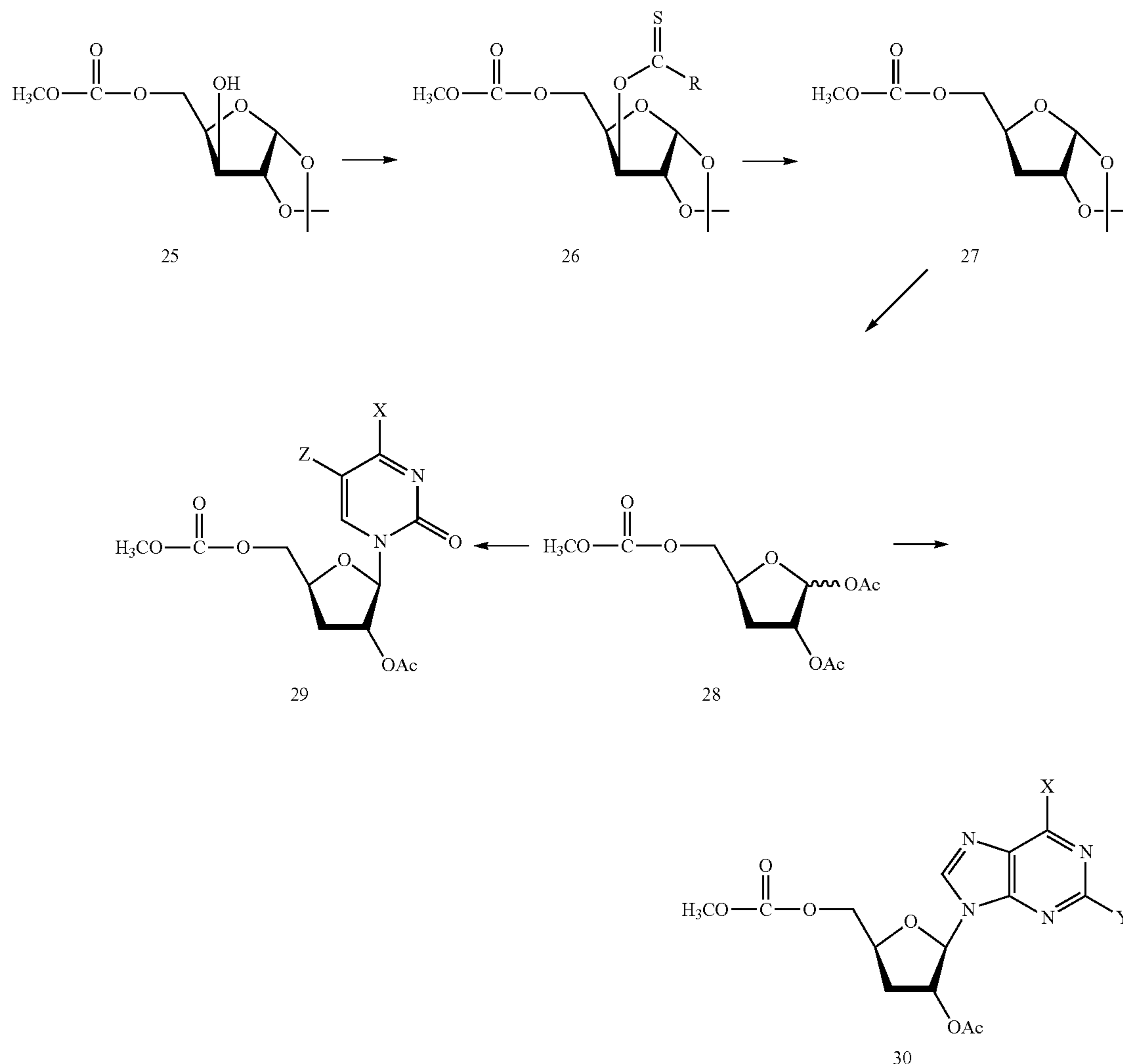
Scheme 5
