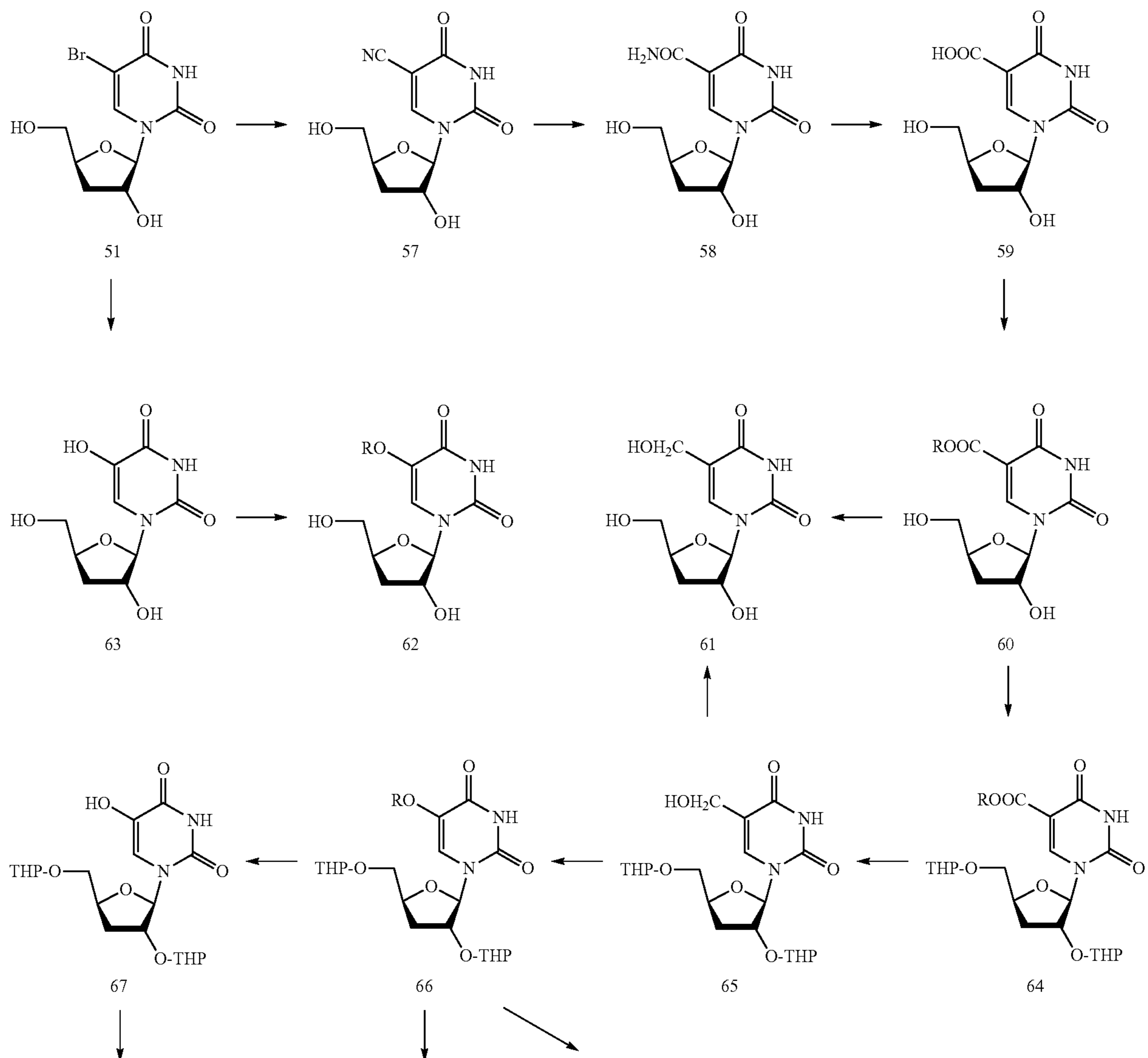
Scheme 10
