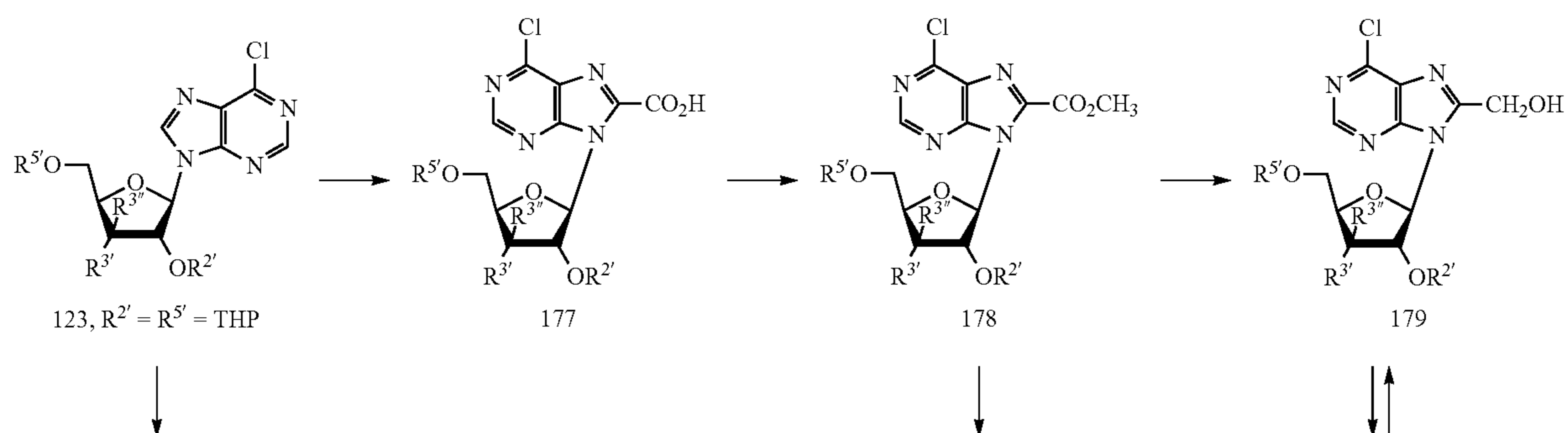
Scheme 23
