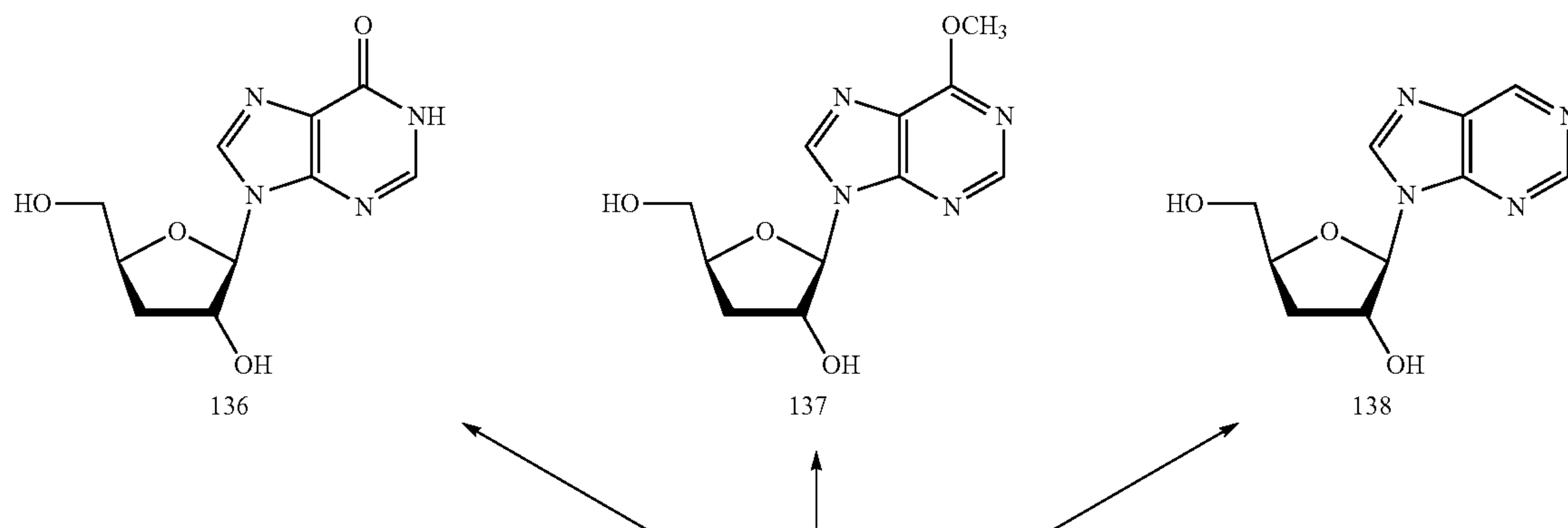
Scheme 19
