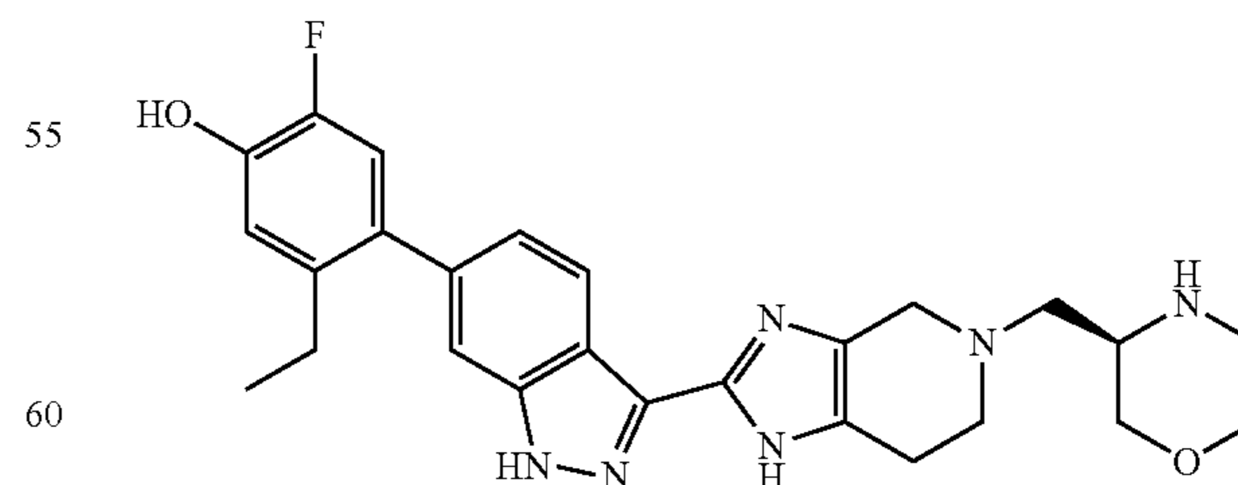
(c) 4-(3-(5-(3-(dimethylamino)-2-fluoropropyl)-4,5,6,7-tetrahydro-1H-imidazo[4,5-c]pyridin-2-yl)-1H-indazol-6-yl)-5-ethyl-2-fluorophenol
