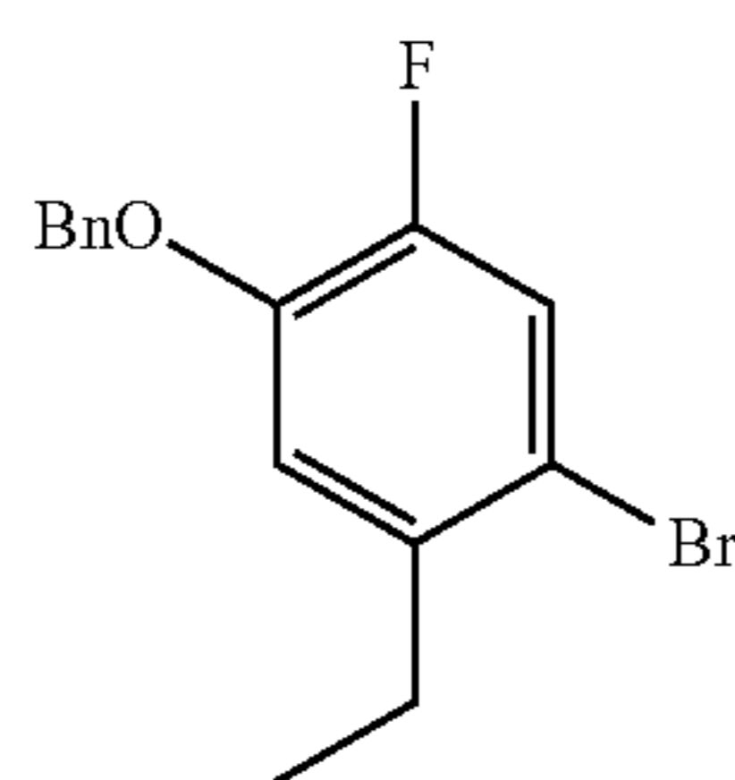
(a) 5-Ethyl-2-fluorophenol
