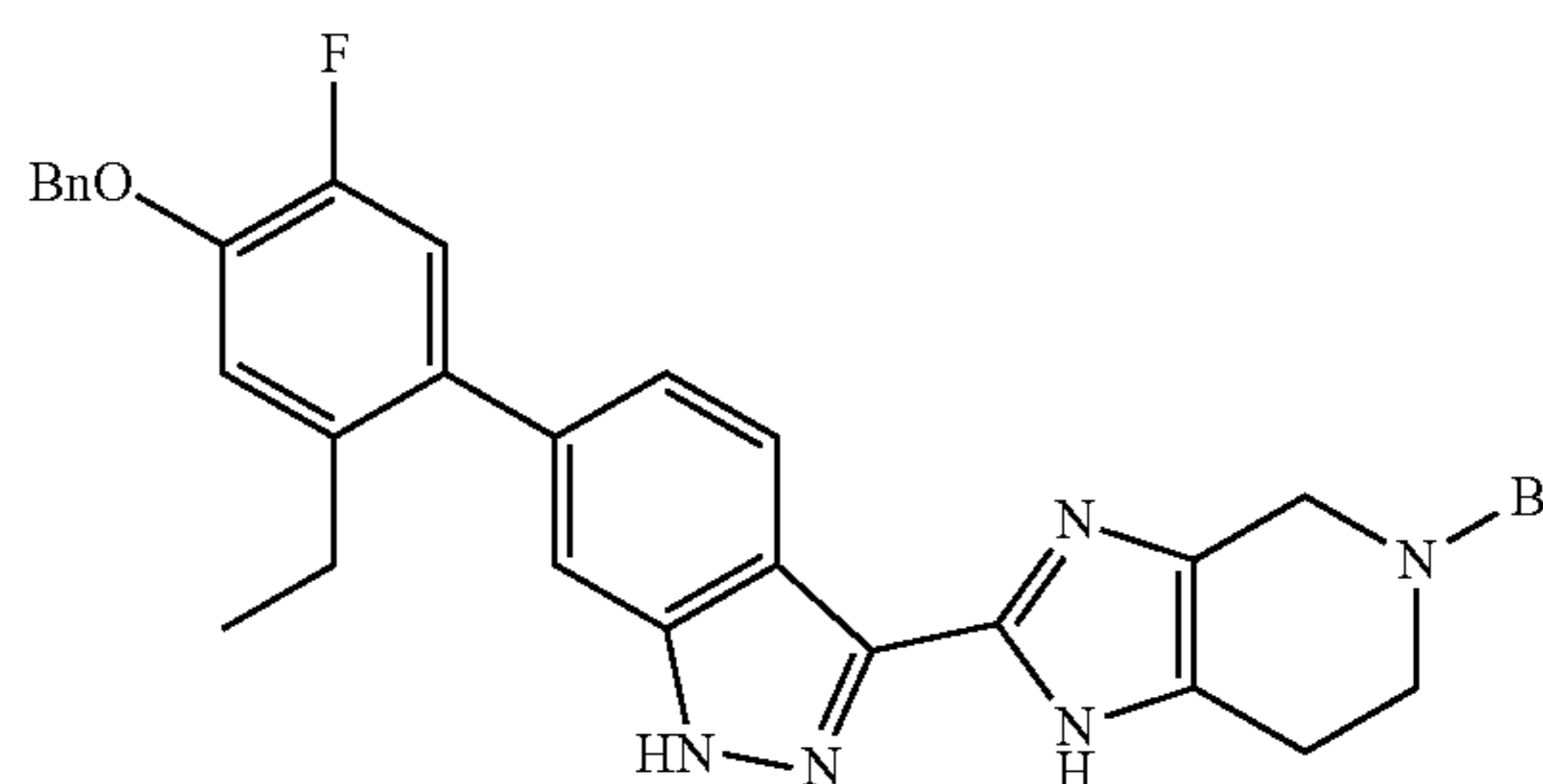
(a) 5-Benzyl-2-(6-(4-(benzyloxy)-2-ethyl-5-fluorophenyl)-1H-indazol-3-yl)-4,5,6,7-tetrahydro-1H-imidazo[4,5-c]pyridine
