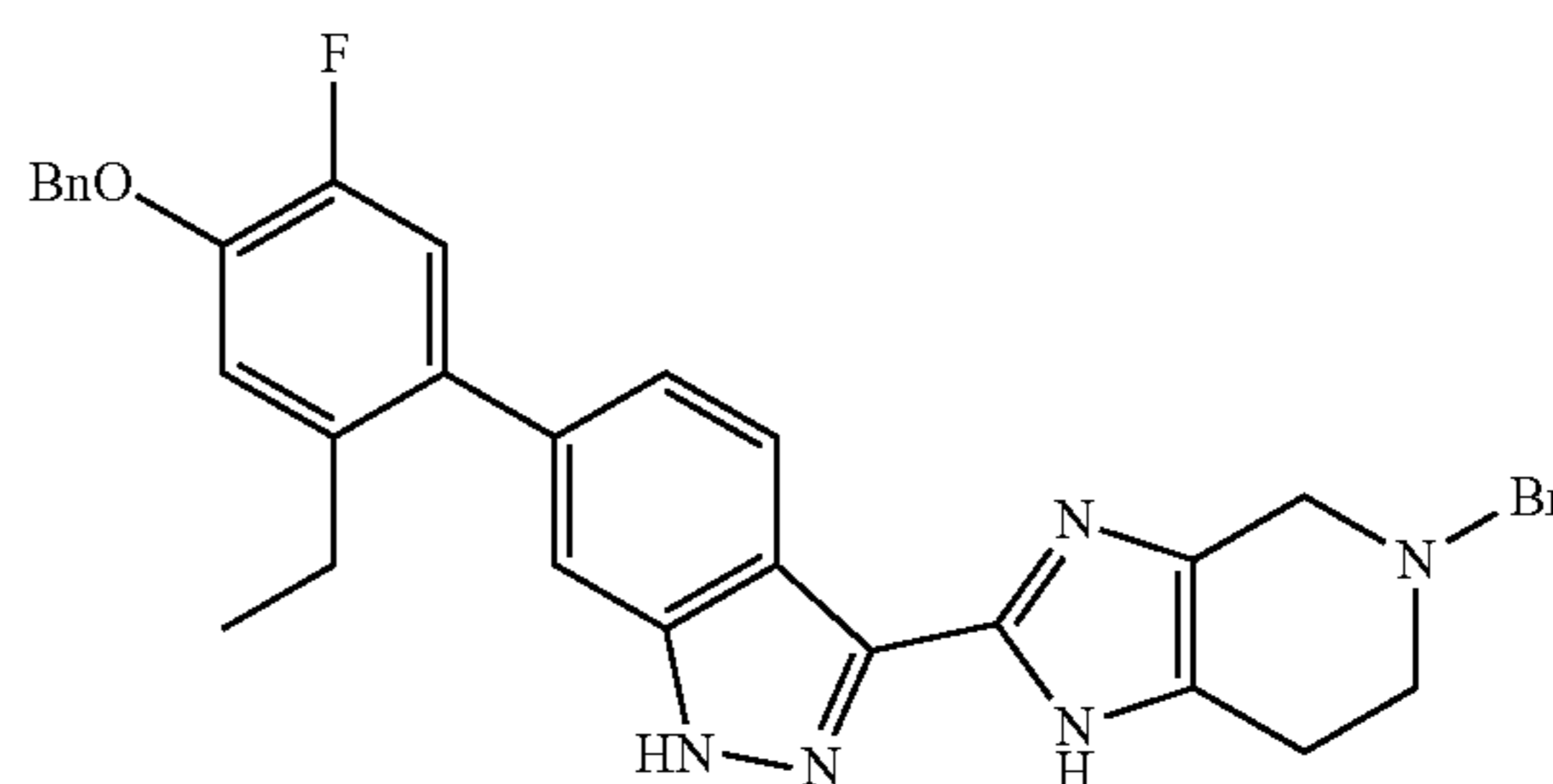
(a) 5-Benzyl-2-(6-(4-(benzyloxy)-2-ethyl-5-fluorophenyl)-1H-indazol-3-yl)-4,5,6,7-tetrahydro-1H-imidazo[4,5-c]pyridine
