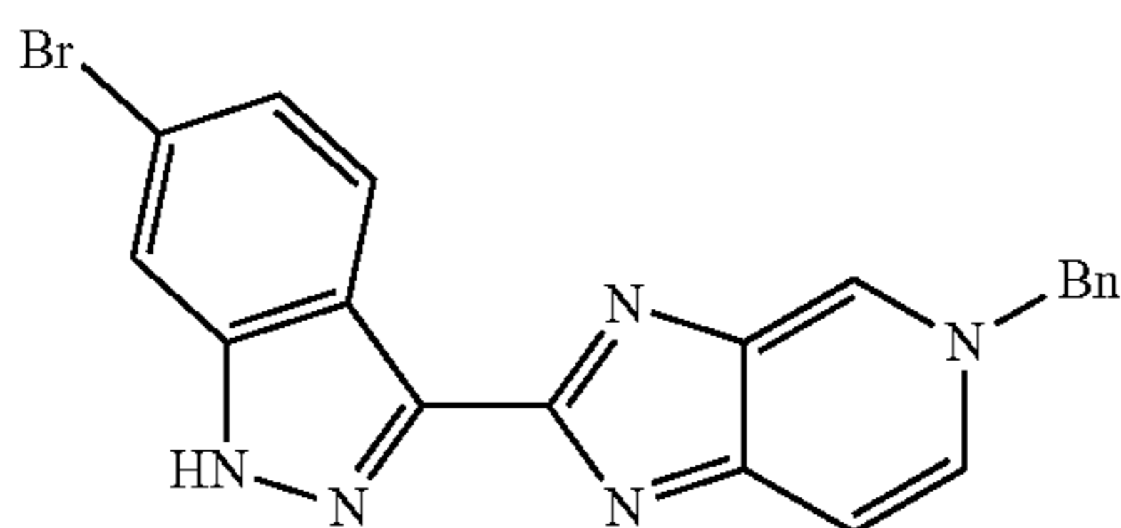
(a) 6-Bromo-1H-indazol-3-yl-carbaldehyde
