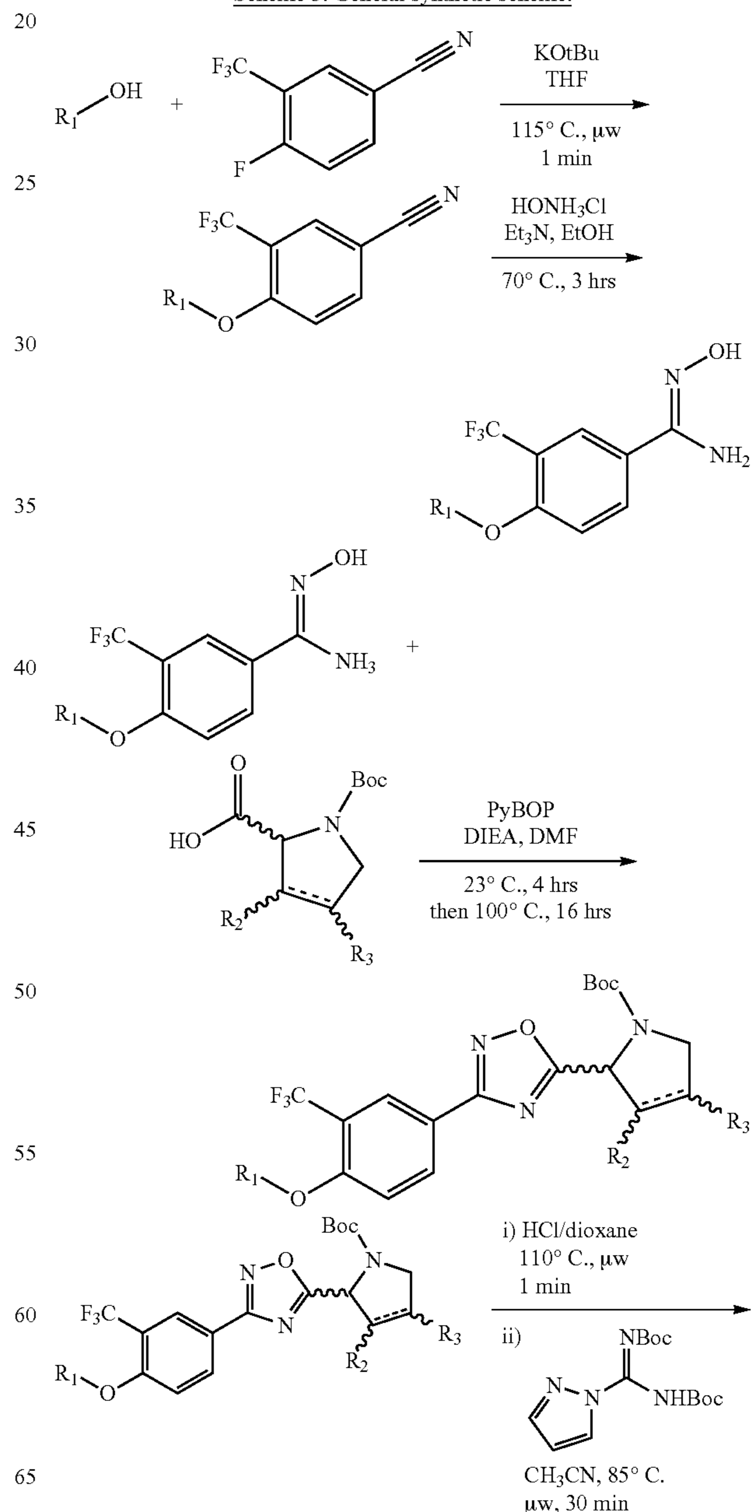
Scheme 3. General synthetic scheme.
