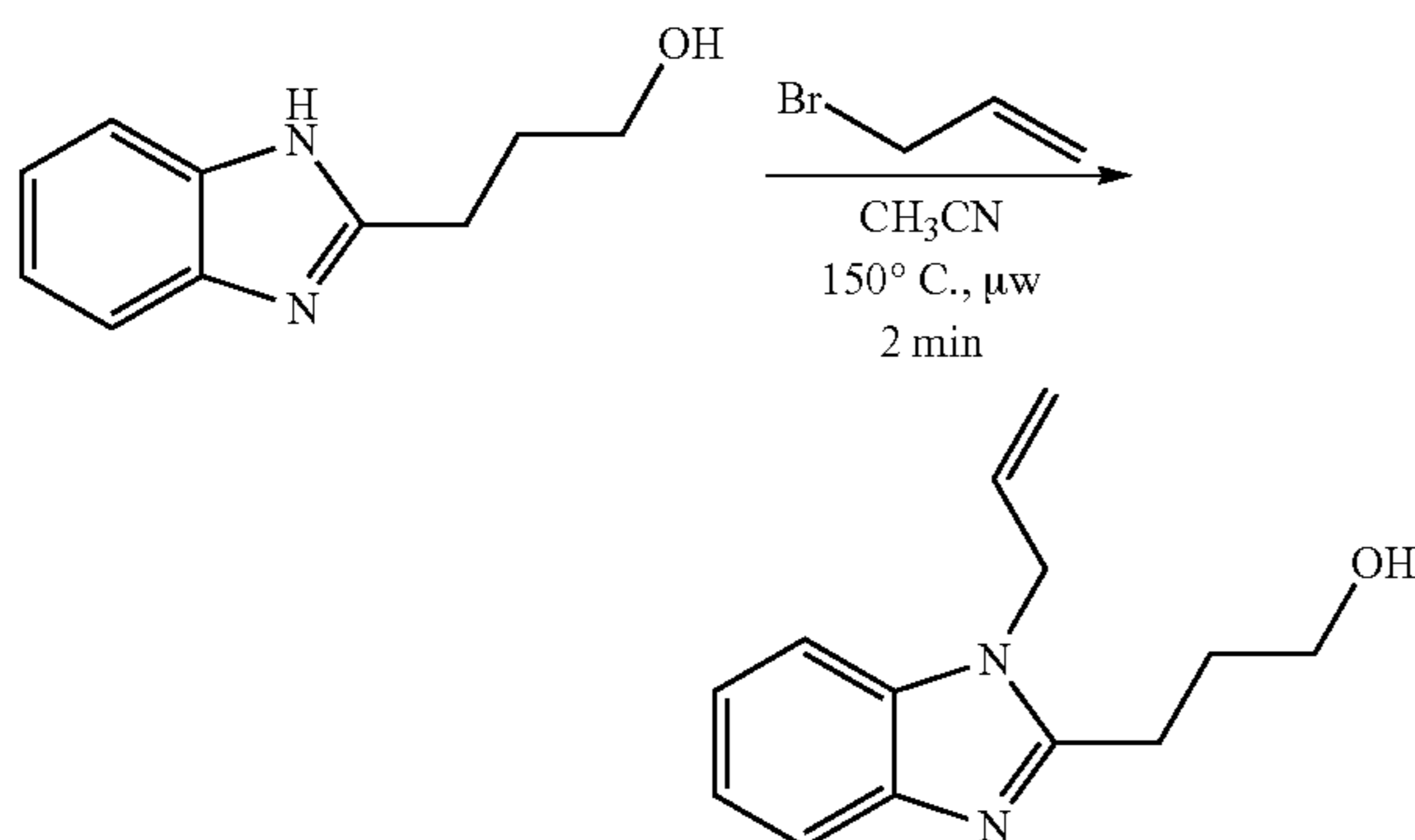
Scheme 8. Allylation of benzimidazole.
