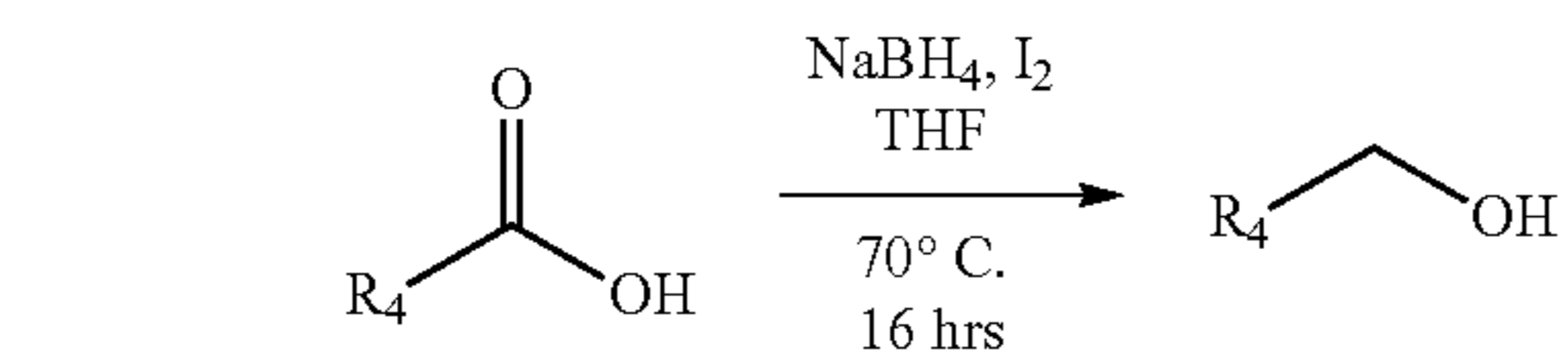
Scheme 4. Synthesis of alcohols from carboxylic acids.
