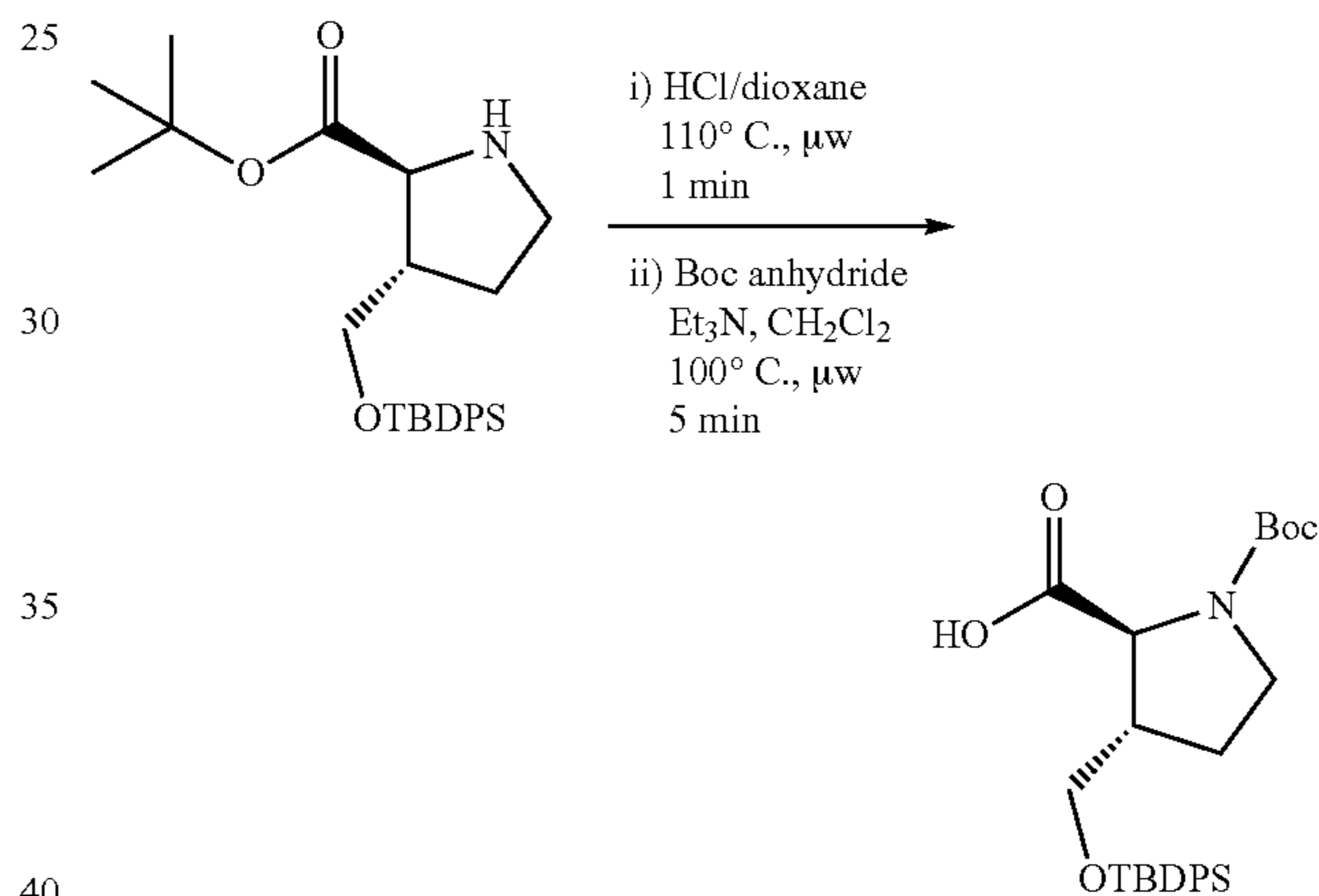
Scheme 6. Tert-butyl ester deprotection and N-Boc protection.
