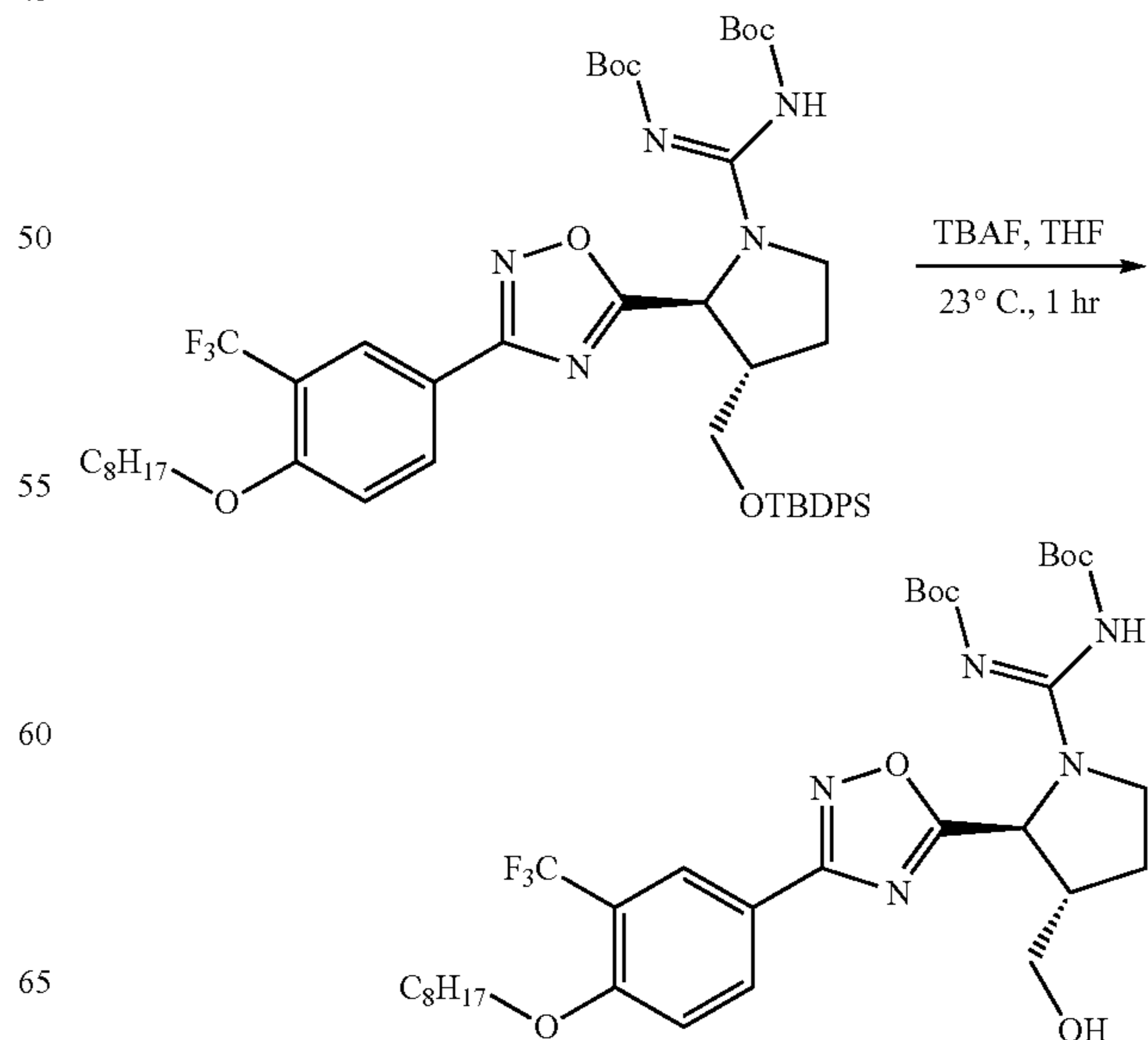
Scheme 7. TBDPS ether deprotection.
