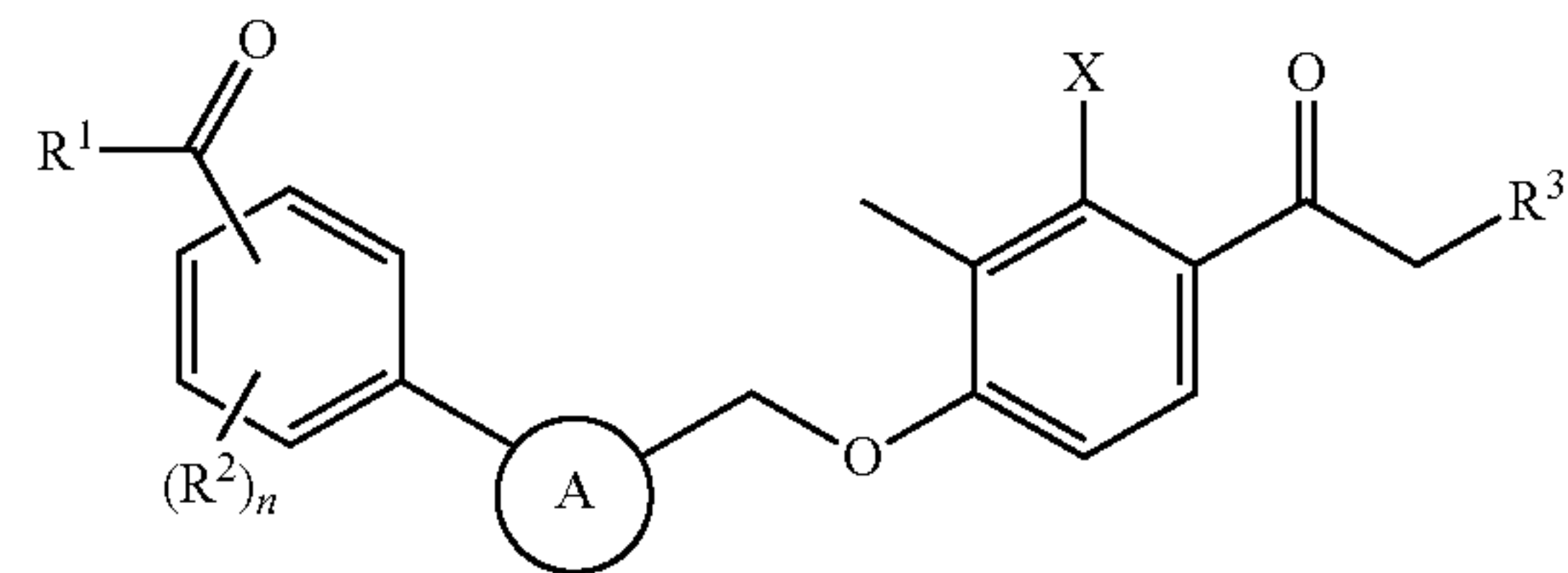
Formula (IIc)
