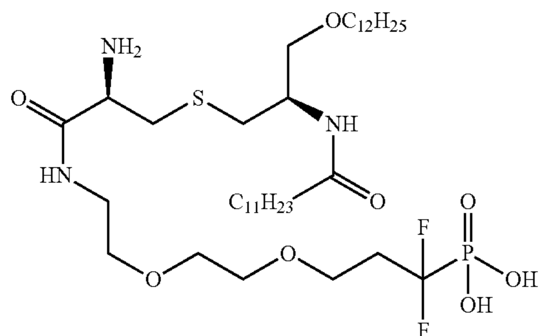
((12R,16R)-12-amino-16-dodecanamido-1,1-difluoro-11-oxo-4,7,18-trioxa-14-thia-10-azatriacontyl)phosphonic acid
