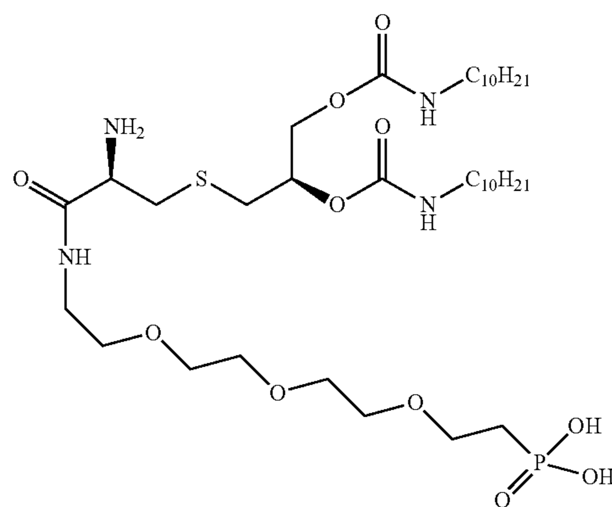
((14R,18R)-14-amino-18-((decylcarbamoyl)oxy)-13,21-dioxo-3,6,9,20-tetraoxa-16-thia-12,22-diazadotriacontyl)phosphonic acid
