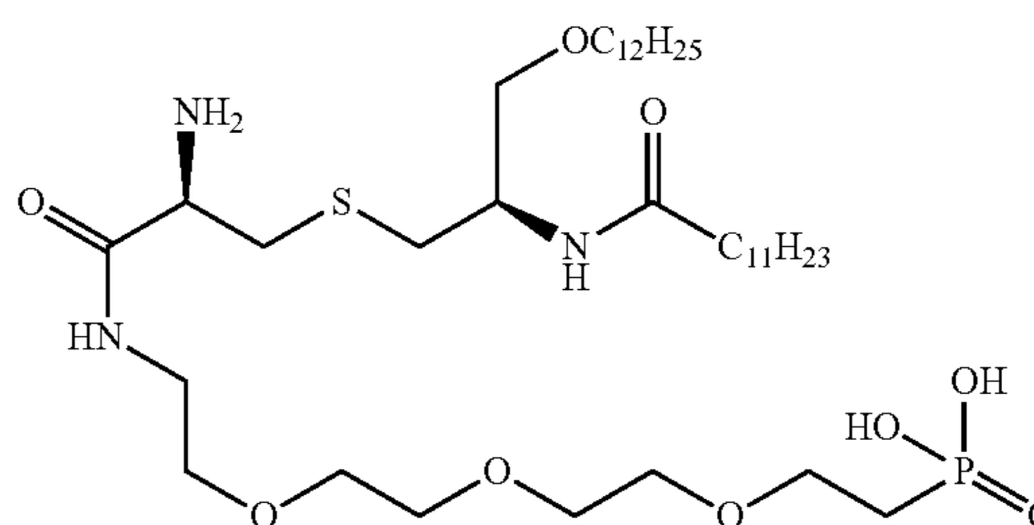
((14R,18R)-14-amino-18-dodecanamido-13-oxo-3,6,9,20-tetraoxa-16-thia-12-azadotriacetyl)phosphonic acid
