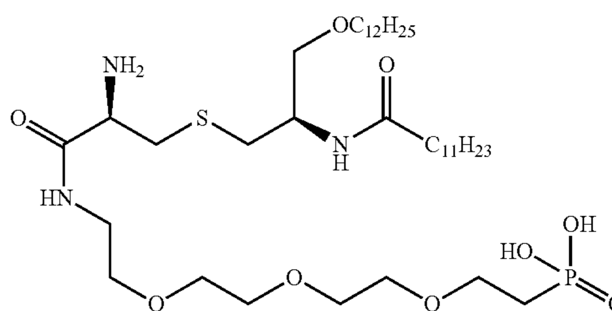
((14R,18R)-14-amino-18-dodecanamido-13-oxo-3,6,9,20-tetraoxa-16-thia-12-azadotriacontyl)phosphonic acid
