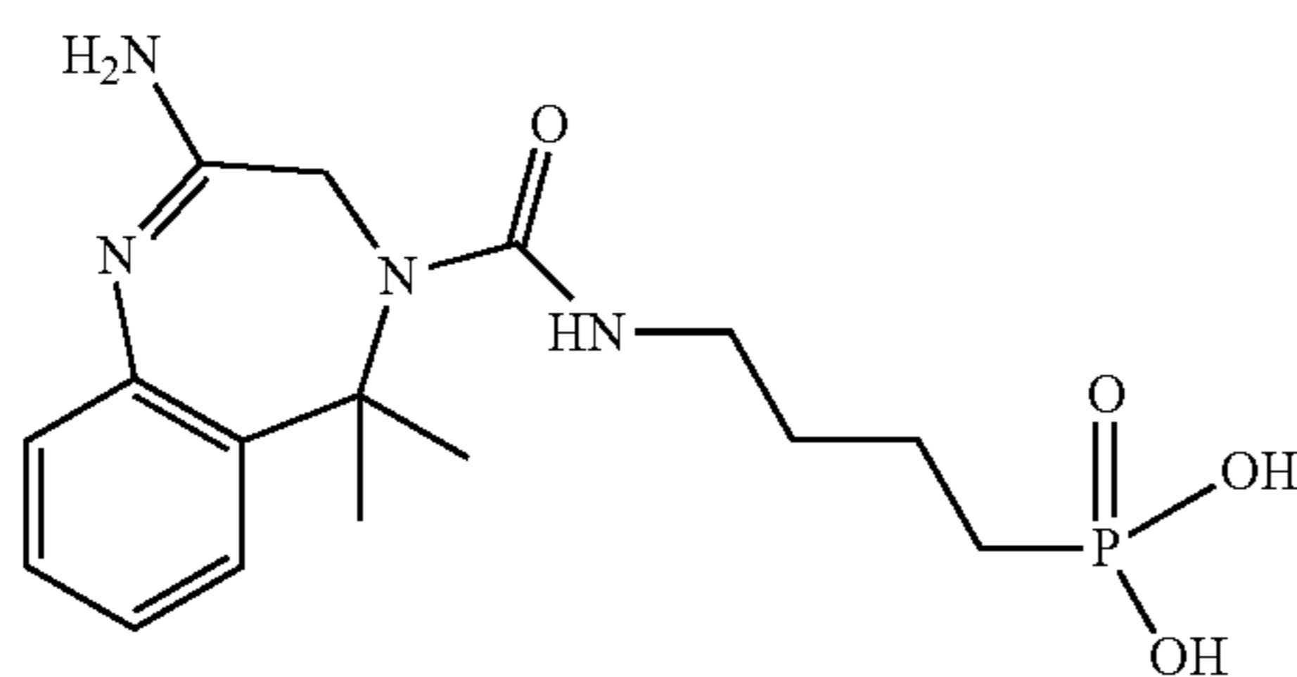
(4-(2-amino-5,5-dimethyl-4,5-dihydro-3H-benzo[e][1,4]diazepine-4-carboxamido)butyl)phosphonic acid
