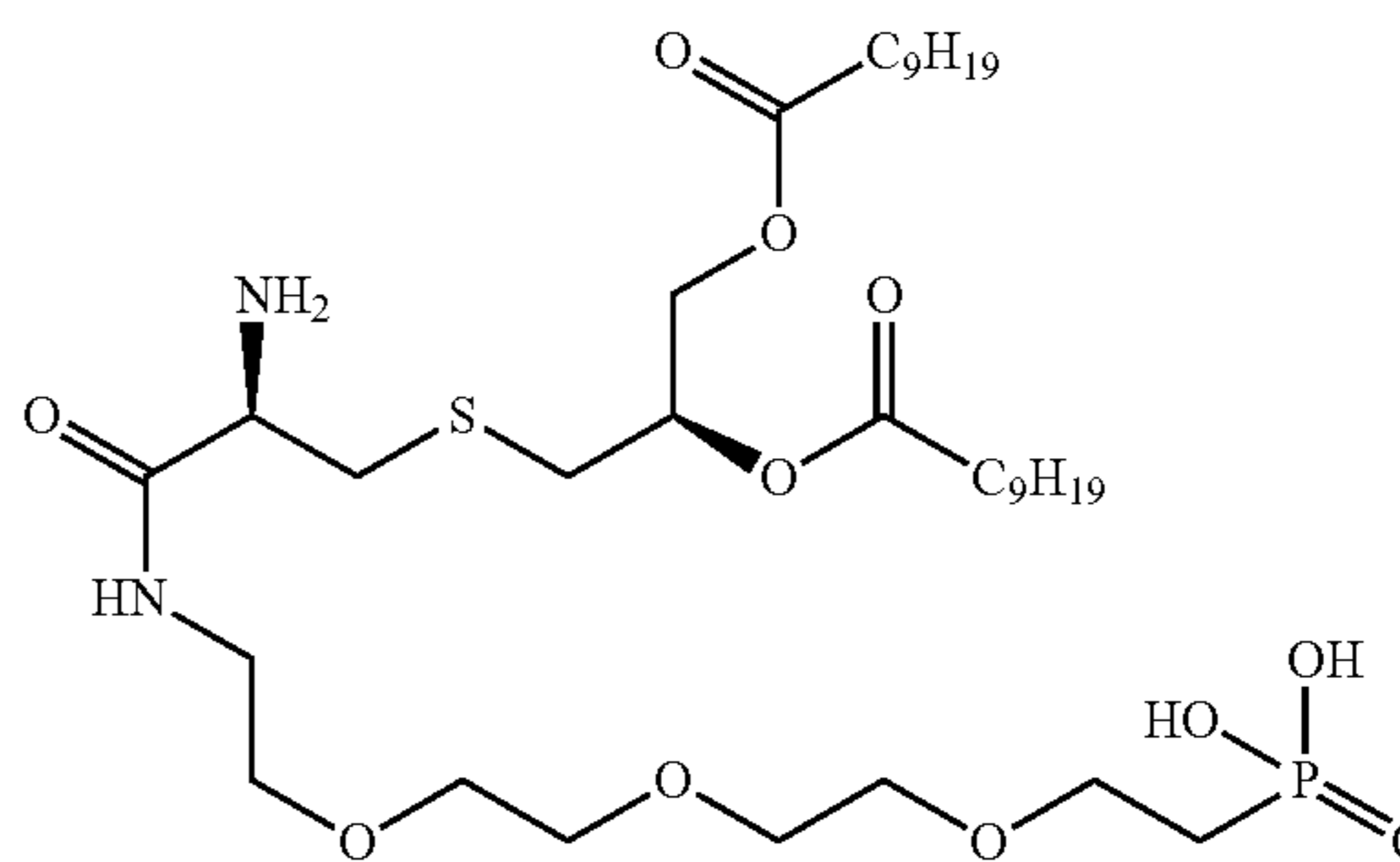
((14R,18R)-14-amino-18-(decanoyloxy)-13,21-dioxo-3,6,9,20-tetraoxa-16-thia-12-azatriacetyl)phosphonic acid
