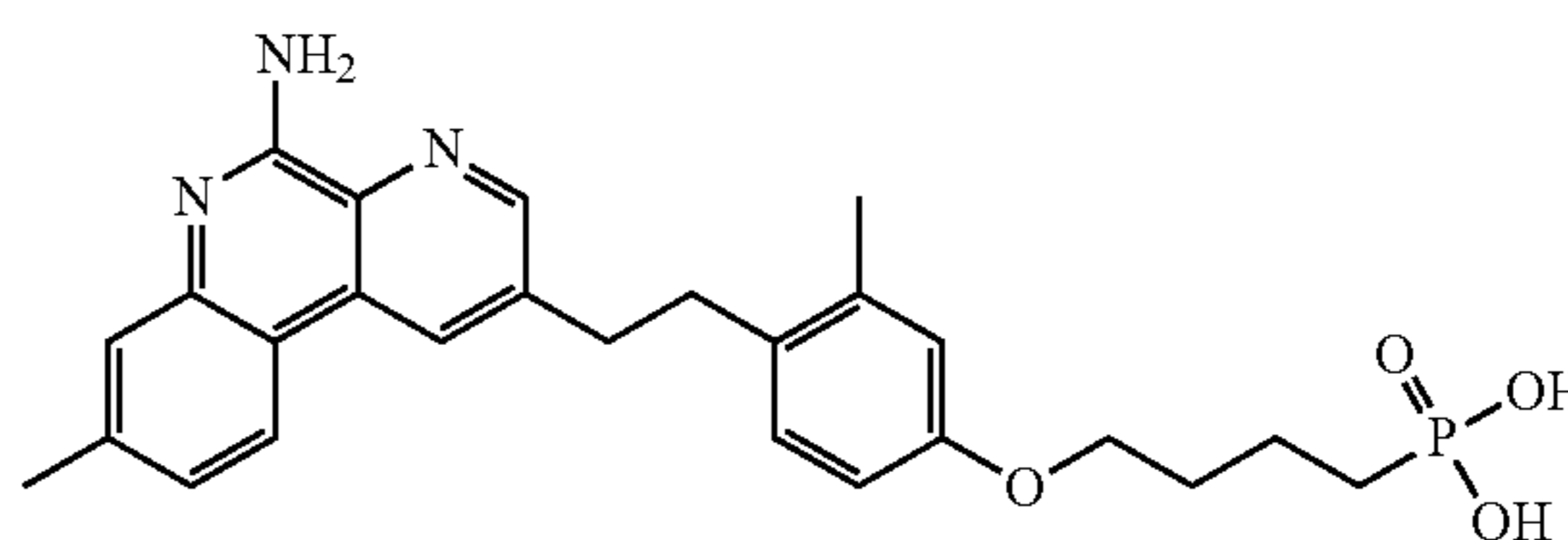
(4-(4-(2-(5-amino-8-methylbenzo[f][1,7]naphthyridin-2-yl)ethyl)-3-methylphenoxy)butyl)phosphonic acid
