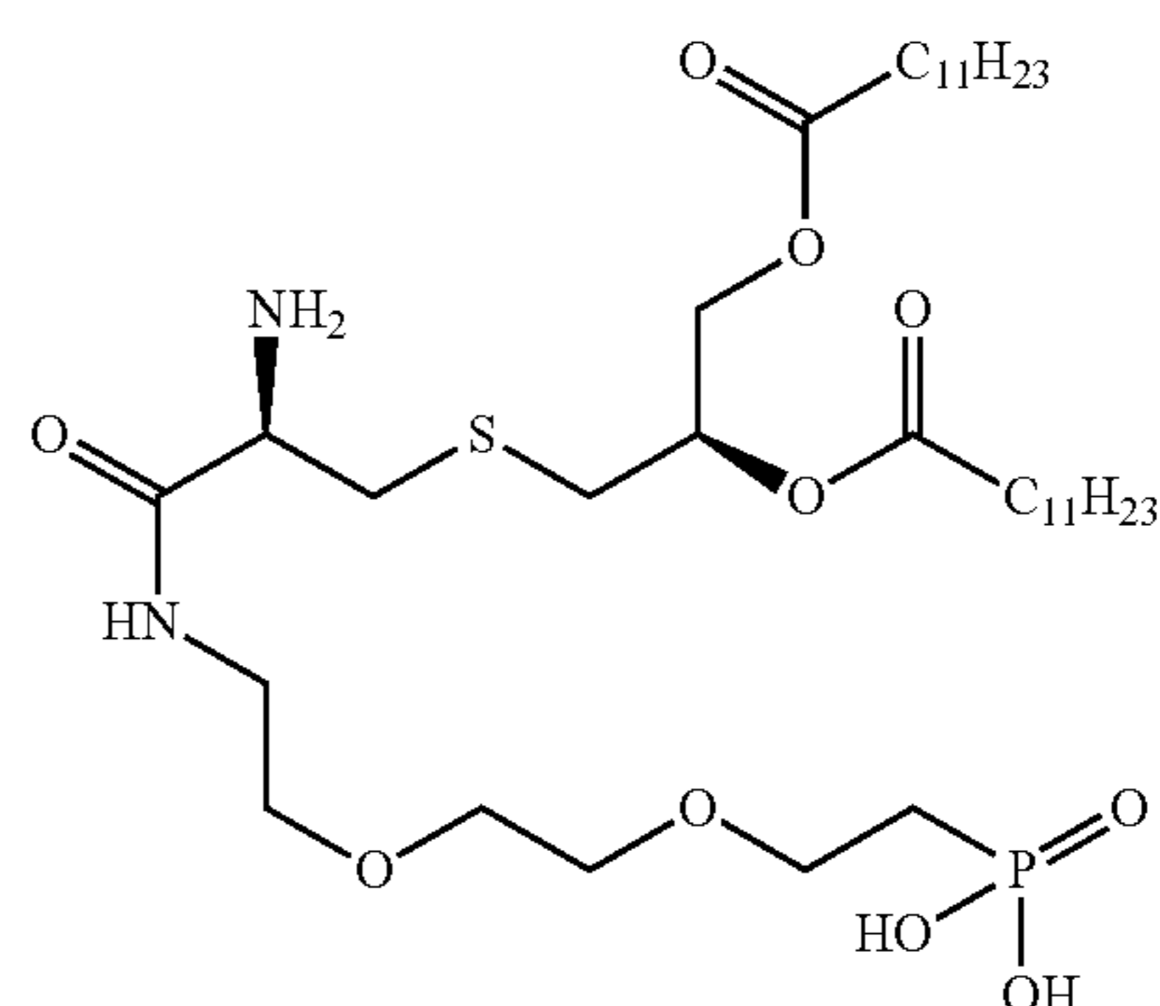
(11R,15R)-11-amino-15-(dodecanoyloxy)-10,18-dioxo-3,6,17-trioxa-13-thia-9-azanonacosyl)phosphonic acid
