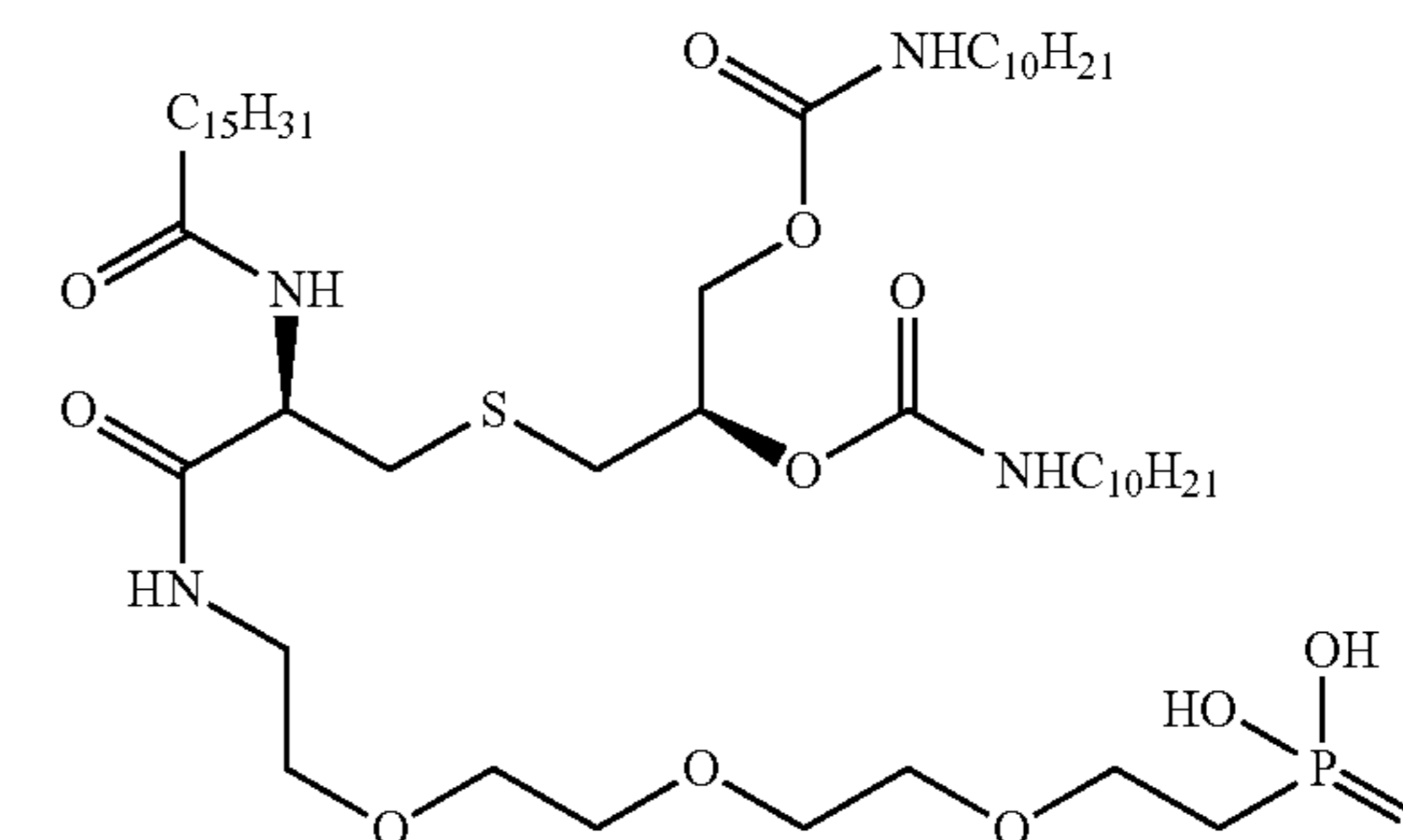
((14R,18R)-18-((decylcarbamoyl)oxy)-13,21-dioxo-14-palmitamido-3,6,9,20-tetraoxa-16-thia-12,22-diazadotriacontyl)phosphonic acid
