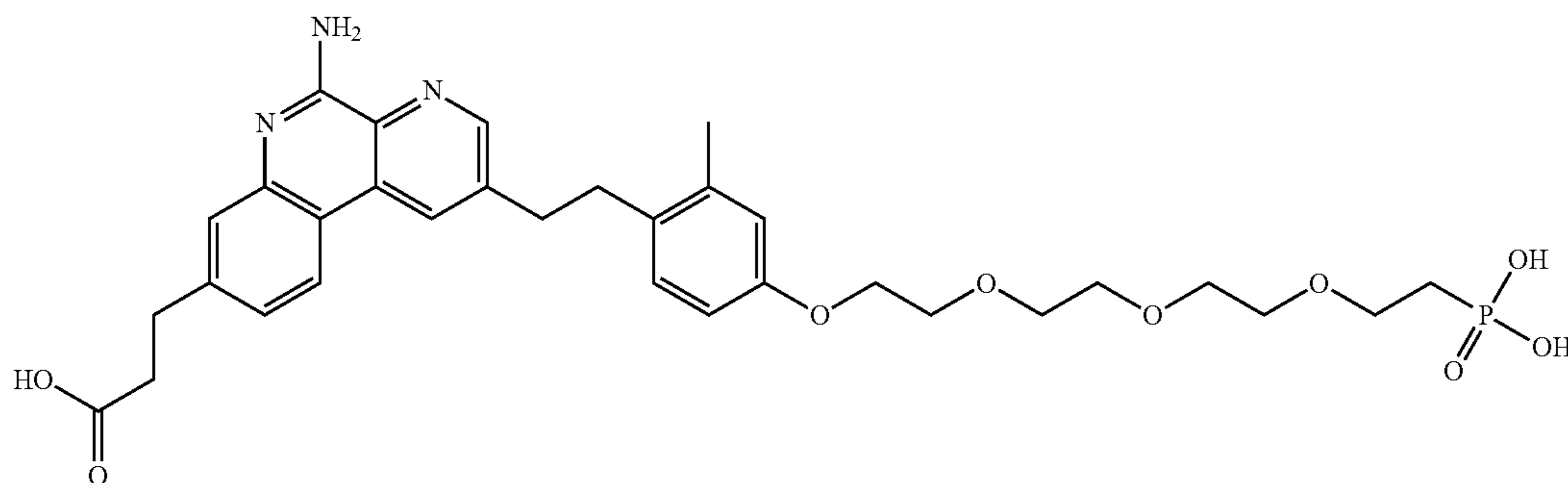
3-(5-amino-2-(2-methyl-4-(2-(2-(2-(2-phosphonoethoxy)ethoxy)ethoxy)ethoxy)phenethyl)benzo[f][1,7]naphthyridin-8-yl)propanoic acid
