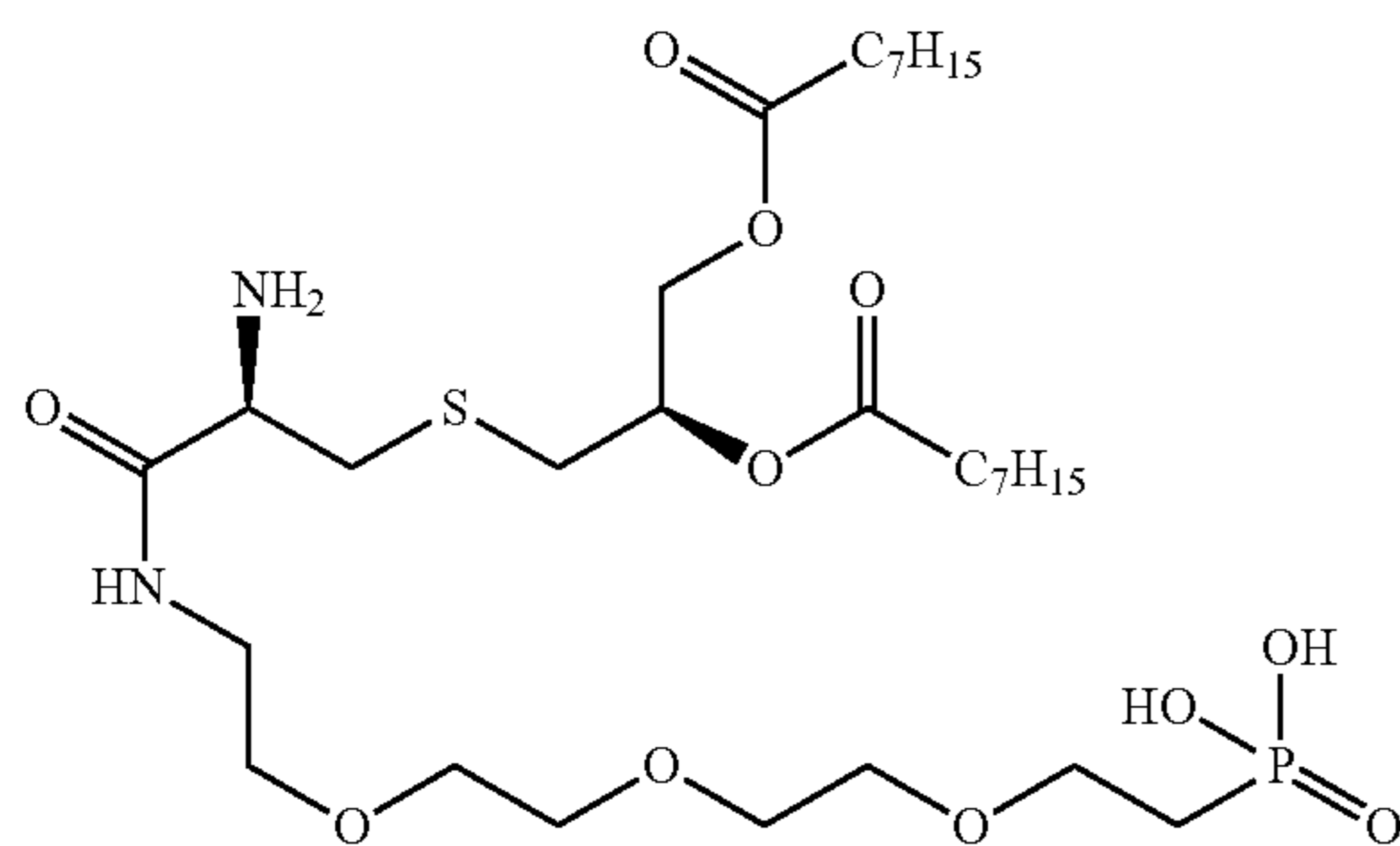
((14R,18R)-14-amino-18-(octanoyloxy)-13,21-dioxo-3,6,9,20-tetraoxa-16-thia-12-azaoctacosyl)phosphonic acid
