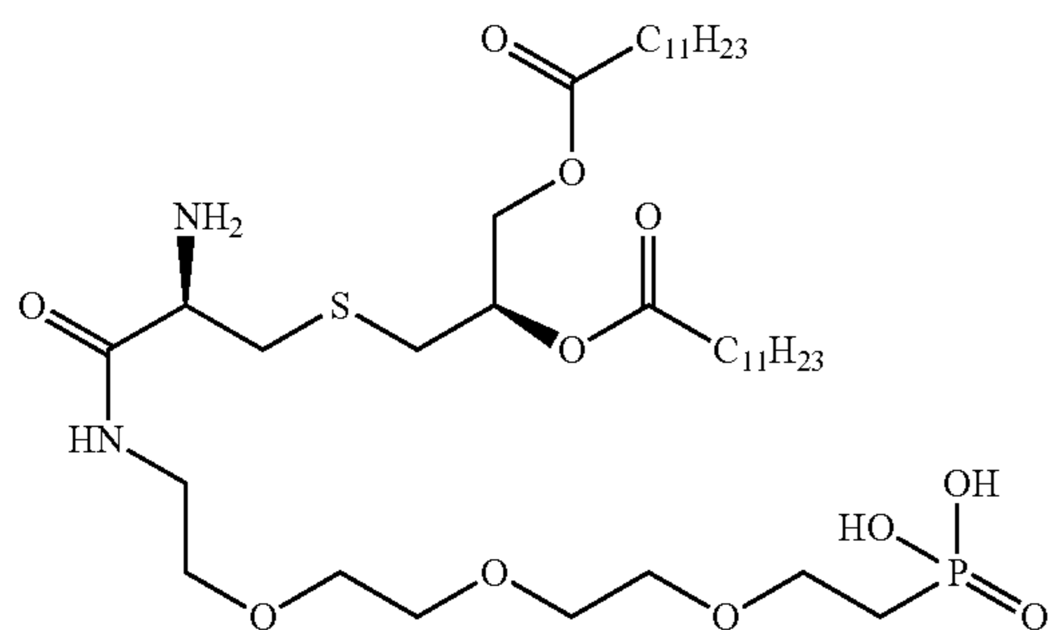
(14R,18R)-14-amino-18-(dodecanoyloxy)-13,21-dioxo-3,6,9,20-tetraoxa-16-thia-12-azadotriacontylphosphonic acid
