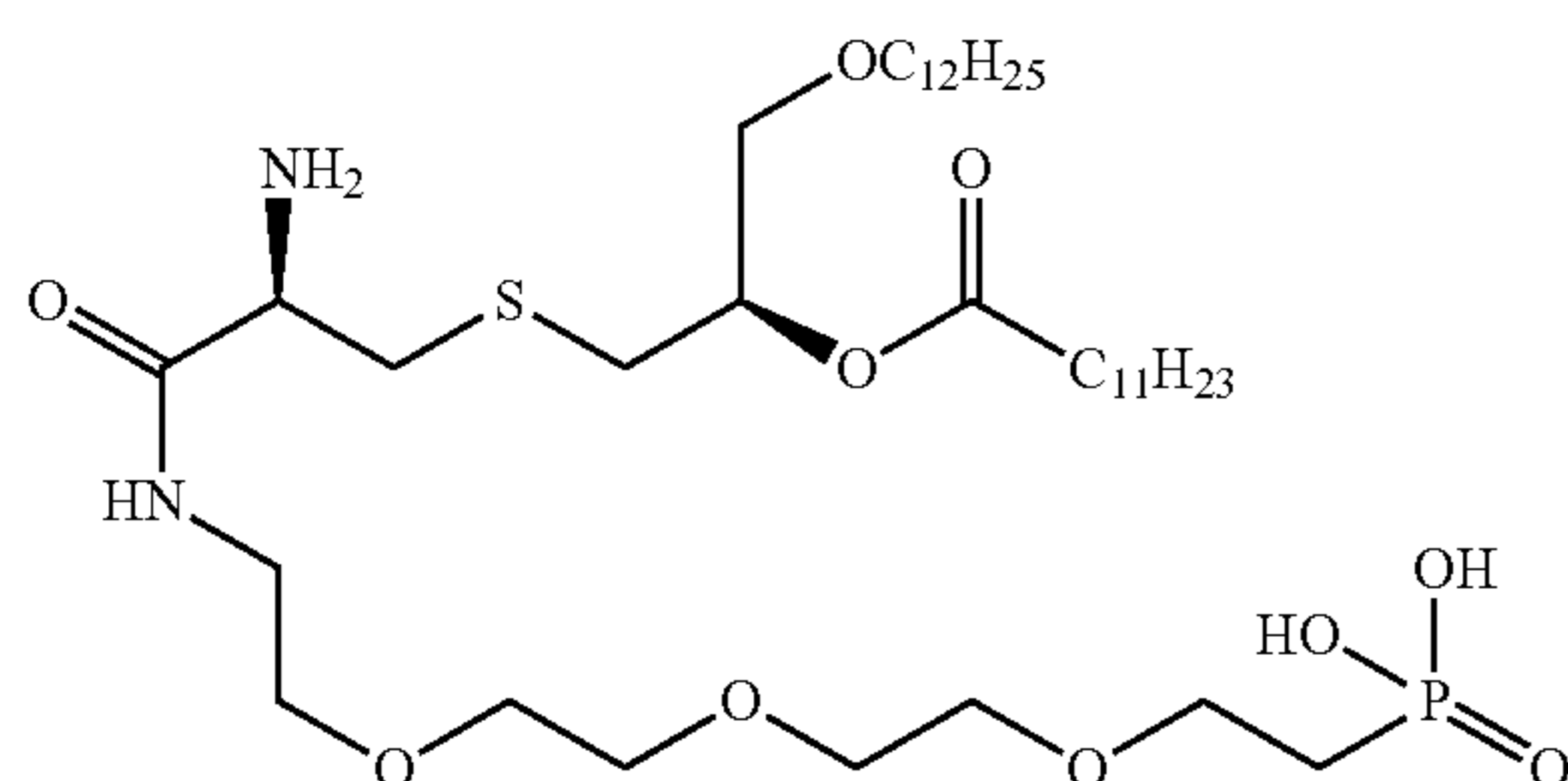
((14R,18R)-14-amino-18-(dodecanoyloxy)-13-oxo-3,6,9,20-tetraoxa-16-thia-12-azatriacetyl)phosphonic acid
