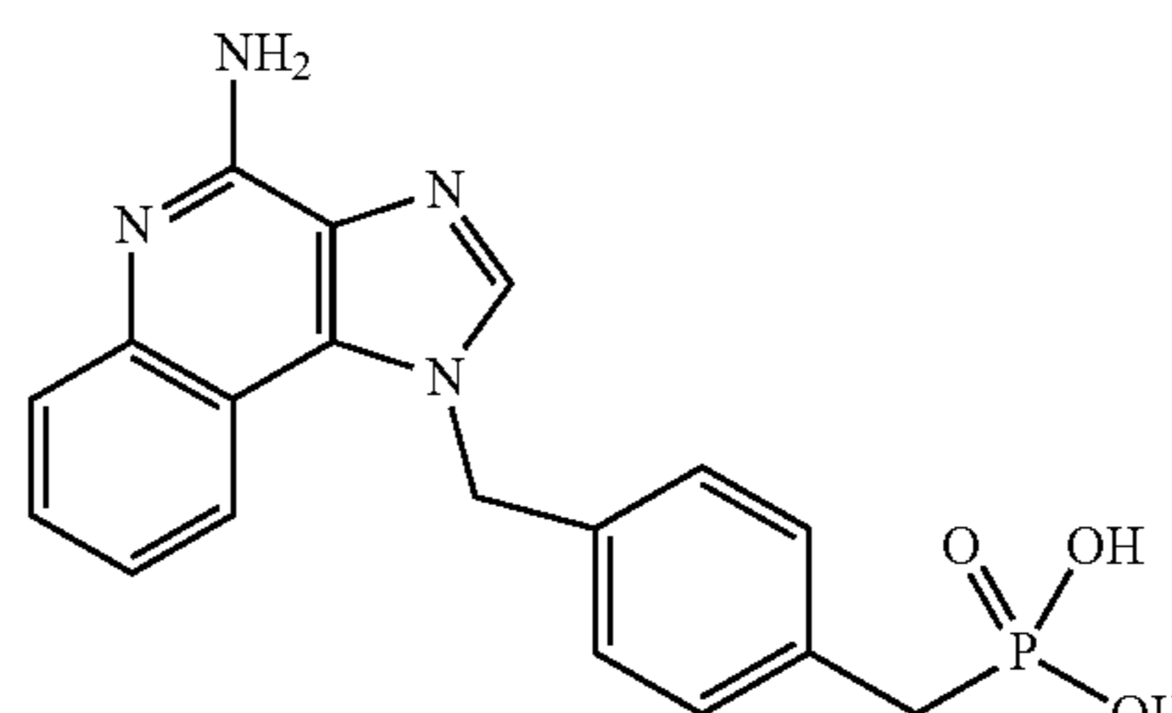
(4-((4-amino-1H-imidazo[4,5-c]quinolin-1-yl)methyl)benzyl)phosphonic acid
