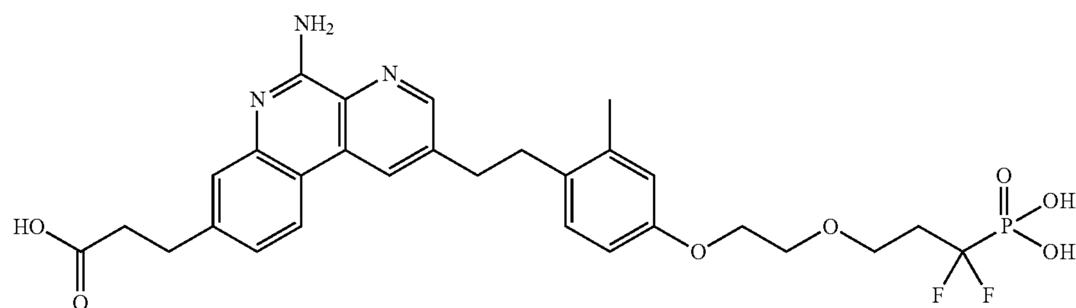
3-(5-amino-2-(4-(2-(3,3-difluoro-3-phosphonopropoxy)ethoxy)-2-methylphenethyl)benzo[f][1,7]naphthyridin-8-yl)propanoic acid
