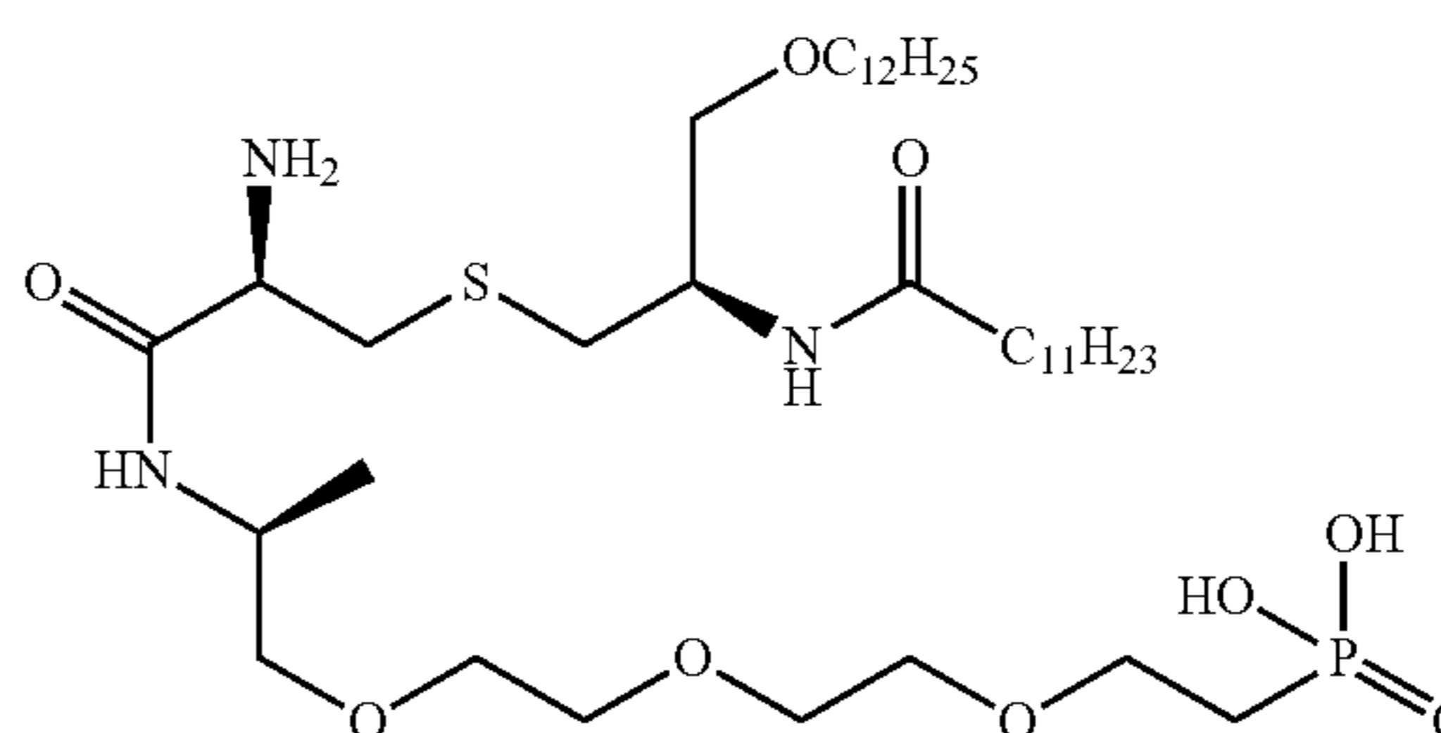
((11S,14R,18R)-14-amino-18-dodecanamido-11-methyl-13-oxo-3,6,9,20-tetraoxa-16-thia-12-azadotriacetyl)phosphonic acid
