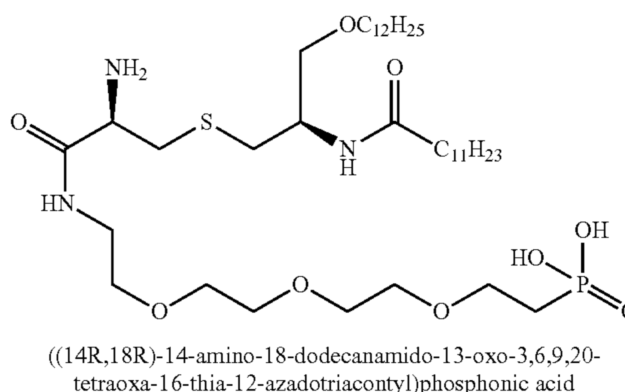
((14R,18R)-14-amino-18-(decanoyloxy)-13,21-dioxo-3,6,9,20-tetraoxa-16-thia-12-azatriacontyl)phosphonic acid
