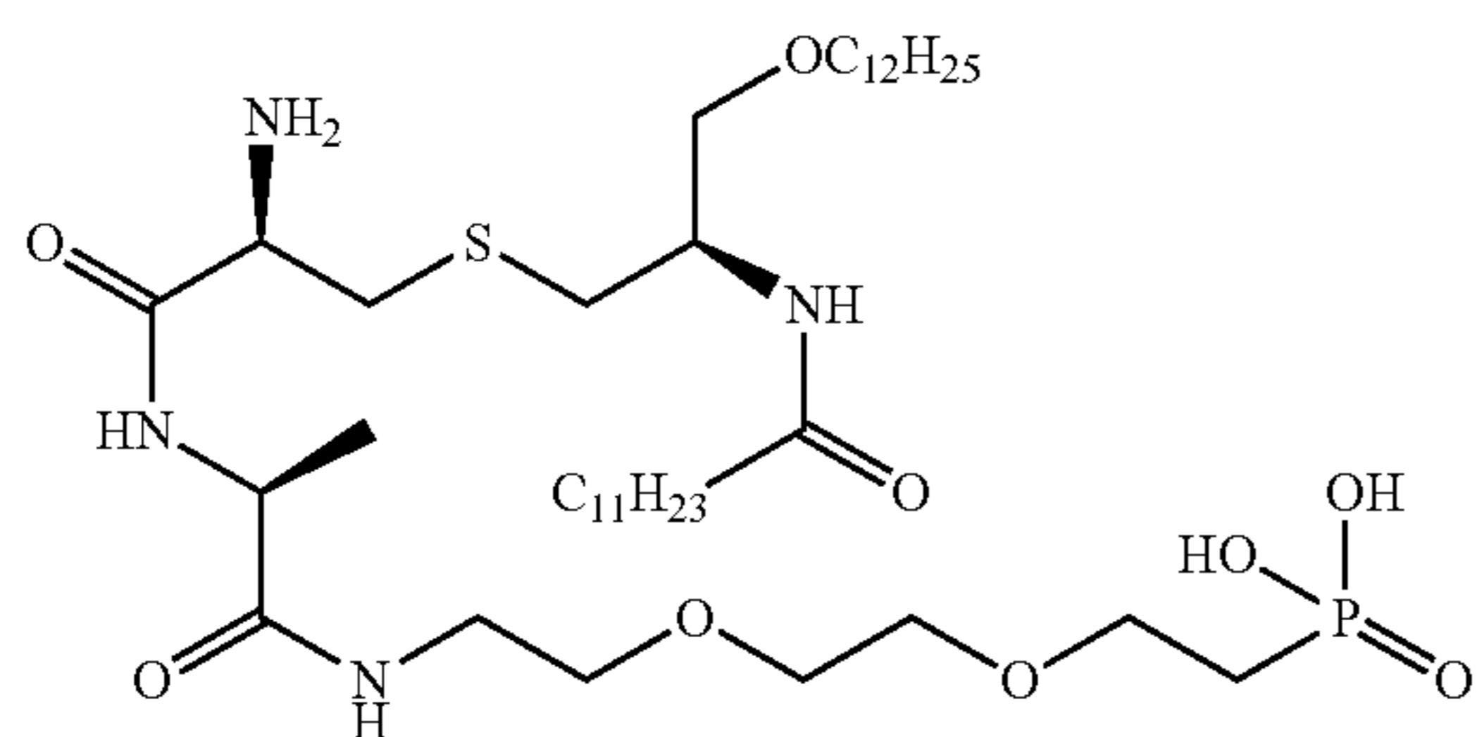
((11S,14R,18R)-14-amino-18-dodecanamido-11-methyl-10,13-dioxo-3,6,20-trioxa-16-thia-9,12-diazadotriacontyl)phosphonic acid
