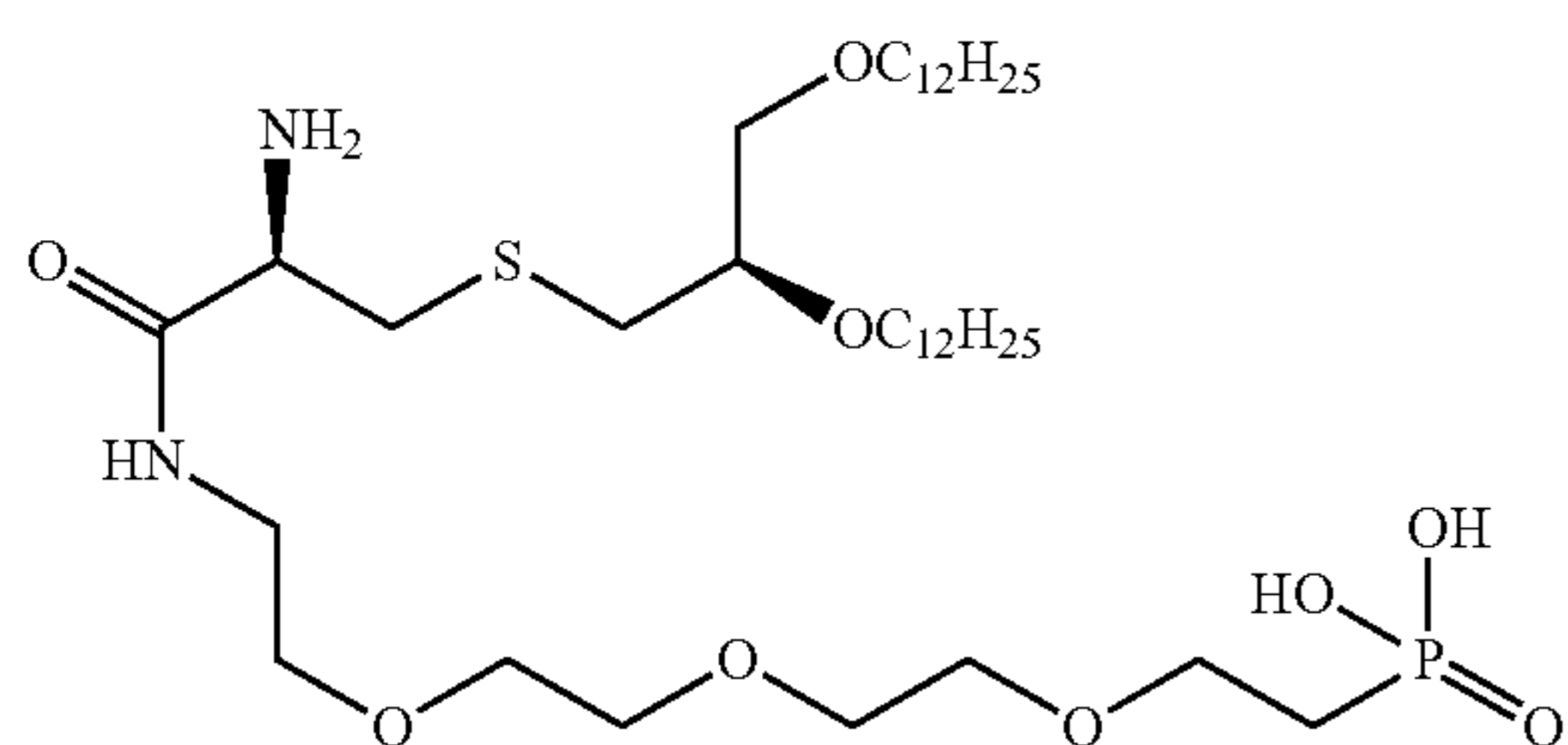
(14R,18R)-14-amino-18-(dodecyloxy)-13-oxo-3,6,9,20-tetraoxa-16-thia-12-azadotriacontylphosphonic acid
