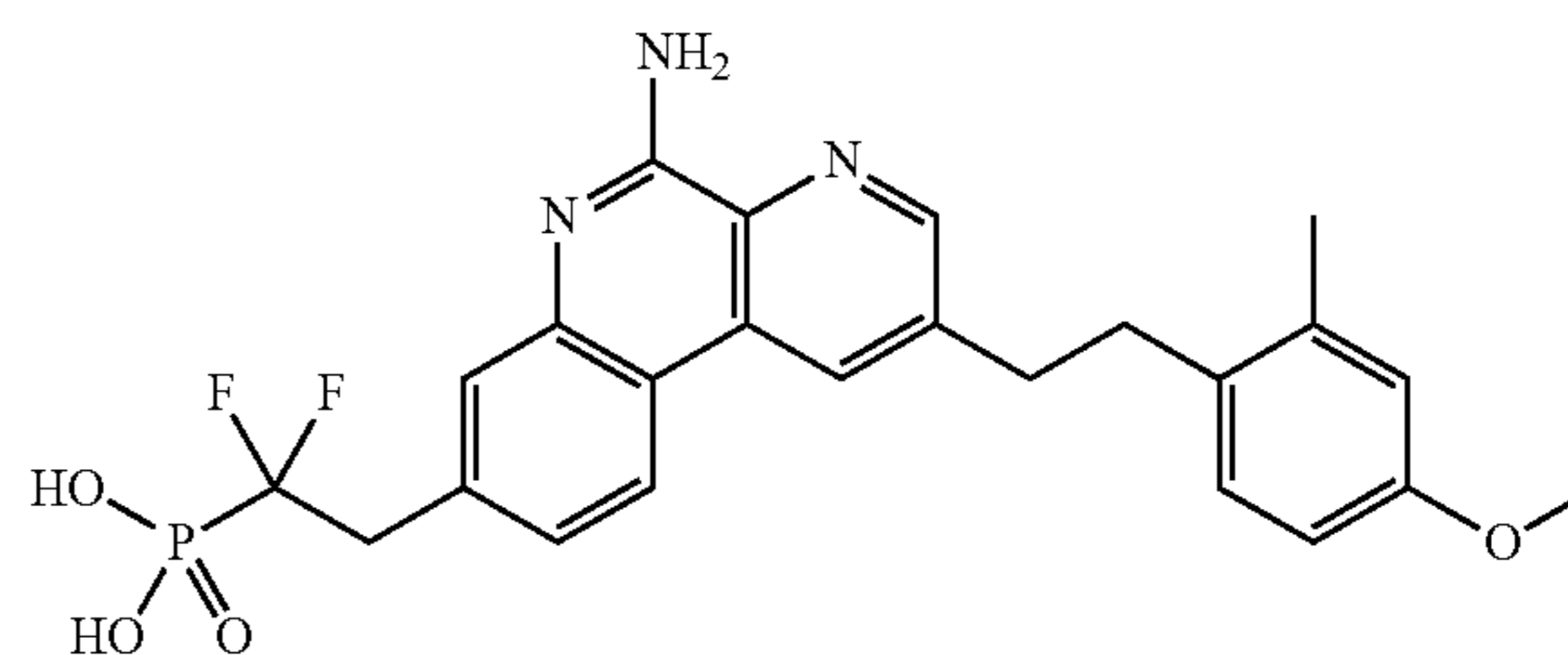
(2-(5-amino-2-(4-methoxy-2-methylphenethyl)benzo[f][1,7]naphthyridin-8-yl)-1,1-difluoroethyl)phosphonic acid
