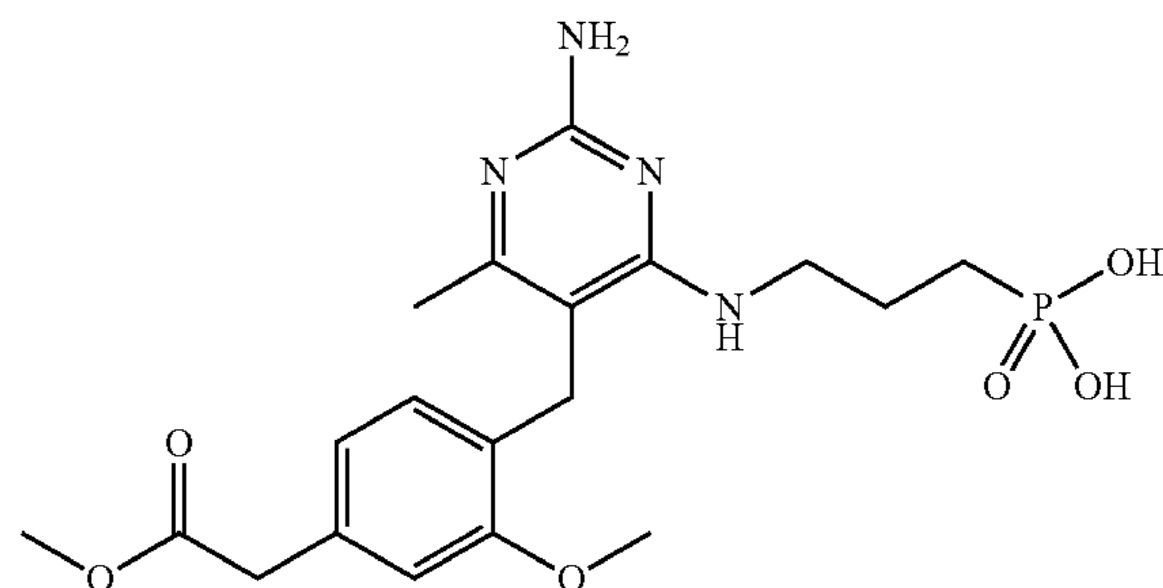
(3-((2-amino-5-(2-methoxy-4-(2-methoxy-2-oxoethyl)benzyl)-6-methylpyrimidin-4-yl)amino)propyl)phosphonic acid
