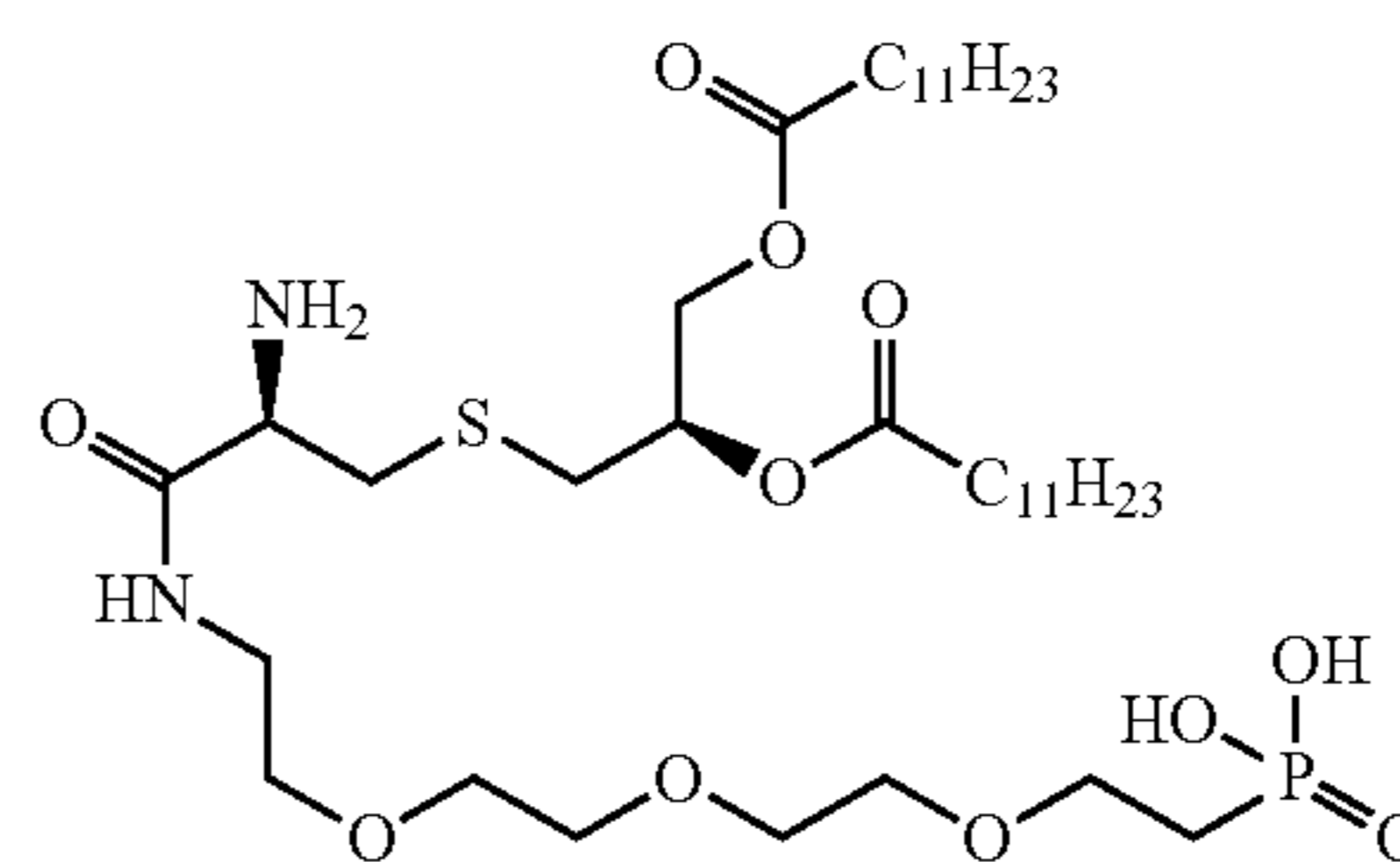
((14R,18R)-14-amino-18-(dodecanoyloxy)-13,21-dioxo-3,6,9,20-tetraoxa-16-thia-12-azadotriacontyl)phosphonic acid
