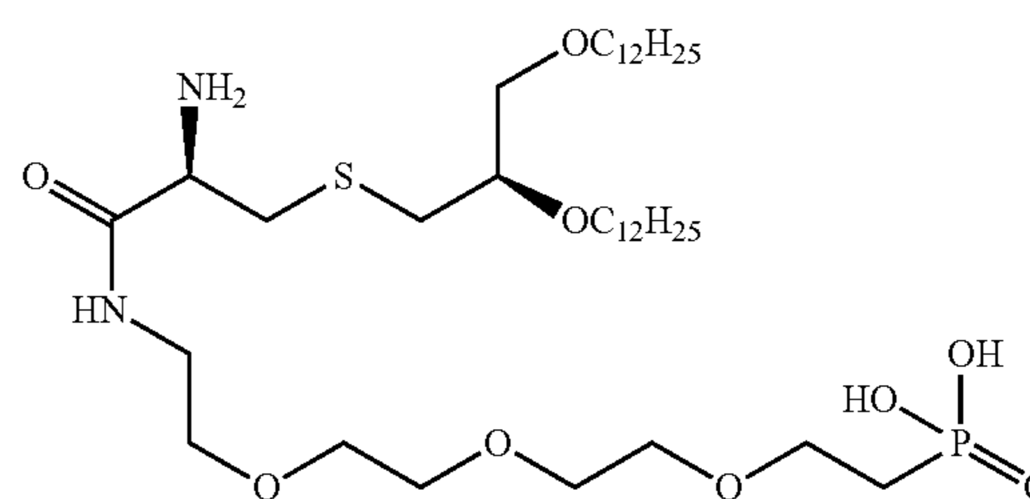
((14R,18R)-14-amino-18-(dodecyloxy)-13-oxo-3,6,9,20-tetraoxa-16-thia-12-azadotriacontyl)phosphonic acid
