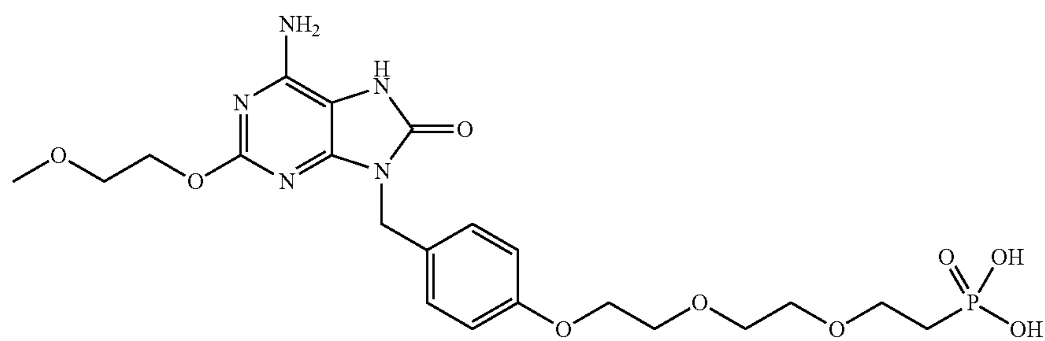
(2-(2-(2-(4-((6-amino-2-(2-methoxyethoxy)-8-oxo-7H-purin-9(8H)-yl)methyl)phenoxy)ethoxy)ethoxy)ethyl)phosphonic acid
