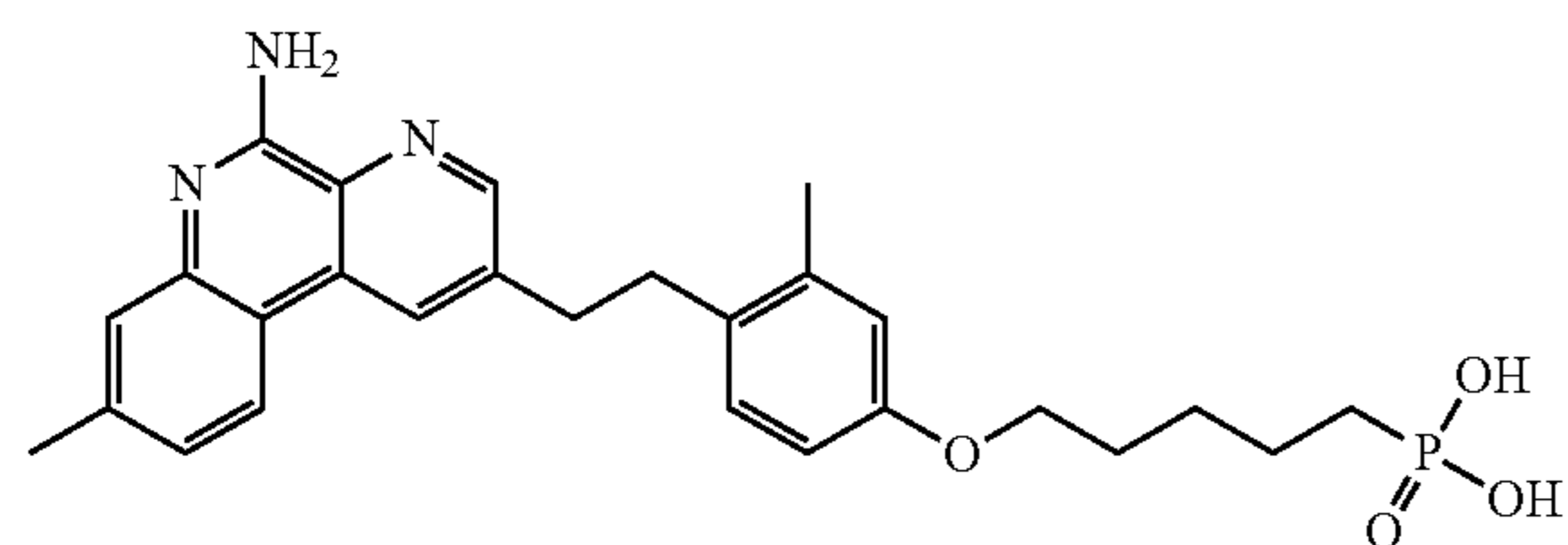
(5-(4-(2-(5-amino-8-methylbenzo[f][1,7]naphthyridin-2-yl)ethyl)-3-methylphenoxy)pentyl)phosphonic acid
