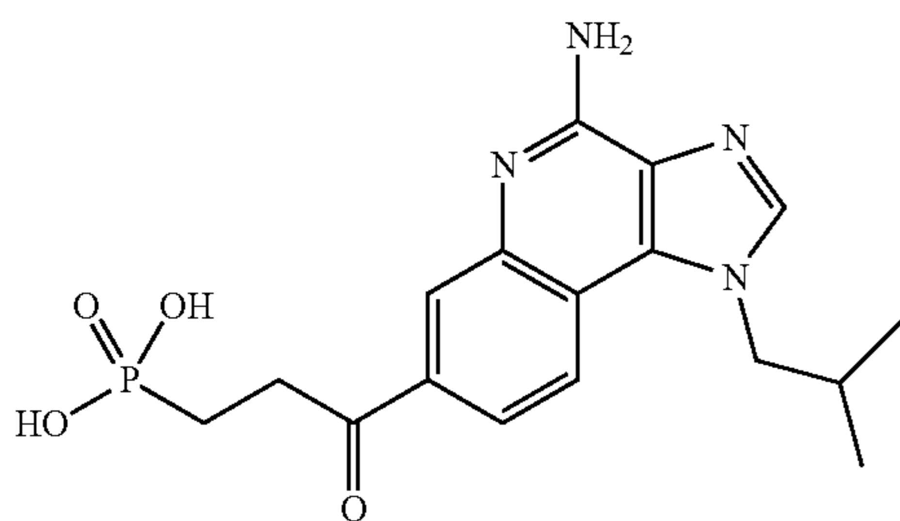
(3-(4-amino-1-isobutyl-1H-imidazo[4,5-c]quinolin-7-yl)oxopropyl)phosphonic acid
