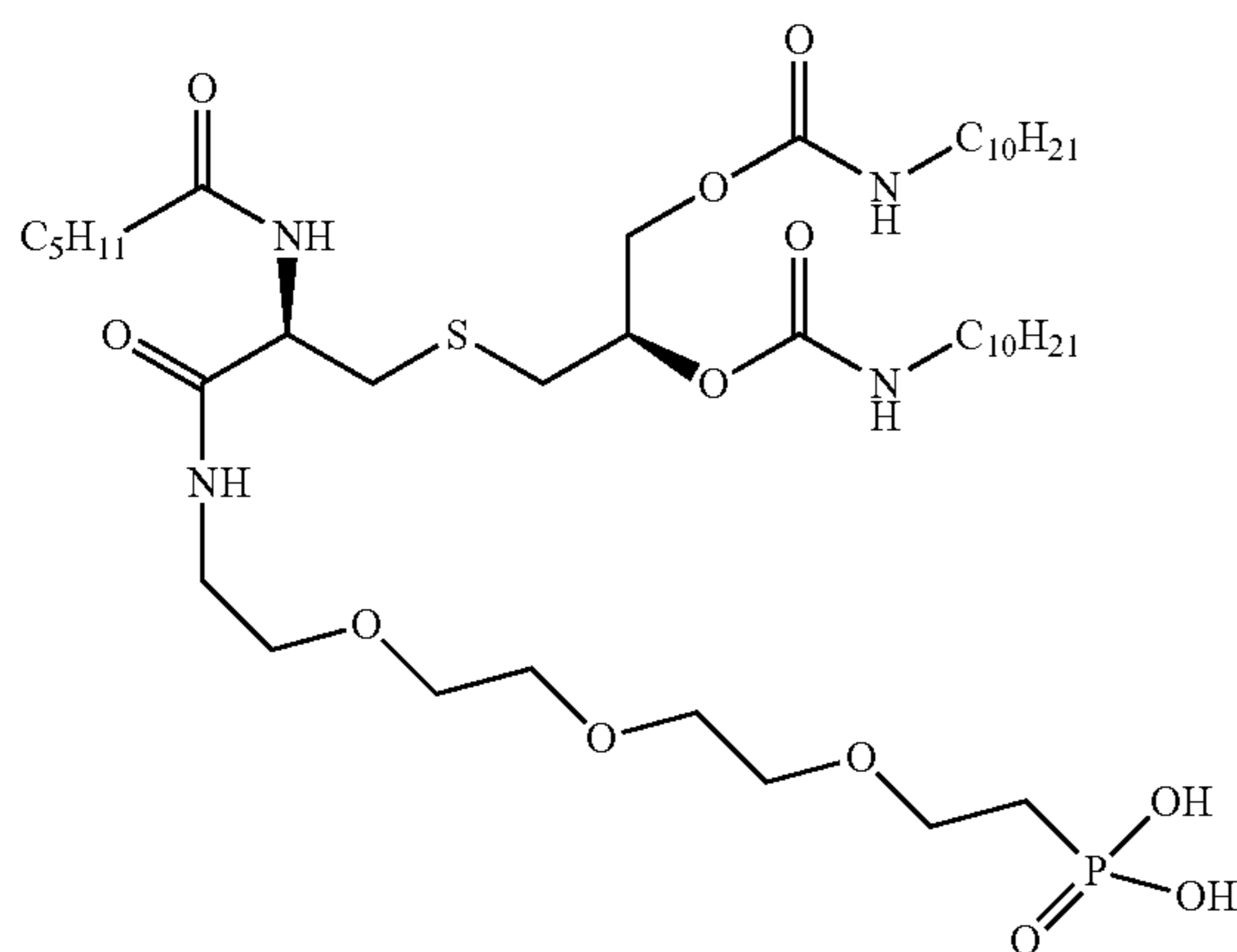
((14R,18R)-18-((decylcarbamoyl)oxy)-14-hexanamido-13,21-dioxo-3,6,9,20-tetraoxa-16-thia-12,22-diazadotriacontyl)phosphonic acid
