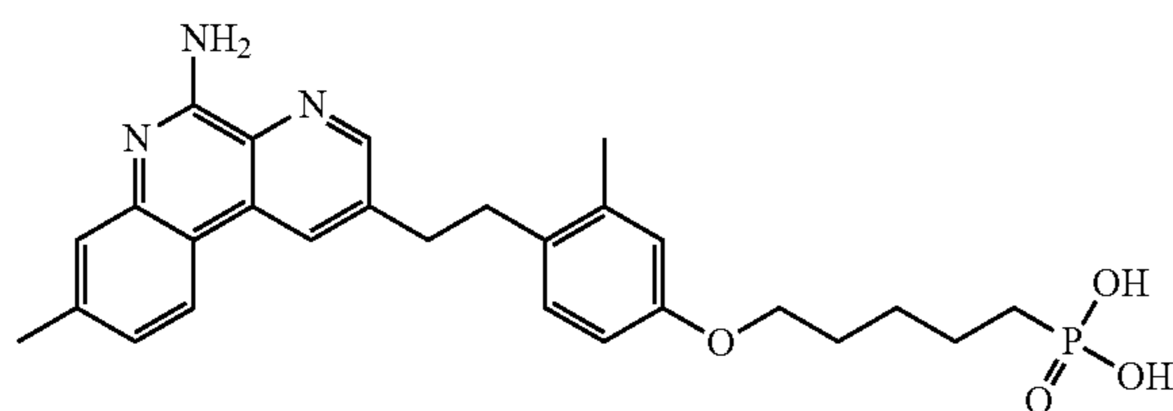
(5-(4-(2-(5-amino-8-methylbenzo[f][1,7]naphthyridin-2-yl)ethyl)-3-methylphenoxy)pentyl)phosphonic acid
