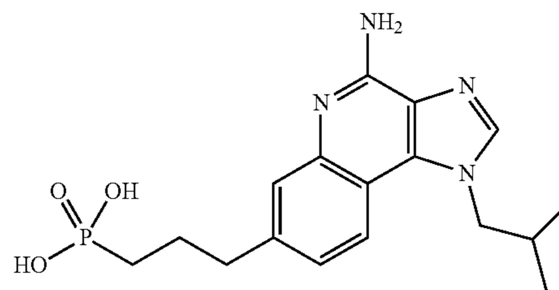
(3-(4-amino-1-isobutyl-1H-imidazo[4,5-c]quinolin-7-yl)propyl)phosphonic acid
