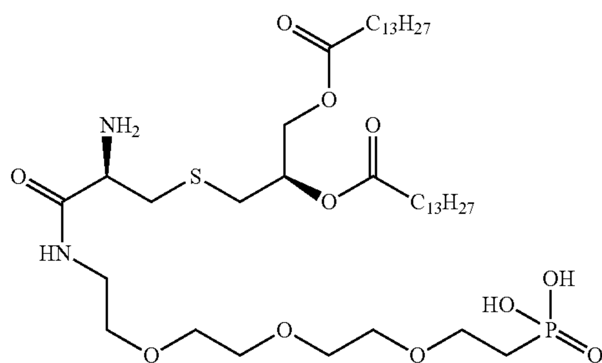
((14R,18R)-14-amino-13,21-dioxo-18-(tetradecanoyloxy)-3,6,9,20-tetraoxa-16-thia-12-azatetraacetyl)phosphonic acid
