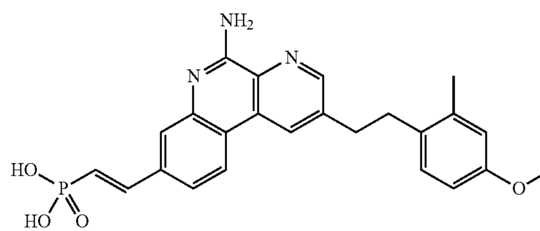
(E)-2-(5-amino-2-(4-methoxy-2-methylphenethyl)benzo[f][1,7]naphthyridin-8-yl)vinyl phosphonic acid
