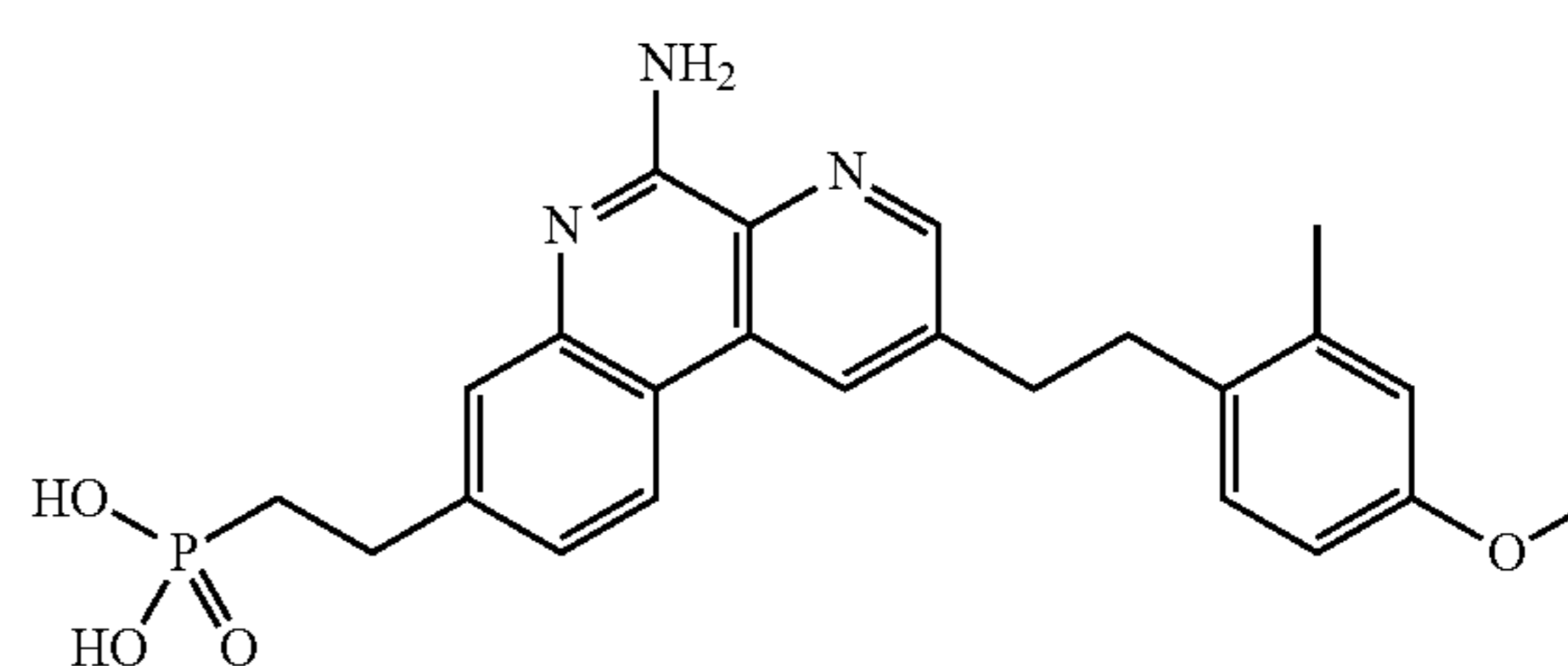
(2-(5-amino-2-(4-methoxy-2-methylphenethyl)benzo[f][1,7]naphthyridin-8-yl)ethyl)phosphonic acid
