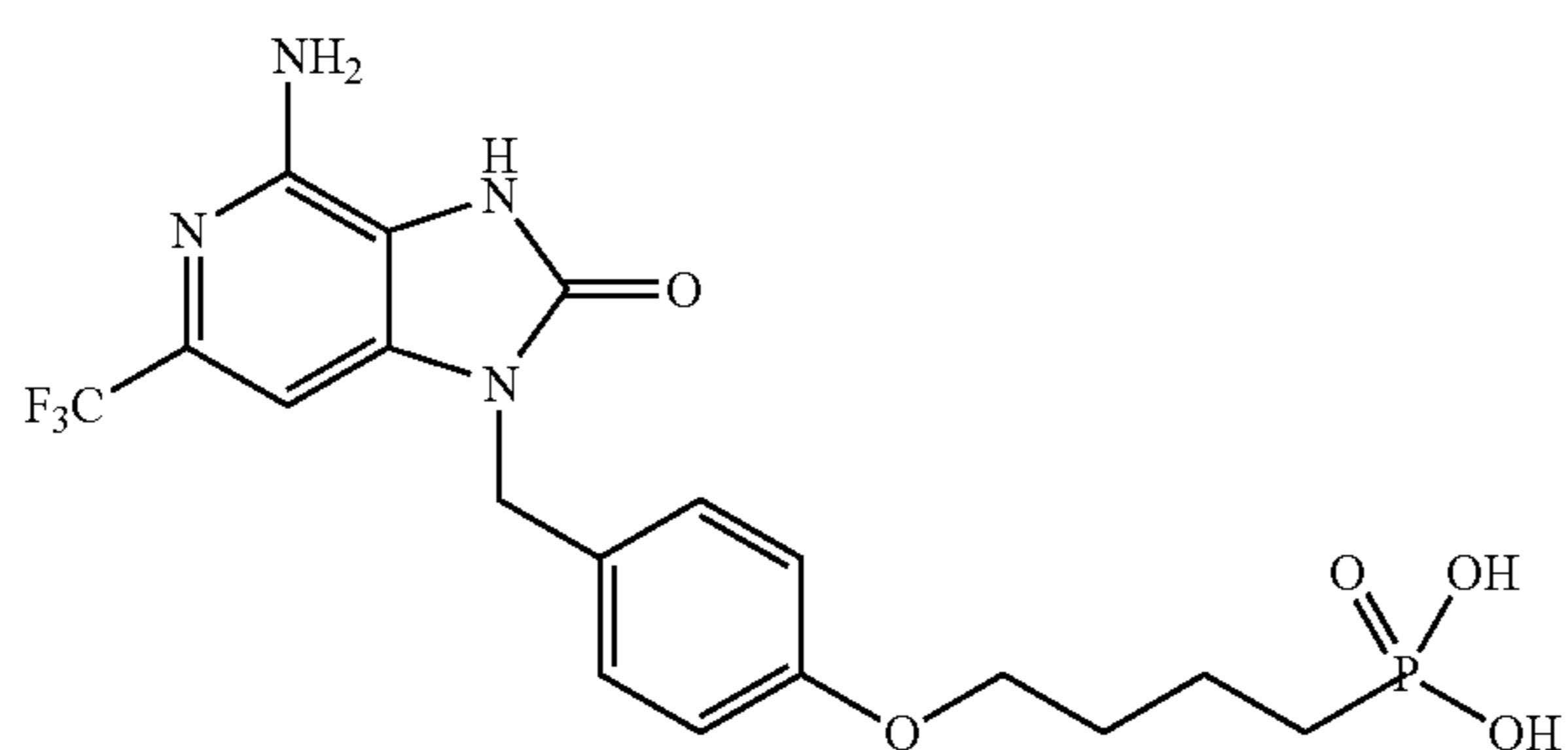
(4-(4-((4-amino-2-oxo-6-(trifluoromethyl)-2,3-dihydro-1H-imidazo[4,5-c]pyridin-1-yl)methyl)phenoxy)butyl)phosphonic acid
