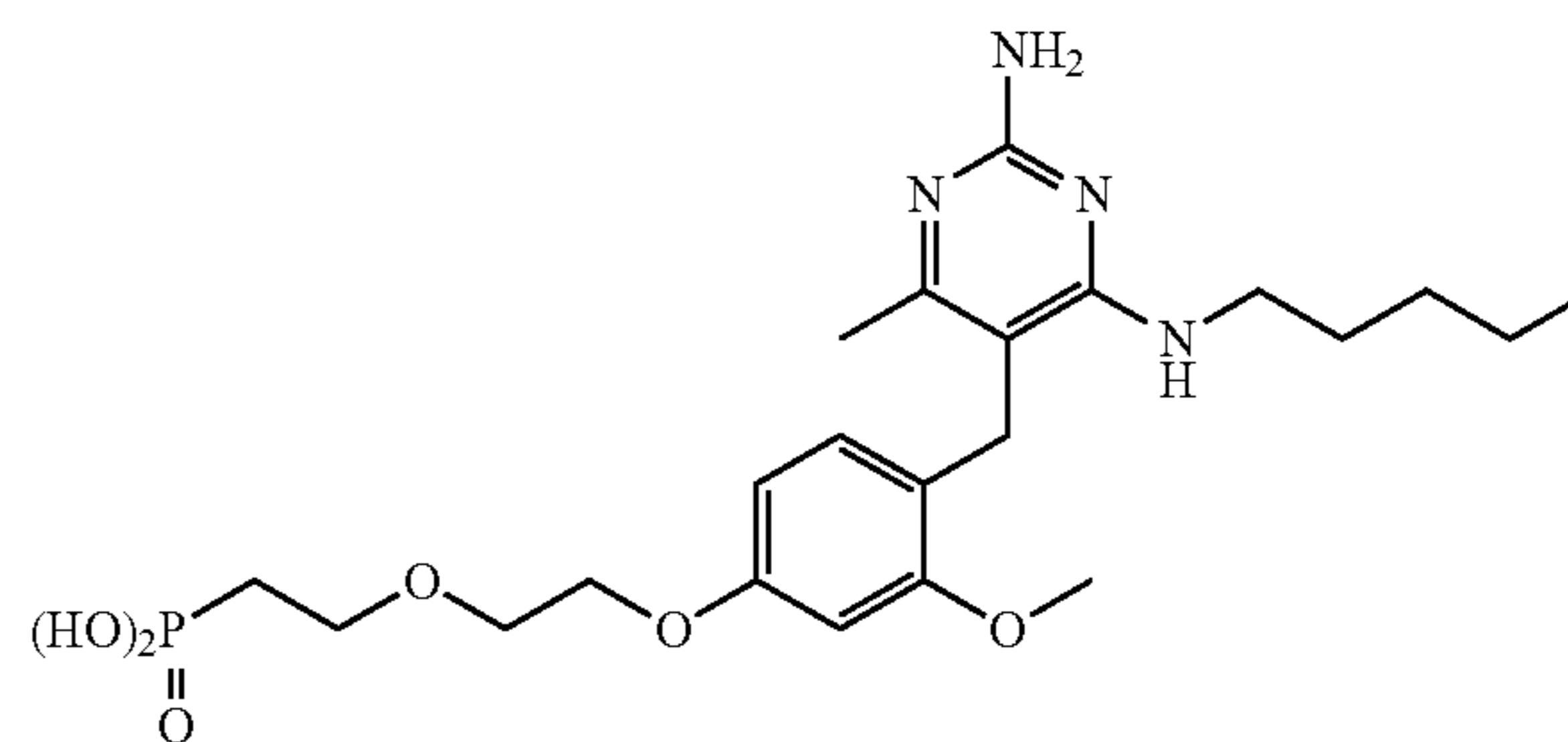
(2-(2-(4-((2-amino-4-methyl-6-(pentylamino)pyrimidin-5-yl)methyl)-3-methoxyphenoxy)ethoxy)ethyl) phosphonic acid
