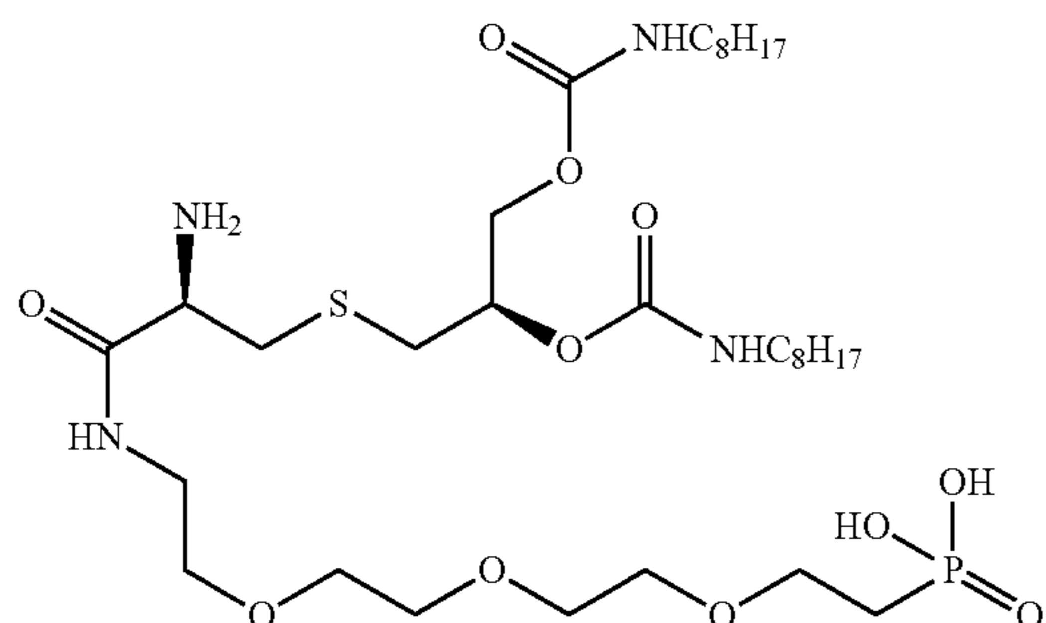
((14R,18R)-14-amino-18-((octylcarbamoyl)oxy)-13,21-dioxo-3,6,9,20-tetraoxa-16-thia-12,22-diazatriacontyl)phosphonic acid
