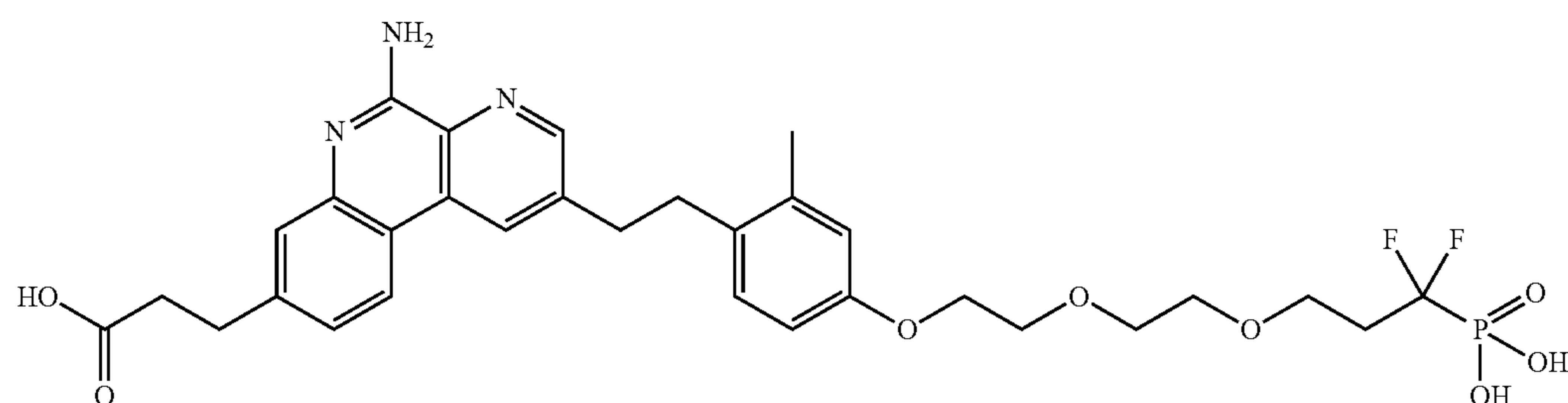
3-(5-amino-2-(4-(2-(2-(3,3-difluoro-3-phosphonopropoxy)ethoxy)ethoxy)-2-methylphenethyl)benzo[f][1,7]naphthyridin-8-yl)propanoic acid
