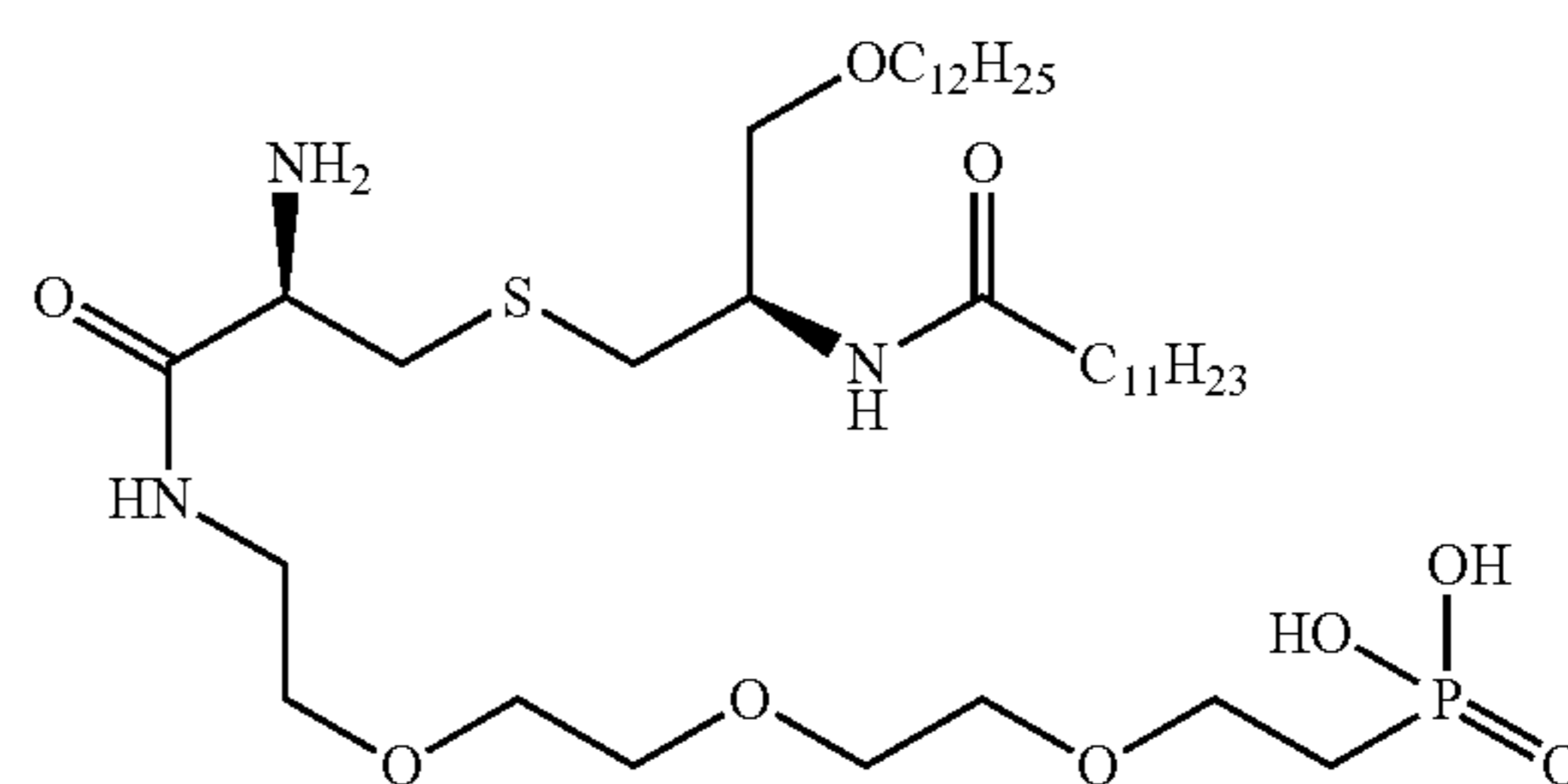
((14R,18R)-14-amino-18-dodecanamido-13-oxo-3,6,9,20-tetraoxa-16-thia-12-azadotriacontyl)phosphonic acid
