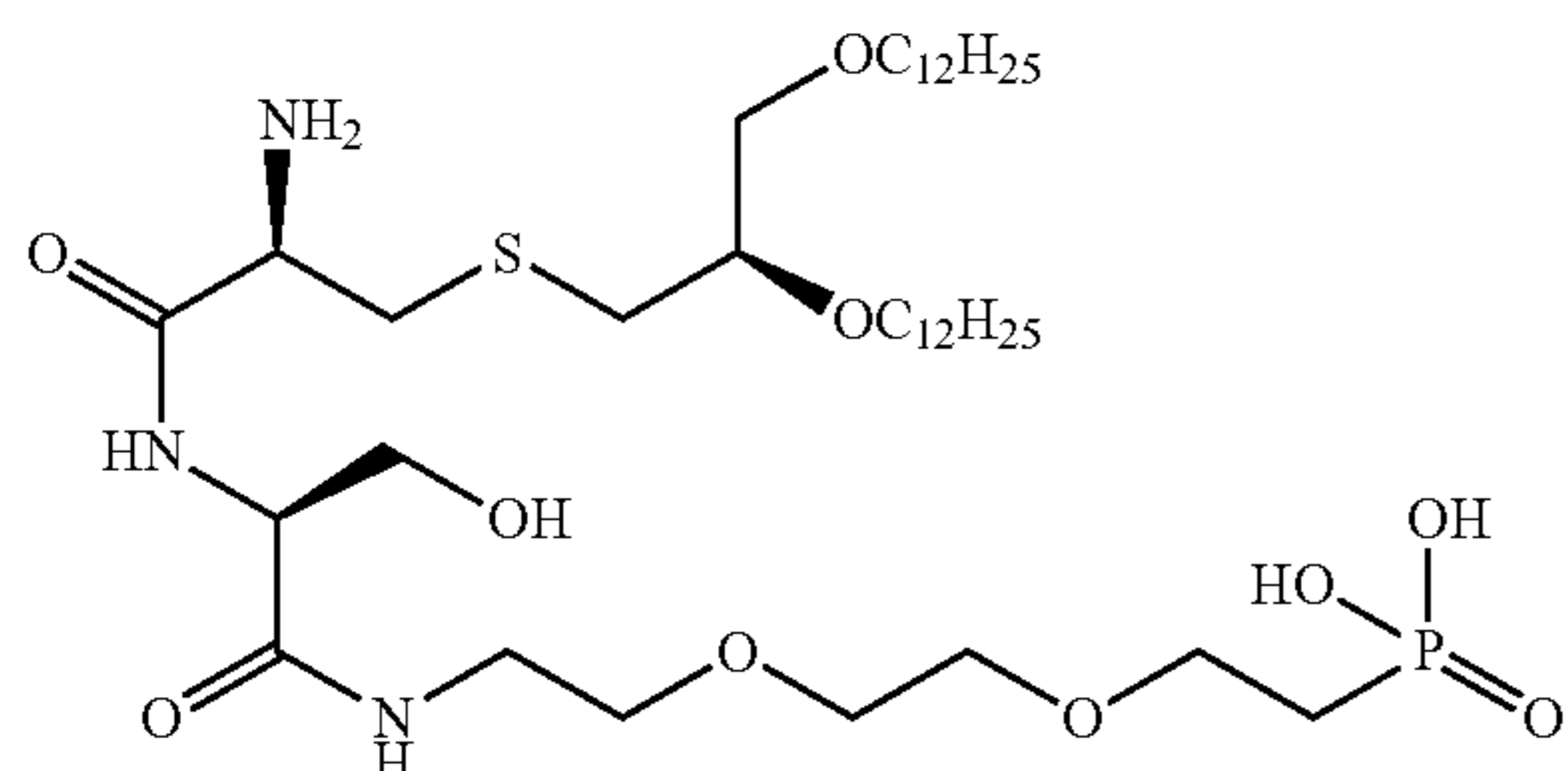
((11S,14R,18R)-14-amino-18-(dodecyloxy)-11-(hydroxymethyl)-10,13-dioxo-3,6,20-trioxa-16-thia-9,12-diazadotriacontyl)phosphonic acid
