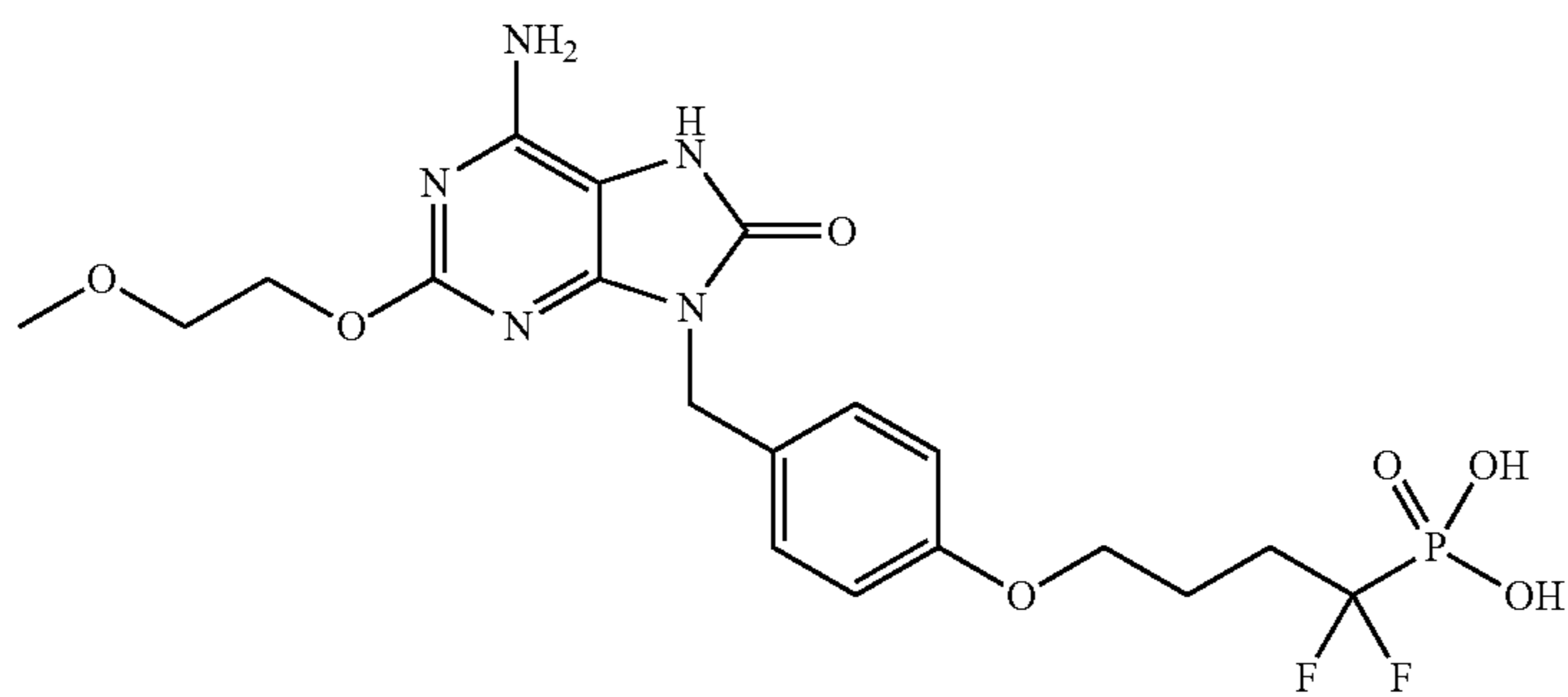
(4-(4-((6-amino-2-(2-methoxyethoxy)-8-oxo-7H-purin-9(8H)-yl)methyl)phenoxy)-1,1-difluorobutyl)phosphonic acid
