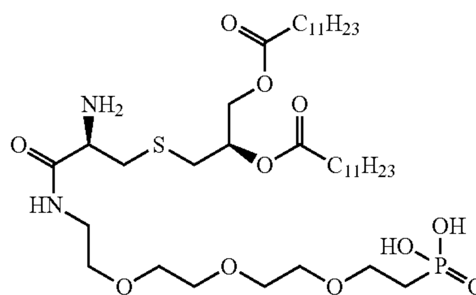
(14R,18R)-14-amino-18-(dodecanoyloxy)-13,21-dioxo-3,6,9,20-tetraoxa-16-thia-12-azadotriacontyl)phosphonic acid
