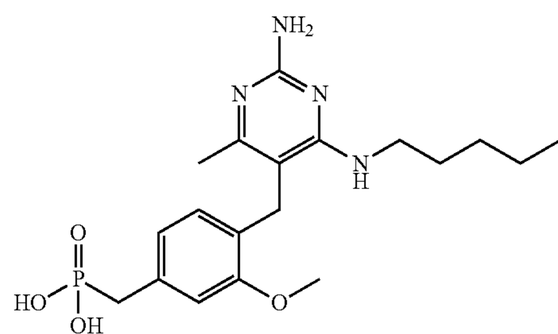
4-((2-amino-4-methyl-6-(pentylamino)pyrimidin-5-yl)methyl)-3-methoxybenzyl phosphonic acid
