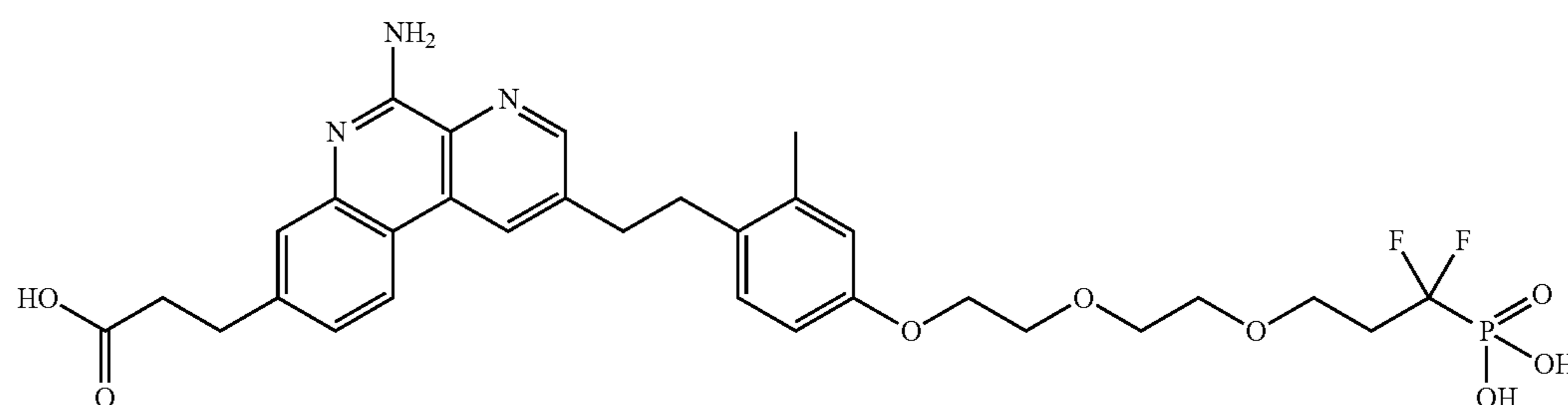
3-(5-amino-2-(4-(2-(2-(3,3-difluoro-3-phosphonopropoxy)ethoxy)ethoxy)-2-methylphenethyl)benzo[f][1,7]naphthyridin-8-yl)propanoic acid
