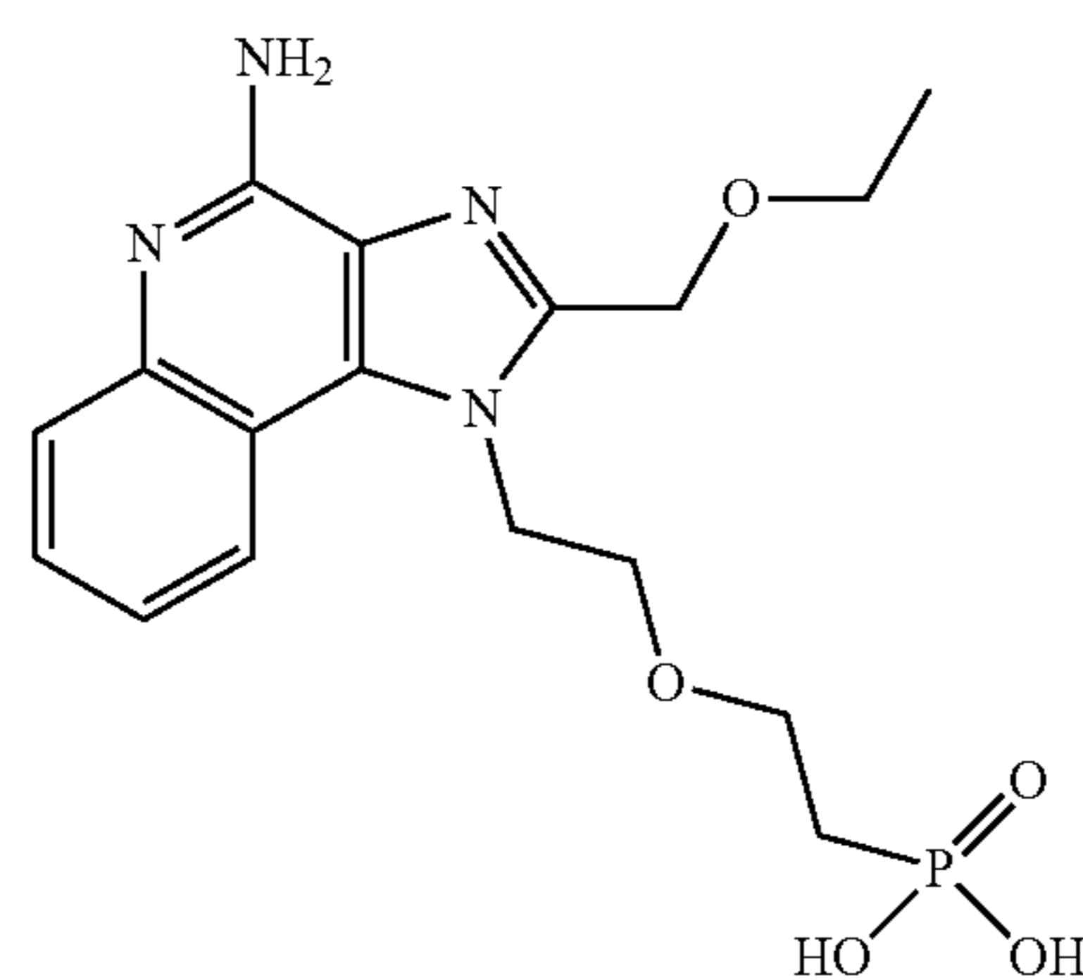
2-(2-(4-amino-2-(ethoxymethyl)-1H-imidazo[4,5-c]quinolin-1-yl)ethoxy)ethyl phosphonic acid
