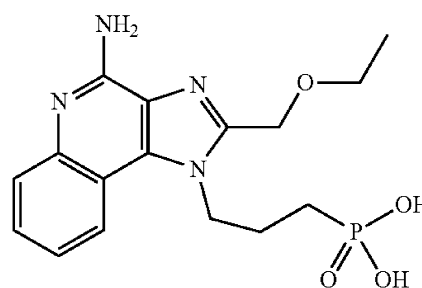
(3-(4-amino-2-(ethoxymethyl)-1H-imidazo[4,5-c]quinolin-1-yl)propyl)phosphonic acid
