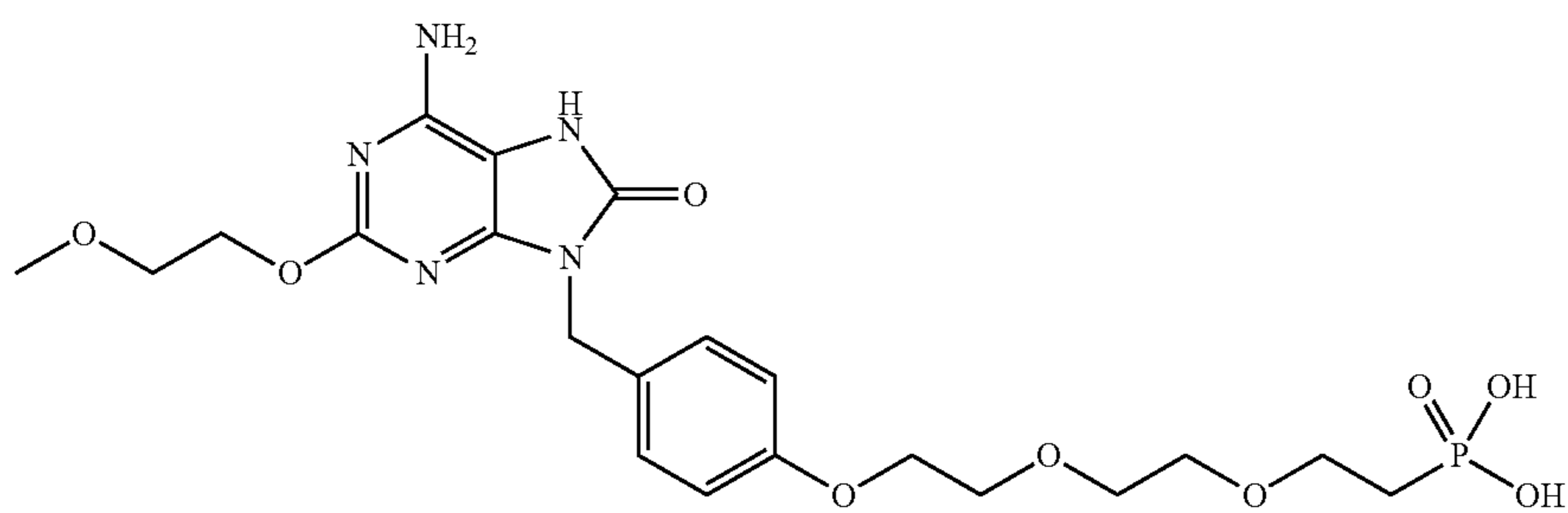
(2-(2-(2-(4-((6-amino-2-(2-methoxyethoxy)-8-oxo-7H-purin-9(8H)-yl)methyl)phenoxy)ethoxy)ethoxy)ethyl)phosphonic acid
