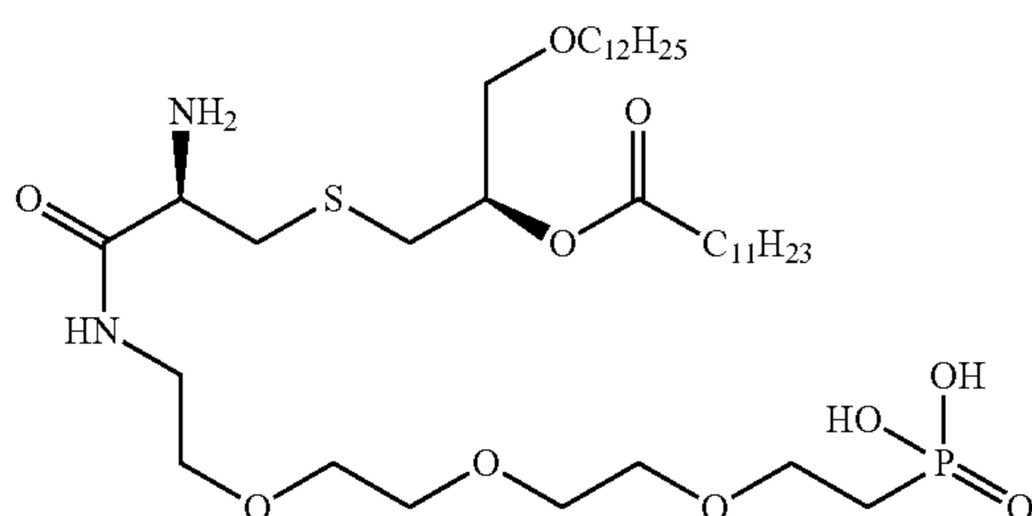
((14R,18R)-14-amino-18-(dodecanoyloxy)-13-oxo-3,6,9,20-tetraoxa-16-thia-12-azatriacontyl)phosphonic acid
