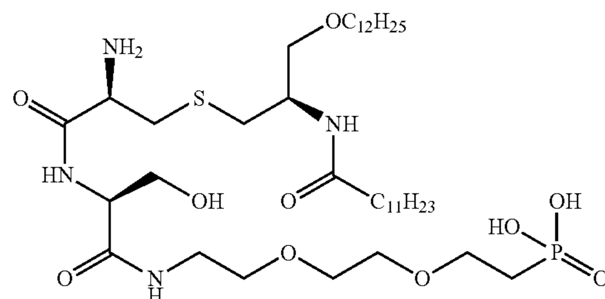
((11S,14R,18R)-14-amino-18-dodecanamido-11-(hydroxymethyl)-10,13-dioxo-3,6,20-trioxa-16-thia-9,12-diazadotriacontyl)phosphonic acid
