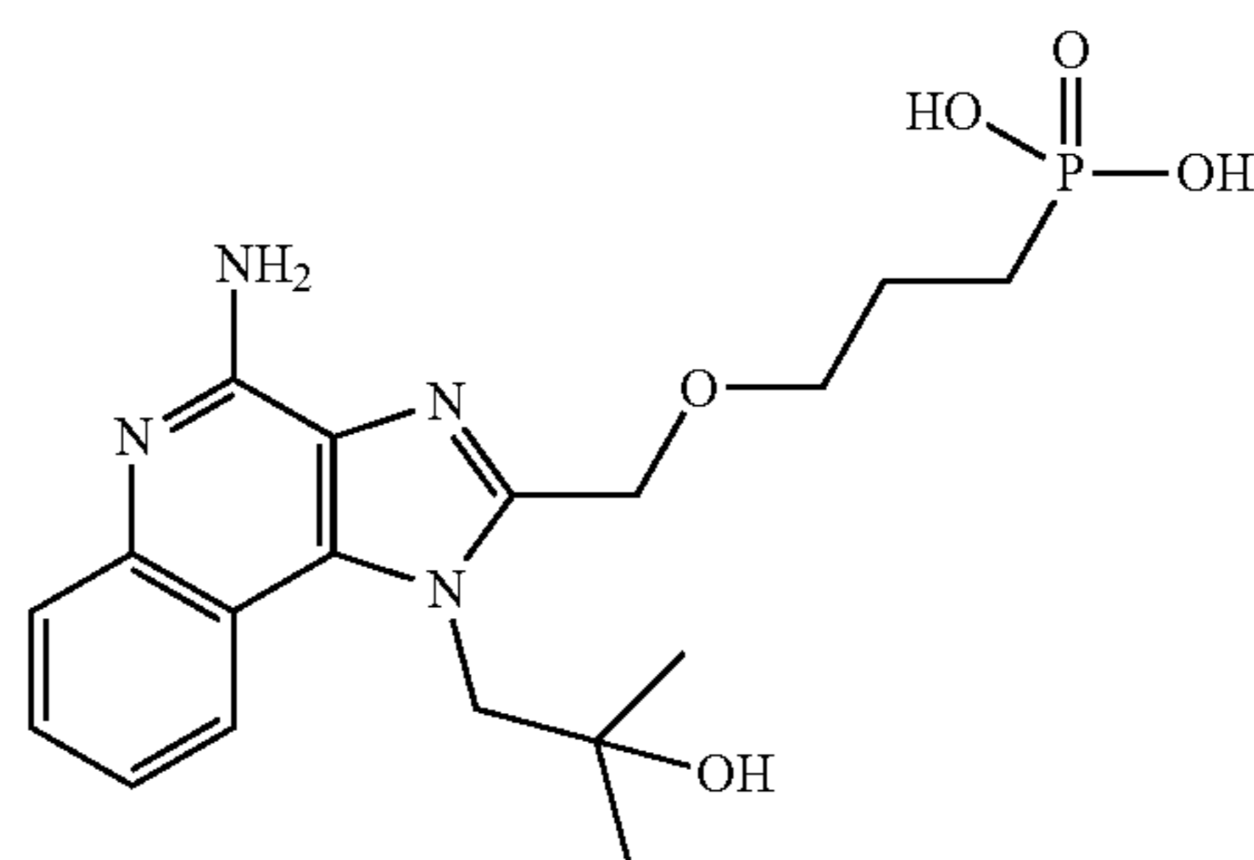
(3-((4-amino-1-(2-hydroxy-2-methylpropyl)-1H-imidazo[4,5-c]quinolin-2-yl)methoxy)propyl)phosphonic acid
