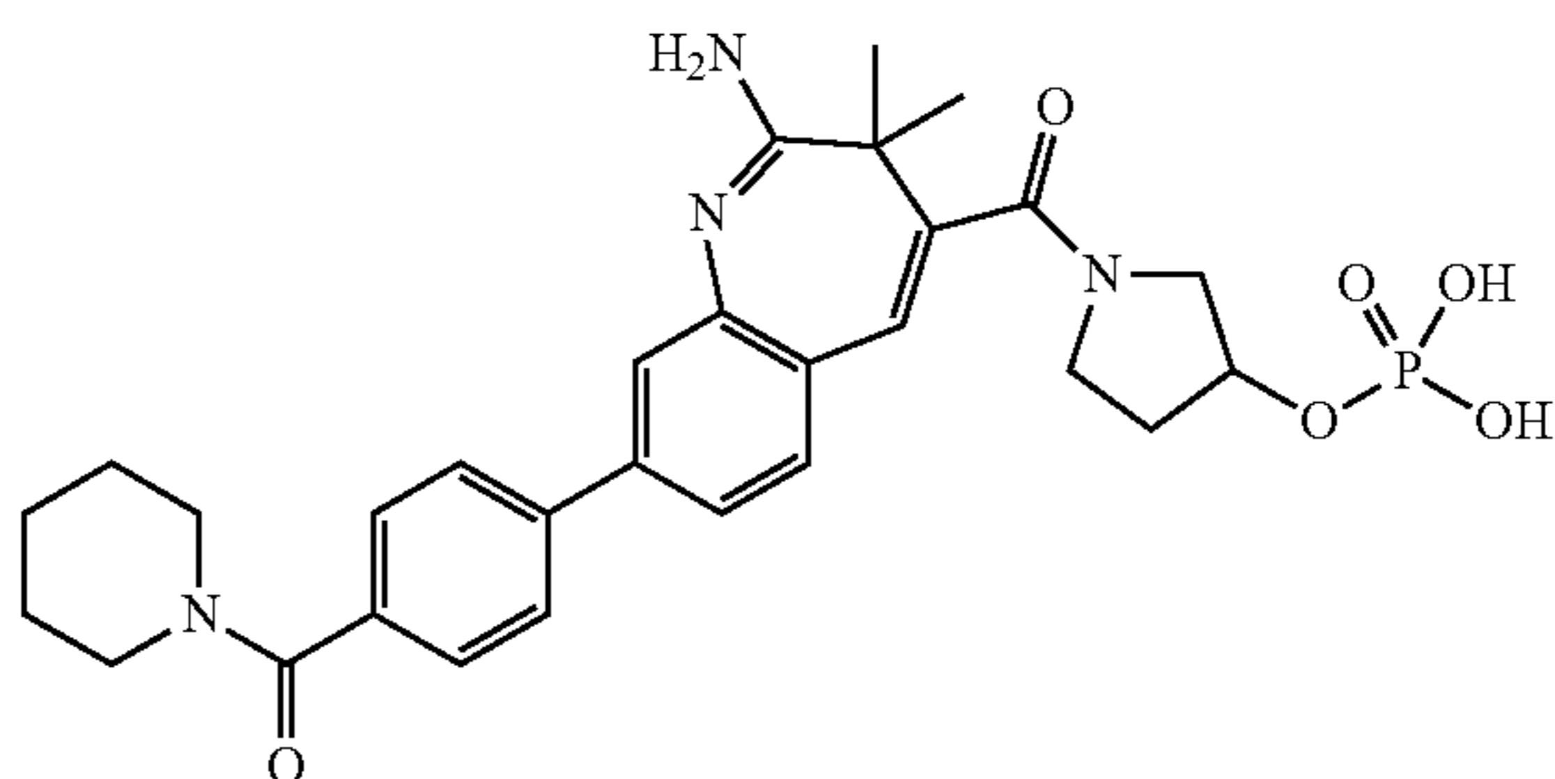
1-(2-amino-3,3-dimethyl-8-(4-(piperidine-1-carbonyl)phenyl)-3H-benzo[b]azepine-4-carbonyl)pyrrolidin-3-yl dihydrogen phosphate
