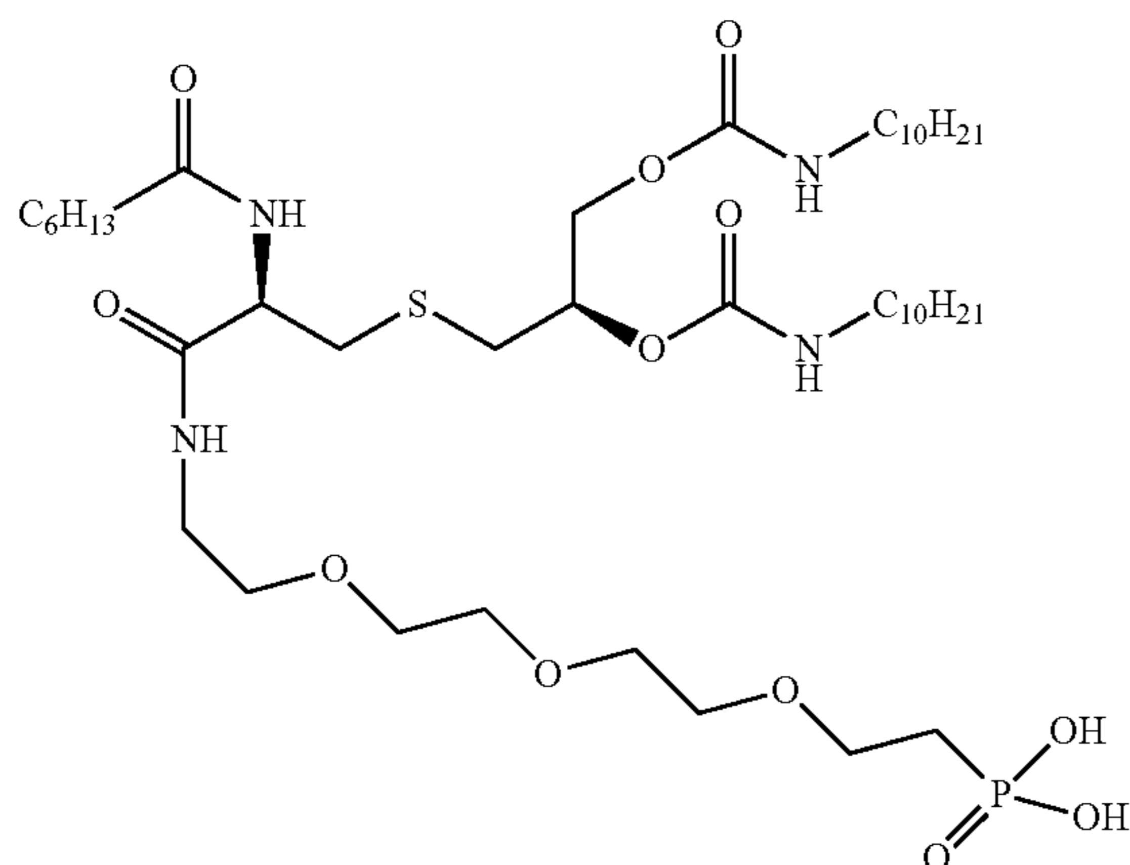
((14R,18R)-18-((decylcarbamoyl)oxy)-14-heptanamido-13,21-dioxo-3,6,9,20-tetraoxa-16-thia-12,22-diazadotriacontyl)phosphonic acid
