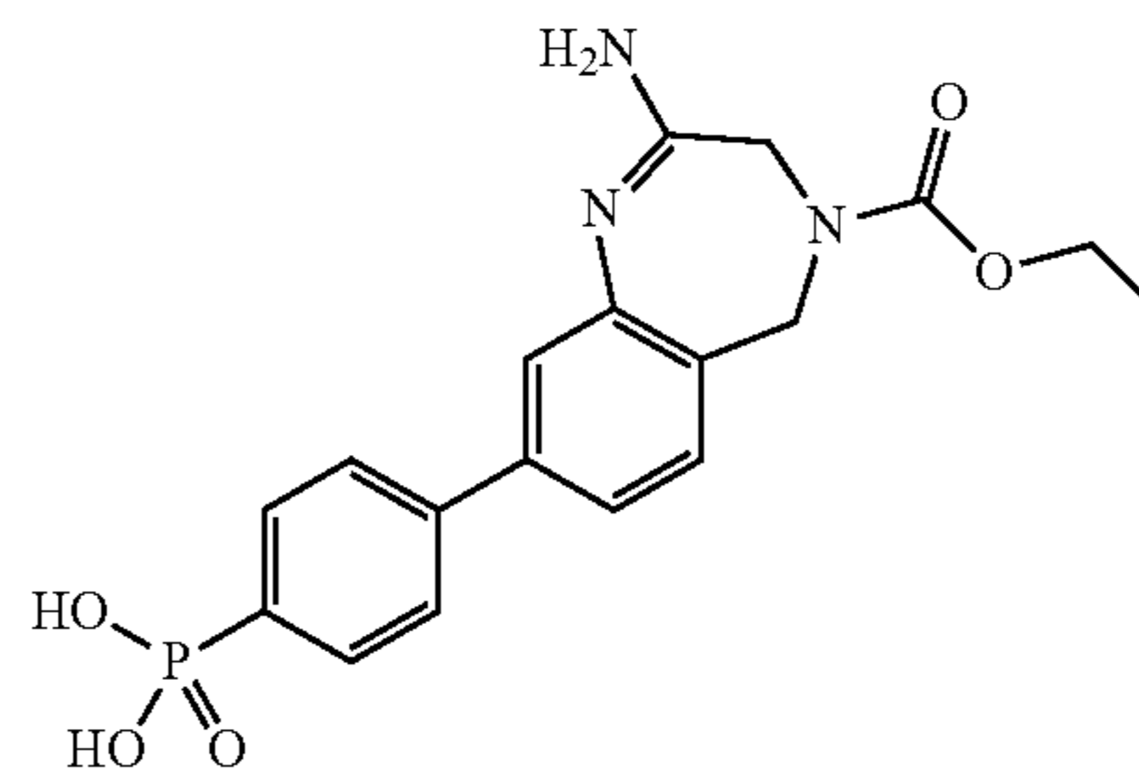
(4-(2-amino-4-(ethoxycarbonyl)-4,5-dihydro-3H-benzo[e][1,4]diazepin-8-yl)phenyl)phosphonic acid
