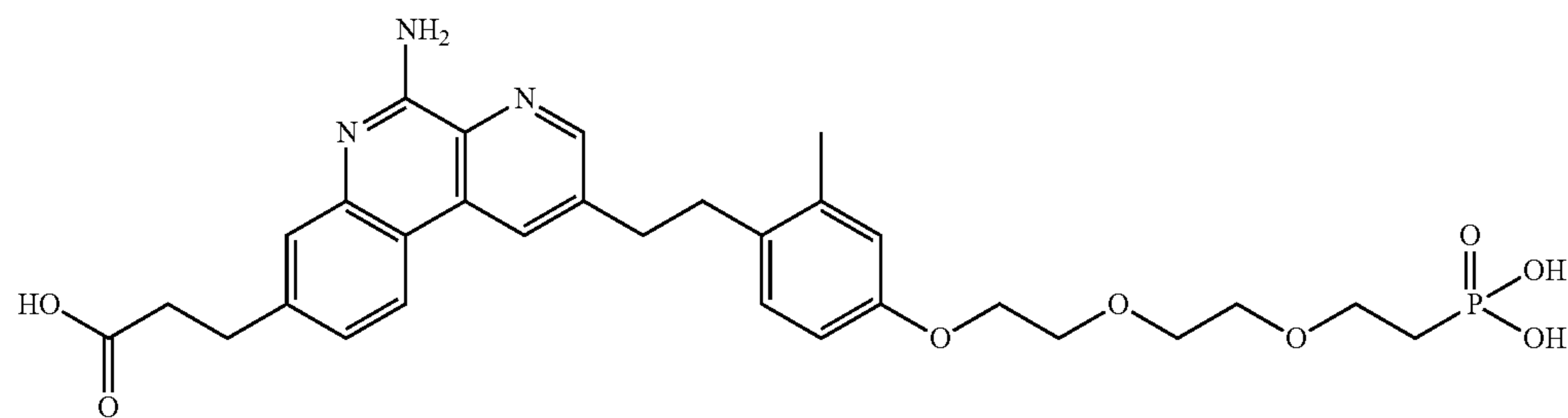
3-(5-amino-2-(2-methyl-4-(2-(2-(2-phosphonoethoxy)ethoxy)ethoxy)phenethyl)benzo[f][1,7]naphthyridin-8-yl)propanoic acid
