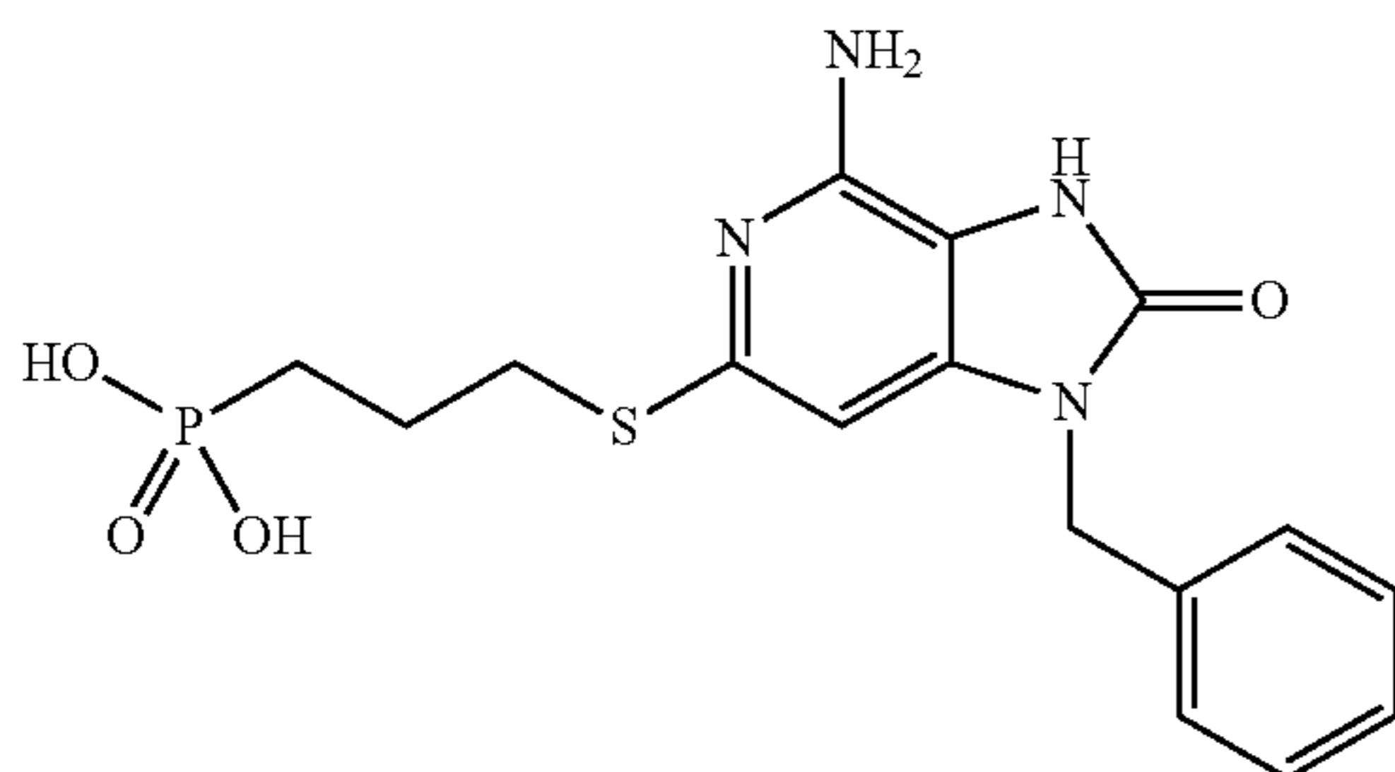
(3-((4-amino-1-benzyl-2-oxo-2,3-dihydro-1H-imidazo[4,5-c]pyridin-6-yl)thio)propyl) phosphonic acid
