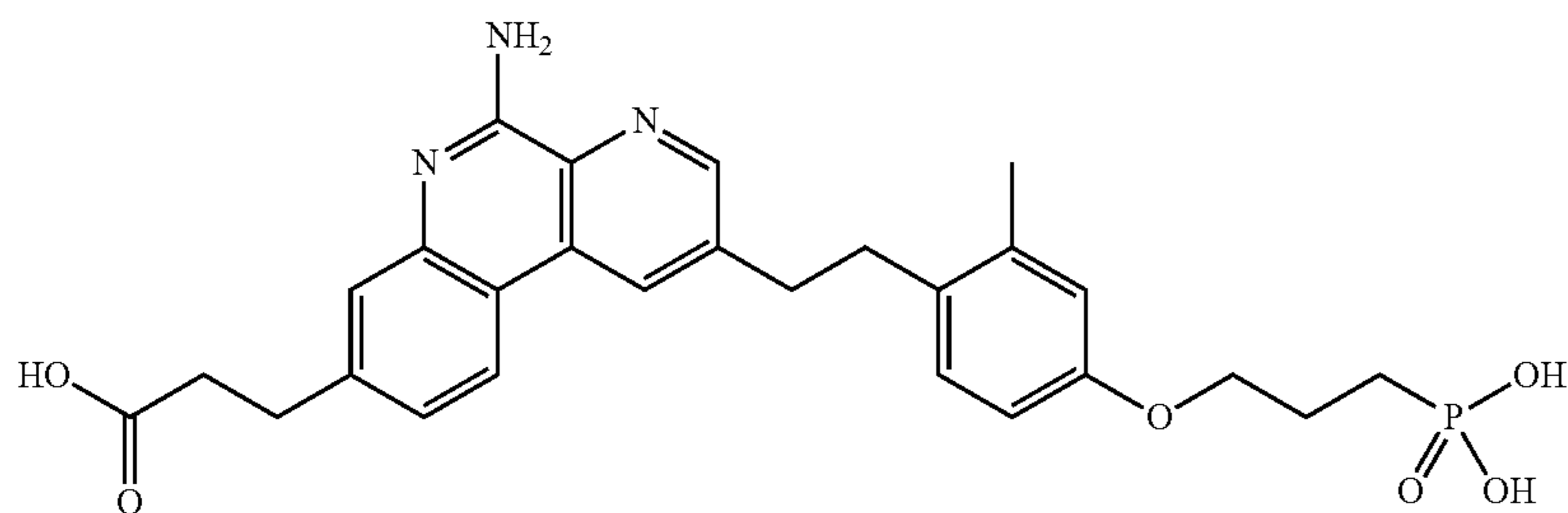
3-(5-amino-2-(2-methyl-4-(3-phosphonopropoxy)phenethyl)benzo[f][1,7]naphthyridin-8-yl)propanoic acid
