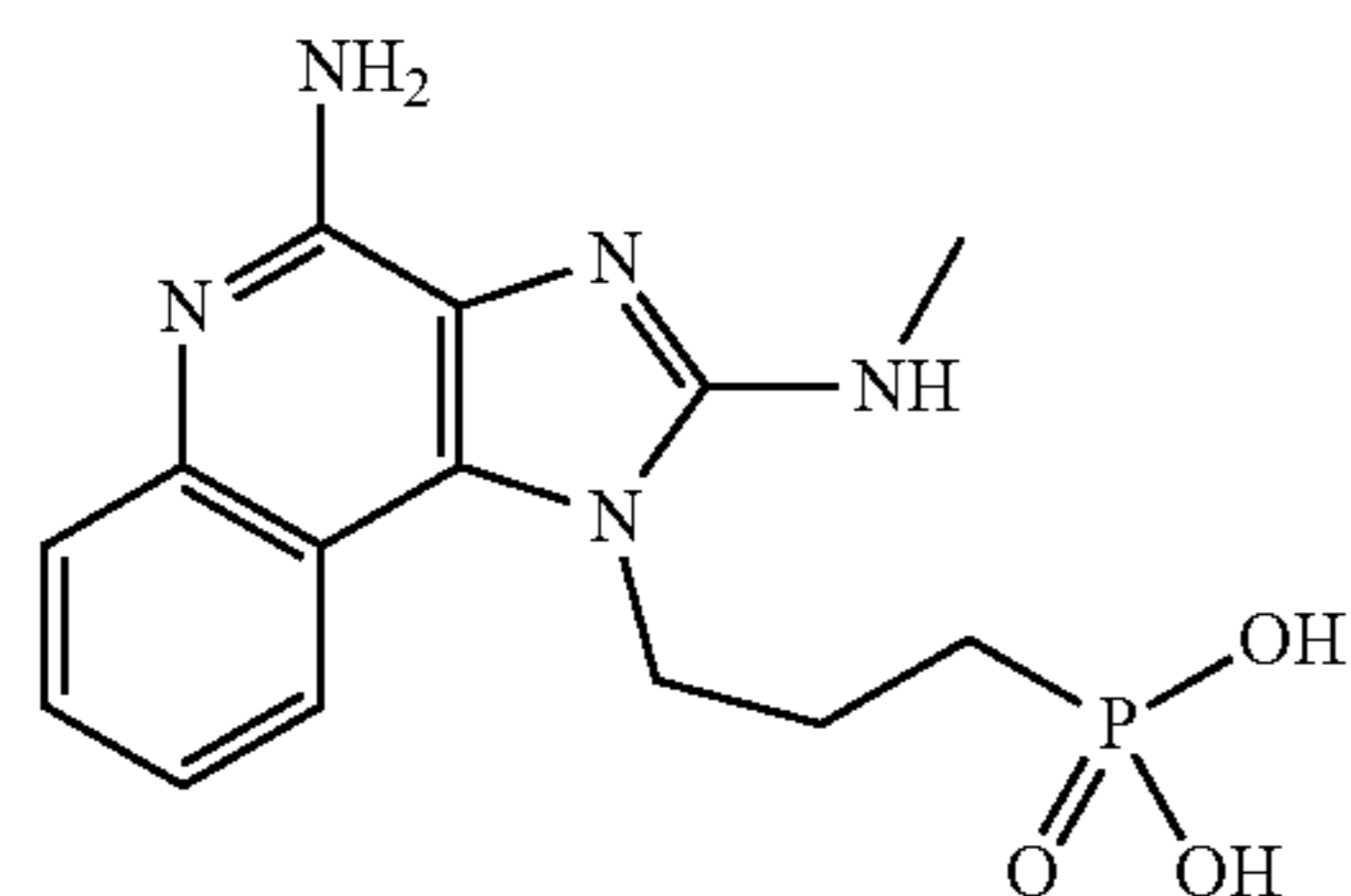
(3-(4-amino-2-(methylamino)-1H-imidazo[4,5-c]quinolin-1-yl)propyl)phosphonic acid
