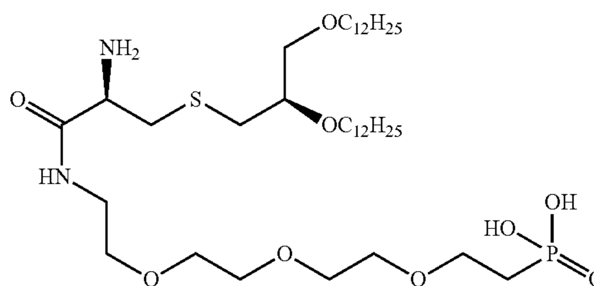
((14R,18R)-14-amino-18-(dodecyloxy)-13-oxo-3,6,9,20-tetraoxa-16-thia-12-azadotriacontyl)phosphonic acid
