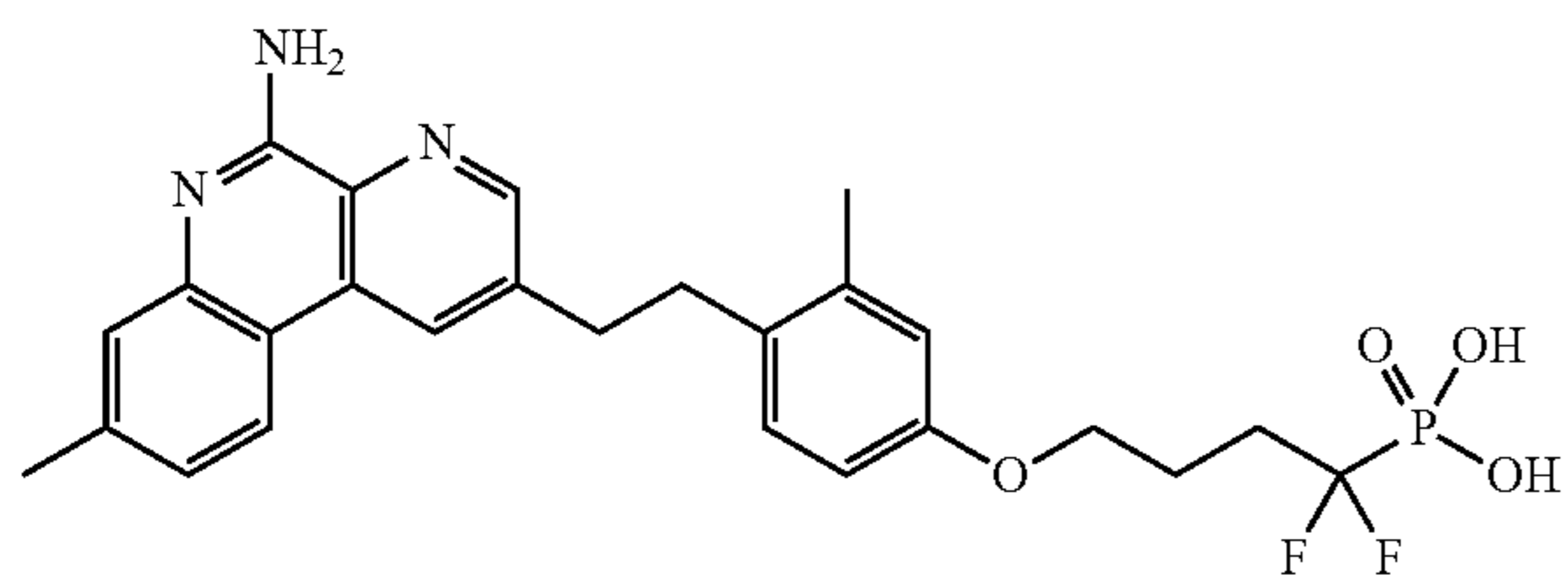
(4-(4-(2-(5-amino-8-methylbenzo[f][1,7]naphthyridin-2-yl)ethyl)-3-methylphenoxy)-1,1-difluorobutyl)phosphonic acid
