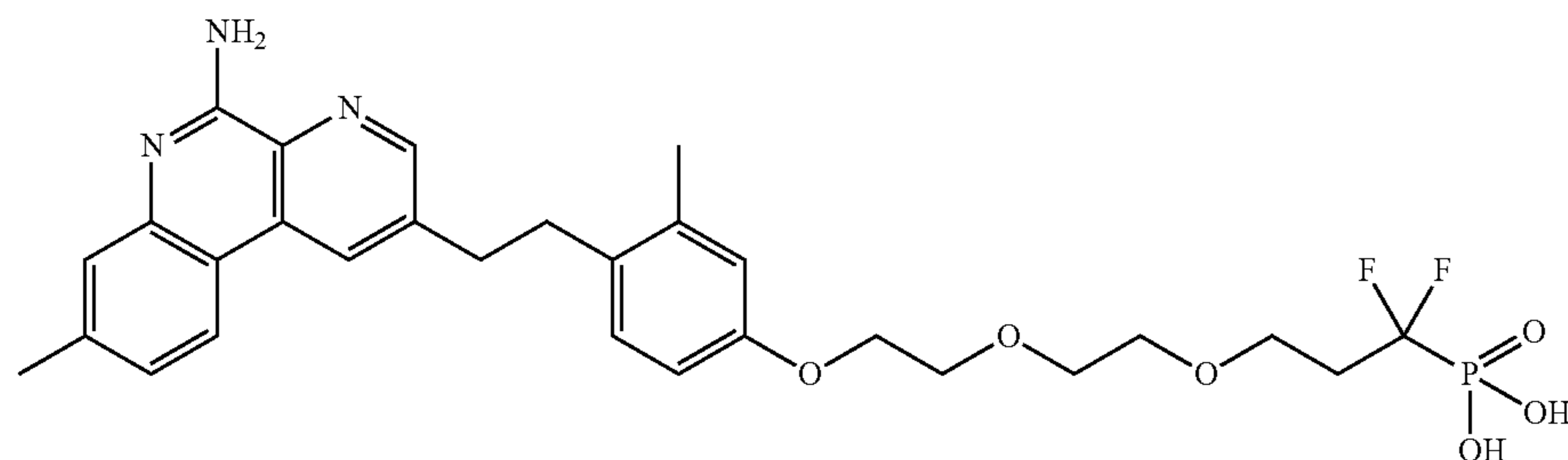
(3-(2-(2-(4-(2-(5-amino-8-methylbenzo[f][1,7]naphthyridin-2-yl)ethyl)-3-methylphenoxy)ethoxy)ethoxy)-1,1-difluoropropyl)phosphonic acid
