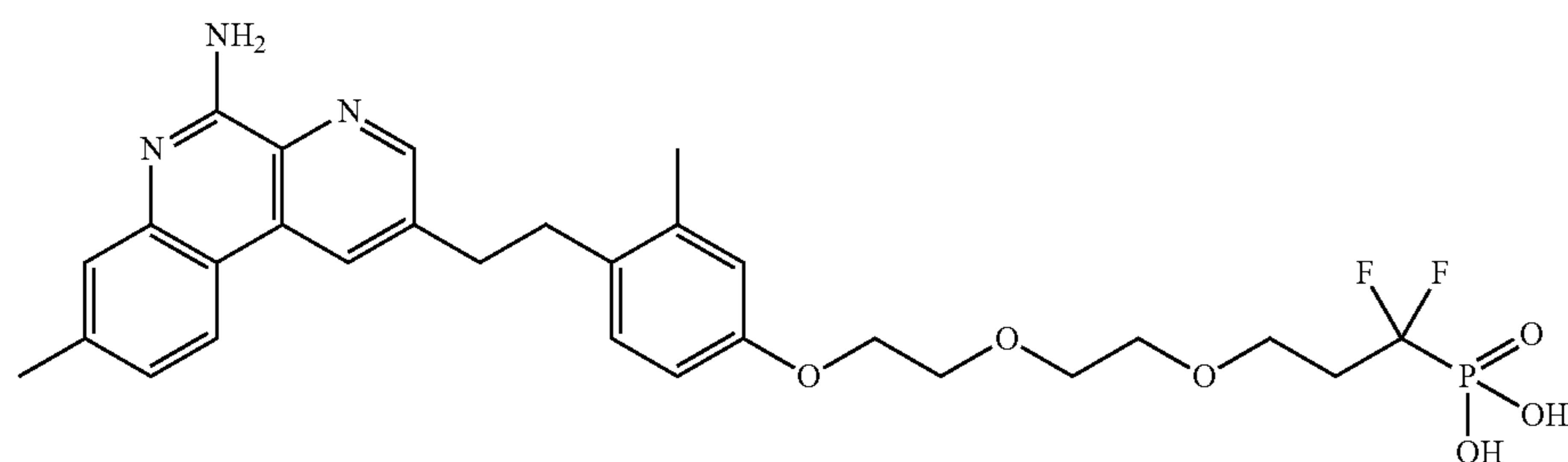
(3-(2-(2-(4-(2-(5-amino-8-methylbenzo[f][1,7]naphthyridin-2-yl)ethyl)-3-methylphenoxy)ethoxy)ethoxy)-1,1-difluoropropyl)phosphonic acid
