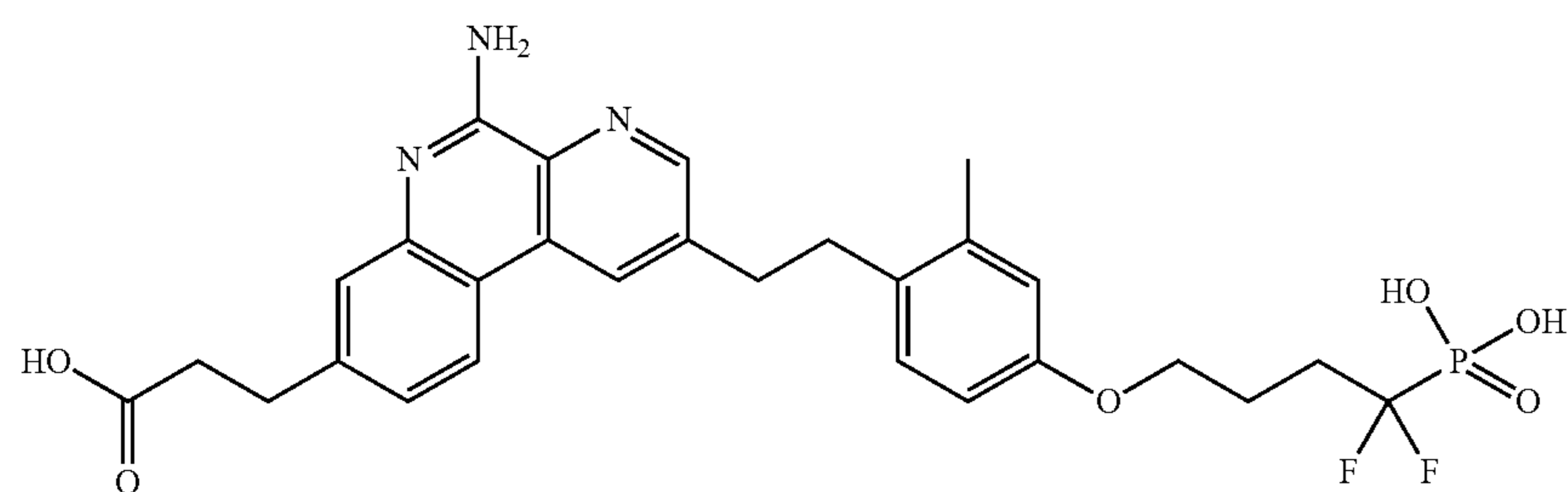
3-(5-amino-2-(4-(4,4-difluoro-4-phosphonobutoxy)-2-methylphenethyl)benzo[f][1,7]naphthyridin-8-yl)propanoic acid
