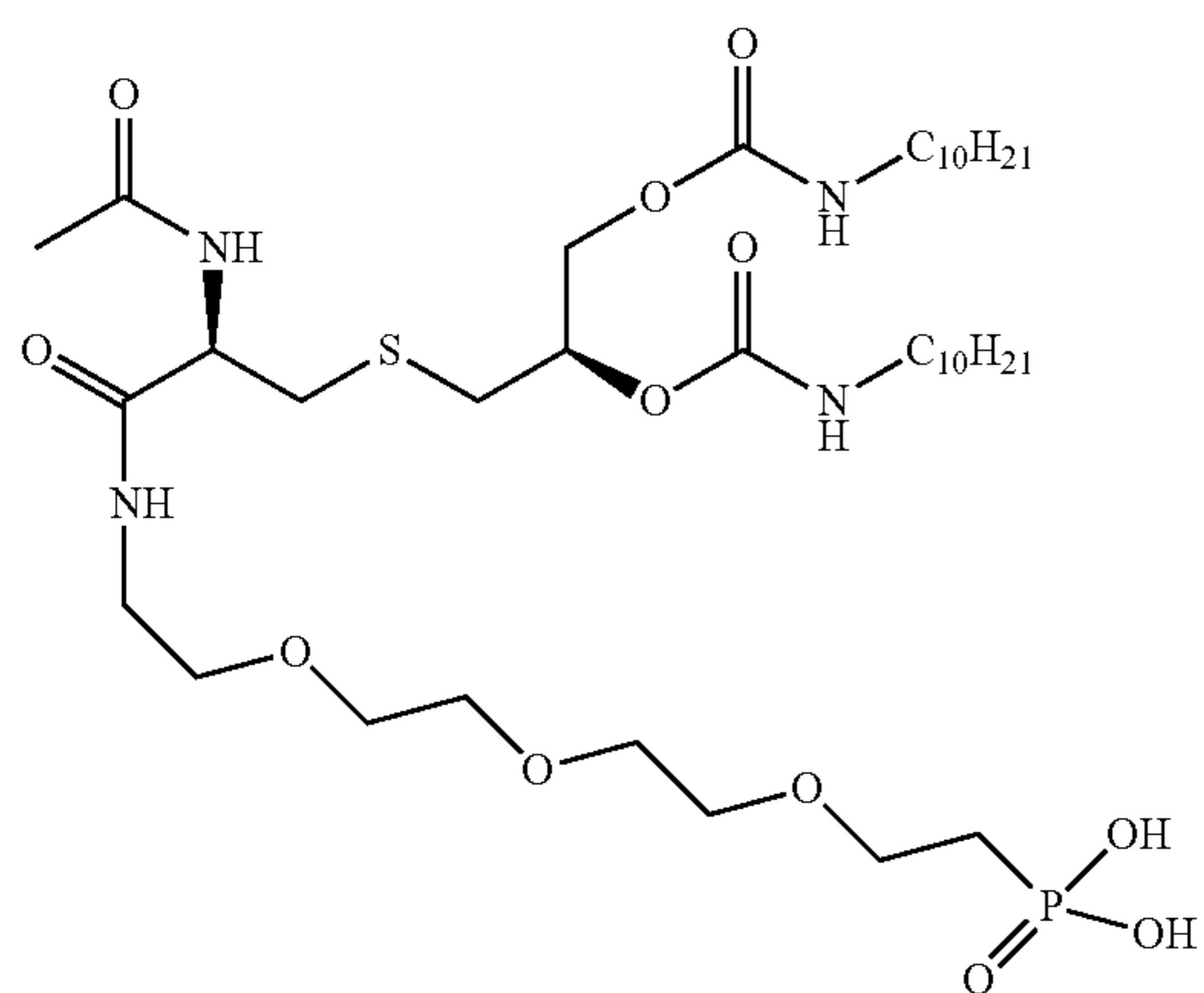
((14R,18R)-14-acetamido-18-((decylcarbamoyl)oxy)-13,21-dioxo-3,6,9,20-tetraoxa-16-thia-12,22-diazadotriacontyl)phosphonic acid
