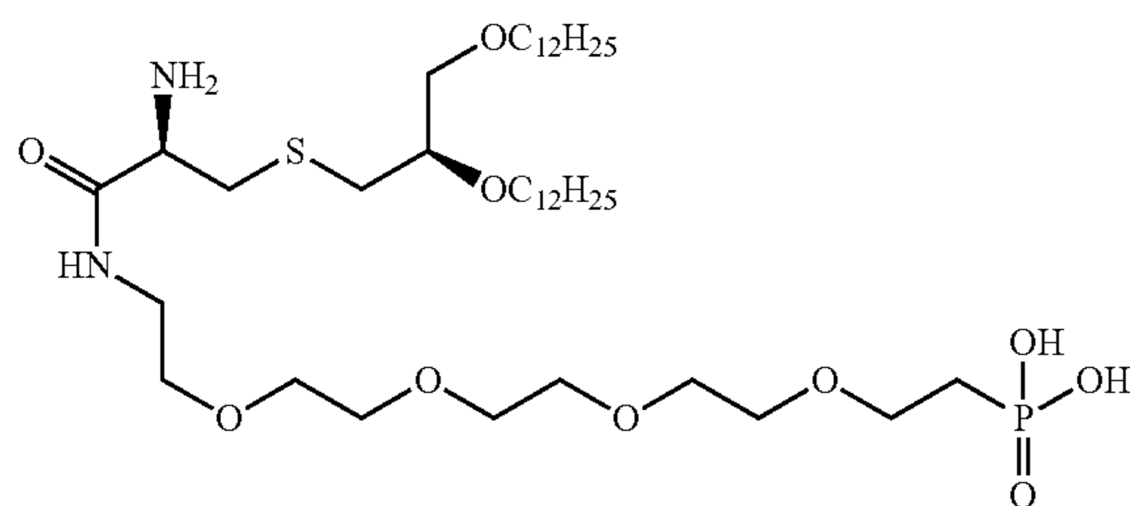
((17R,21R)-17-amino-21-(dodecyloxy)-16-oxo-3,6,9,12,23-pentaoxa-19-thia-15-azapentatriacontyl)phosphonic acid
