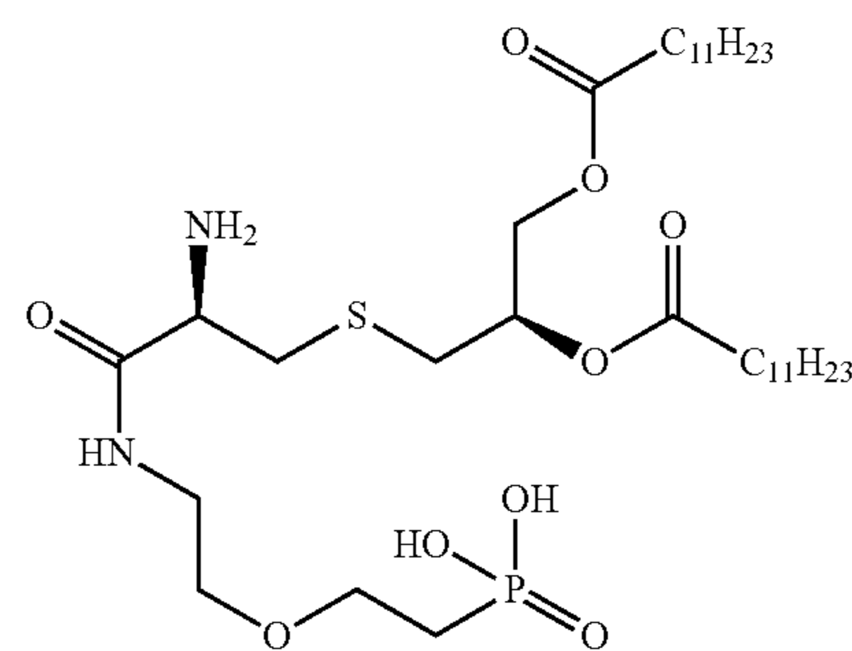
((8R,12R)-8-amino-12-(dodecanoyloxy)-7,15-dioxo-3,14-dioxo-10-thia-6-azahexacosyl)phosphonic acid
