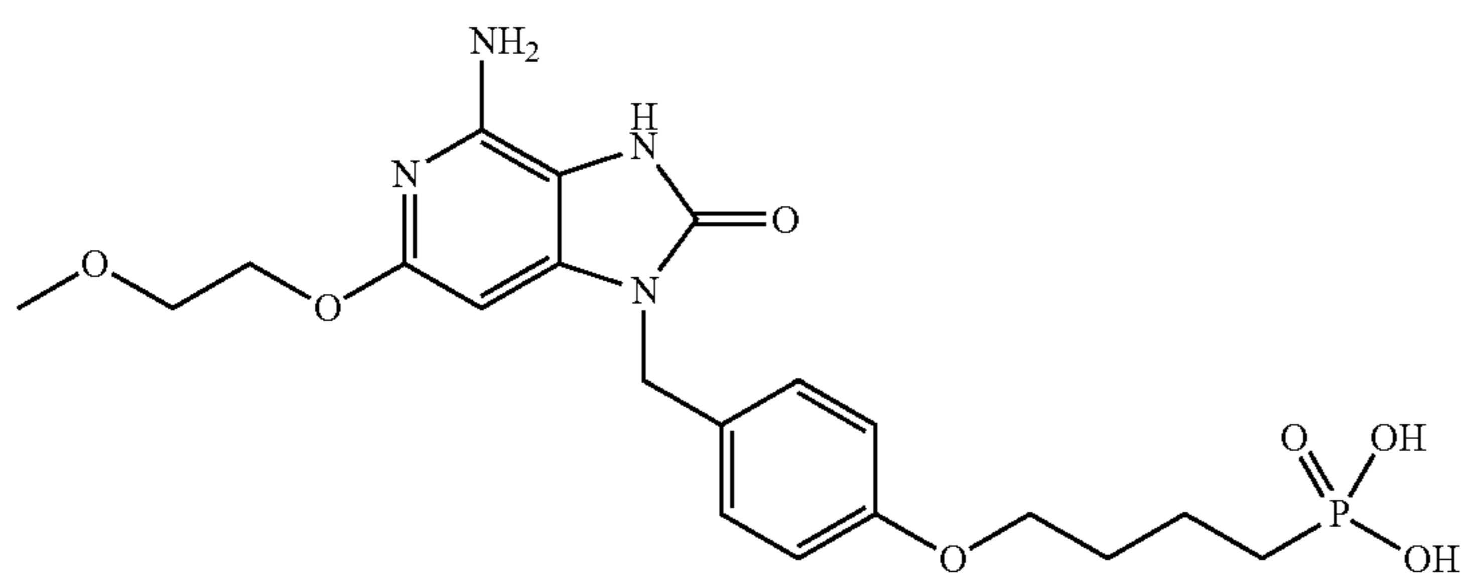
(4-(4-((4-amino-6-(2-methoxyethoxy)-2-oxo-2,3-dihydro-1H-imidazo[4,5-c]pyridin-1-yl)methyl)phenoxy)butyl)phosphonic acid
