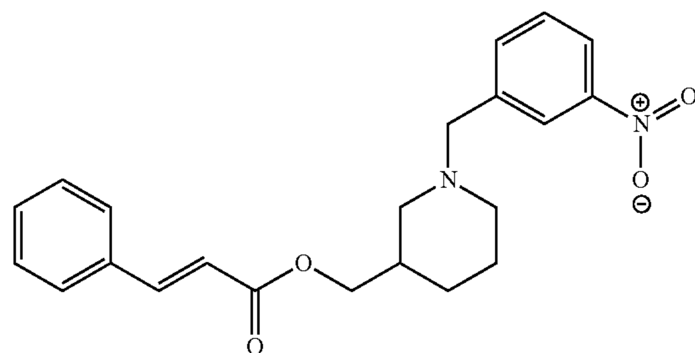
[1-(3-nitrobenzyl)-3-piperidiny]methyl 3-phenylacrylate
