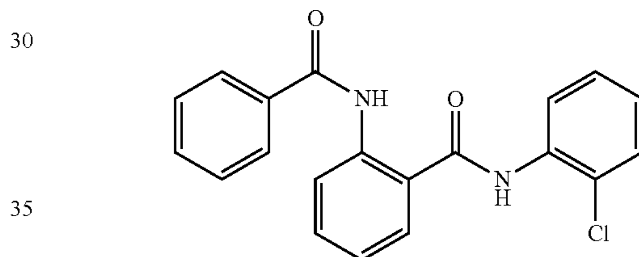
2-(benzoylamino)-N-(2-chlorophenyl)benzamide
