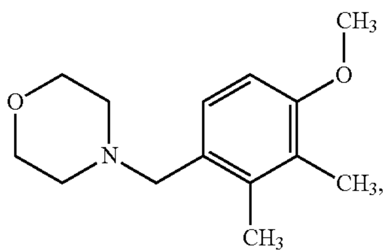
4-(4-methoxy-2,3-dimethylbenzyl)morpholine
