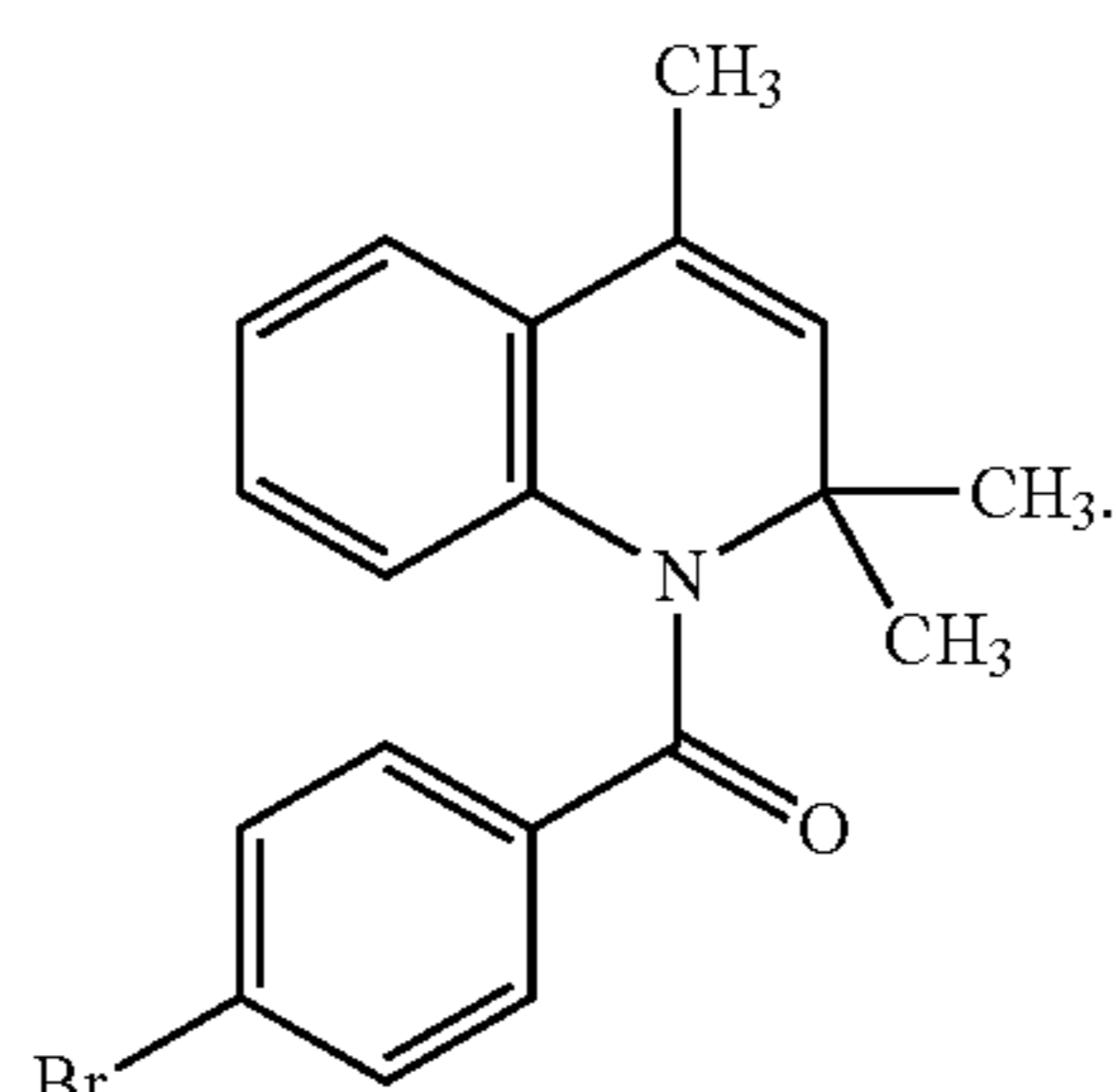
1-(4-bromobenzoyl)-2,2,4-trimethyl- 1,2-dihydroquinoline
