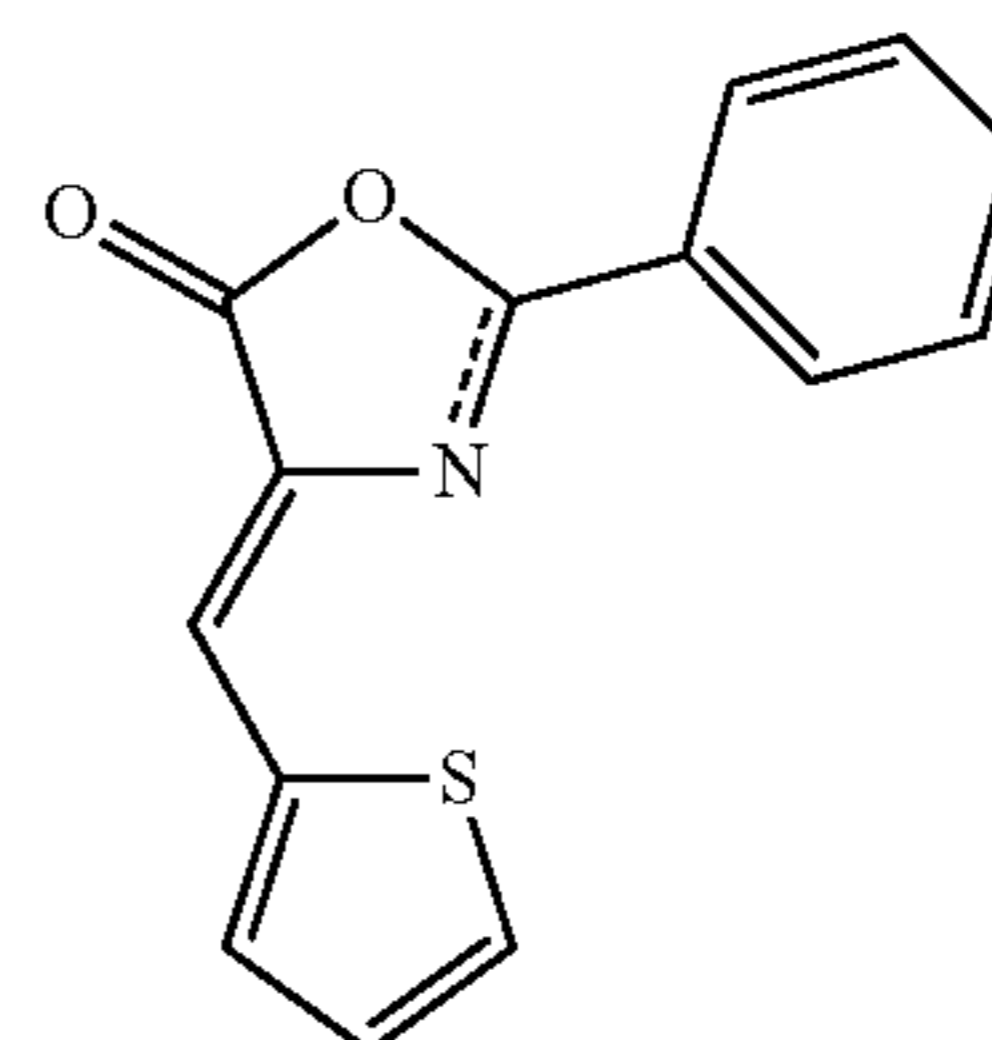
2-phenyl-4-(2-thienylmethylene)-1,3-oxazol-5(4H)-one
