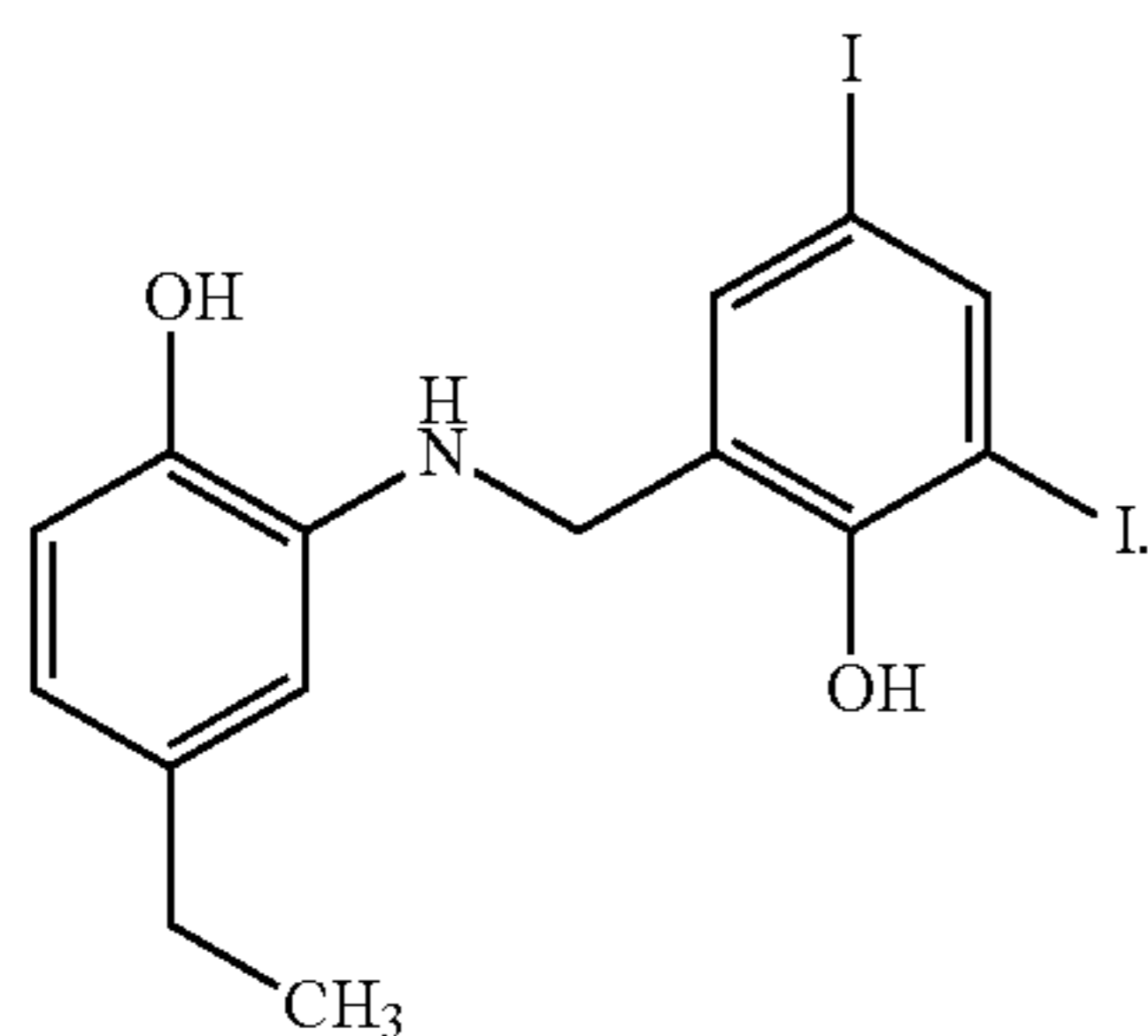
2-([(5-ethyl-2-hydroxyphenyl)imino]methyl)-4,6-diiodophenol
