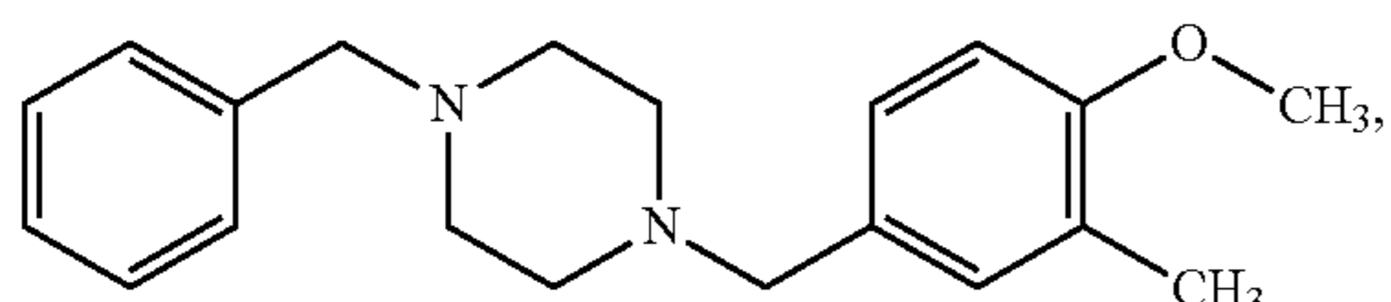
1-benzyl-4-(4-methoxy-3-methylbenzyl)piperazine
