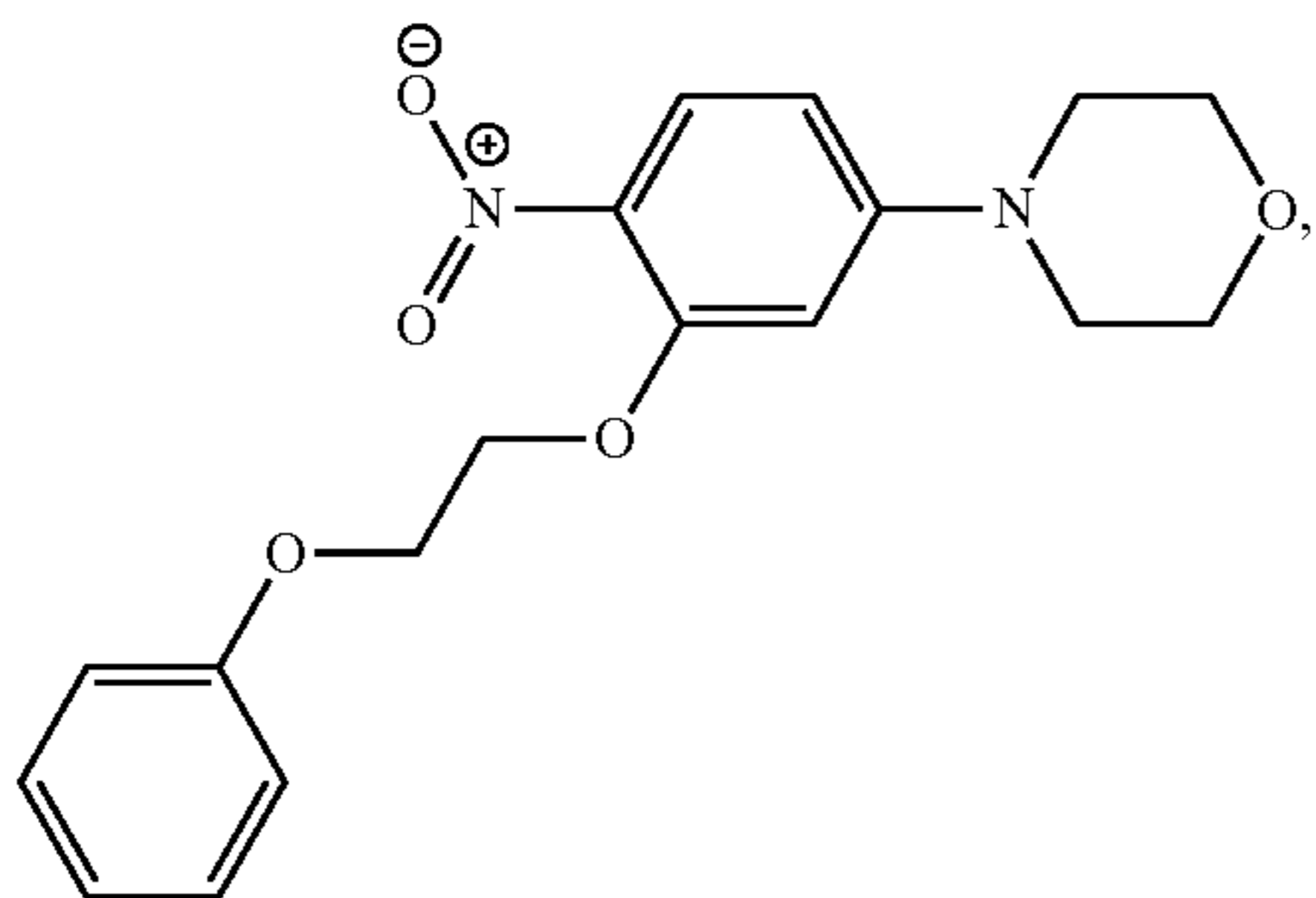
4-[4-nitro-3-(2-phenoxyethoxy)phenyl]morpholine
