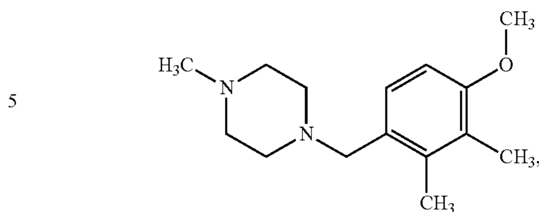
1-(4-methoxy-2,3-dimethylbenzyl)-4-methylpiperazine
