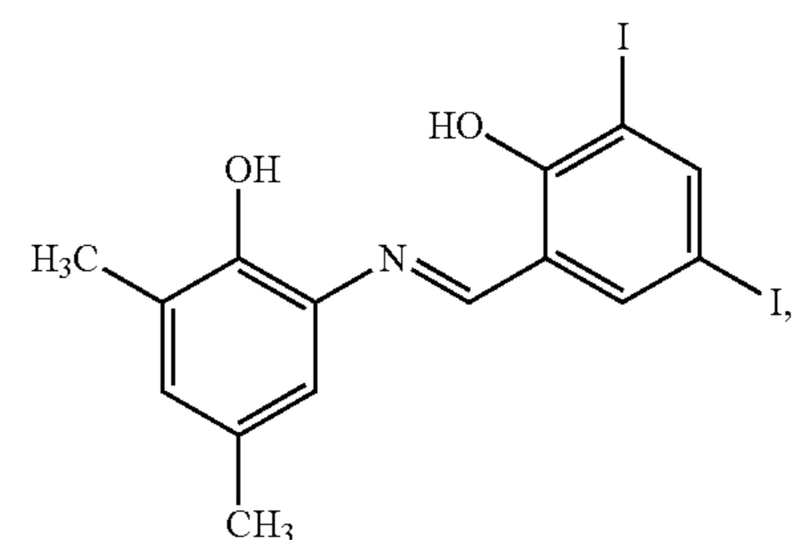
2-[(hydroxy-3,5-diiodobenzylidene)amino]4,6-dimethylphenol
