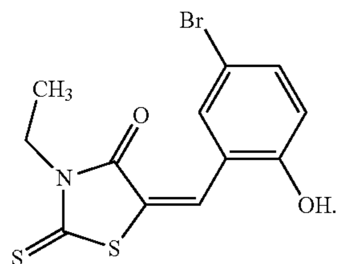
5-(5-bromo-2-hydroxybenzylidene)-3-ethyl-2-thioxo-1,3-thiazolidin-4-one
