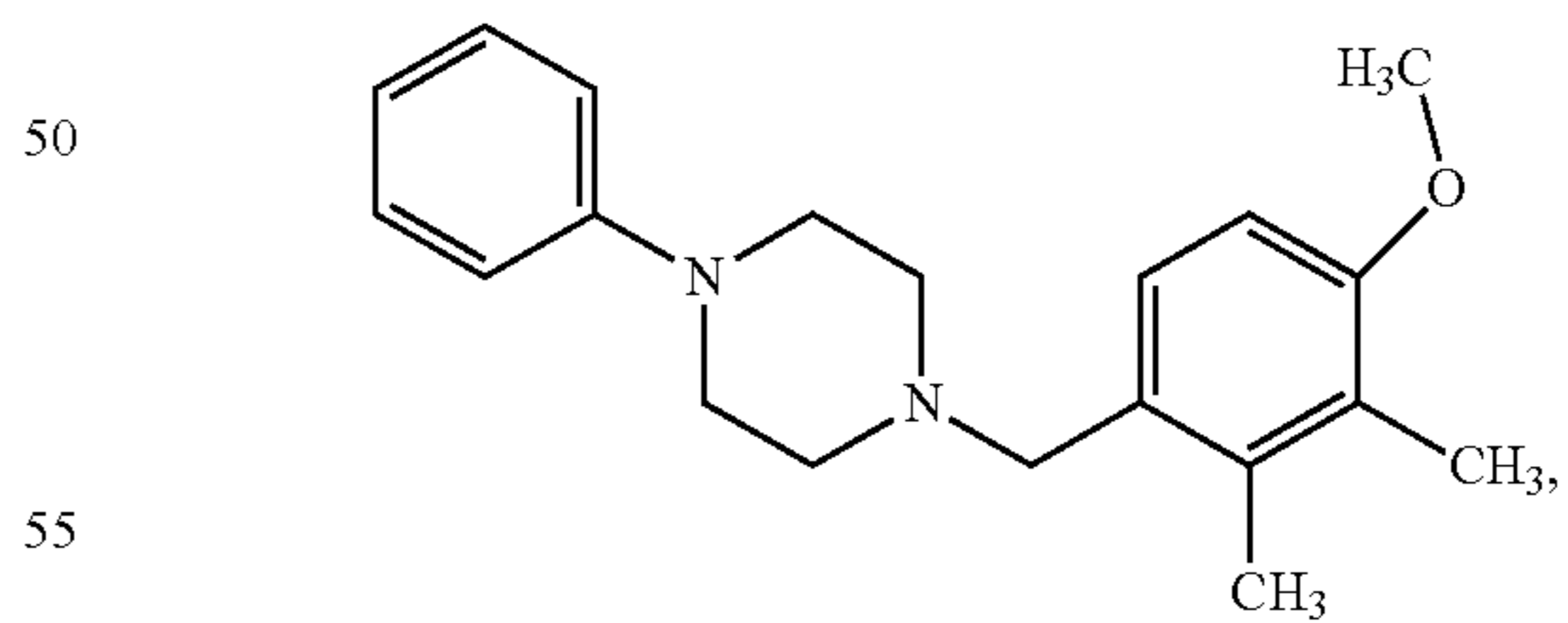
1-(4-methoxy-2,3-dimethylbenzyl)-4-phenylpiperazine
