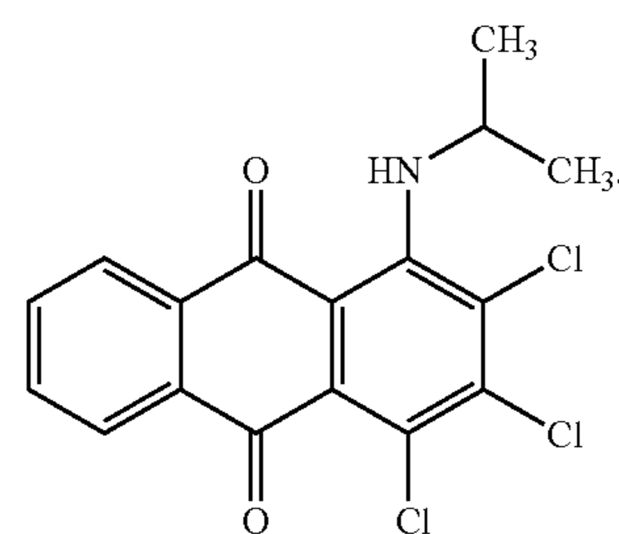
1,2,3-trichloro-4-(isopropylamino) anthra-9,10-quinone
