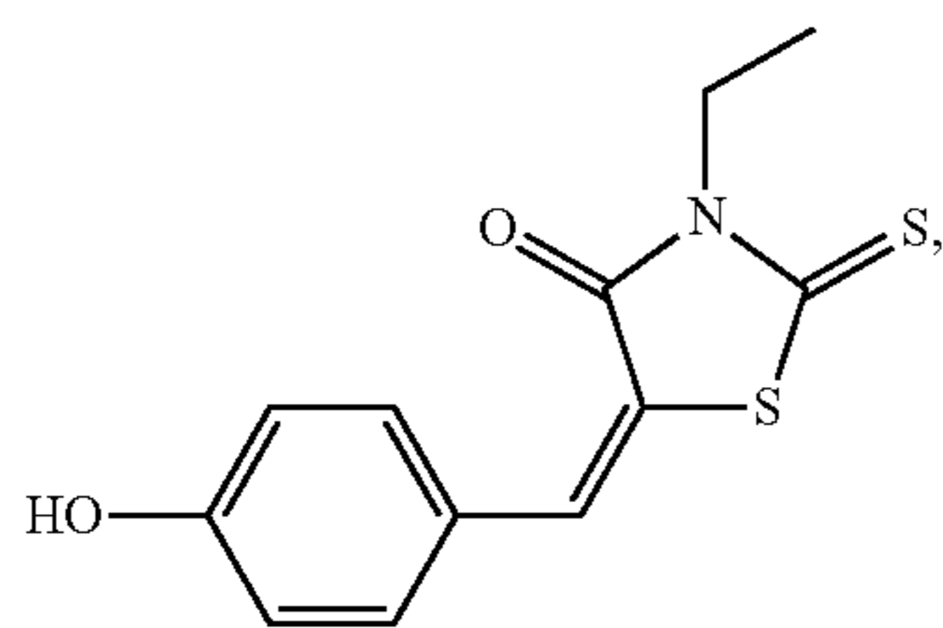
3-ethyl-5-(4-hydroxybenzylidene)-2-thioxo-1,3-thiazolidin-4-one
