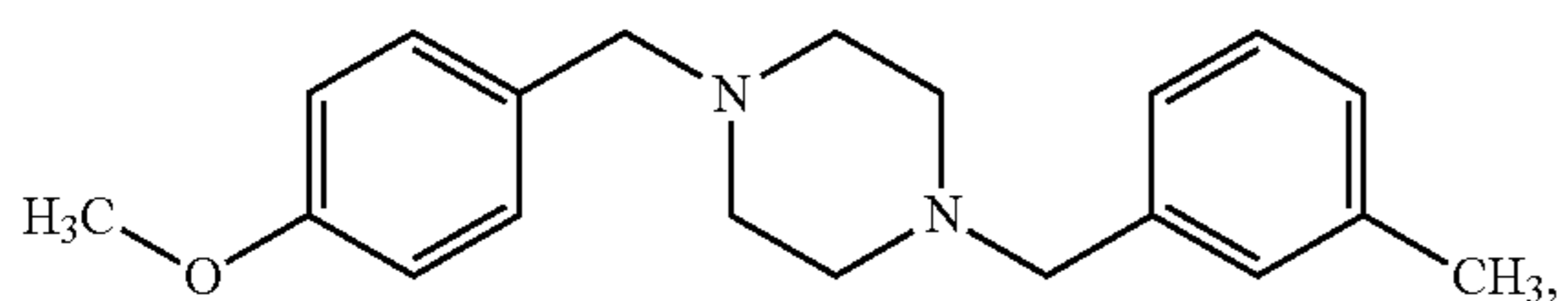
1-(4-methoxybenzyl)-4-(3-methylbenzyl)piperazine
