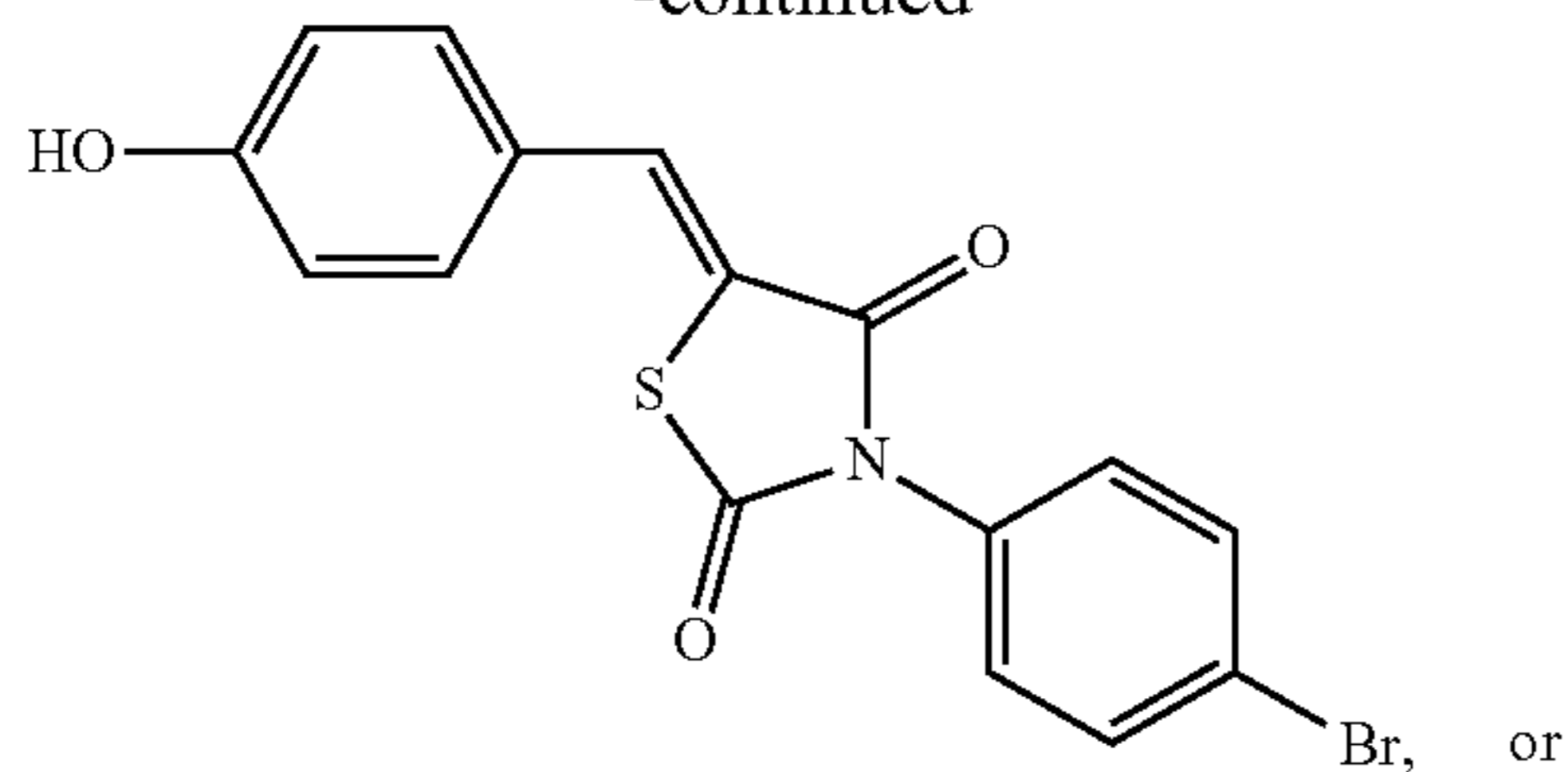
3-(4-bromophenyl)-5-(4-hydroxybenzylidene)-2-thioxo-1,3-thiazolidin-4-one
