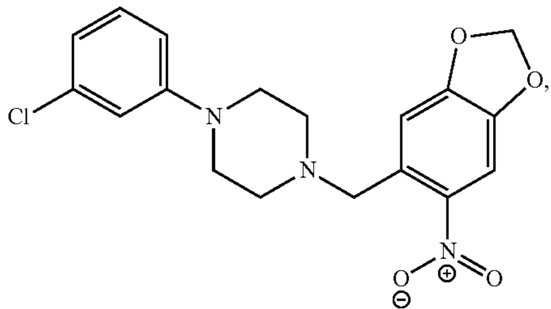
1-(3-chlorophenyl)-4-[(6-nitro-1,3-benzodioxol-5-yl)methyl]piperazine
