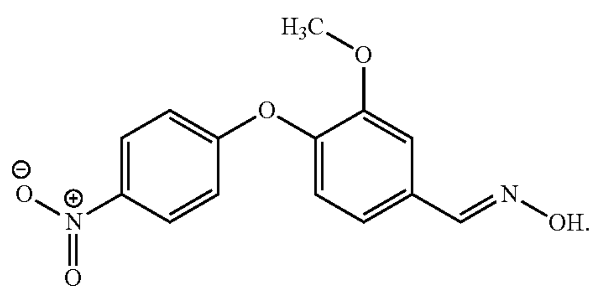
3-methoxy-4-(4-nitrophenoxy)benzaldehyde oxime
