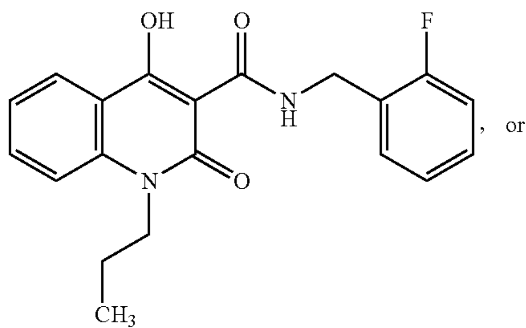
N-(2-fluorobenzyl)-4-hydroxy-2-oxo-1-propyl-1,2-dihydro-3-quinolinecarboxamide
