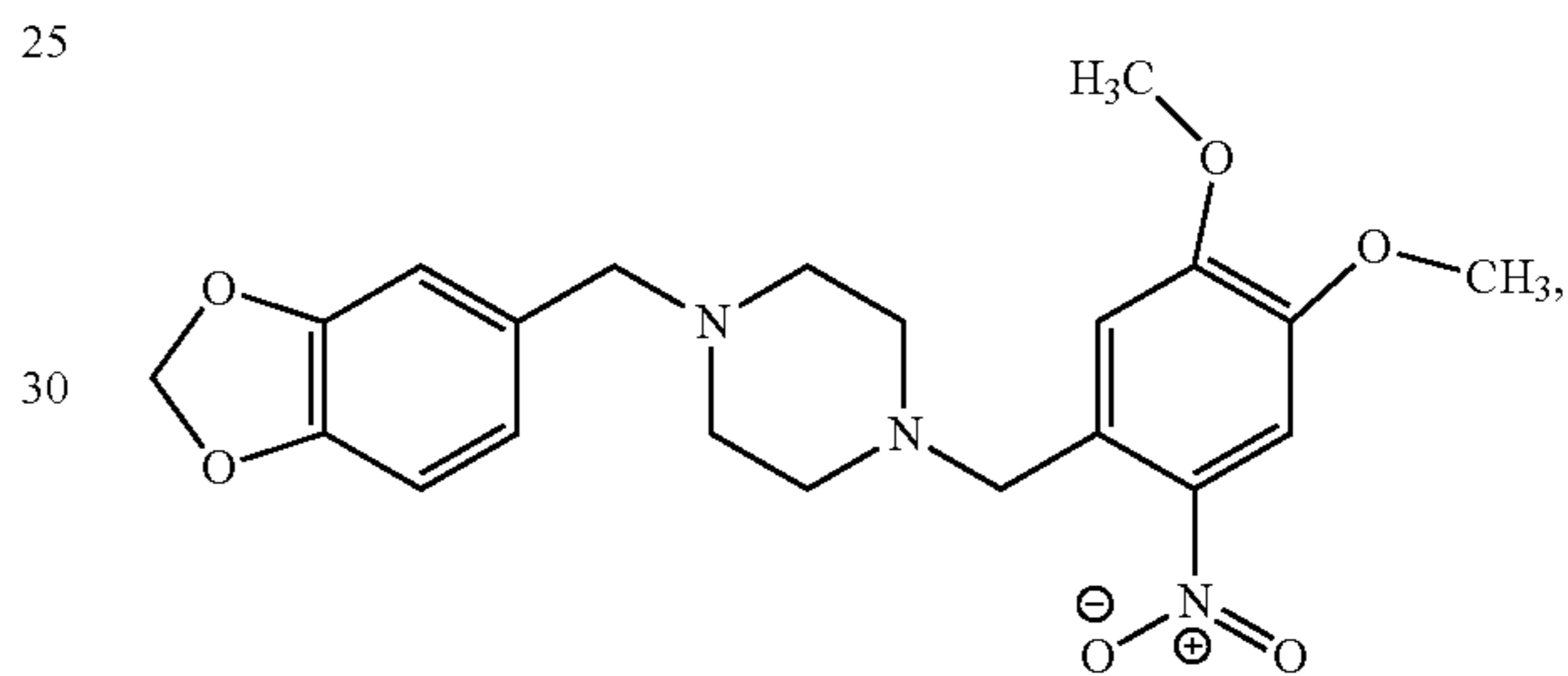
1-(1,3-benzodioxol-5-ylmethyl)-4-(4,5-dimethoxy-2-nitrobenzyl)piperazine
