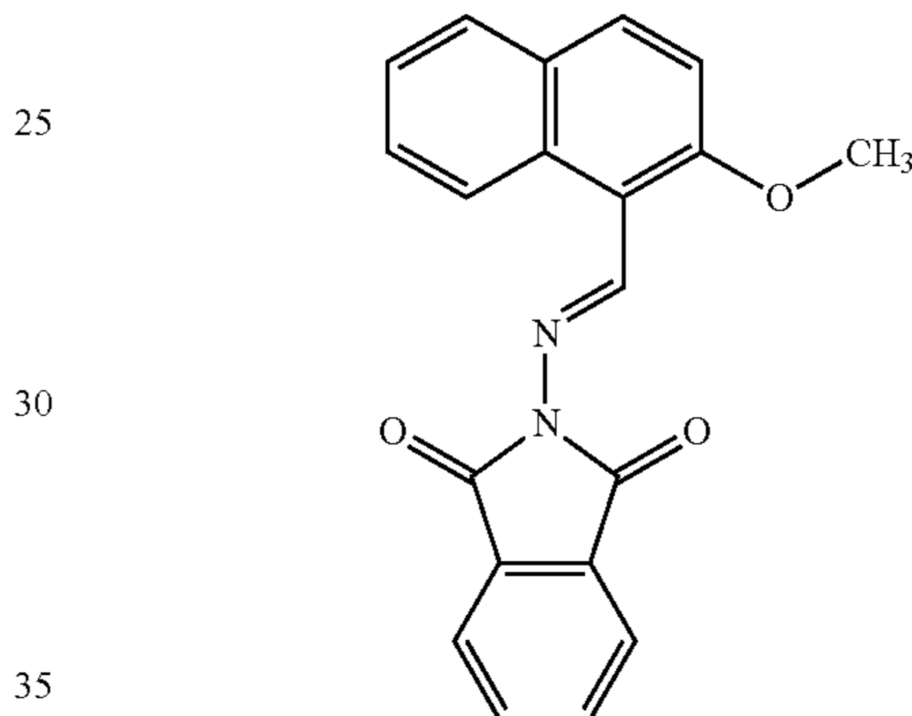
2-[(2-methoxy-1-naphthyl)methylene]amino]-1H-isoidole-1,3(2H)-dione
