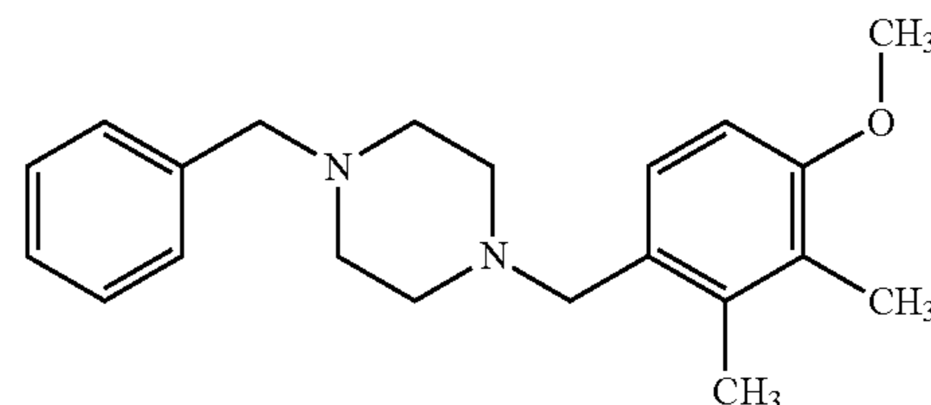
1-benzyl-4-(4-methoxy-2,3-dimethylbenzyl)piperazine
