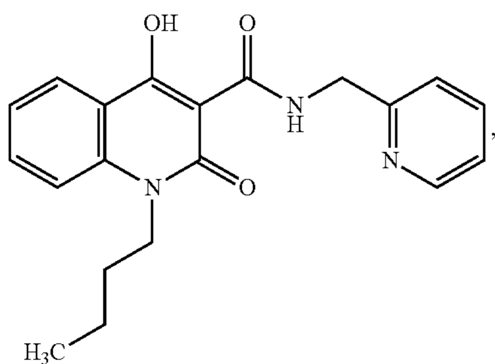
1-butyl-4-hydroxy-2-oxo-N-(2-pyridinylmethyl)-1,2-dihydro-3-quinolinecarboxamide
