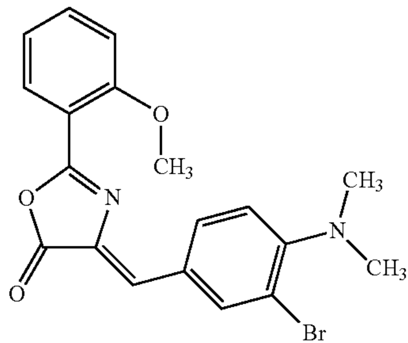
4-[3-bromo-4-(dimethylamino)benzylidene]-2-(2-methoxyphenyl)-1,3-oxazol-5(4H)-one
