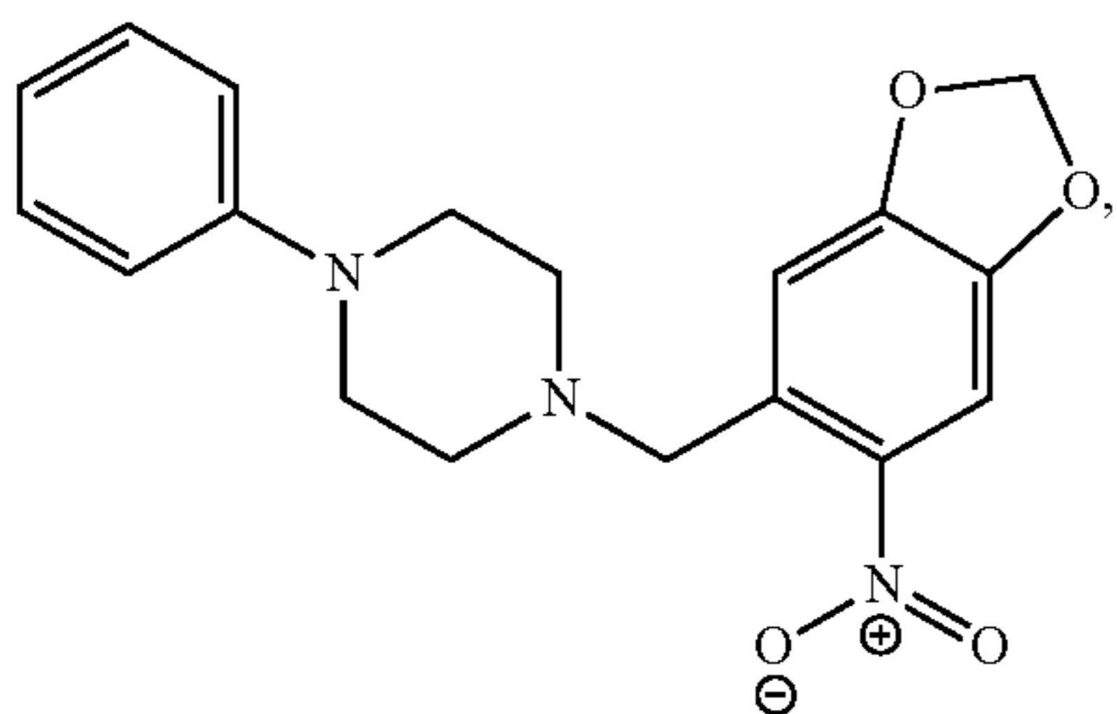
1-[(6-nitro-1,3-benzodioxol-5-yl)methyl]-4-phenylpiperazine
