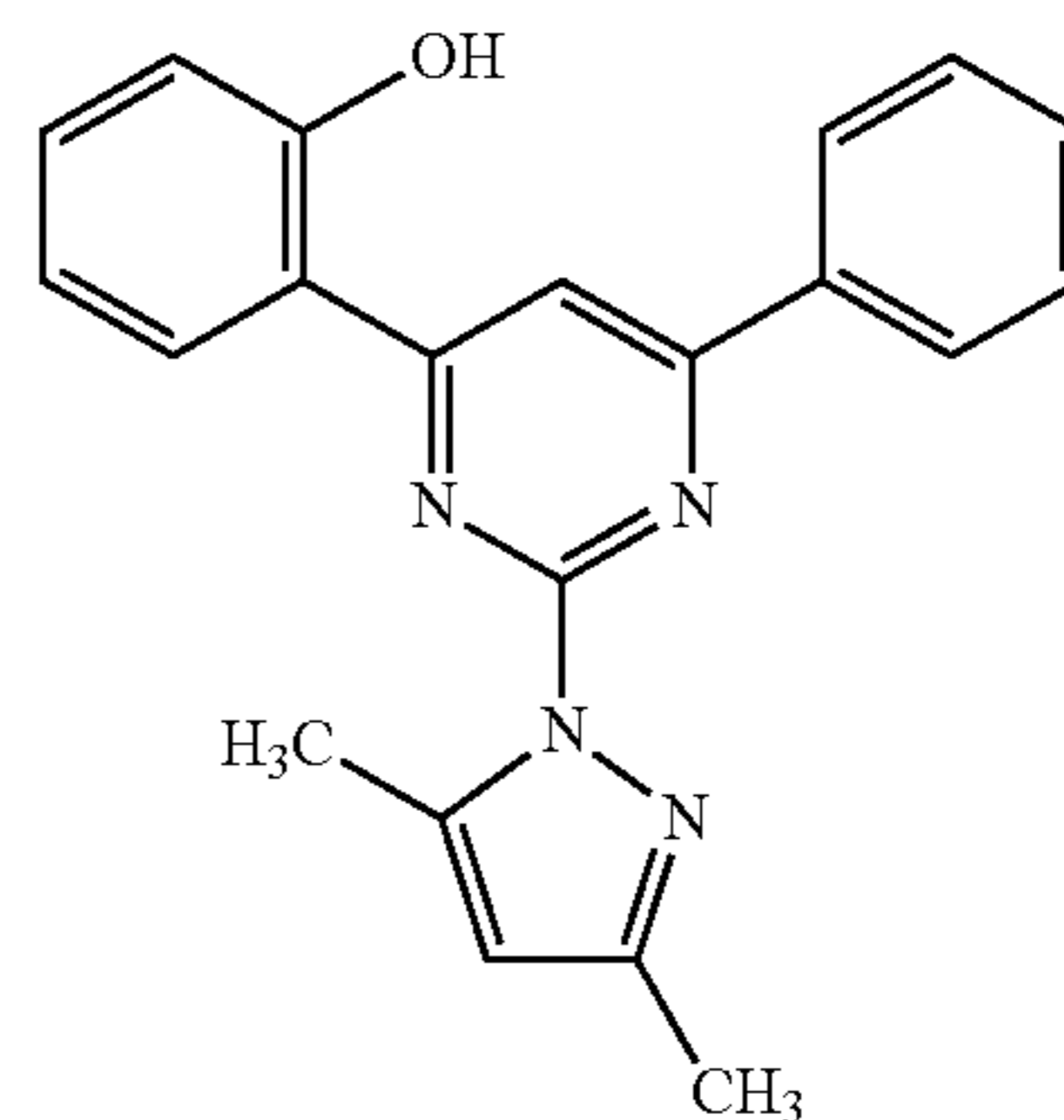
2-[2-(3,5-dimethyl-1H-pyrazol-1-yl)-6-phenyl-4-pyrimidinyl]phenol.
