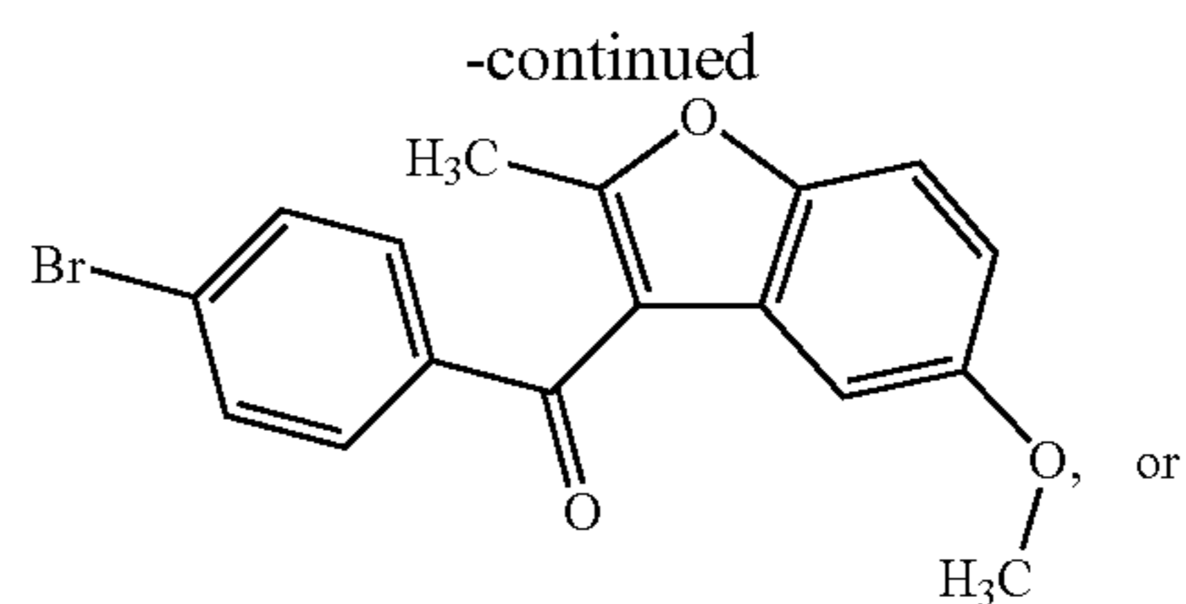
(4-(4-bromophenyl)(5-methoxy-2-methyl-1-benzofuran-3-yl)methanone
