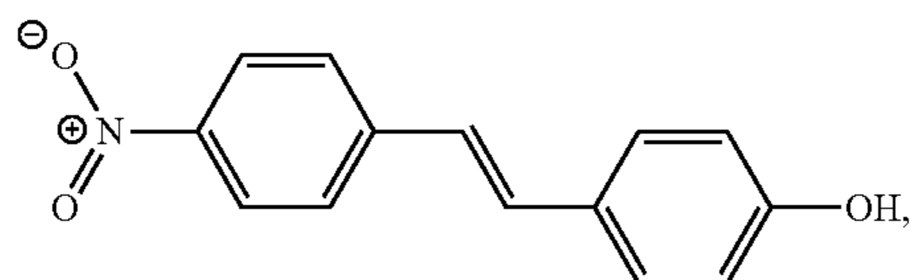
4-[2-(4-nitrophenyl)vinyl]phenol
