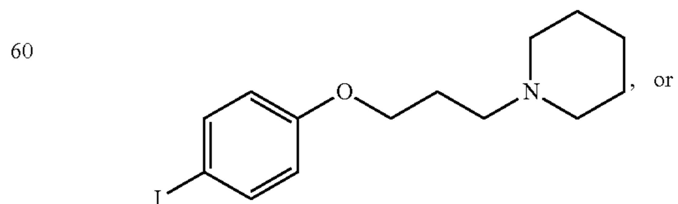
1-[3-(4-iodophenoxy)propyl]piperidine
