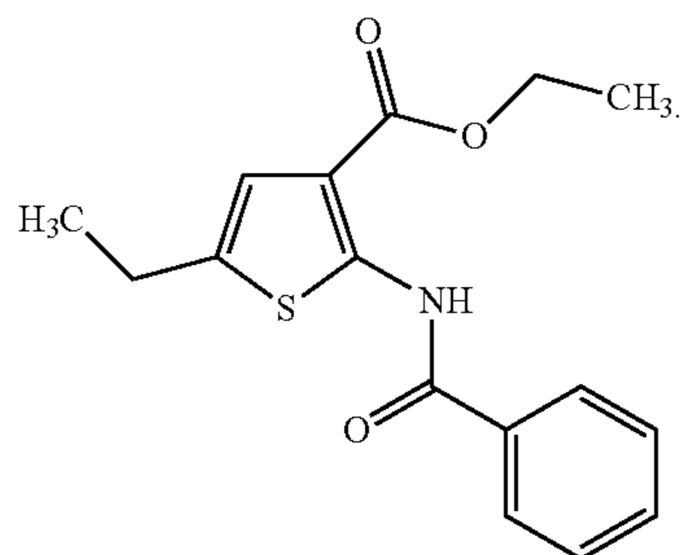
ethyl 2-(benzoylamino)-5-ethyl-3-thiophenecarboxylate
