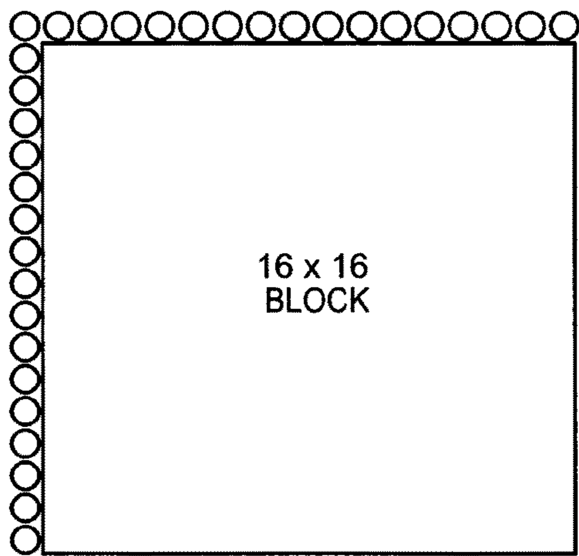
Intra_16 x 16
