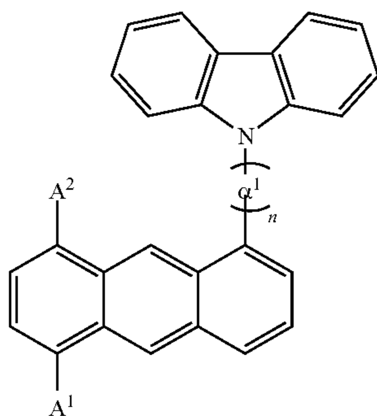
[Chemical formula 10]
