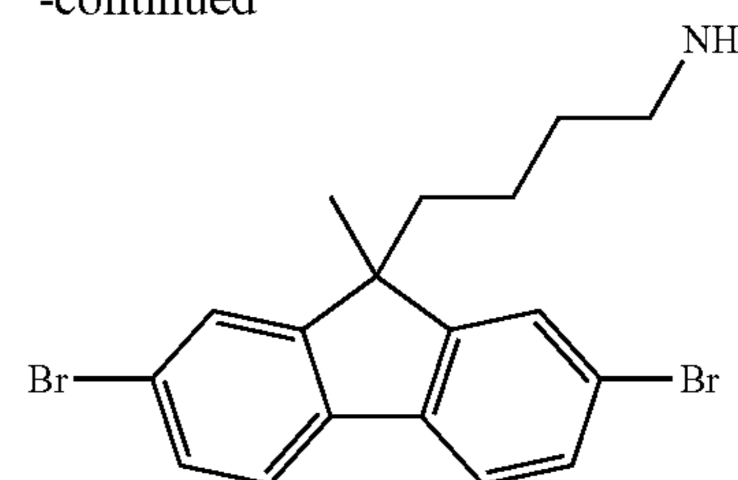
Step 3: 4-(2,7-dibromo-9-methyl-9H-fluoren-9-yl)butan-1-amine
