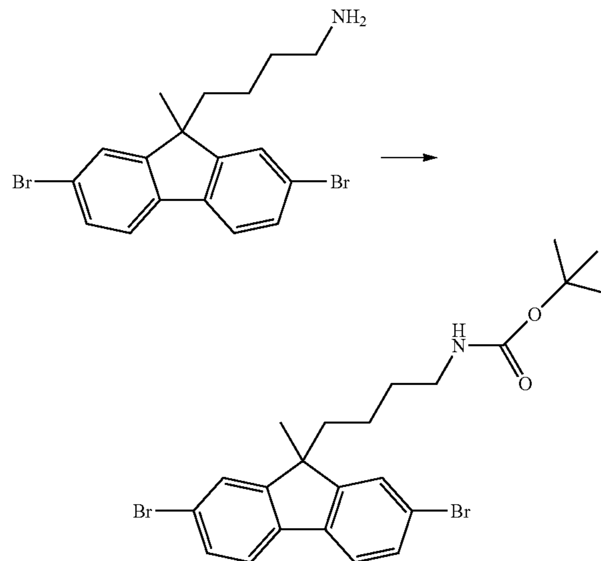
Step 4: tert-butyl-4-(2,7-dibromo-9-methyl-9H-fluoren-9-yl)butylcarbamate
