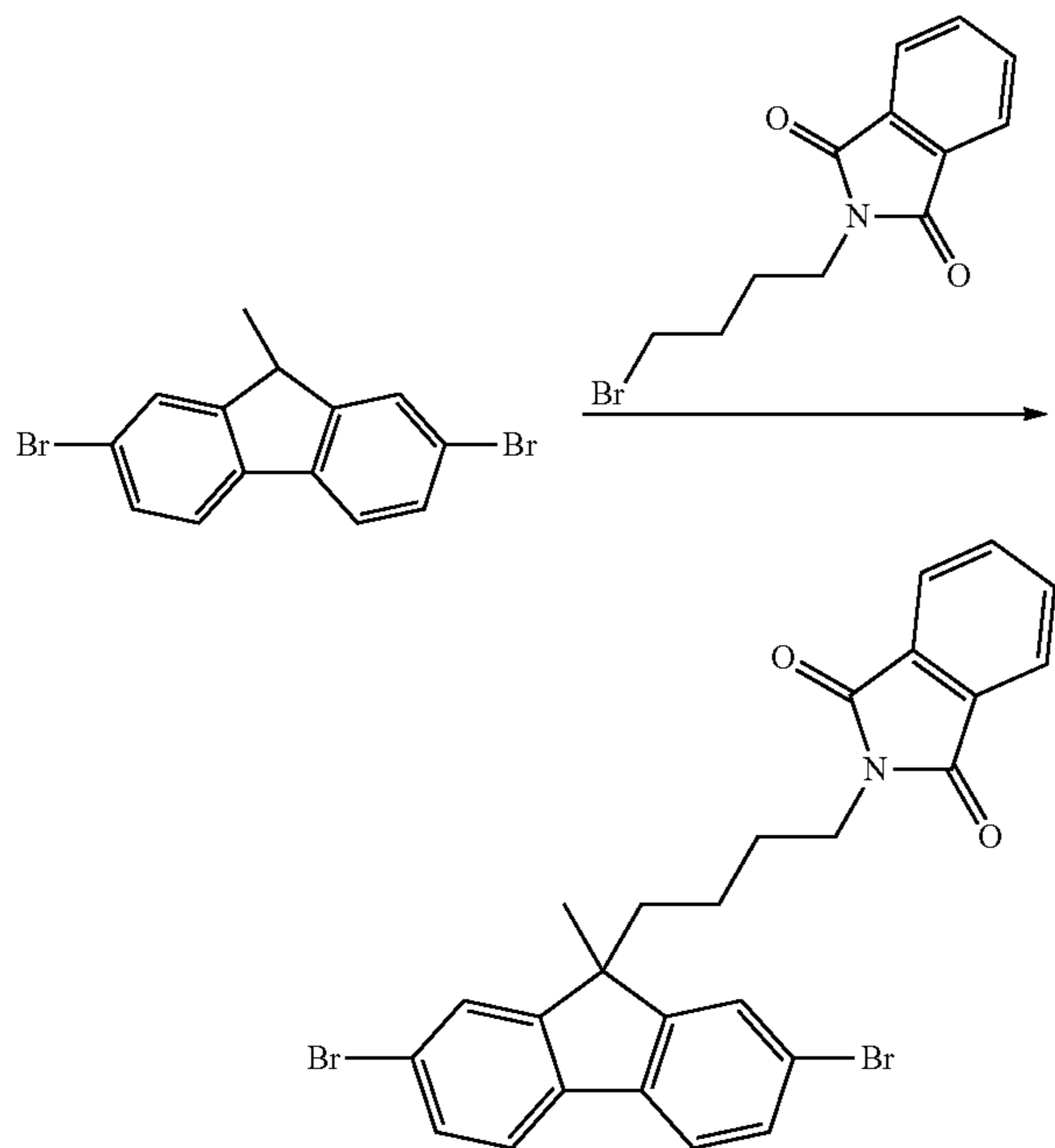
Step 2: 2-(4-(2,7-dibromo-9-methyl-9H-fluoren-9-yl)butyl)isoindoline-1,3-dione
