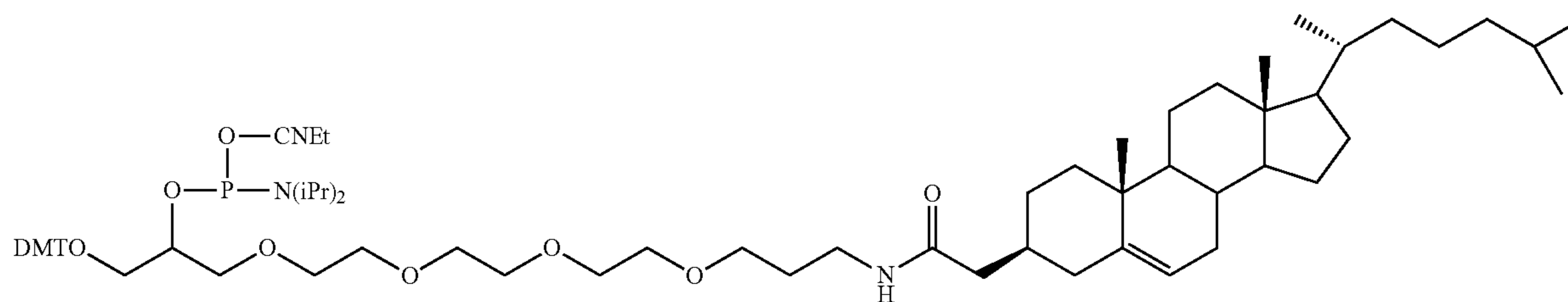
Cholesteryl-TEG Phosphoramidite
