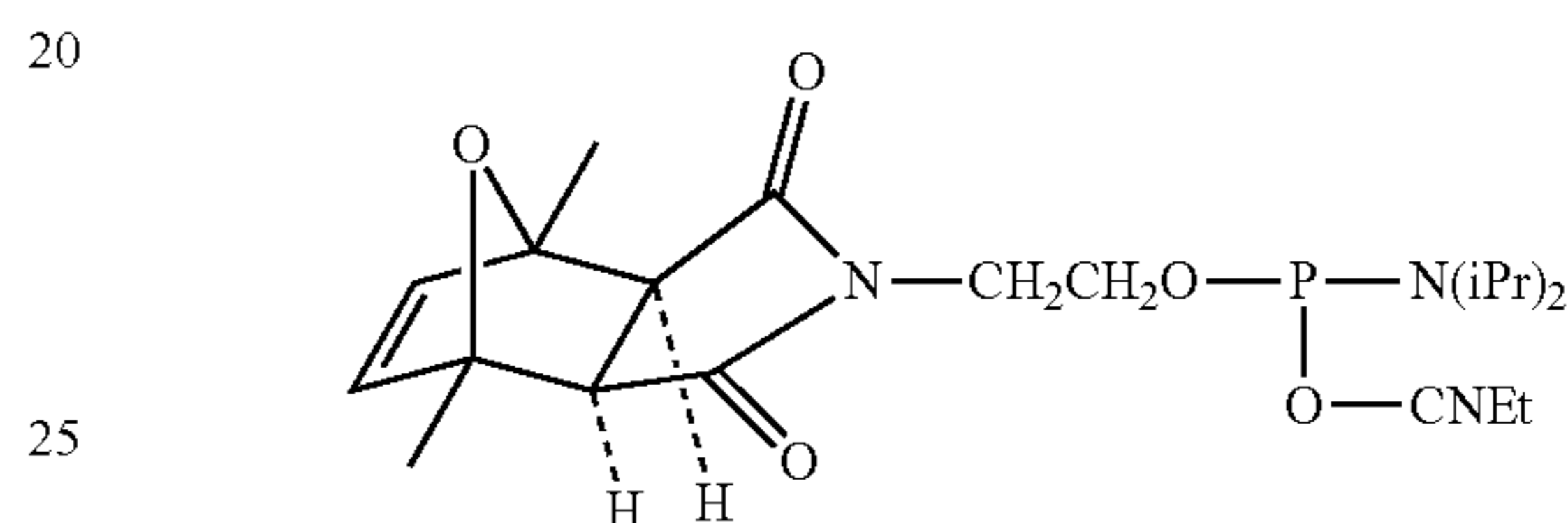
5'-Maleimide-Modifier Phosphoramidite
