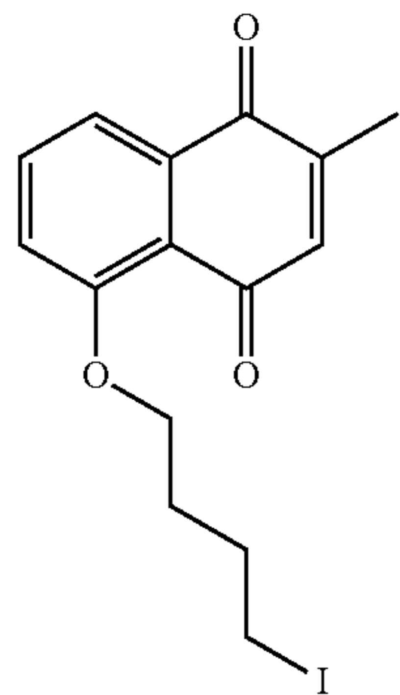
(F48) 5-(4-iodobutoxy)-2-methyl-1,4-naphthoquinone
