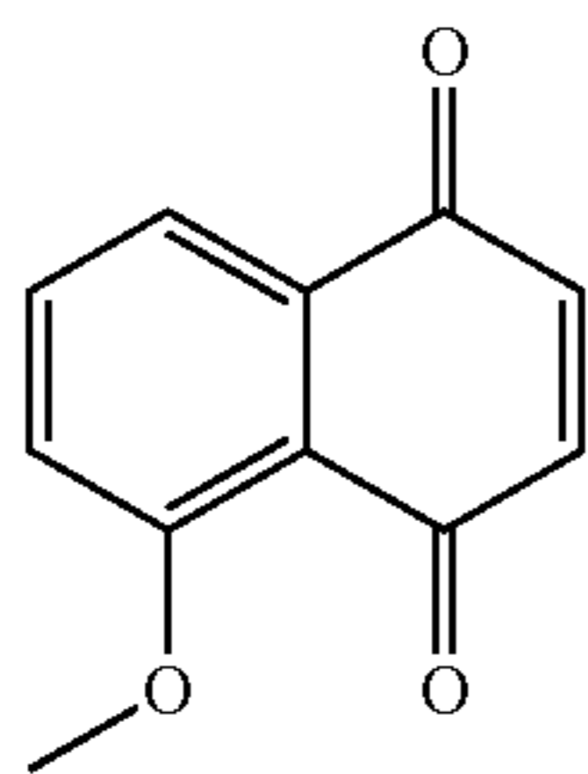
(F51) 5-methoxy-1,4-naphthoquinone
