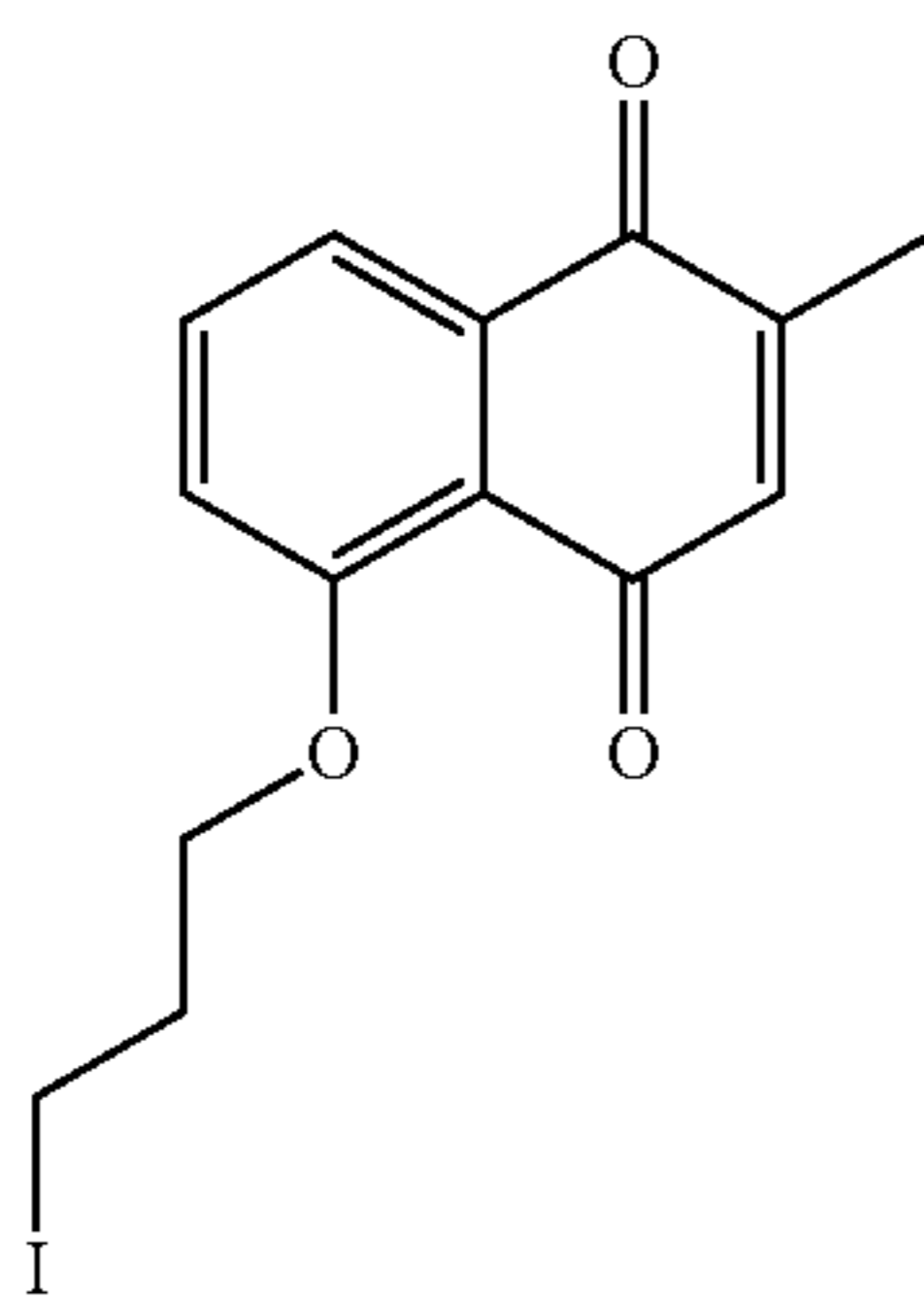
(F49) 5-(3-iodopropoxy)-2-methyl-1,4-naphthoquinone
