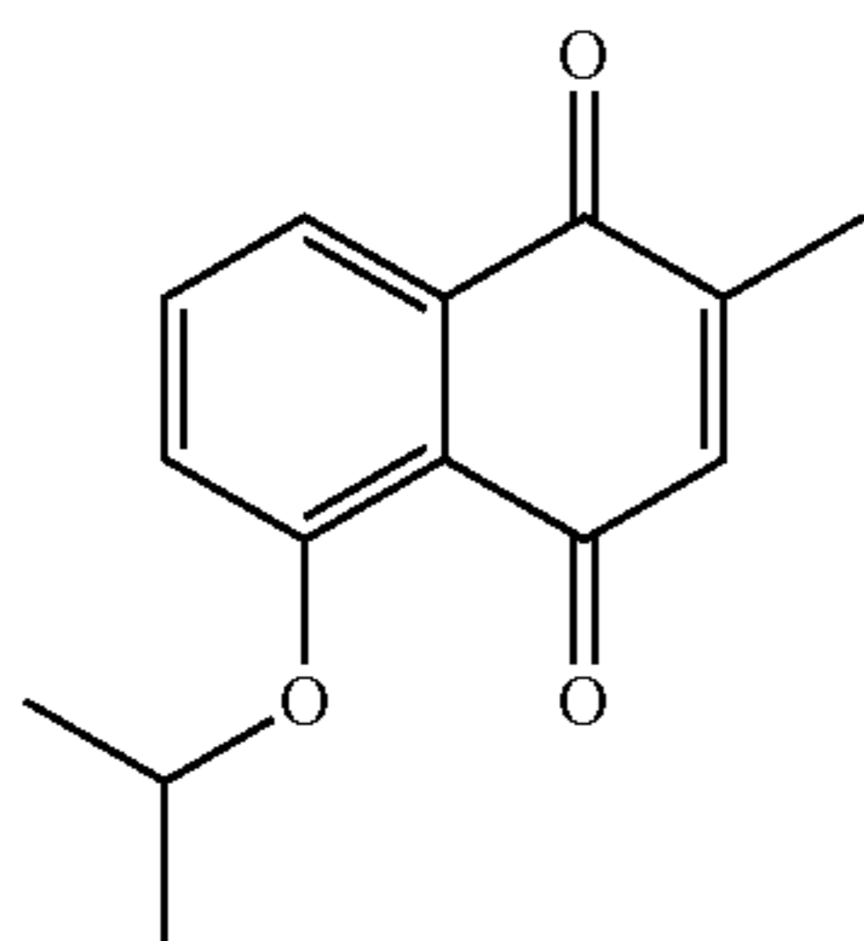
(F50) 5-isopropoxy-2-methyl-1,4-naphthoquinone
