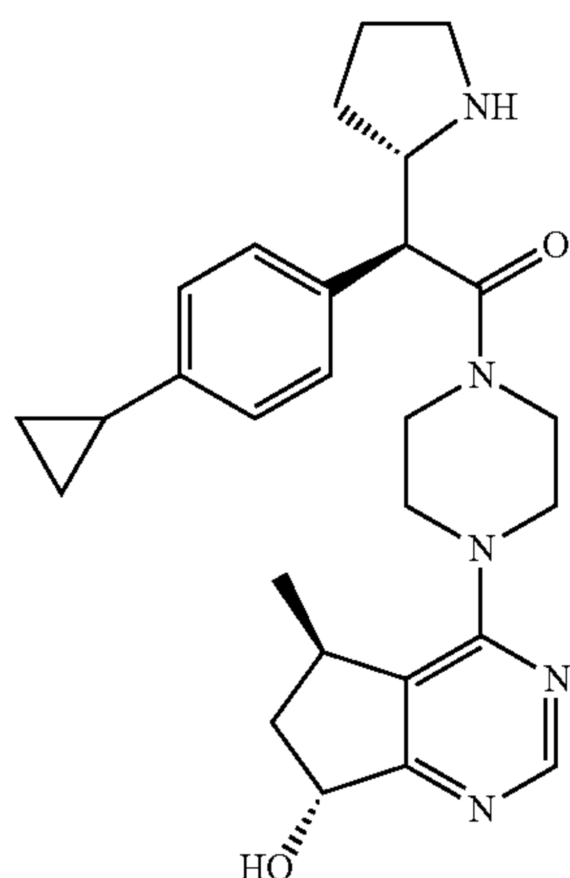
(S)-2-(4-cyclopropylphenyl)-1-(4-((5R,7R)-7-hydroxy-5-methyl-6,7-dihydro-5H-cyclopenta[d]pyrimidin-4-yl)piperazin-1-yl)-2-((S)-pyrrolidin-2-yl)ethanone
