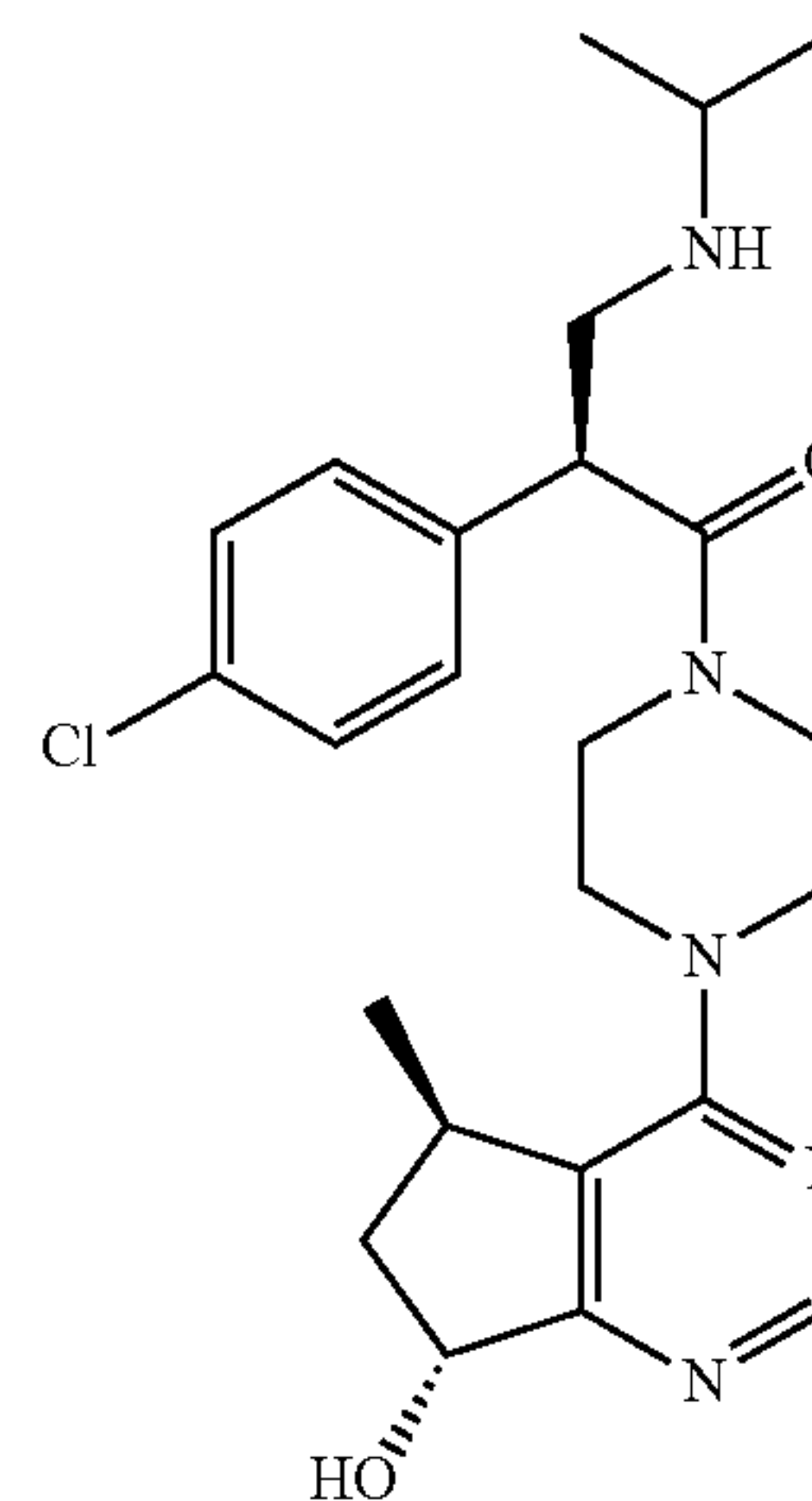
(S)-2-(4-chlorophenyl)-1-(4-((5R,7R)-7-hydroxy-5-methyl-6,7-dihydro-5H-cyclopenta[d]pyrimidin-4-yl)piperazin-1-yl)-3-(isopropylamino)propan-1-one
