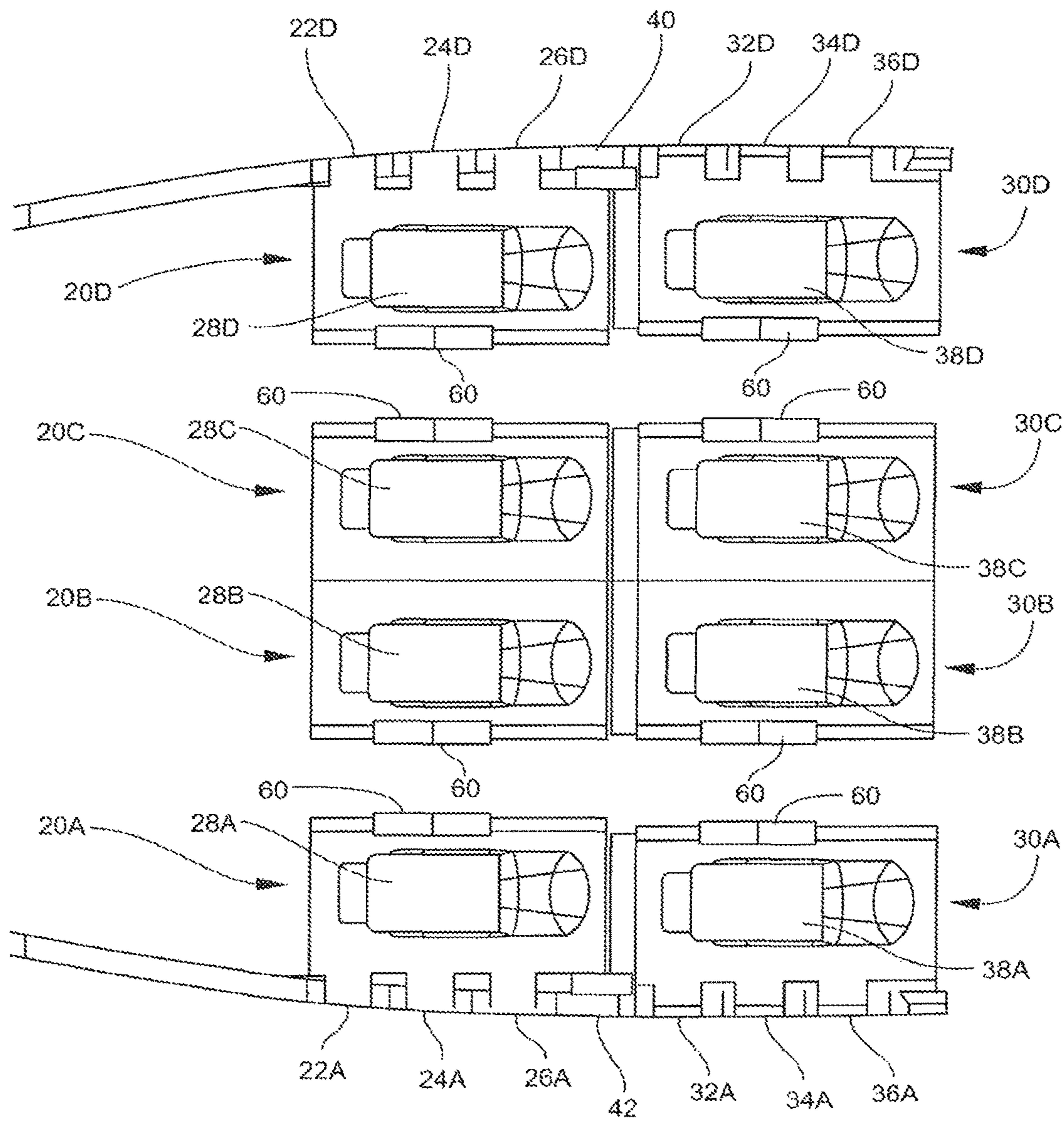
FIG. 1 PRIOR ART
