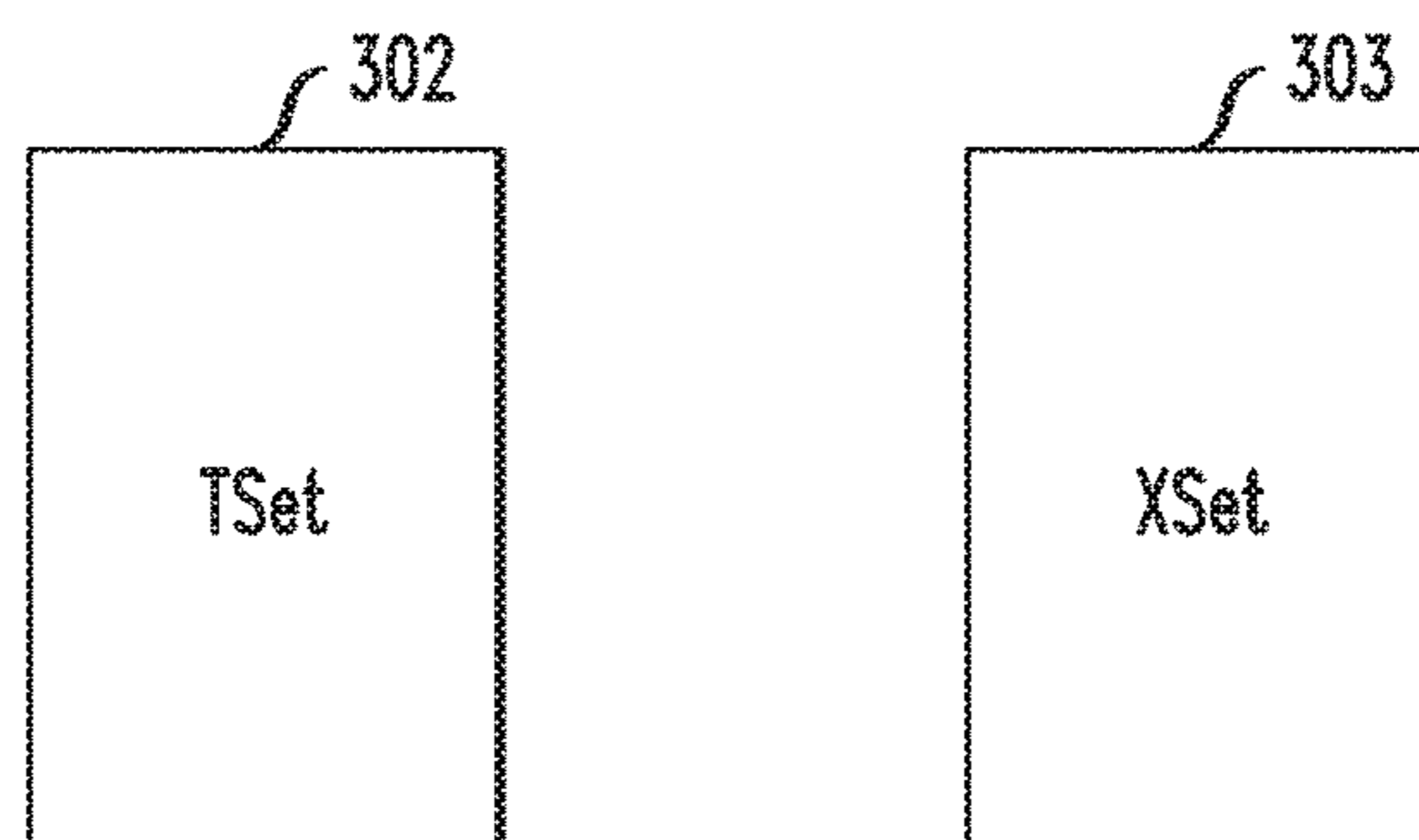
ENCRYPTED DATABASE 301
