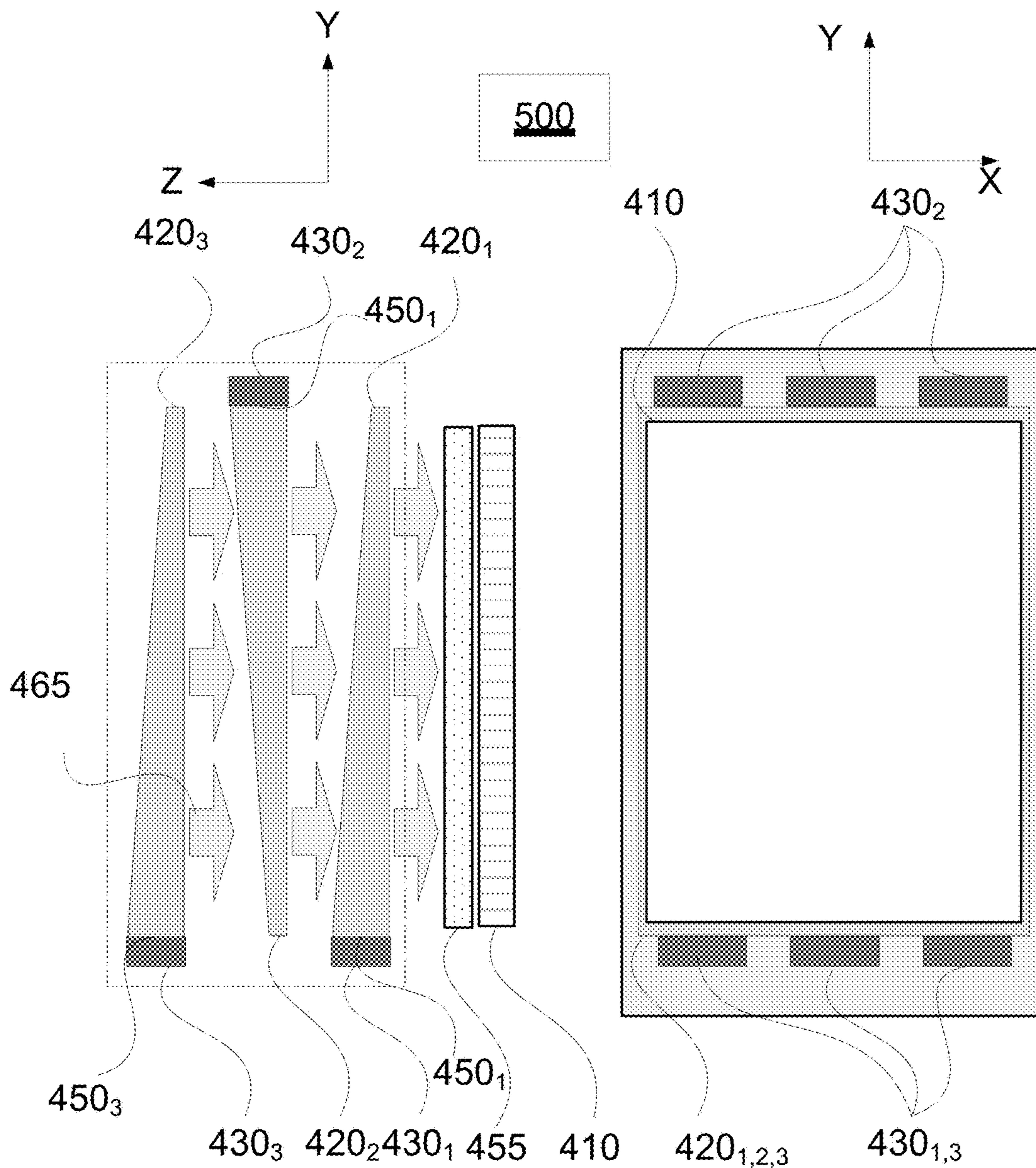
Side View
