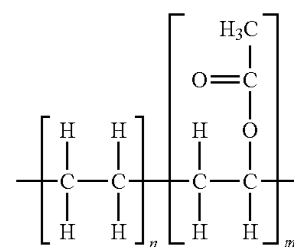
Ethylene-vinyl acetate
