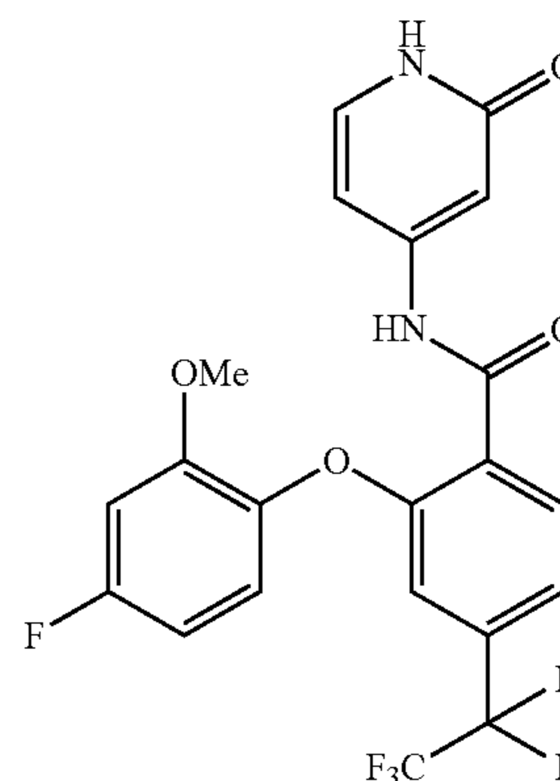
2-(4-fluoro-2-methoxyphenoxy)-N-(2-oxo-1,2-dihydropyridin-4-yl)-4-(perfluoroethyl)benzamide.
