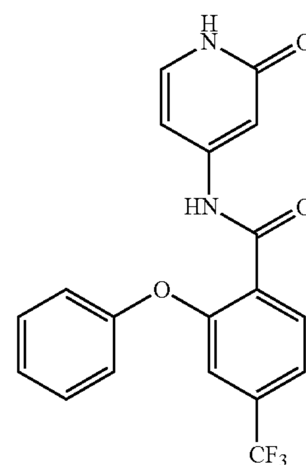
N-(2-oxo-1,2-dihydropyridin-4-yl)-2-phenoxy-4-(trifluoromethyl)benzamide
