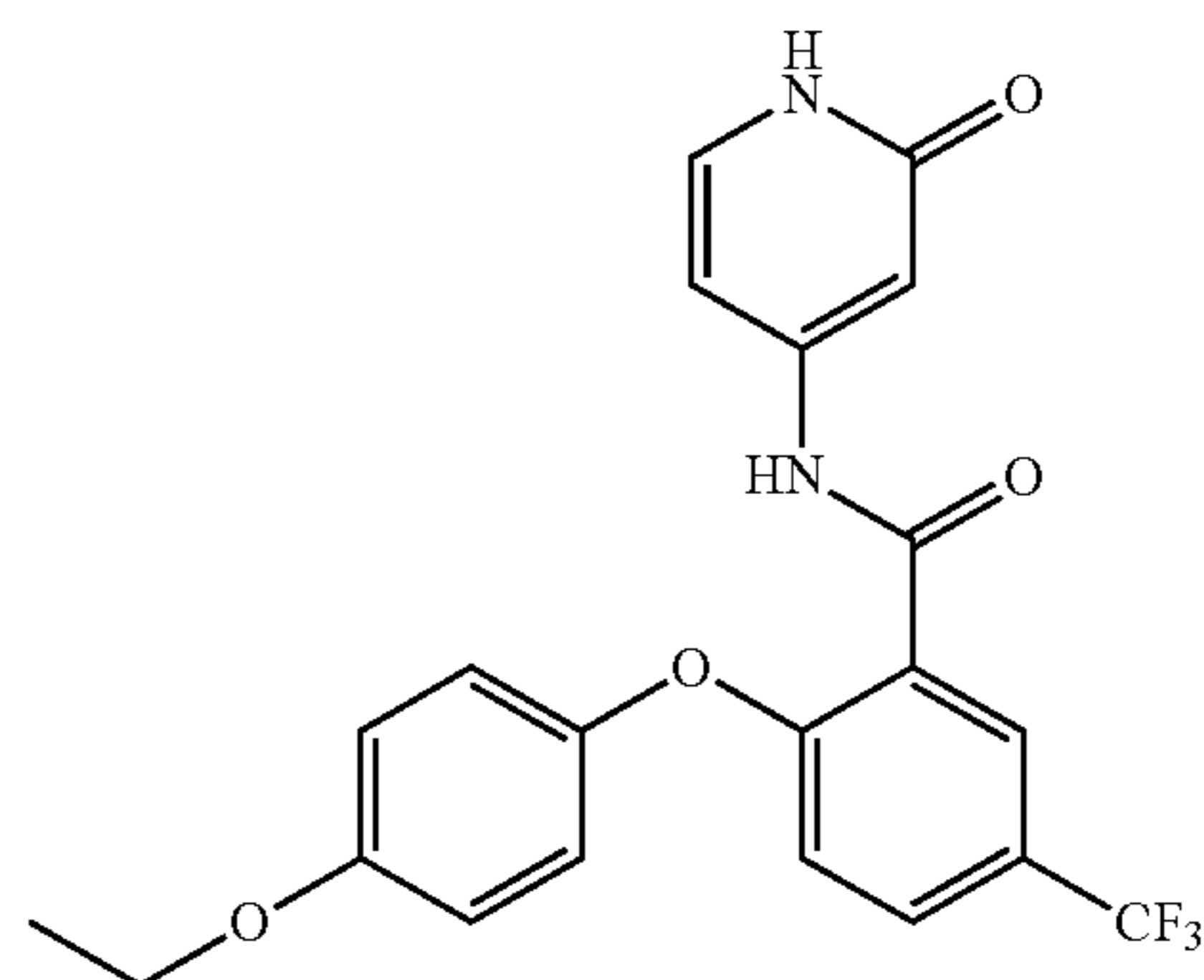
2-(4-ethoxyphenoxy)-N-(2-oxo-1,2-dihydropyridin-4-yl)-5-(trifluoromethyl)benzamide
