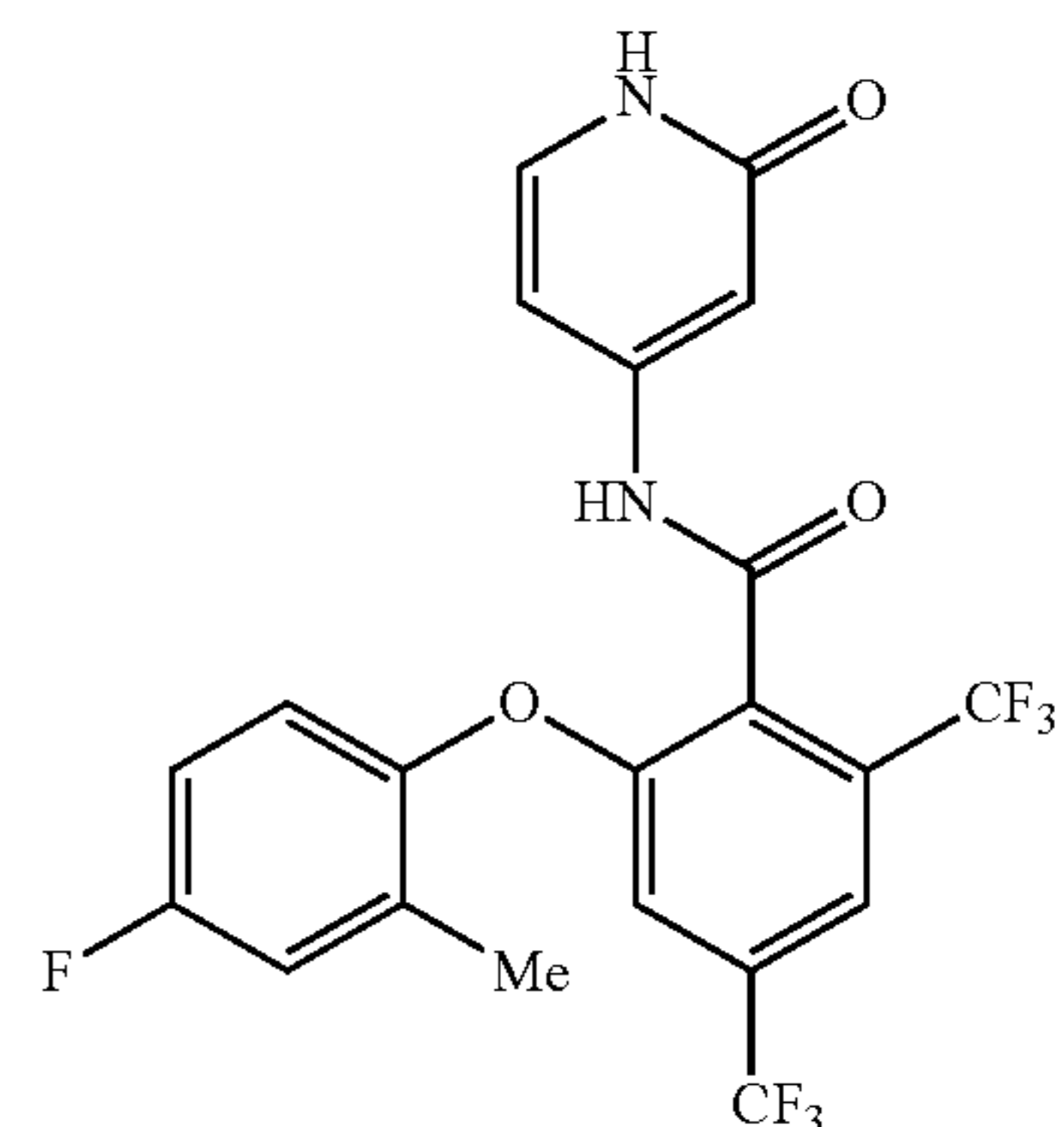
2-(4-fluoro-2-methylphenoxy)-N-(2-oxo-1,2-dihydropyridin-4-yl)-4,6-bis(trifluoromethyl)benzamide
