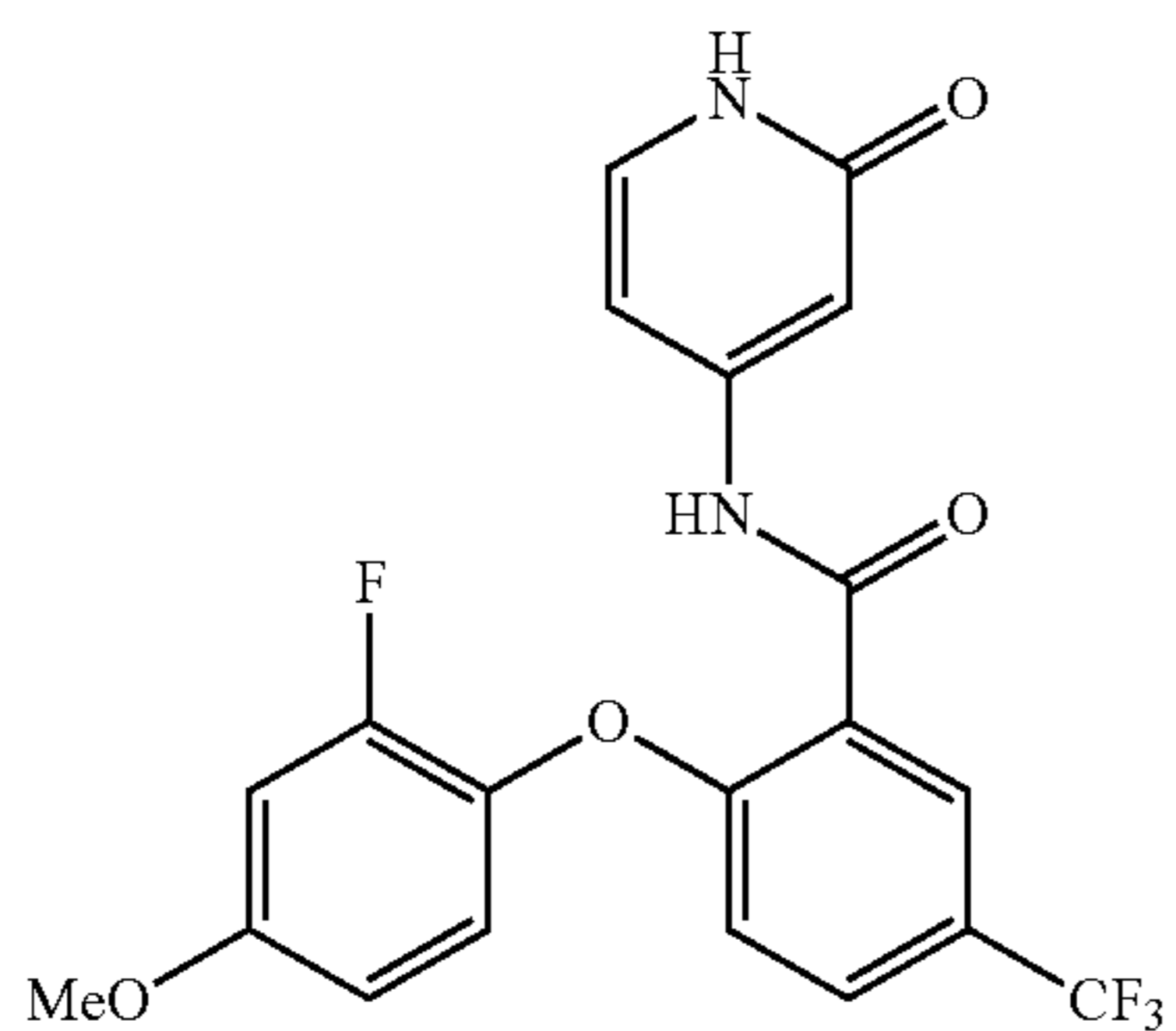
2-(2-fluoro-4-methoxyphenoxy)-N-(2-oxo-1,2-dihydropyridin-4-yl)-5-(trifluoromethyl)benzamide
