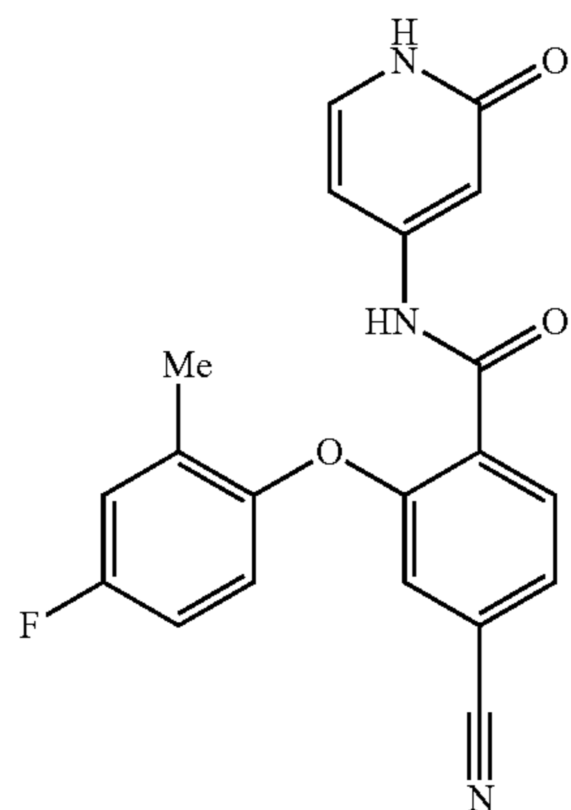
4-cyano-2-(4-fluoro-2-methylphenoxy)-N-(2-oxo-1,2-dihydropyridin-4-yl)benzamide
