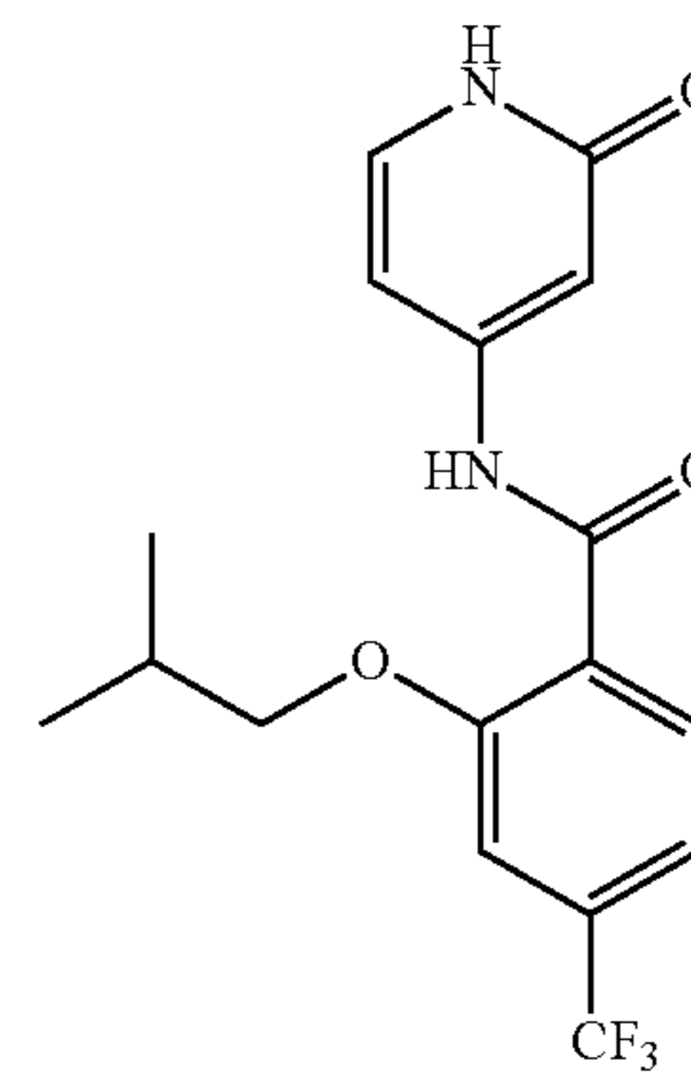
2-isobutoxy-N-(2-oxo-1,2-dihydropyridin-4-yl)-4-(trifluoromethyl)benzamide
