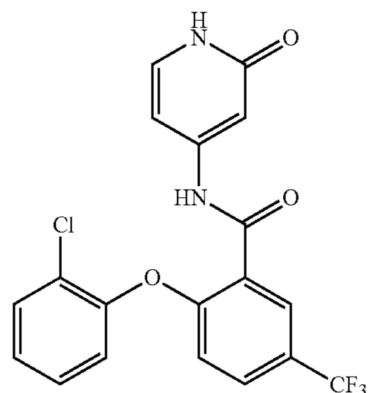
2-(2-chlorophenoxy)-N-(2-oxo-1,2-dihydropyridin-4-yl)-5-(trifluoromethyl)benzamide
