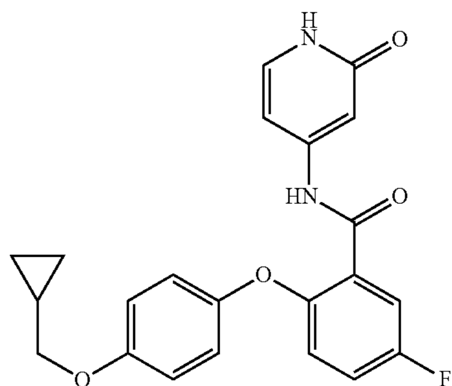
2-(4-(cyclopropylmethoxy)phenoxy)-5-fluoro-N-(2-oxo-1,2-dihydropyridin-4-yl)benzamide
