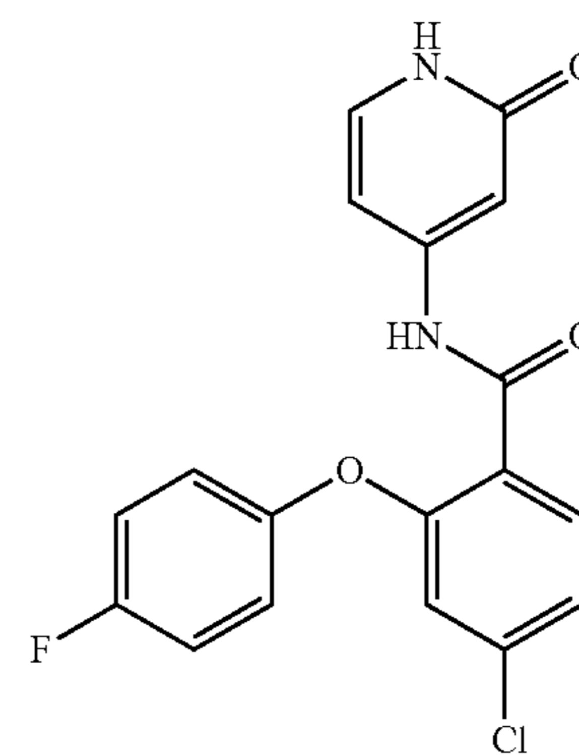
4-chloro-2-(4-fluorophenoxy)-N-(2-oxo-1,2-dihydropyridin-4-yl)benzamide
