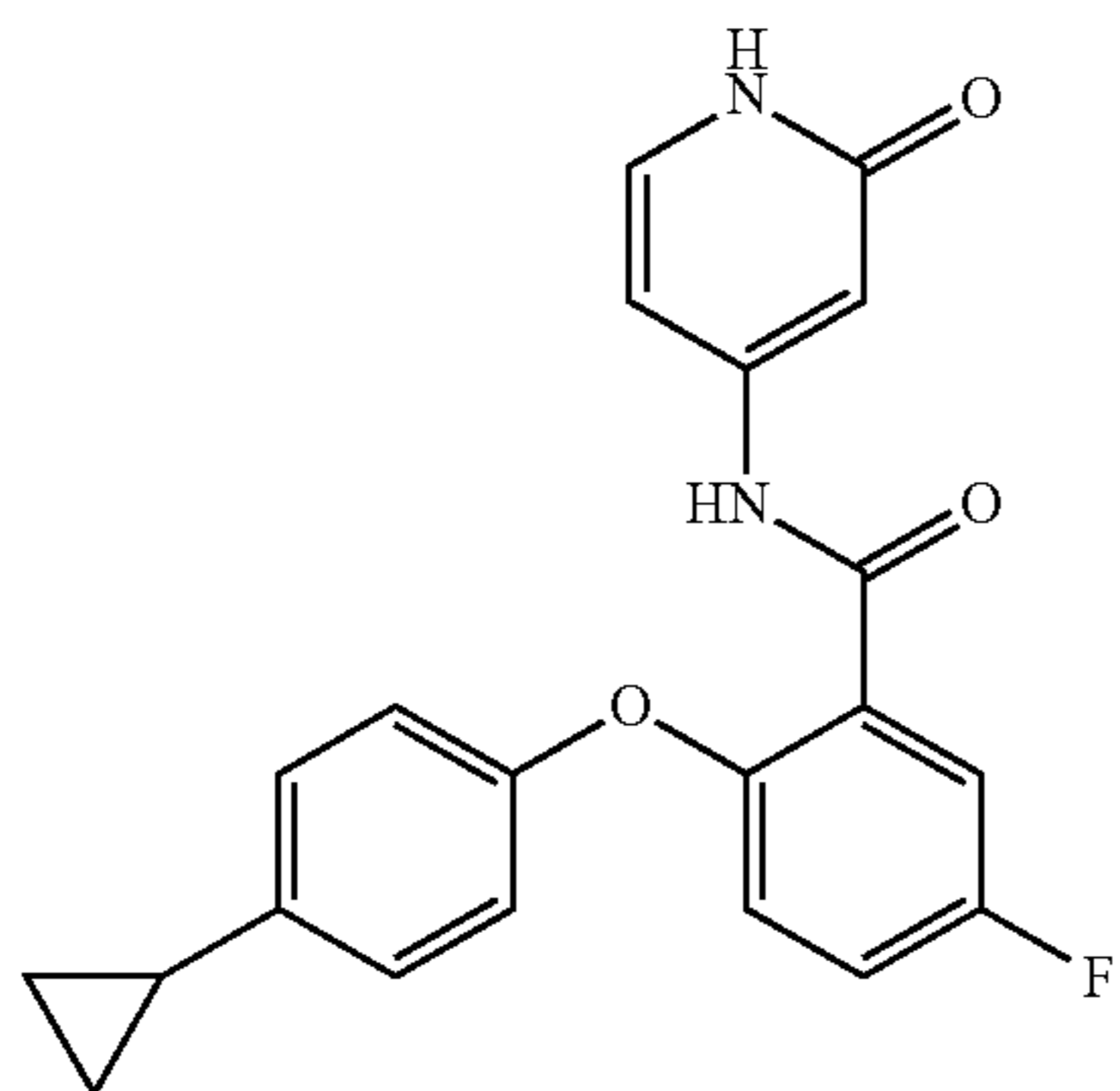
2-(4-cyclopropylphenoxy)-5-fluoro-N-(2-oxo-1,2-dihydropyridin-4-yl)benzamide
