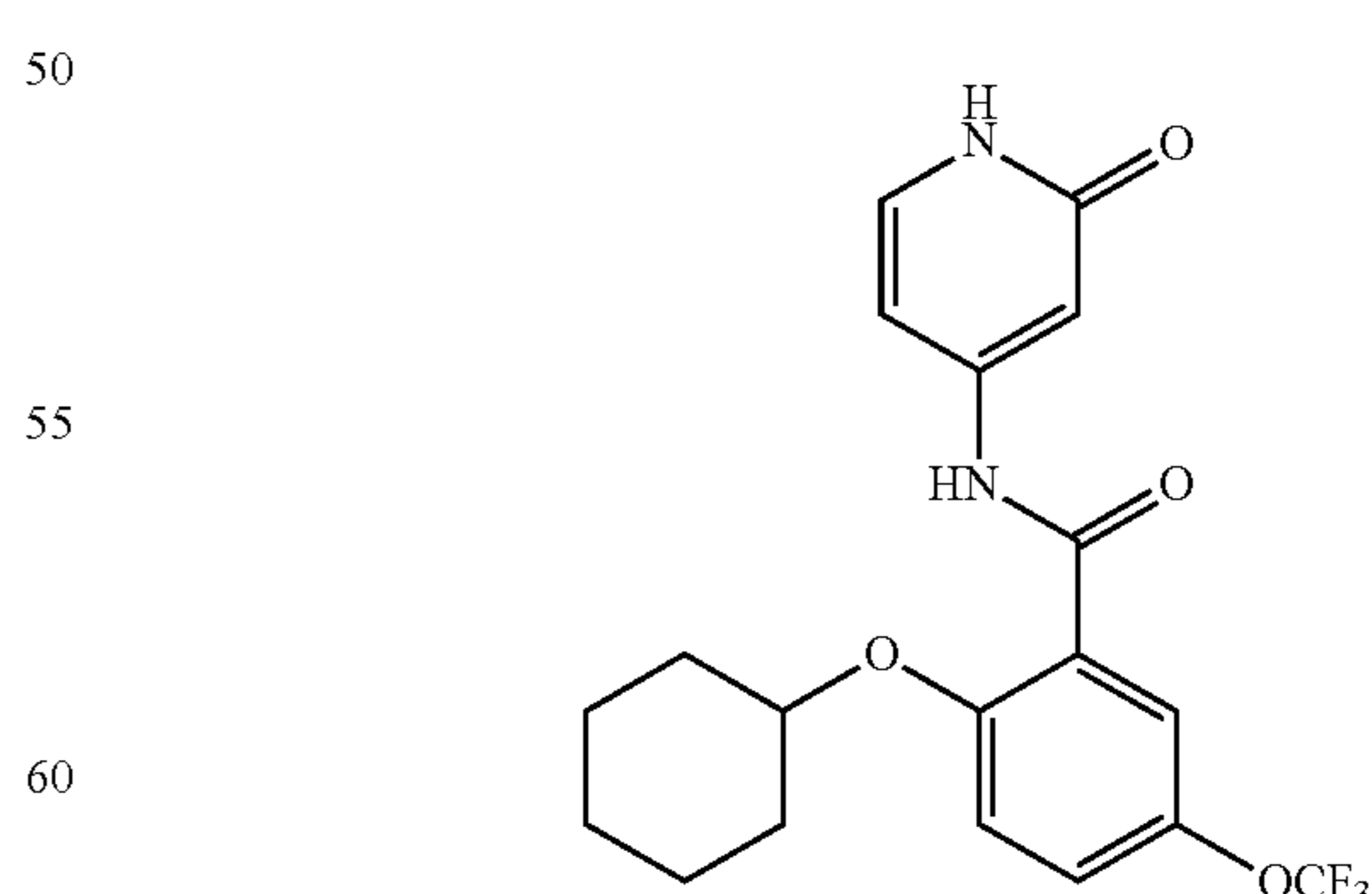
2-(cyclohexyloxy)-N-(2-oxo-1,2-dihydropyridin-4-yl)-5-(trifluoromethoxy)benzamide
