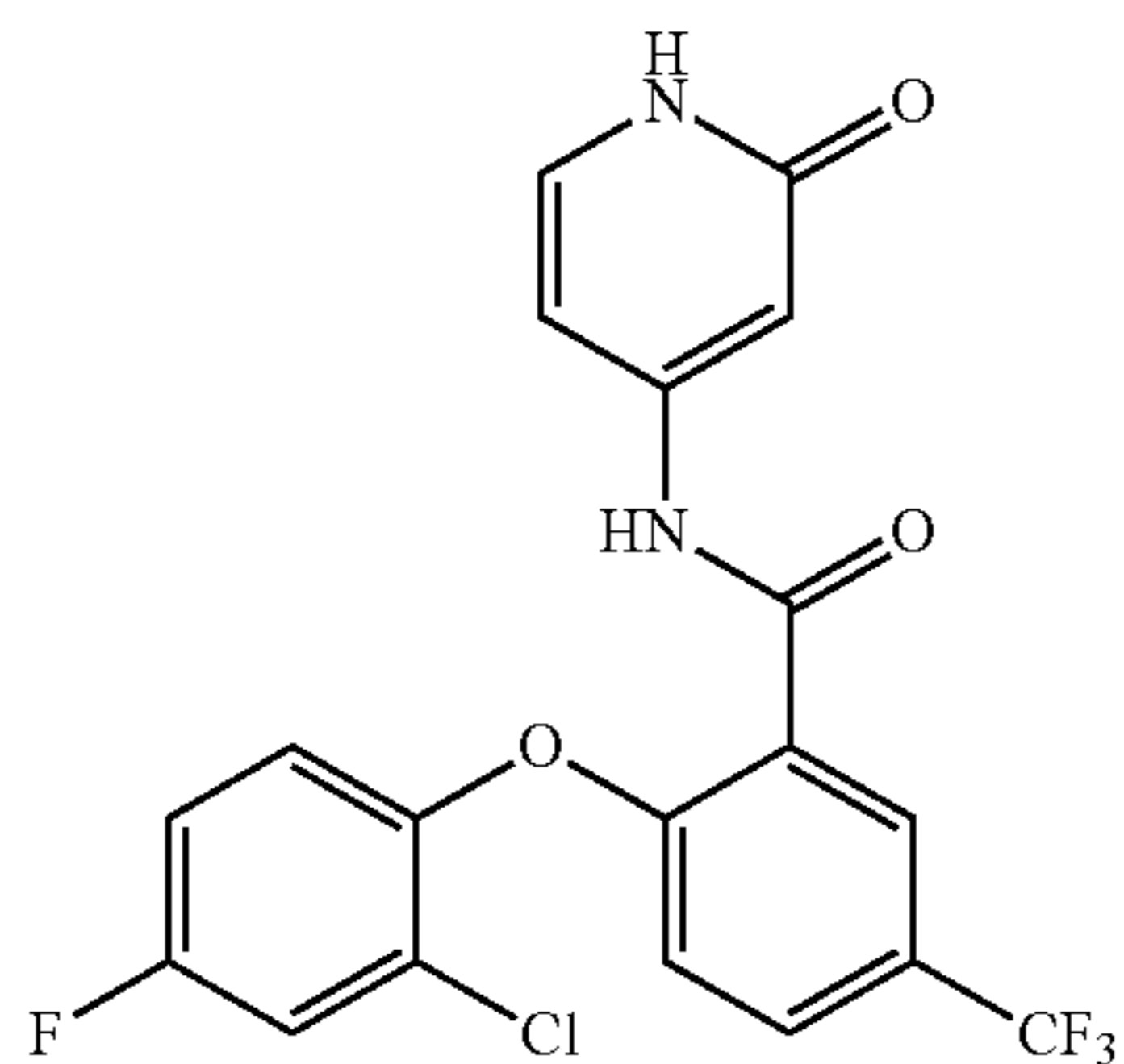
2-(2-chloro-4-fluorophenoxy)-N-(2-oxo-1,2-dihydropyridin-4-yl)-5-(trifluoromethyl)benzamide
