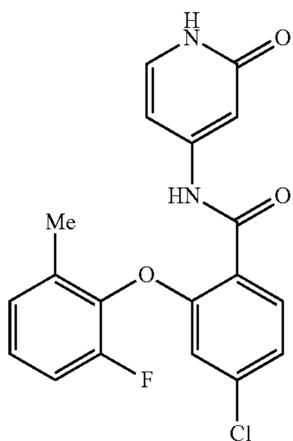
4-chloro-2-(2-fluoro-6-methylphenoxy)-N-(2-oxo-1,2-dihydropyridin-4-yl)benzamide
