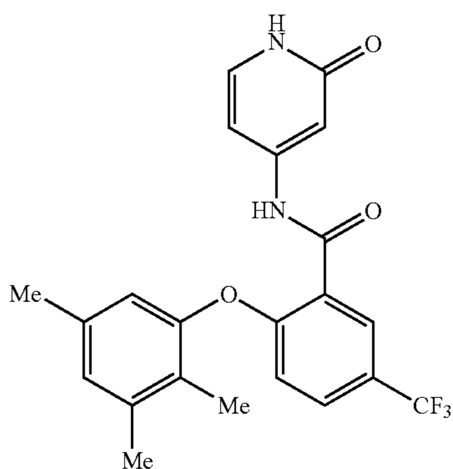
N-(2-oxo-1,2-dihydropyridin-4-yl)-5-(trifluoromethyl)-2-(2,3,5-trimethylphenoxy)benzamide
