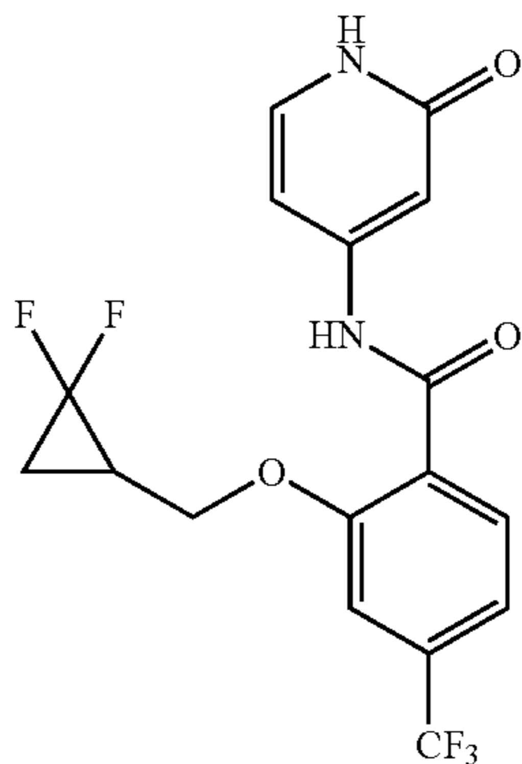
2-((2,2-difluorocyclopropyl)methoxy)-N-(2-oxo-1,2-dihydropyridin-4-yl)-4-(trifluoromethyl)benzamide
