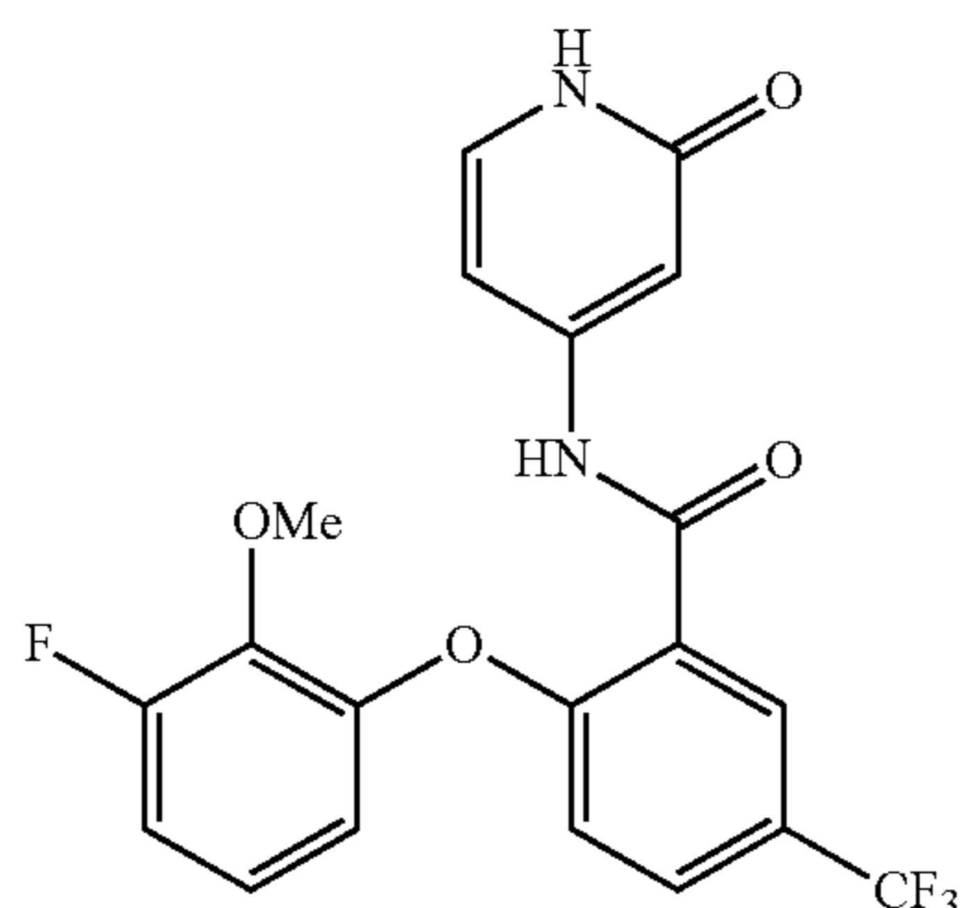
2-(3-fluoro-2-methoxyphenoxy)-N-(2-oxo-1,2-dihydropyridin-4-yl)-5-(trifluoromethyl)benzamide
