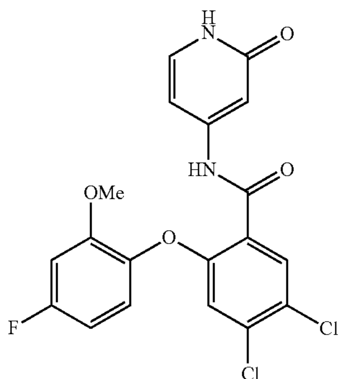
4,5-dichloro-2-(4-fluoro-2-methoxyphenoxy)-N-(2-oxo-1,2-dihydropyridin-4-yl)benzamide
