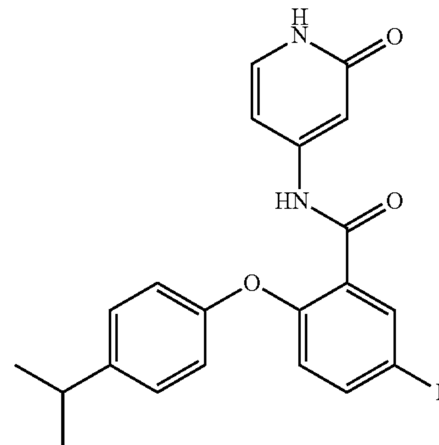
5-fluoro-2-(4-isopropylphenoxy)-N-(2-oxo-1,2-dihydropyridin-4-yl)benzamide
