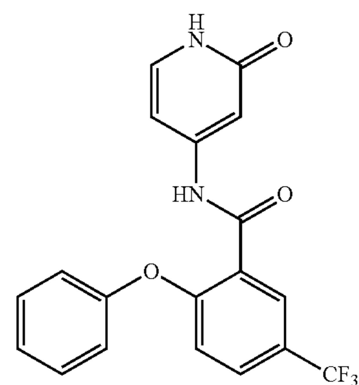
N-(2-oxo-1,2-dihydropyridin-4-yl)-2-phenoxy-5-(trifluoromethyl)benzamide
