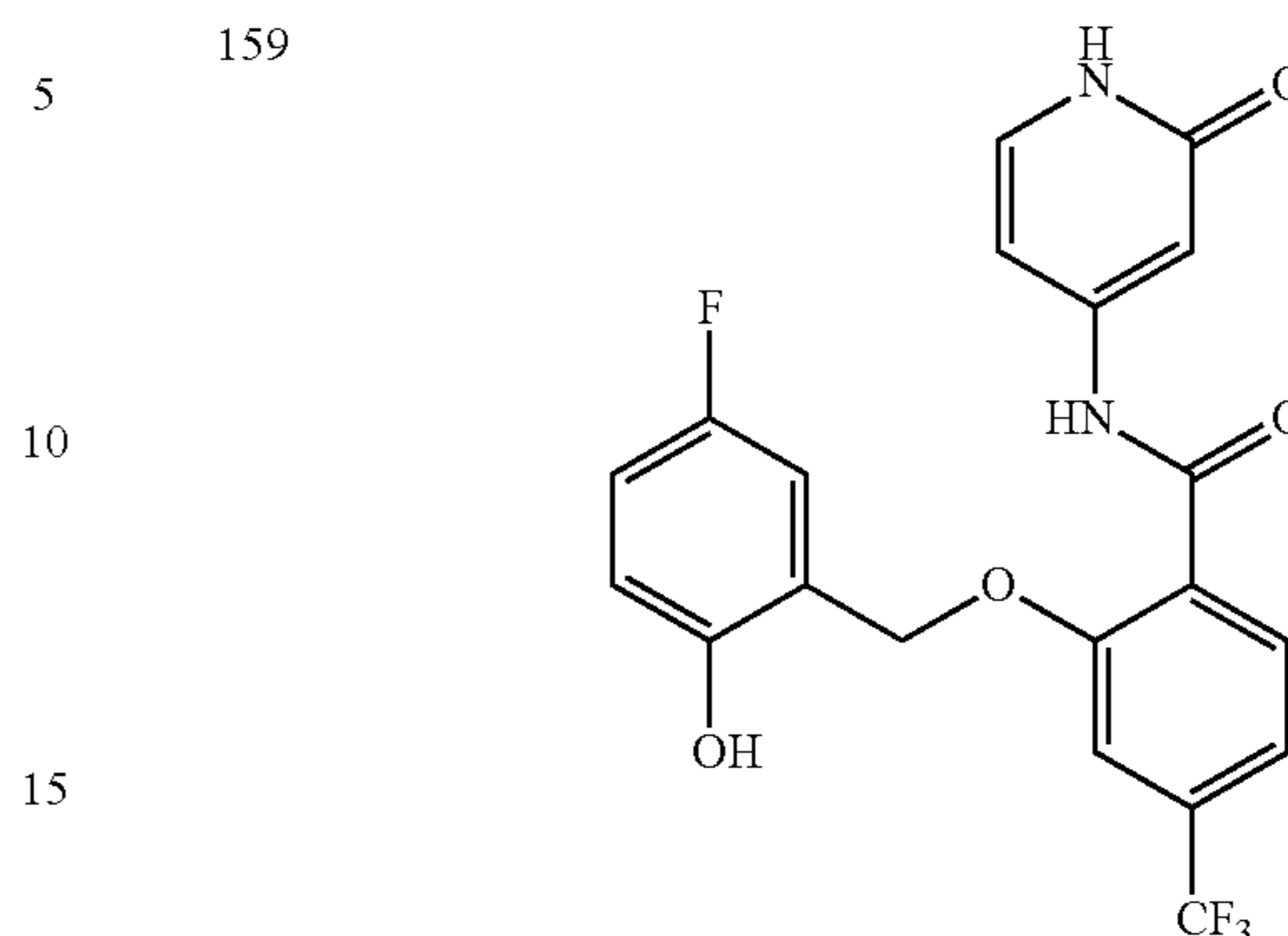
2-((5-fluoro-2-hydroxybenzyl)oxy)-N-(2-oxo-1,2-dihydropyridin-4-yl)-4-(trifluoromethyl)benzamide
