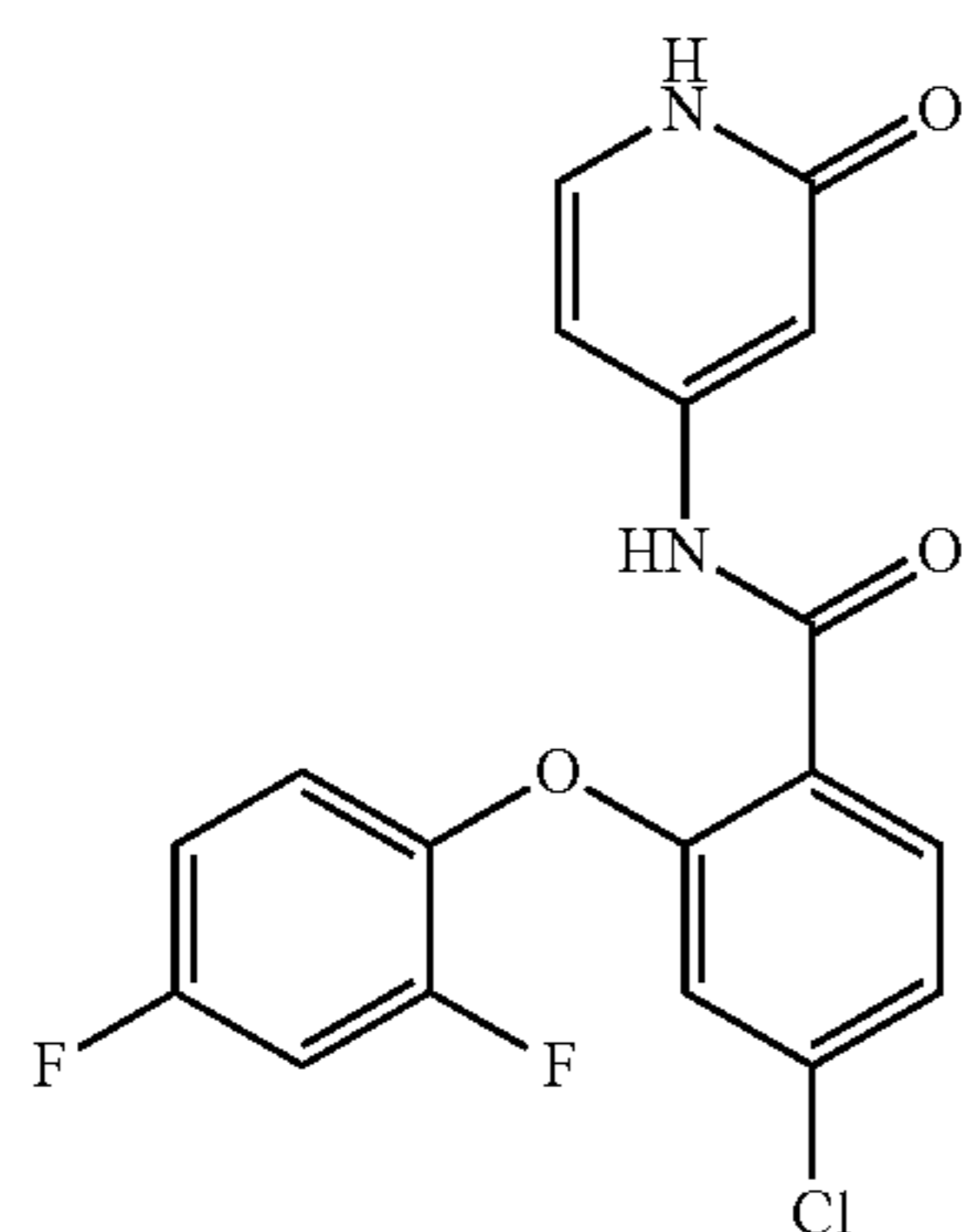
4-chloro-2-(2,4-difluorophenoxy)-N-(2-oxo-1,2-dihydropyridin-4-yl)benzamide
