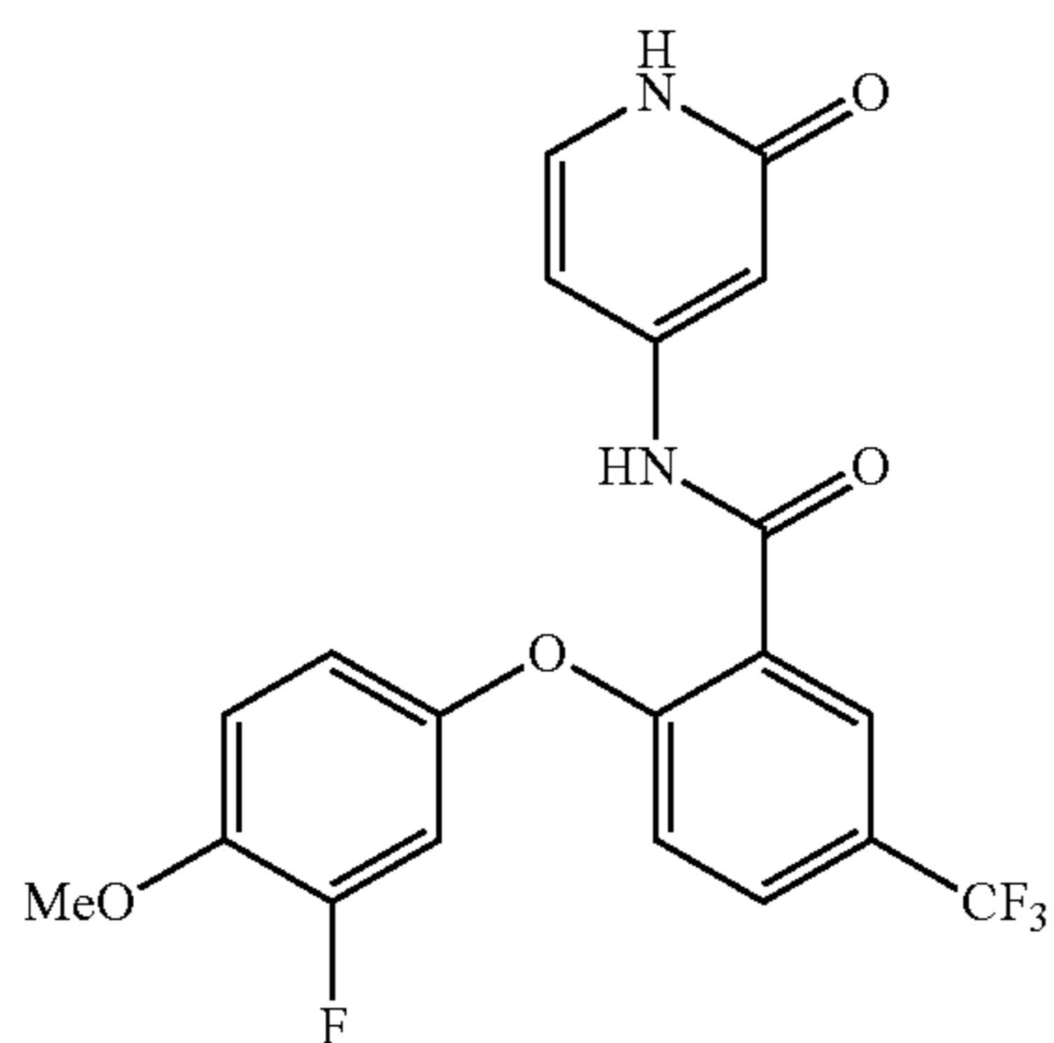
2-(3-fluoro-4-methoxyphenoxy)- N-(2-oxo-1,2-dihydropyridin-4-yl)-5-(trifluoromethyl)benzamide
