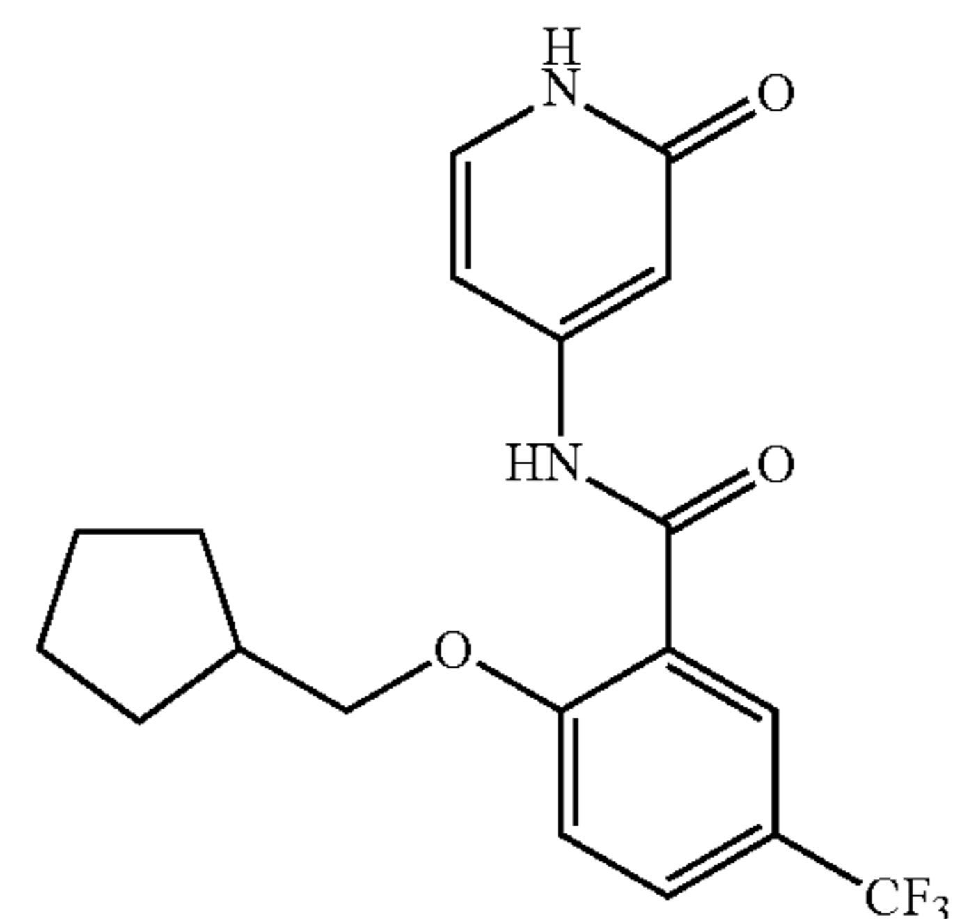
2-(cyclopentylmethoxy)-N-(2-oxo-1,2-dihydropyridin-4-yl)-5-(trifluoromethyl)benzamide
