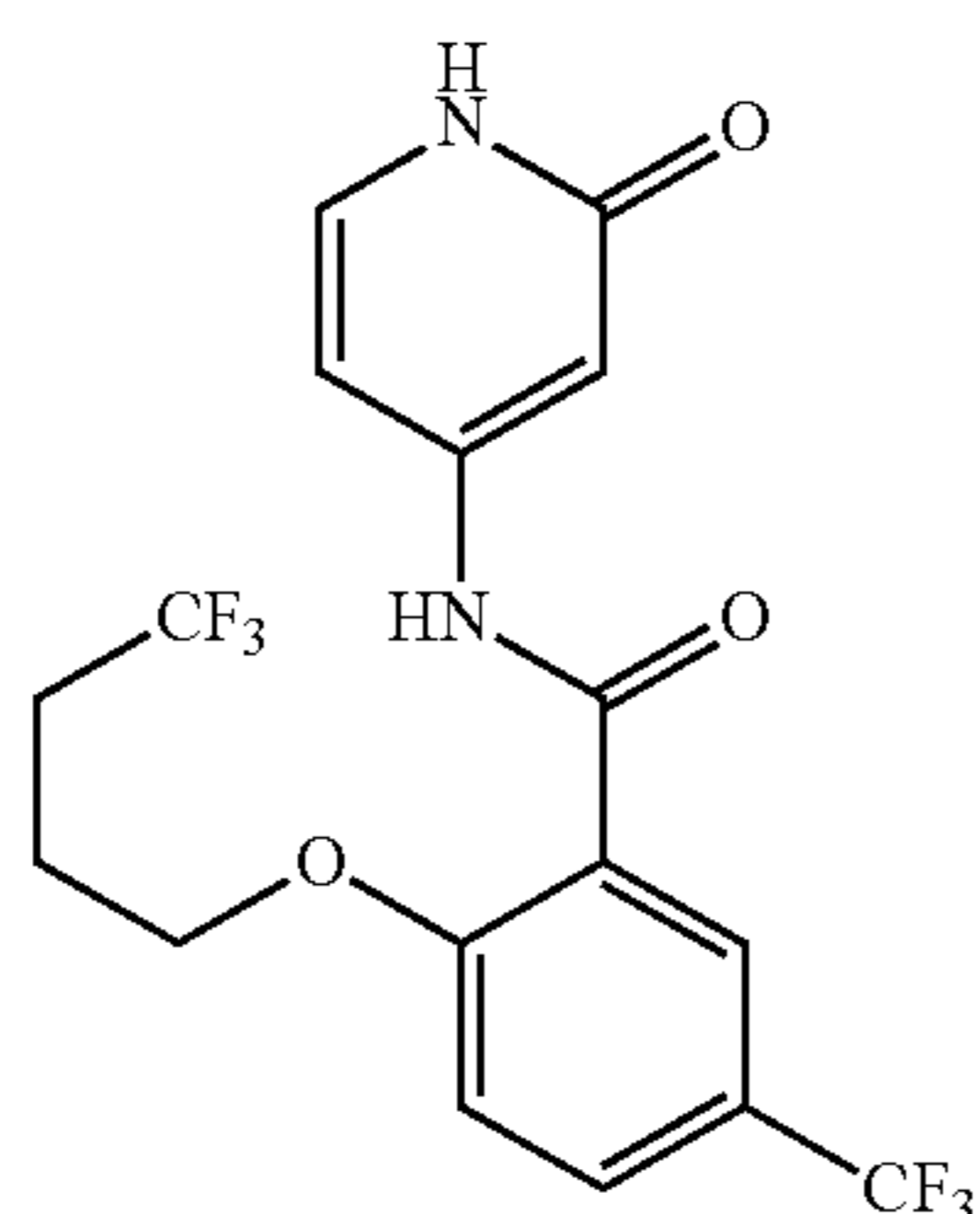
N-(2-oxo-1,2-dihydropyridin-4-yl)-2-(4,4,4-trifluorobutoxy)-5-(trifluoromethyl)benzamide
