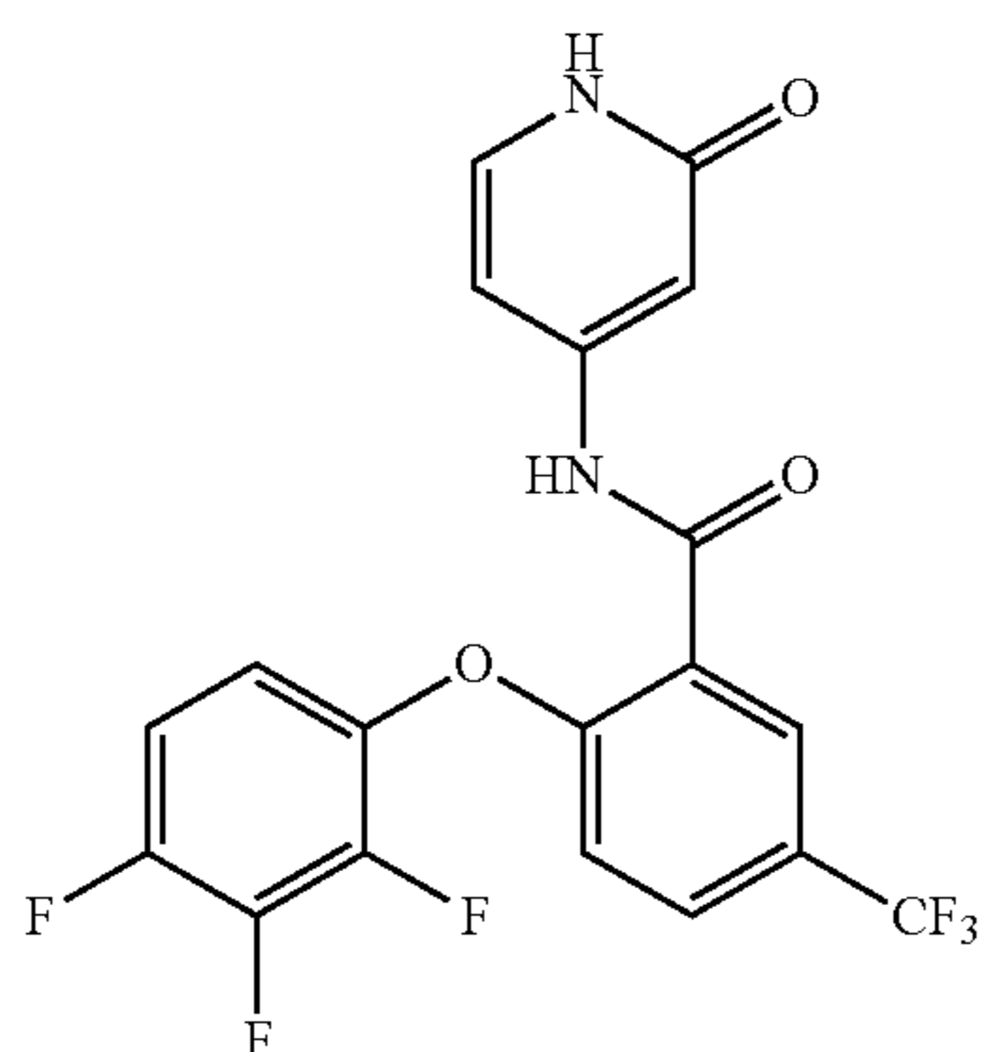
N-(2-oxo-1,2-dihydropyridin-4-yl)-5-(trifluoromethyl)-2-(2,3,4-trifluorophenoxy)benzamide
