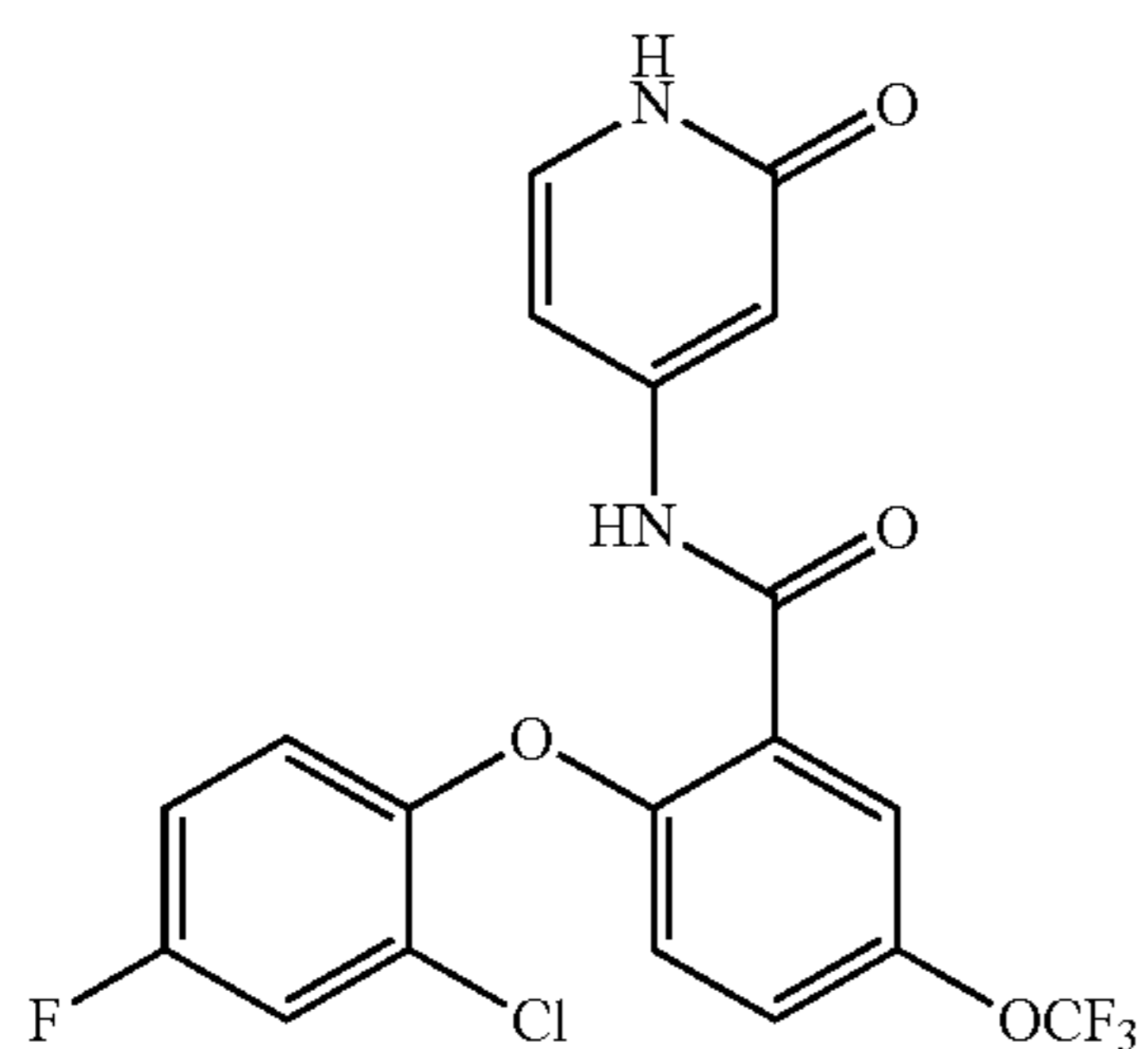
2-(2-chloro-4-fluorophenoxy)-N-(2-oxo-1,2-dihydropyridin-4-yl)-5-(trifluoromethoxy)benzamide
