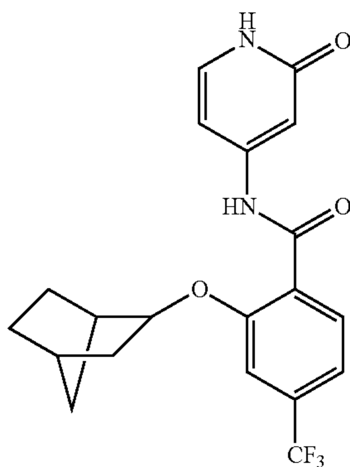
2-(bicyclo[2.2.1]heptan-2-yloxy)-N-(2-oxo-1,2-dihydropyridin-4-yl)-4-(trifluoromethyl)benzamide
