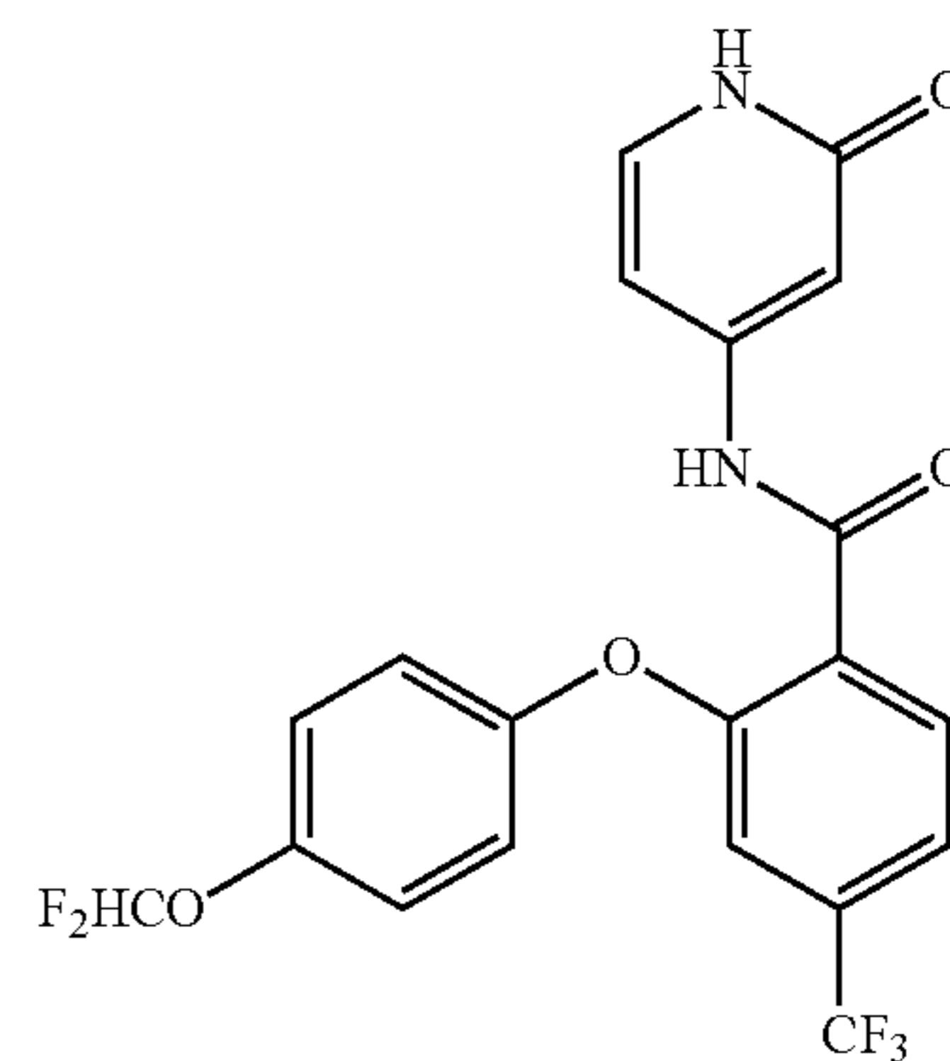
2-(2-(difluoromethoxy)phenoxy)-N-(2-oxo-1,2-dihydropyridin-4-yl)-4-(trifluoromethyl)benzamide
