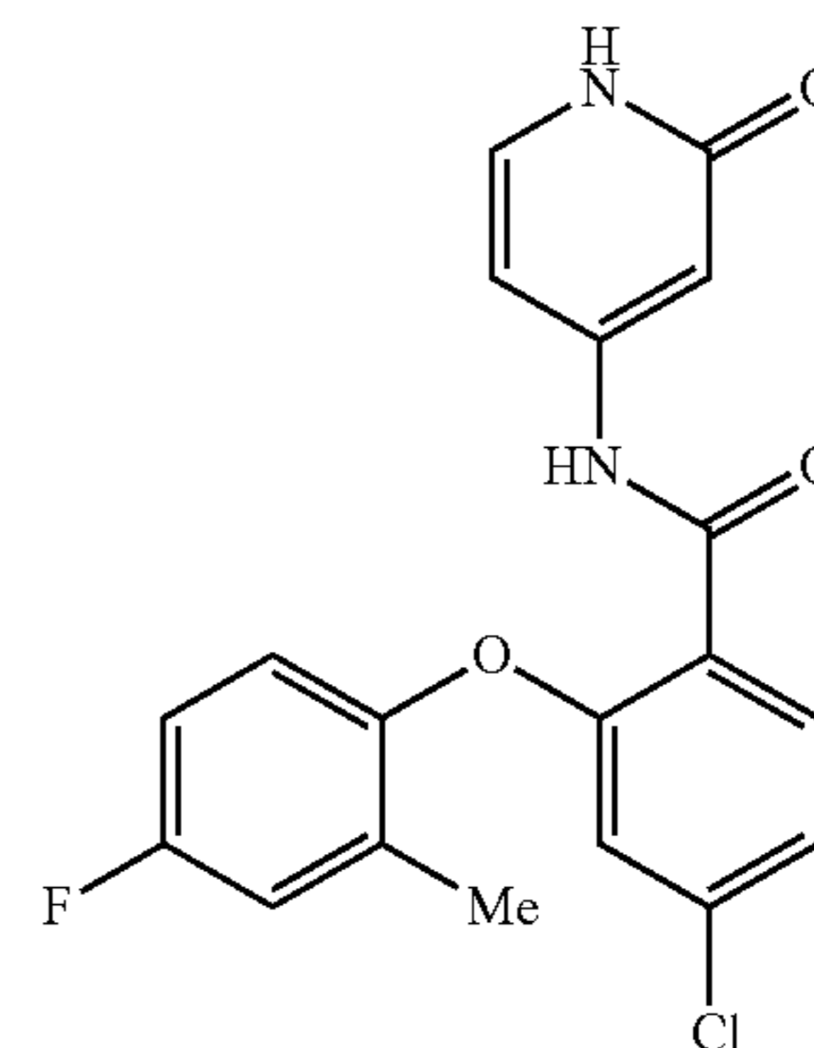
4-chloro-2-(4-fluoro-2-methylphenoxy)-N-(2-oxo-1,2-dihydropyridin-4-yl)benzamide
