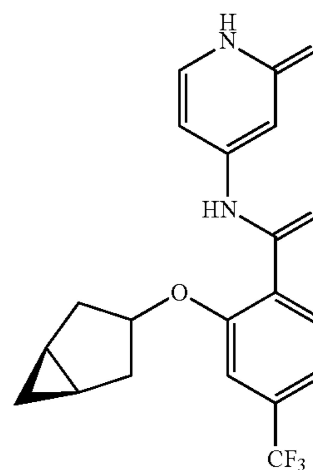
2-((1R,5S)-bicyclo[3.1.0]hexan-3-yloxy)-N-(2-oxo-1,2-dihydropyridin-4-yl)-4-(trifluoromethyl)benzamide
