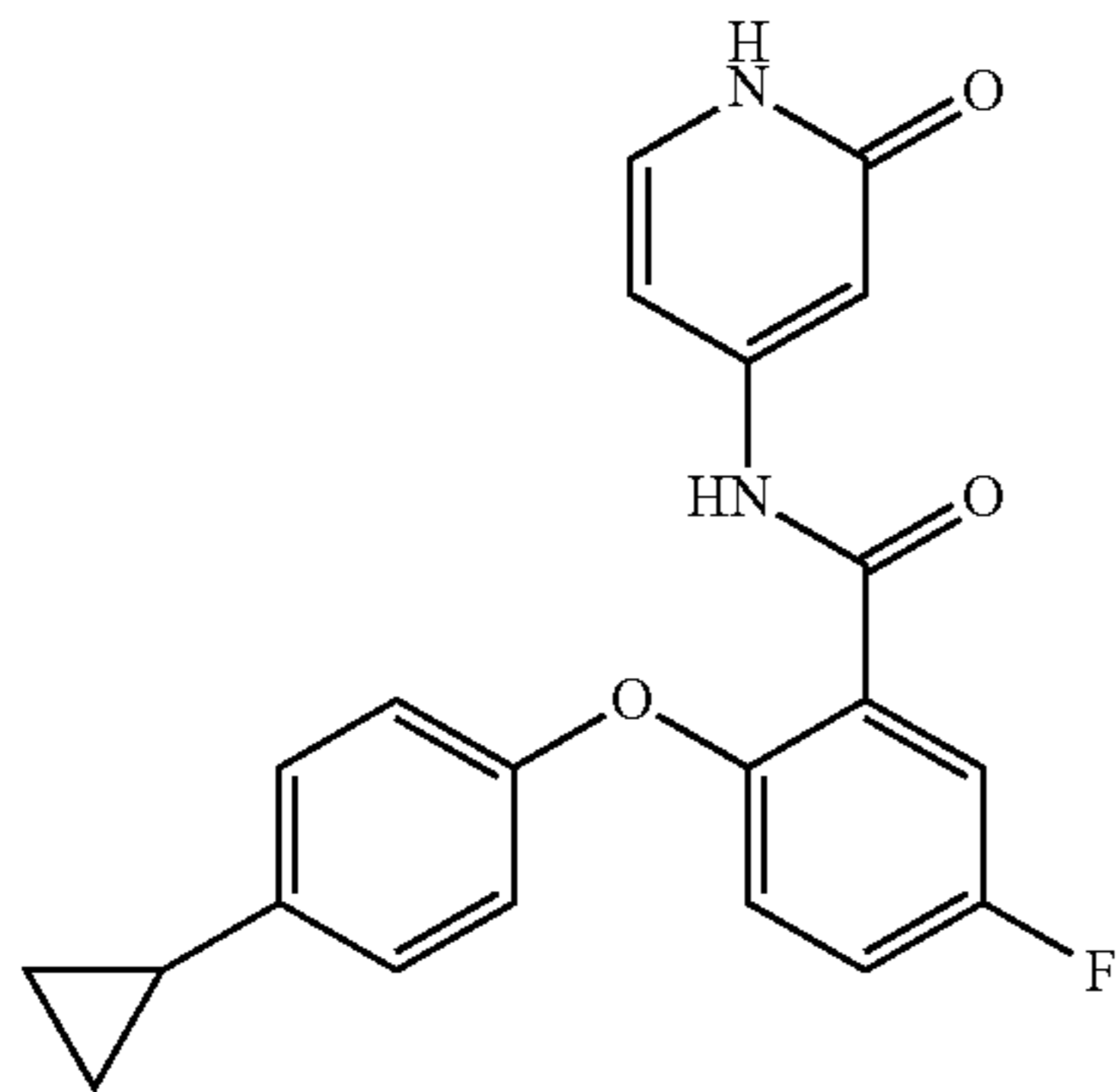
2-(4-cyclopropylphenoxy)-5-fluoro-N-(2-oxo-1,2-dihydropyridin-4-yl)benzamide
