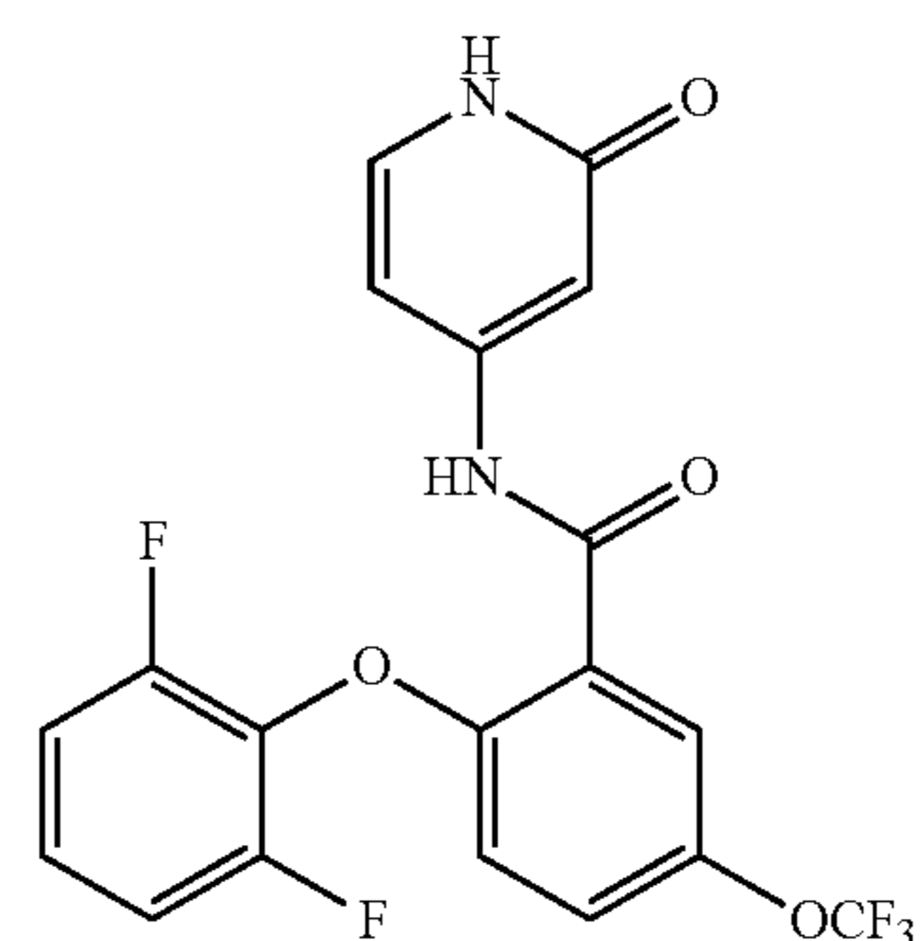
2-(2,6-difluorophenoxy)-N-(2-oxo-1,2-dihydropyridin-4-yl)-5-(trifluoromethoxy)benzamide
