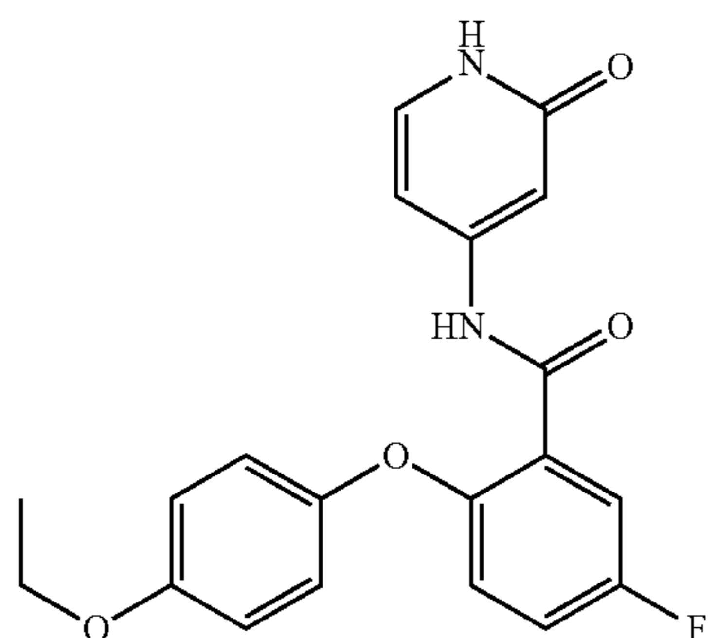
2-(4-ethoxyphenoxy)-5-fluoro-N-(2-oxo-1,2-dihydropyridin-4-yl)benzamide
