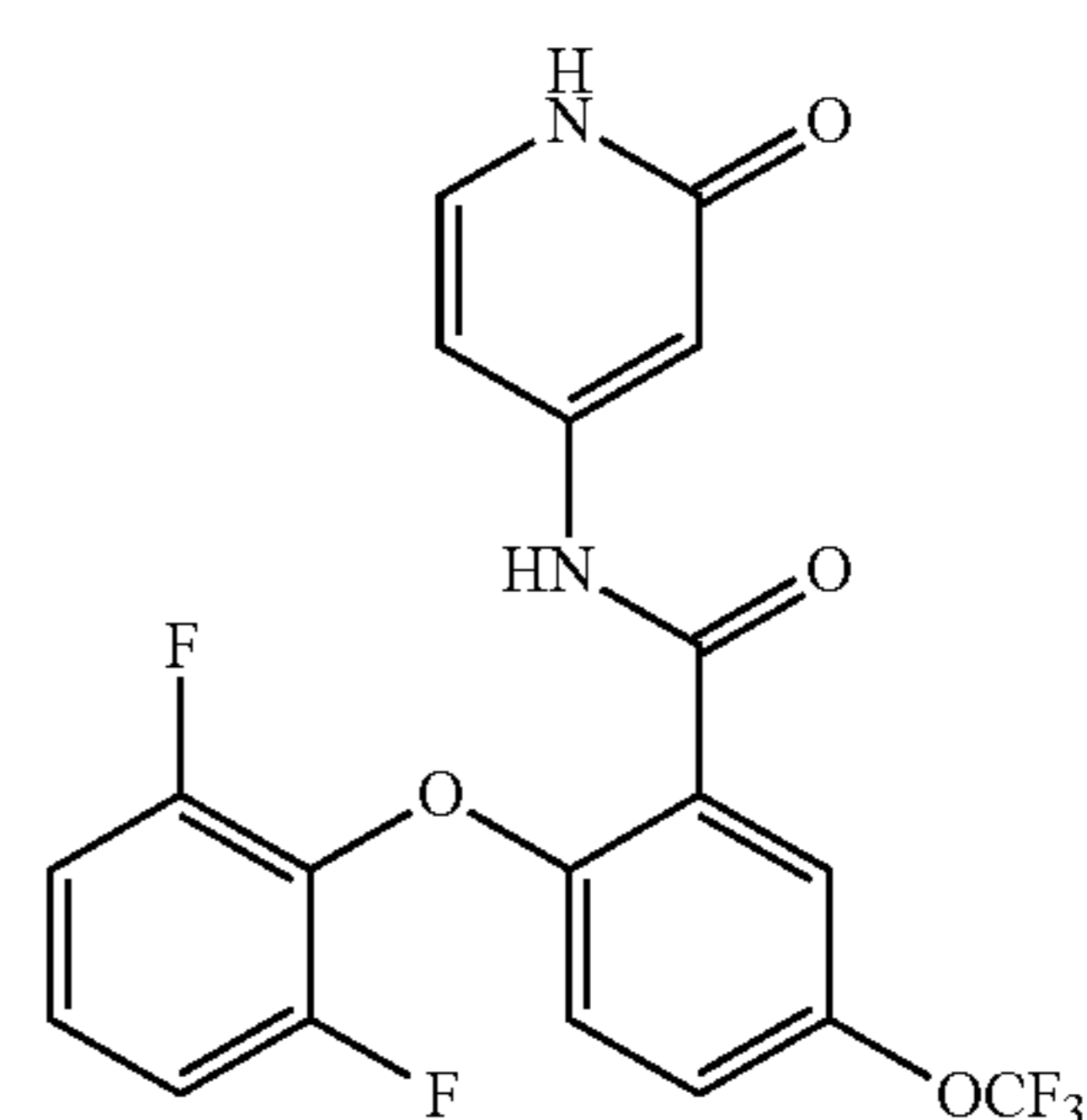
2-(2,6-difluorophenoxy)-N-(2-oxo-1,2-dihydropyridin-4-yl)-5-(trifluoromethoxy)benzamide
