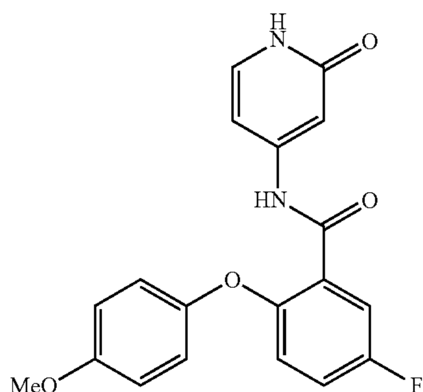
5-fluoro-2-(4-methoxyphenoxy)-N-(2-oxo-1,2-dihydropyridin-4-yl)benzamide
