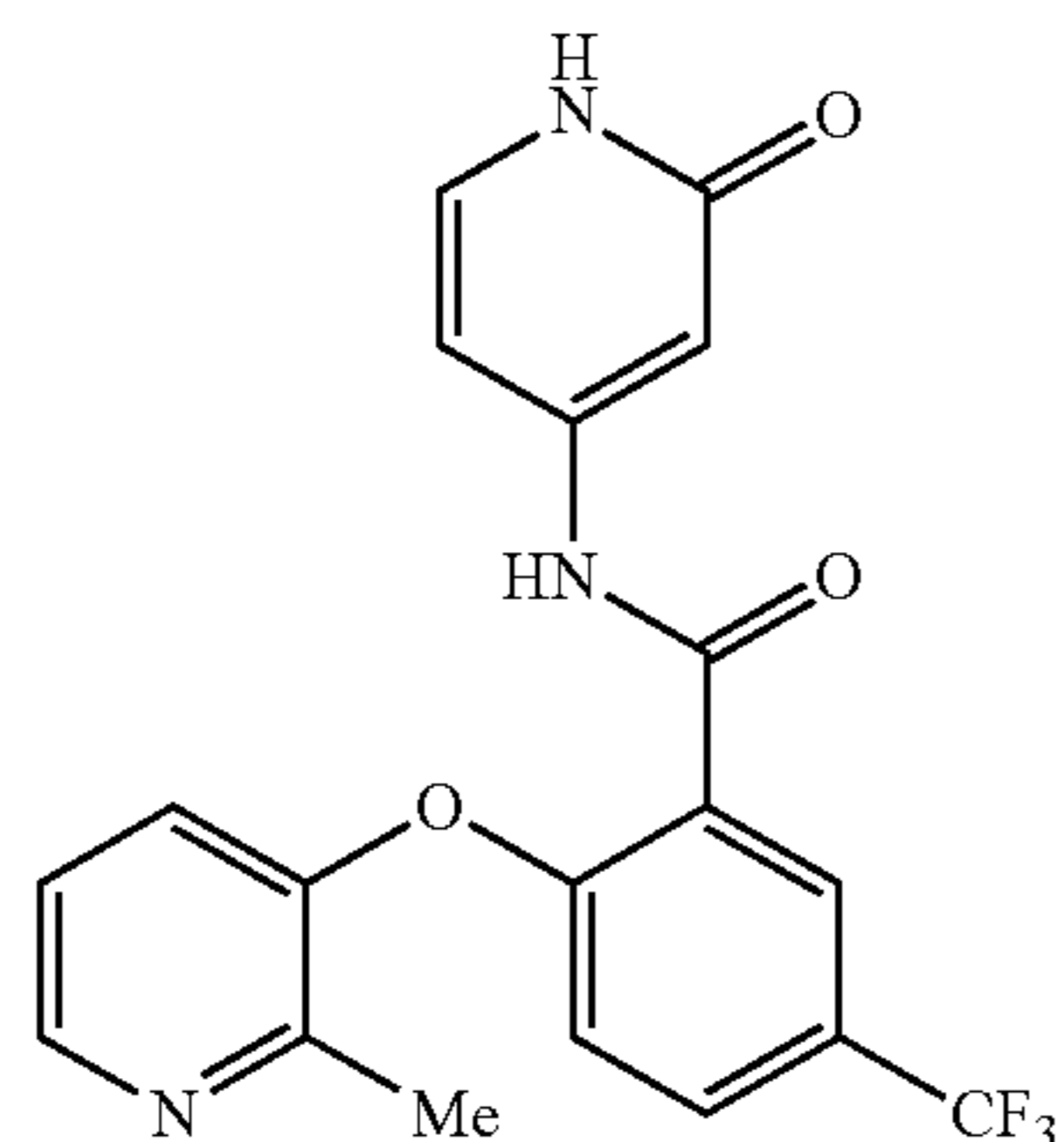
2-((2-methylpyridin-3-yl)oxy)-N-(2-oxo-1,2-dihydropyridin-4-yl)-5-(trifluoromethyl)benzamide
