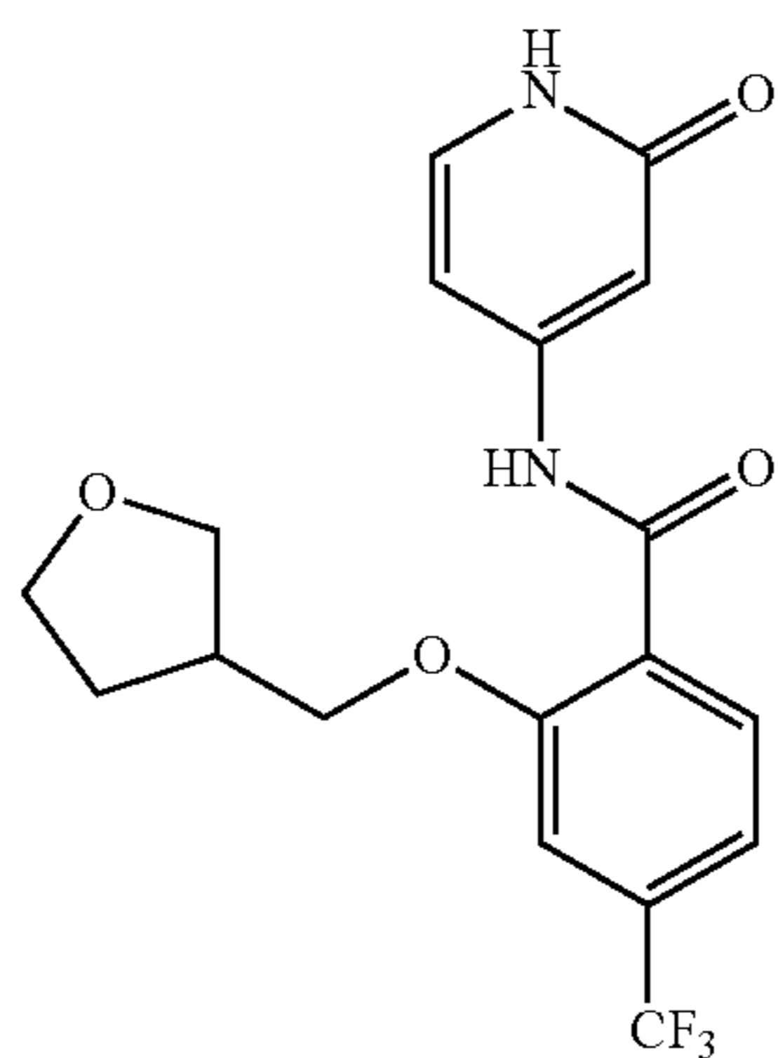
N-(2-oxo-1,2-dihydropyridin-4-yl)-2-((tetrahydrofuran-3-yl)methoxy)-4-(trifluoromethyl)benzamide
