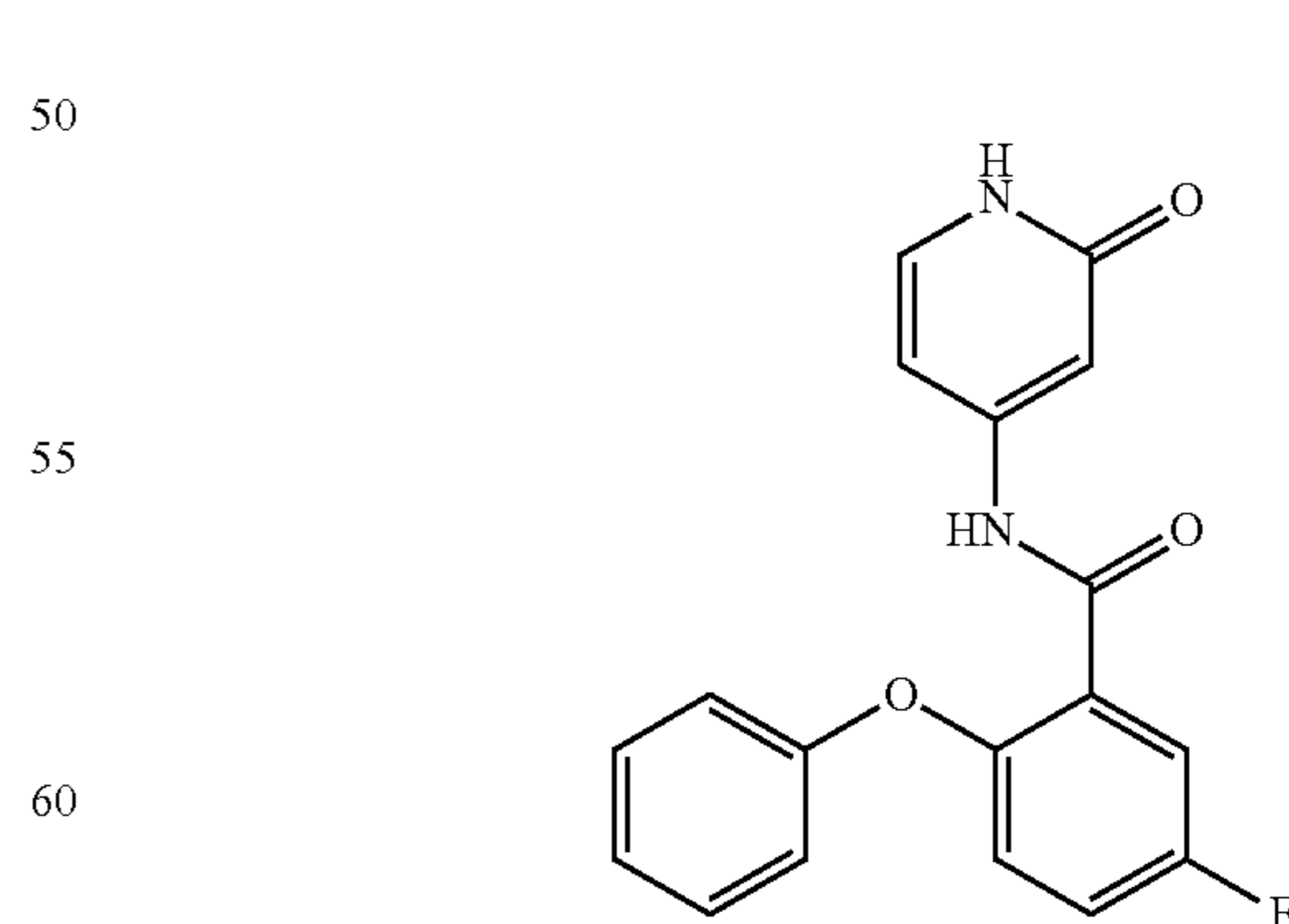
5-fluoro-N-(2-oxo-1,2-dihydropyridin-4-yl)-2-phenoxybenzamide
