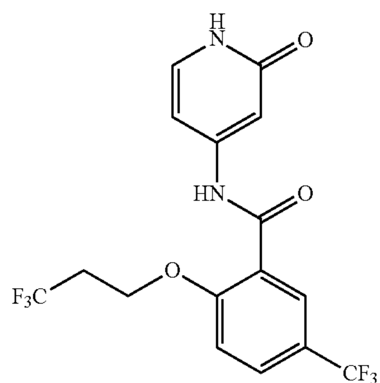
N-(2-oxo-1,2-dihydropyridin-4-yl)-5-(trifluoromethyl)-2-(3,3,3-trifluoropropoxy)benzamide
