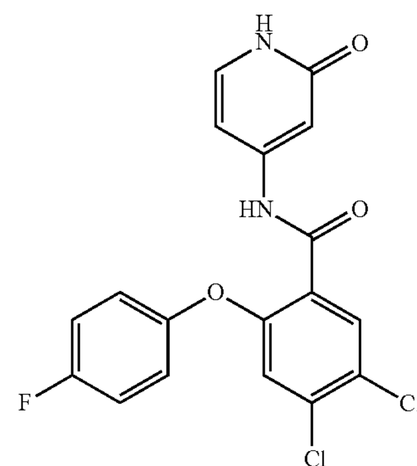
4,5-dichloro-2-(4-fluorophenoxy)-N-(2-oxo-1,2-dihydropyridin-4-yl)benzamide
