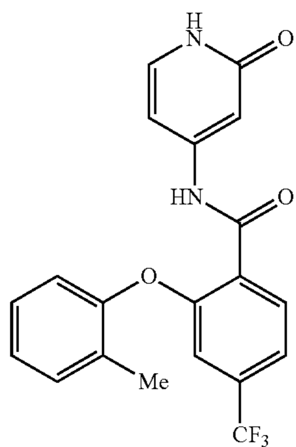
N-(2-oxo-1,2-dihydropyridin-4-yl)-2-(o-tolyloxy)-4-(trifluoromethyl)benzamide
