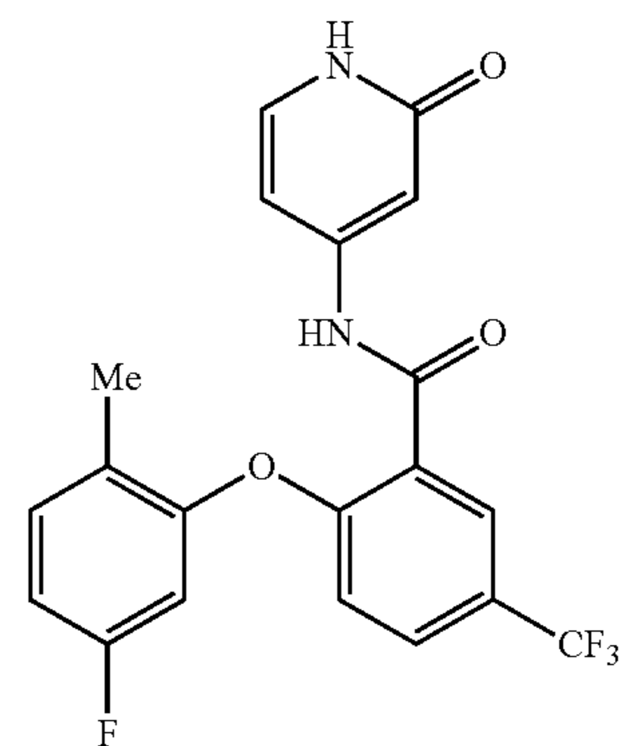
2-(5-fluoro-2-methylphenoxy)-N-(2-oxo-1,2-dihydropyridin-4-yl)-5-(trifluoromethyl)benzamide
