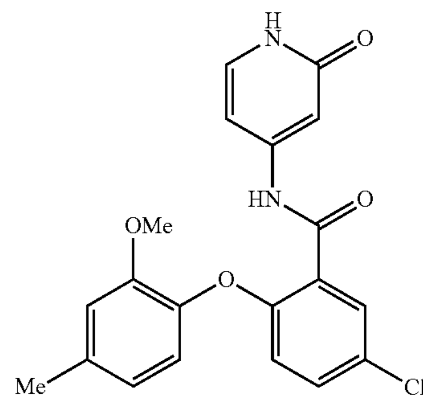
5-chloro-2-(4-fluoro-2-methoxyphenoxy)-N-(2-oxo-1,2-dihydropyridin-4-yl)benzamide
