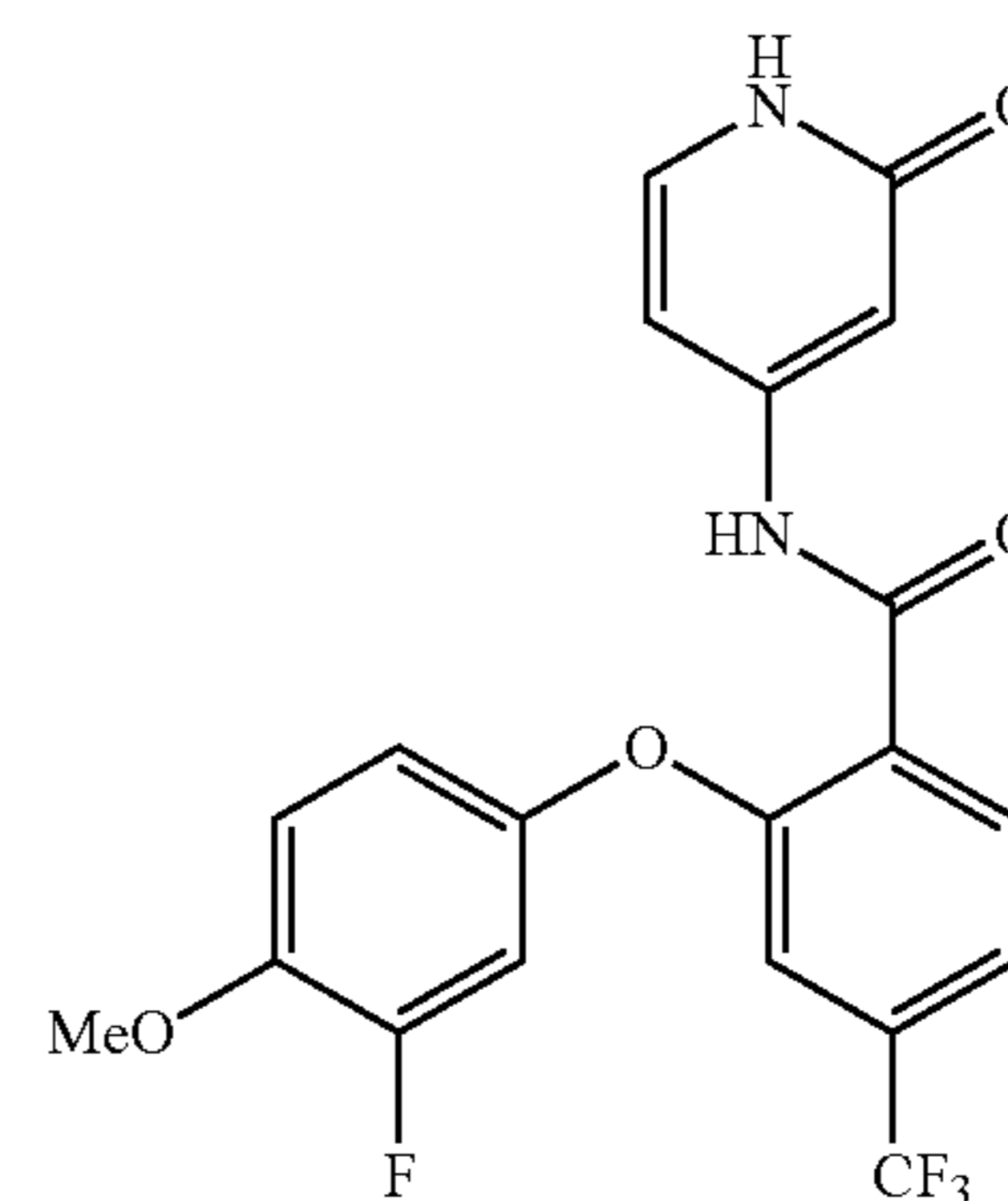
2-(3-fluoro-4-methoxyphenoxy)-N-(2-oxo-1,2-dihydropyridin-4-yl)-4-(trifluoromethyl)benzamide
