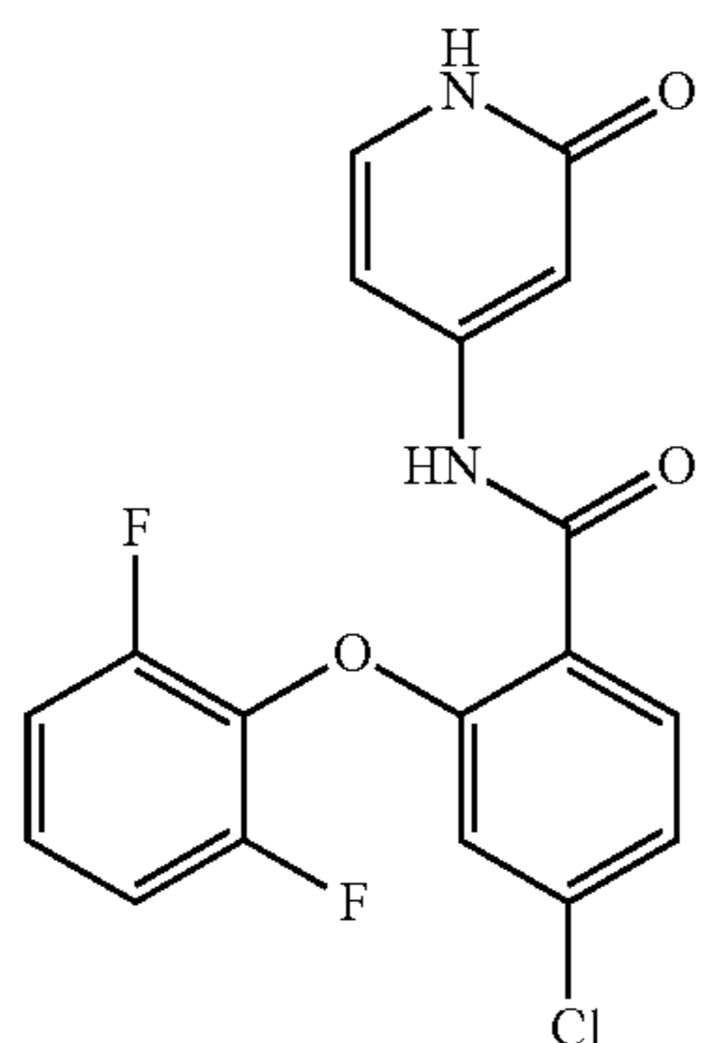
4-chloro-2-(2,6-difluorophenoxy)-N-(2-oxo-1,2-dihydropyridin-4-yl)benzamide
