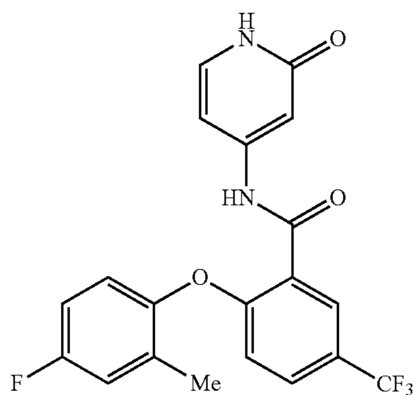
2-(4-fluoro-2-methylphenoxy)-N-(2-oxo-1,2-dihydropyridin-4-yl)-5-(trifluoromethyl)benzamide
