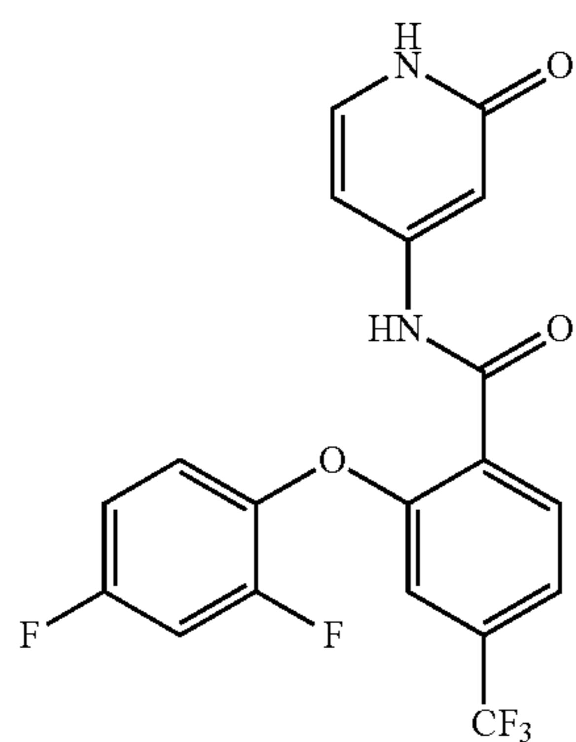
2-(2,4-difluorophenoxy)-N-(2-oxo-1,2-dihydropyridin-4-yl)-4-(trifluoromethyl)benzamide
