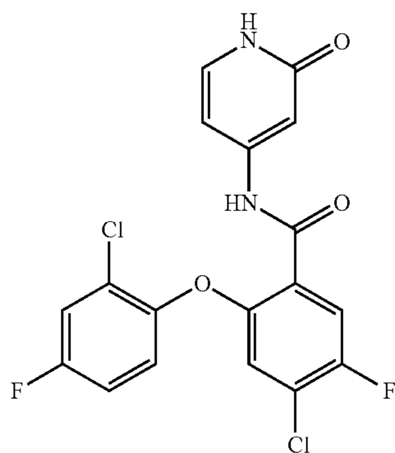
4-chloro-2-(2-chloro-4-fluorophenoxy)-5-fluoro-N-(2-oxo-1,2-dihydropyridin-4-yl)benzamide
