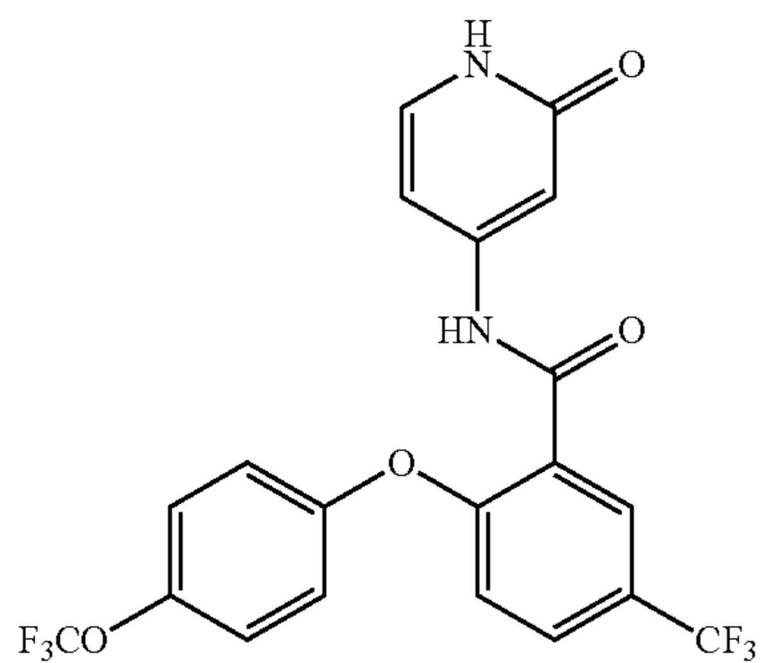
N-(2-oxo-1,2-dihydropyridin-4-yl)-2-(4-(trifluoromethoxy)phenoxy)-5-(trifluoromethyl)benzamide
