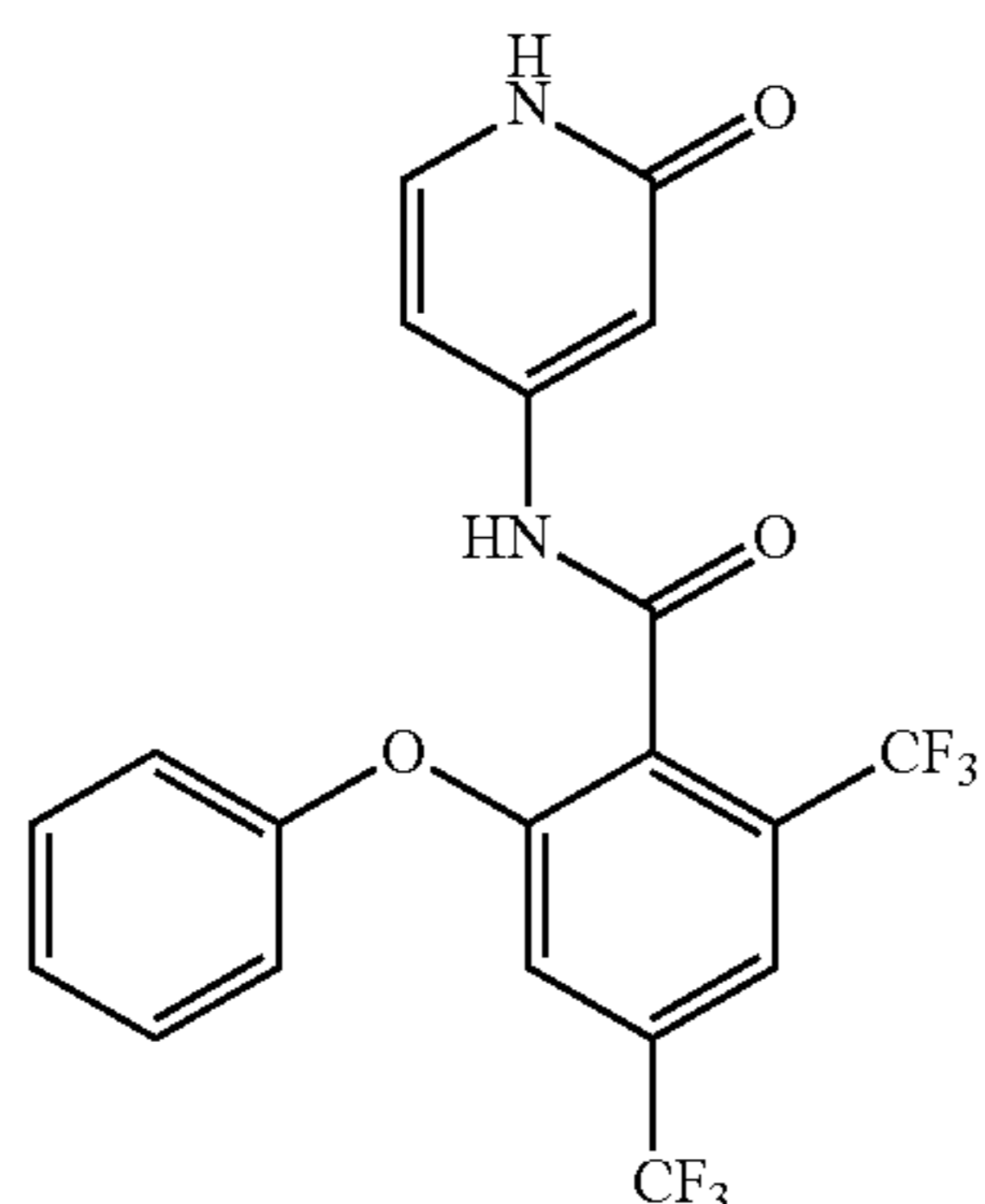
N-(2-oxo-1,2-dihydropyridin-4-yl)-2-phenoxy-4,6-bis(trifluoromethyl)benzamide
