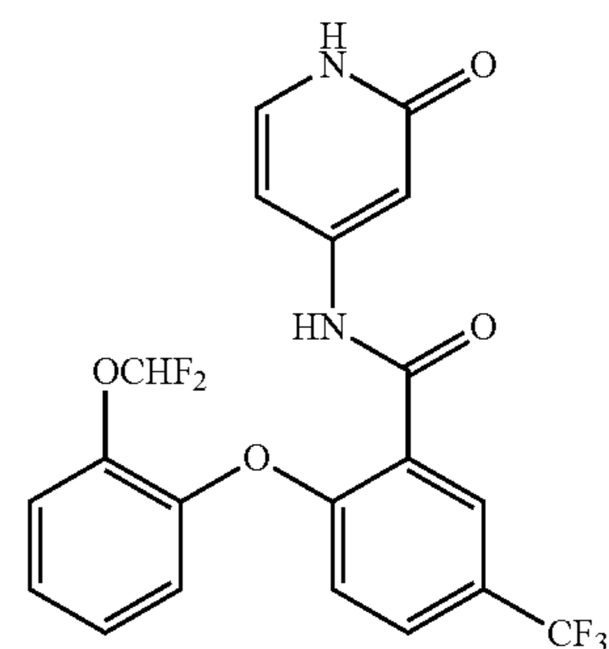
2-(2-(difluoromethoxy)phenoxy)-N-(2-oxo-1,2-dihydropyridin-4-yl)-5-(trifluoromethyl)benzamide
