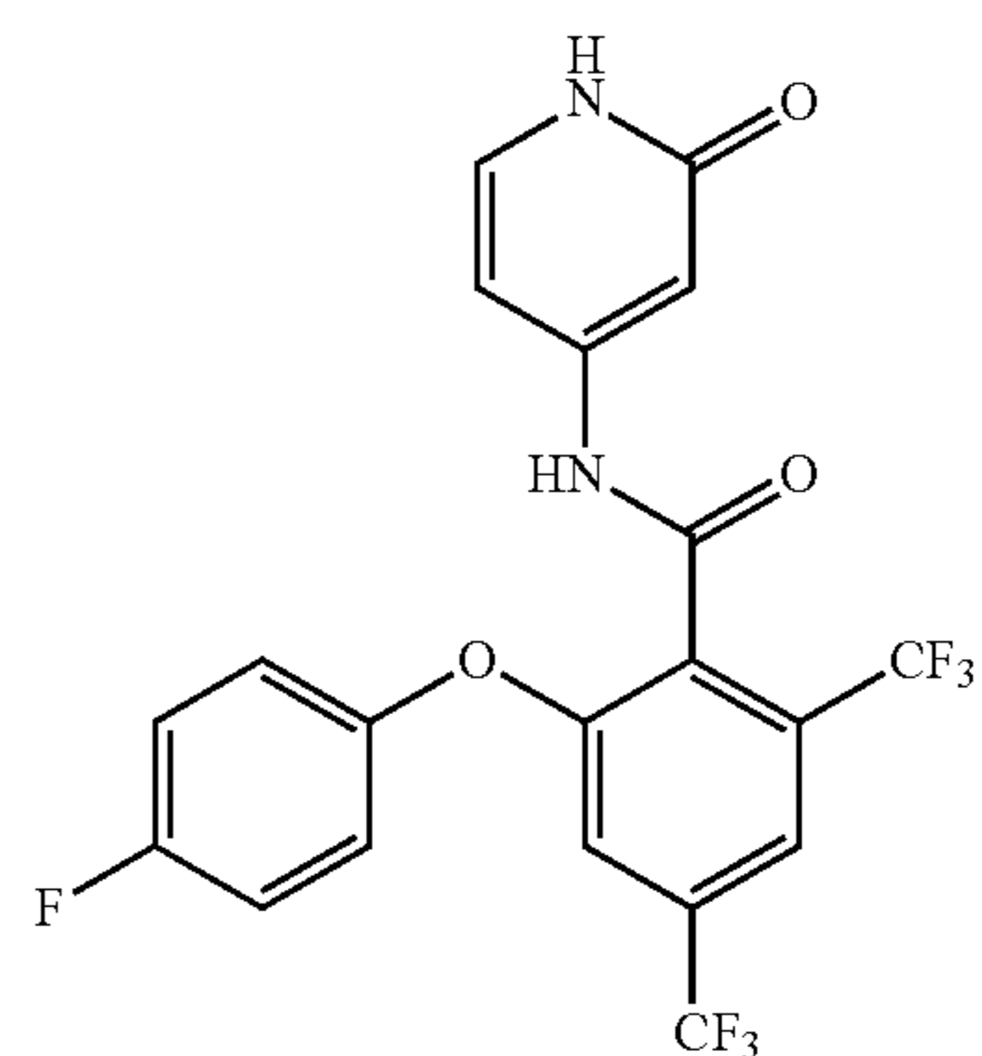
2-(4-fluorophenoxy)-N-(2-oxo-1,2-dihydropyridin-4-yl)-4,6-bis(trifluoromethyl)benzamide
