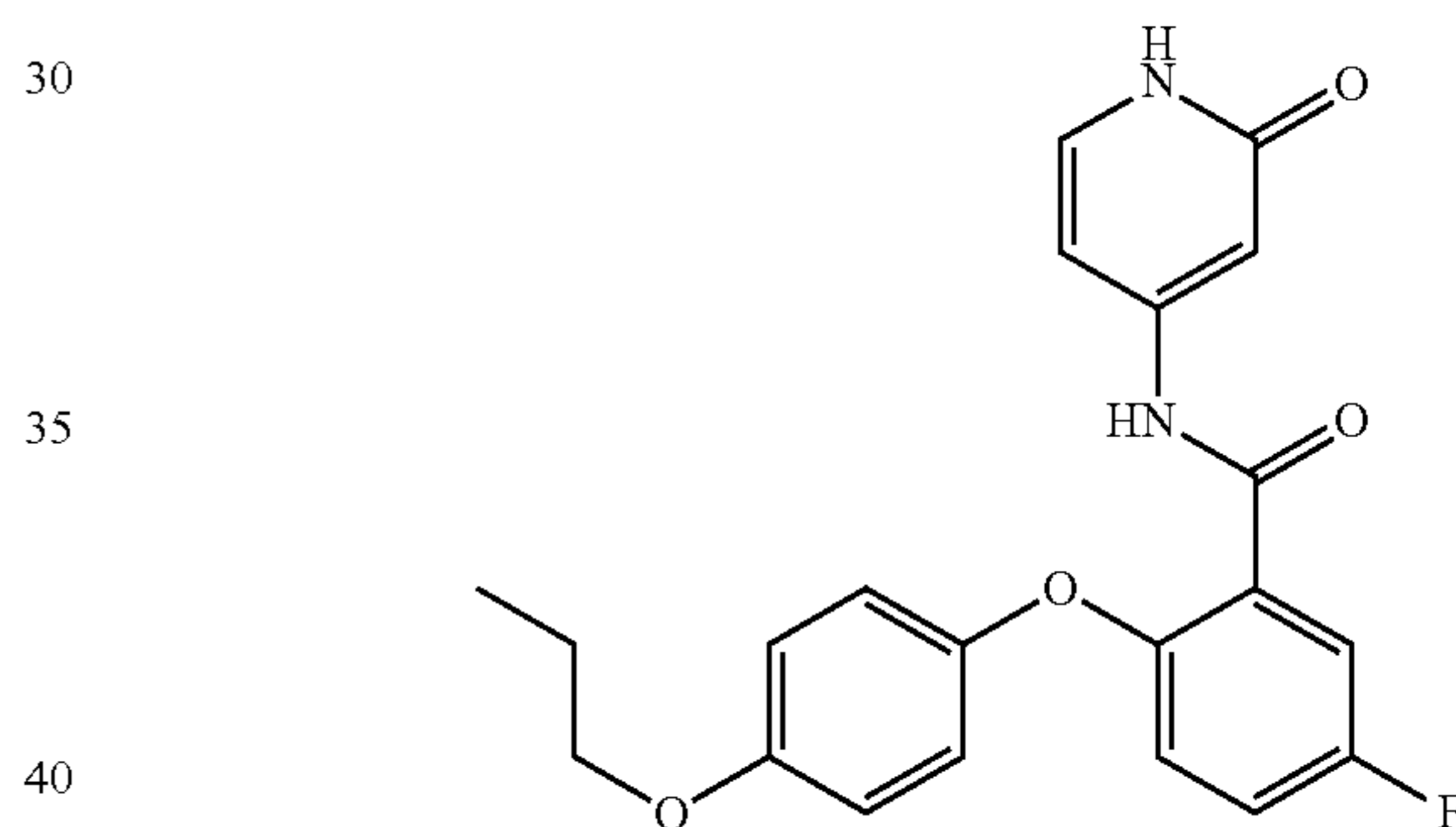
5-fluoro-N-(2-oxo-1,2-dihydropyridin-4-yl)-2-(4-propoxyphenoxy)benzamide
