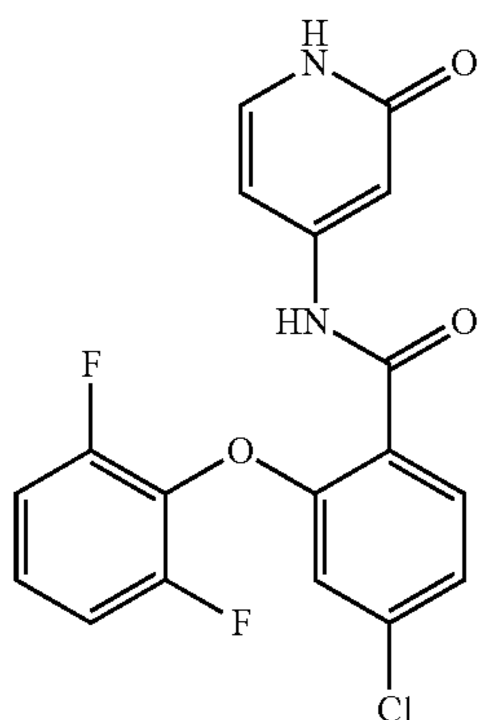
4-chloro-2-(2,6-difluorophenoxy)-N-(2-oxo-1,2-dihydropyridin-4-yl)benzamide
