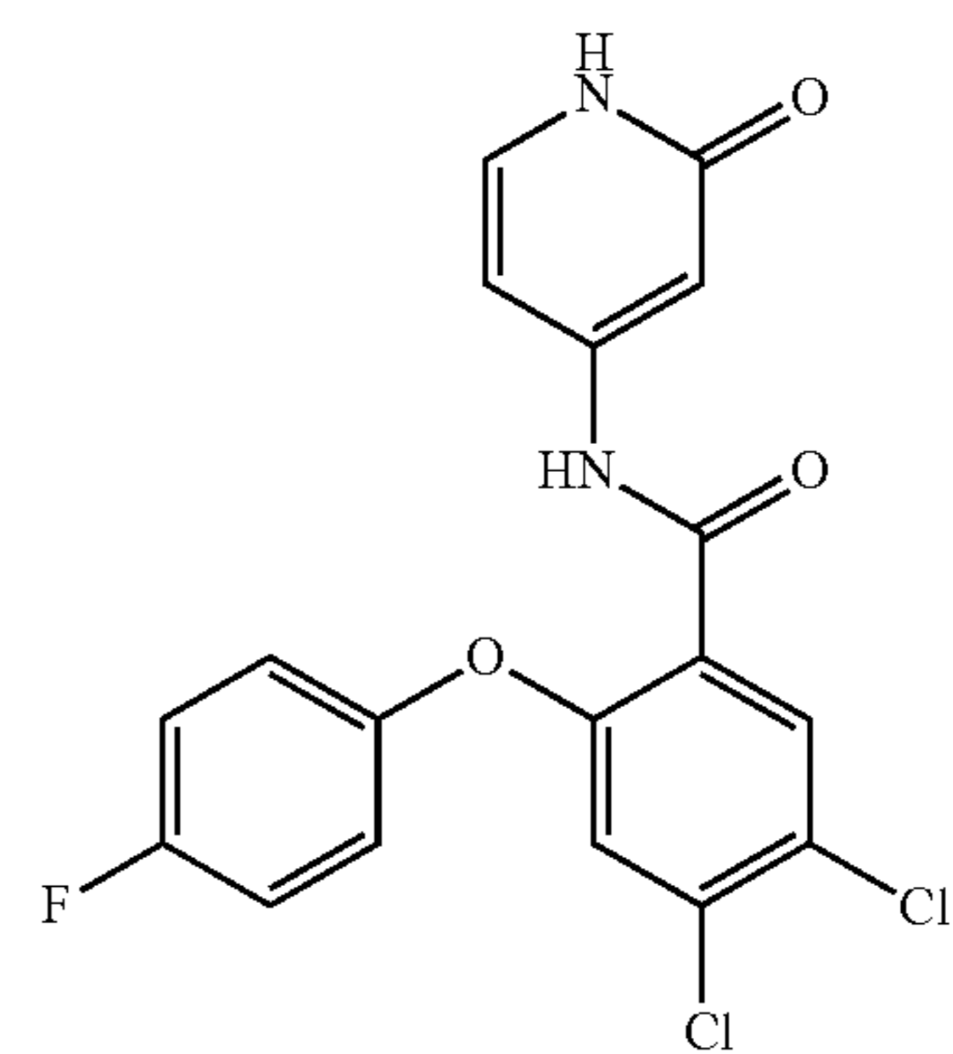
4,5-dichloro-2-(4-fluorophenoxy)-N-(2-oxo-1,2-dihydropyridin-4-yl)benzamide
