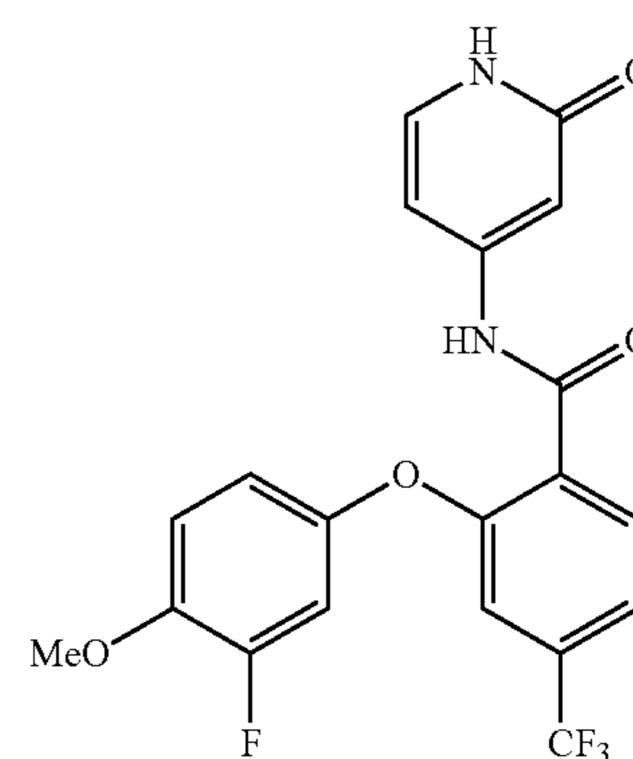
2-(3-fluoro-4-methoxyphenoxy)-N-(2-oxo-1,2-dihydropyridin-4-yl)-4-(trifluoromethyl)benzamide
