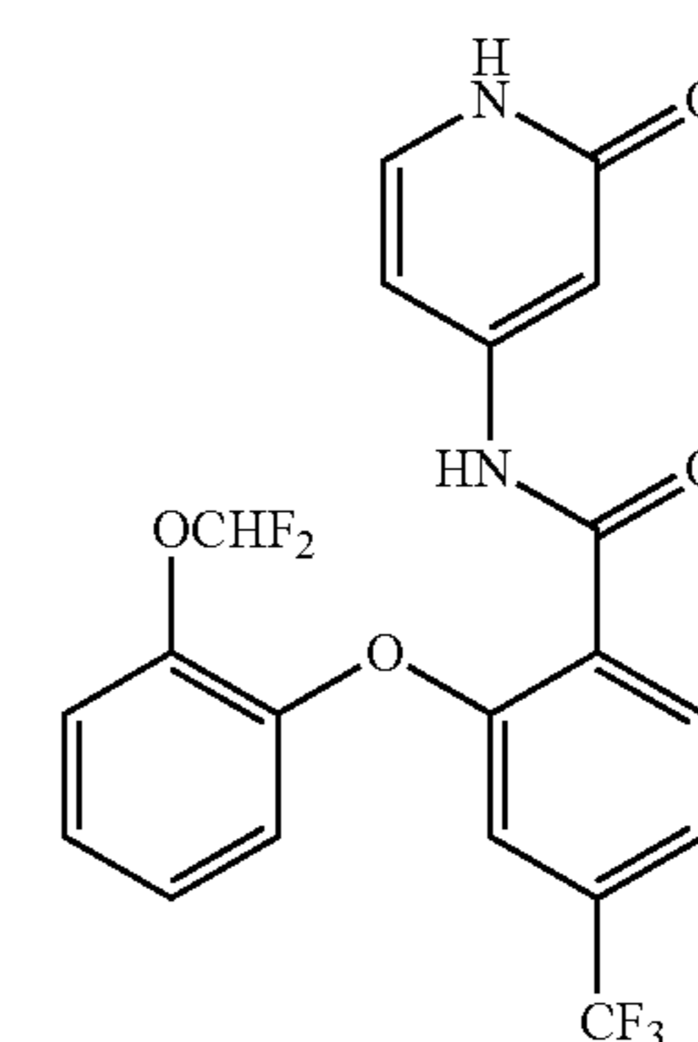
2-(2-(difluoromethoxy)phenoxy)-N-(2-oxo-1,2-dihydropyridin-4-yl)-4-(trifluoromethyl)benzamide
