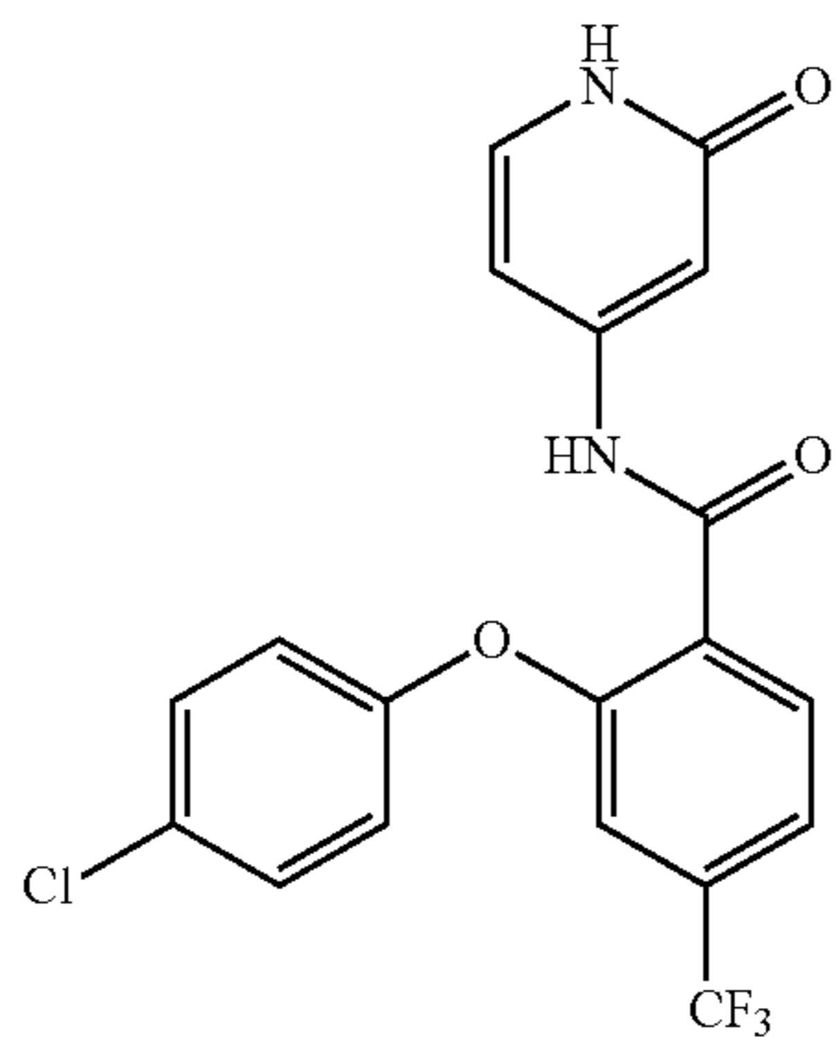
2-(4-chlorophenoxy)-N-(2-oxo-1,2-dihydropyridin-4-yl)-4-(trifluoromethyl)benzamide
