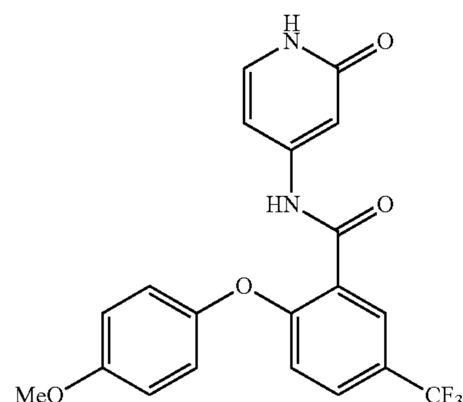
2-(4-methoxyphenoxy)-N-(2-oxo-1,2-dihydropyridin-4-yl)-5-(trifluoromethyl)benzamide
