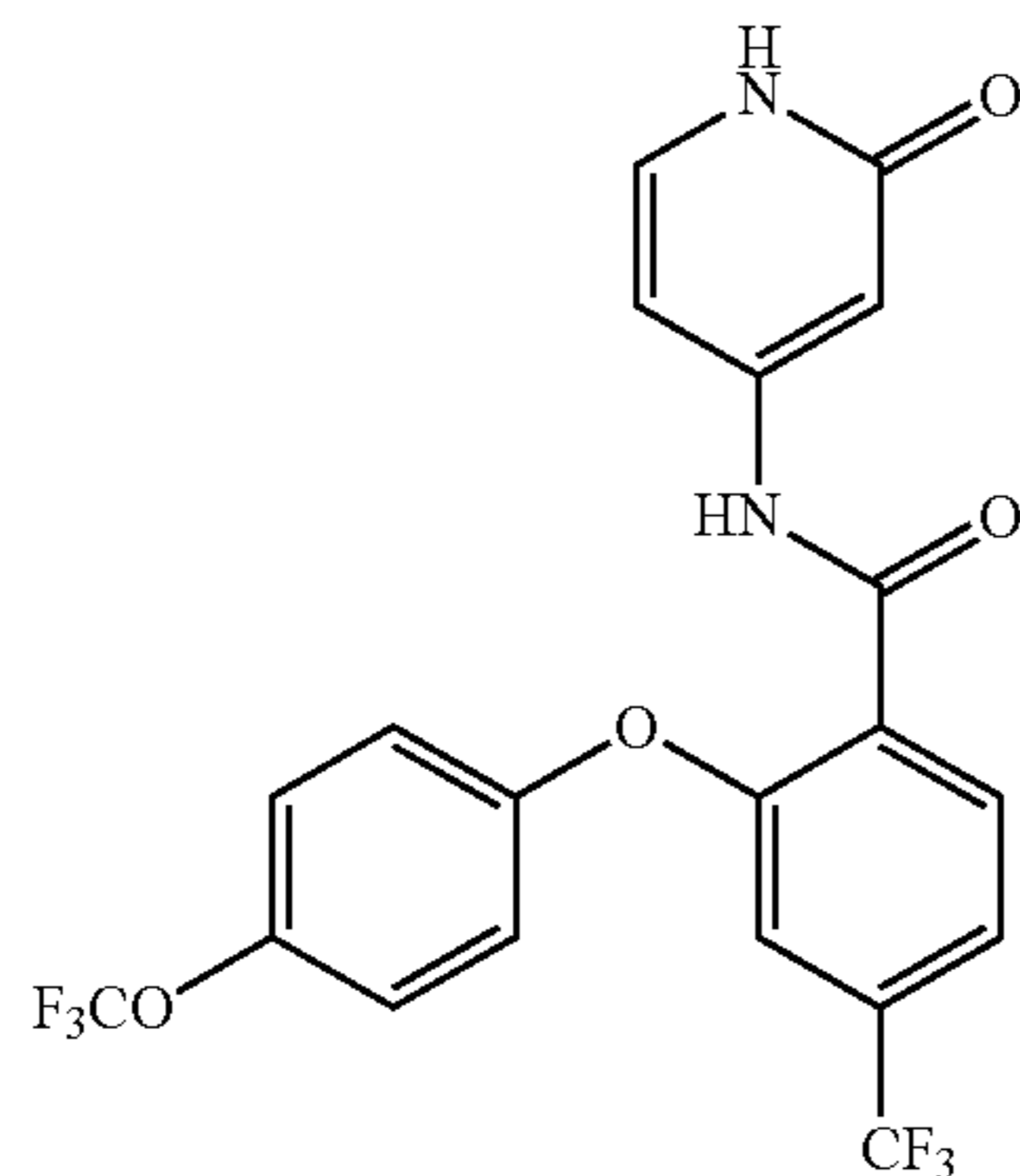
N-(2-oxo-1,2-dihydropyridin-4-yl)-2-(4-(trifluoromethoxy)phenoxy)-4-(trifluoromethyl)benzamide
