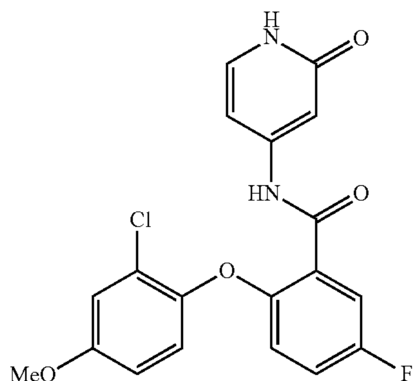
2-(2-chloro-4-methoxyphenoxy)-5-fluoro-N-(2-oxo-1,2-dihydropyridin-4-yl)benzamide
