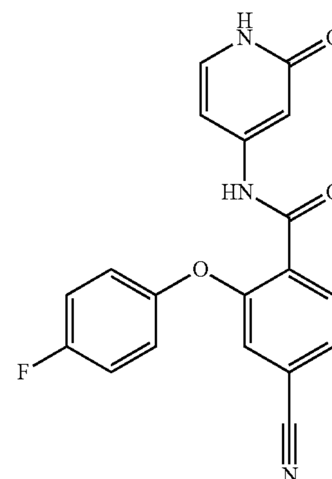
4-cyano-2-(4-fluorophenoxy)-N-(2-oxo-1,2-dihydropyridin-4-yl)benzamide
