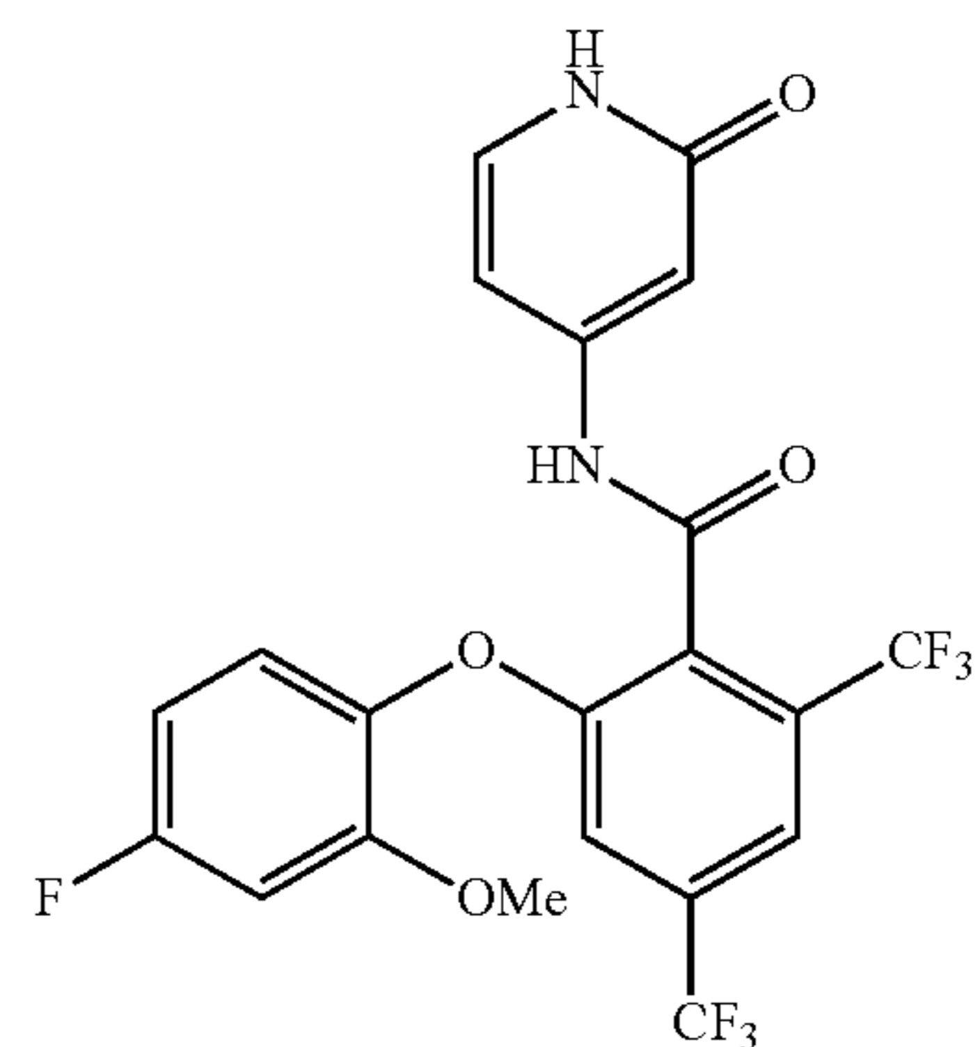
2-(4-fluoro-2-methoxyphenoxy)-N-(2-oxo-1,2-dihydropyridin-4-yl)-4,6-bis(trifluoromethyl)benzamide
