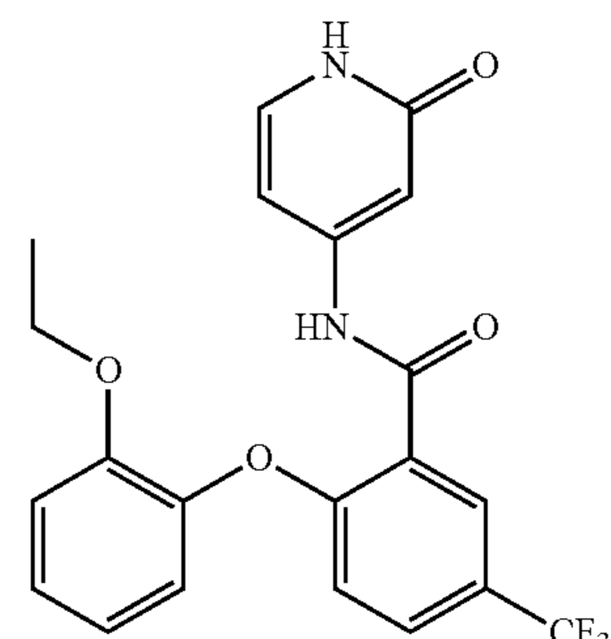
2-(2-ethoxyphenoxy)-N-(2-oxo-1,2-dihydropyridin-4-yl)-5-(trifluoromethyl)benzamide
