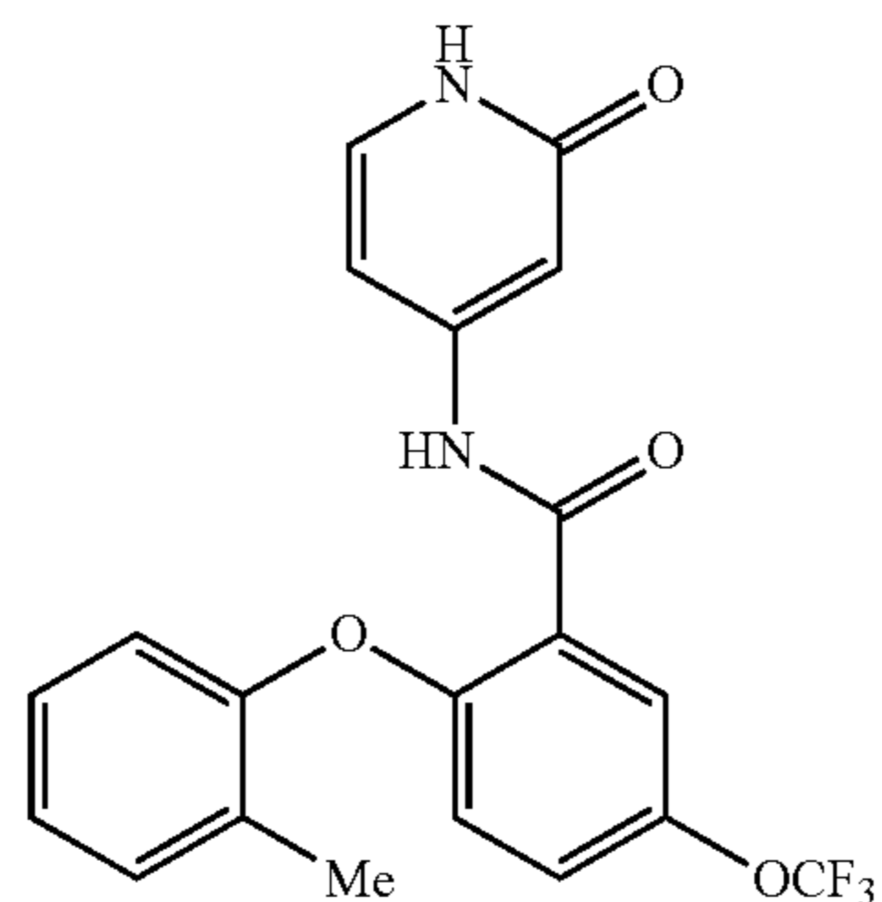
N-(2-oxo-1,2-dihydropyridin-4-yl)-2-(o-tolyloxy)-5-(trifluoromethoxy)benzamide
