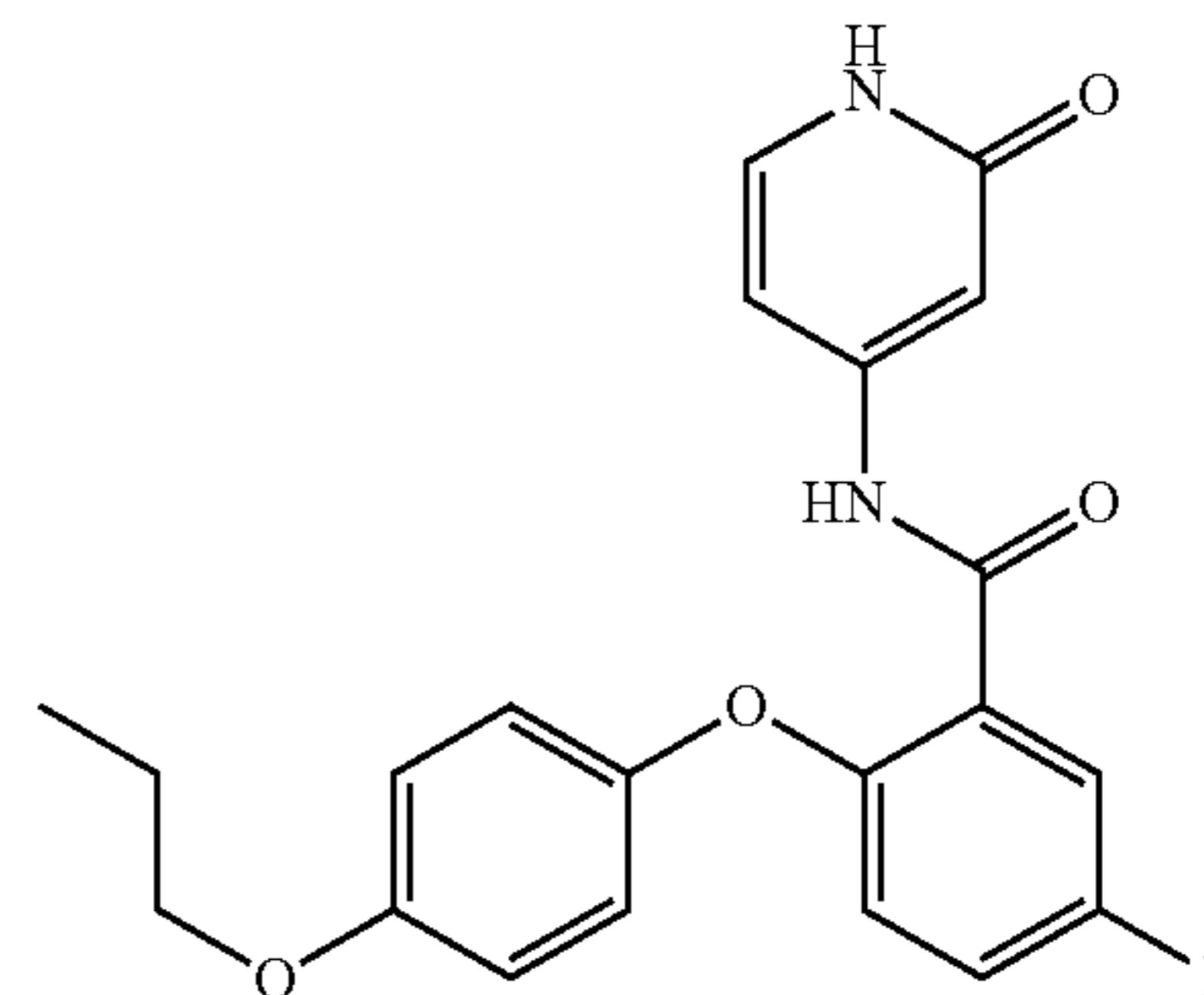
5-fluoro-N-(2-oxo-1,2-dihydropyridin-4-yl)-2-(4-propoxyphenoxy)benzamide
