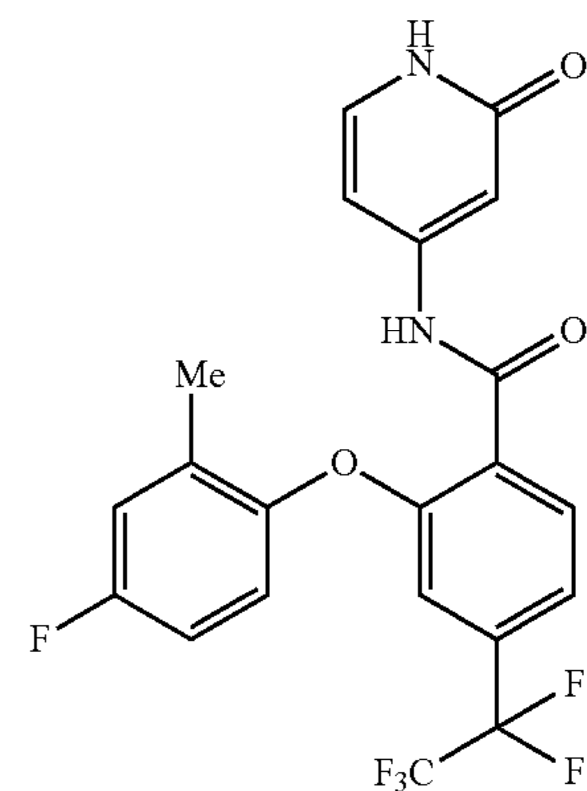
2-(4-fluoro-2-methylphenoxy)-N-(2-oxo-1,2-dihydropyridin-4-yl)-4-(perfluoroethyl)benzamide
