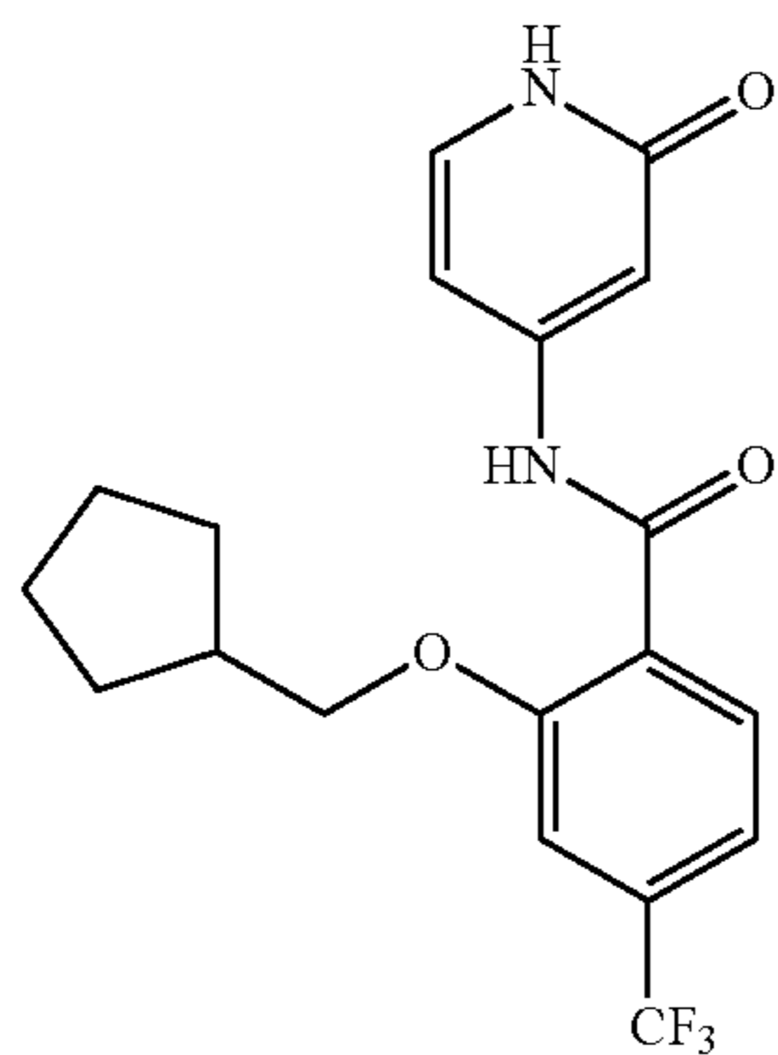
2-(cyclopentylmethoxy)-N-(2-oxo-1,2-dihydropyridin-4-yl)-4-(trifluoromethyl)benzamide
