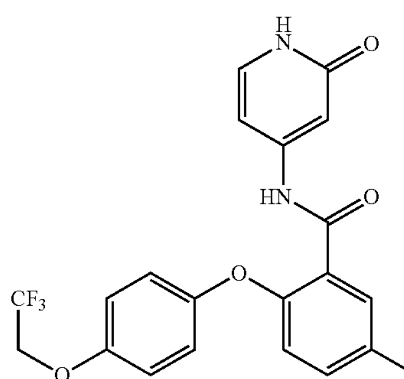
5-fluoro-N-(2-oxo-1,2-dihydropyridin-4-yl)-2-(4-(2,2,2-trifluoroethoxy)phenoxy)benzamide
