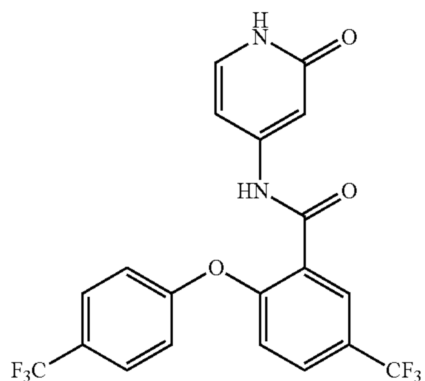
N-(2-oxo-1,2-dihydropyridin-4-yl)-5-(trifluoromethyl)-2-(4-(trifluoromethyl)phenoxy)benzamide
