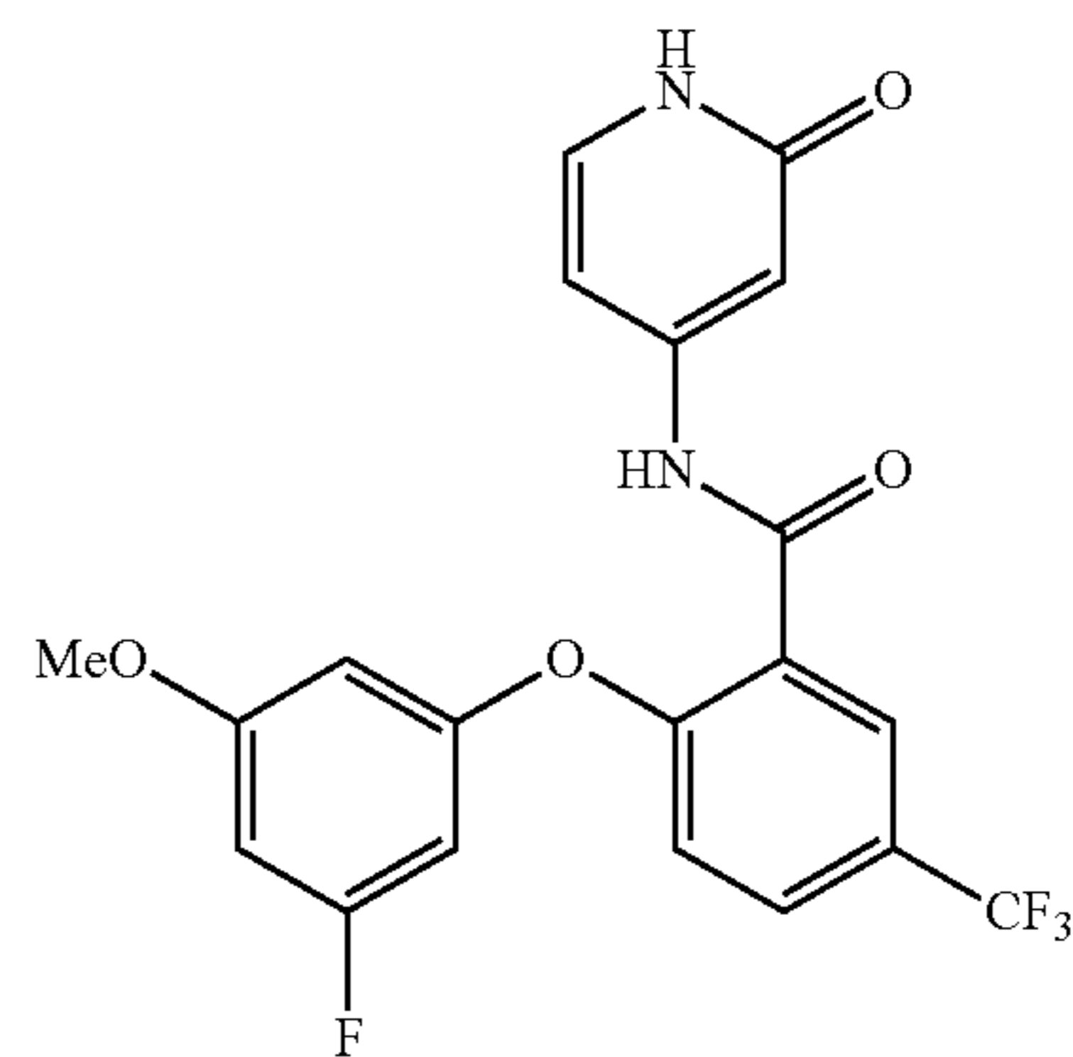
2-(3-fluoro-5-methoxyphenoxy)-N-(2-oxo-1,2-dihydropyridin-4-yl)-5-(trifluoromethyl)benzamide
