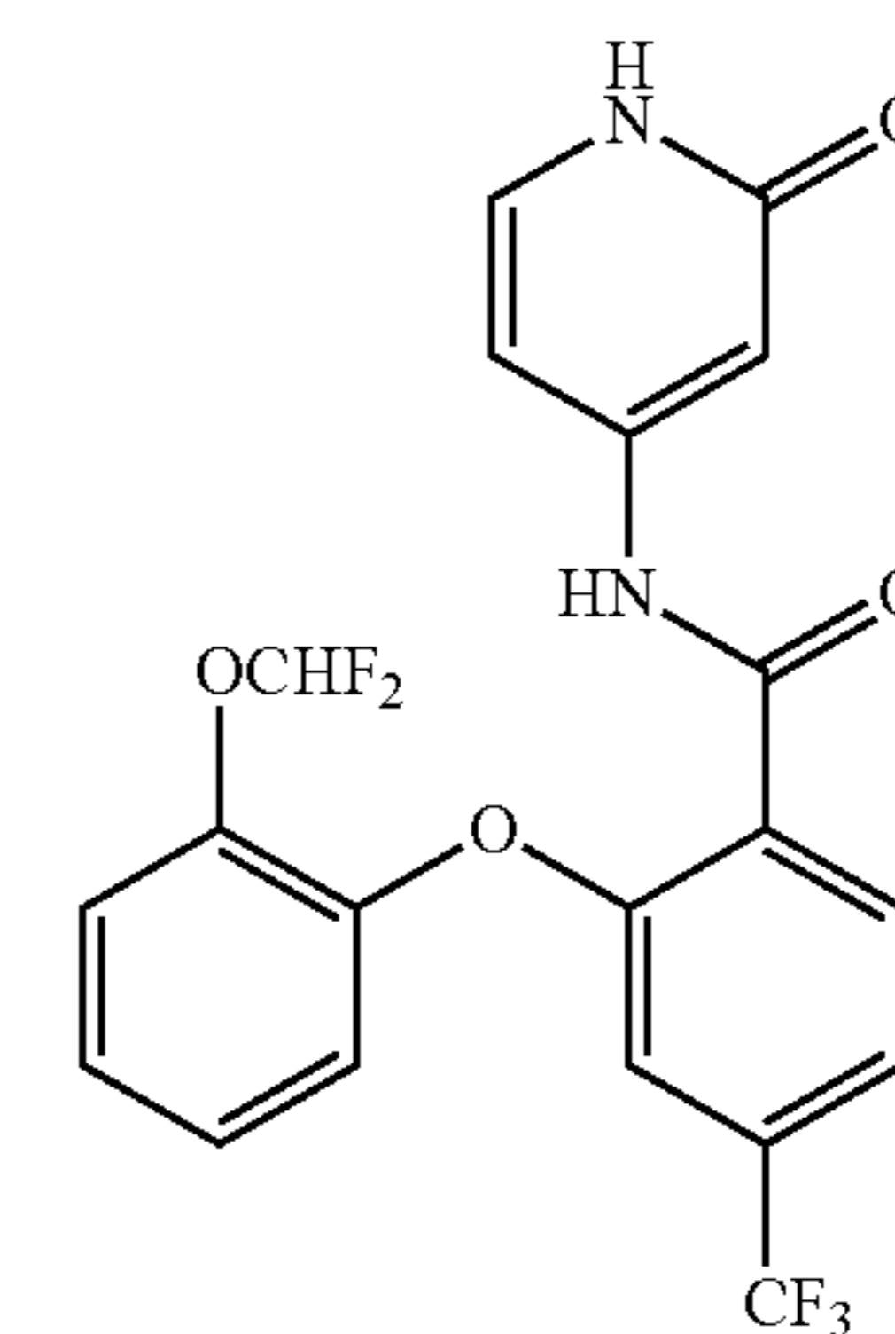
2-(2-(difluoromethoxy)phenoxy)-N-(2-oxo-1,2-dihydropyridin-4-yl)-4-(trifluoromethyl)benzamide
