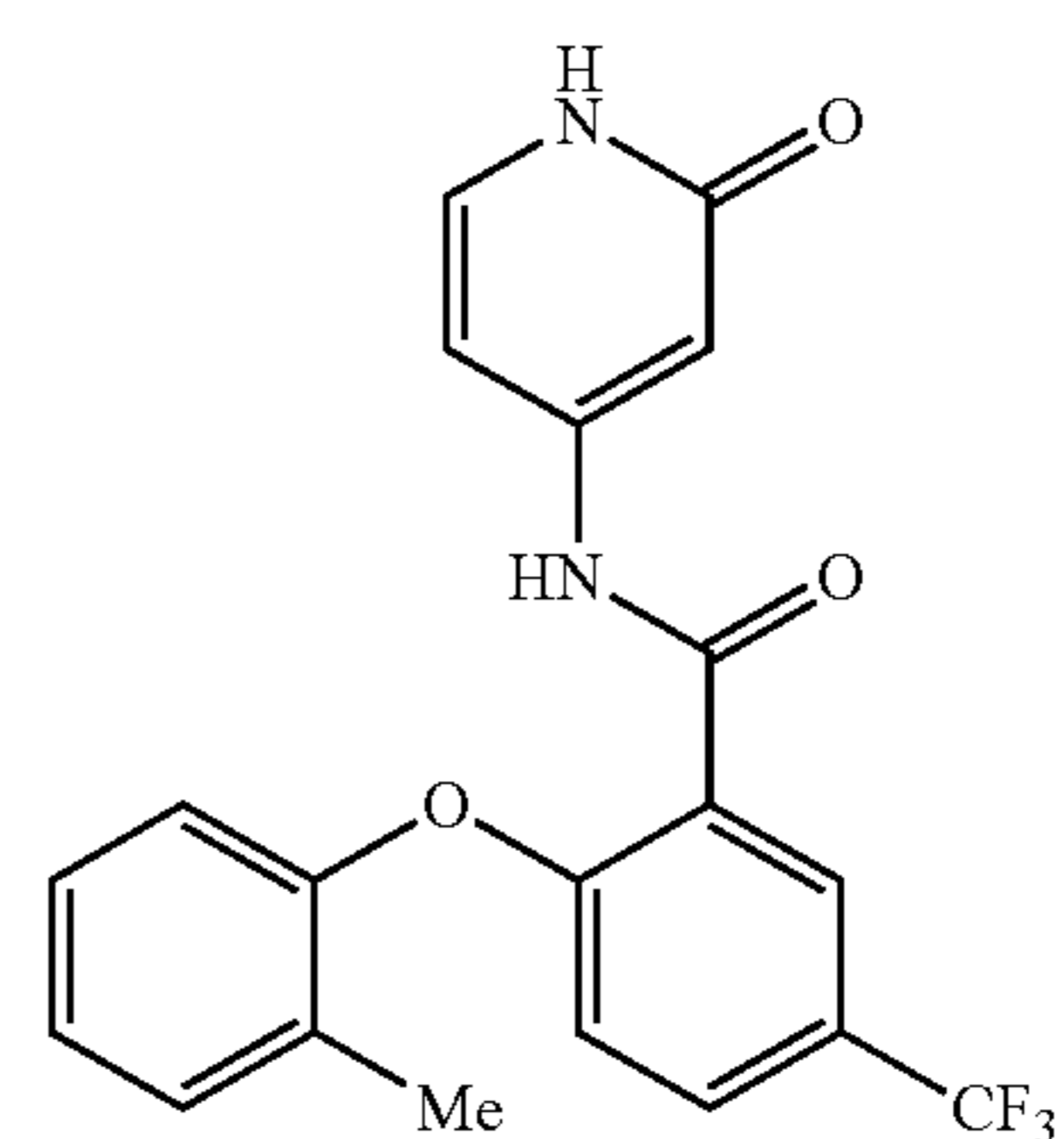
N-(2-oxo-1,2-dihydropyridin-4-yl)-2-(o-tolyloxy)-5-(trifluoromethyl)benzamide
