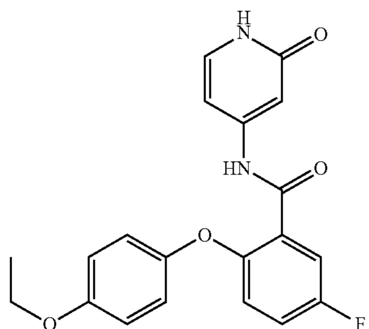
2-(4-ethoxyphenoxy)-5-fluoro-N-(2-oxo-1,2-dihydropyridin-4-yl)benzamide
