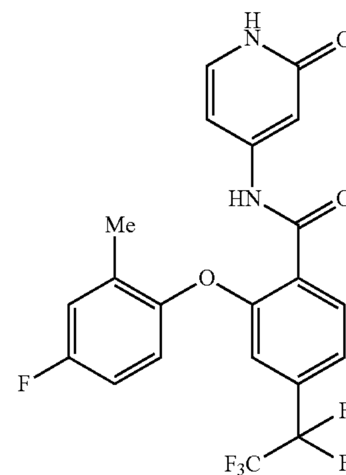
2-(4-fluoro-2-methylphenoxy)-N-(2-oxo-1,2-dihydropyridin-4-yl)-4-(perfluoroethyl)benzamide
