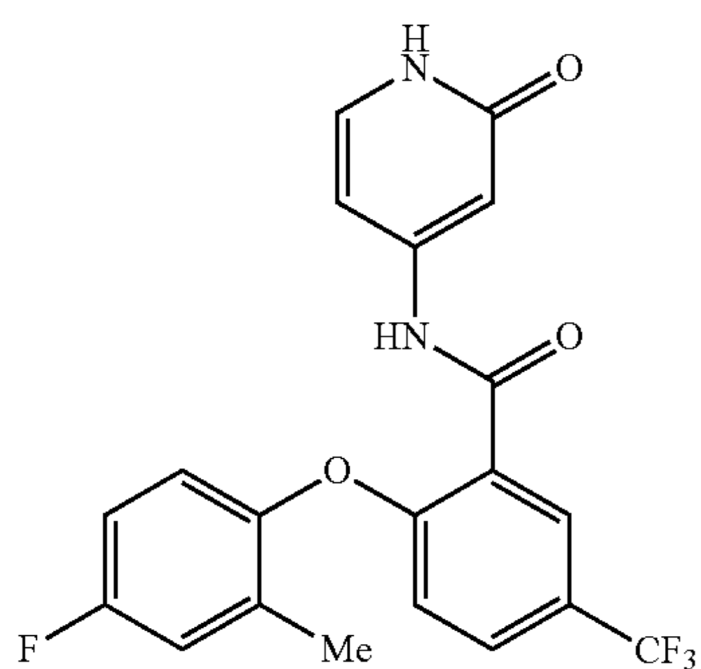
2-(4-fluoro-2-methylphenoxy)-N-(2-oxo-1,2-dihydropyridin-4-yl)-5-(trifluoromethyl)benzamide
