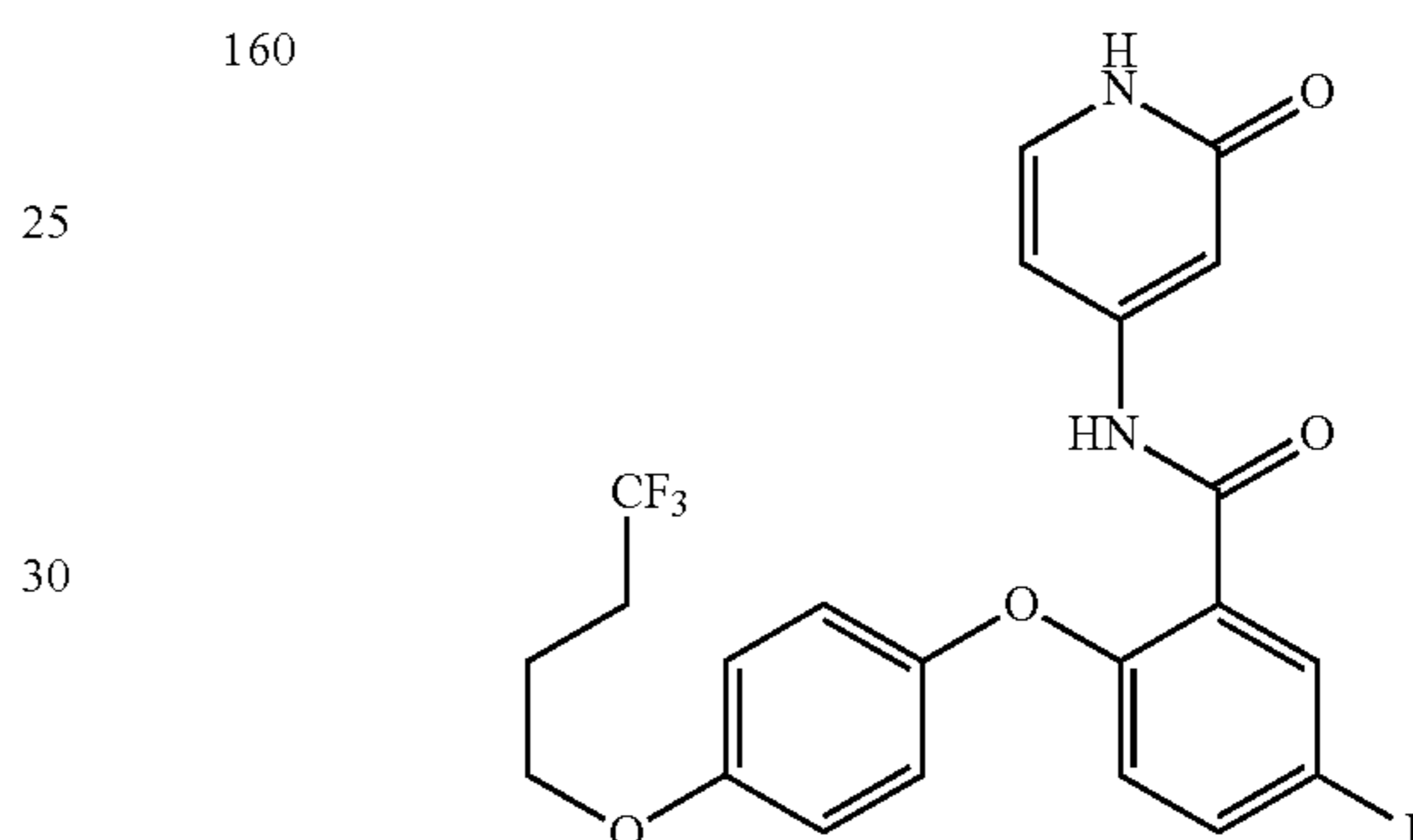
5-fluoro-N-(2-oxo-1,2-dihydropyridin-4-yl)-2-(4-(4,4,4-trifluorobutoxy)phenoxy)benzamide
