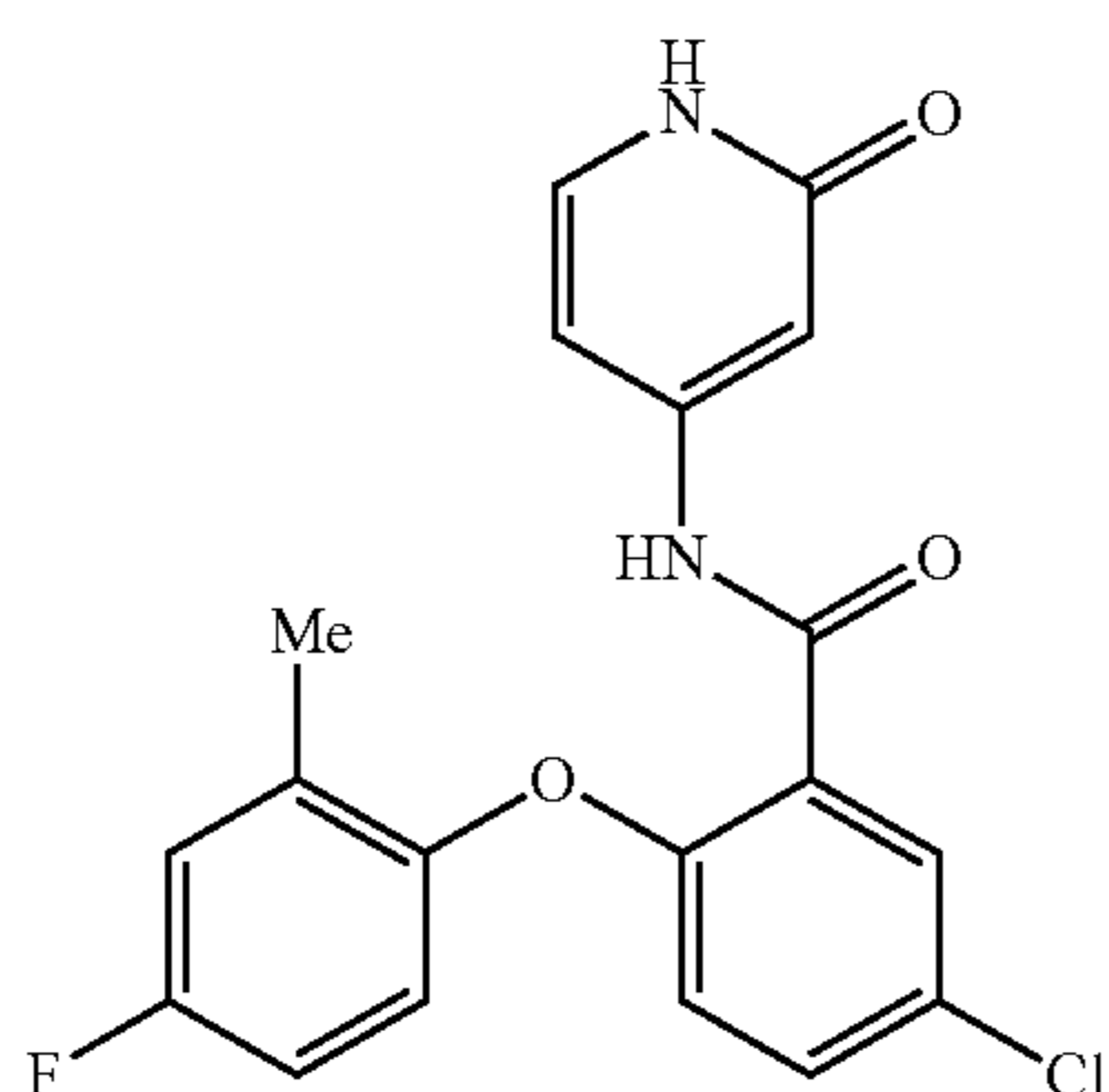
5-chloro-2-(4-fluoro-2-methylphenoxy)-N-(2-oxo-1,2-dihydropyridin-4-yl)benzamide
