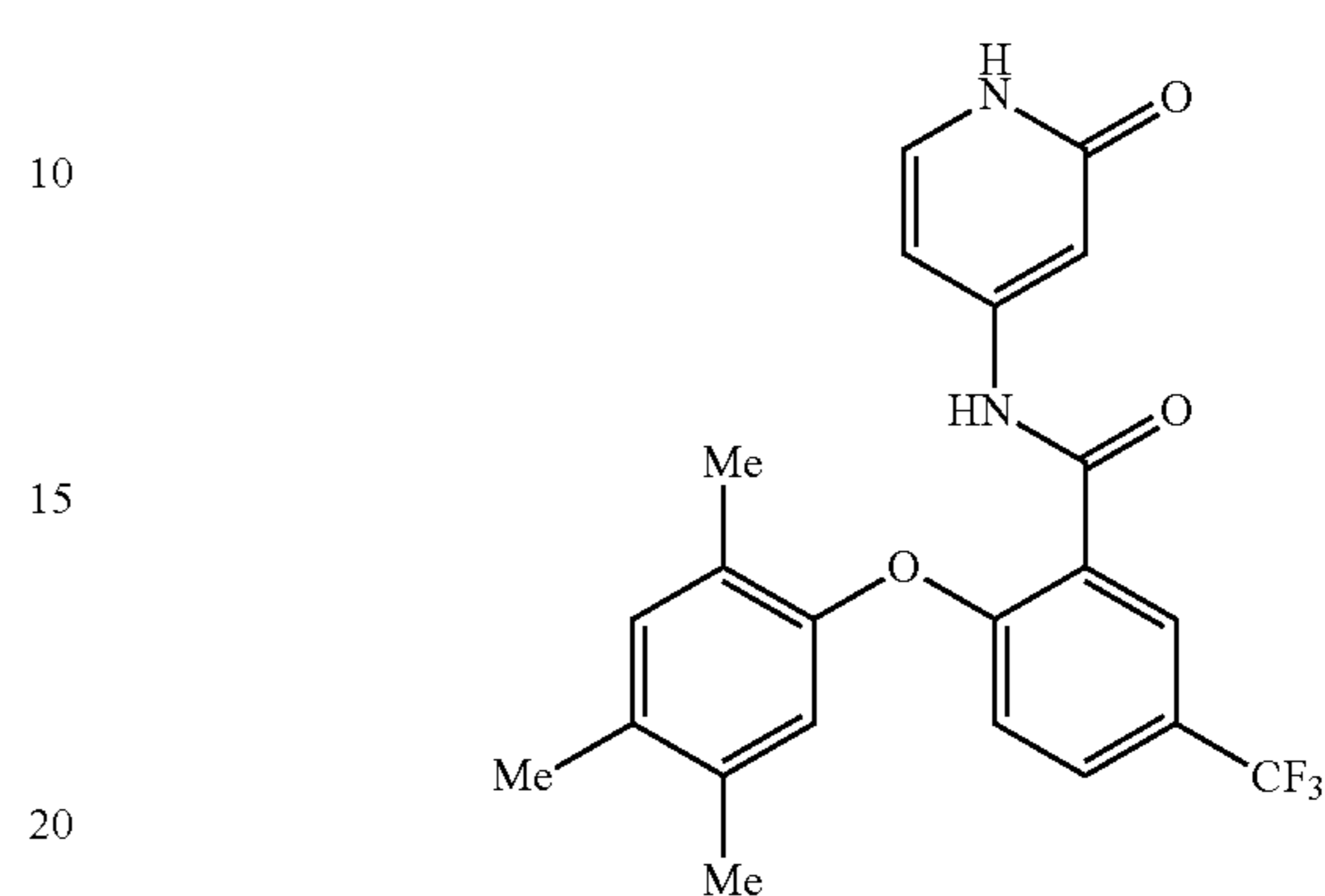
N-(2-oxo-1,2-dihydropyridin-4-yl)-5-(trifluoromethyl)-2-(2,4,5-trimethylphenoxy)benzamide
