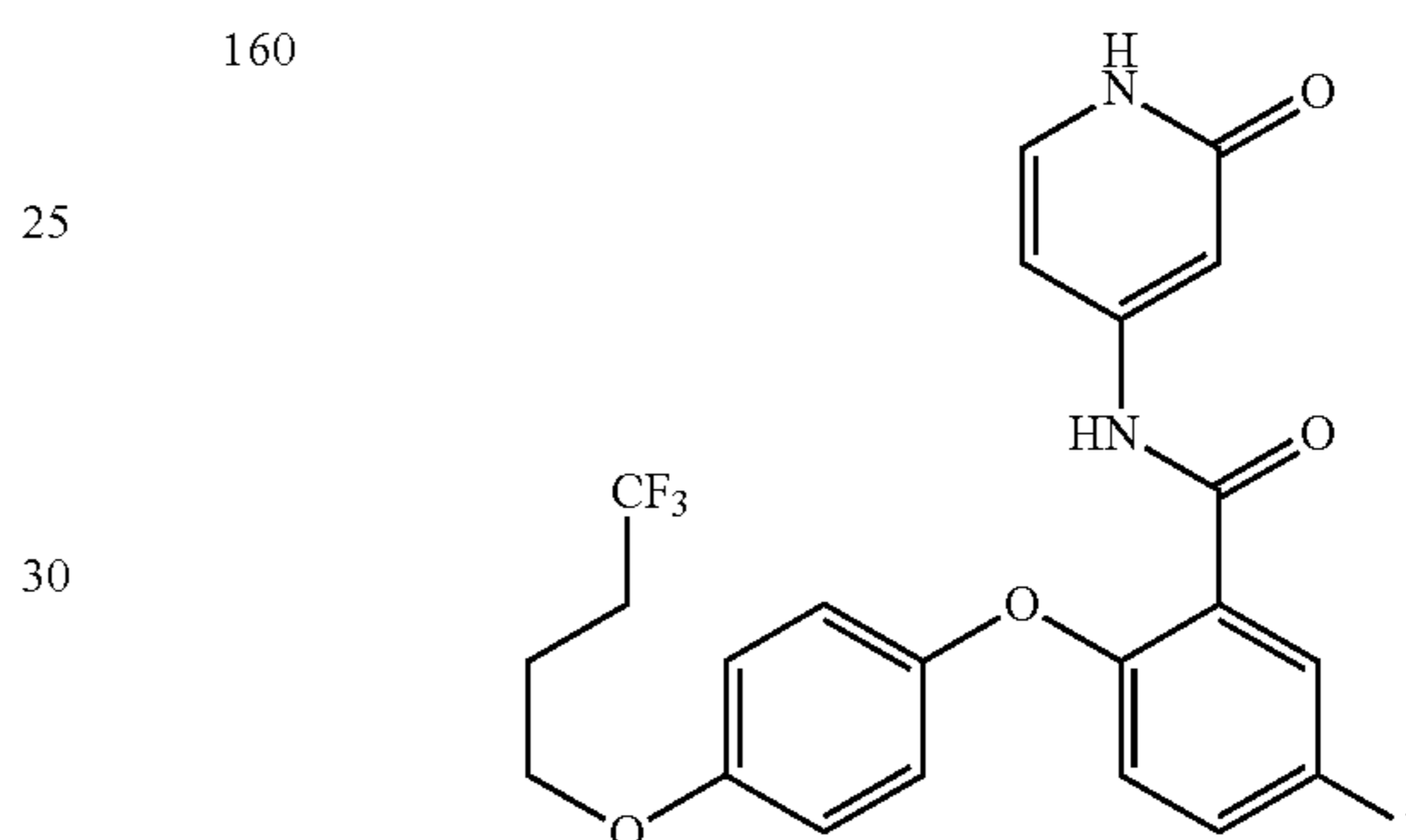
5-fluoro-N-(2-oxo-1,2-dihydropyridin-4-yl)-2-(4-(4,4,4-trifluorobutoxy)phenoxy)benzamide
