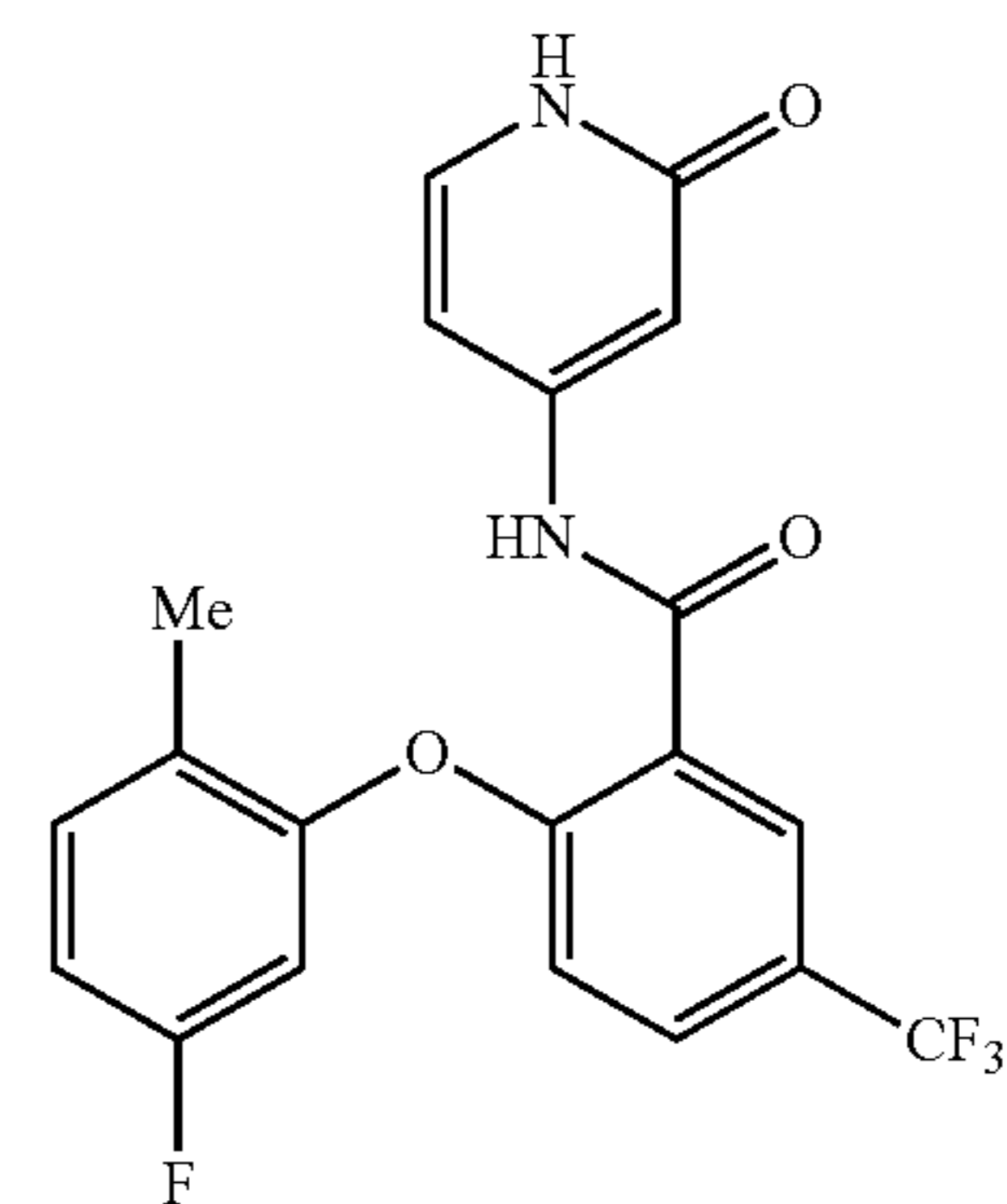
2-(5-fluoro-2-methylphenoxy)-N-(2-oxo-1,2-dihydropyridin-4-yl)-5-(trifluoromethyl)benzamide
