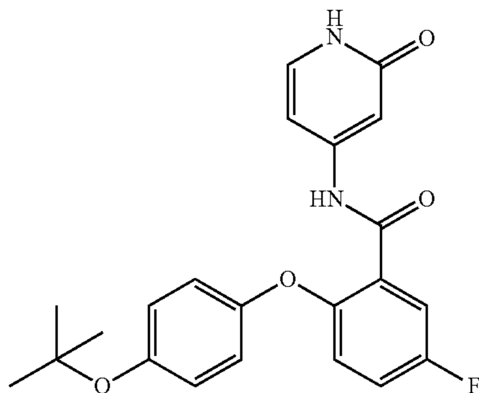
2-(4-(tert-butoxy)phenoxy)-5-fluoro-N-(2-oxo-1,2-dihydropyridin-4-yl)benzamide
