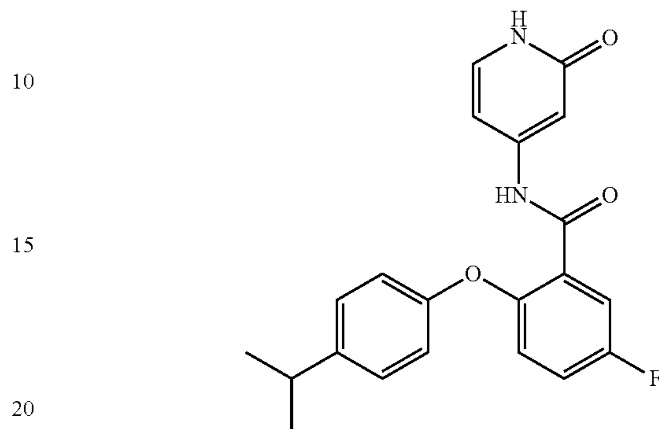
5-fluoro-2-(4-isopropylphenoxy)-N-(2-oxo-1,2-dihydropyridin-4-yl)benzamide
