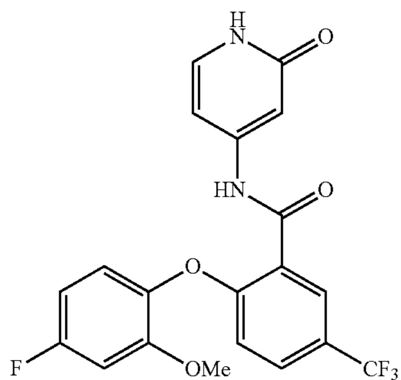
2-(4-fluoro-2-methoxyphenoxy)-N-(2-oxo-1,2-dihydropyridin-4-yl)-5-(trifluoromethyl)benzamide
