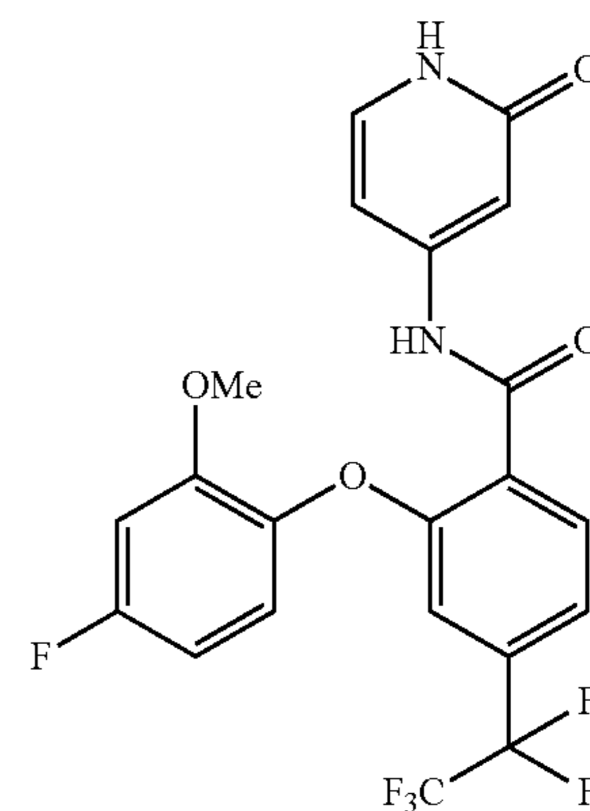
2-(4-fluoro-2-methoxyphenoxy)-N-(2-oxo-1,2-dihydropyridin-4-yl)-4-(perfluoroethyl)benzamide
