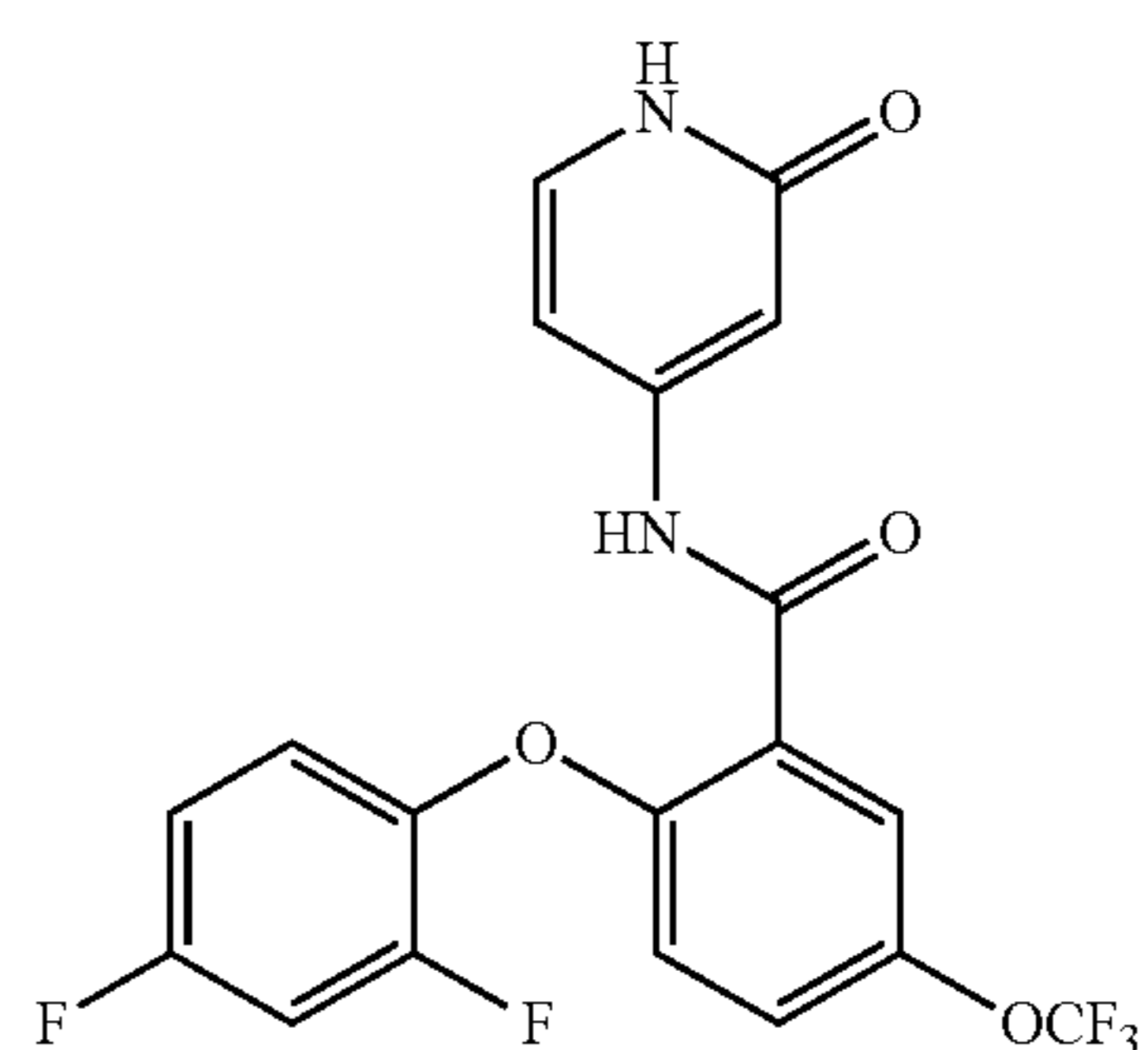
2-(2,4-difluorophenoxy)-N-(2-oxo-1,2-dihydropyridin-4-yl)-5-(trifluoromethoxy)benzamide
