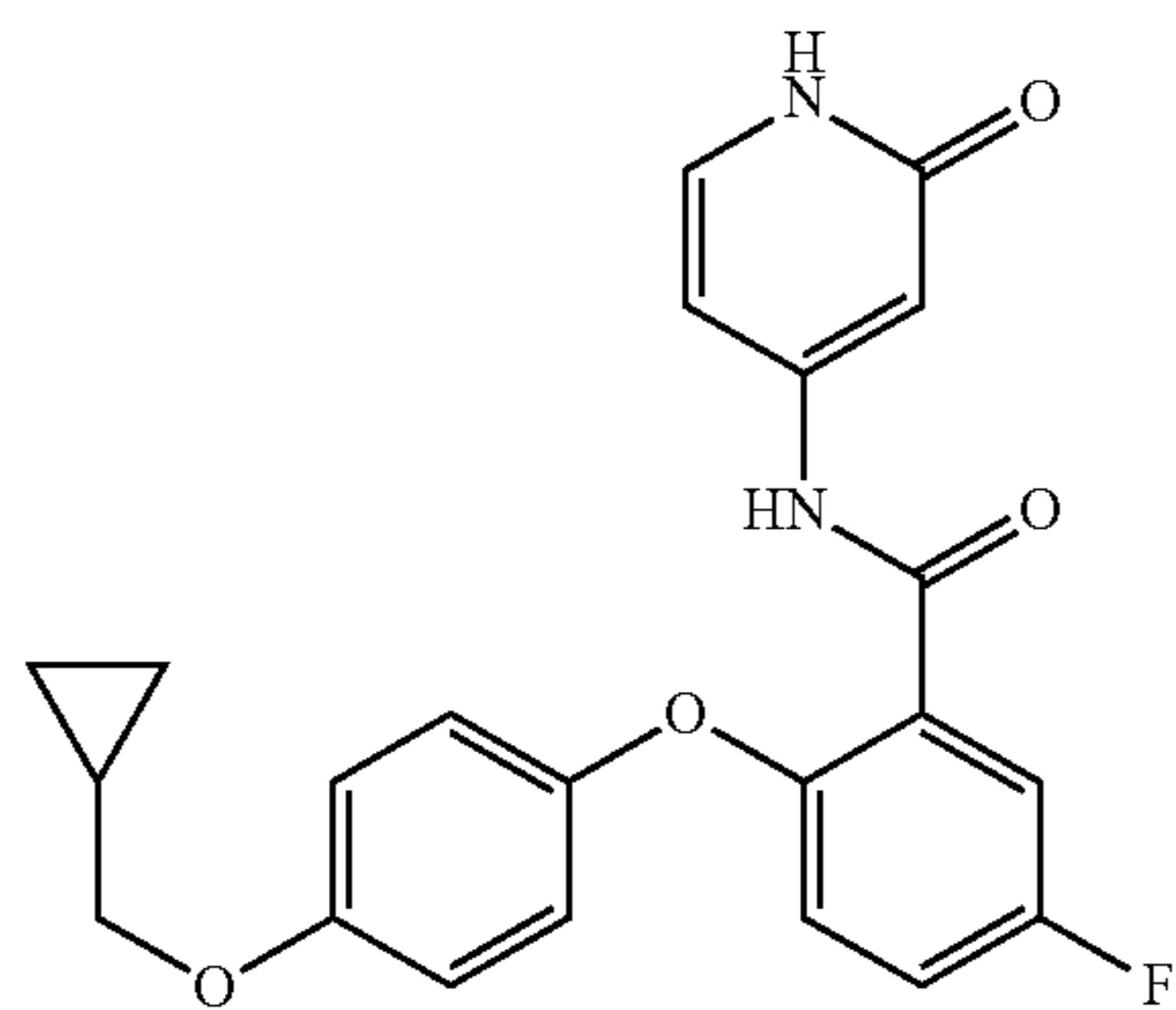
2-(4-(cyclopropylmethoxy)phenoxy)-5-fluoro-N-(2-oxo-1,2-dihydropyridin-4-yl)benzamide
