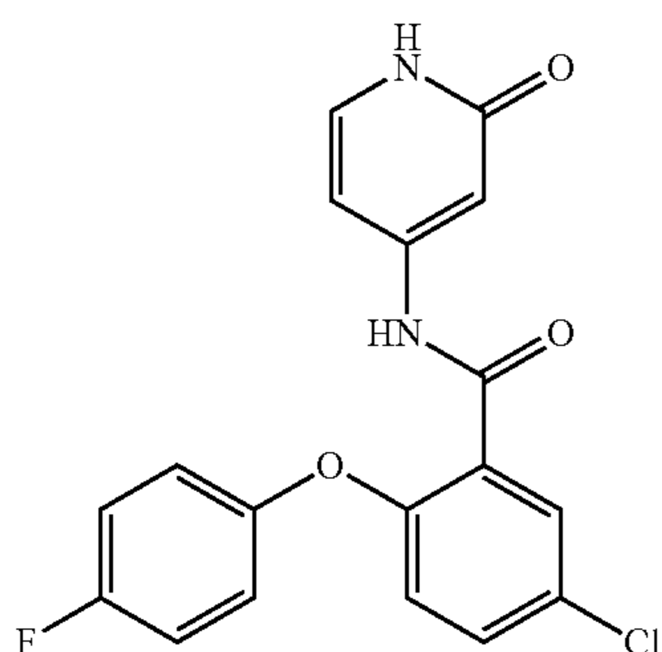
5-chloro-2-(4-fluorophenoxy)-N-(2-oxo-1,2-dihydropyridin-4-yl)benzamide
