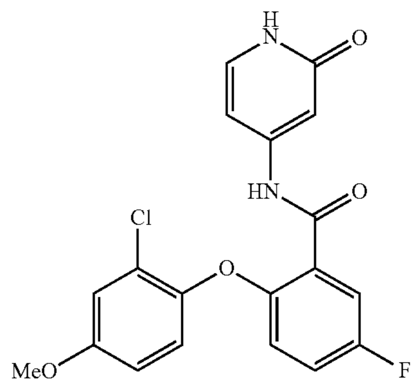
2-(2-chloro-4-methoxyphenoxy)-5-fluoro-N-(2-oxo-1,2-dihydropyridin-4-yl)benzamide
