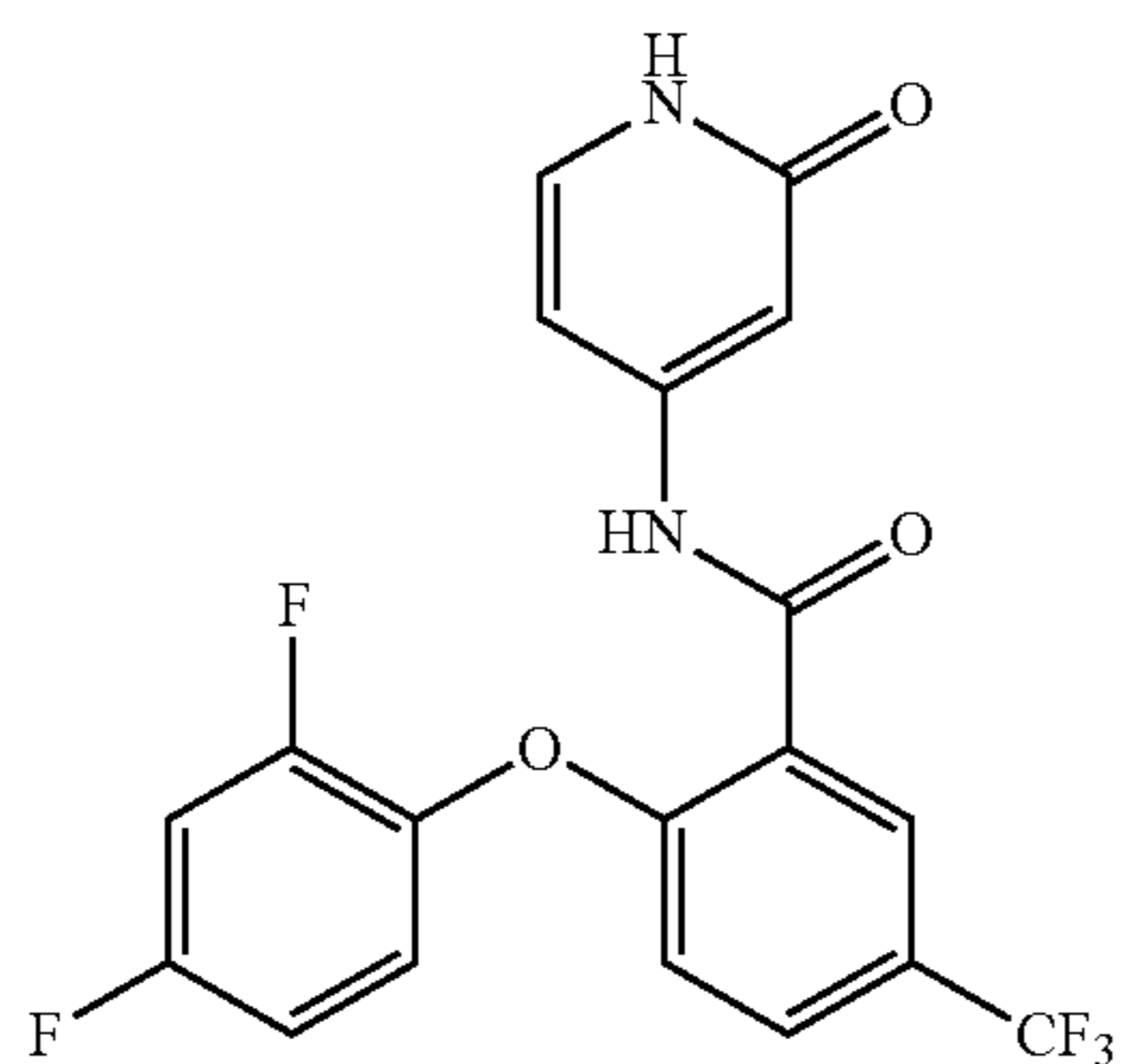
2-(2,4-difluorophenoxy)-N-(2-oxo-1,2-dihydropyridin-4-yl)-5-(trifluoromethyl)benzamide
