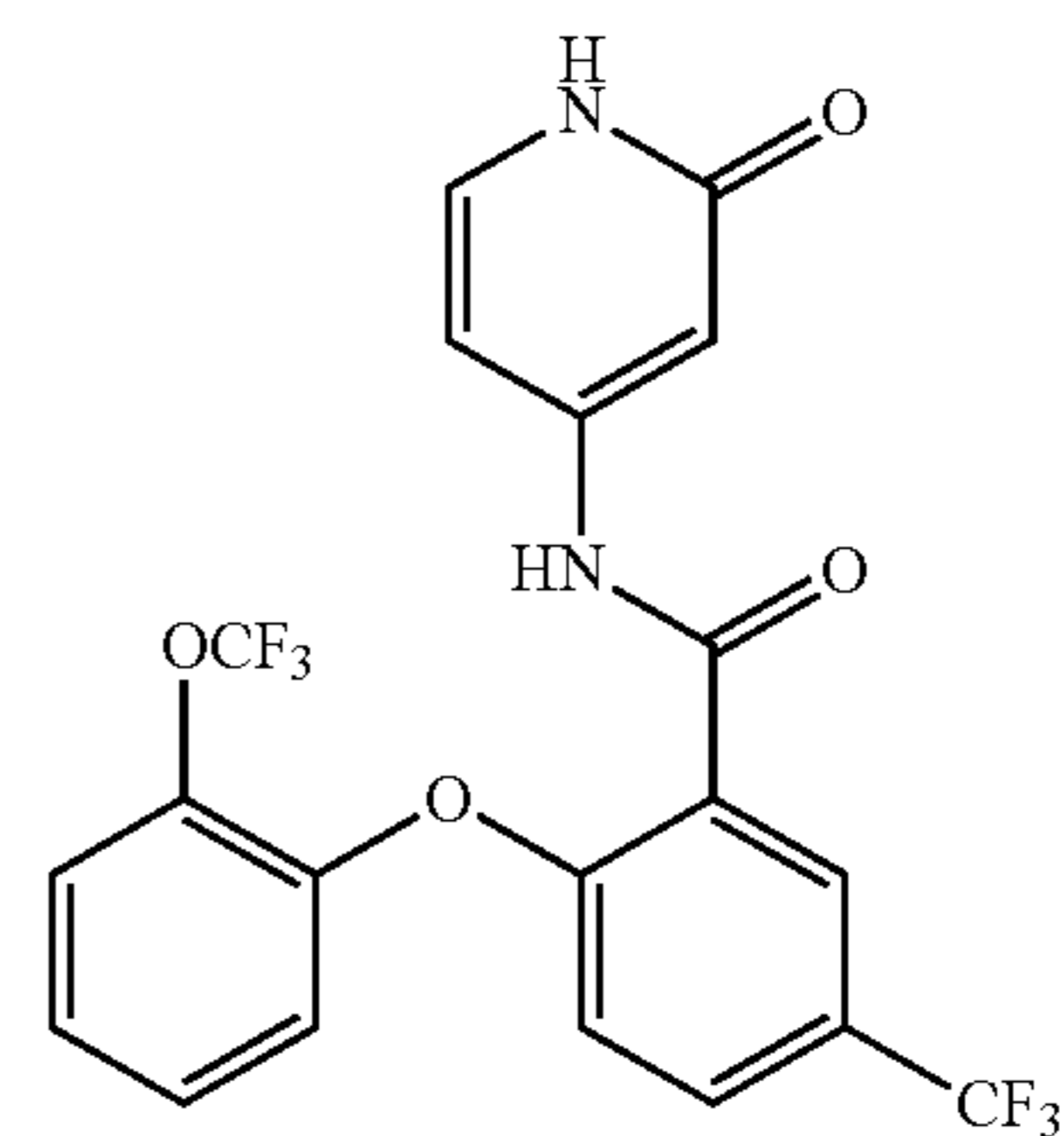
N-(2-oxo-1,2-dihydropyridin-4-yl)-2-(2-(trifluoromethoxy)phenoxy)-5-(trifluoromethyl)benzamide
