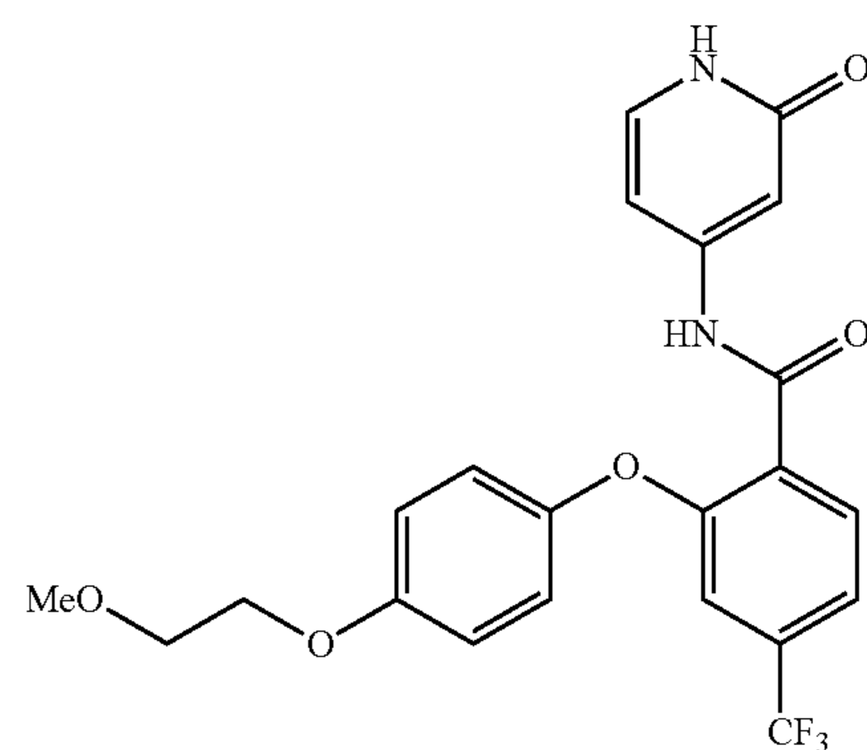
2-(4-(2-methoxyethoxy)phenoxy)-N-(2-oxo-1,2-dihydropyridin-4-yl)-4-(trifluoromethyl)benzamide
