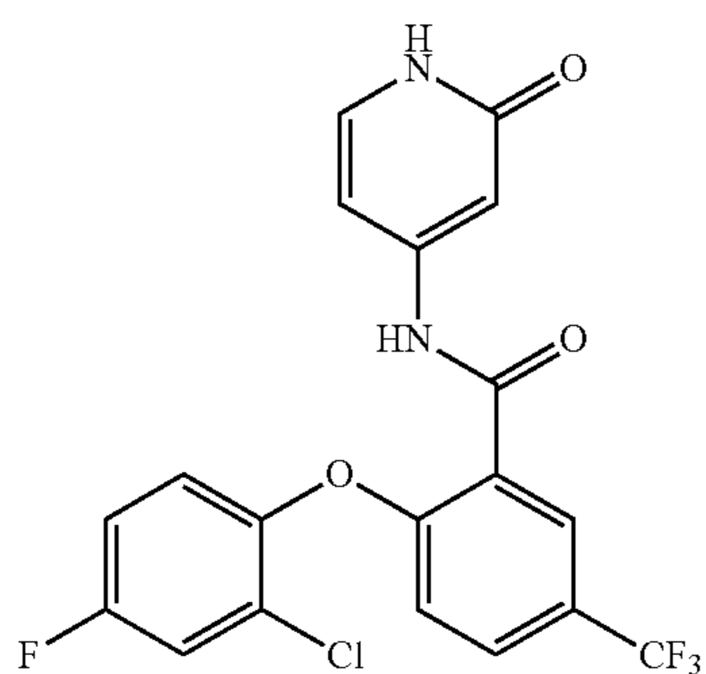
2-(2-chloro-4-fluorophenoxy)-N-(2-oxo-1,2-dihydropyridin-4-yl)-5-(trifluoromethyl)benzamide
