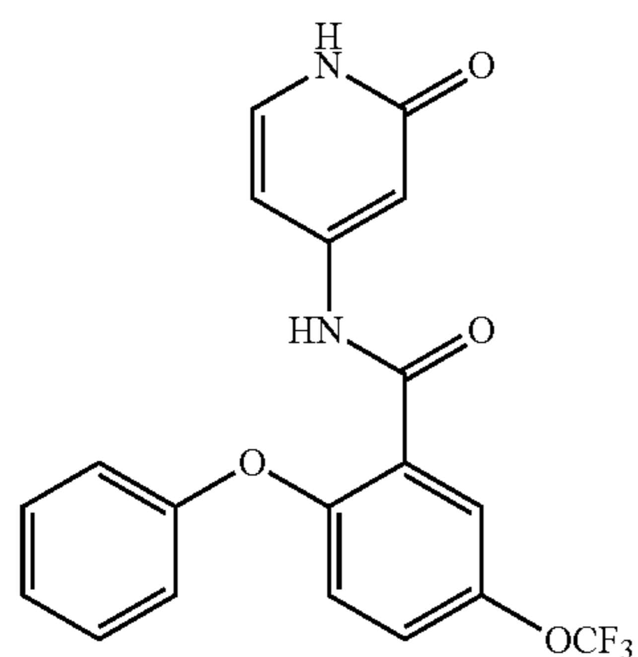
N-(2-oxo-1,2-dihydropyridin-4-yl)-2-phenoxy-5-(trifluoromethoxy)benzamide
