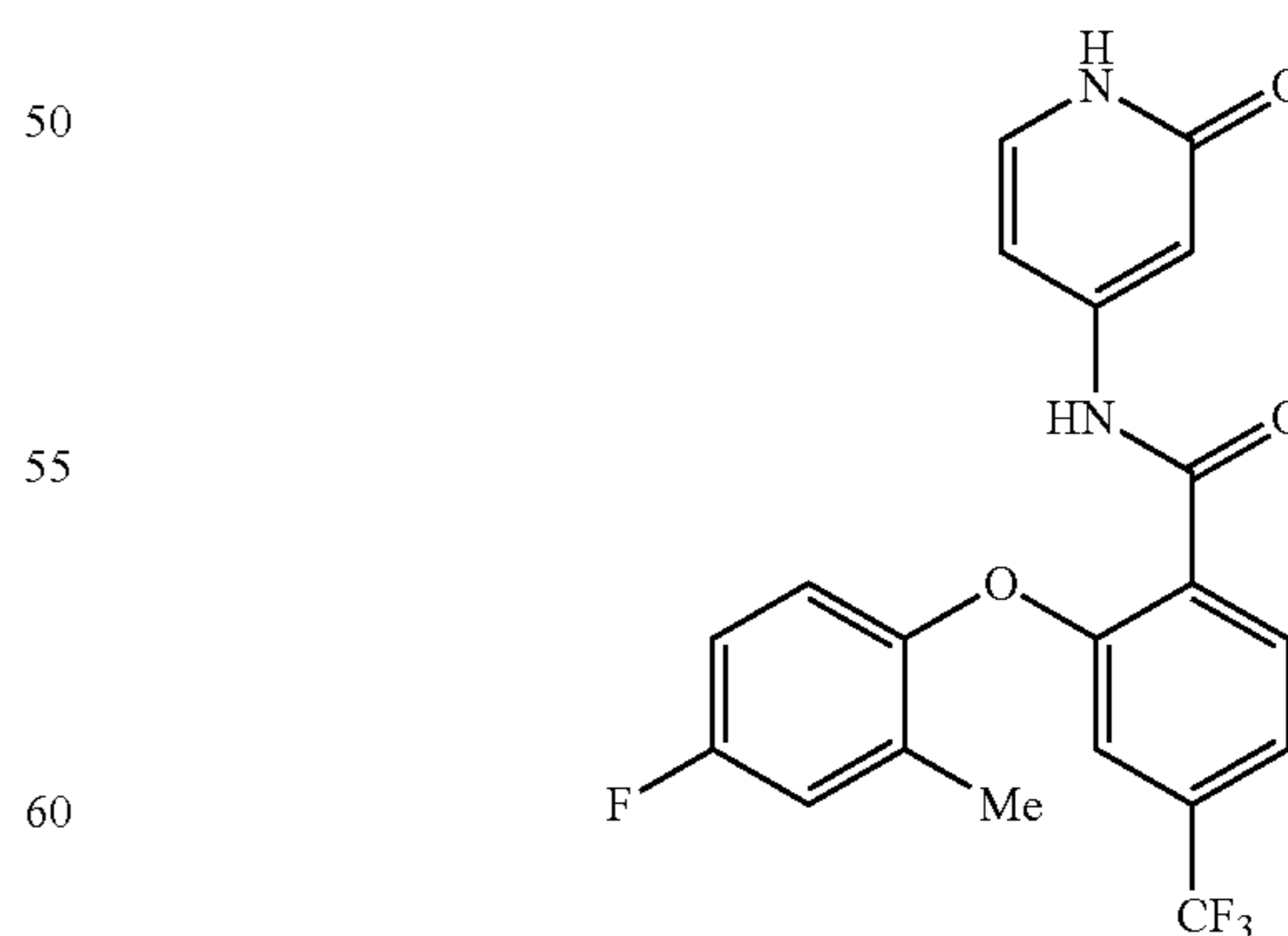
2-(4-fluoro-2-methylphenoxy)-N-(2-oxo-1,2-dihydropyridin-4-yl)-4-(trifluoromethyl)benzamide
