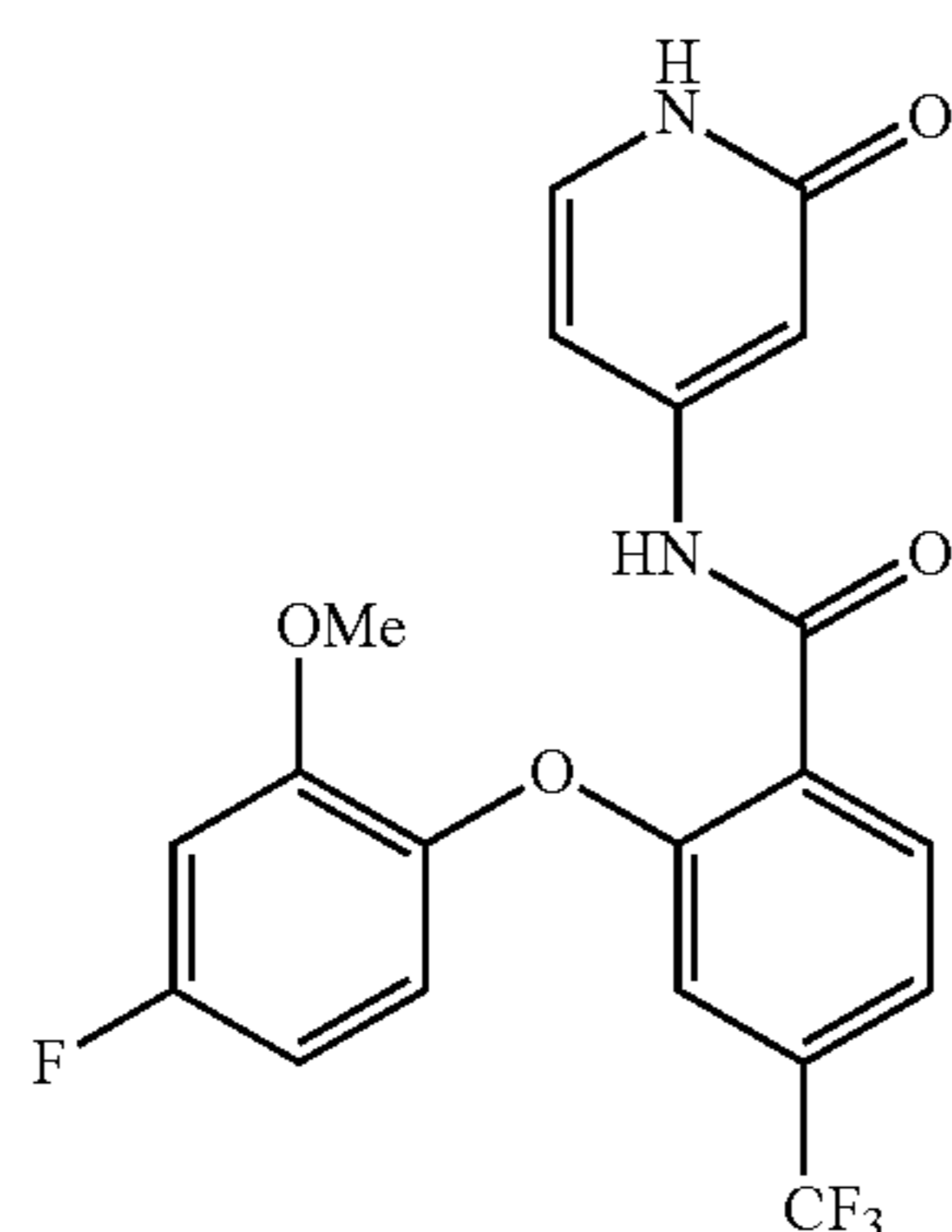
2-(4-fluoro-2-methoxyphenoxy)-N-(2-oxo-1,2-dihydropyridin-4-yl)-4-(trifluoromethyl)benzamide
