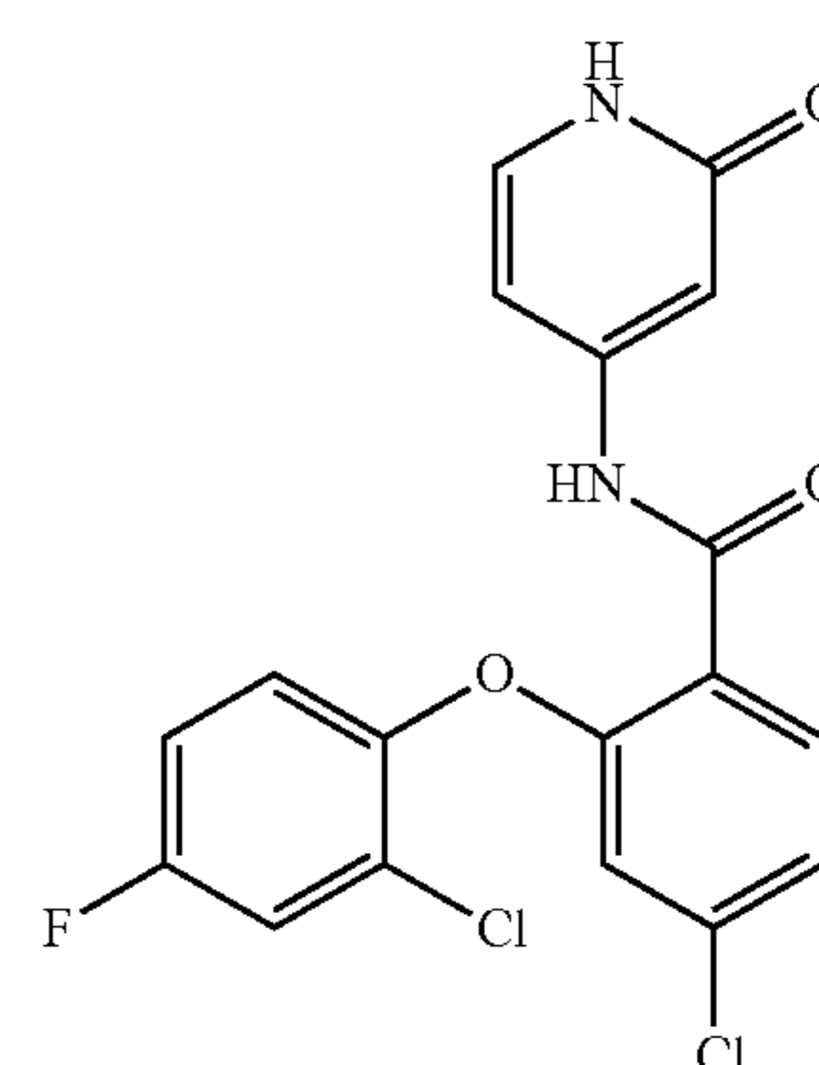
4-chloro-2-(2-chloro-4-fluorophenoxy)-N-(2-oxo-1,2-dihydropyridin-4-yl)benzamide
