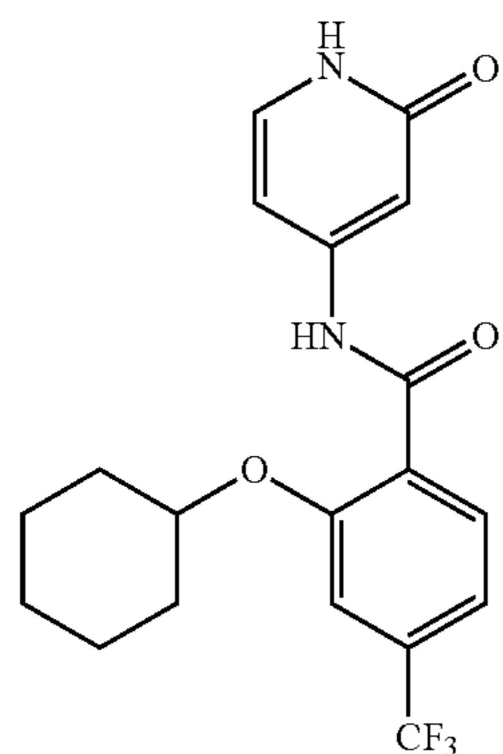
2-(cyclohexyloxy)-N-(2-oxo-1,2-dihydropyridin-4-yl)-4-(trifluoromethyl)benzamide
