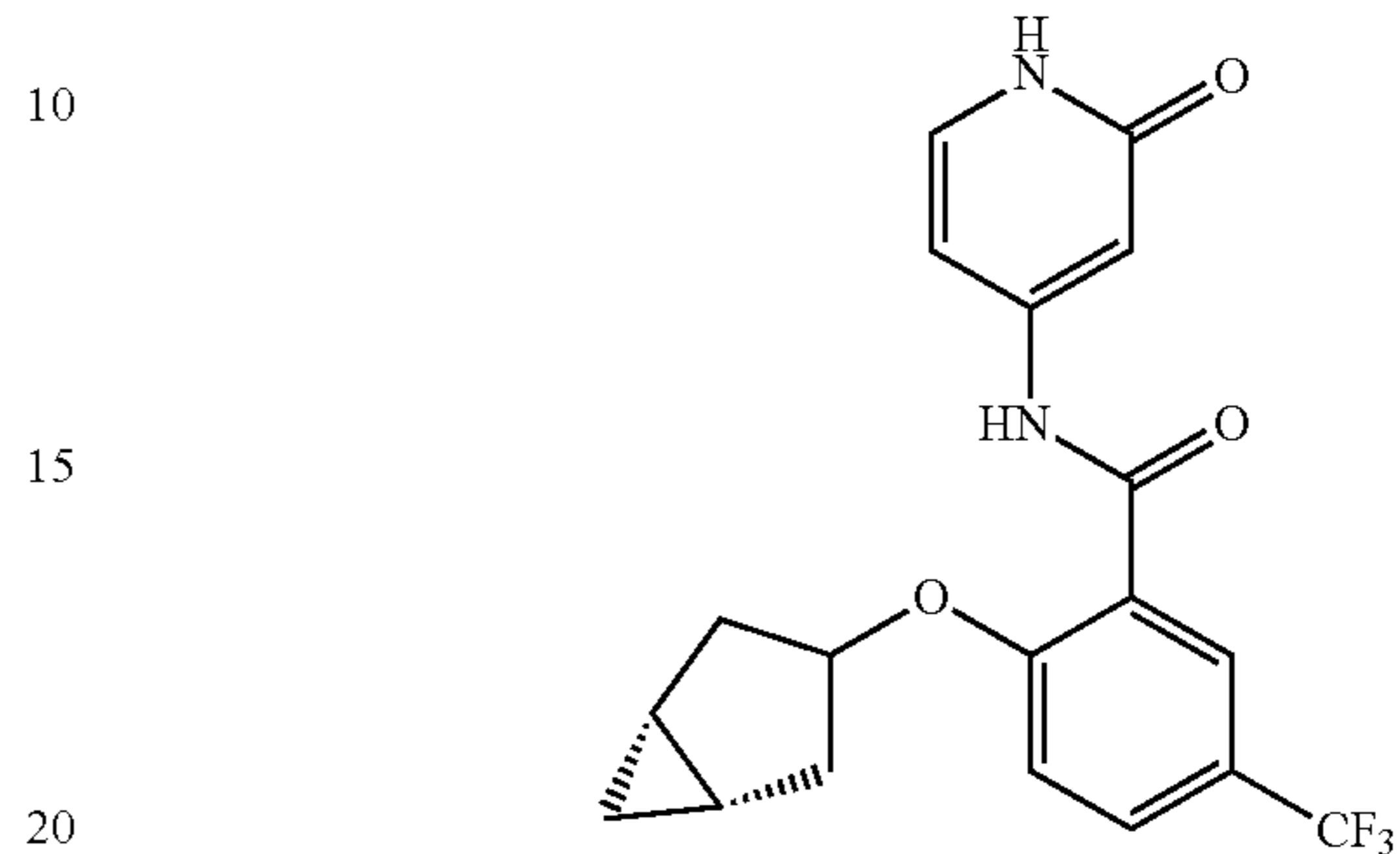
2-((1R,5S)-bicyclo[3.1.0]hexan-3-ylmethoxy)-N-(2-oxo-1,2-dihydropyridin-4-yl)-5-(trifluoromethyl)benzamide
