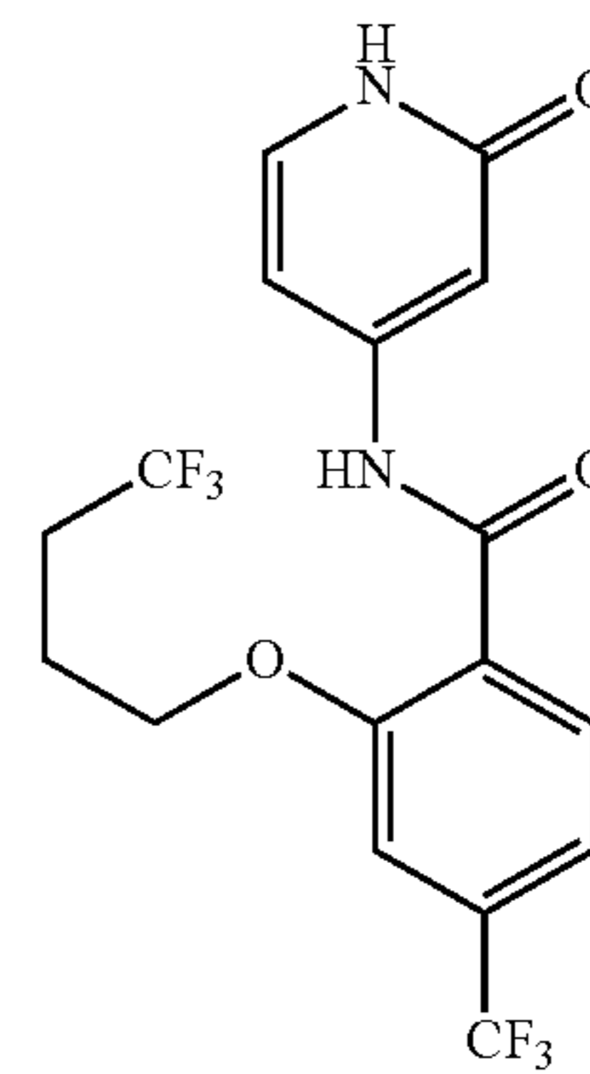
N-(2-oxo-1,2-dihydropyridin-4-yl)-2-(4,4,4-trifluorobutoxy)-4-(trifluoromethyl)benzamide
