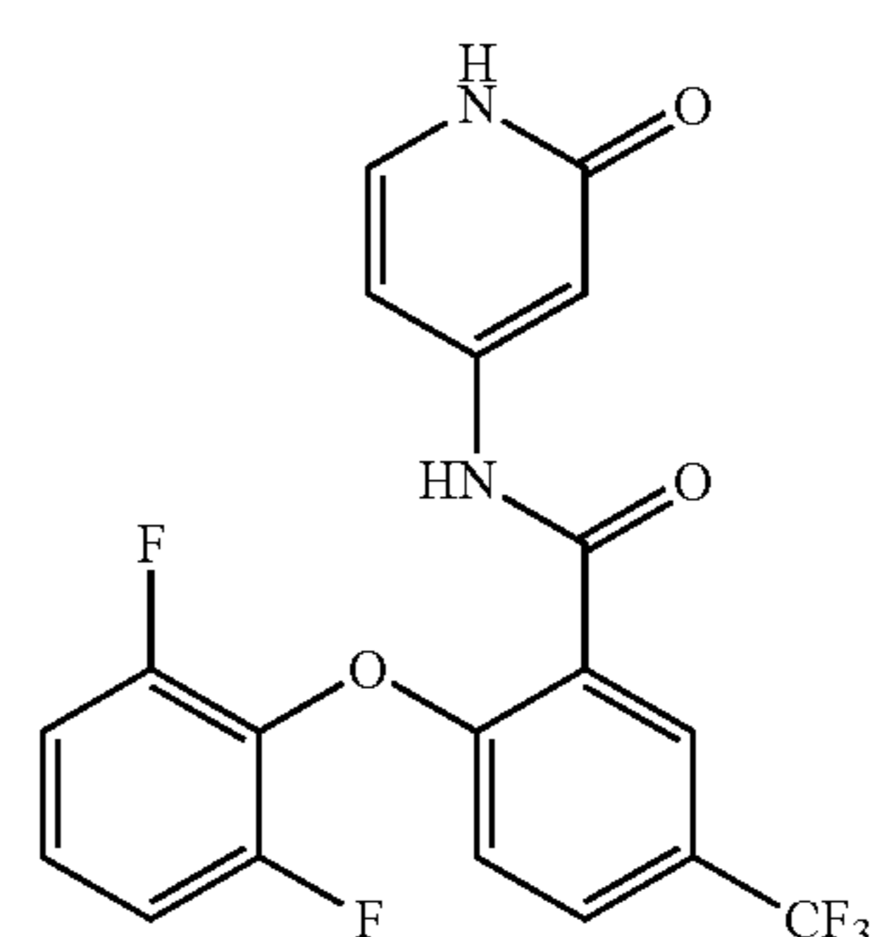
2-(2,6-difluorophenoxy)-N-(2-oxo-1,2-dihydropyridin-4-yl)-5-(trifluoromethyl)benzamide
