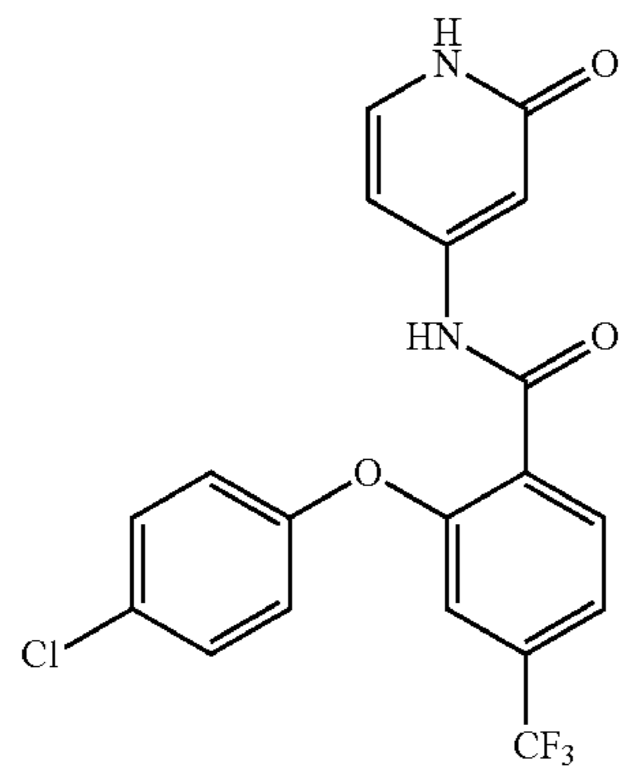
2-(4-chlorophenoxy)-N-(2-oxo-1,2-dihydropyridin-4-yl)-4-(trifluoromethyl)benzamide
