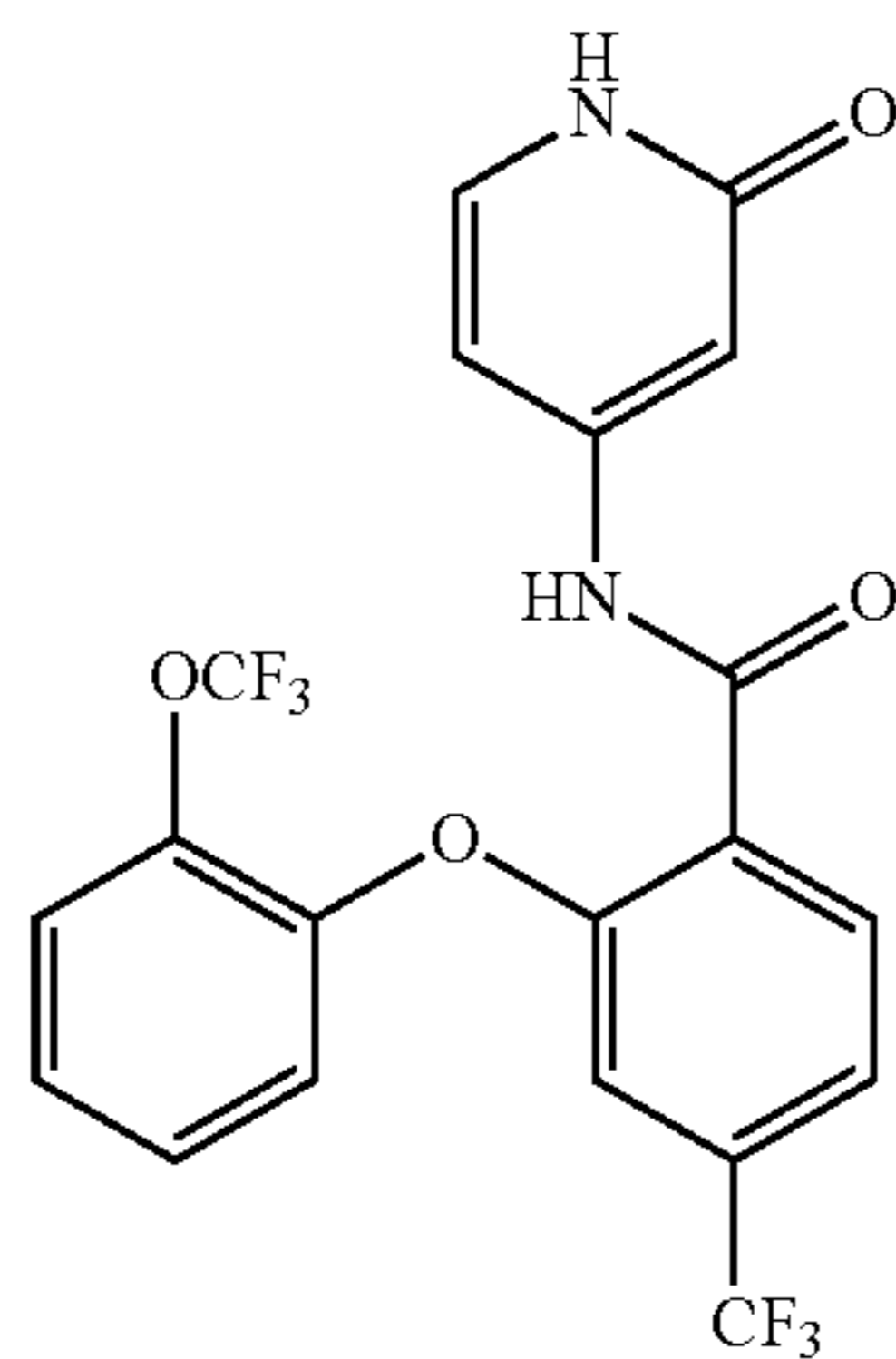
N-(2-oxo-1,2-dihydropyridin-4-yl)-2-(2-(trifluoromethoxy)phenoxy)-4-(trifluoromethyl)benzamide
