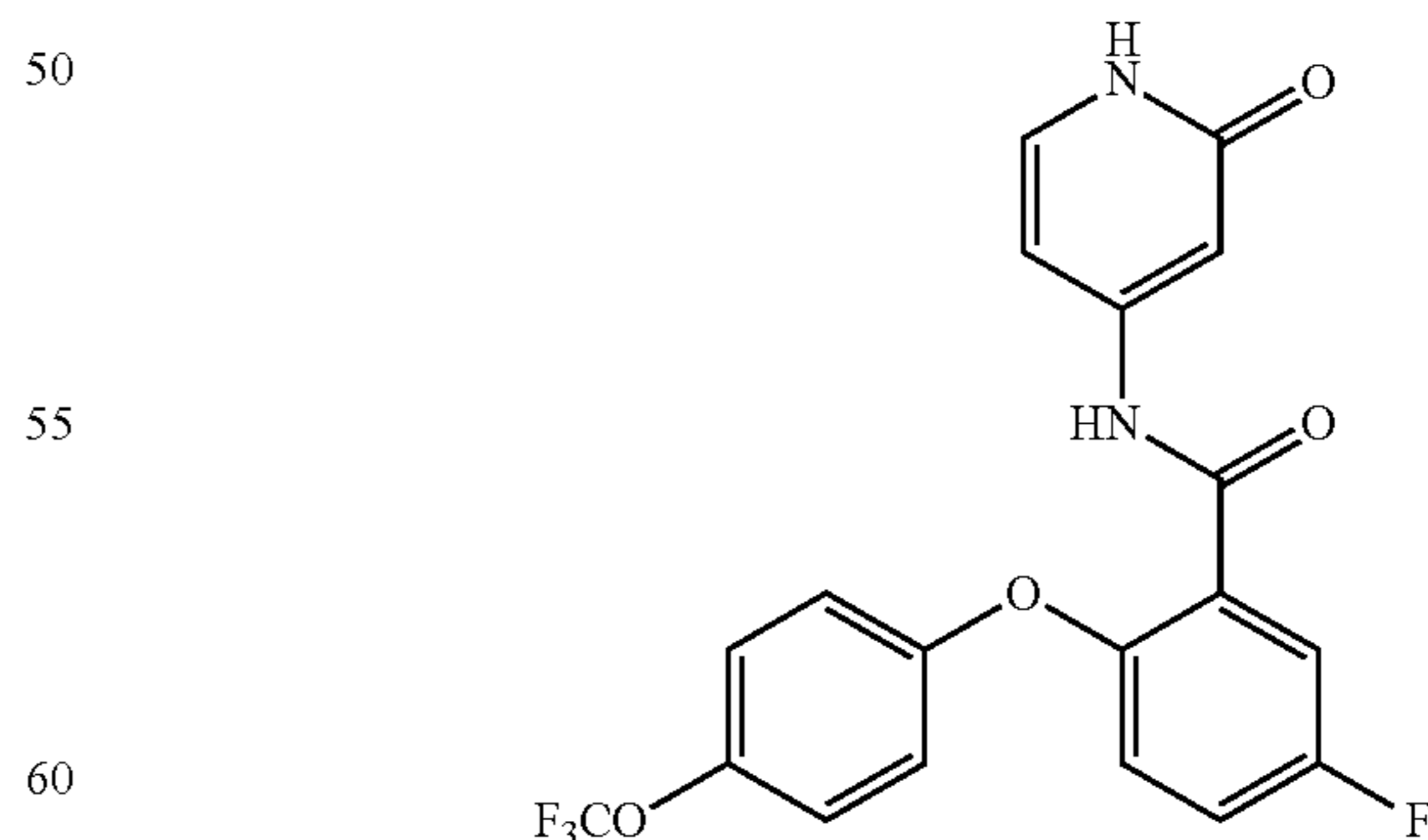
5-fluoro-N-(2-oxo-1,2-dihydropyridin-4-yl)-2-(4-(trifluoromethoxy)phenoxy)benzamide
