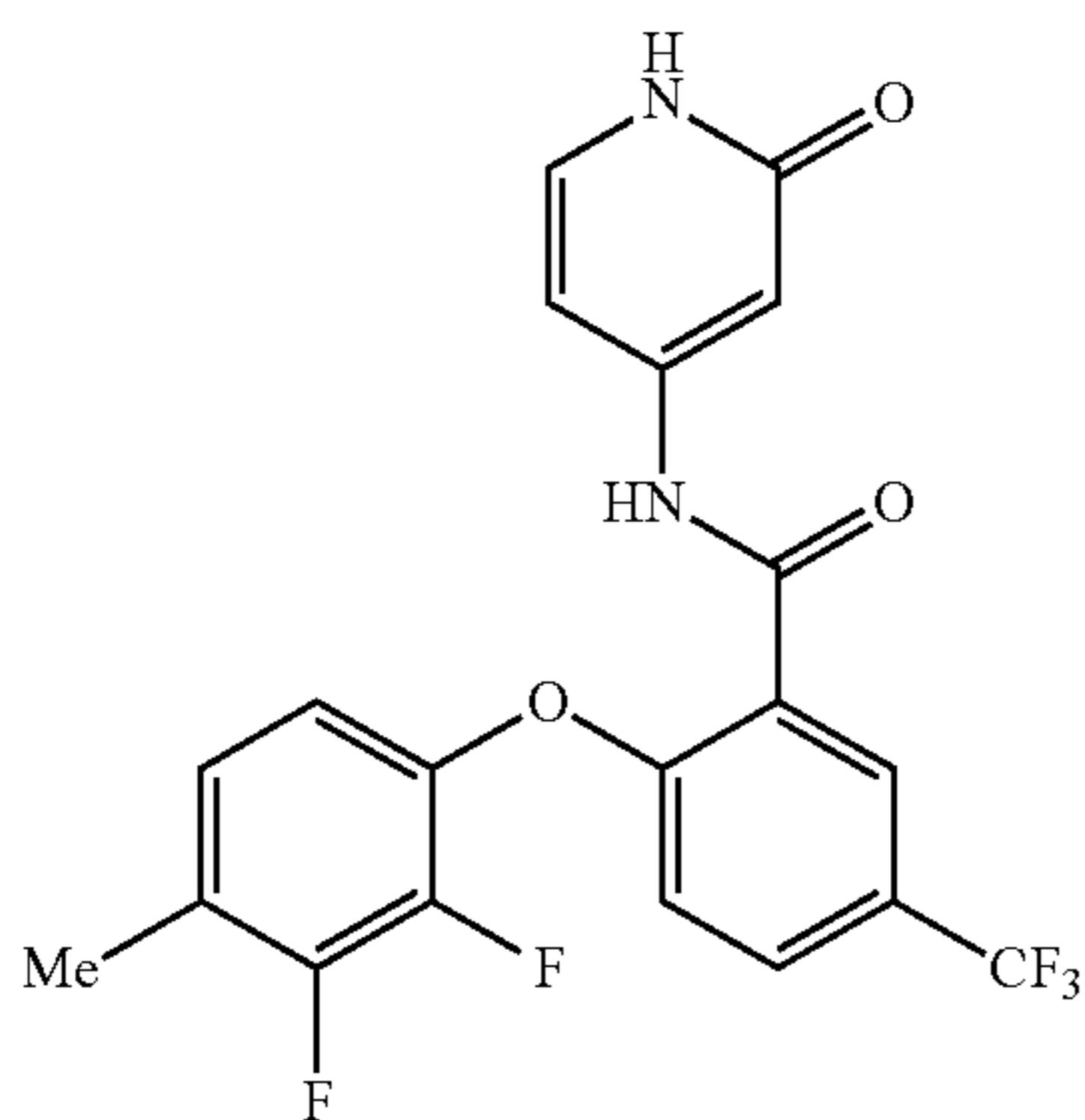
2-(2,3-difluoro-4-methylphenoxy)-N-(2-oxo-1,2-dihydropyridin-4-yl)-5-(trifluoromethyl)benzamide
