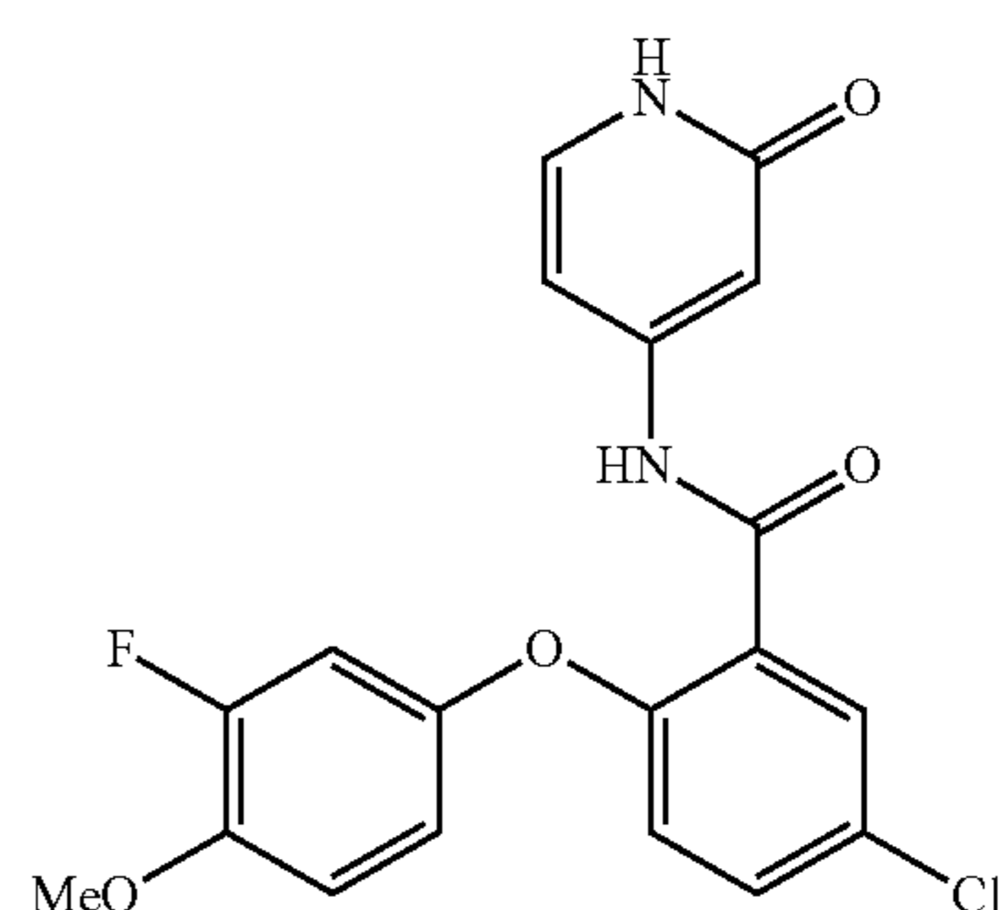
5-chloro-2-(3-fluoro-4-methoxyphenoxy)-N-(2-oxo-1,2-dihydropyridin-4-yl)benzamide
