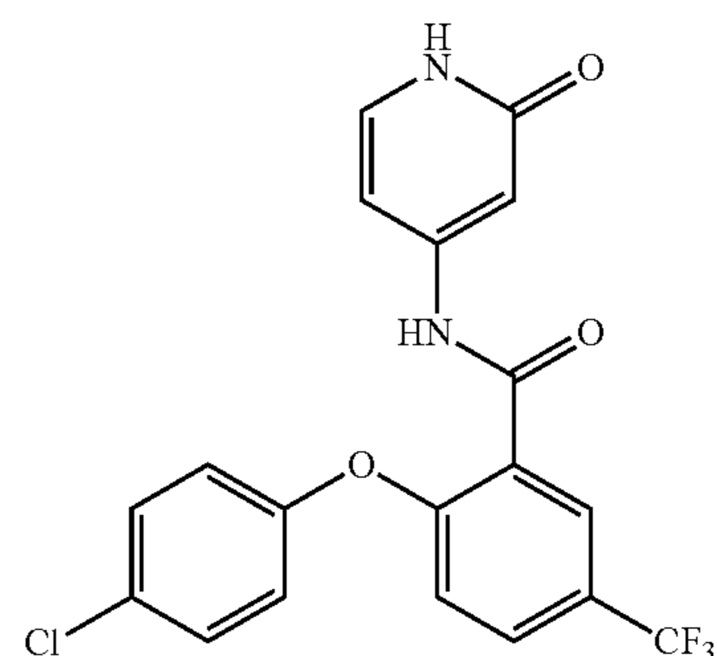
2-(4-chlorophenoxy)-N-(2-oxo-1,2-dihydropyridin-4-yl)-5-(trifluoromethyl)benzamide
