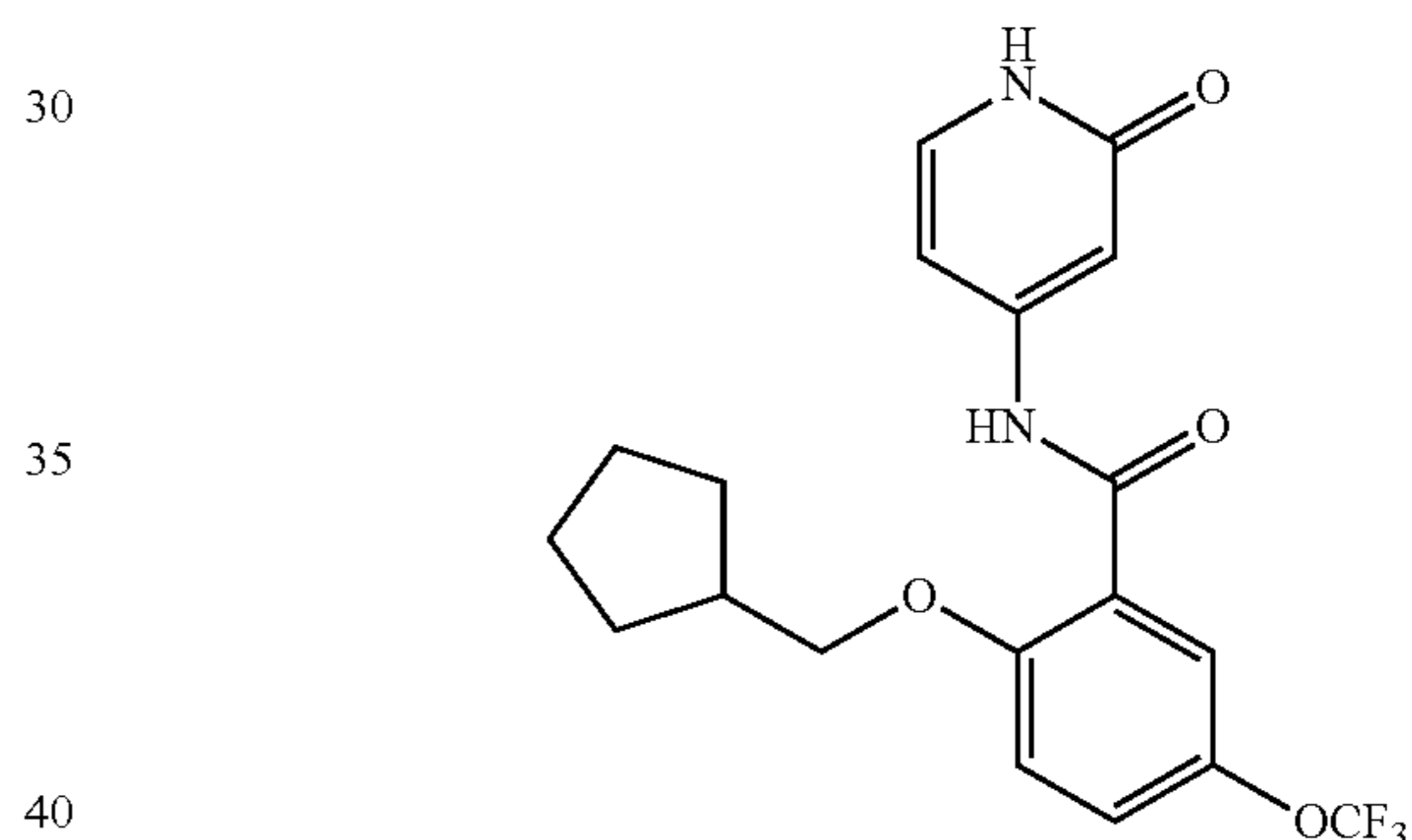
2-(cyclopentylmethoxy)-N-(2-oxo-1,2-dihydropyridin-4-yl)-5-(trifluoromethoxy)benzamide
