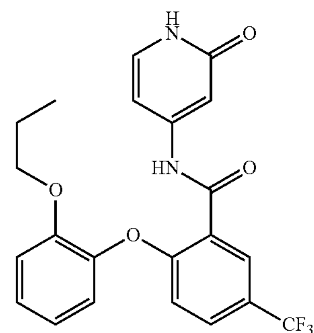
N-(2-oxo-1,2-dihydropyridin-4-yl)-2-(2-propoxyphenoxy)-5-(trifluoromethyl)benzamide
