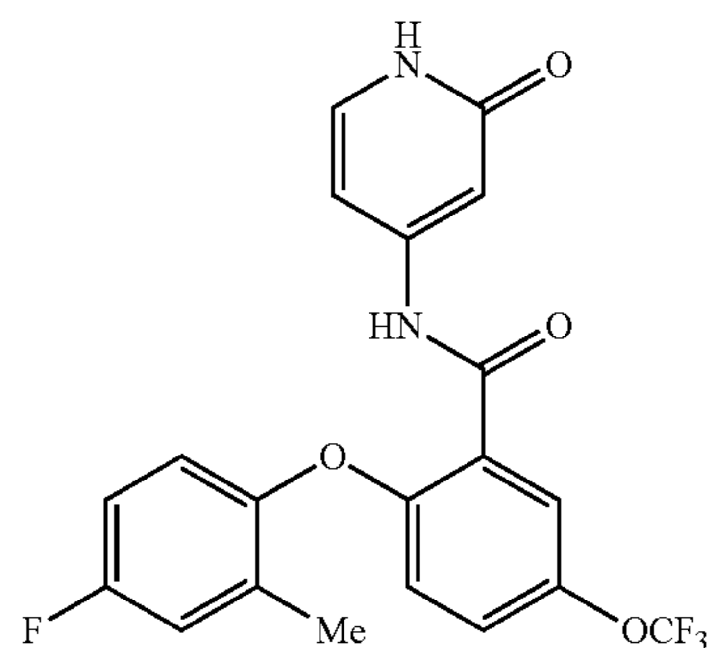
2-(4-fluoro-2-methylphenoxy)-N-(2-oxo-1,2-dihydropyridin-4-yl)-5-(trifluoromethoxy)benzamide
