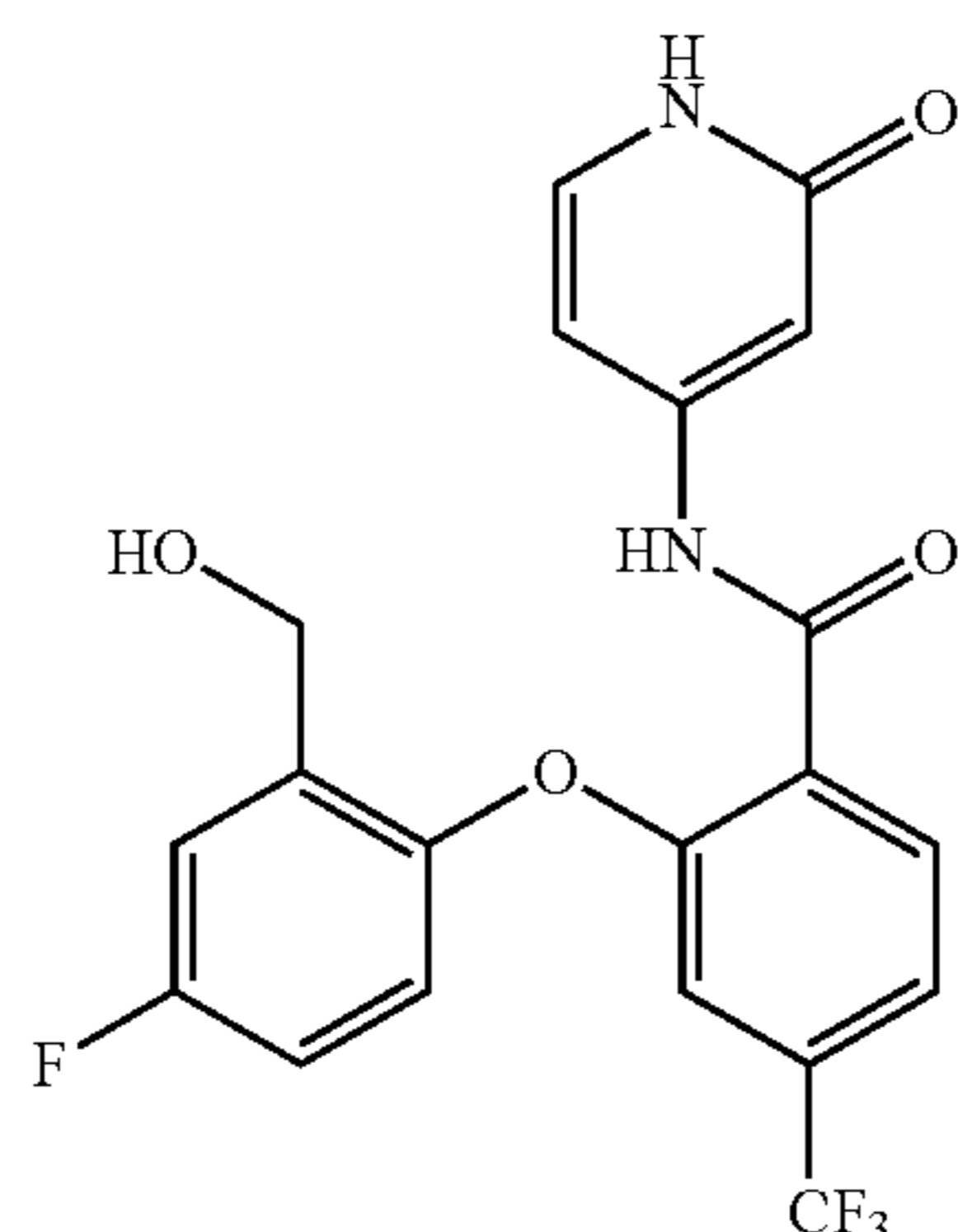
2-(4-fluoro-2-(hydroxymethyl)phenoxy)-N-(2-oxo-1,2-dihydropyridin-4-yl)-4-(trifluoromethyl)benzamide
