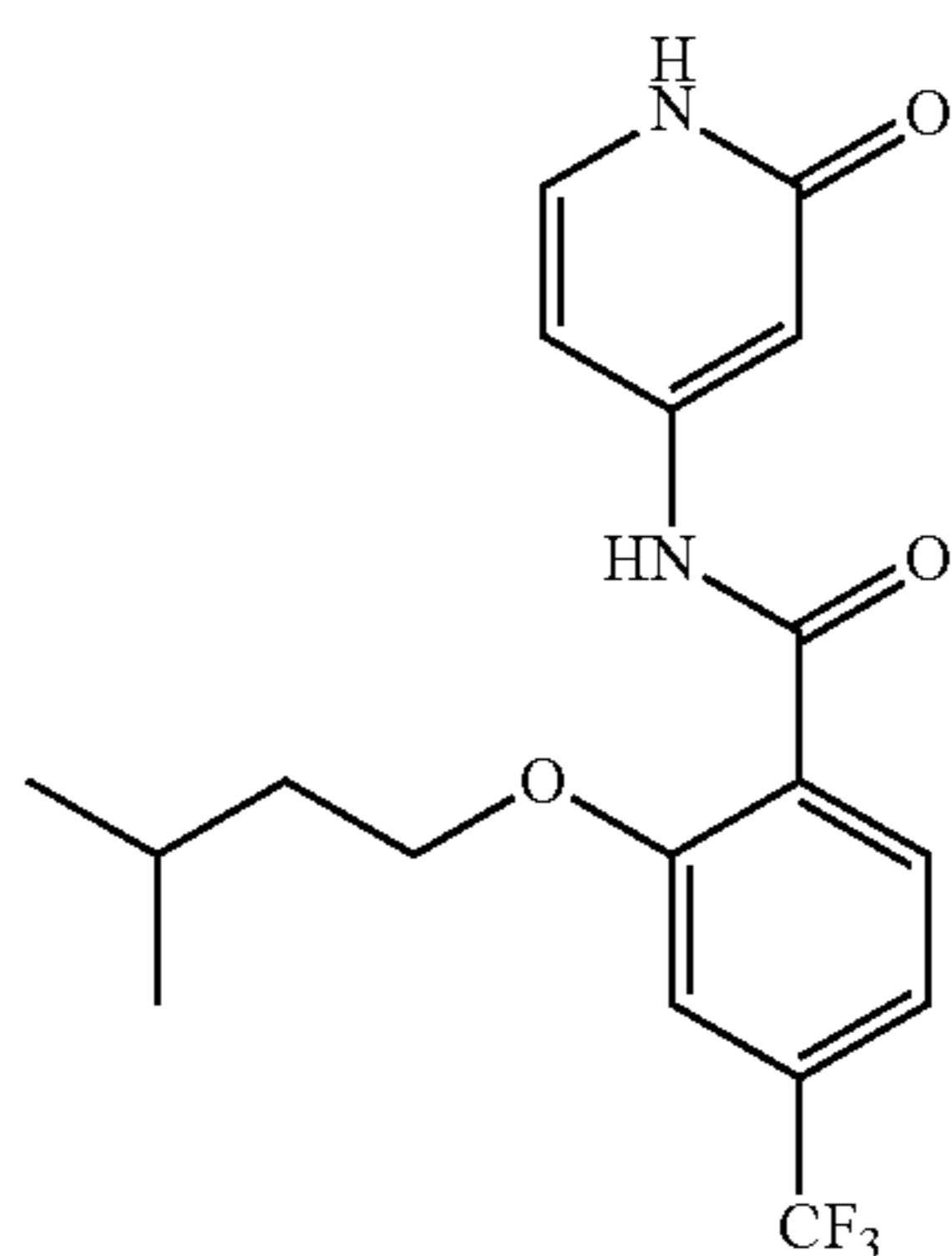
2-(isopentyloxy)-N-(2-oxo-1,2-dihydropyridin-4-yl)-4-(trifluoromethyl)benzamide
