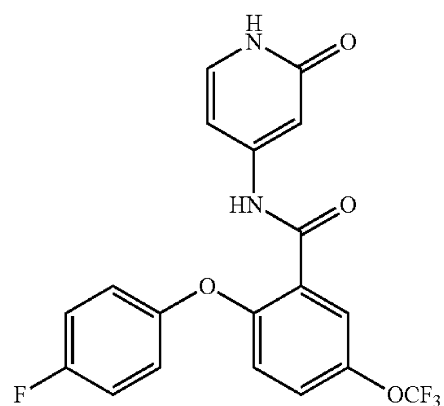
2-(4-fluorophenoxy)-N-(2-oxo-1,2-dihydropyridin-4-yl)-5-(trifluoromethoxy)benzamide
