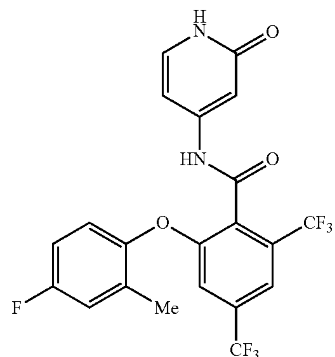
2-(4-fluoro-2-methylphenoxy)-N-(2-oxo-1,2-dihydropyridin-4-yl)-4,6-bis(trifluoromethyl)benzamide
