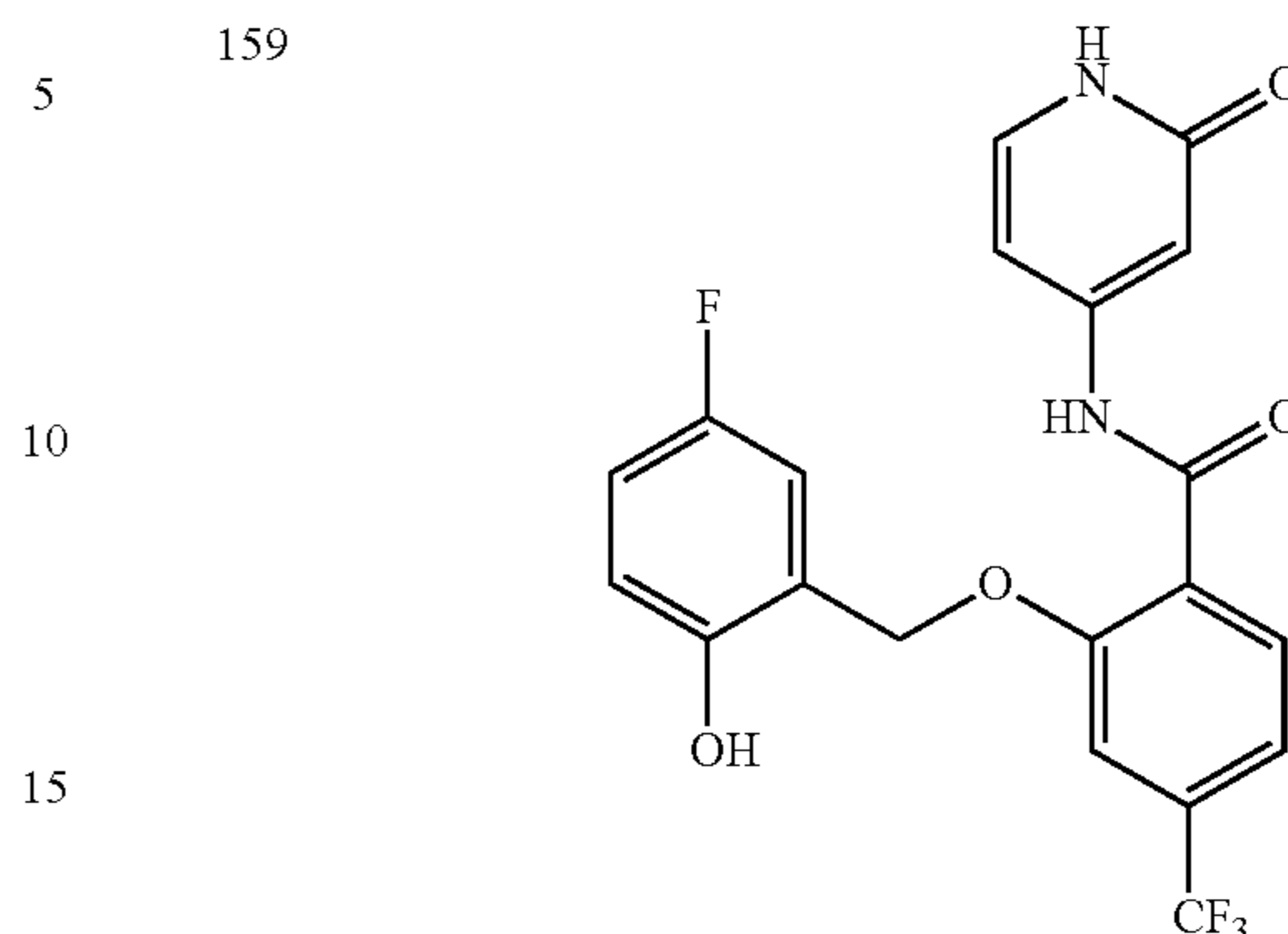
2-((5-fluoro-2-hydroxybenzyl)oxy)-N-(2-oxo-1,2-dihydropyridin-4-yl)-4-(trifluoromethyl)benzamide
