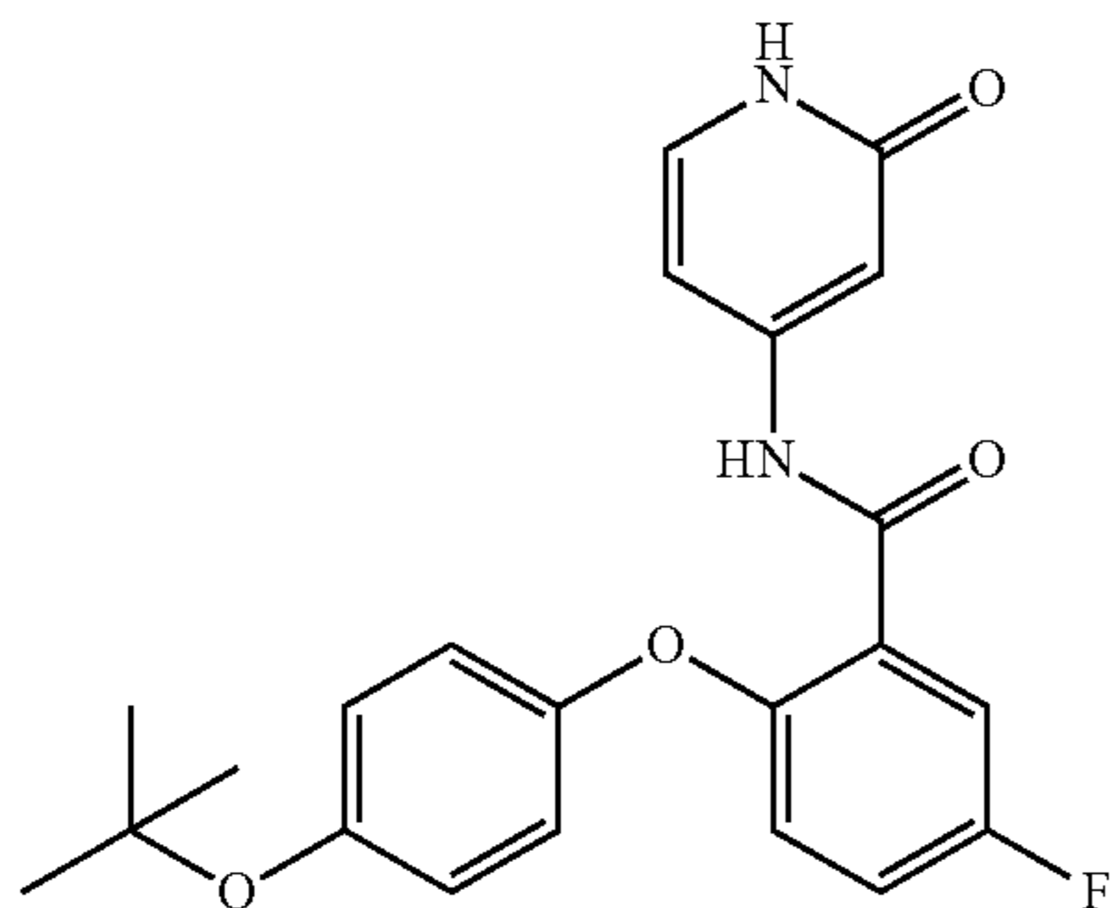
2-(4-(tert-butoxy)phenoxy)-5-fluoro-N-(2-oxo-1,2-dihydropyridin-4-yl)benzamide
