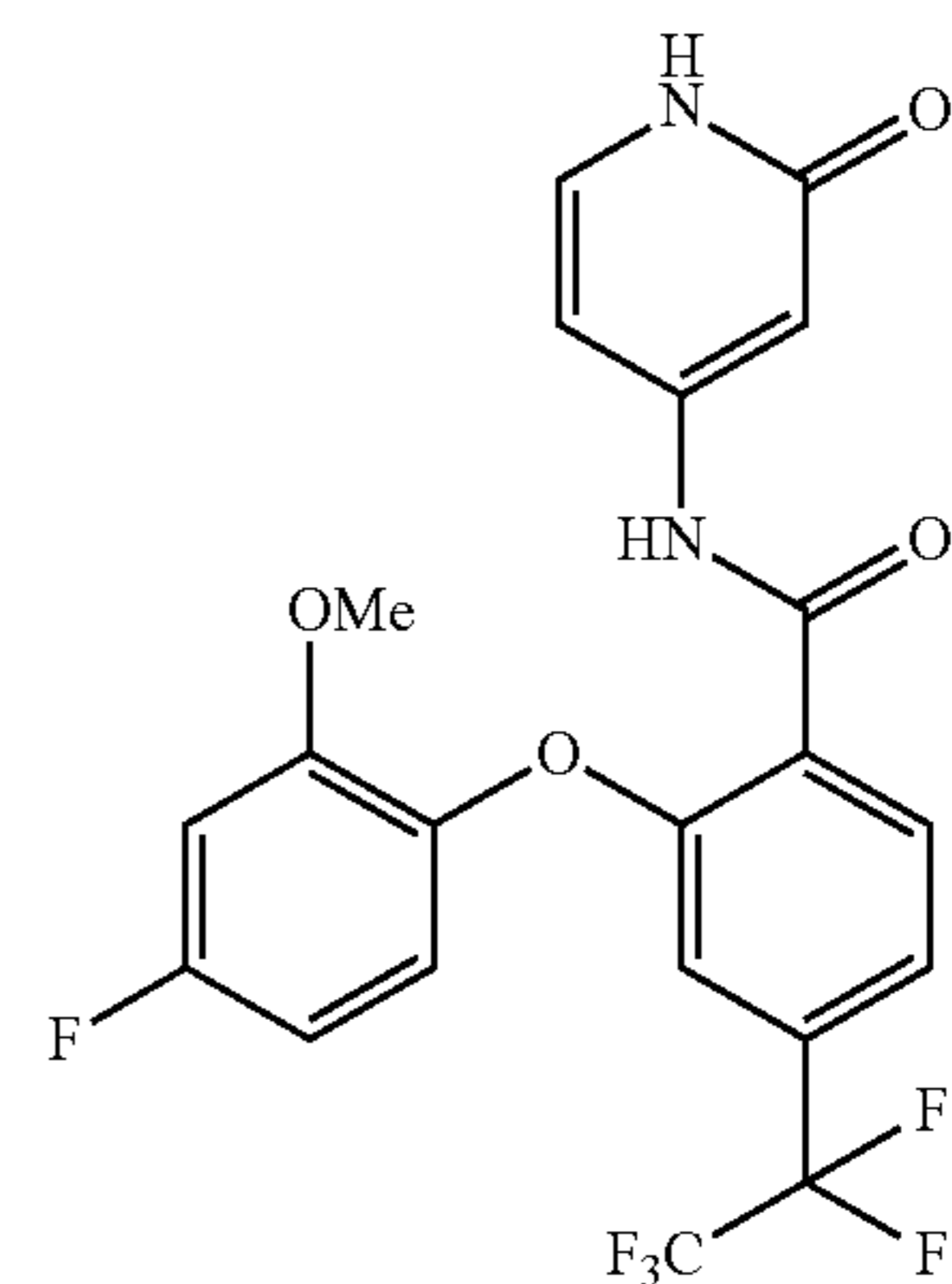
2-(4-fluoro-2-methoxyphenoxy)-N-(2-oxo-1,2-dihydropyridin-4-yl)-4-(perfluoroethyl)benzamide
