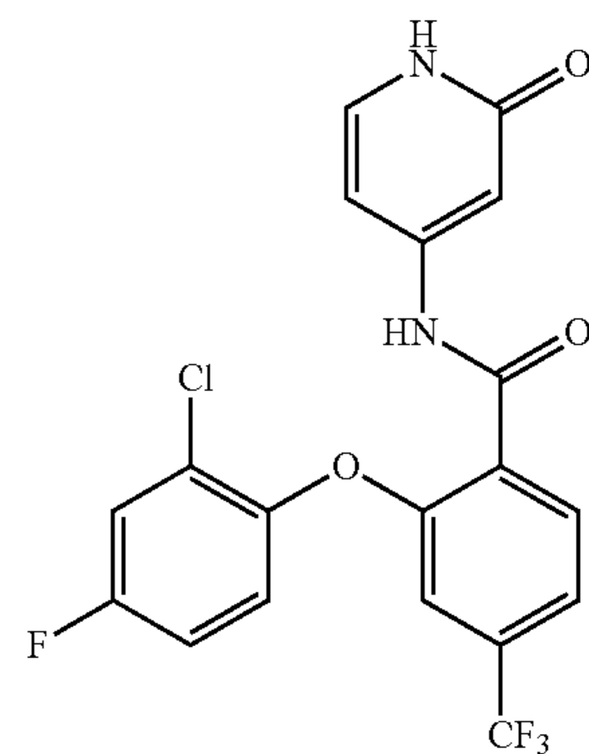
2-(2-chloro-4-fluorophenoxy)-N-(2-oxo-1,2-dihydropyridin-4-yl)-4-(trifluoromethyl)benzamide
