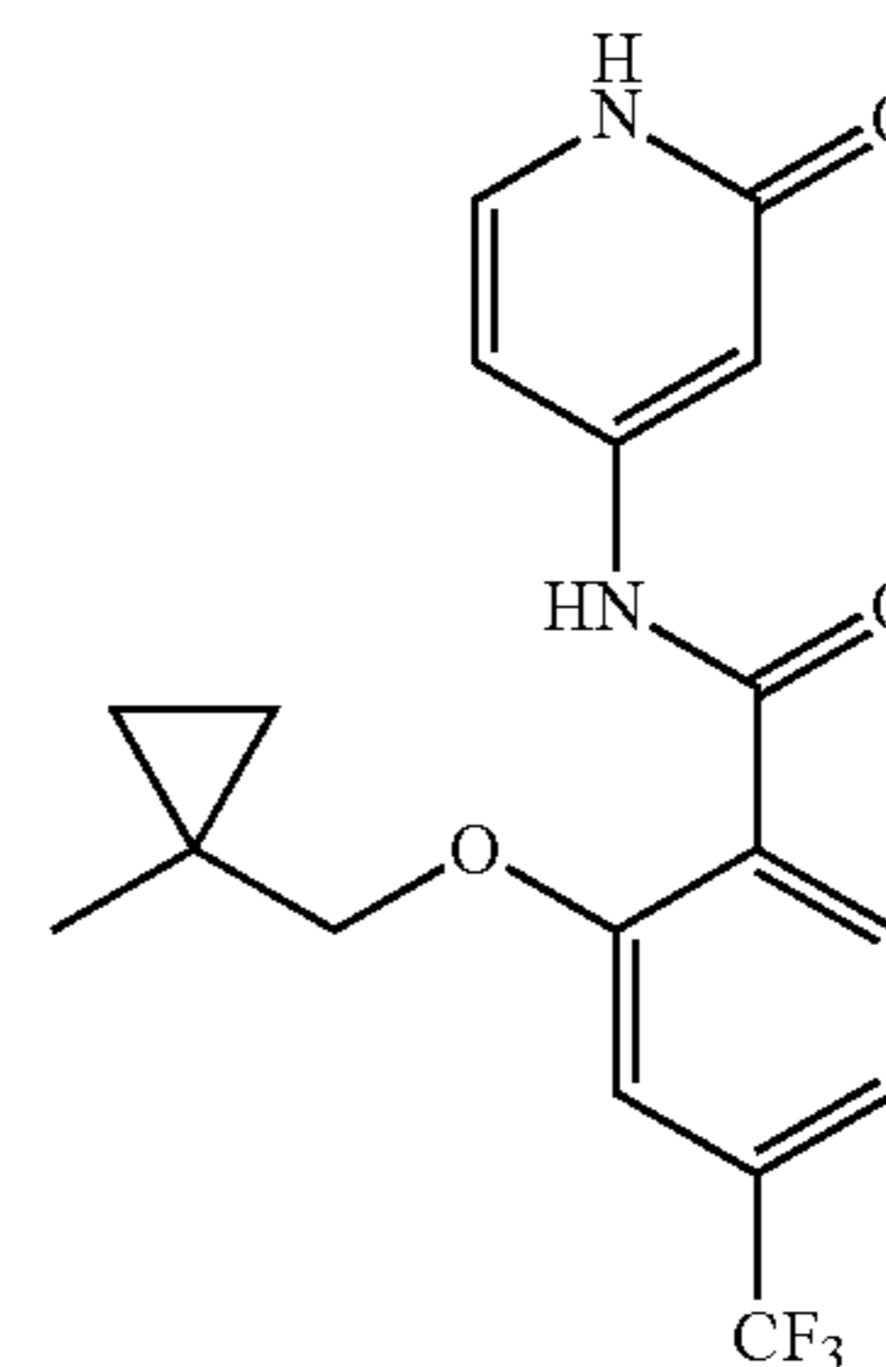
2-((1-methylcyclopropyl)methoxy)-N-(2-oxo-1,2-dihydropyridin-4-yl)-4-(trifluoromethyl)benzamide
