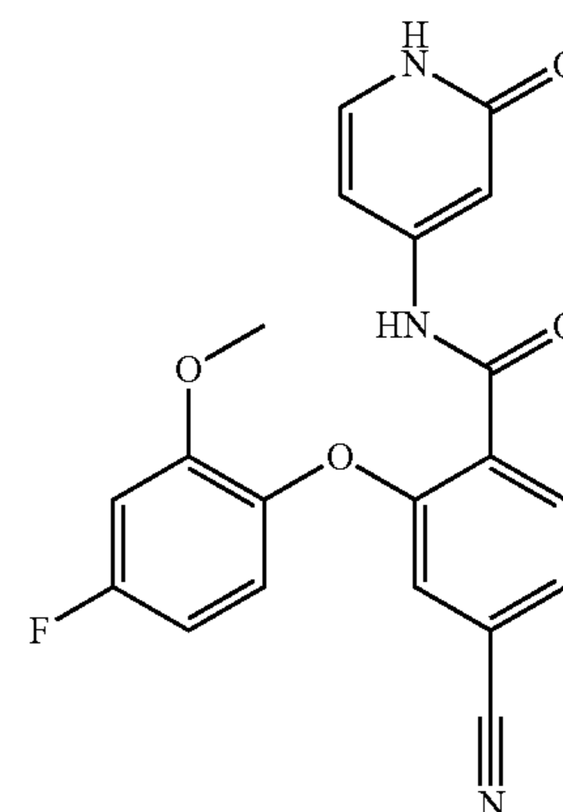
4-cyano-2-(4-fluoro-2-methoxyphenoxy)-N-(2-oxo-1,2-dihydropyridin-4-yl)benzamide
