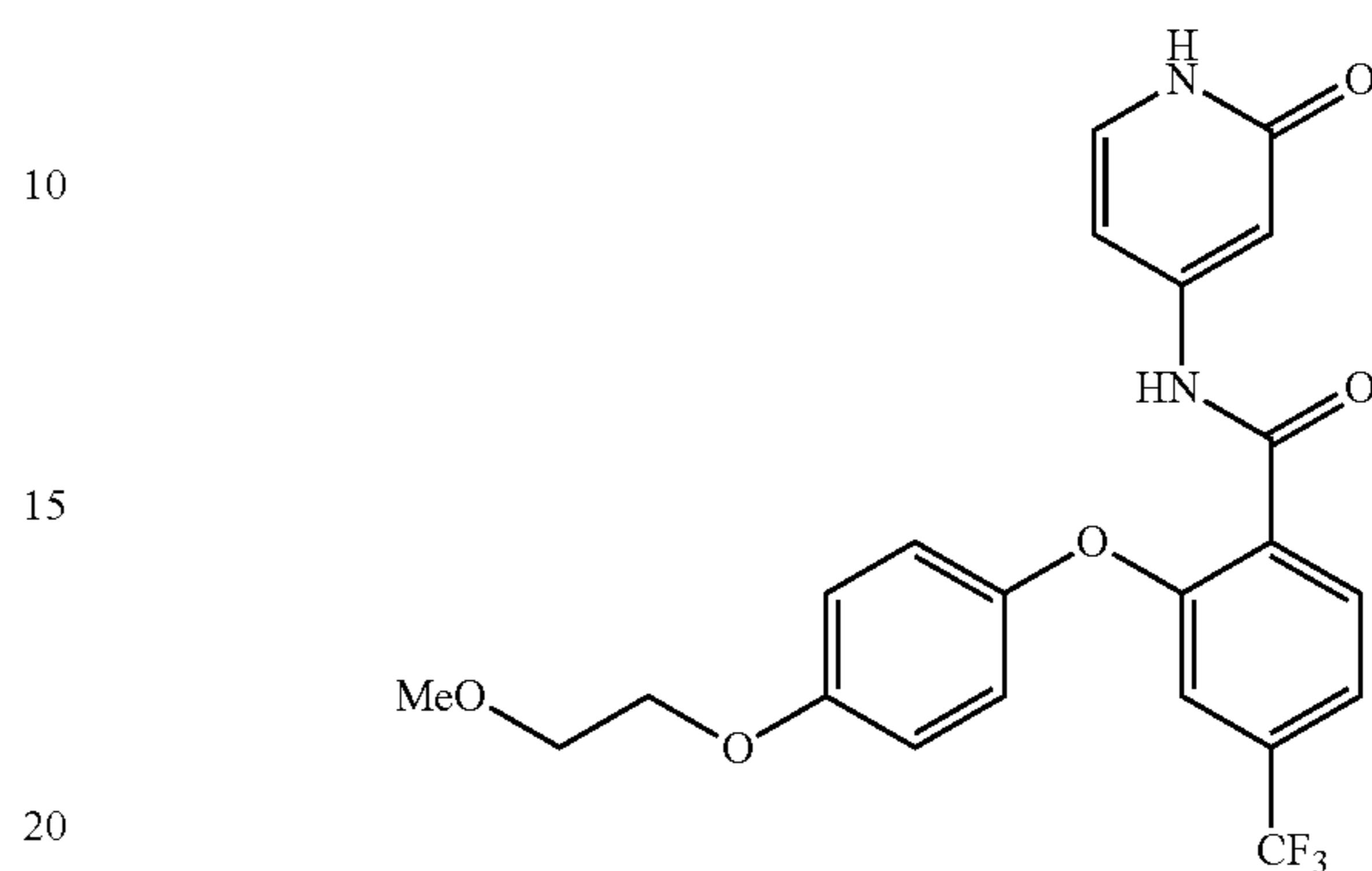
2-(4-(2-methoxyethoxy)phenoxy)-N-(2-oxo-1,2-dihydropyridin-4-yl)-4-(trifluoromethyl)benzamide
