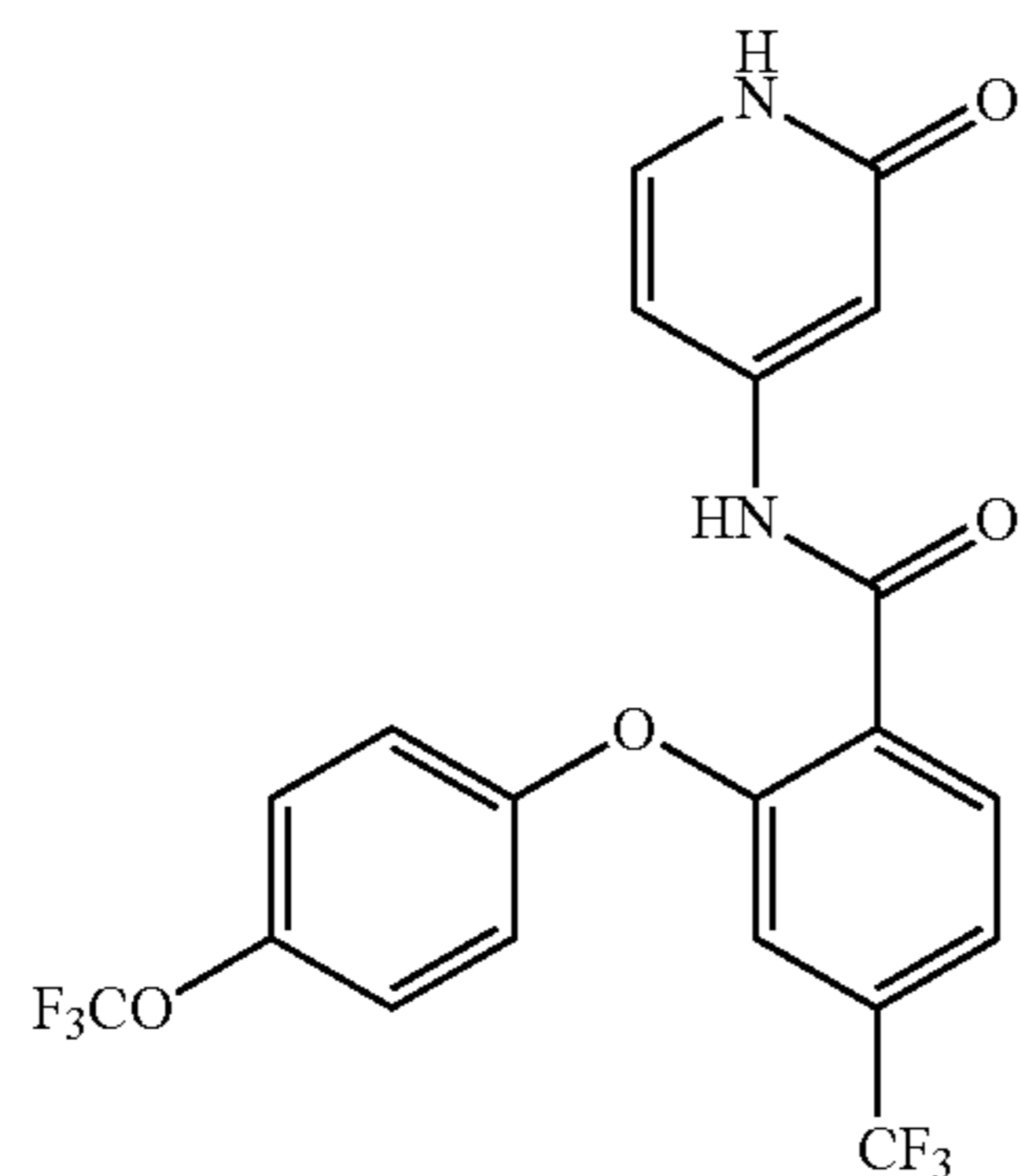
N-(2-oxo-1,2-dihydropyridin-4-yl)-2-(4-(trifluoromethoxy)phenoxy)-4-(trifluoromethyl)benzamide
