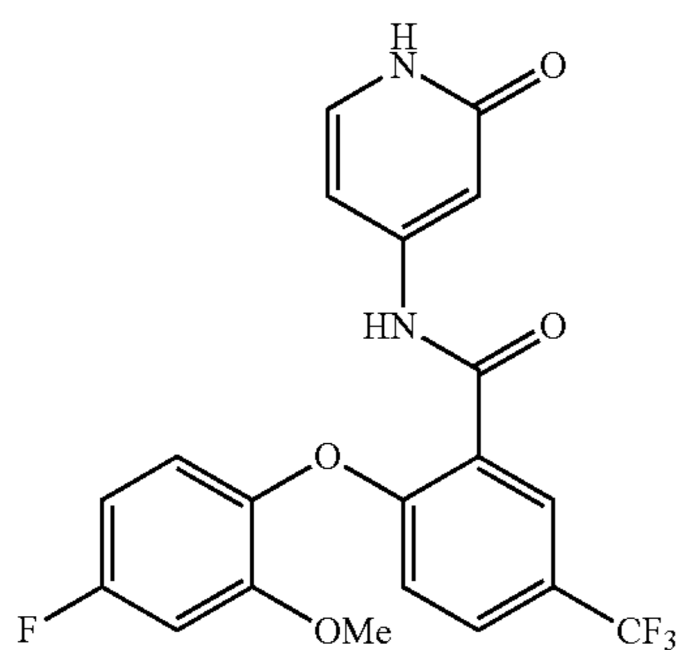
2-(4-fluoro-2-methoxyphenoxy)-N-(2-oxo-1,2-dihydropyridin-4-yl)-5-(trifluoromethyl)benzamide
