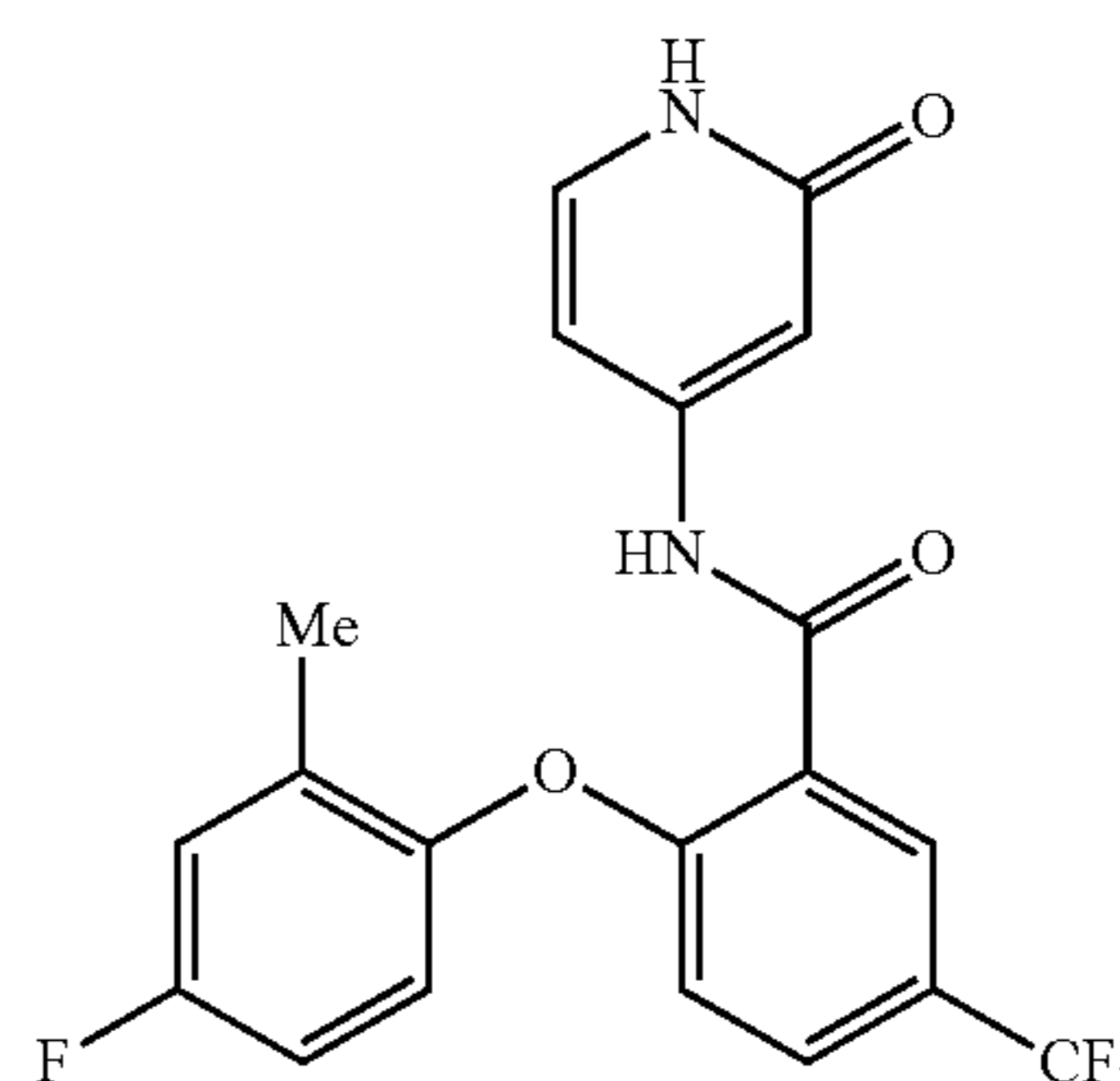
2-(4-fluoro-2-methylphenoxy)-N-(2-oxo-1,2-dihydropyridin-4-yl)-5-(trifluoromethyl)benzamide
