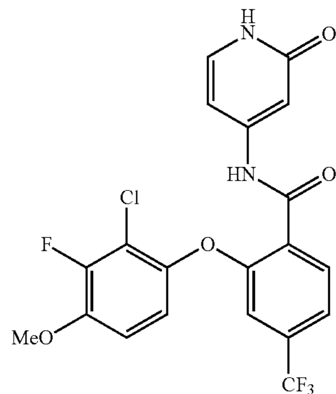
2-(2-chloro-3-fluoro-4-methoxyphenoxy)-N-(2-oxo-1,2-dihydropyridin-4-yl)-4-(trifluoromethyl)benzamide
