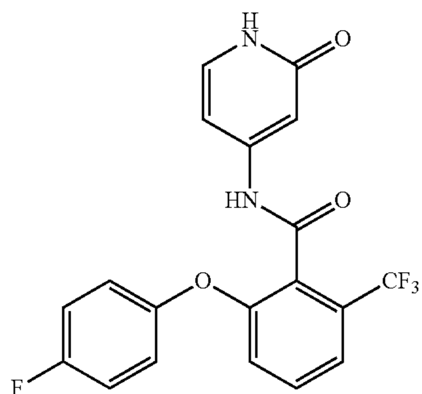
2-(4-fluorophenoxy)-N-(2-oxo-1,2-dihydropyridin-4-yl)-6-(trifluoromethyl)benzamide
