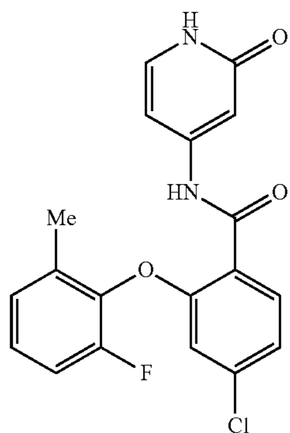
4-chloro-2-(2-fluoro-6-methylphenoxy)-N-(2-oxo-1,2-dihydropyridin-4-yl)benzamide
