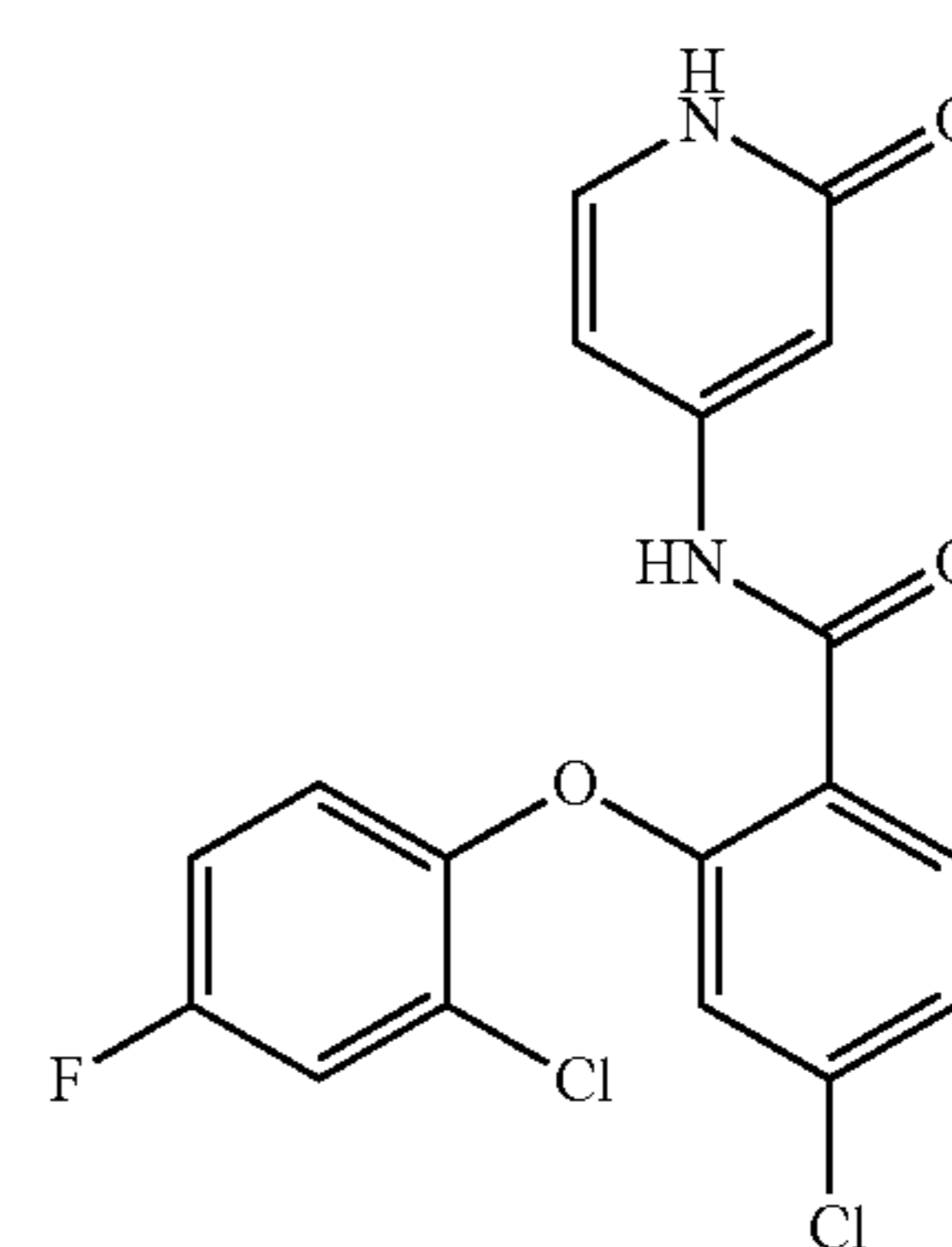
4-chloro-2-(2-chloro-4-fluorophenoxy)-N-(2-oxo-1,2-dihydropyridin-4-yl)benzamide
