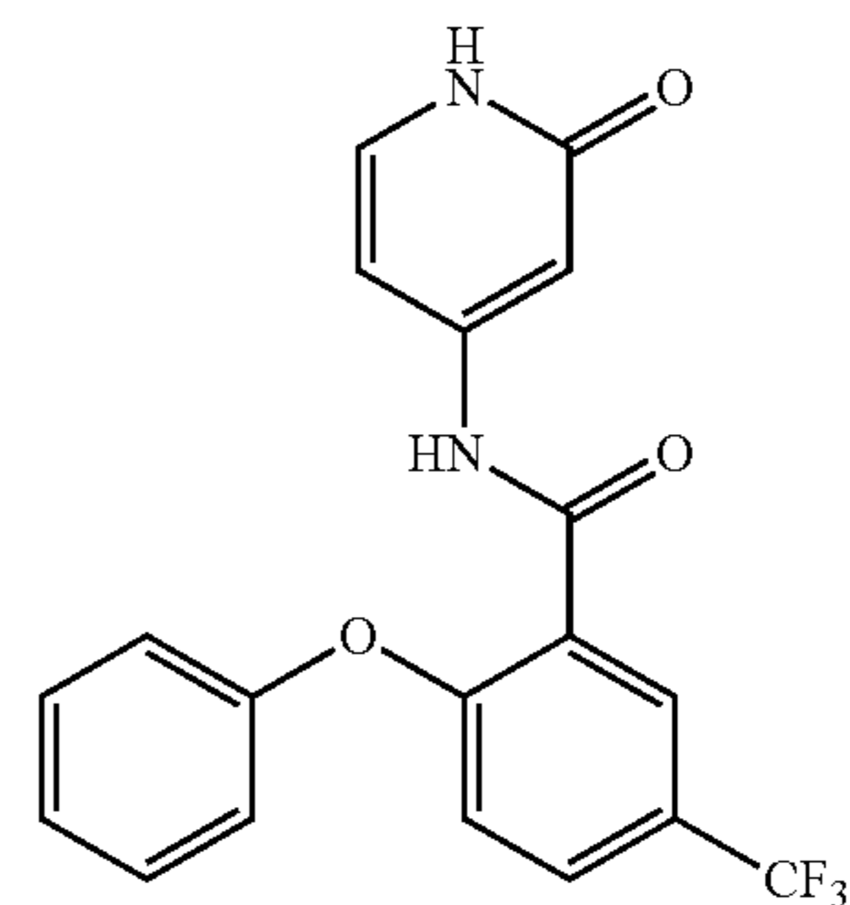
N-(2-oxo-1,2-dihydropyridin-4-yl)-2-phenoxy-5-(trifluoromethyl)benzamide
