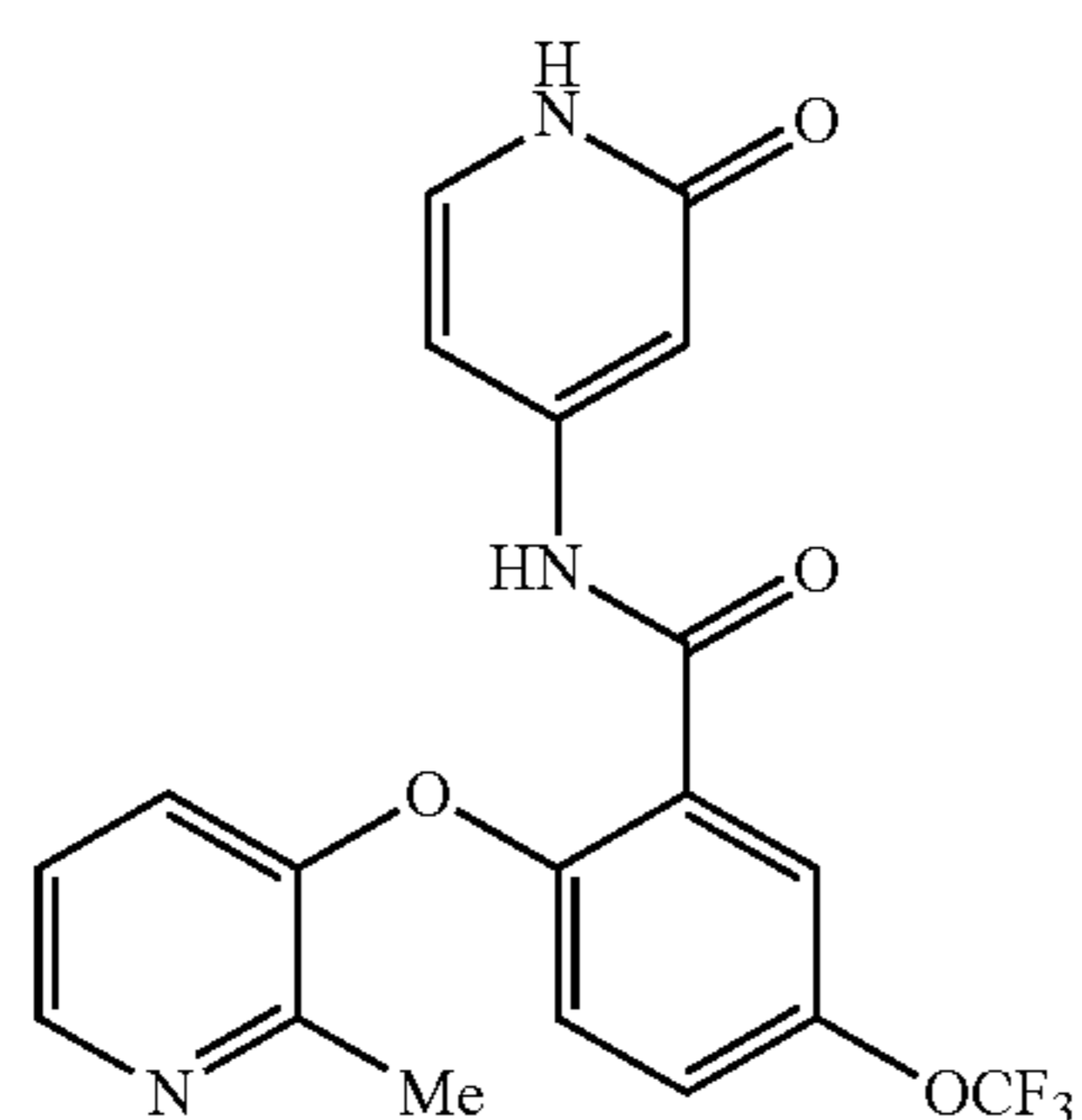
2-((2-methylpyridin-3-yl)oxy)-N-(2-oxo-1,2-dihydropyridin-4-yl)-5-(trifluoromethoxy)benzamide
