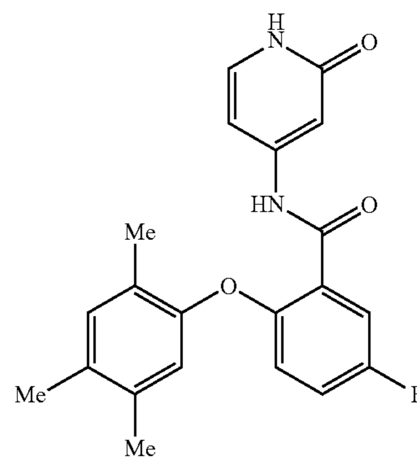
5-fluoro-N-(2-oxo-1,2-dihydropyridin-4-yl)-2-(2,4,5-trimethylphenoxy)benzamide
