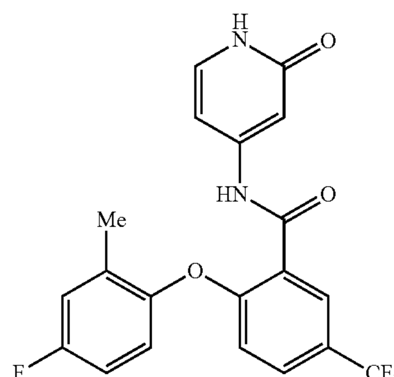
2-(4-fluoro-2-methylphenoxy)-N-(2-oxo-1,2-dihydropyridin-4-yl)-5-(trifluoromethyl)benzamide
