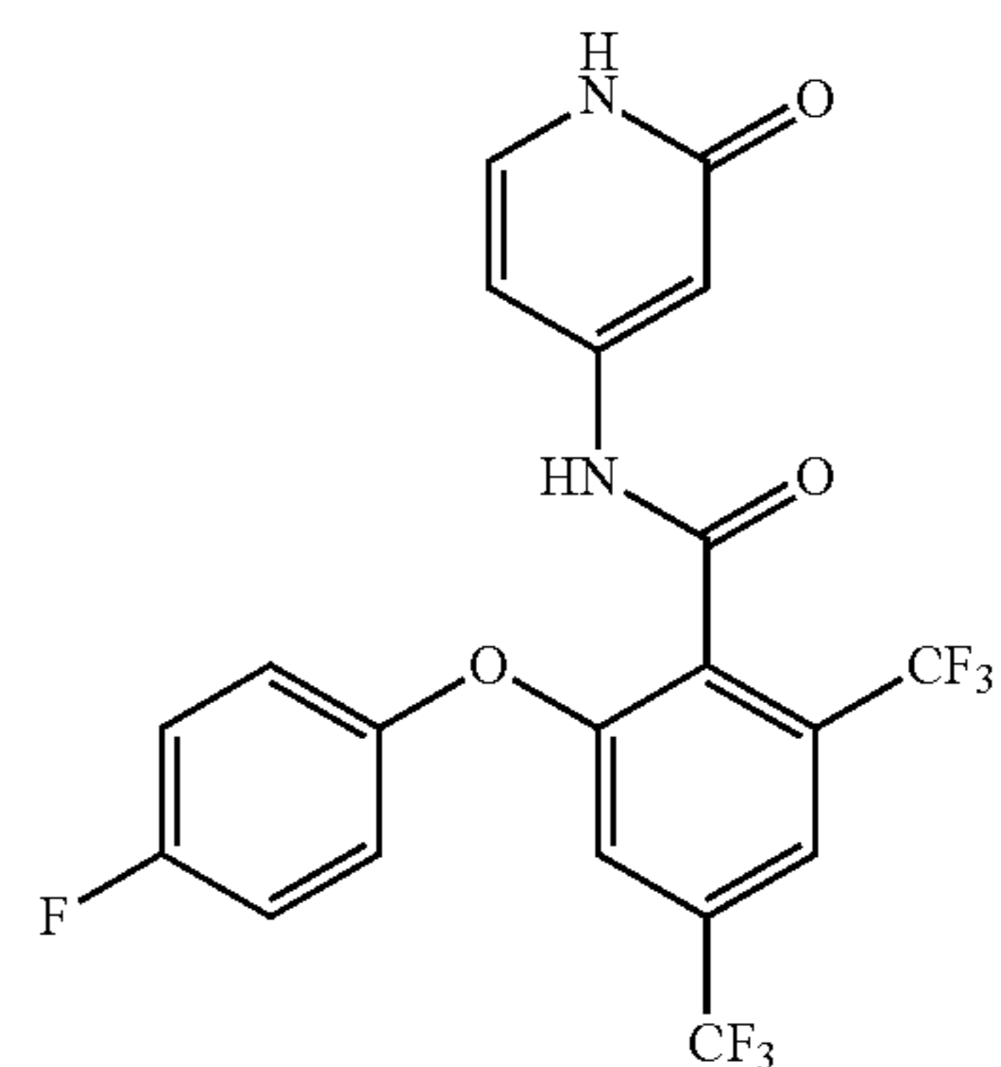
2-(4-fluorophenoxy)-N-(2-oxo-1,2-dihydropyridin-4-yl)-4,6-bis(trifluoromethyl)benzamide
