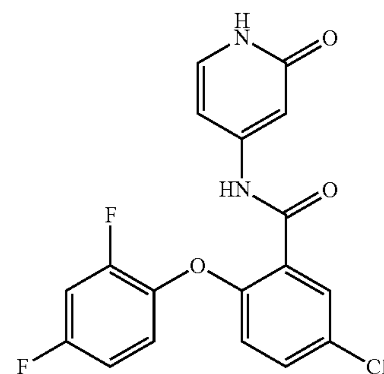
5-chloro-2-(2,4-difluorophenoxy)-N-(2-oxo-1,2-dihydropyridin-4-yl)benzamide
