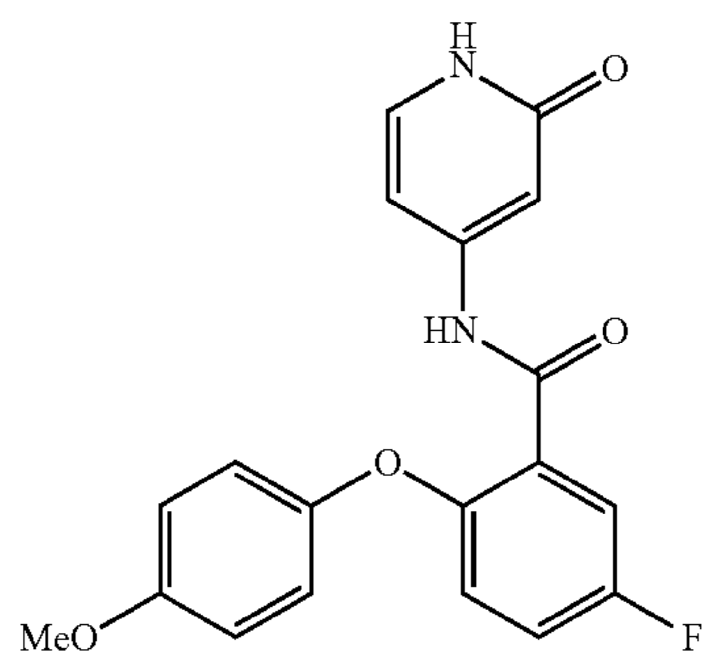
5-fluoro-2-(4-methoxyphenoxy)-N-(2-oxo-1,2-dihydropyridin-4-yl)benzamide
