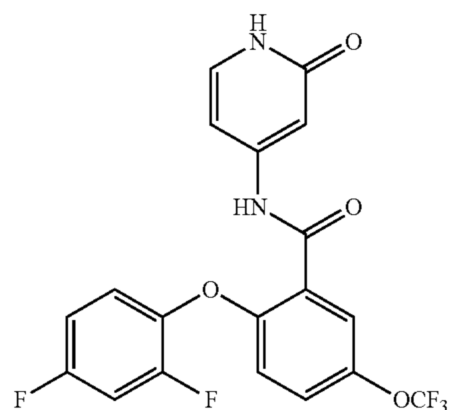
2-(2,4-difluorophenoxy)-N-(2-oxo-1,2-dihydropyridin-4-yl)-5-(trifluoromethoxy)benzamide
