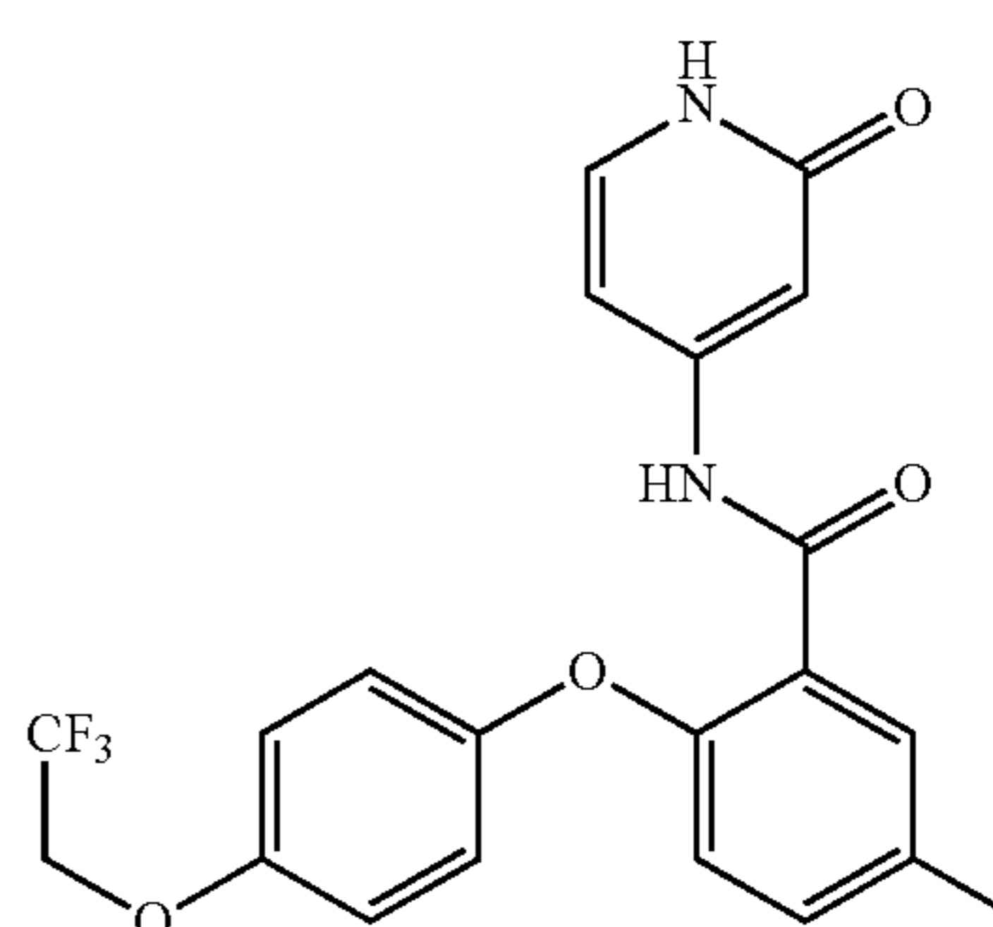
5-fluoro-N-(2-oxo-1,2-dihydropyridin-4-yl)-2-(4-(2,2,2-trifluoroethoxy)phenoxy)benzamide
