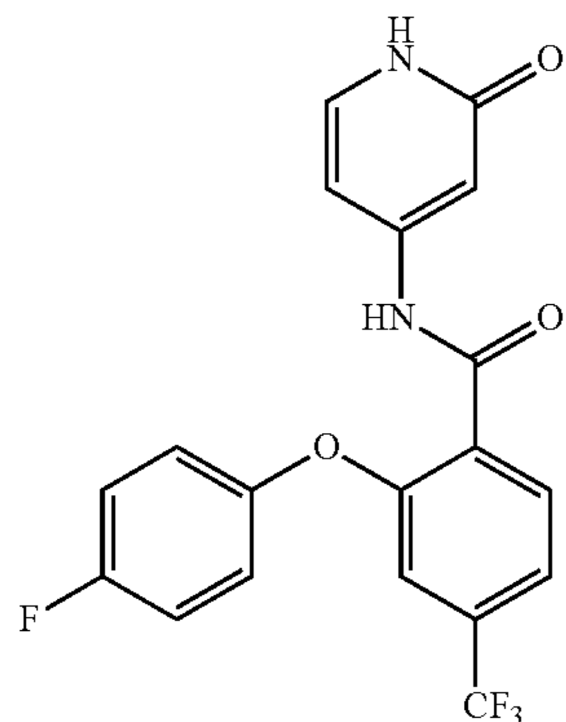
2-(4-fluorophenoxy)-N-(2-oxo-1,2-dihydropyridin-4-yl)-4-(trifluoromethyl)benzamide
