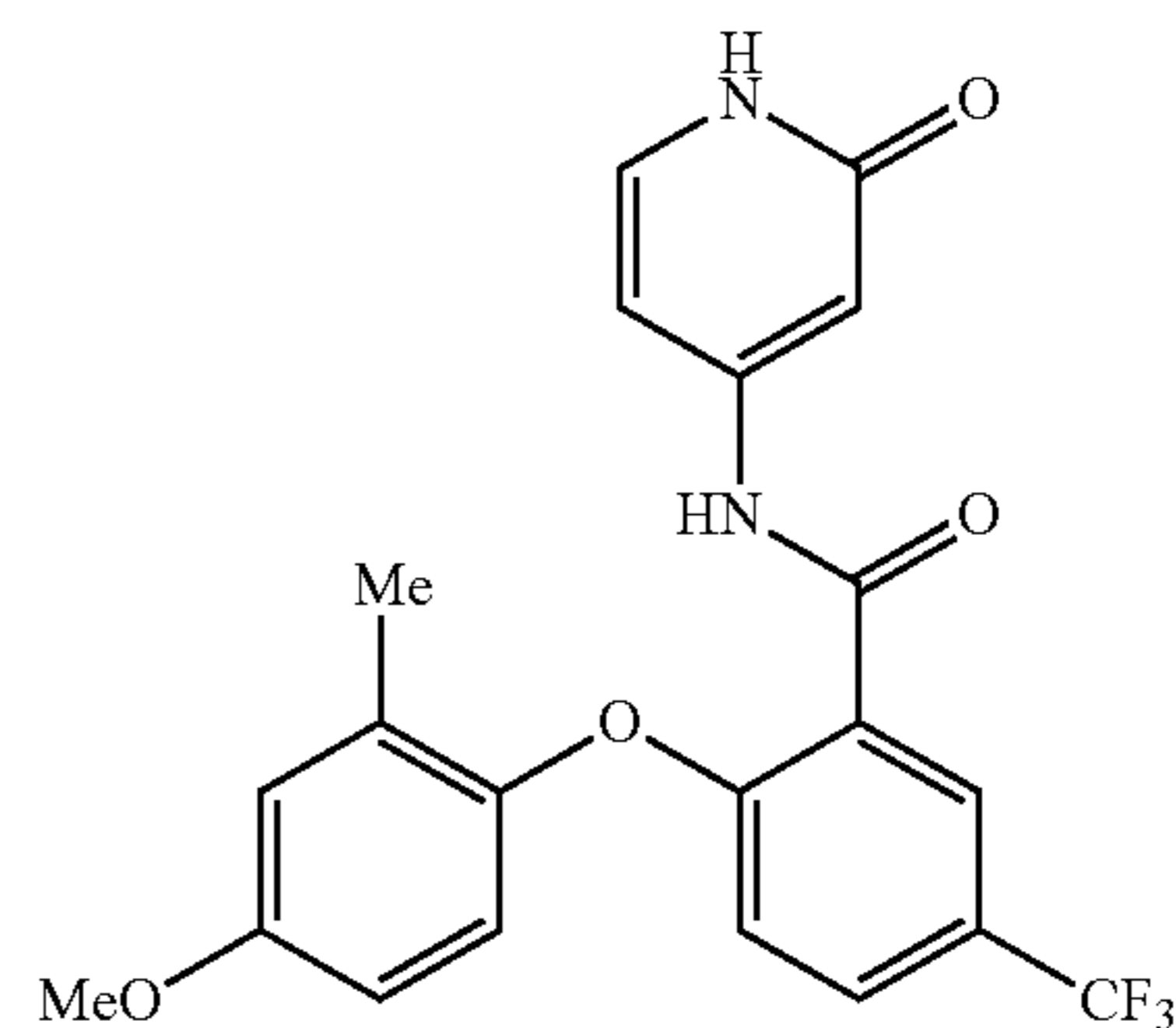
2-(4-methoxy-2-methylphenoxy)- N-(2-oxo-1,2-dihydropyridin-4-yl)-5-(trifluoromethyl)benzamide
