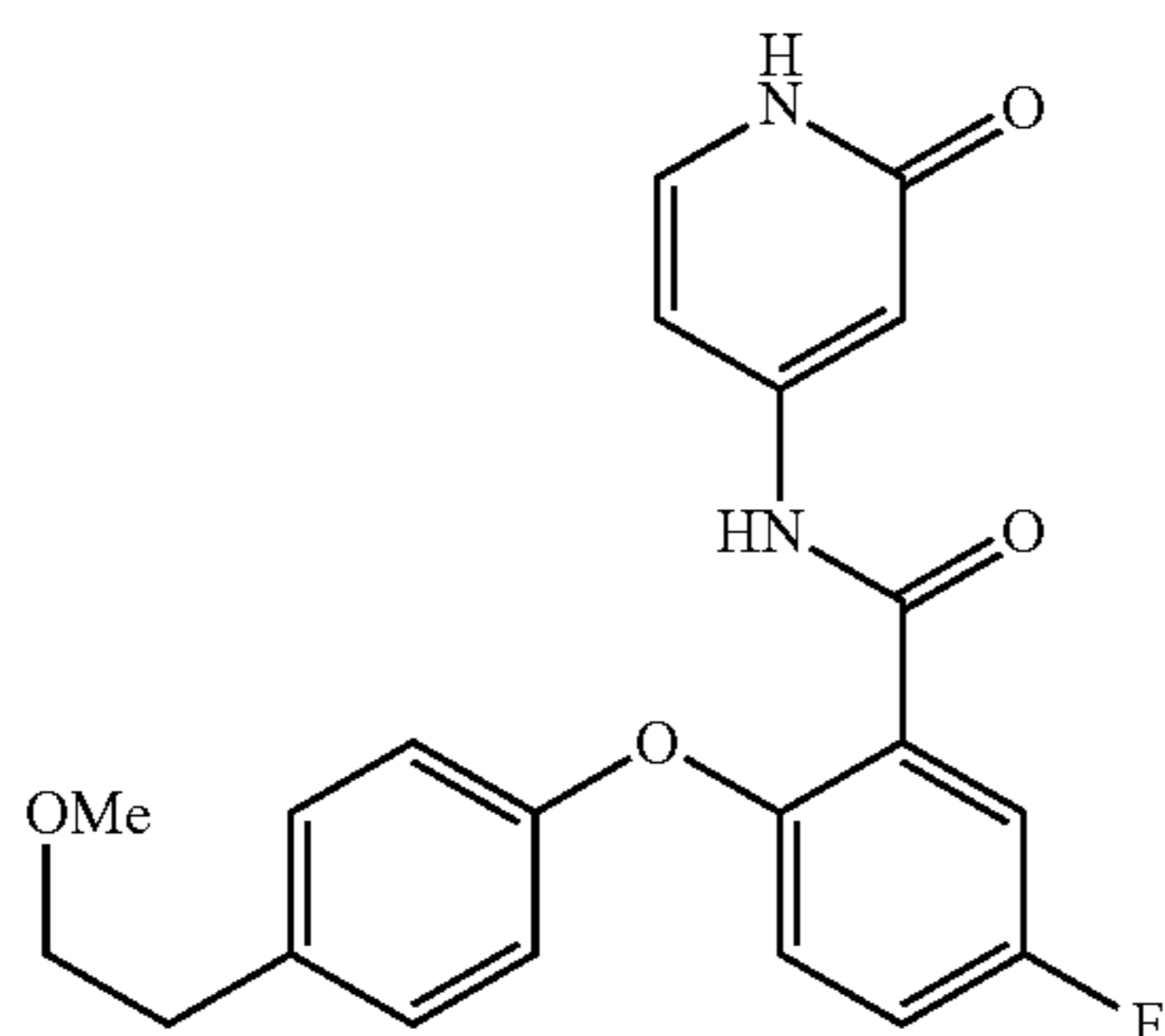
5-fluoro-2-(4-(2-methoxyethyl)phenoxy)-N-(2-oxo-1,2-dihydropyridin-4-yl)benzamide
