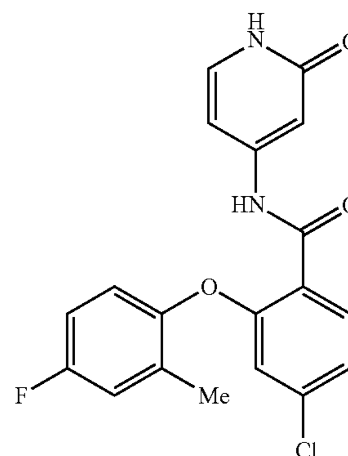
4-chloro-2-(4-fluoro-2-methylphenoxy)-N-(2-oxo-1,2-dihydropyridin-4-yl)benzamide.
