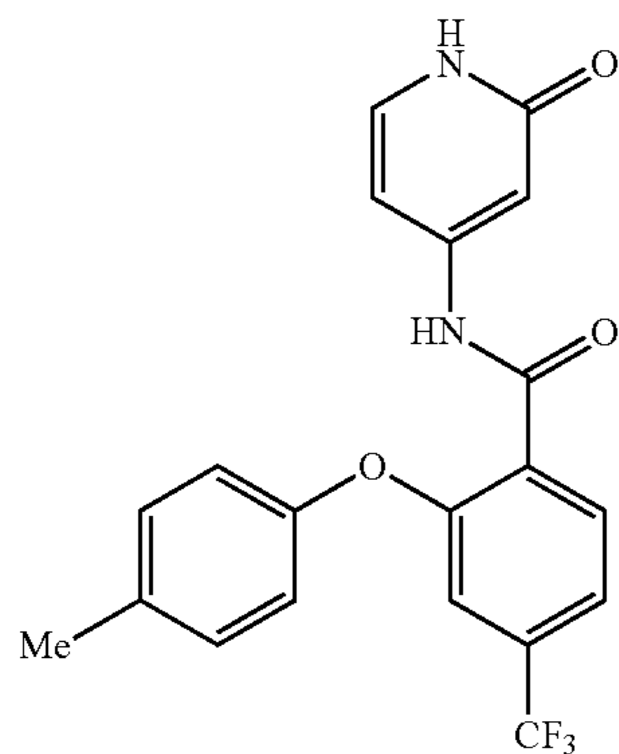
N-(2-oxo-1,2-dihydropyridin-4-yl)-2-(p-tolyloxy)-4-(trifluoromethyl)benzamide
