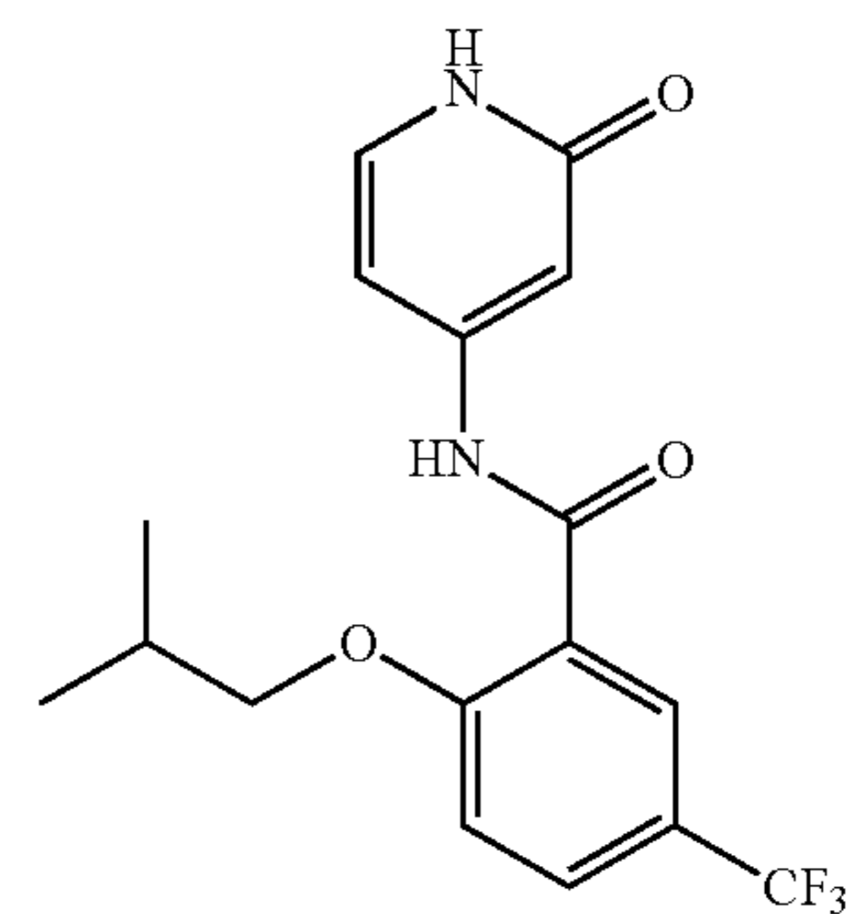
2-isobutoxy-N-(2-oxo-1,2-dihydropyridin-4-yl)-5-(trifluoromethyl)benzamide
