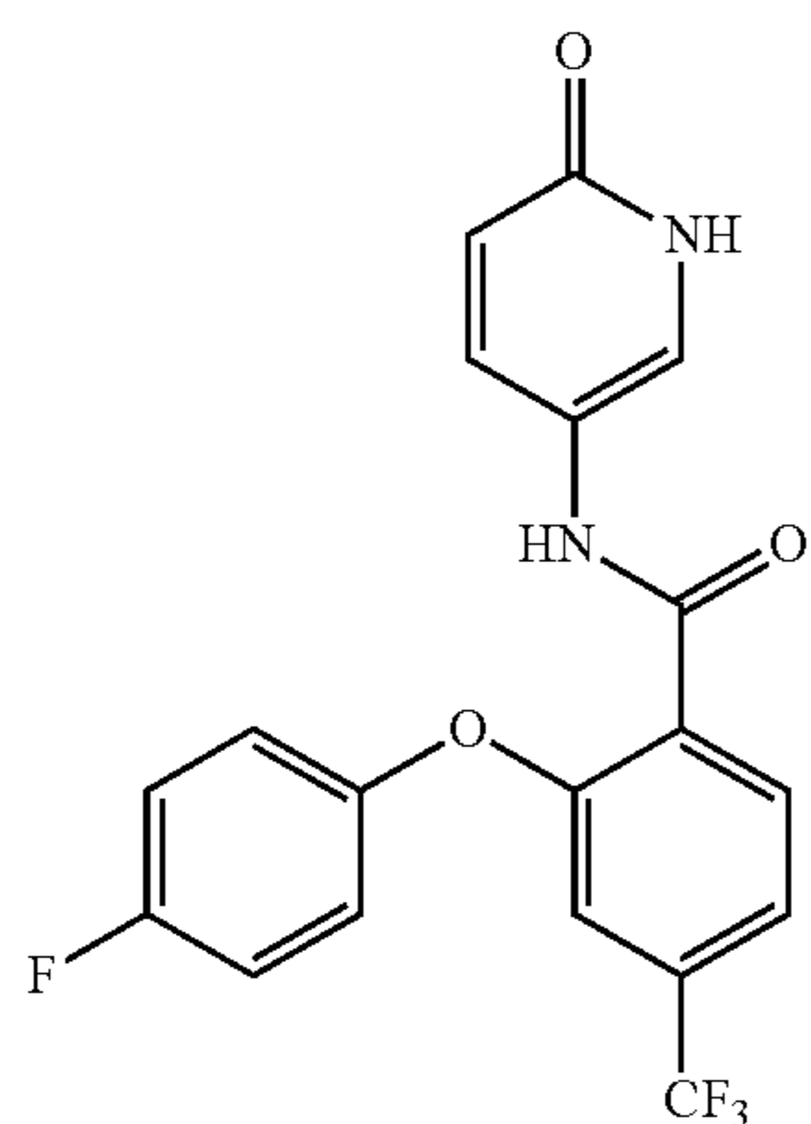
2-(4-fluorophenoxy)-N-(6-oxo-1,6-dihydropyridin-3-yl)-4-(trifluoromethyl)benzamide
