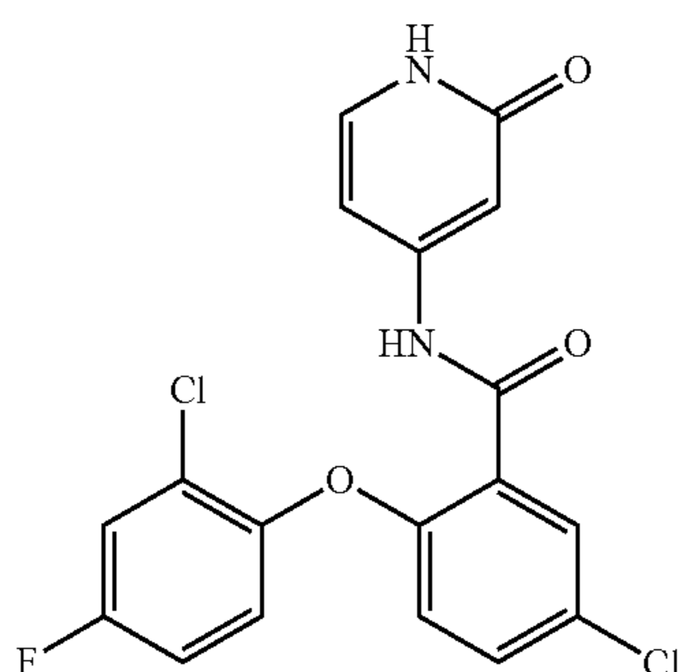
5-chloro-2-(2-chloro-4-fluorophenoxy)-N-(2-oxo-1,2-dihydropyridin-4-yl)benzamide
