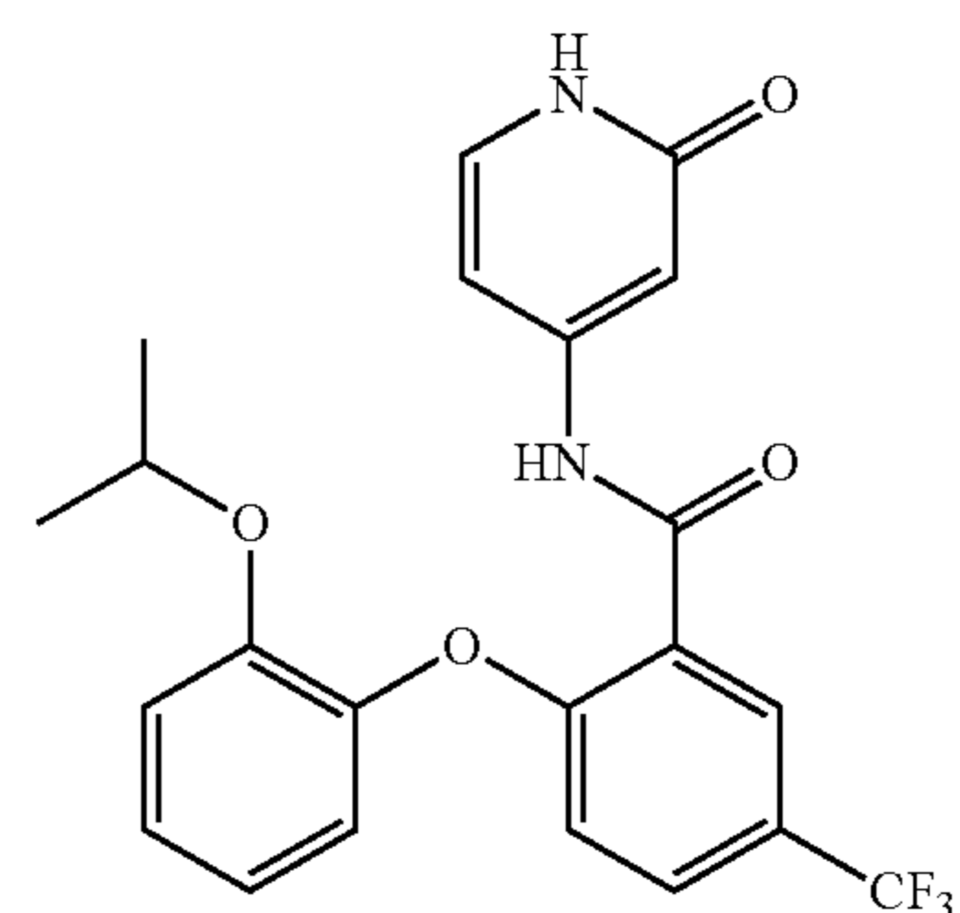
2-(2-isopropoxyphenoxy)-N-(2-oxo-1,2-dihydropyridin-4-yl)-5-(trifluoromethyl)benzamide
