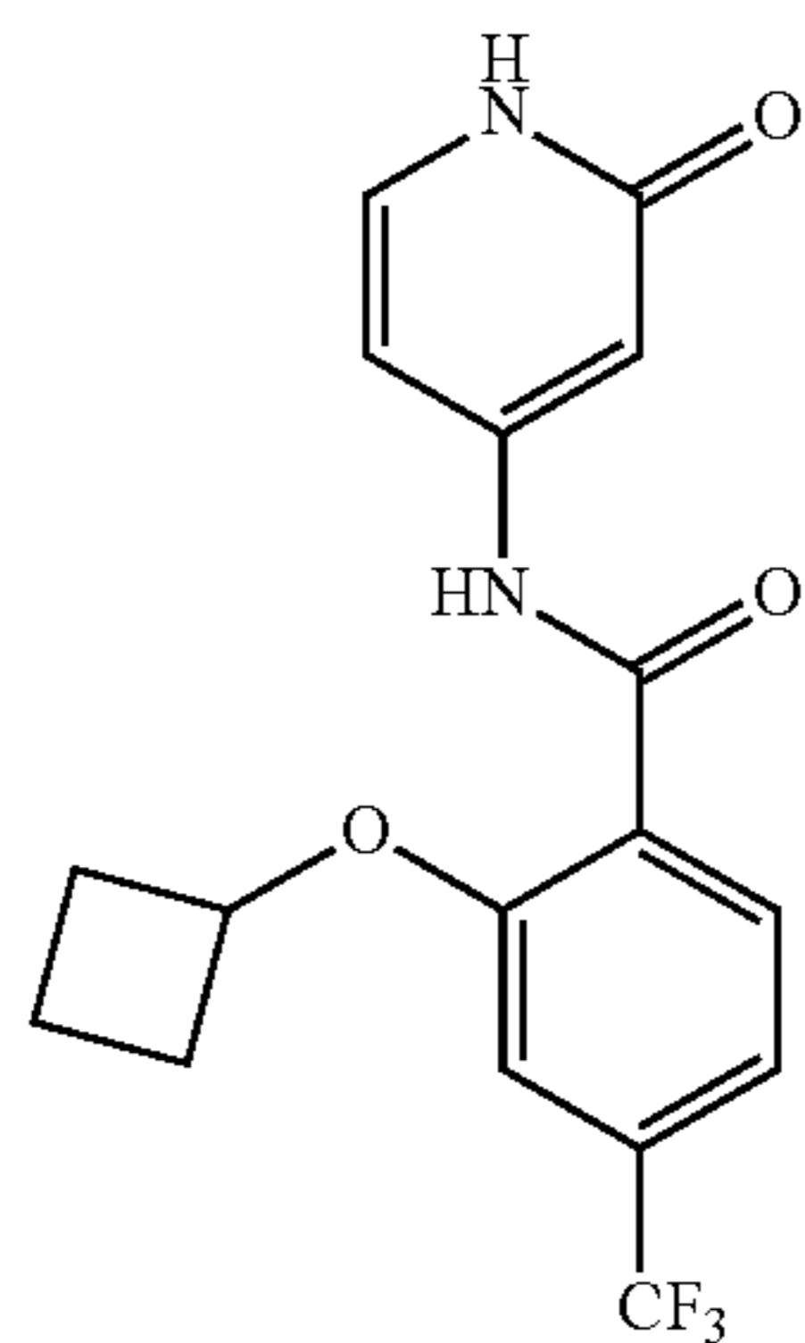
2-cyclobutoxy-N-(2-oxo-1,2-dihydropyridin-4-yl)-4-(trifluoromethyl)benzamide
