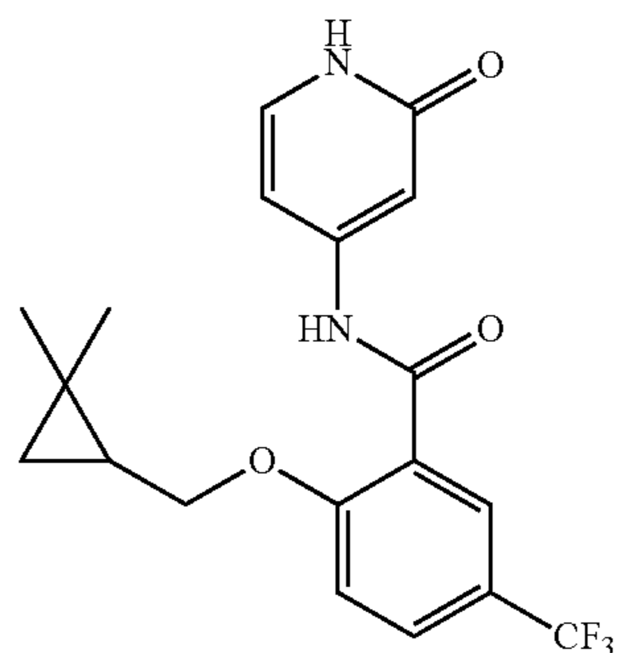
2-((2,2-dimethylcyclopropyl)methoxy)-N-(2-oxo-1,2-dihydropyridin-4-yl)-5-(trifluoromethyl)benzamide
