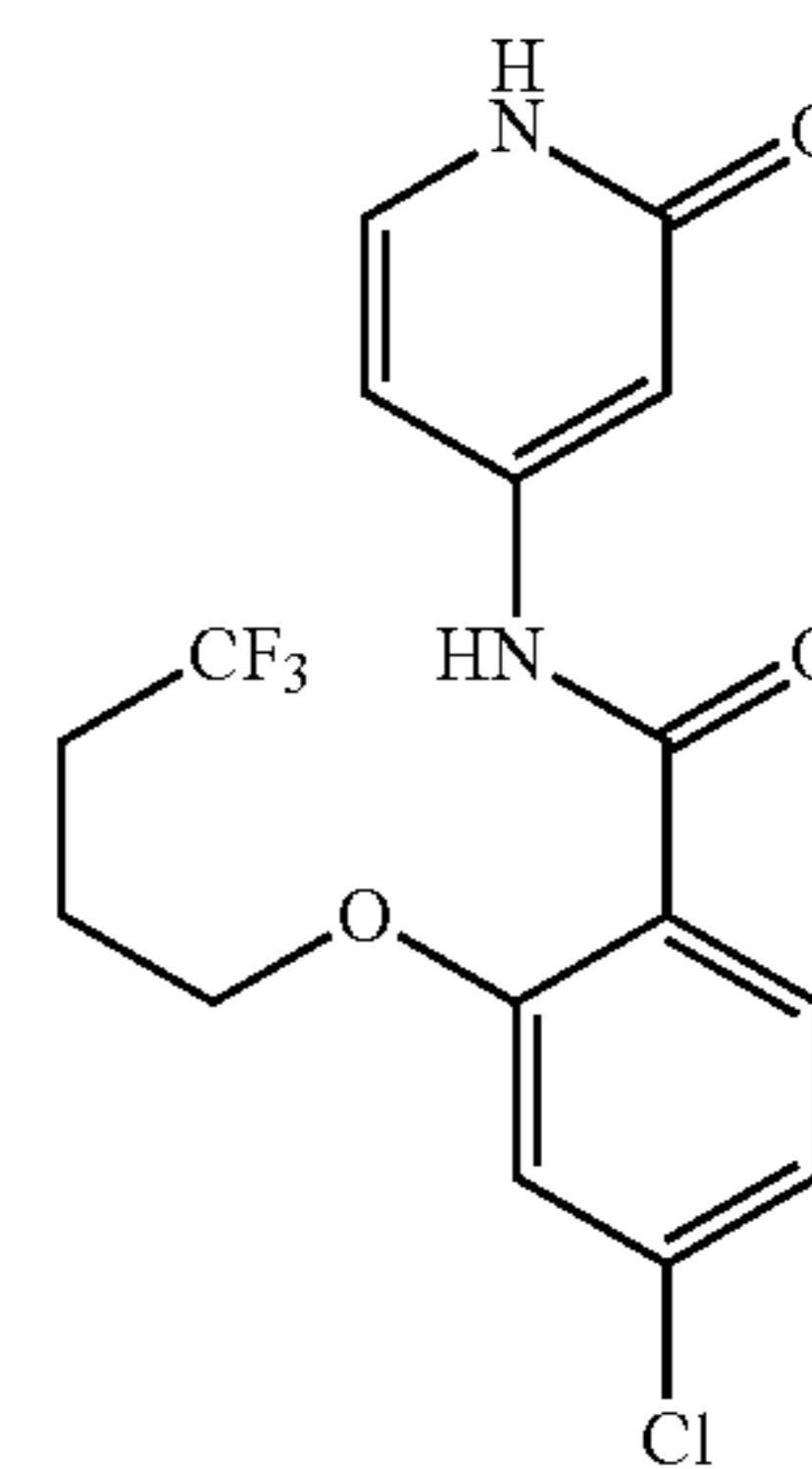
4-chloro-N-(2-oxo-1,2-dihydropyridin-4-yl)-2-(4,4,4-trifluorobutoxy)benzamide
