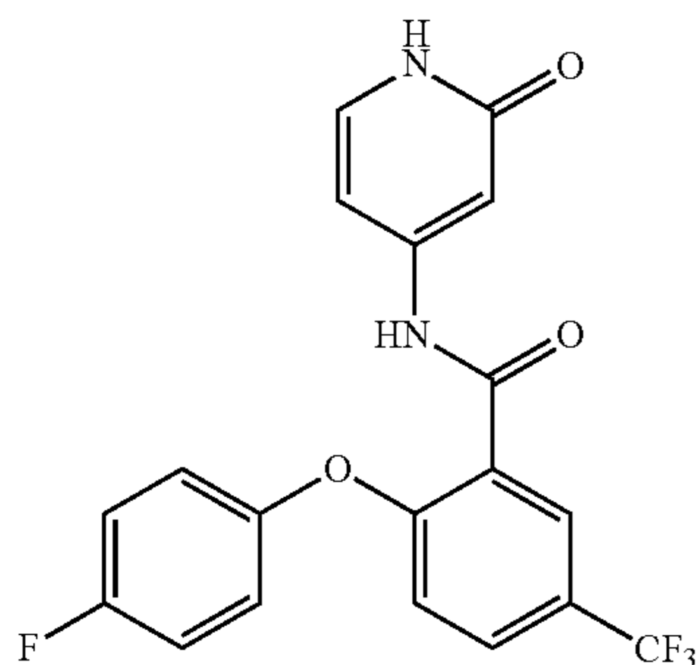
2-(4-fluorophenoxy)-N-(2-oxo-1,2-dihydropyridin-4-yl)-5-(trifluoromethyl)benzamide.
