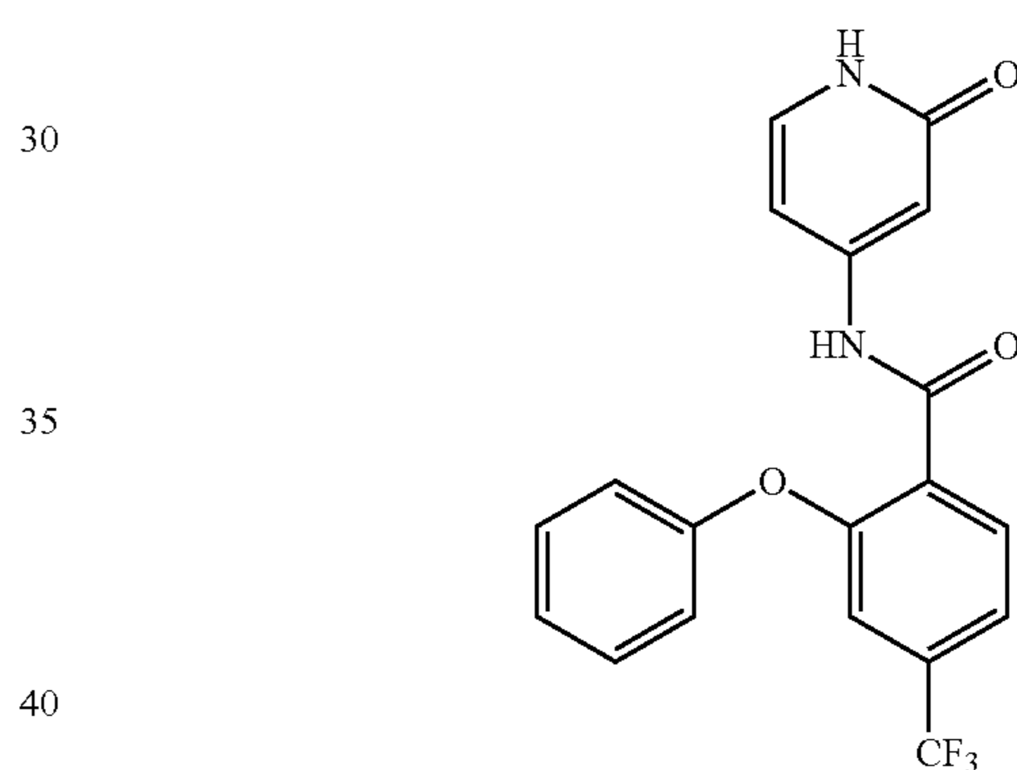
N-(2-oxo-1,2-dihydropyridin-4-yl)-2-phenoxy-4-(trifluoromethyl)benzamide
