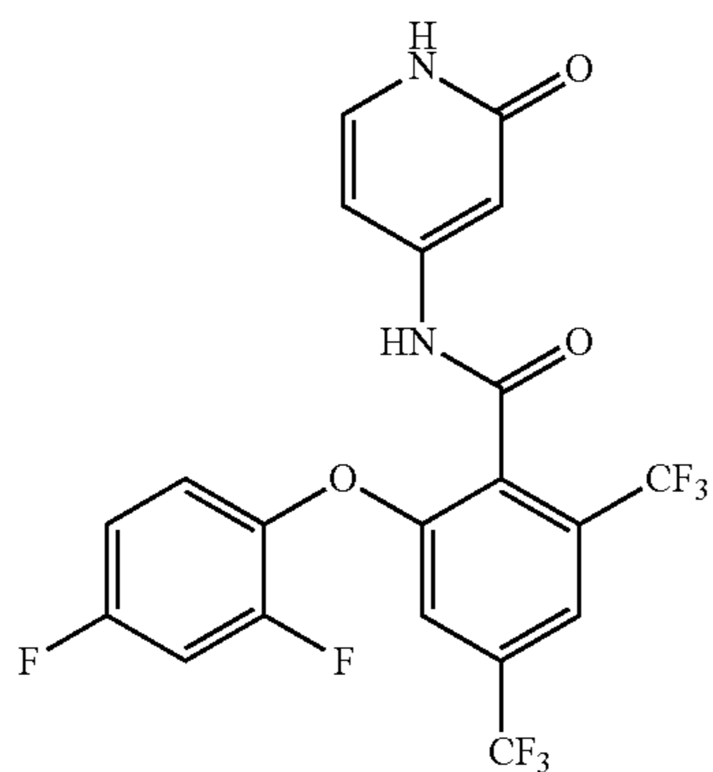
2-(2,4-difluorophenoxy)-N-(2-oxo-1,2-dihydropyridin-4-yl)-4,6-bis(trifluoromethyl)benzamide
