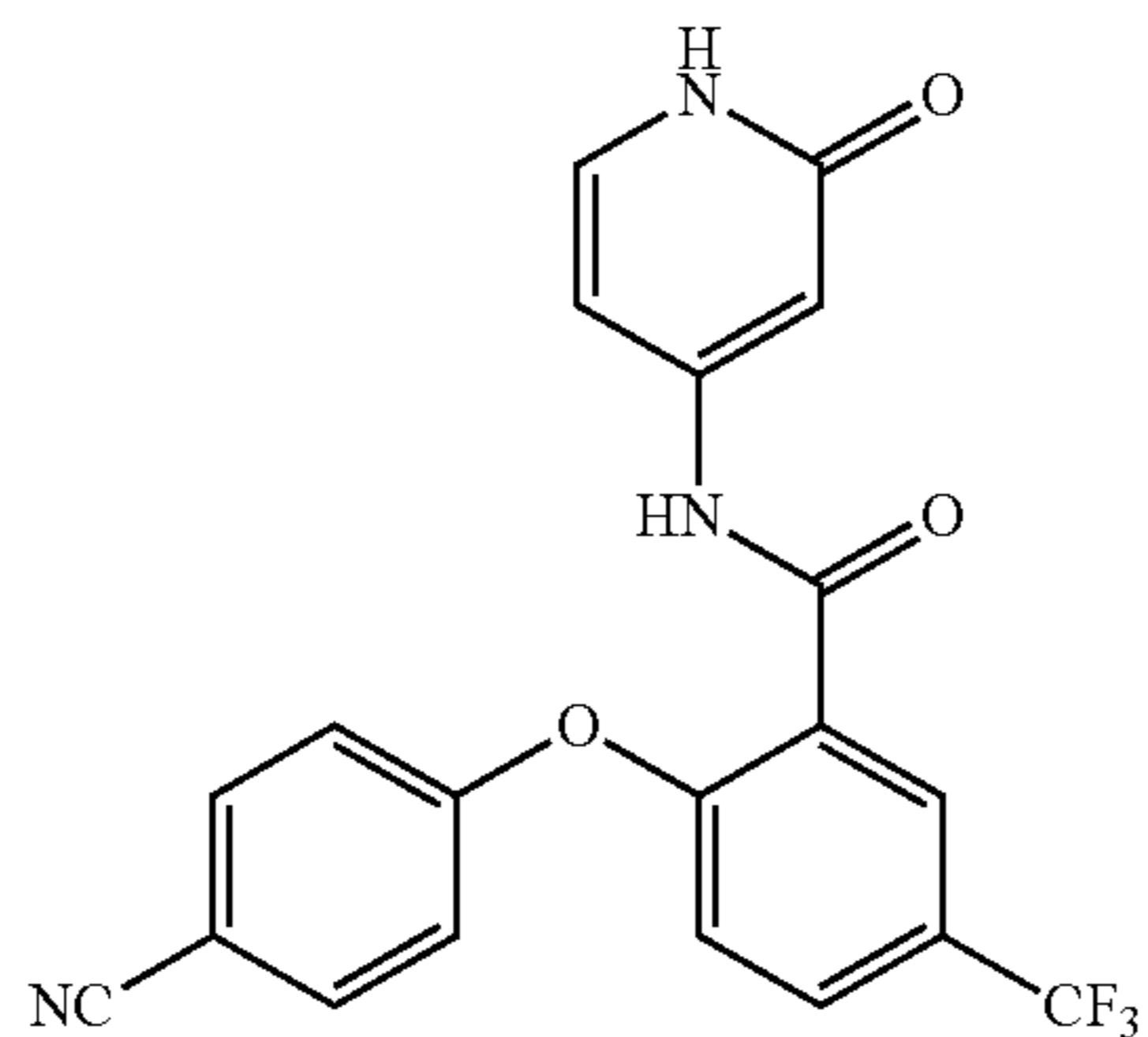
2-(4-cyanophenoxy)-N-(2-oxo-1,2-dihydropyridin-4-yl)-5-(trifluoromethyl)benzamide
