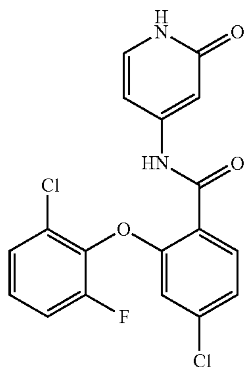
4-chloro-2-(2-chloro-6-fluorophenoxy)-N-(2-oxo-1,2-dihydropyridin-4-yl)benzamide
