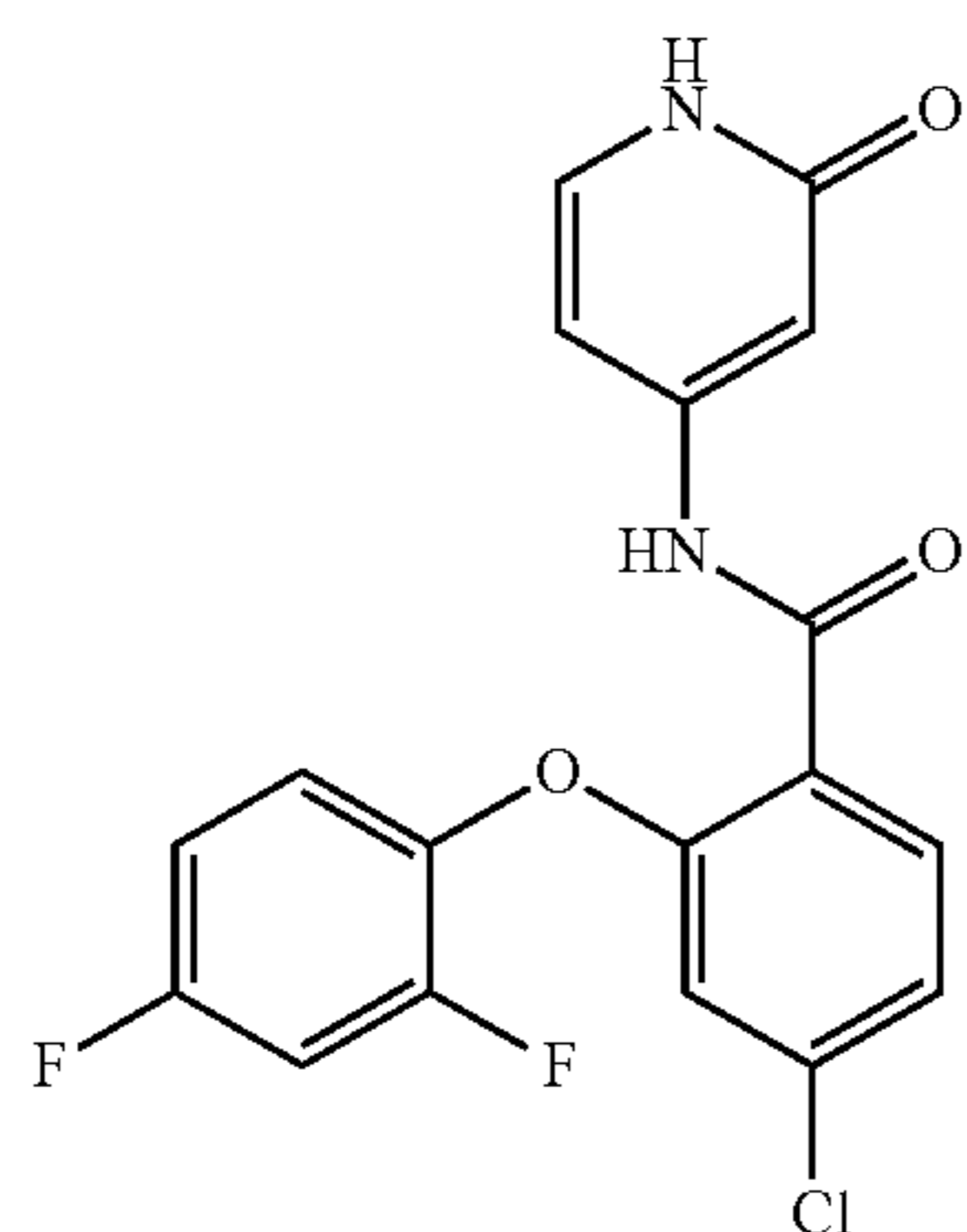
4-chloro-2-(2,4-difluorophenoxy)-N-(2-oxo-1,2-dihydropyridin-4-yl)benzamide
