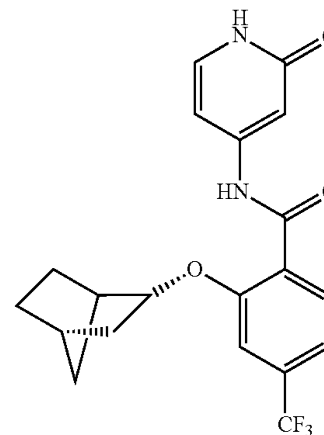
2-((2R)-bicyclo[2.2.1]heptan-2-yloxy)-N-(2-oxo-1,2-dihydropyridin-4-yl)-4-(trifluoromethyl)benzamide
