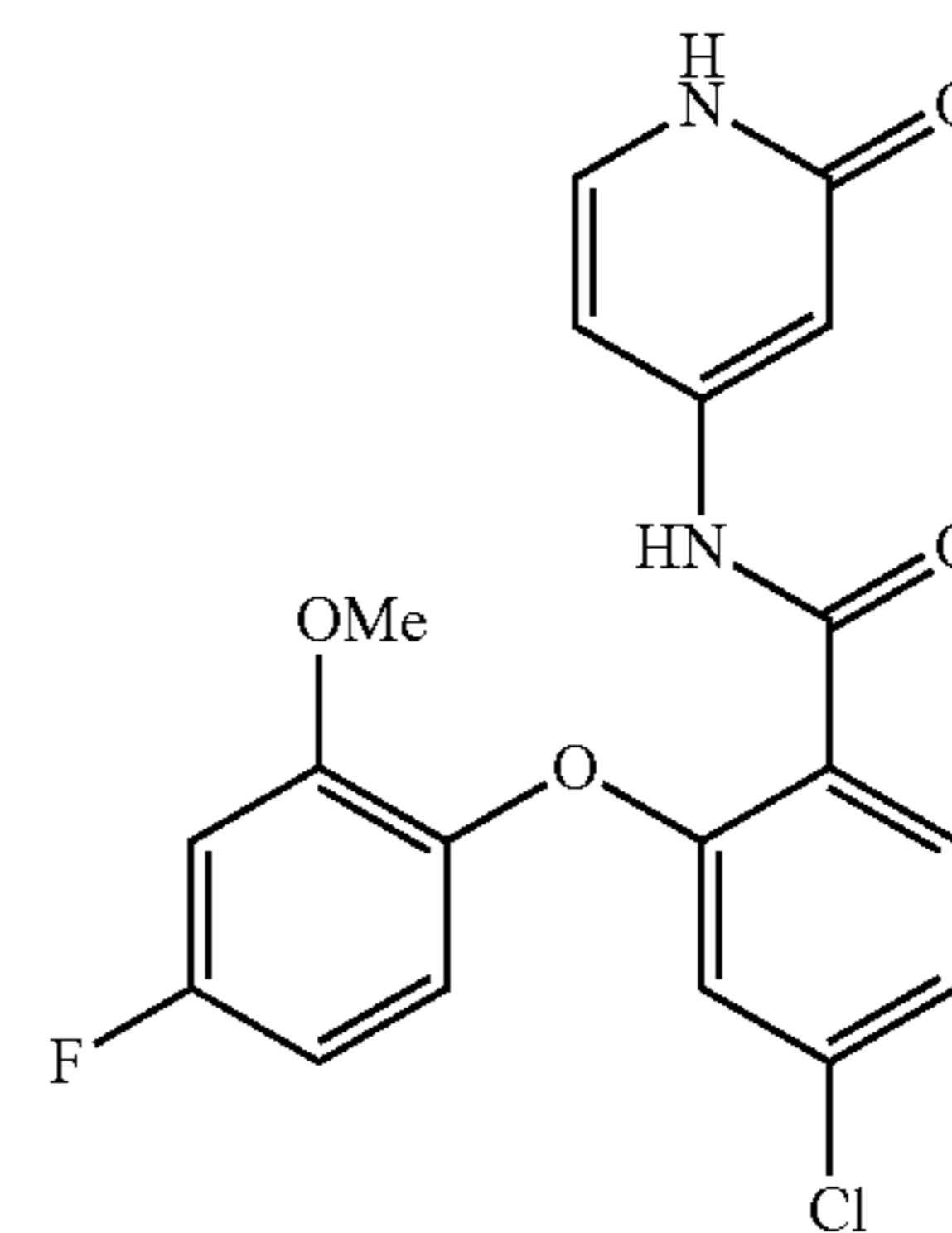
4-chloro-2-(4-fluoro-2-methoxyphenoxy)-N-(2-oxo-1,2-dihydropyridin-4-yl)benzamide
