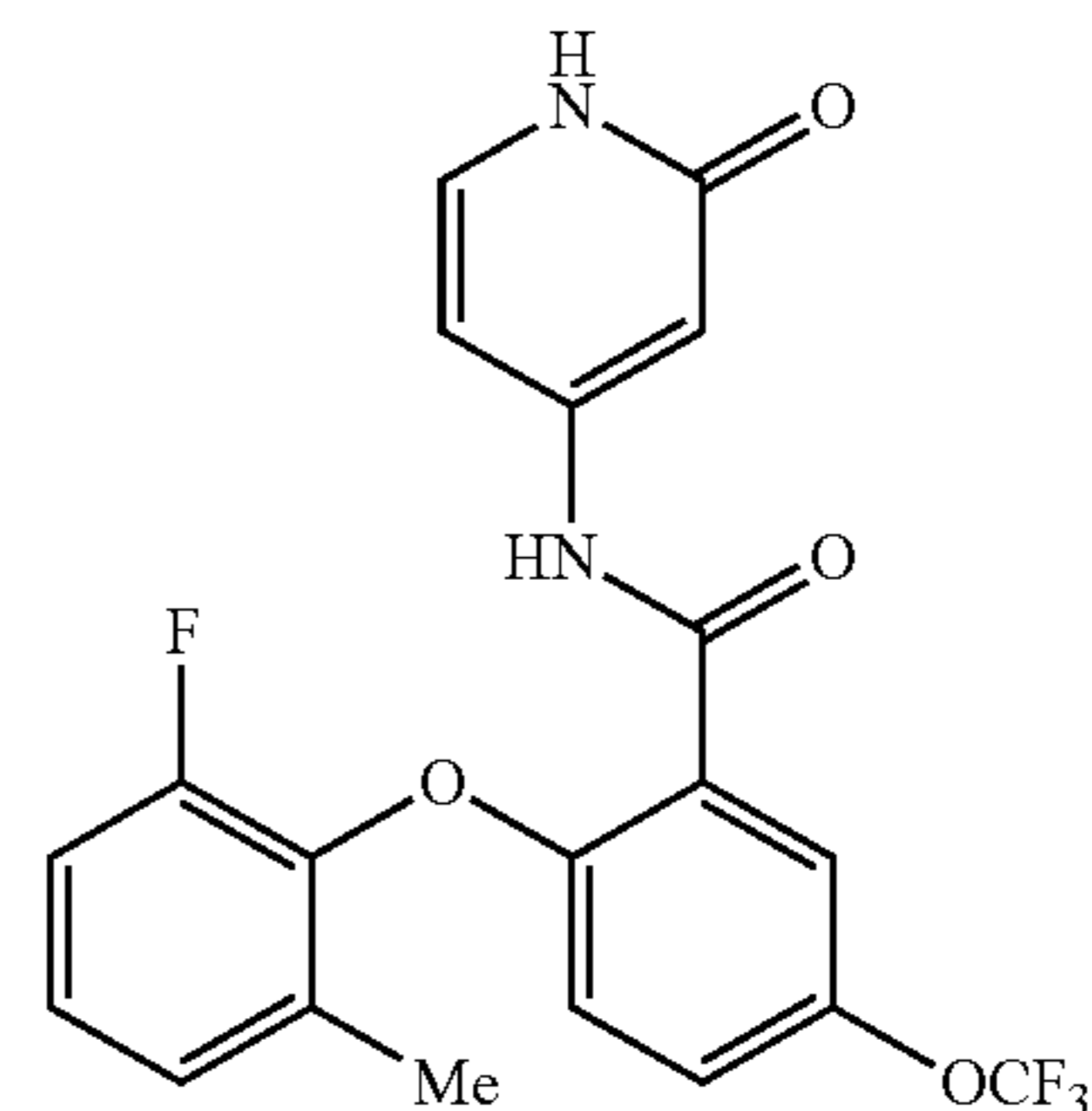
2-(2-fluoro-6-methylphenoxy)-N-(2-oxo-1,2-dihydropyridin-4-yl)-5-(trifluoromethoxy)benzamide
