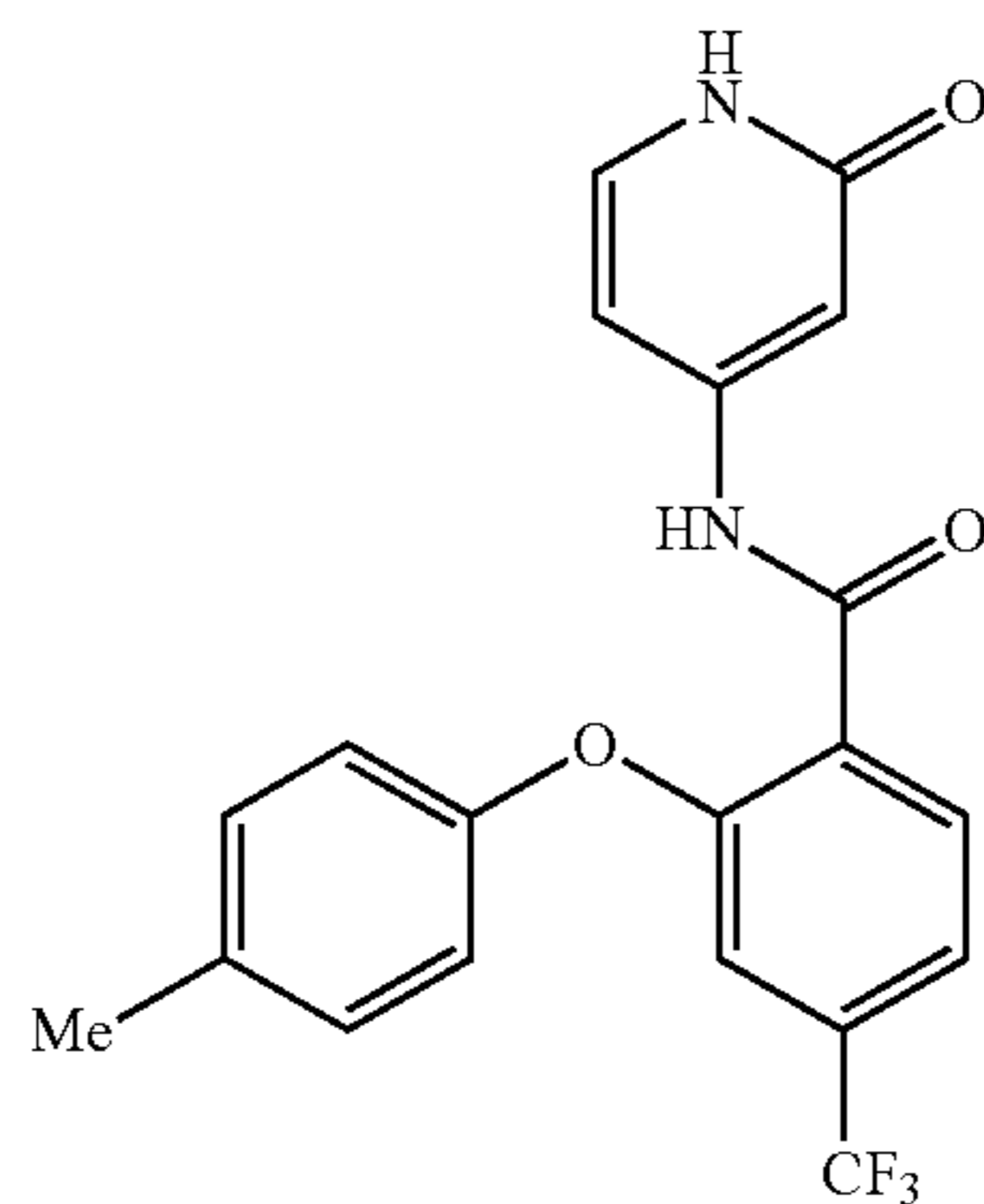
N-(2-oxo-1,2-dihydropyridin-4-yl)-2-(p-tolyloxy)-4-(trifluoromethyl)benzamide
