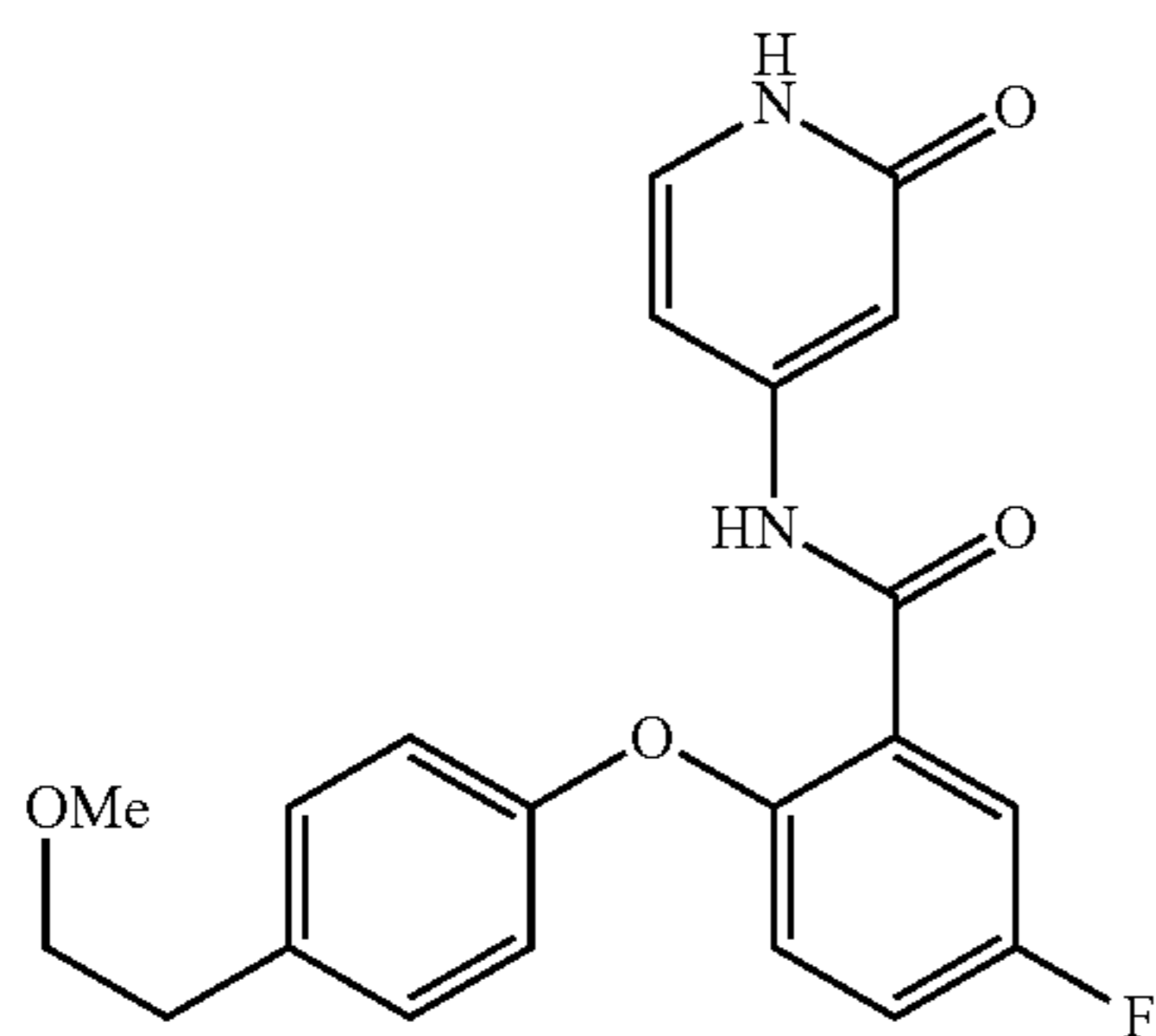
5-fluoro-2-(4-(2-methoxyethyl)phenoxy)-N-(2-oxo-1,2-dihydropyridin-4-yl)benzamide
