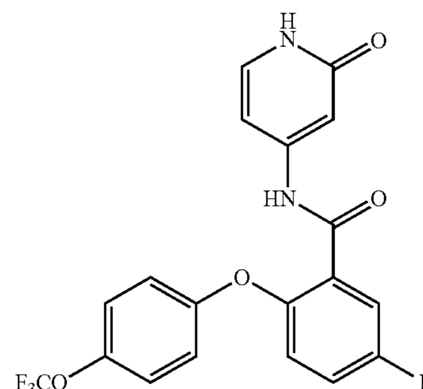
5-fluoro-N-(2-oxo-1,2-dihydropyridin-4-yl)-2-(4-(trifluoromethoxy)phenoxy)benzamide
