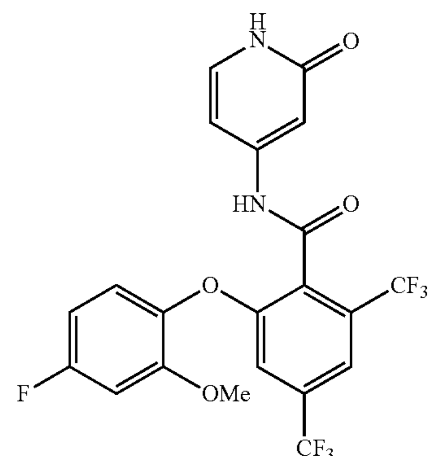
2-(4-fluoro-2-methoxyphenoxy)-N-(2-oxo-1,2-dihydropyridin-4-yl)-4,6-bis(trifluoromethyl)benzamide
