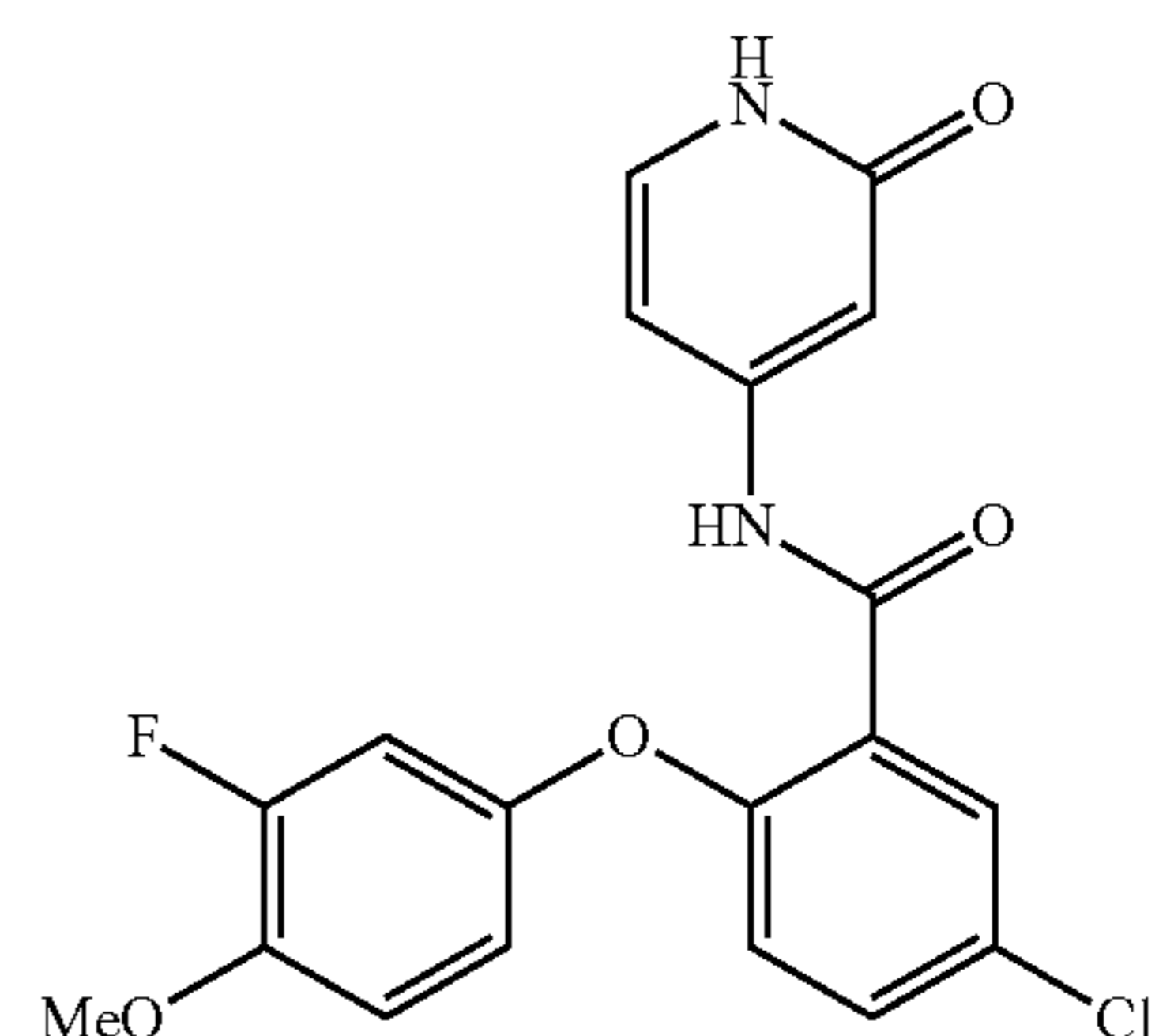
5-chloro-2-(3-fluoro-4-methoxyphenoxy)-N-(2-oxo-1,2-dihydropyridin-4-yl)benzamide
