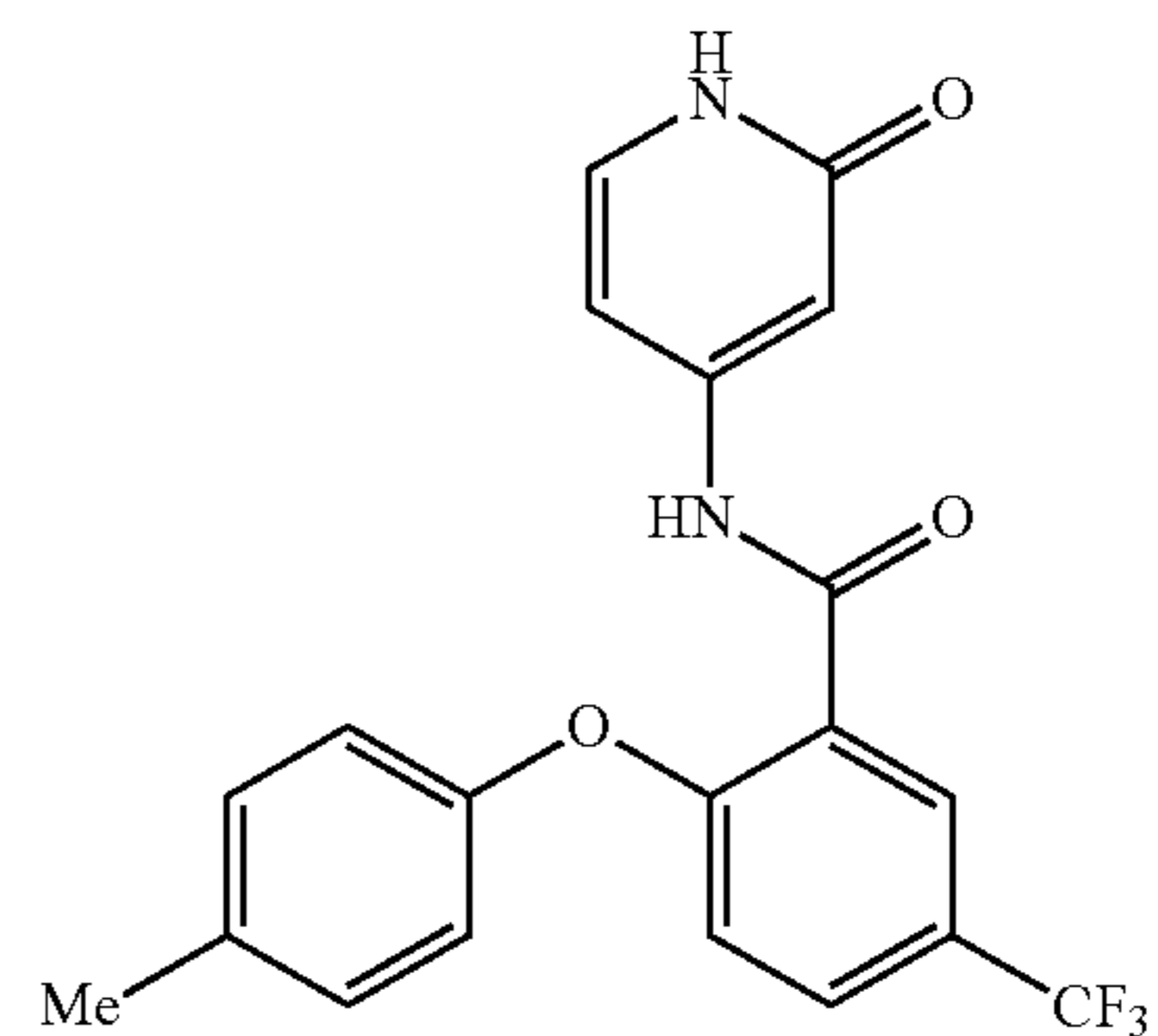
N-(2-oxo-1,2-dihydropyridin-4-yl)-2-(p-tolyloxy)-5-(trifluoromethyl)benzamide
