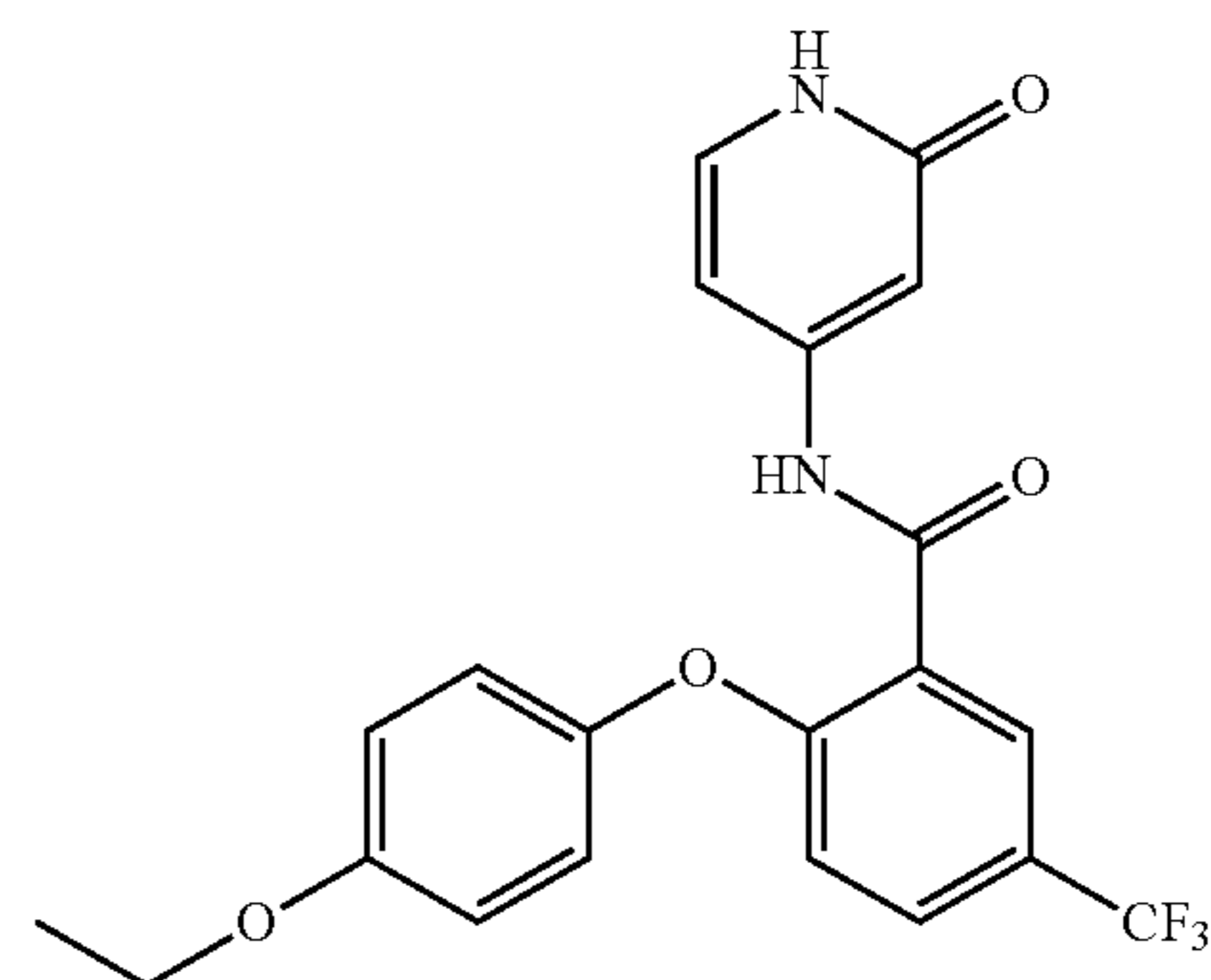
2-(4-ethoxyphenoxy)-N-(2-oxo-1,2-dihydropyridin-4-yl)-5-(trifluoromethyl)benzamide
