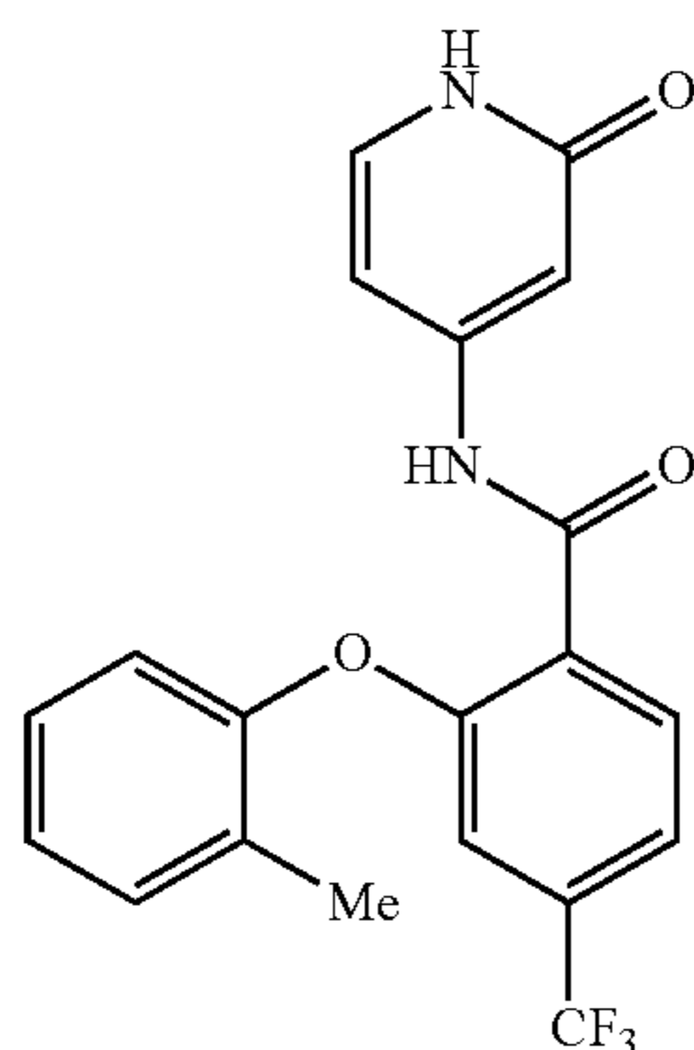
N-(2-oxo-1,2-dihydropyridin-4-yl)-2-(o-tolyloxy)-4-(trifluoromethyl)benzamide
