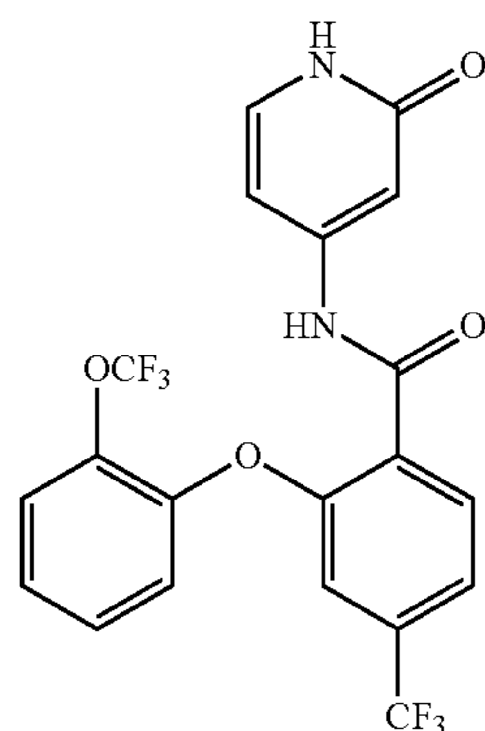
N-(2-oxo-1,2-dihydropyridin-4-yl)-2-(2-(trifluoromethoxy)phenoxy)-4-(trifluoromethyl)benzamide
