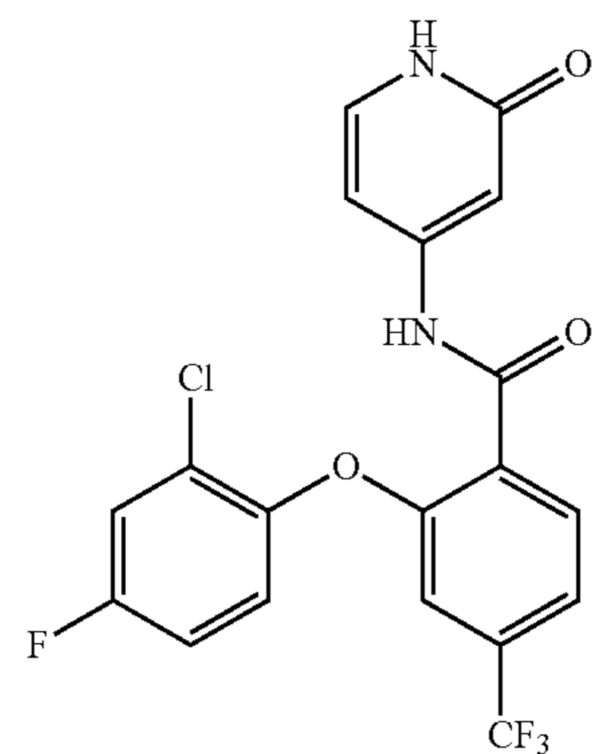
2-(2-chloro-4-fluorophenoxy)-N-(2-oxo-1,2-dihydropyridin-4-yl)-4-(trifluoromethyl)benzamide
