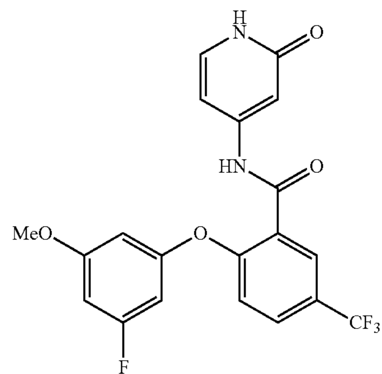
2-(3-fluoro-5-methoxyphenoxy)-N-(2-oxo-1,2-dihydropyridin-4-yl)-5-(trifluoromethyl)benzamide
