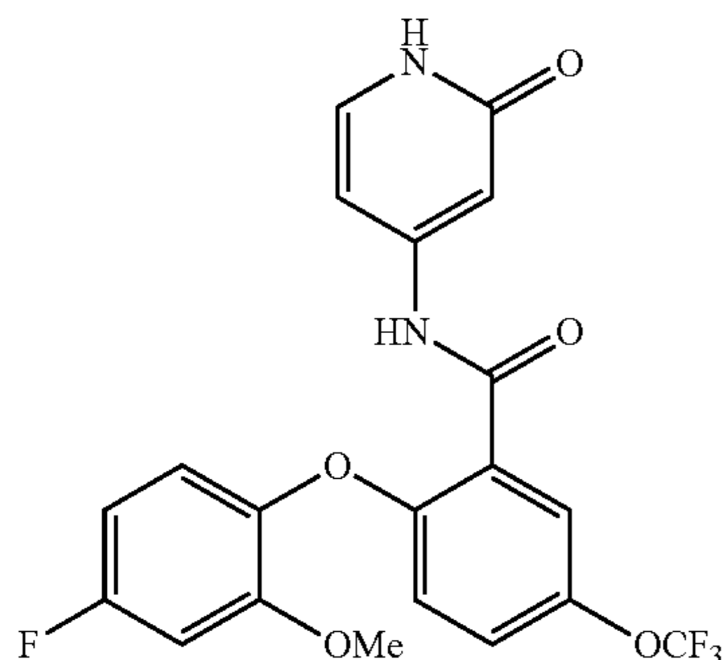
2-(4-fluoro-2-methoxyphenoxy)-N-(2-oxo-1,2-dihydropyridin-4-yl)-5-(trifluoromethoxy)benzamide
