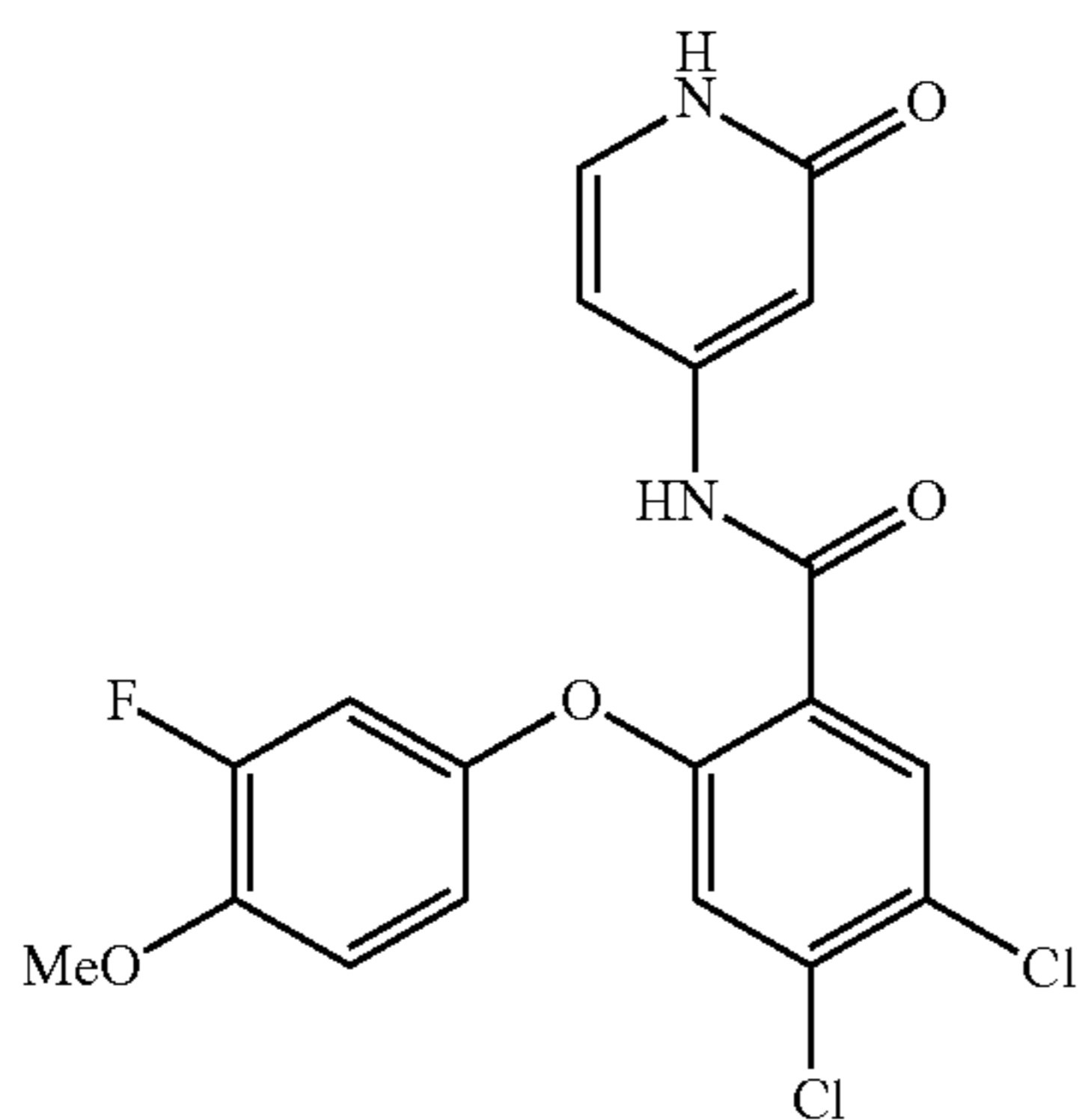
4,5-dichloro-2-(3-fluoro-4-methoxyphenoxy)-N-(2-oxo-1,2-dihydropyridin-4-yl)benzamide
