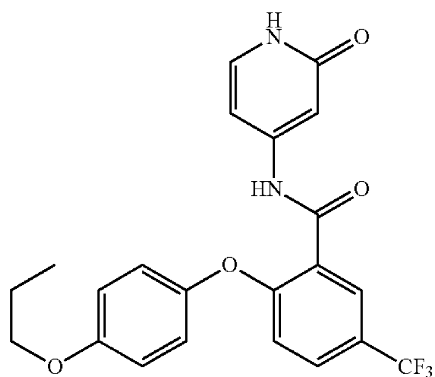
N-(2-oxo-1,2-dihydropyridin-4-yl)-2-(4-propoxyphenoxy)-5-(trifluoromethyl)benzamide
