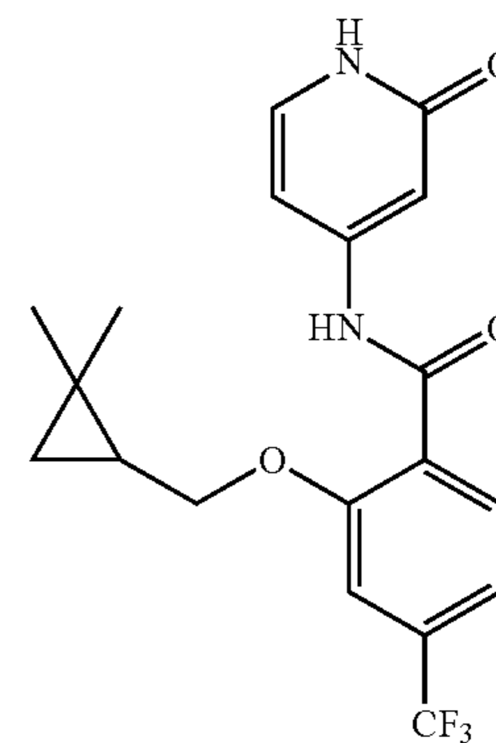
2-((2,2-dimethylcyclopropyl)methoxy)-N-(2-oxo-1,2-dihydropyridin-4-yl)-4-(trifluoromethyl)benzamide
