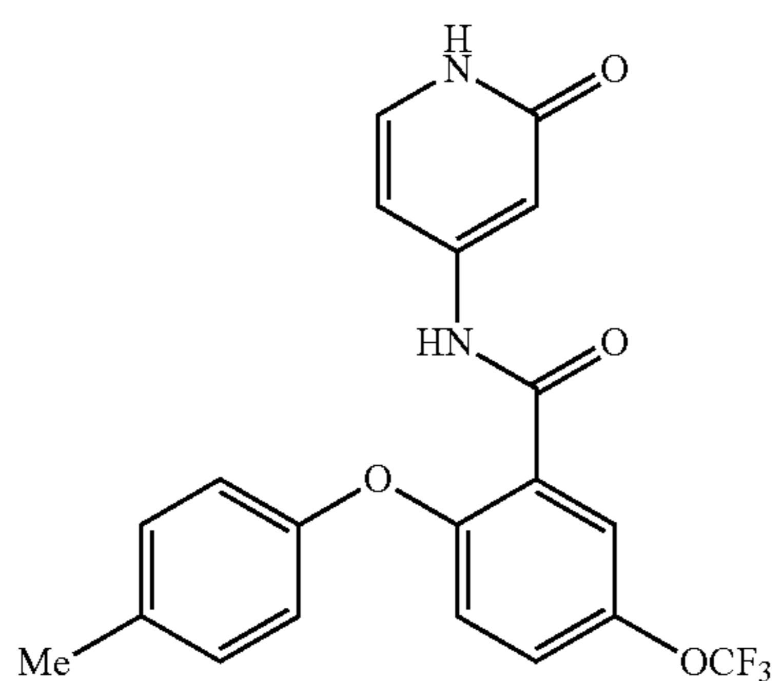
N-(2-oxo-1,2-dihydropyridin-4-yl)-2-(p-tolyloxy)-5-(trifluoromethoxy)benzamide
