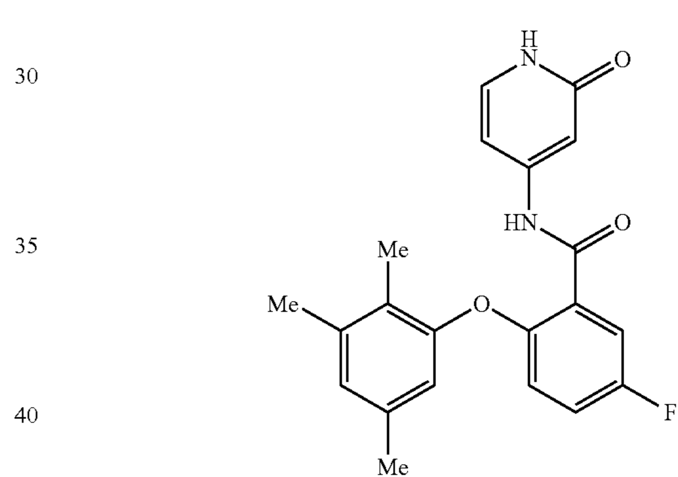
5-fluoro-N-(2-oxo-1,2-dihydropyridin-4-yl)-2-(2,3,5-trimethylphenoxy)benzamide
