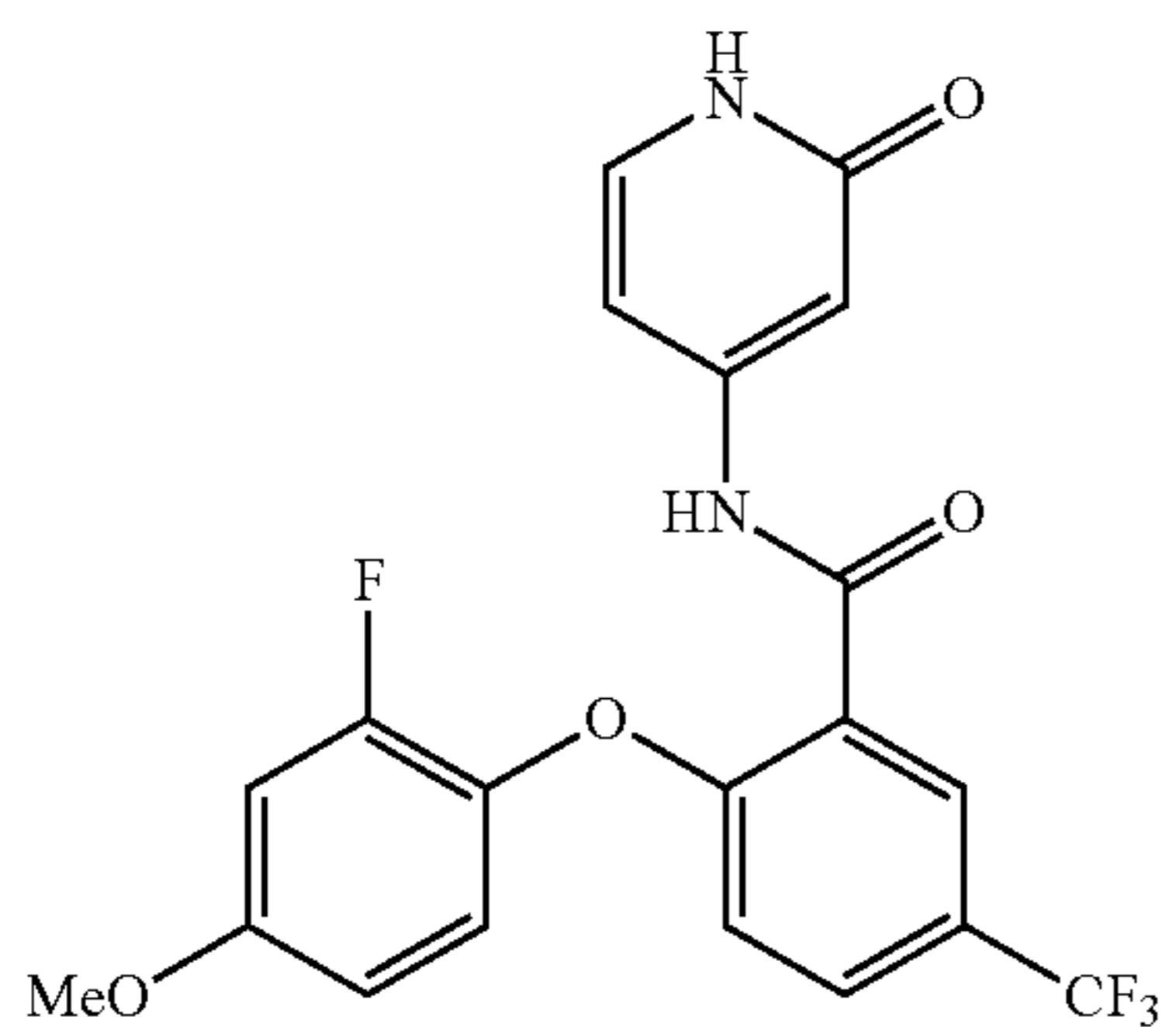
2-(2-fluoro-4-methoxyphenoxy)-N-(2-oxo-1,2-dihydropyridin-4-yl)-5-(trifluoromethyl)benzamide
