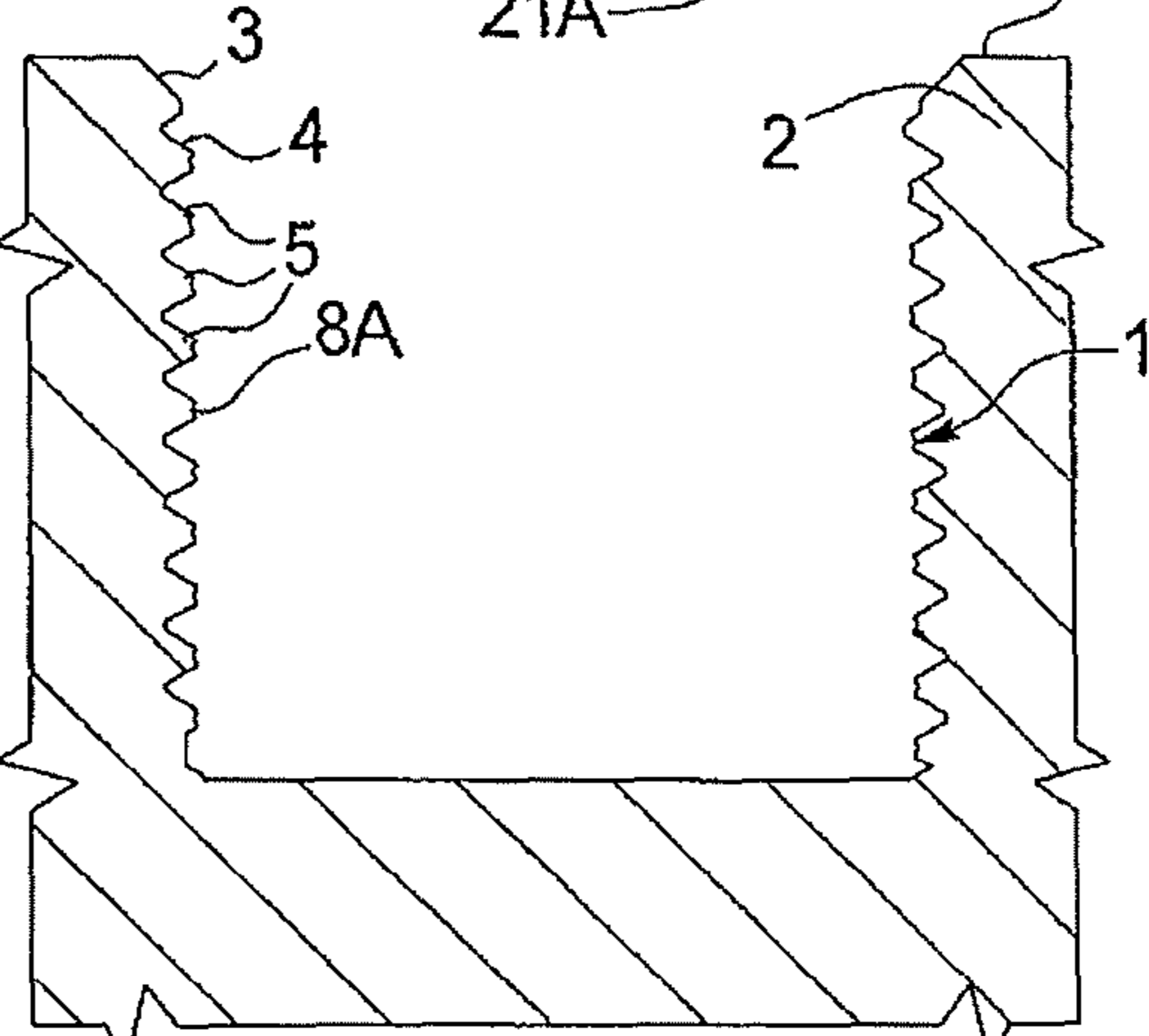
FIG. 2C (PRIOR ART)
