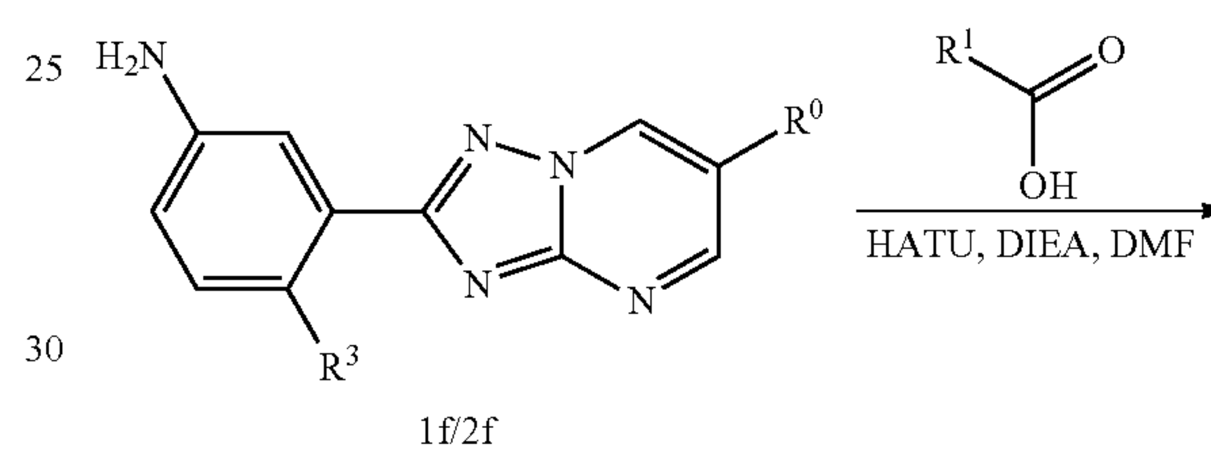
Scheme 3. Coupling of —C(O)—R¹ where R¹ is C 5-6 heteroaryl or C 3-6 cycloalkyl to the phenyl-triazolopyrimidine
