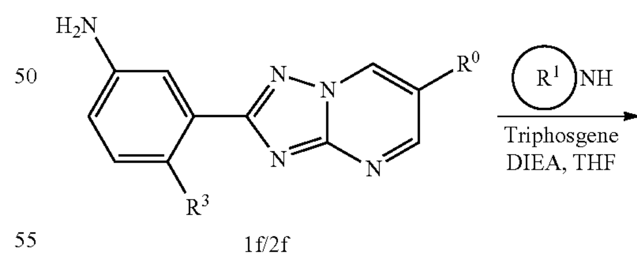
Scheme 4. Coupling of —C(O)—R¹ where R¹ is and N-linked C 4-6 heterocycloalkyl to the phenyl-triazolopyrimidine
