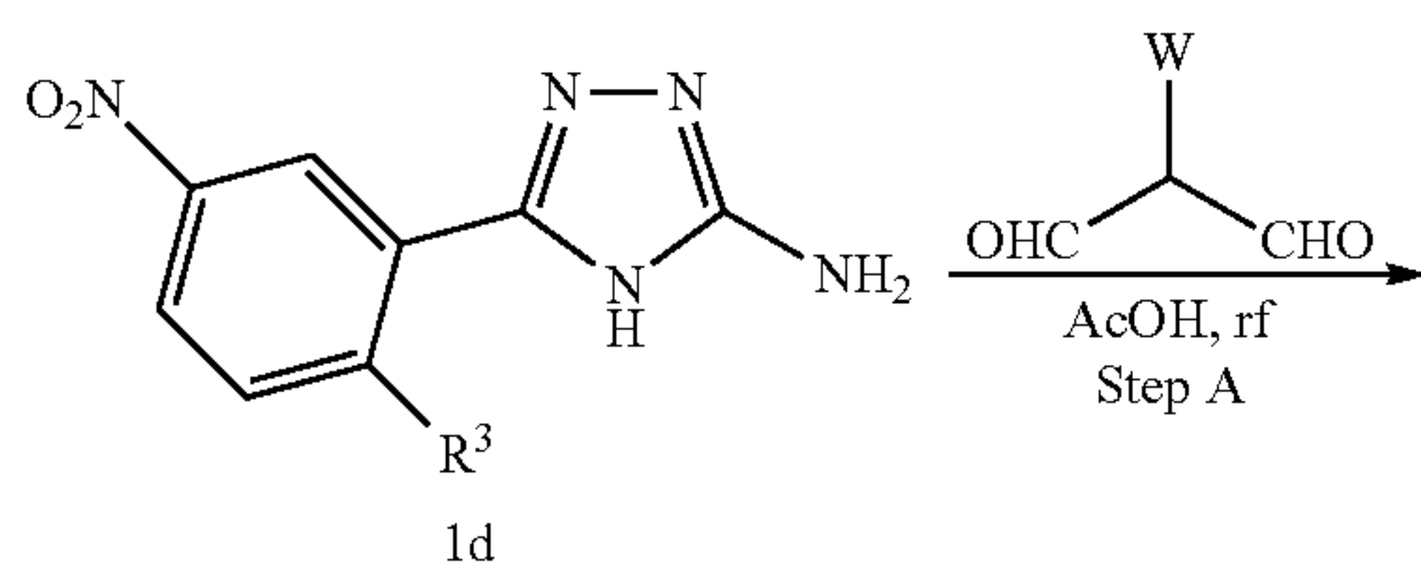
Scheme 2. Preparation of triazolopyridine compounds where W is halo.
