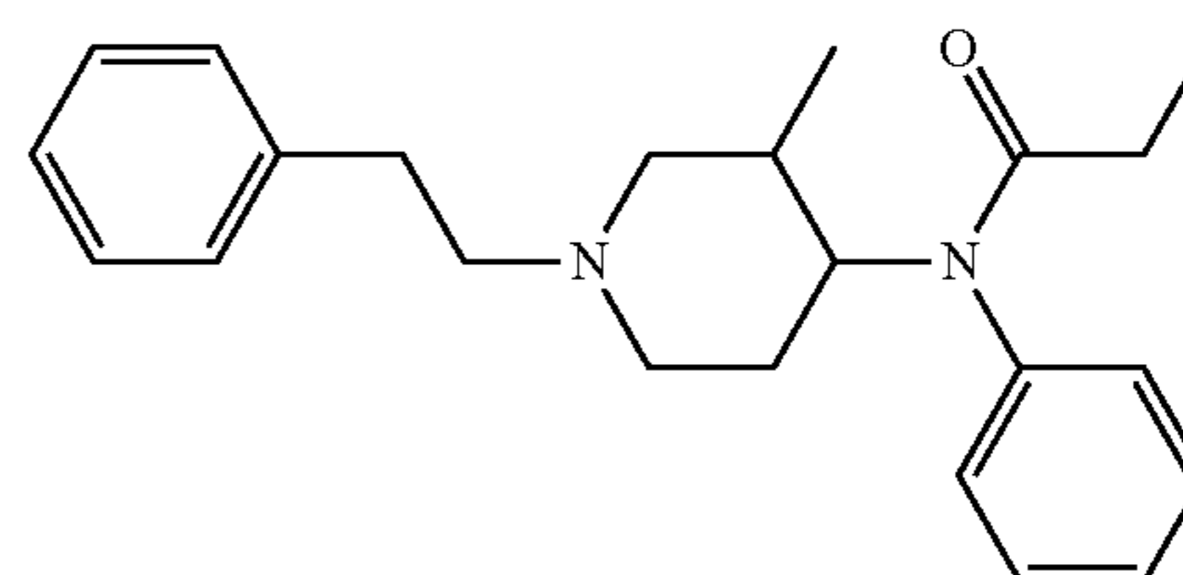
3-Methylfentanyl
