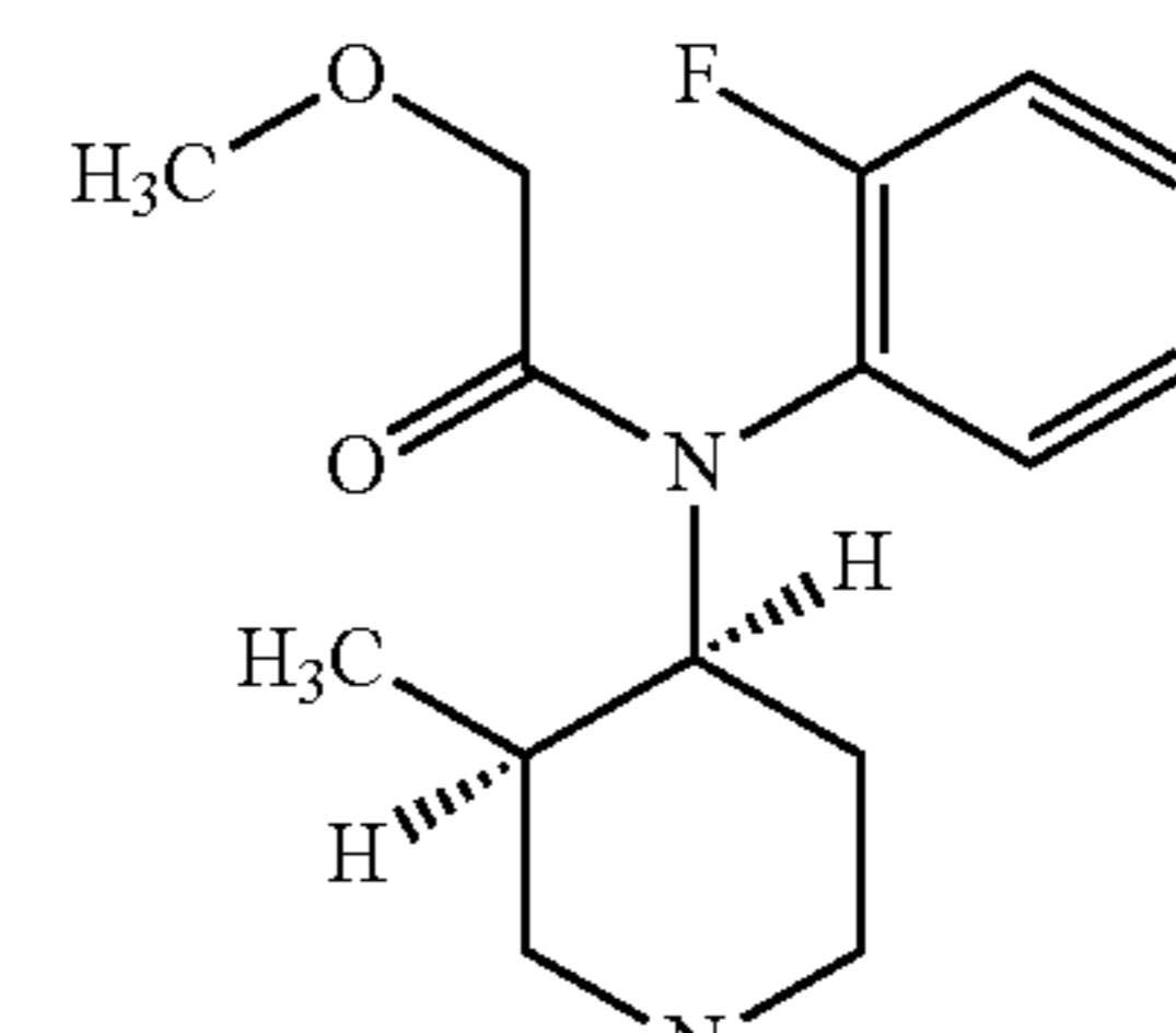
Butyrfentanyl
