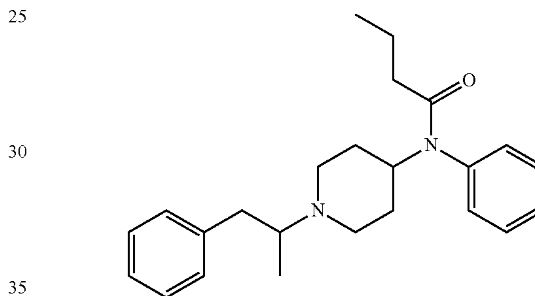
\alpha -Methylbutyrfentanyl
