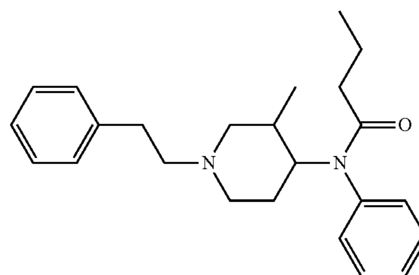
3-Methylbutyrfentanyl
