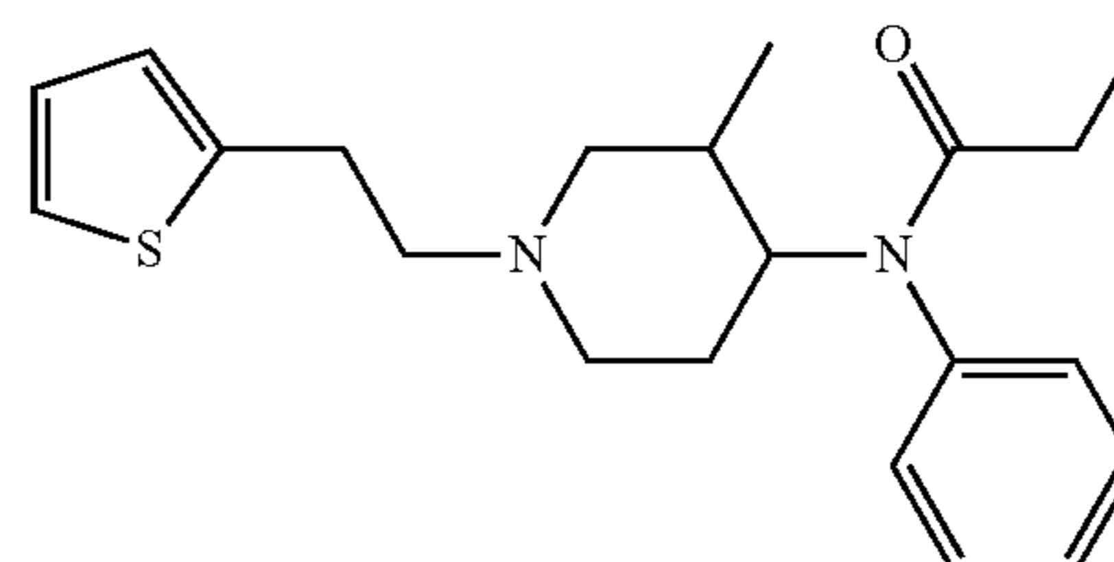
3-Methylthiofentanyl
