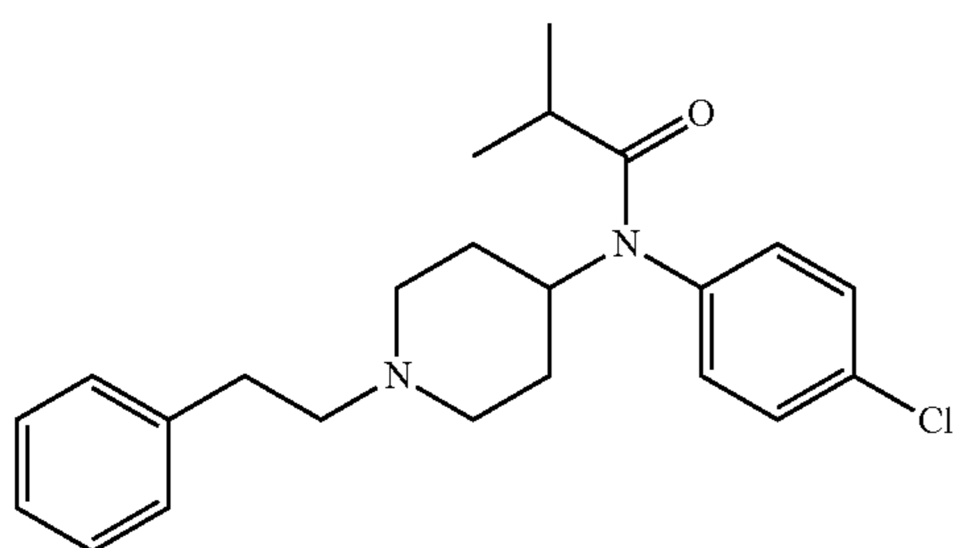
p-chloroisobutyrfentanyl
