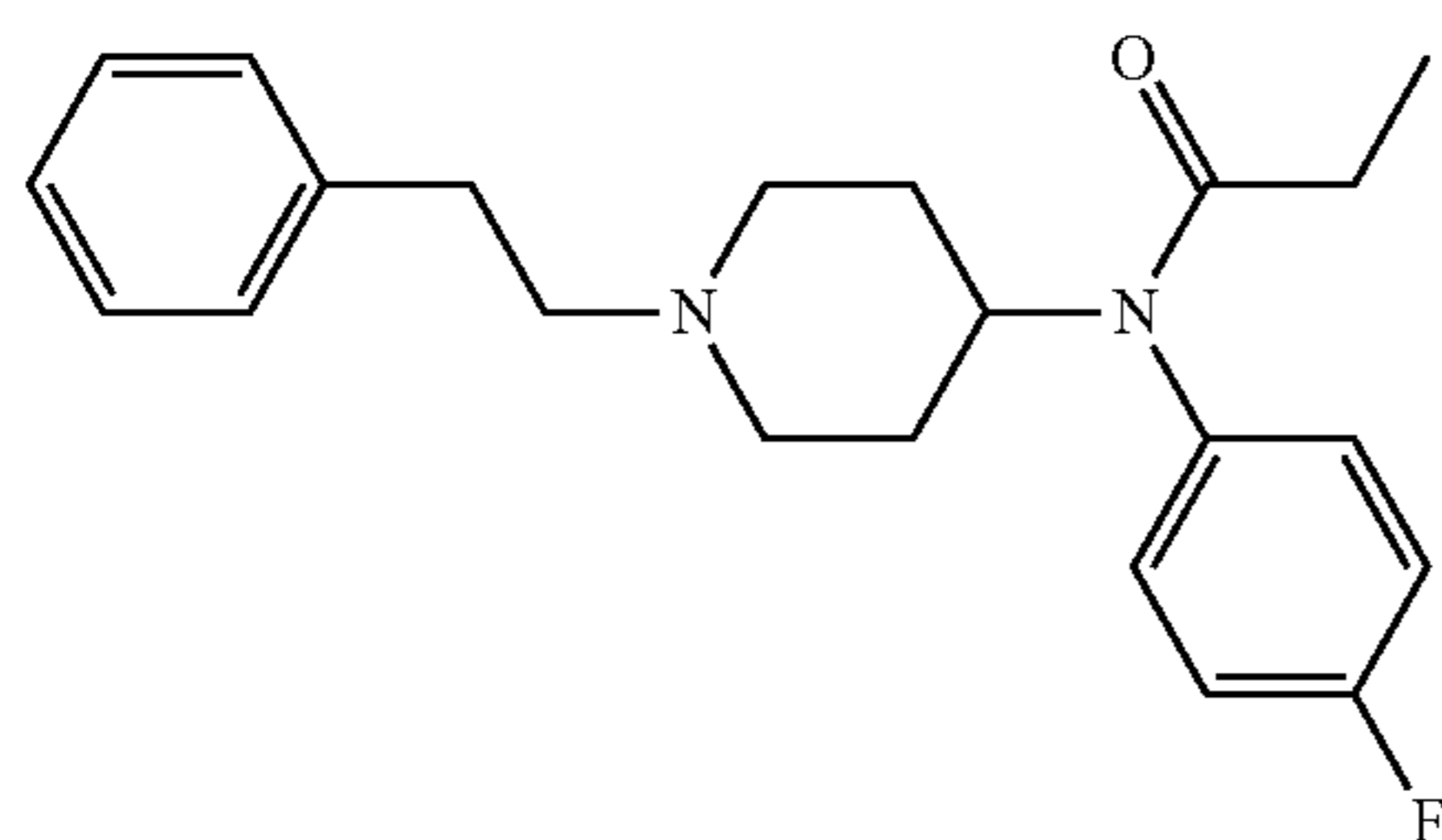
4-Fluorofentanyl
