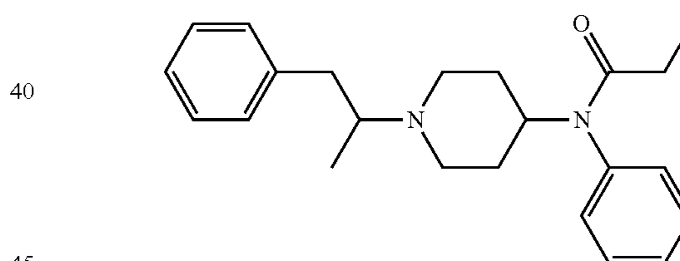
\alpha -Methylfentanyl
