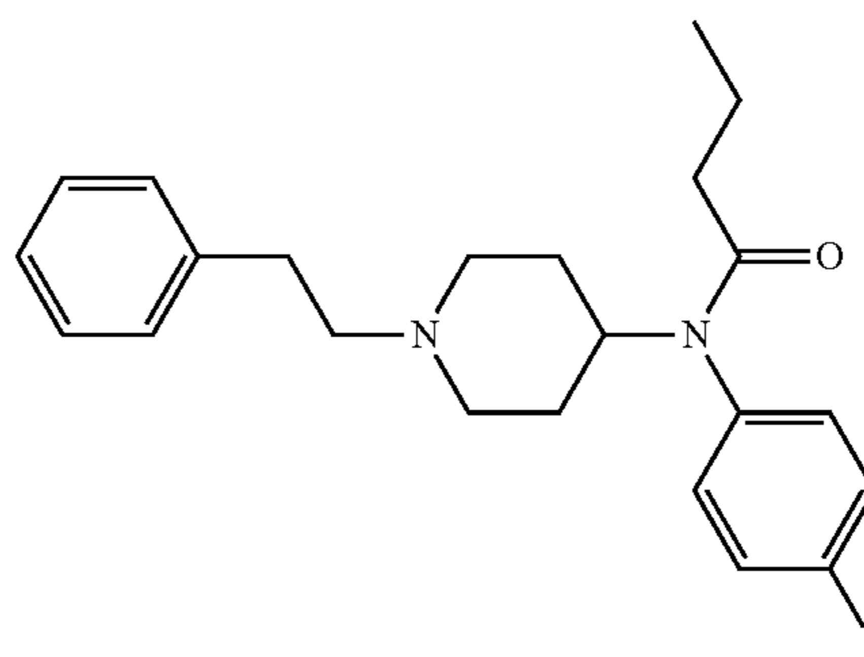
4-Fluorobutyrfentanyl
