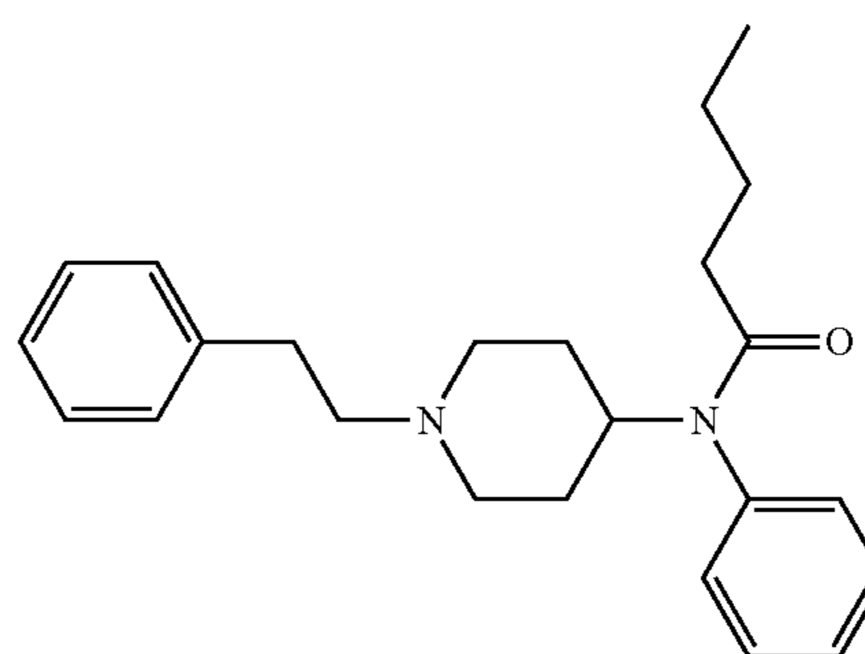
Valeryl fentanyl
