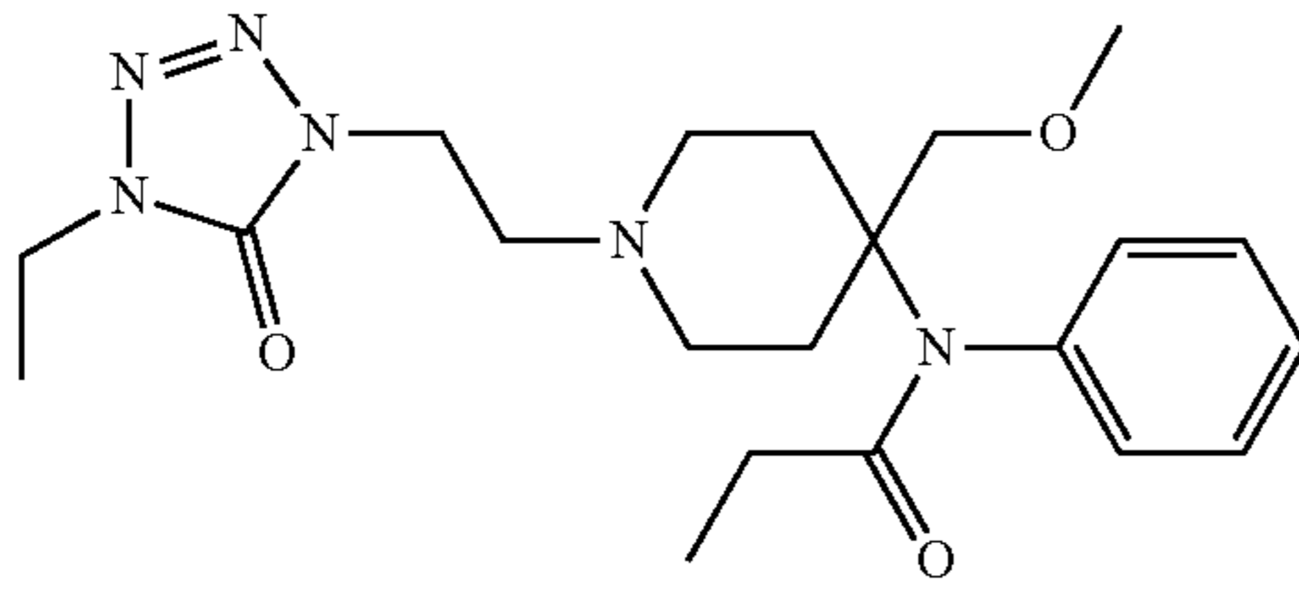
Alfentanyl
