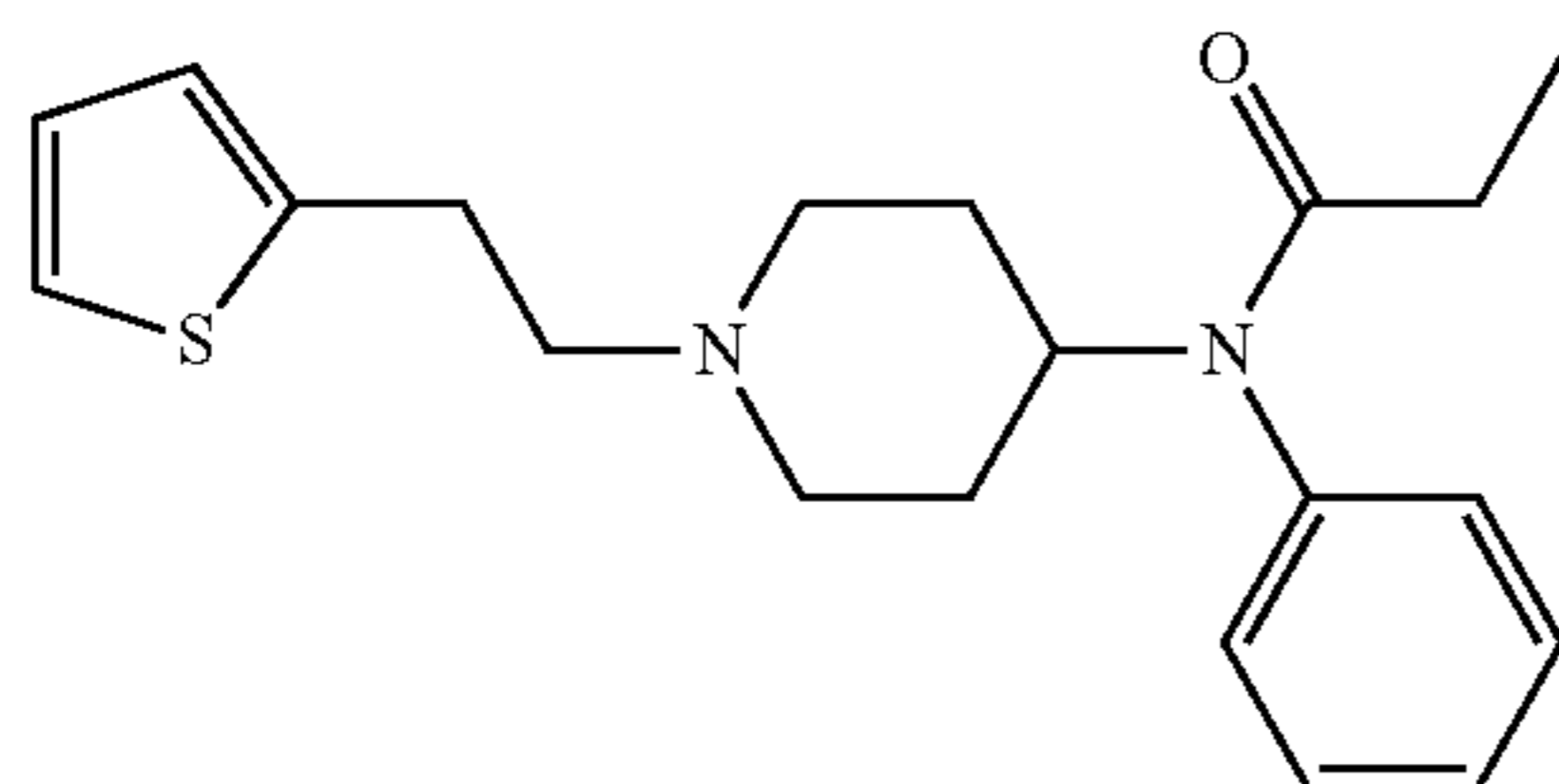
Thiofentanyl
