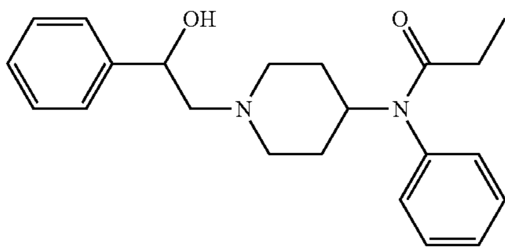
\beta -Hydroxyfentanyl
