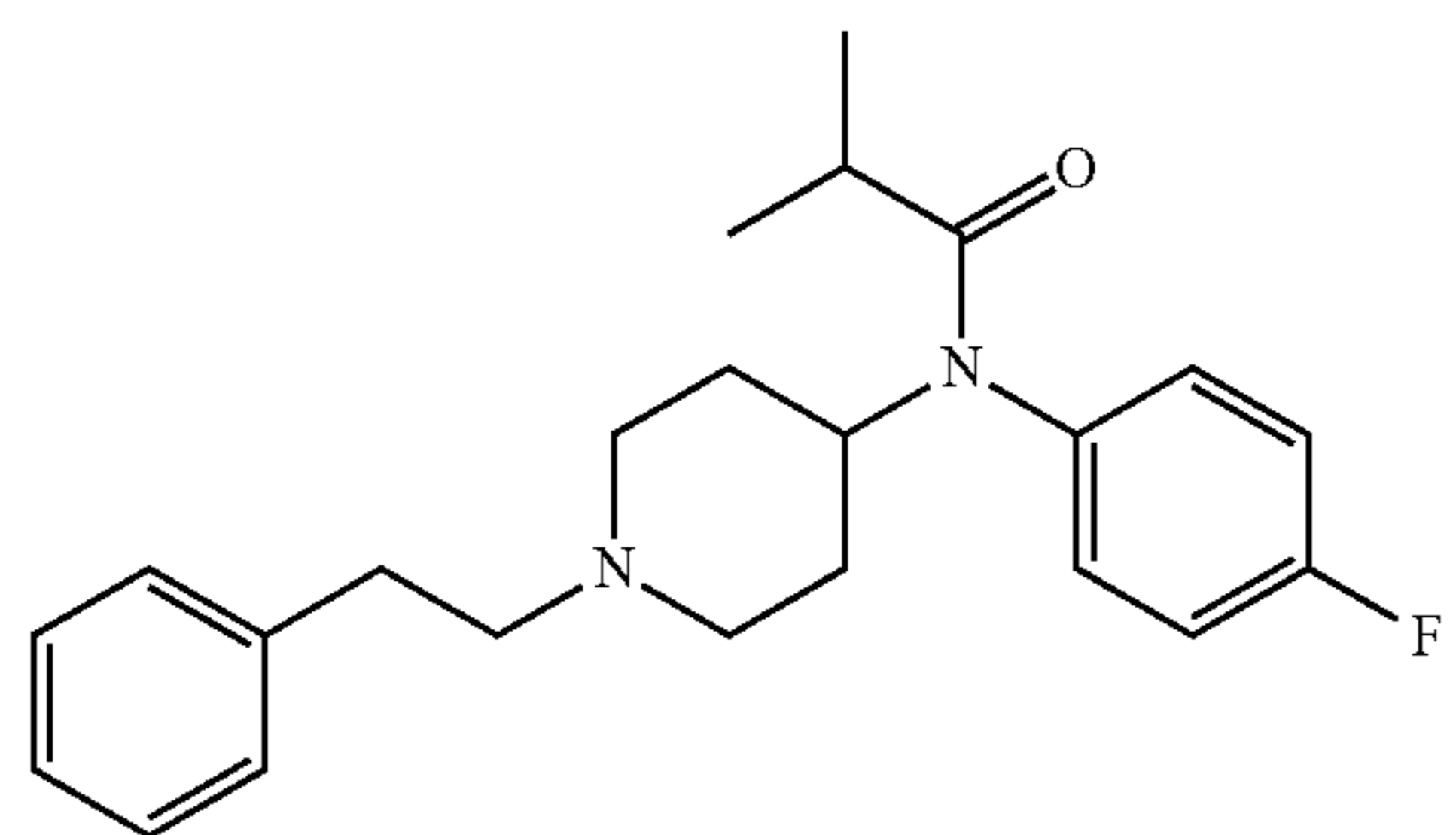
p-fluoroisobutyrfentanyl
