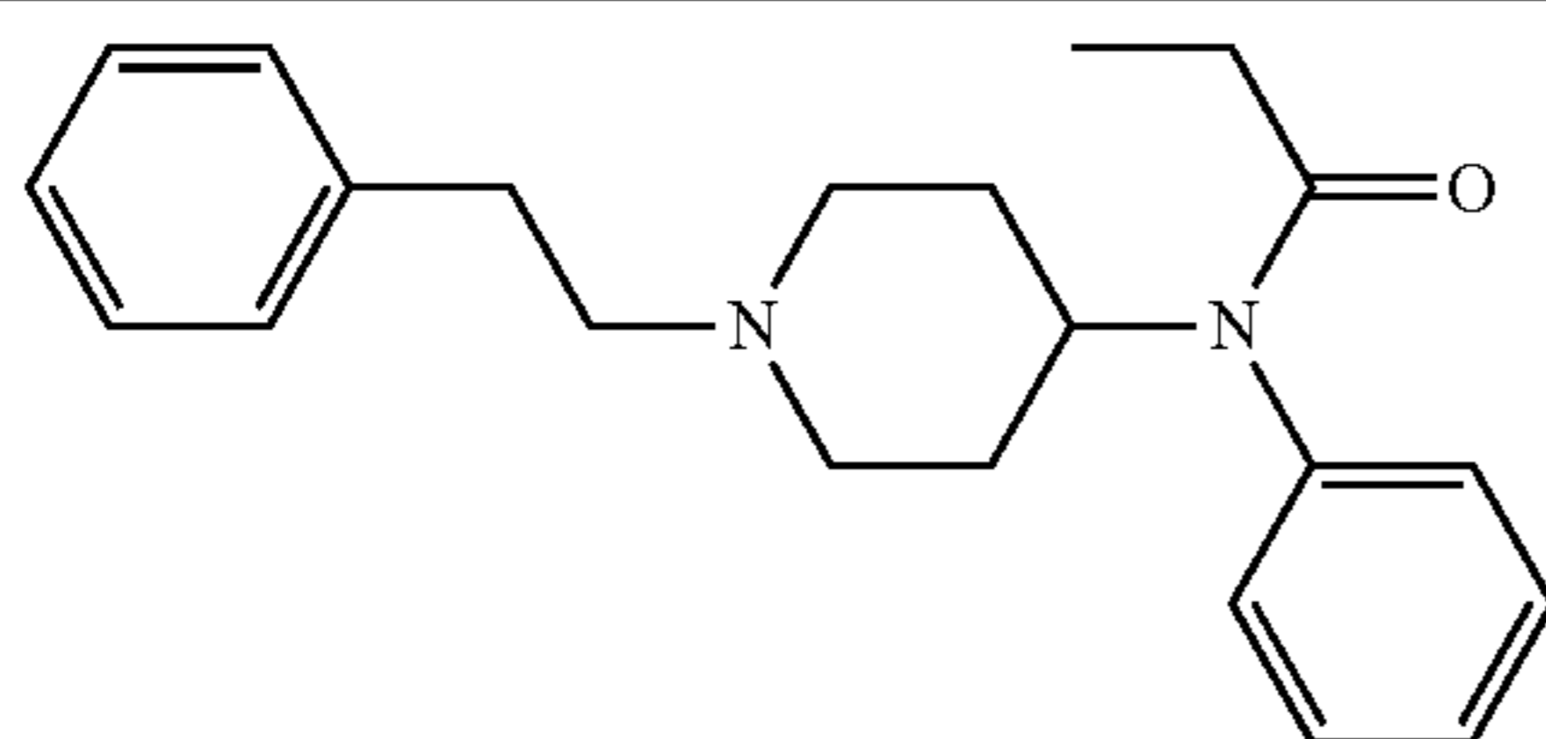
Fentanyl
