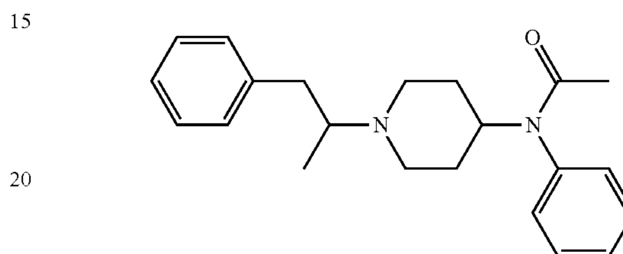
\alpha -Methylacetylfentanyl
