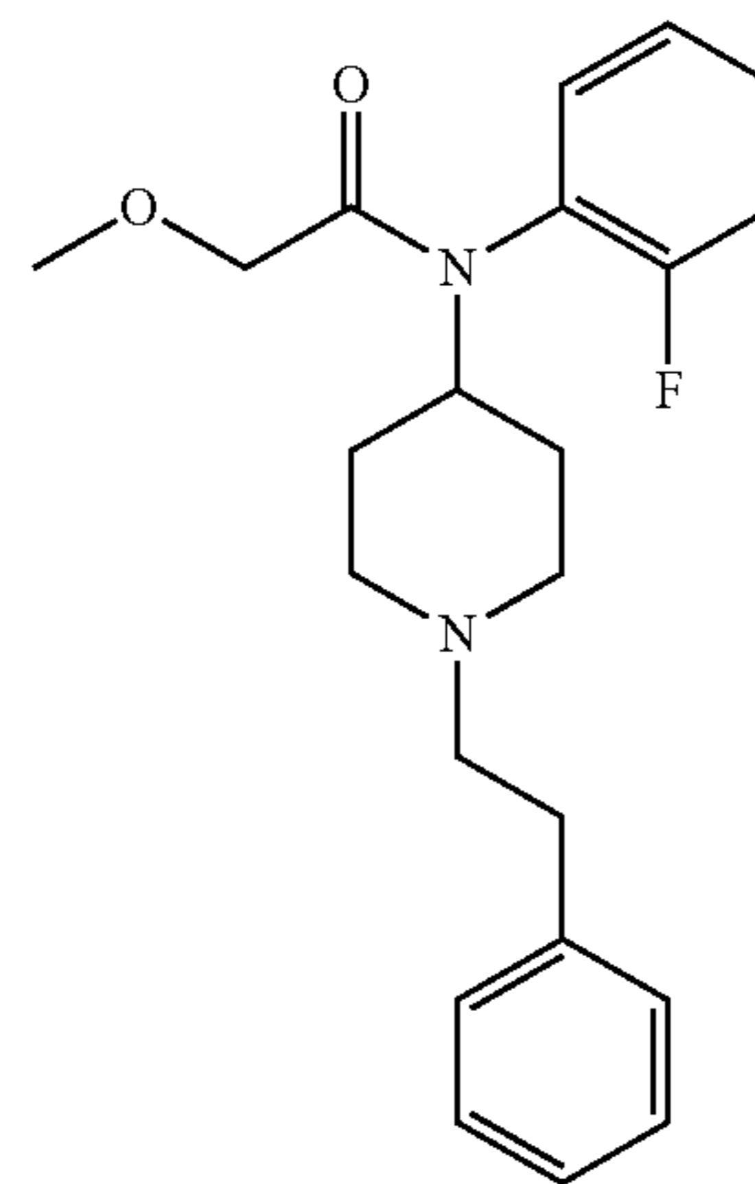
Ocfentanyl
