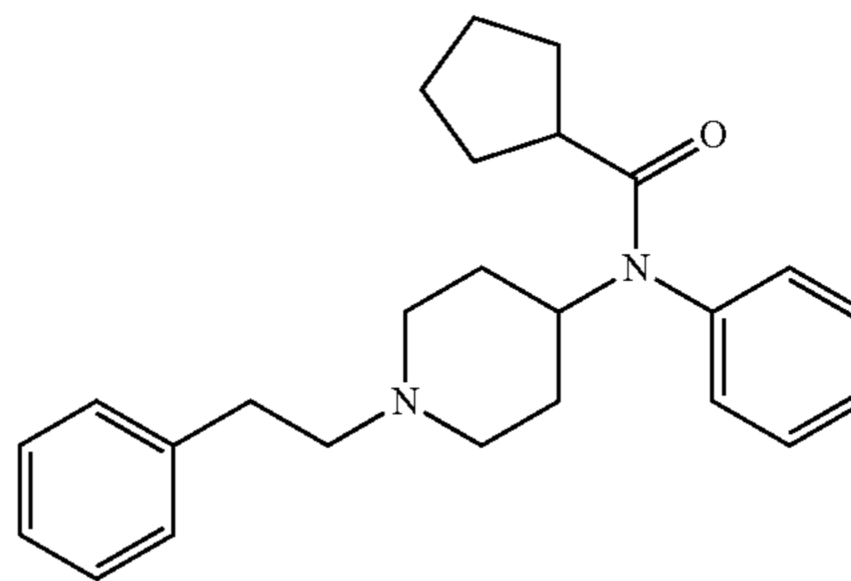
Cyclopentylfentanyl
