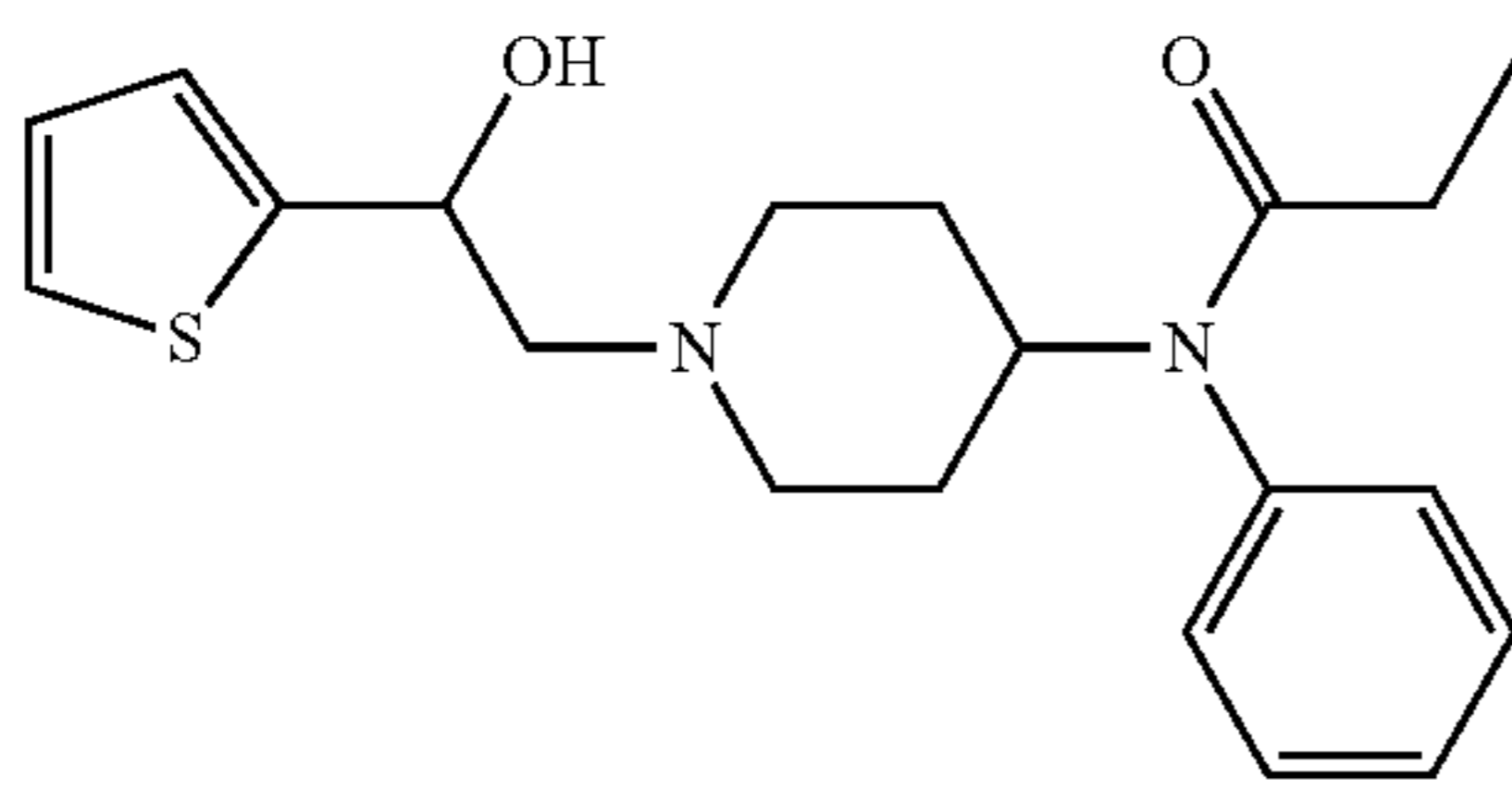
\beta -Hydroxythiofentanyl
