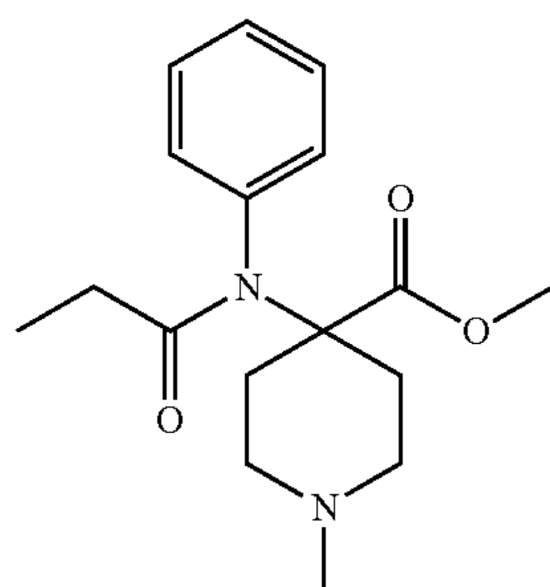
N-Methylcarfentanyl
