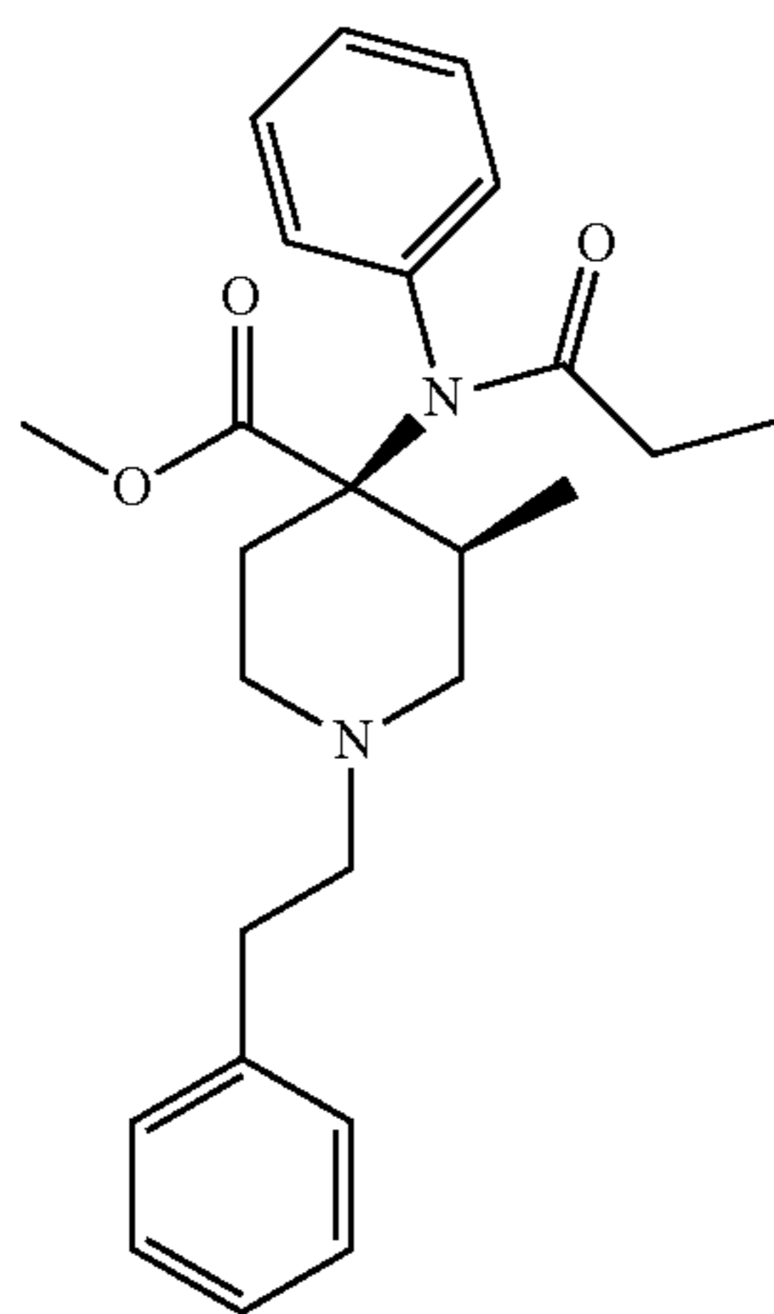
Lofentanyl
