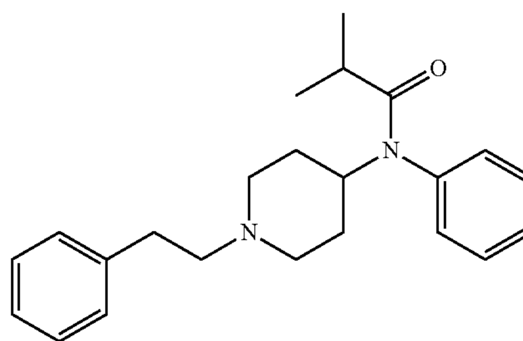
Isobutyrfentanyl
