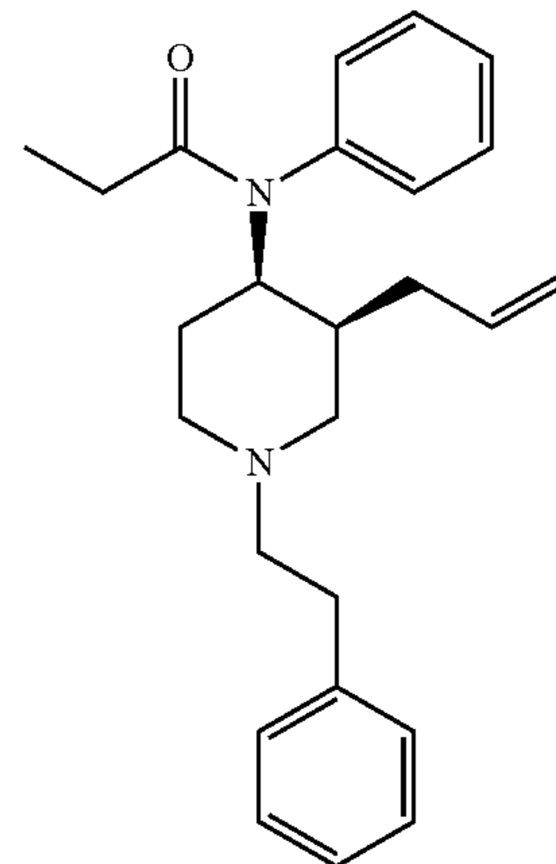
3-Allylfentanyl
