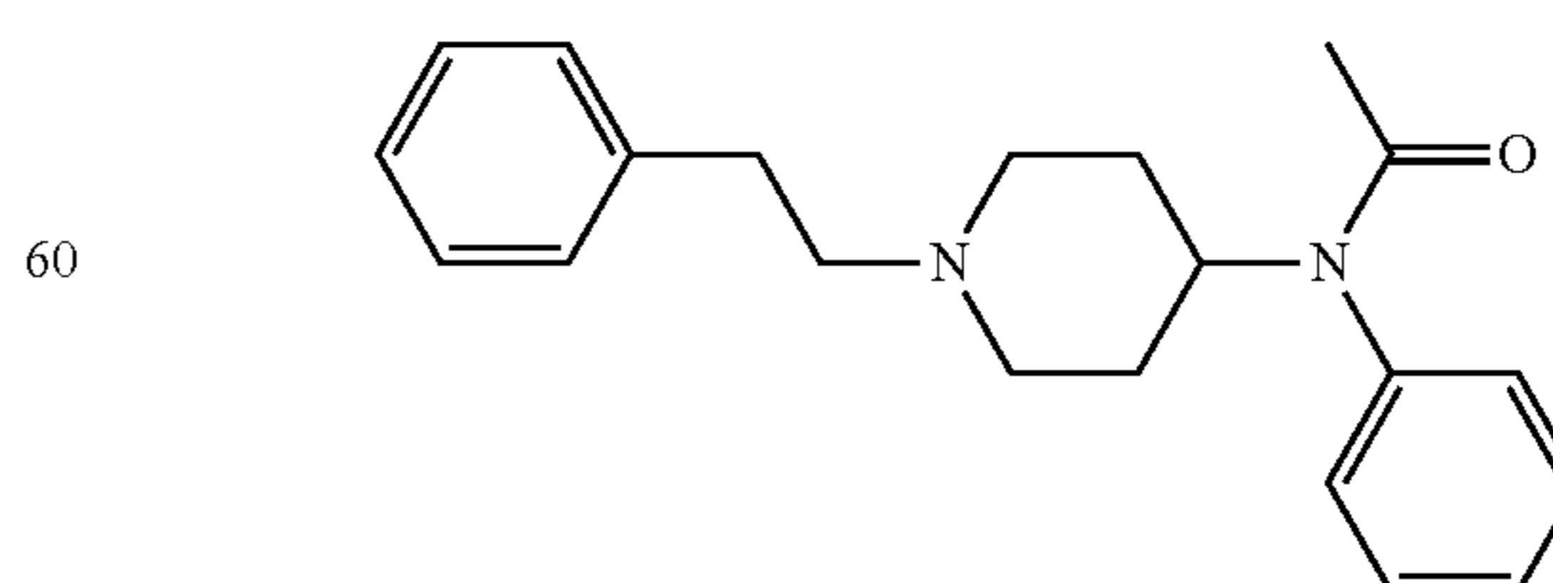
Acetylfentanyl
