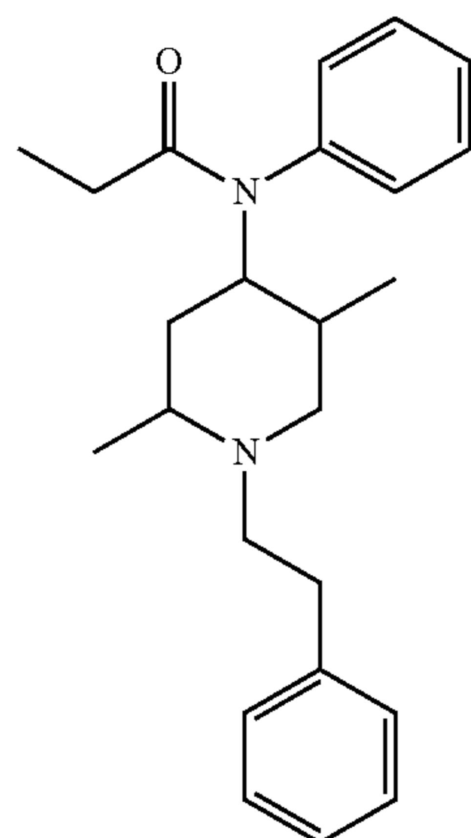
2,5-Dimethylfentanyl
