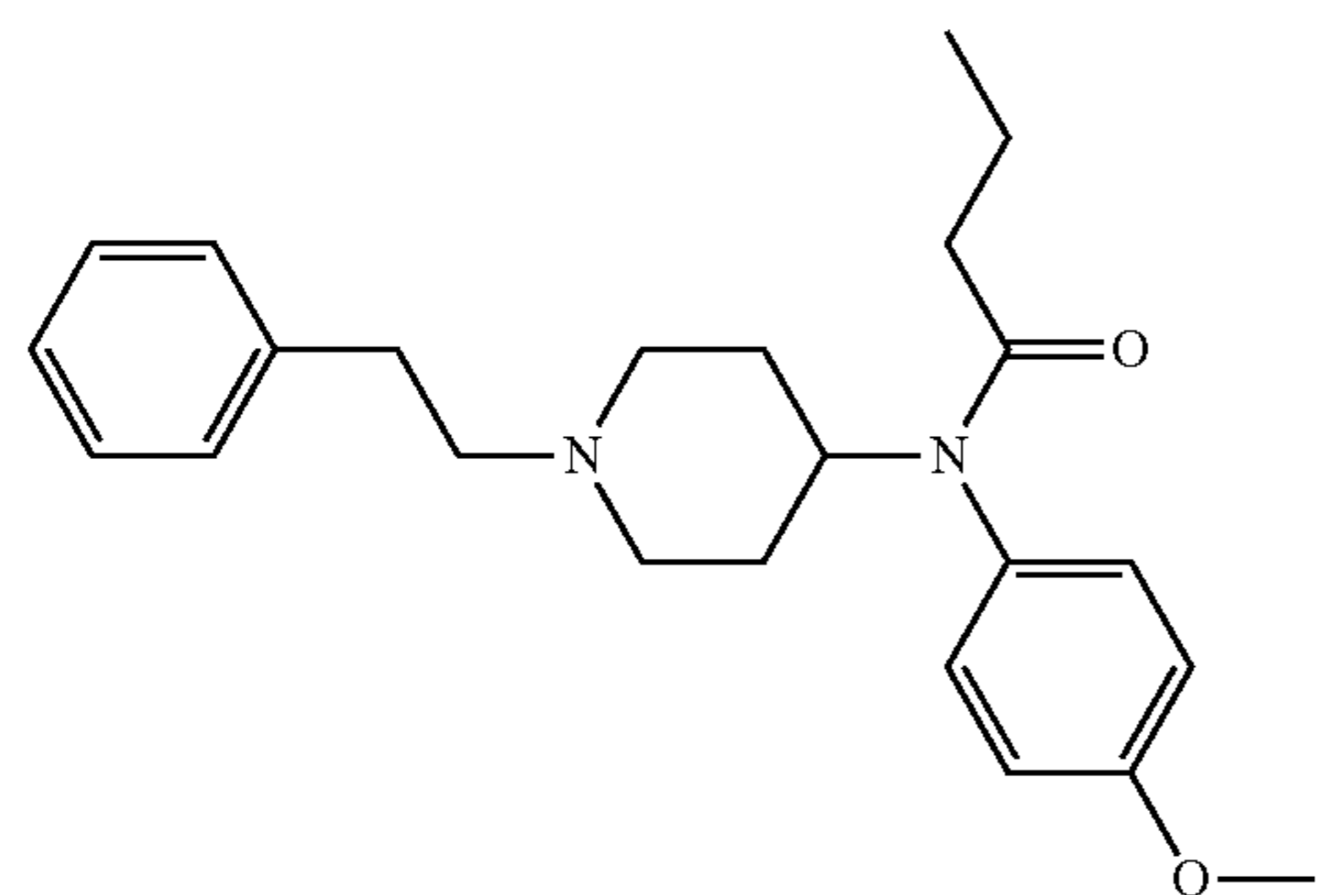
4-Methoxybutyrfentanyl
