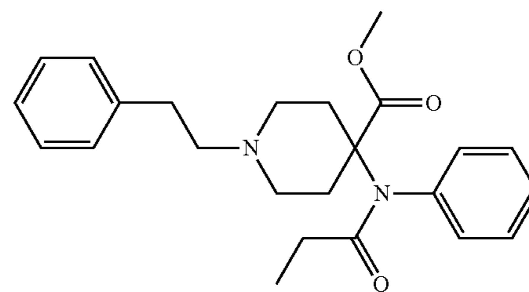
Carfentanyl
