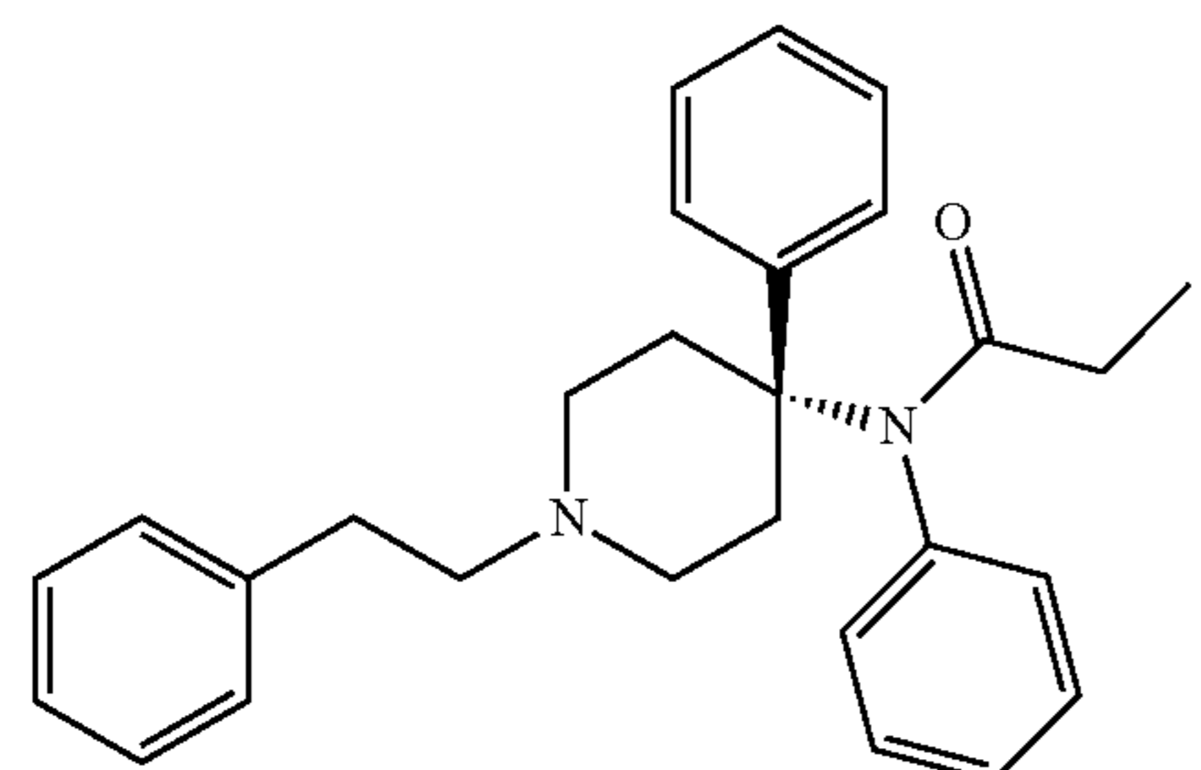
4-Phenylfentanyl
