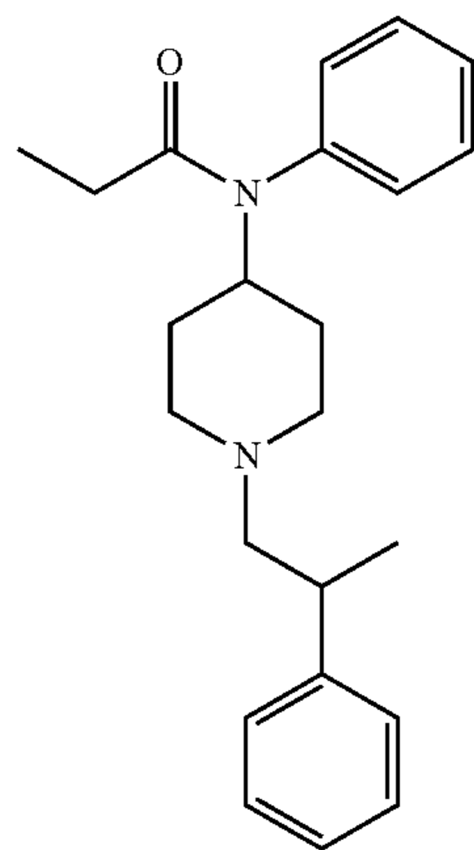
\beta -Methylfentanyl
