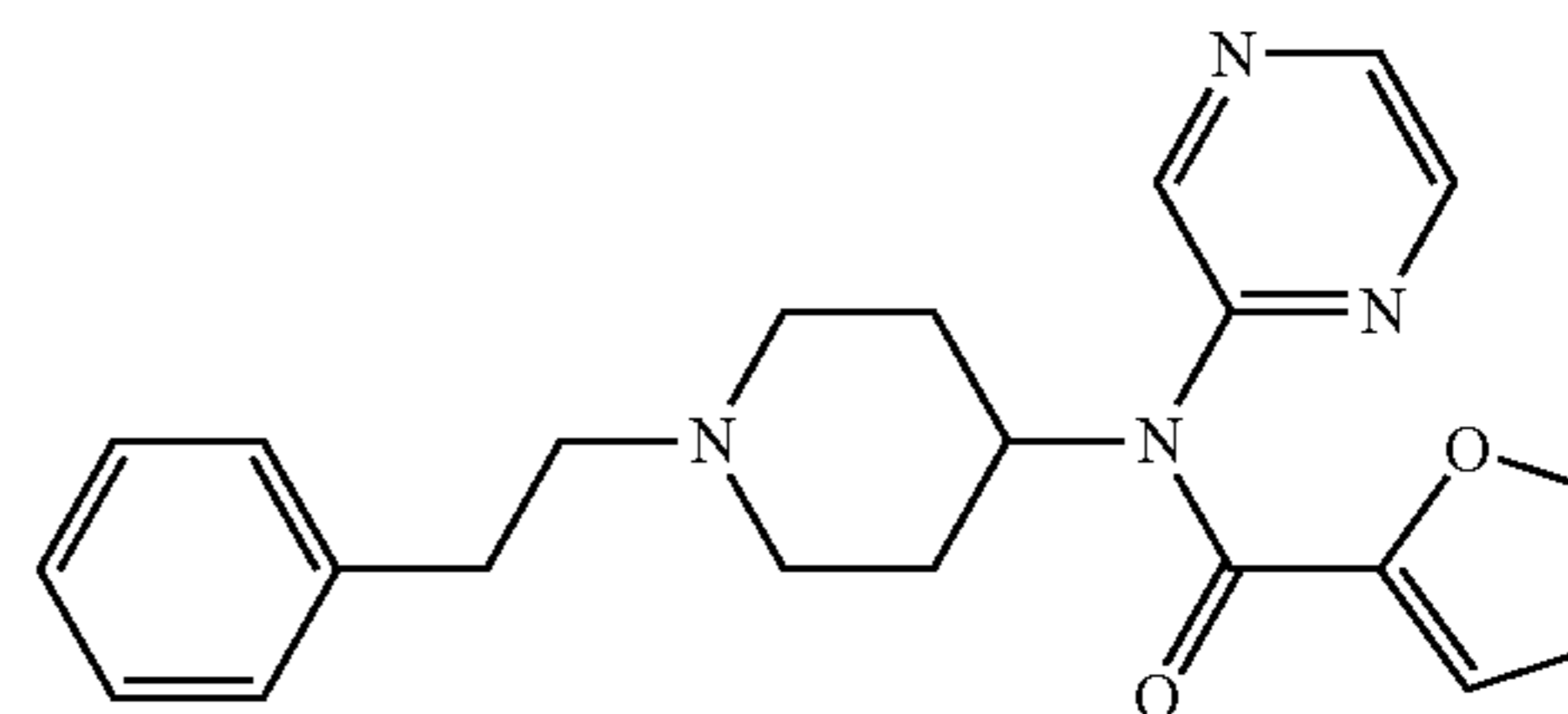
Mirfentanyl
