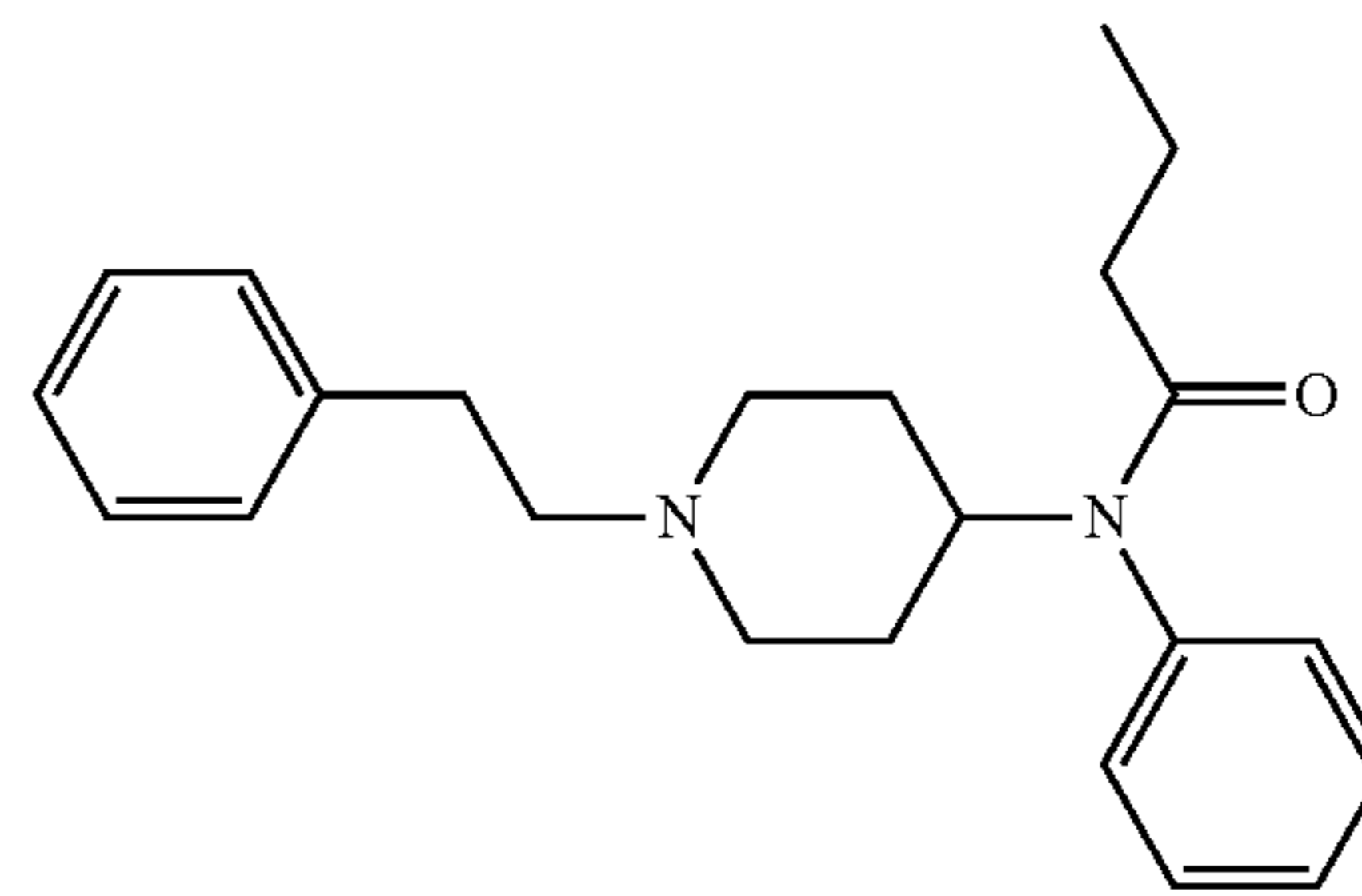
Butyrfentanyl
