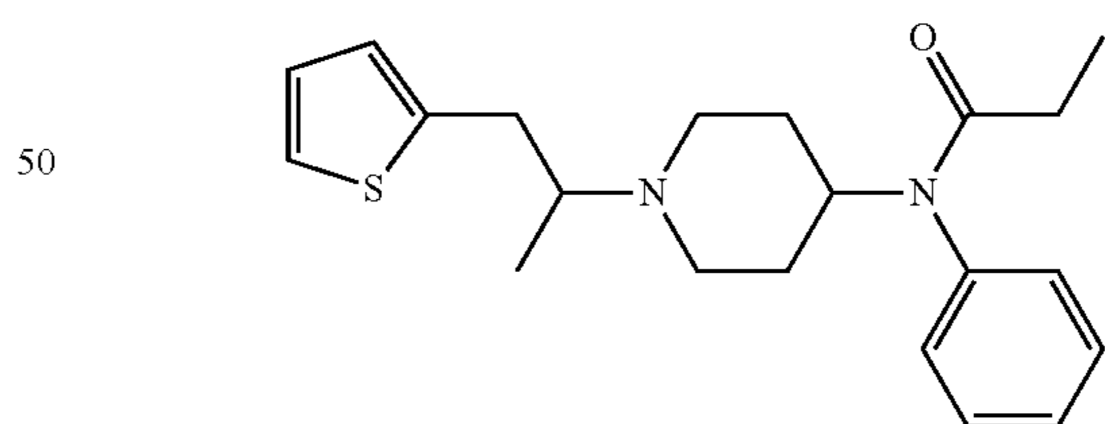
\alpha -Methylthiofentanyl
