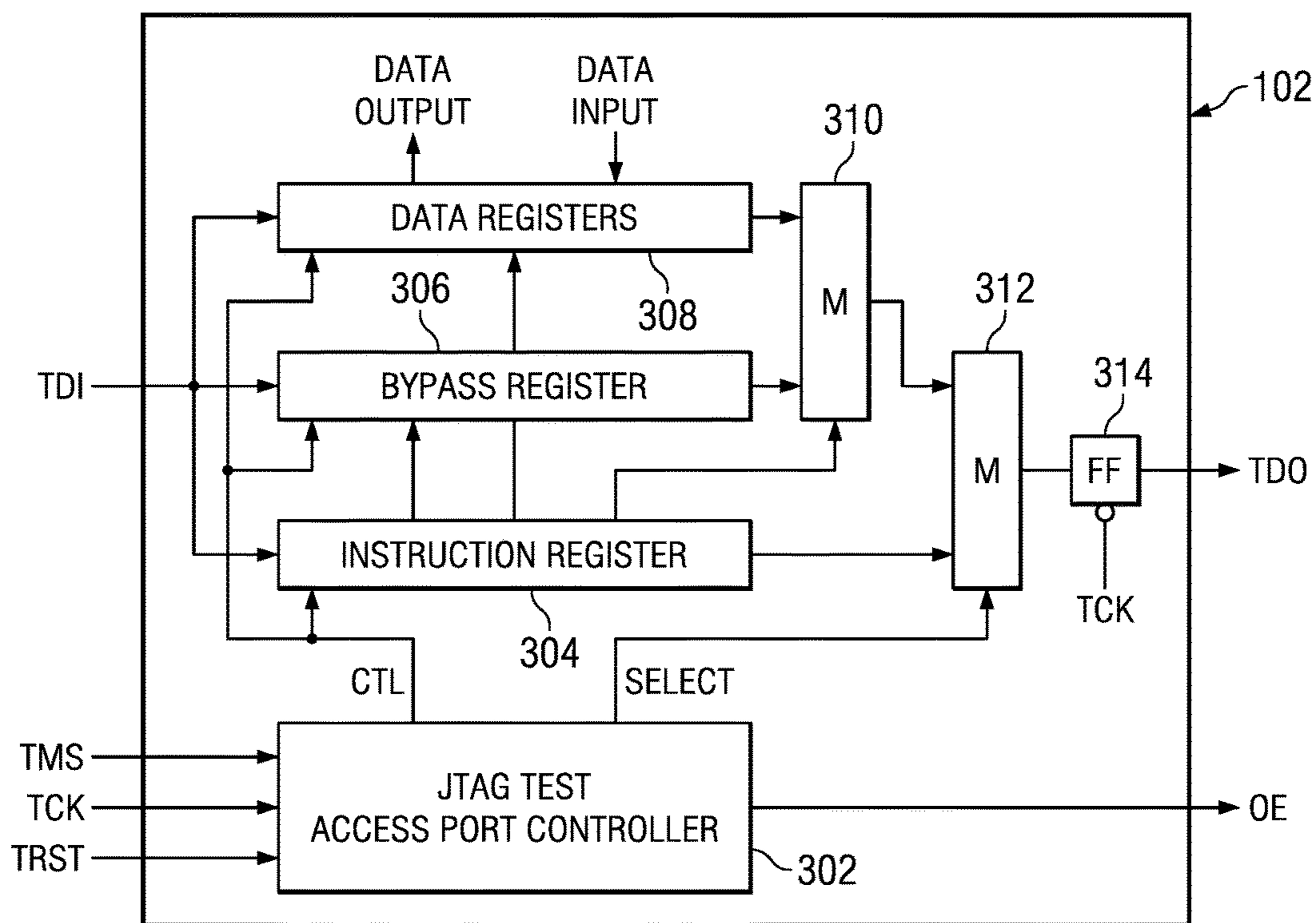
FIG. 3 (PRIOR ART)
