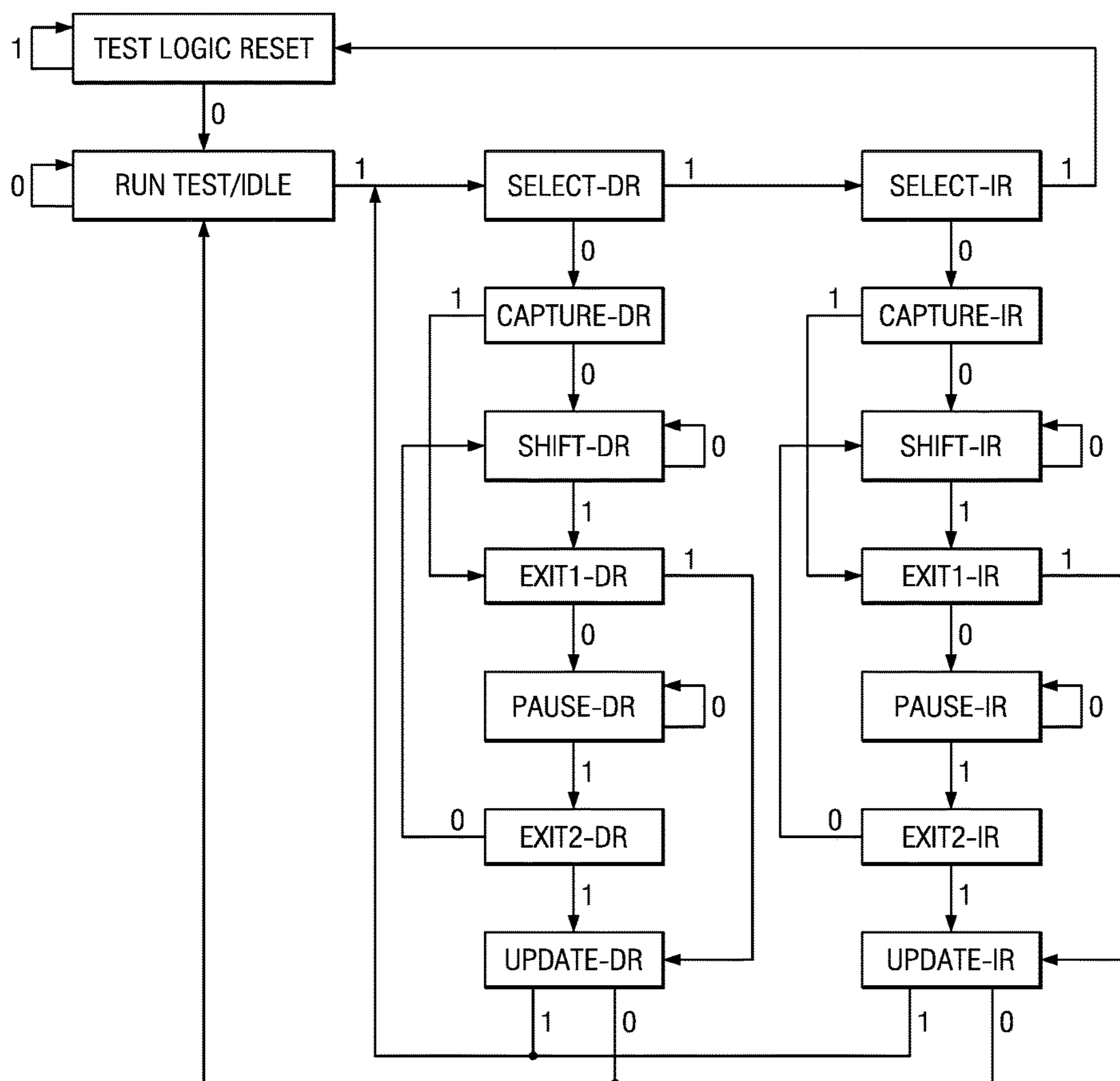
FIG. 4 (PRIOR ART)
