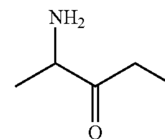
2-Amino-pentan-3-one
