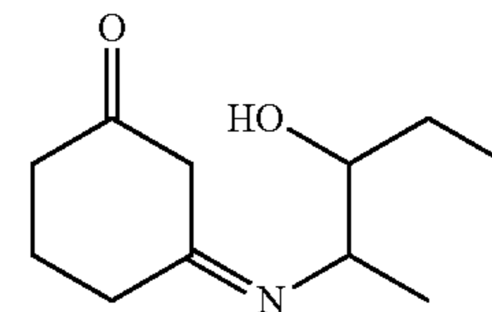
3-(2-Hydroxy-1-methyl-butylimino)-cyclohexanone
