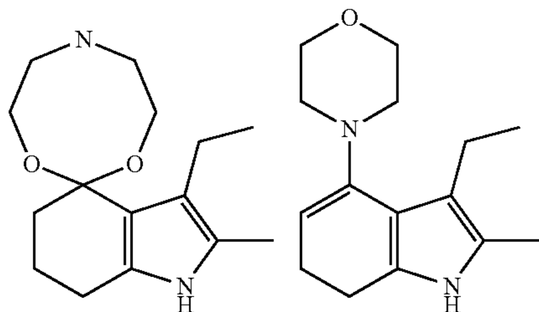
Impurity 3
