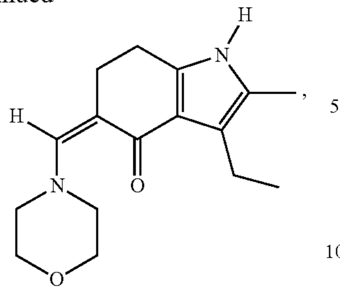
Intermediate 2, Enamine
