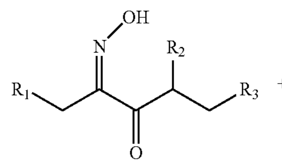
SUMO-1 Analogs
