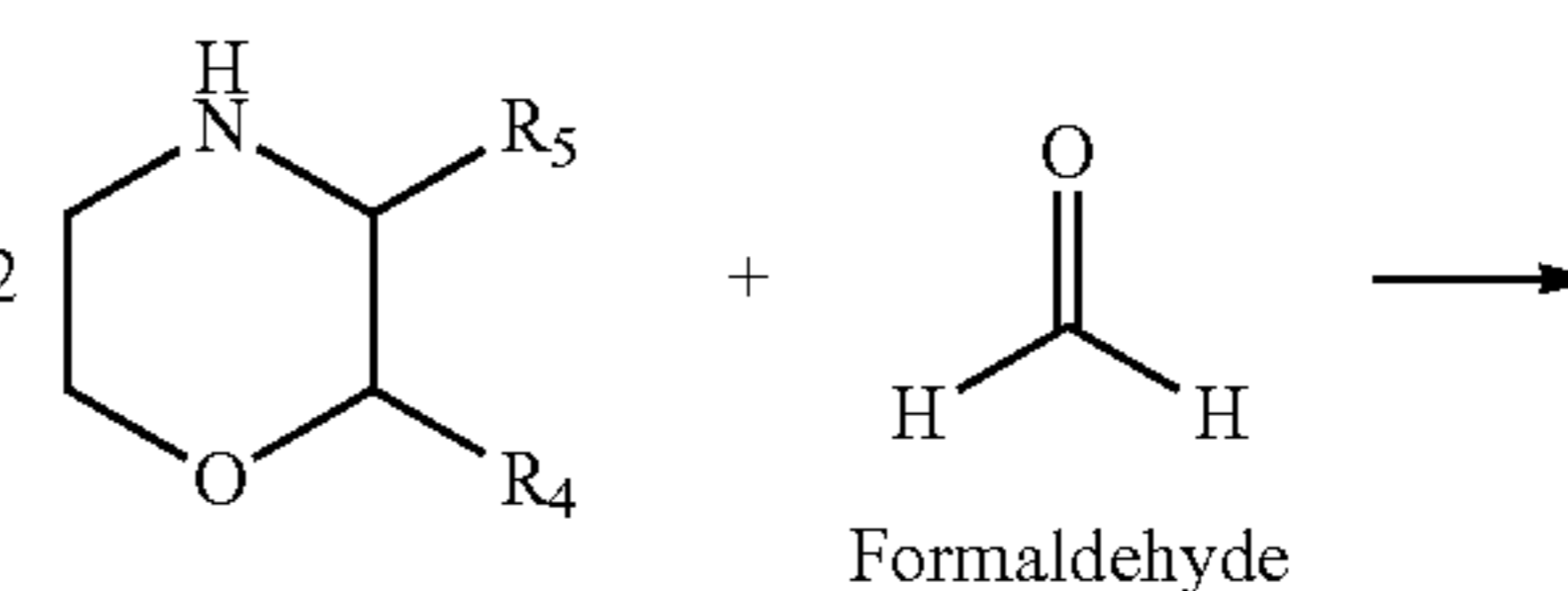
Substituted Morpholine
