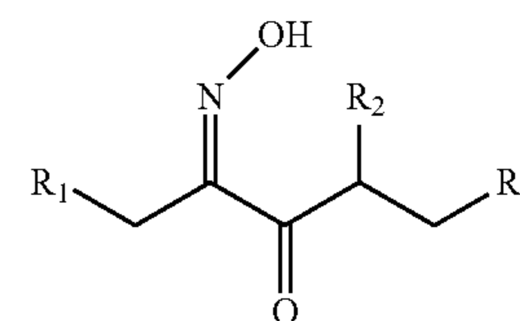
SUMO-1 Analogs
