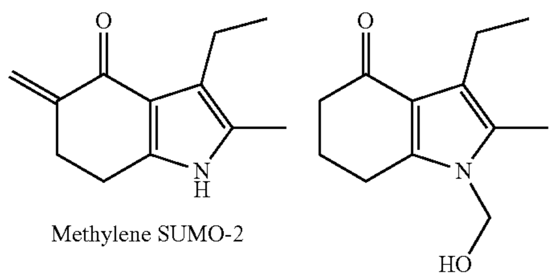
Hydroxymethyl SUMO-2
