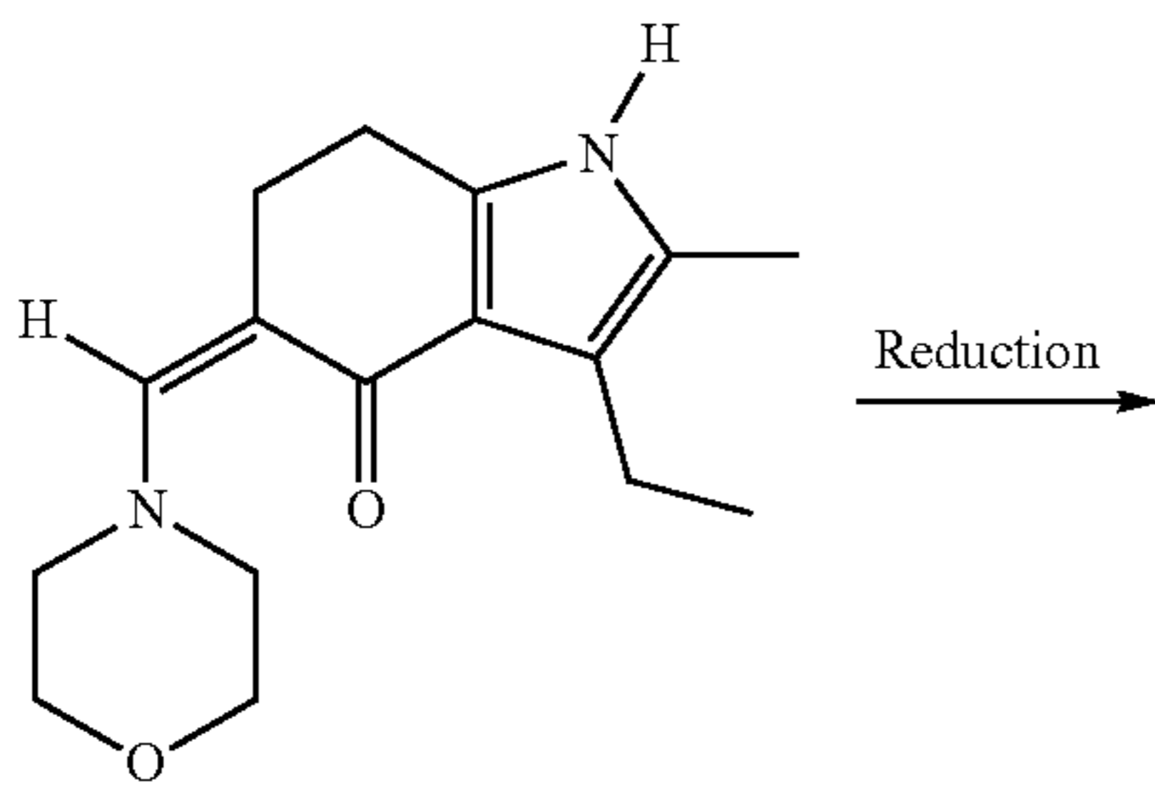
Intermediate 2, Enamine
