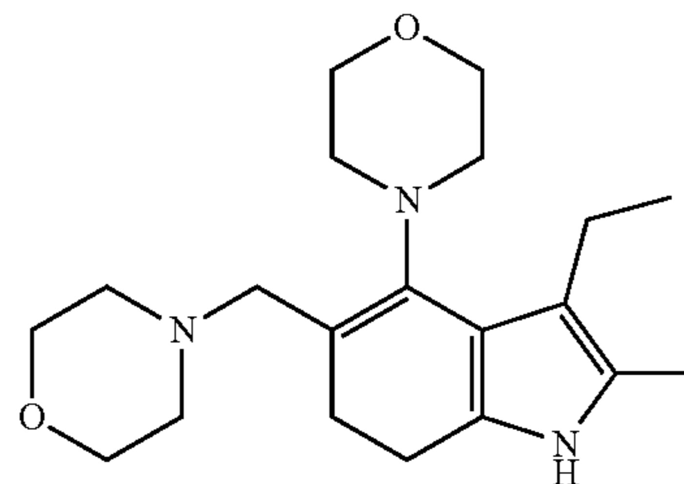
Impurity 5
