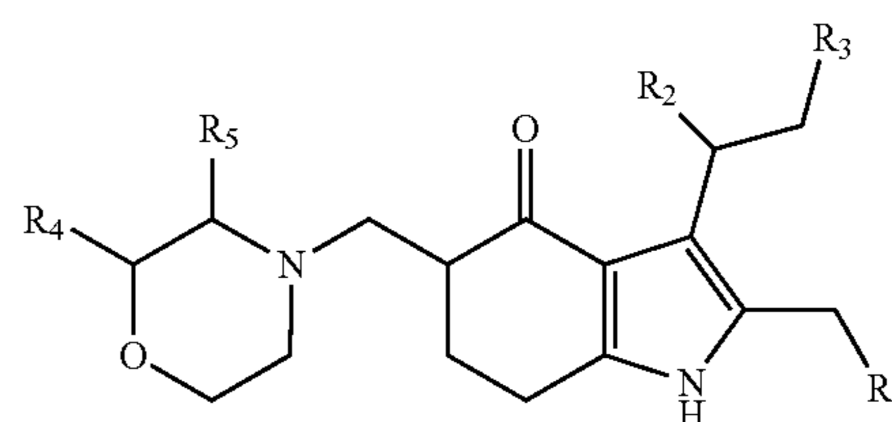
Molindone Analogs
