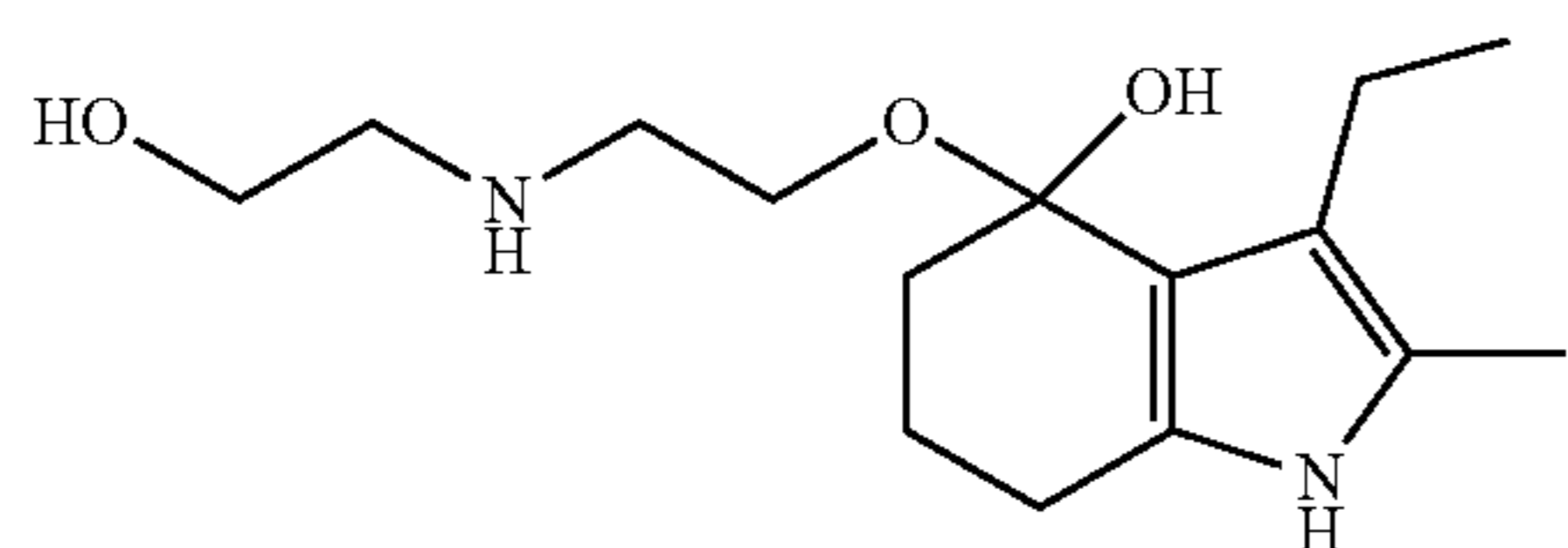
Impurity 1
