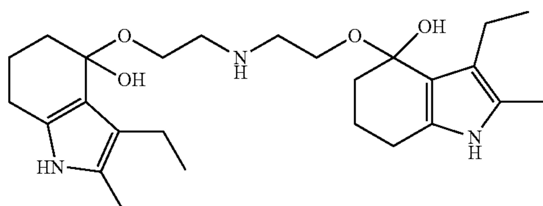
Impurity 2
