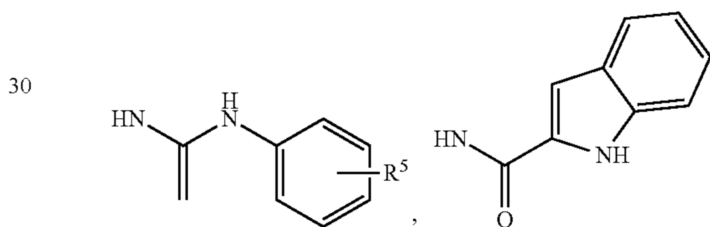
Formula I
