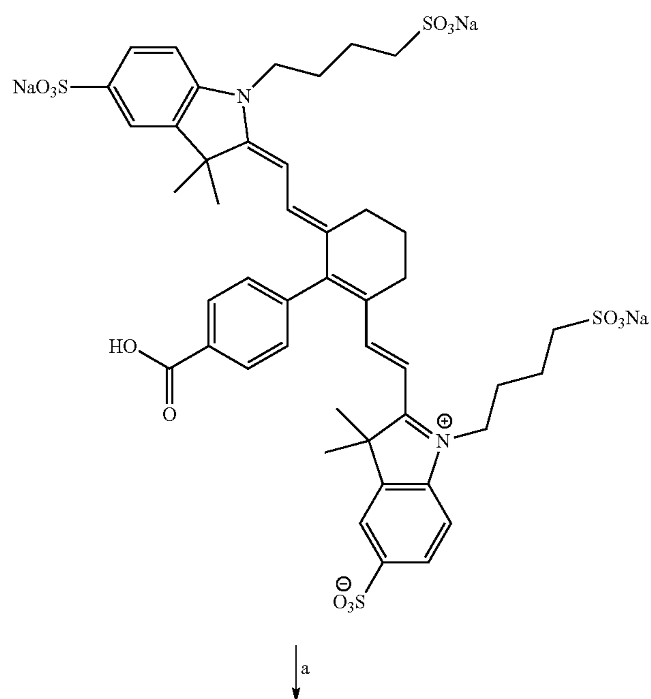
Scheme 5
