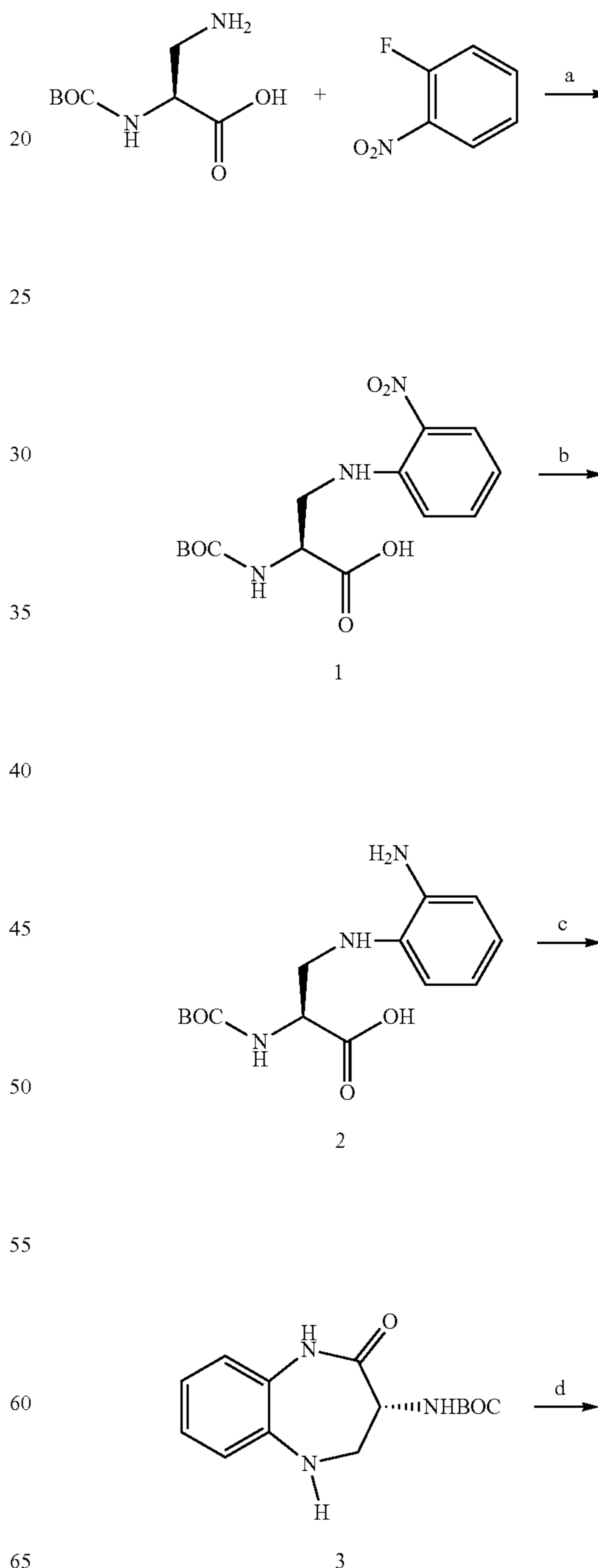
Scheme 1: Synthesis of Z-360
