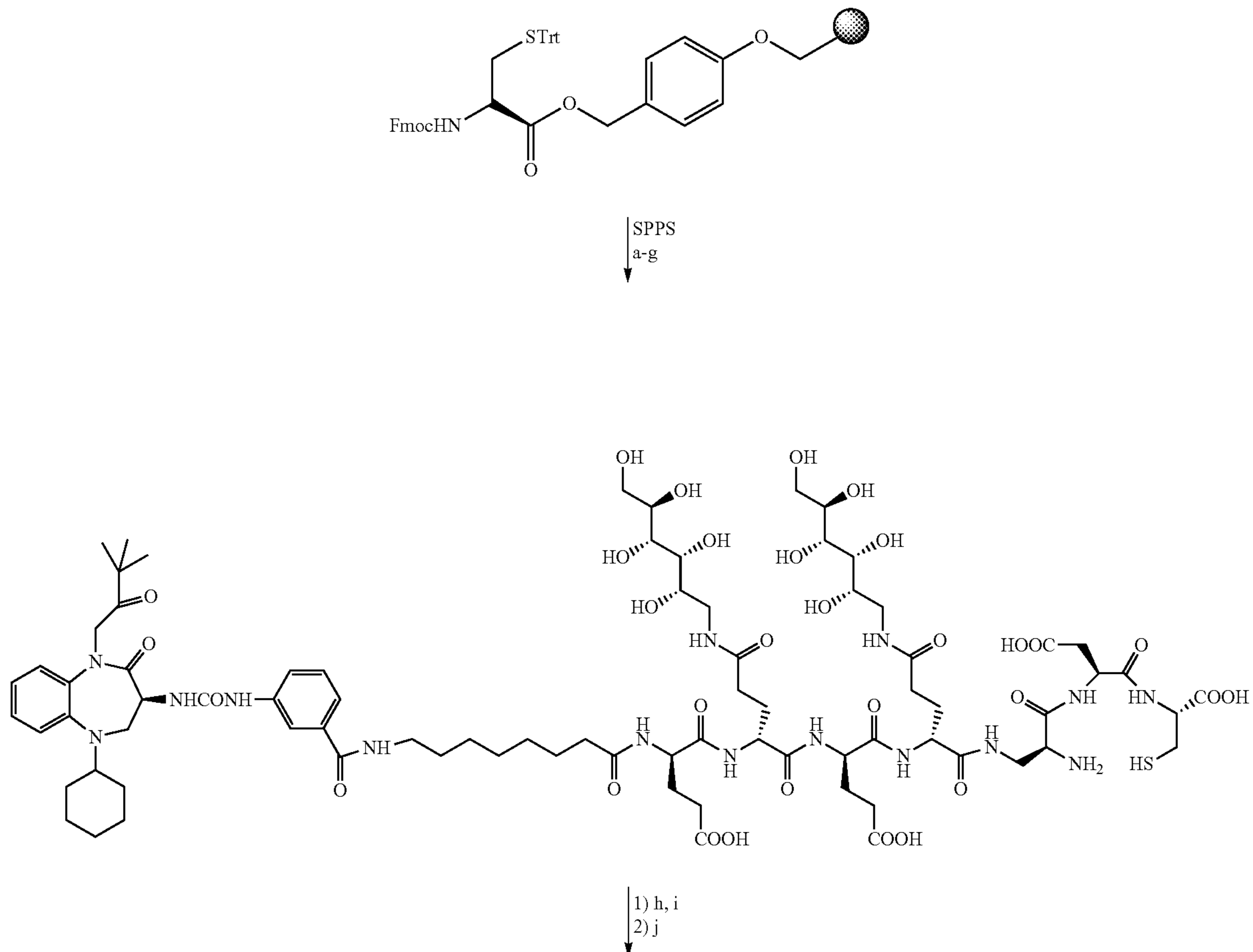
Scheme 3: Synthesis and Formulation of CRL-3 99m Tc
