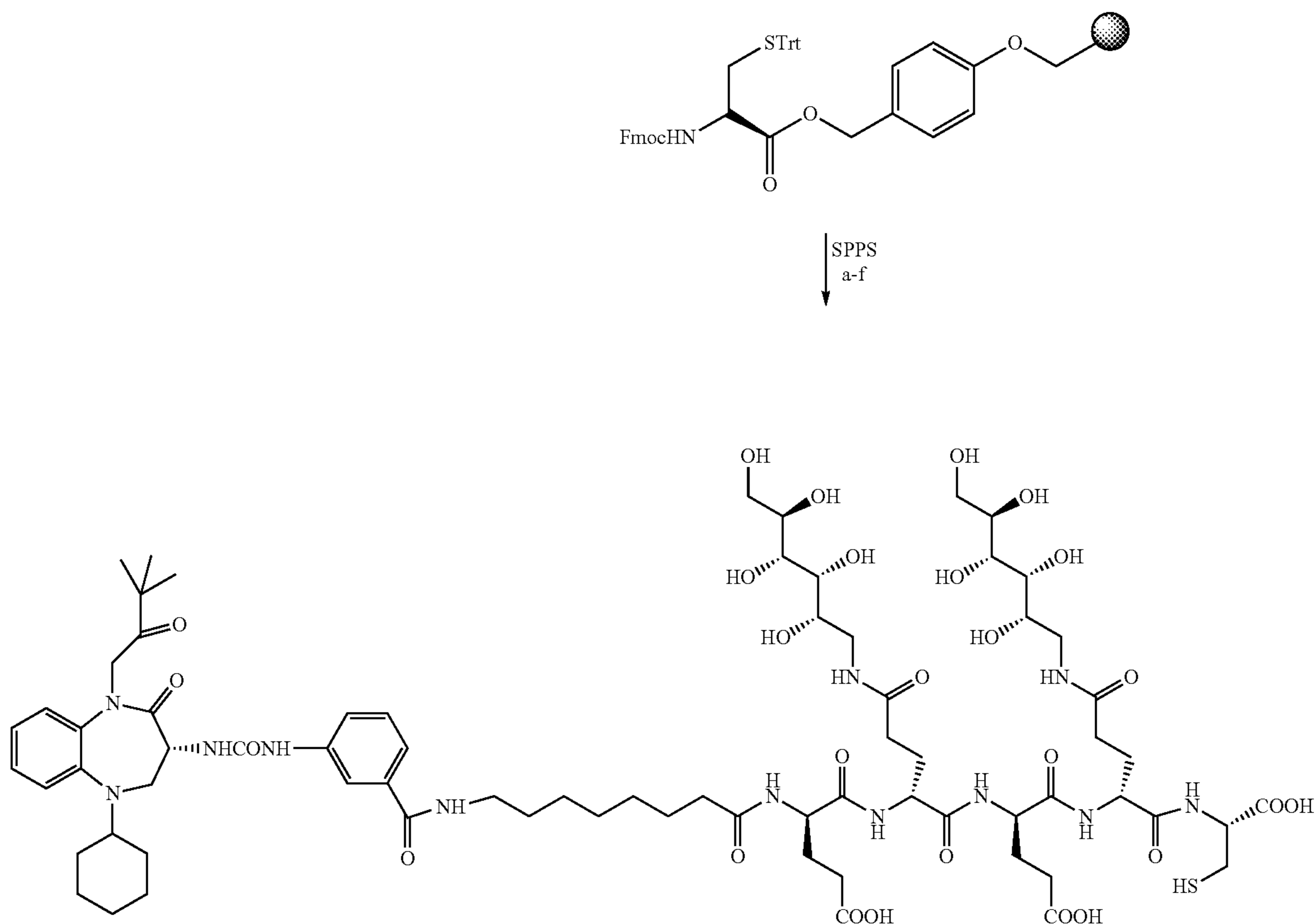
Scheme 6
