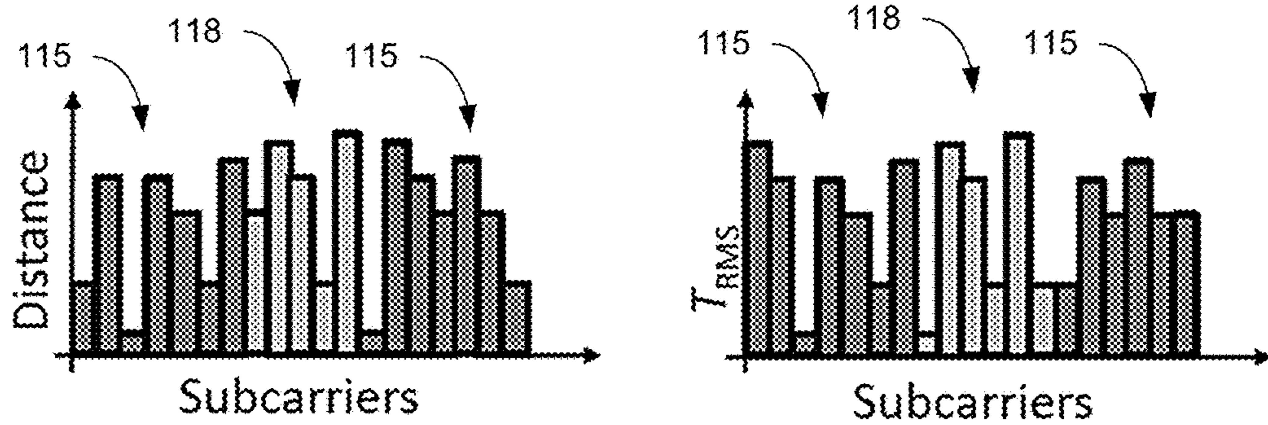
Random scheduling.
