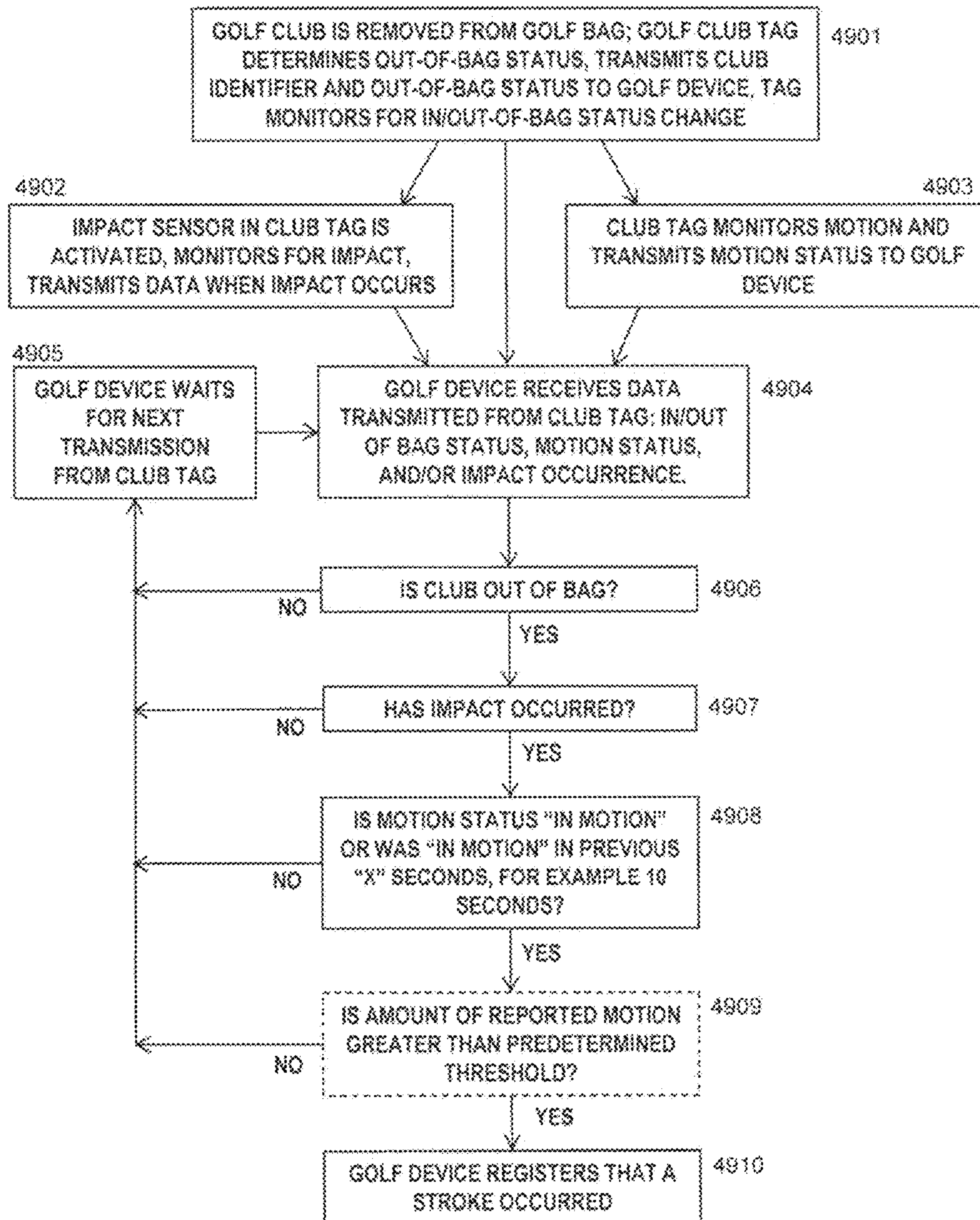
FIGURE 49 COMBINATION OF MOTION & IMPACT DATA
