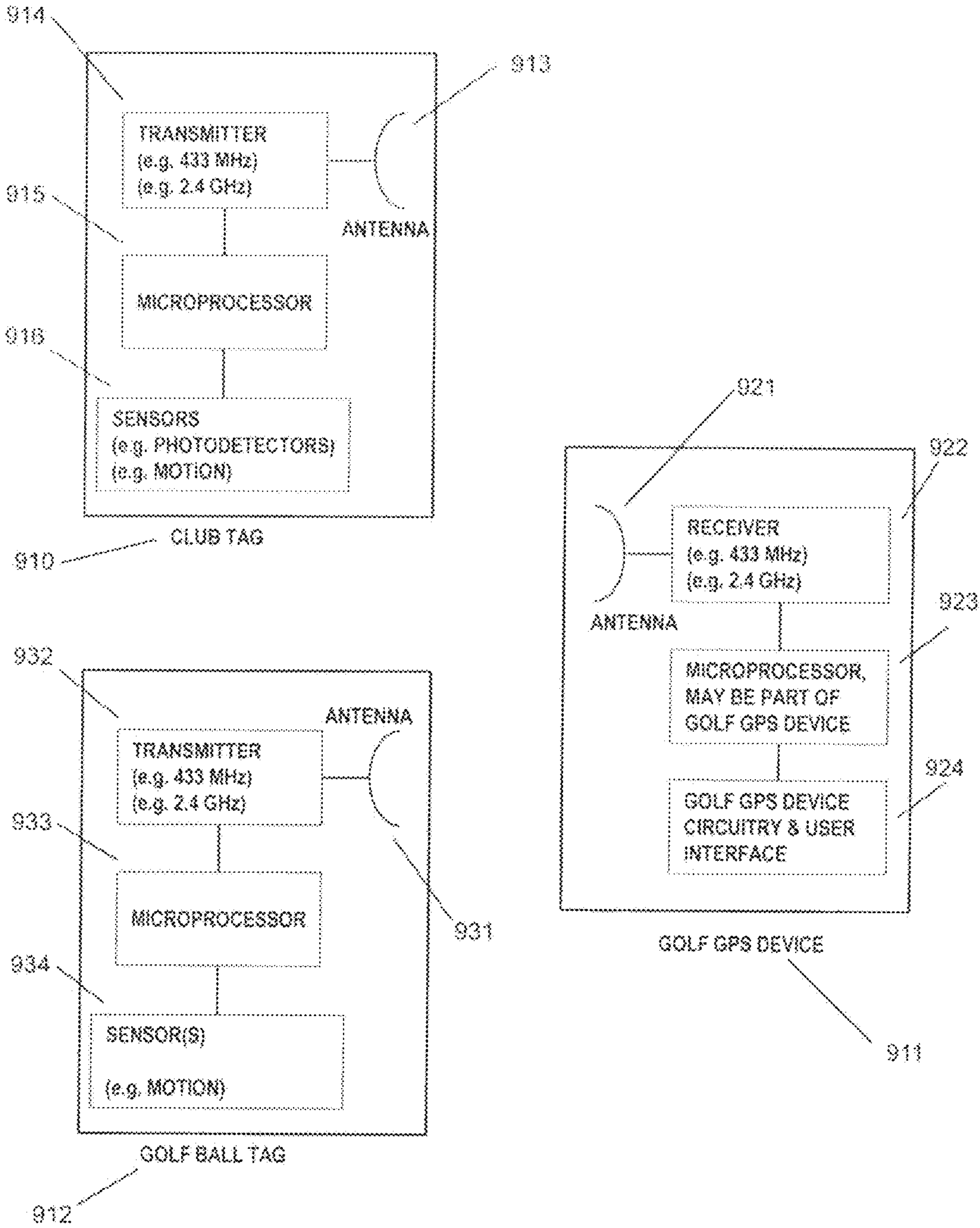
Figure 24A Tag System Block Diagram
