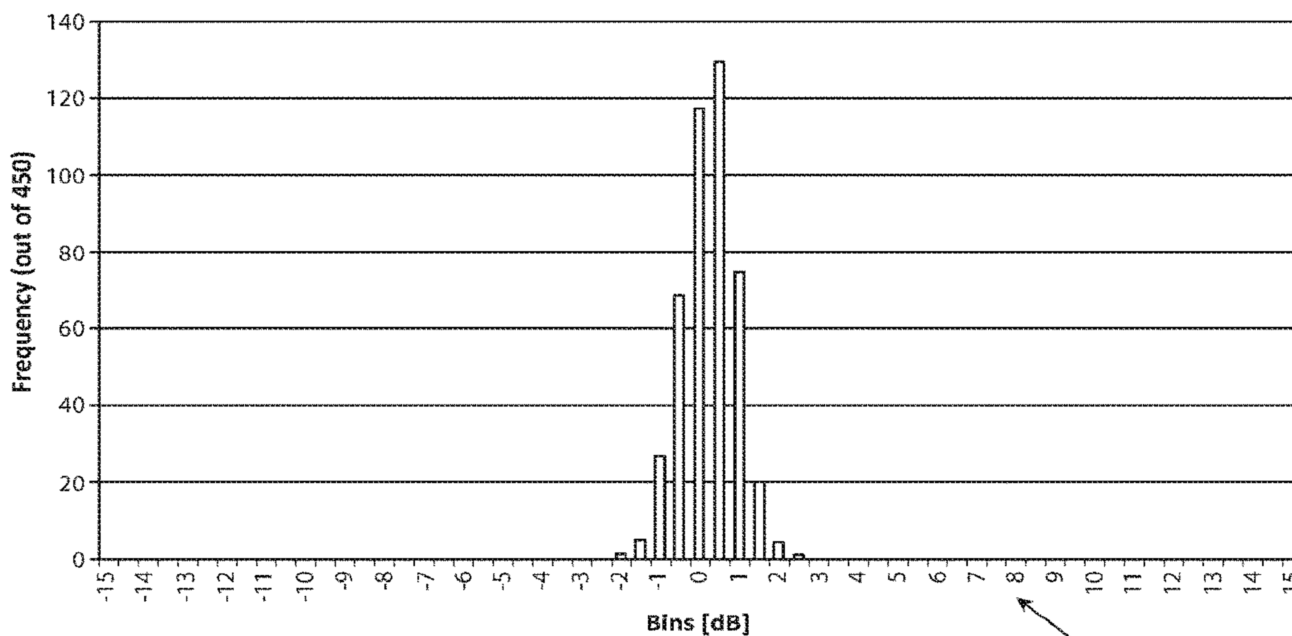
Distribution of samples after 64 averages
