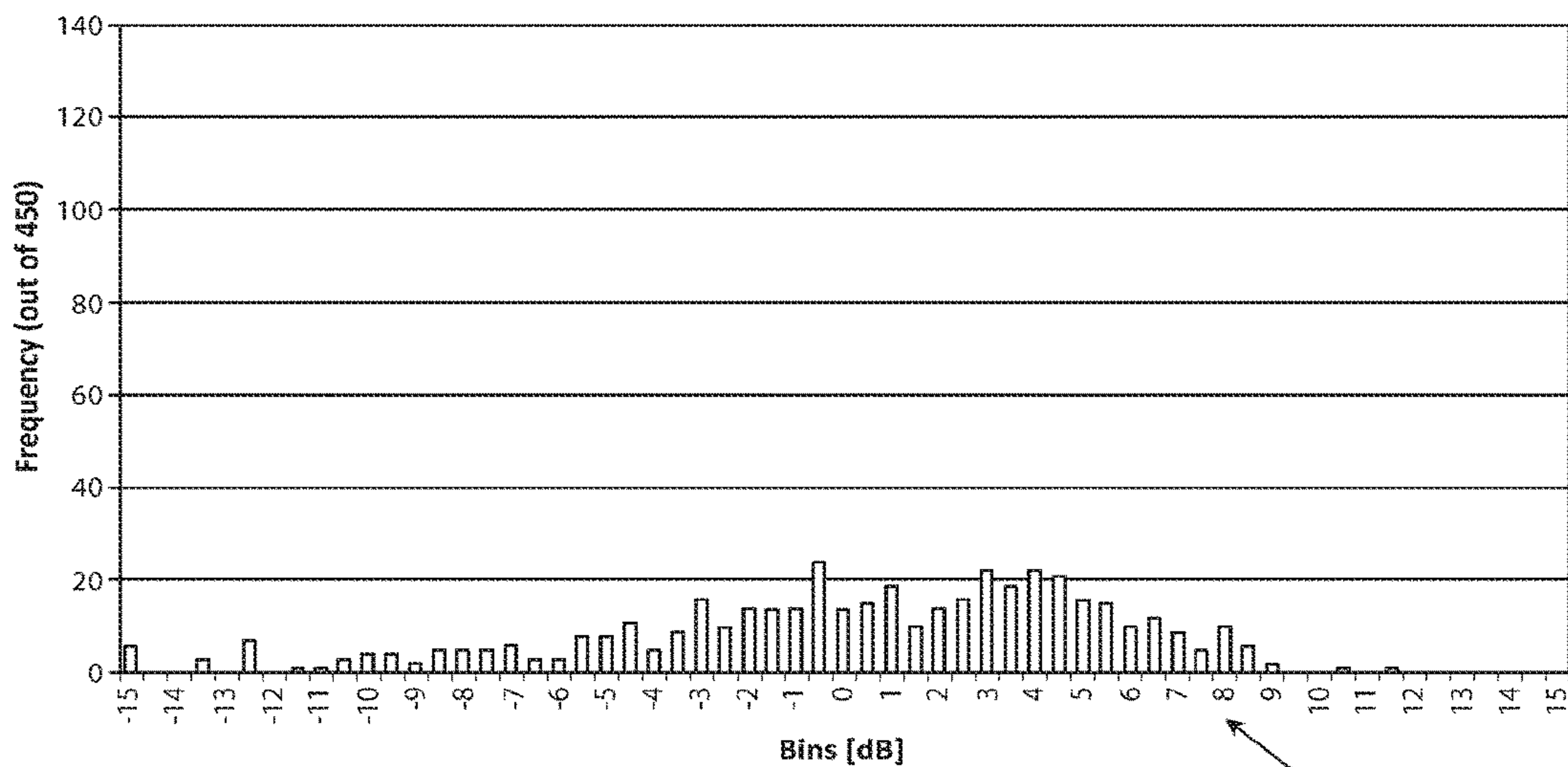
Distribution of samples after 0 averages
