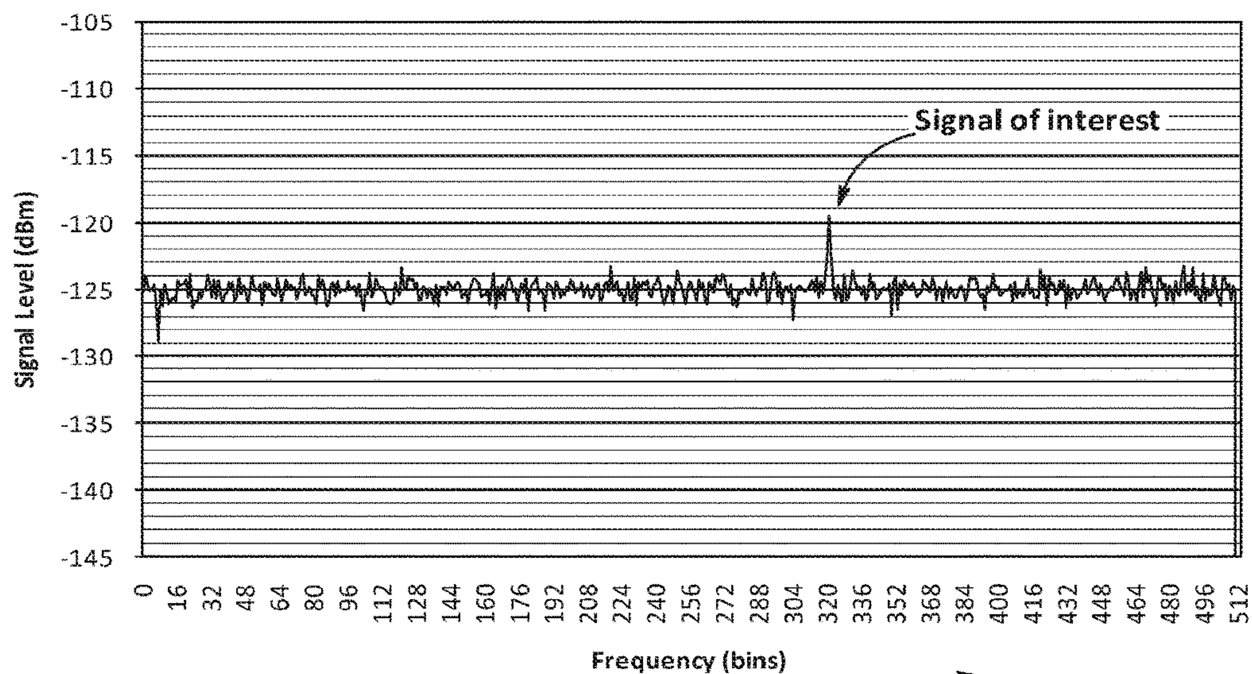
Frequency plot after 64 averages
