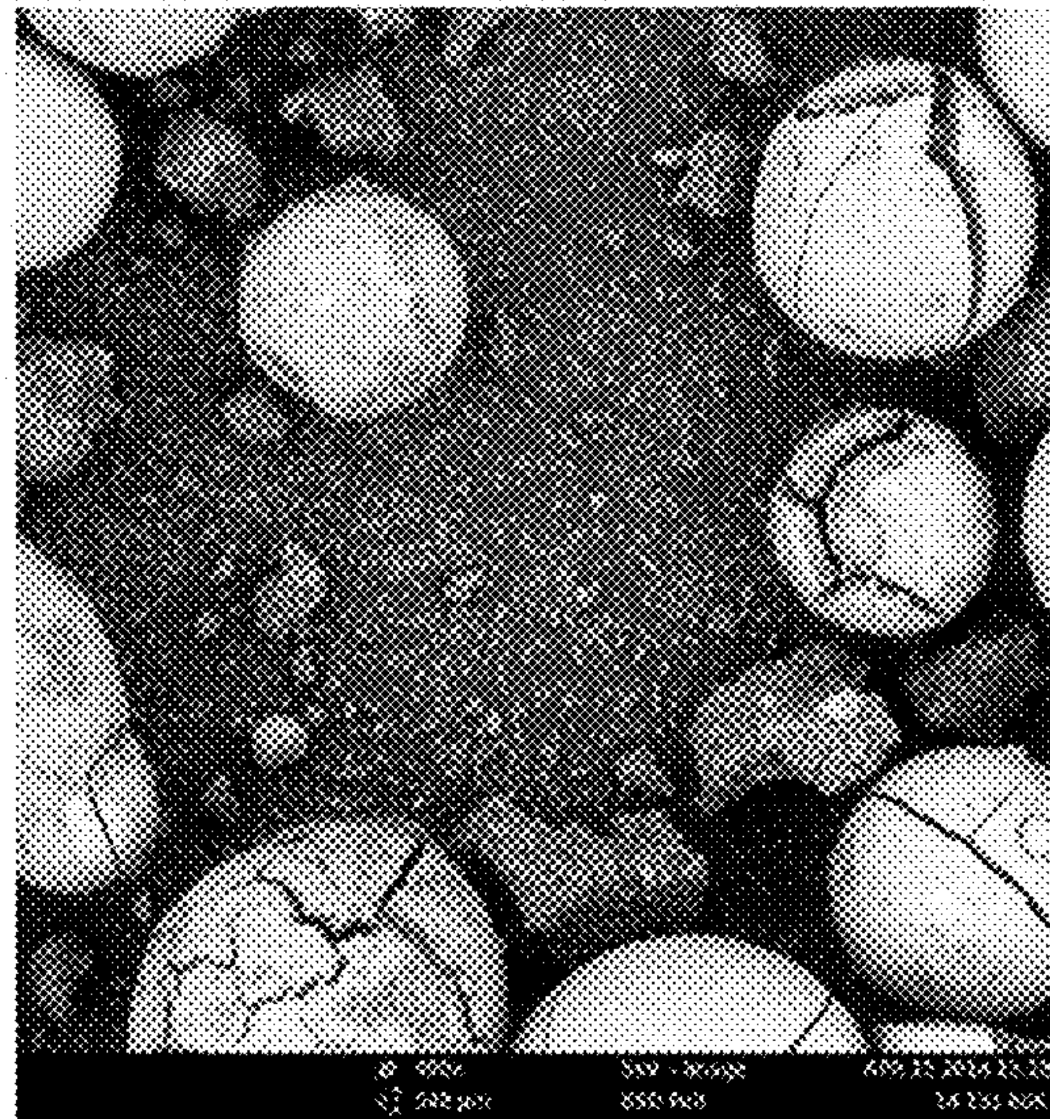
FIG. 7: sMAO AGC D150-60A Silica (High Temperature)
