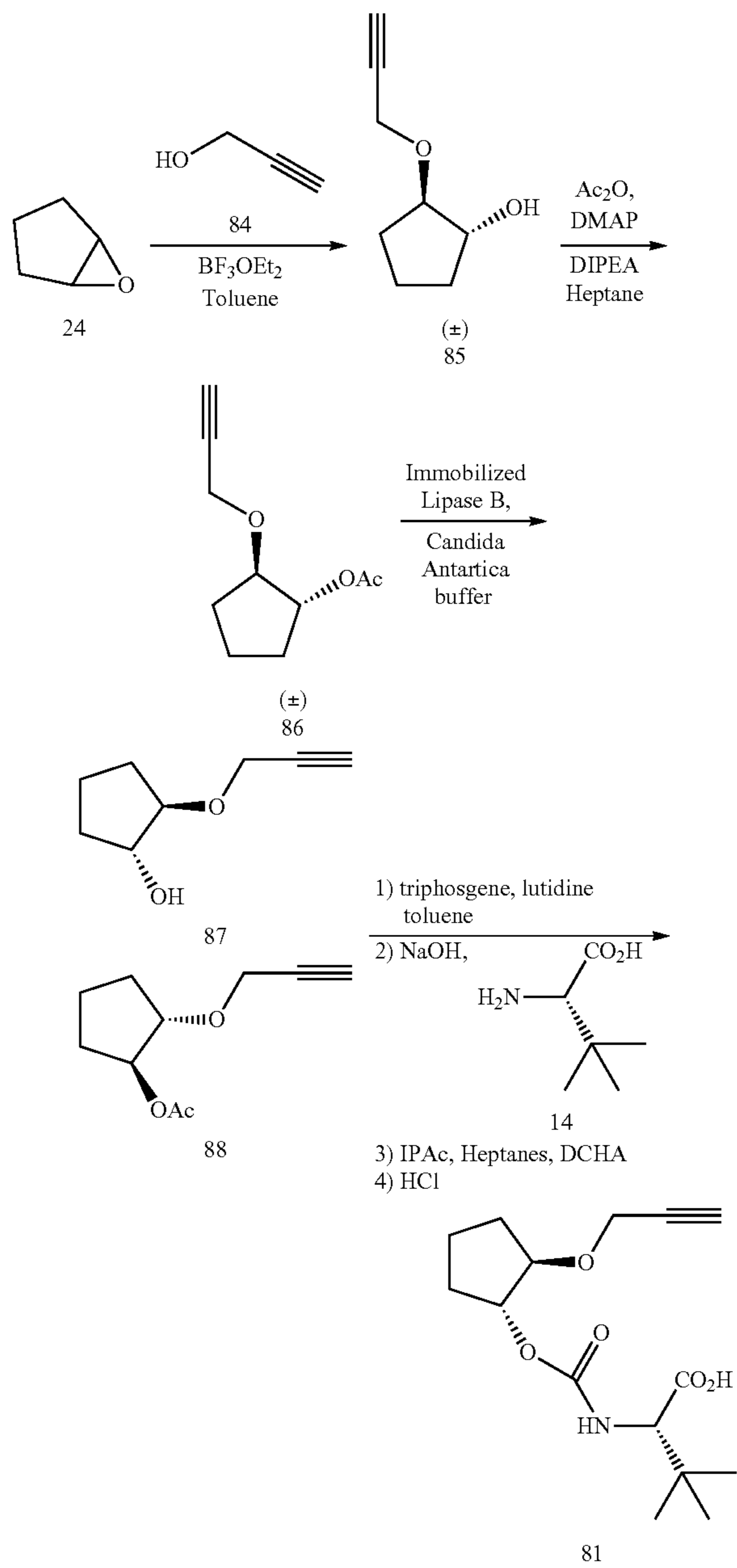
Scheme 5. Synthesis of 81
