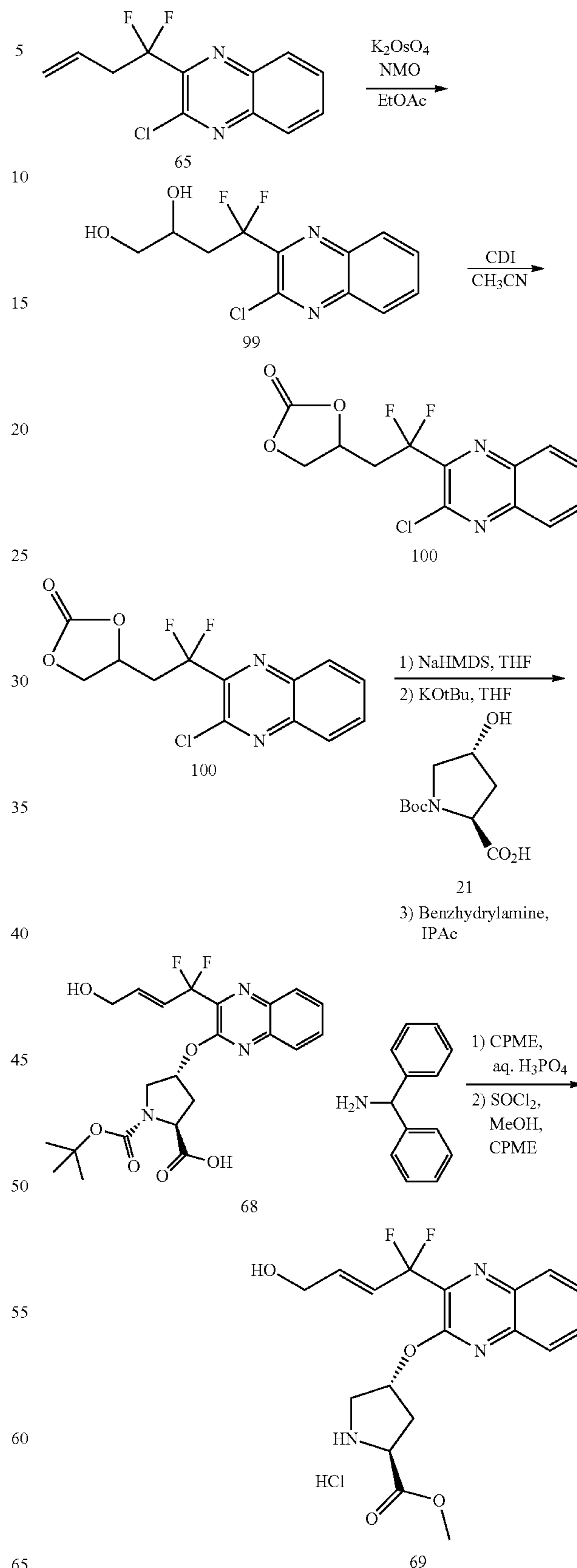
Scheme 11. Alternative Synthesis of 69
