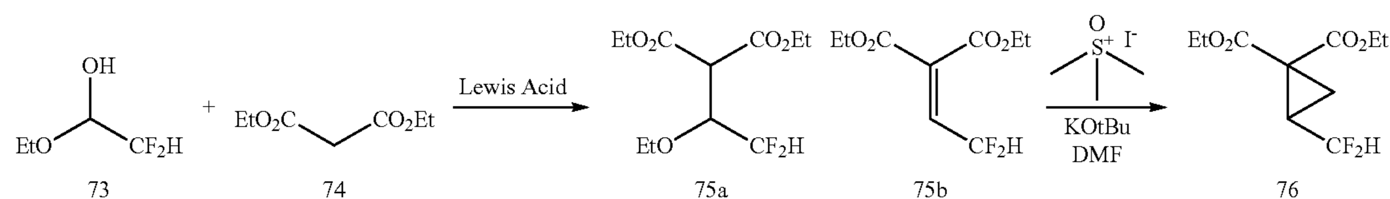
Scheme 7. Cyclopropanation Route for the Synthesis of 54
