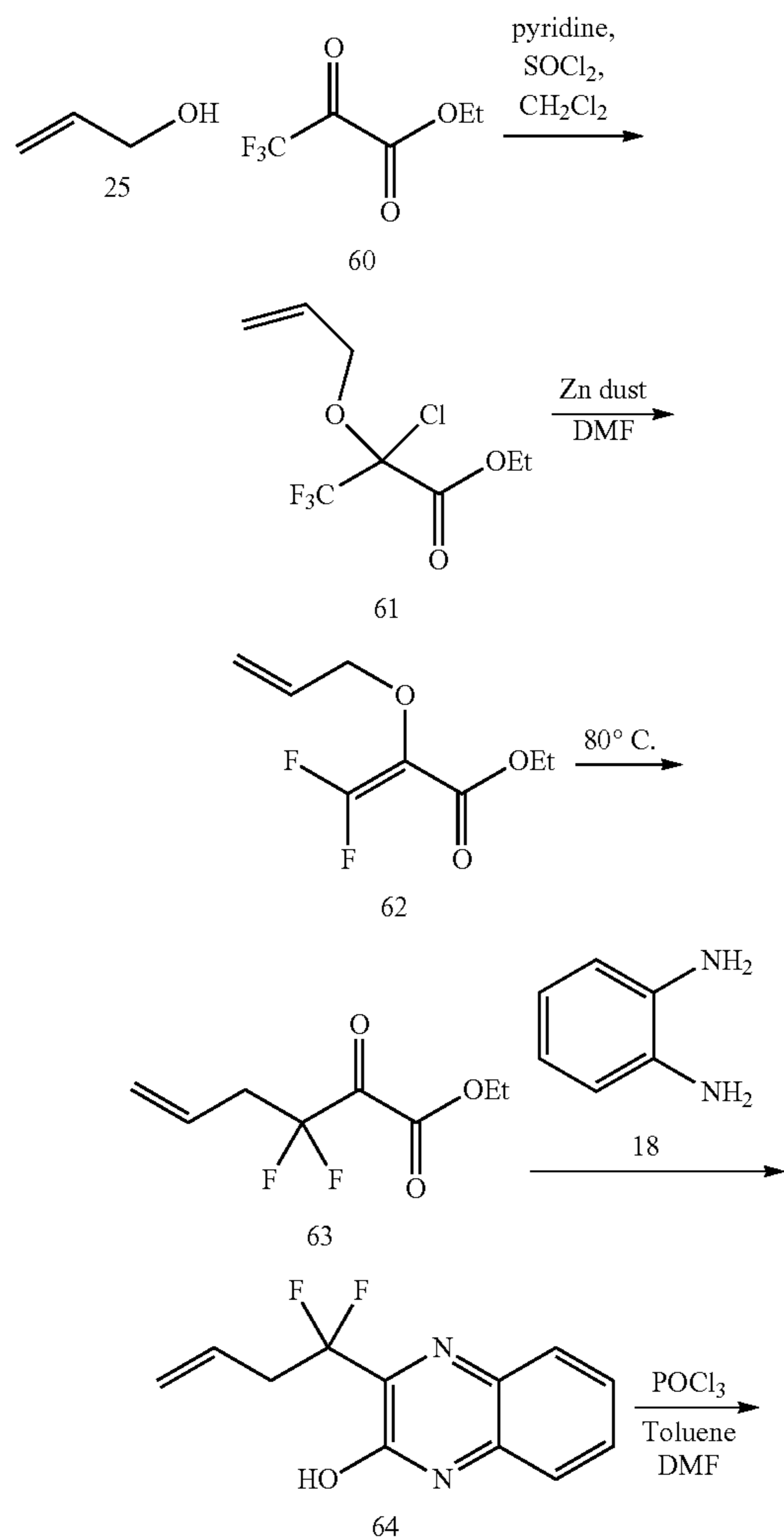
Scheme 3. Synthesis of 69
