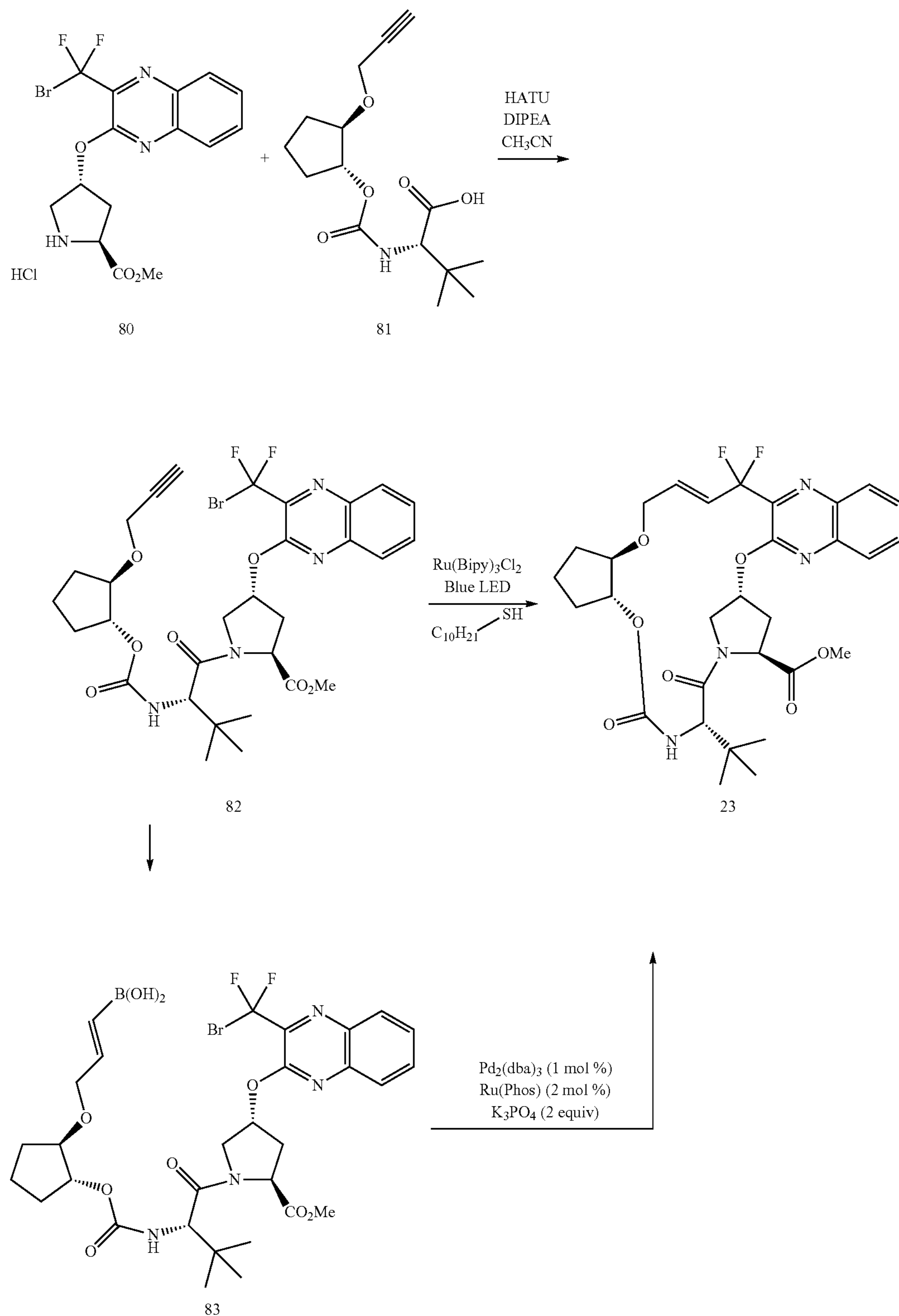
Scheme 4. Alternate Syntheses of 23
