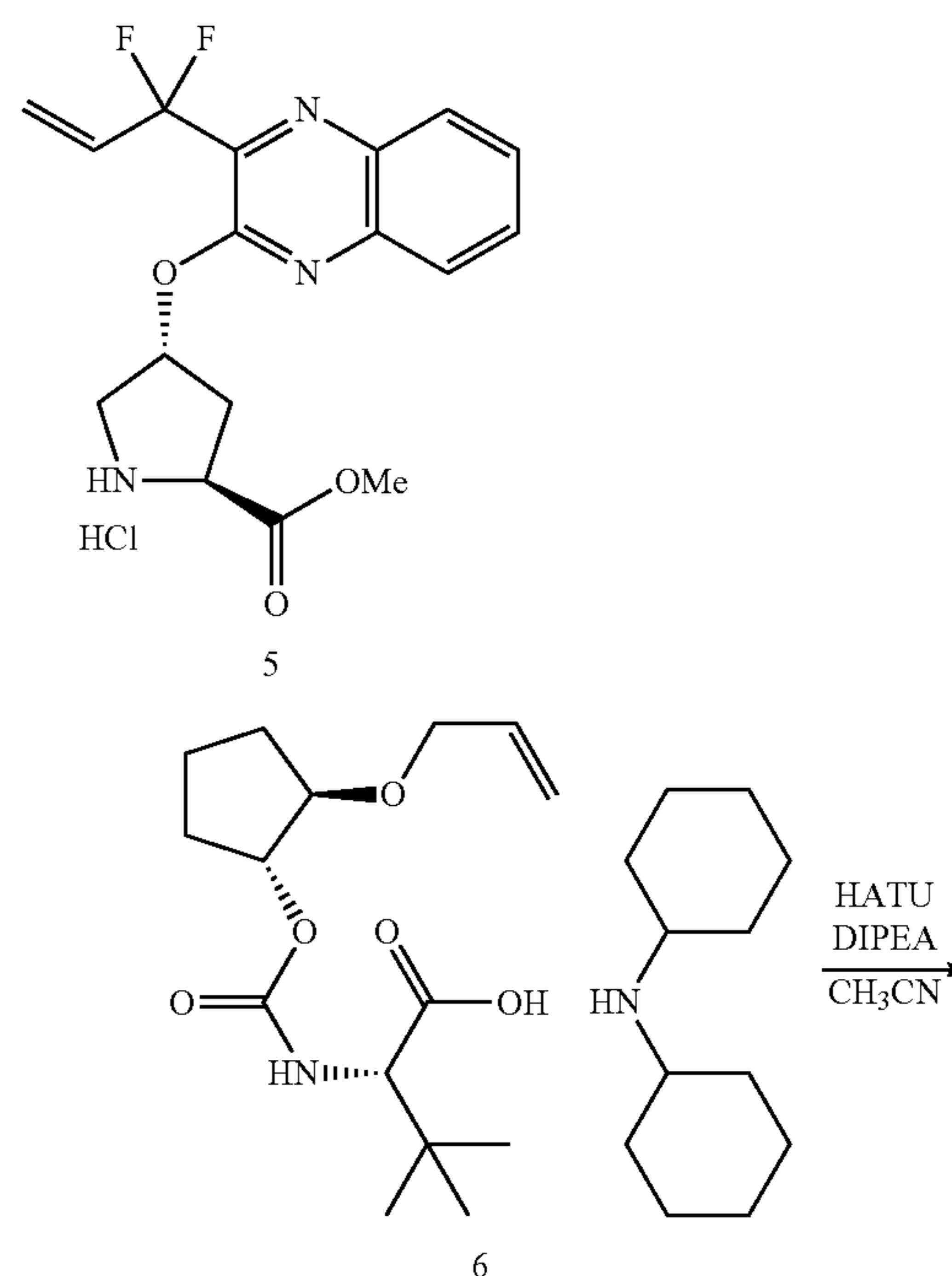
Scheme 9. RCM Route for the Synthesis of 1
