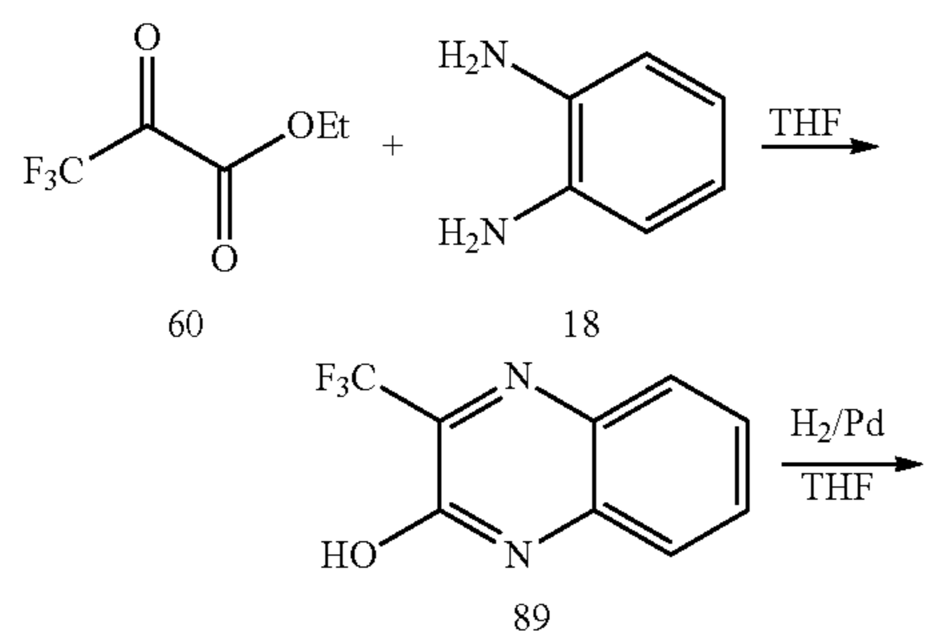
Scheme 6. Synthesis of 80
