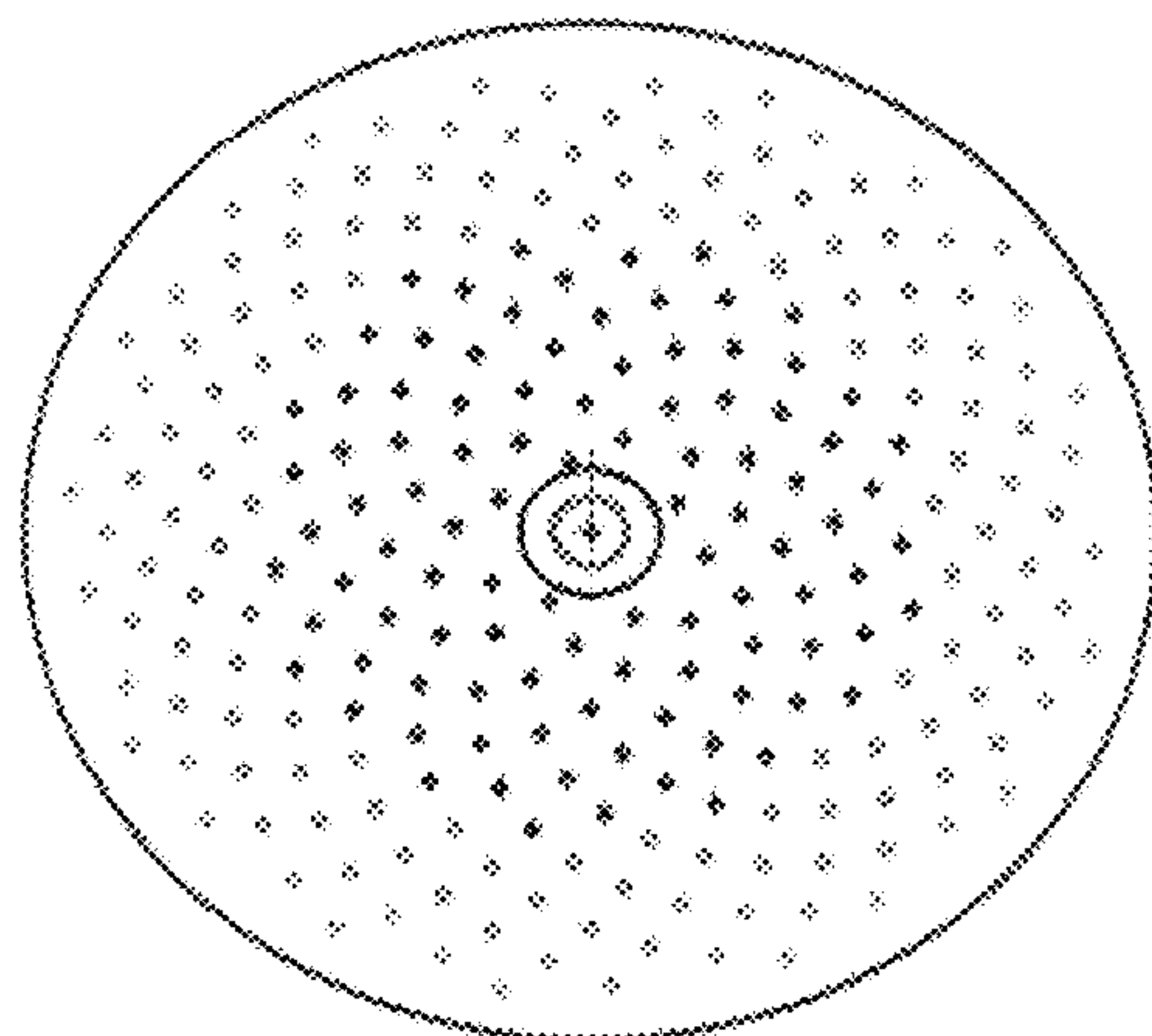
1.5 mm dia 246 holes 5" disc 5.0% removed area
