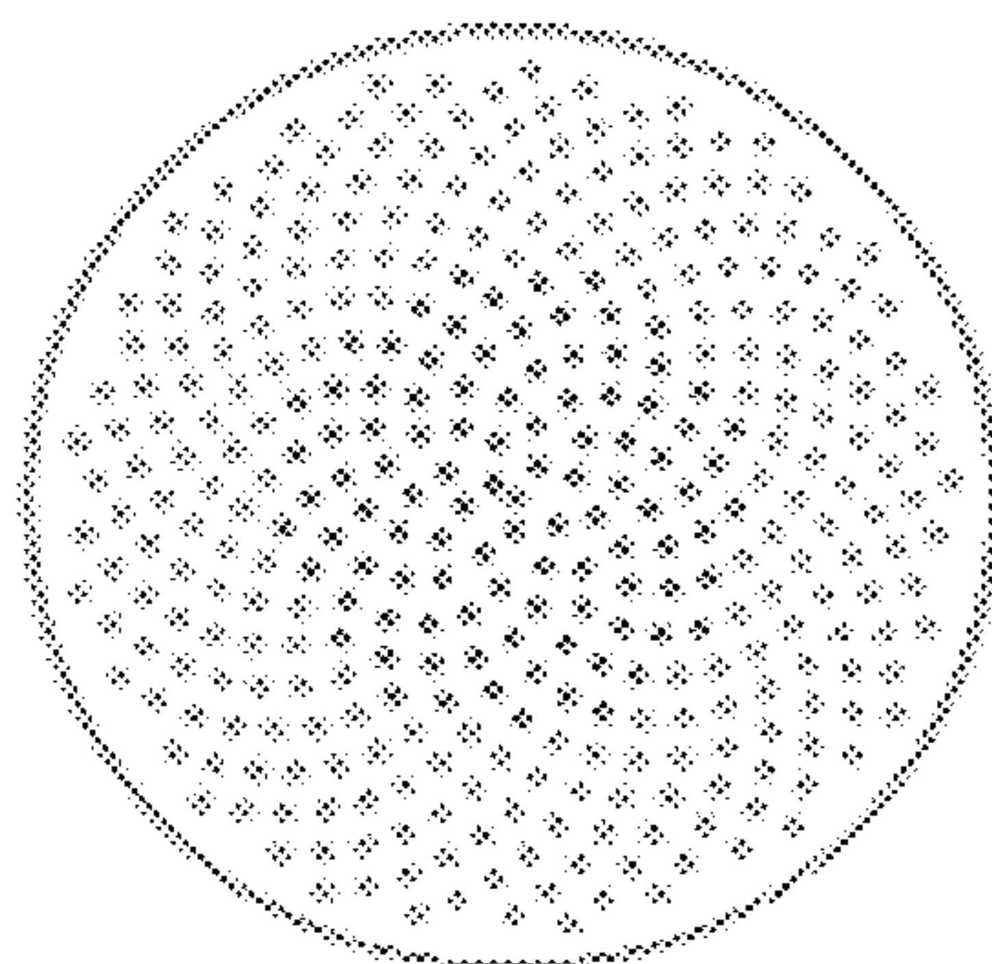
2.225 mm dia 350 holes 5" disc 10.7% removed area
