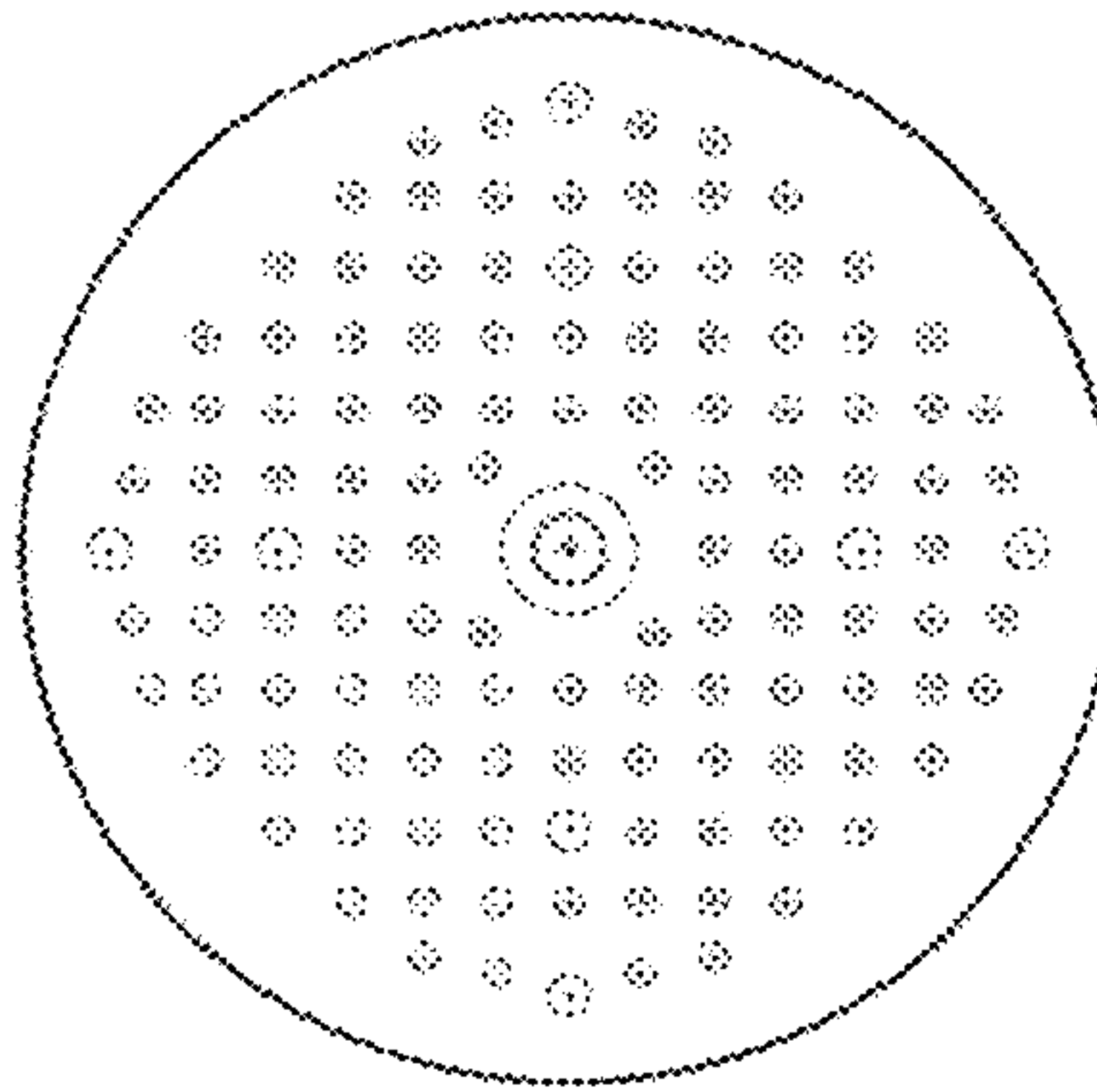
MultiAir 5" 125 holes 10.5% removed area
