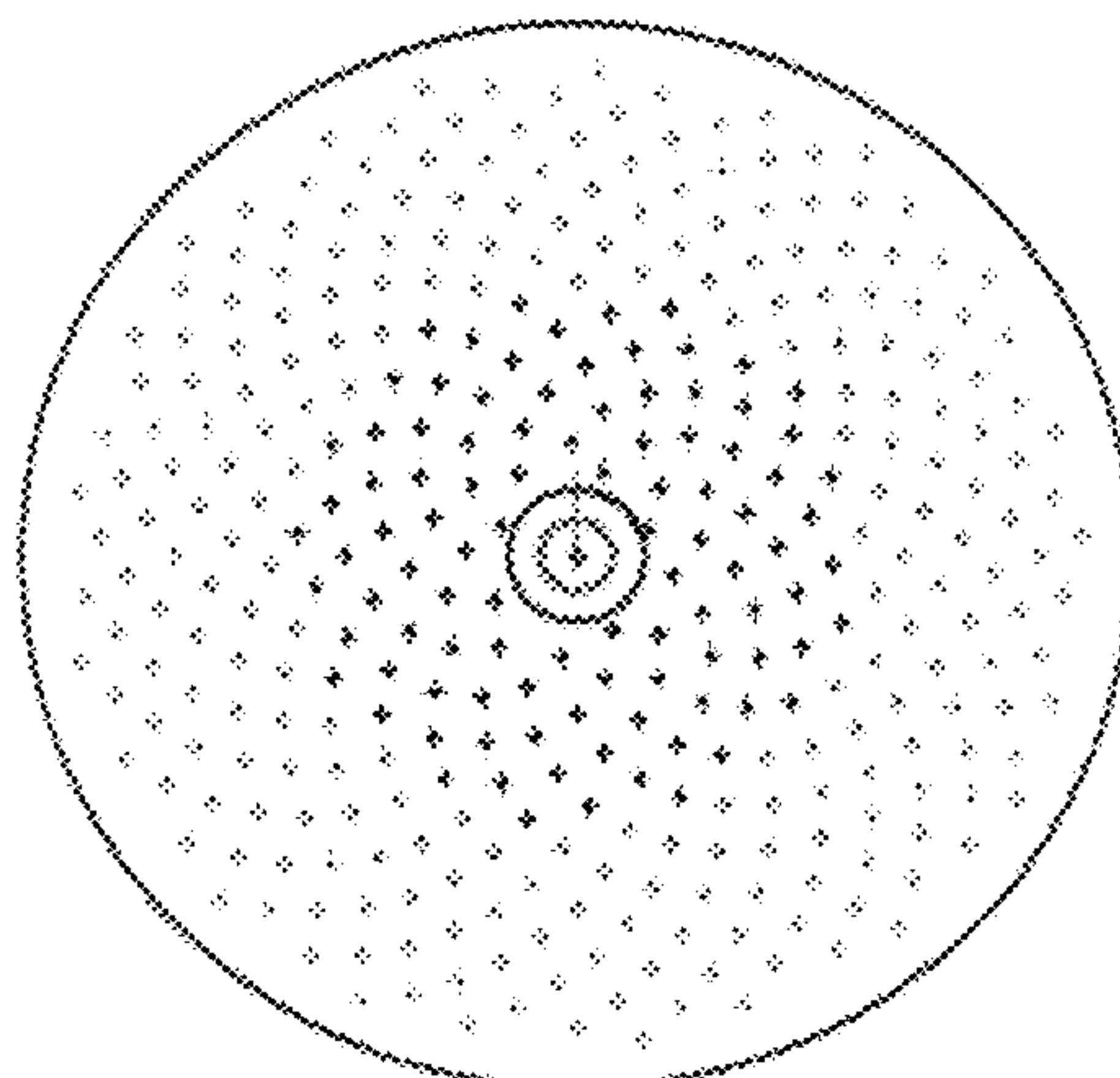
1.0 mm dia 344 holes 5" disc 3.7% removed area
