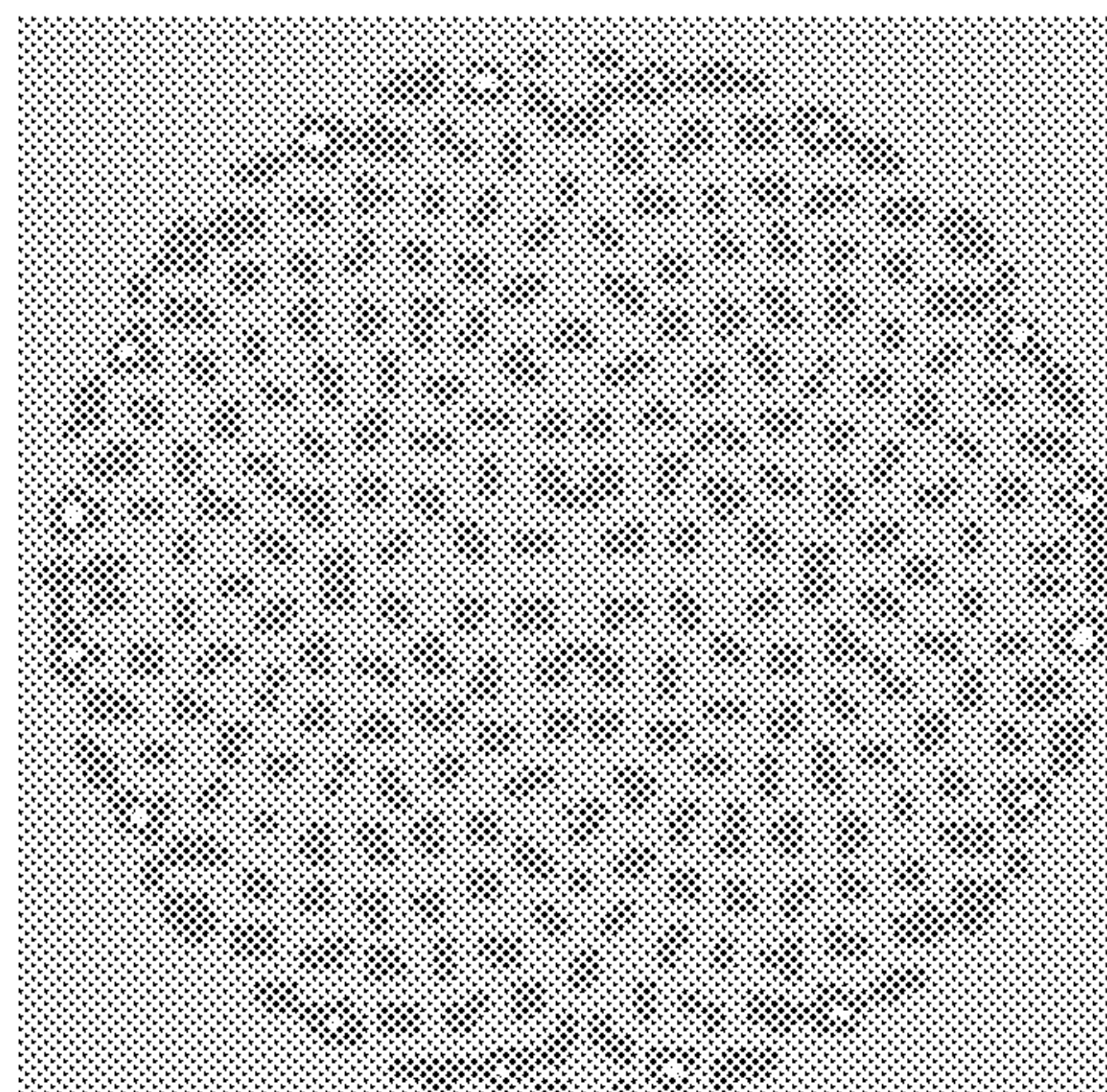
2.65 mm dia 250 holes 5" disc 10.8% removed area
