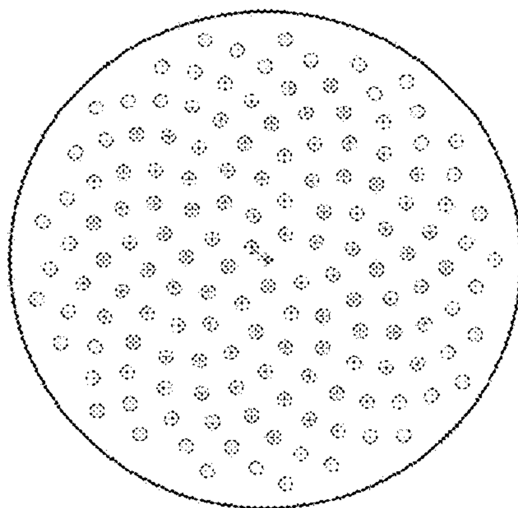
3.4 mm dia 150 holes 5" disc 10.7% removed area
