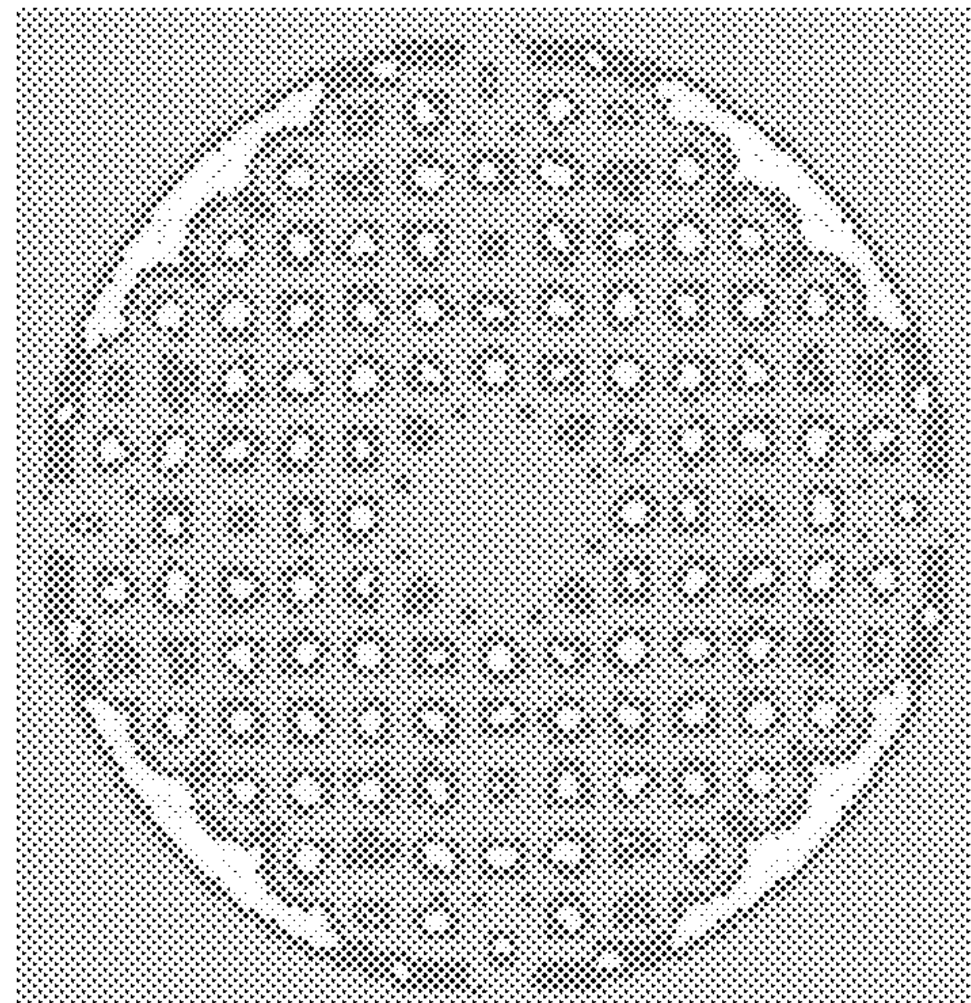
MultiAir 5" 125 holes 10.5% removed area
