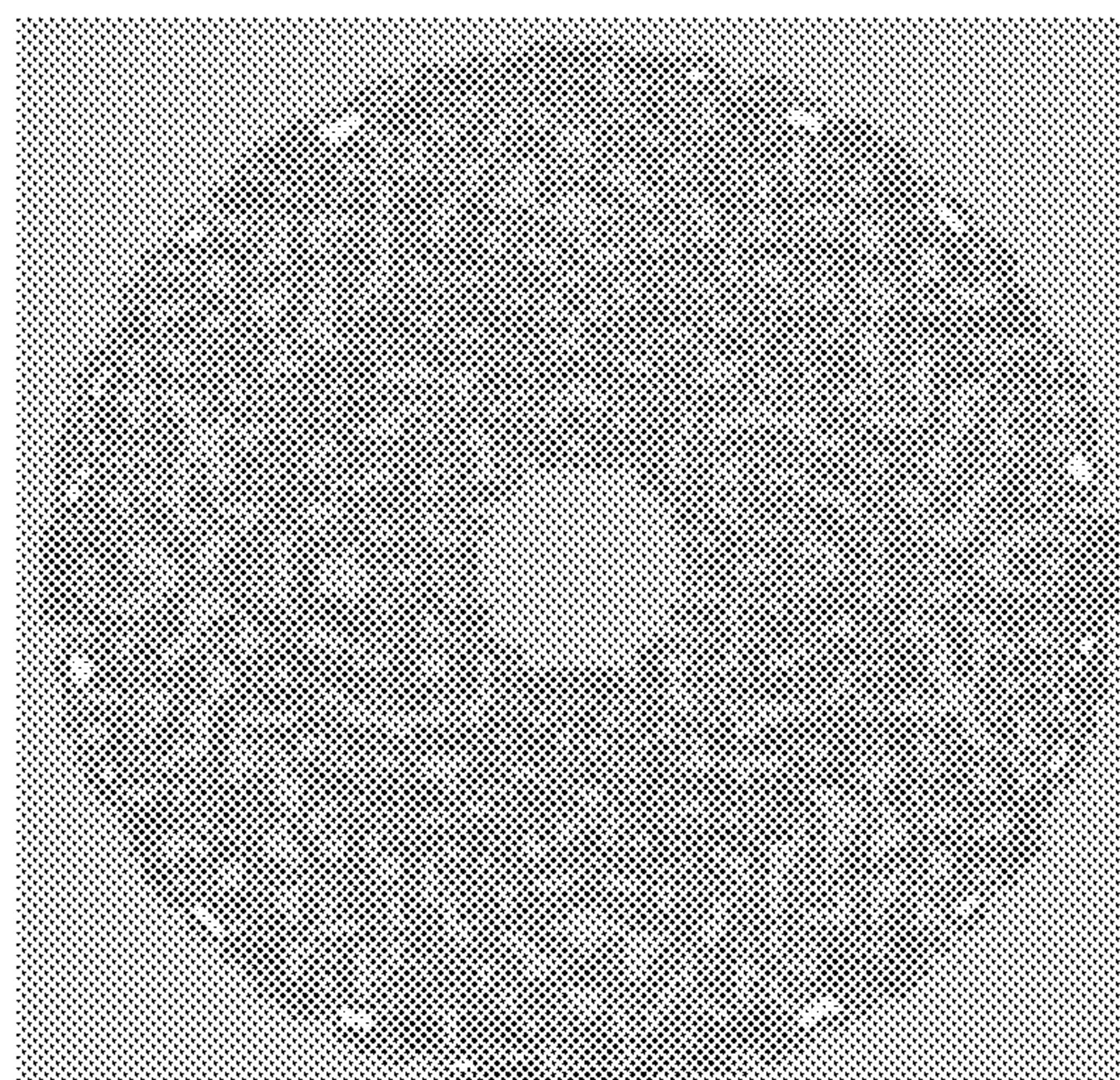
1.0 mm dia 344 holes 5" disc 3.7% removed area
