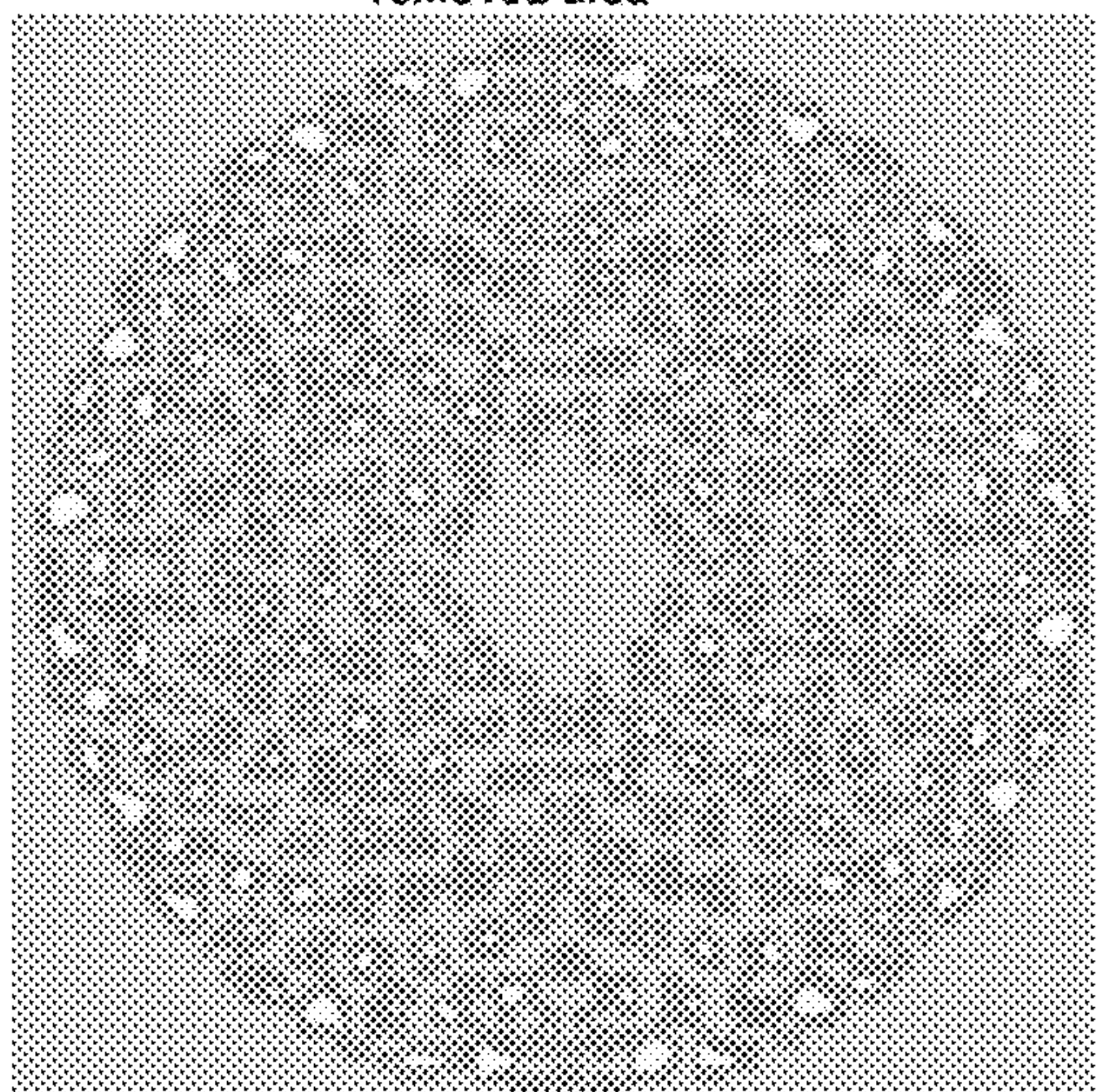
1.5 mm dia 246 holes 5" disc 5.0% removed area
