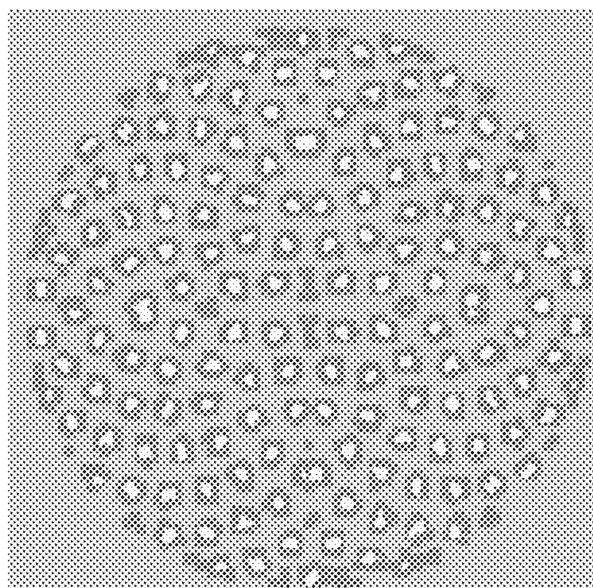
3.4 mm dia 150 holes 5" disc 10.7% removed area
