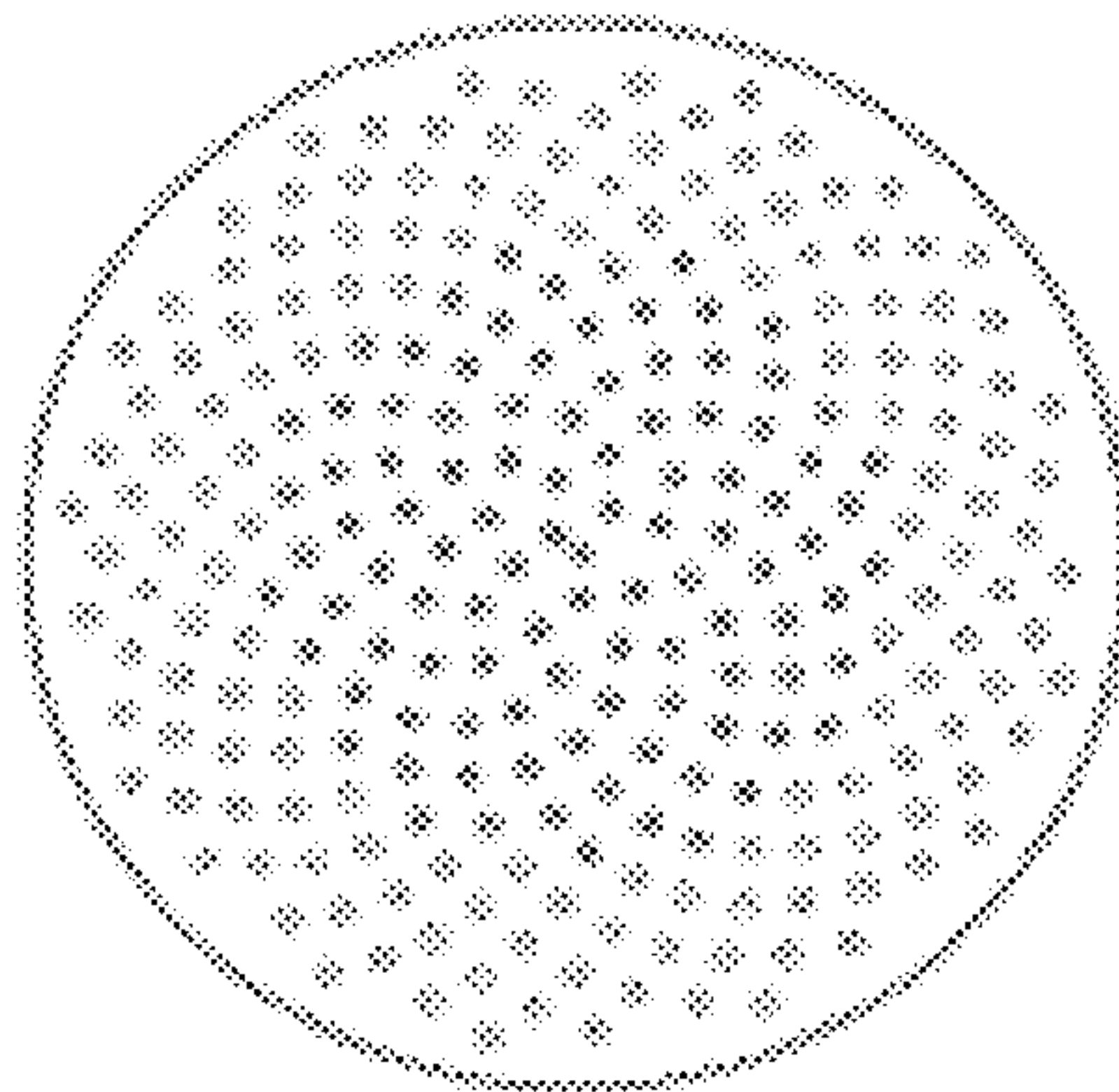
2.65 mm dia 250 holes 5" disc 10.8% removed area
