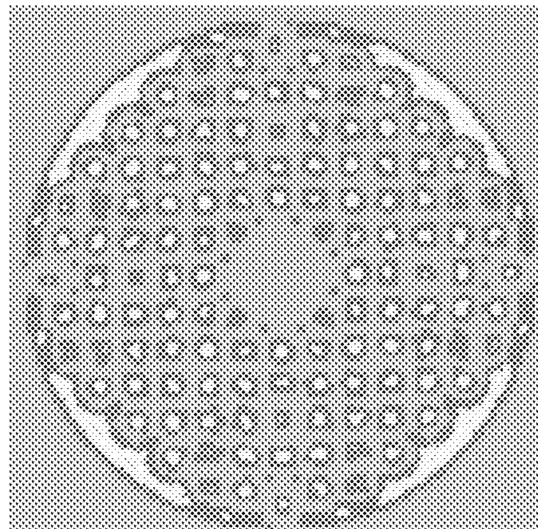
MultiAir 5" 125 holes 10.5% removed area
