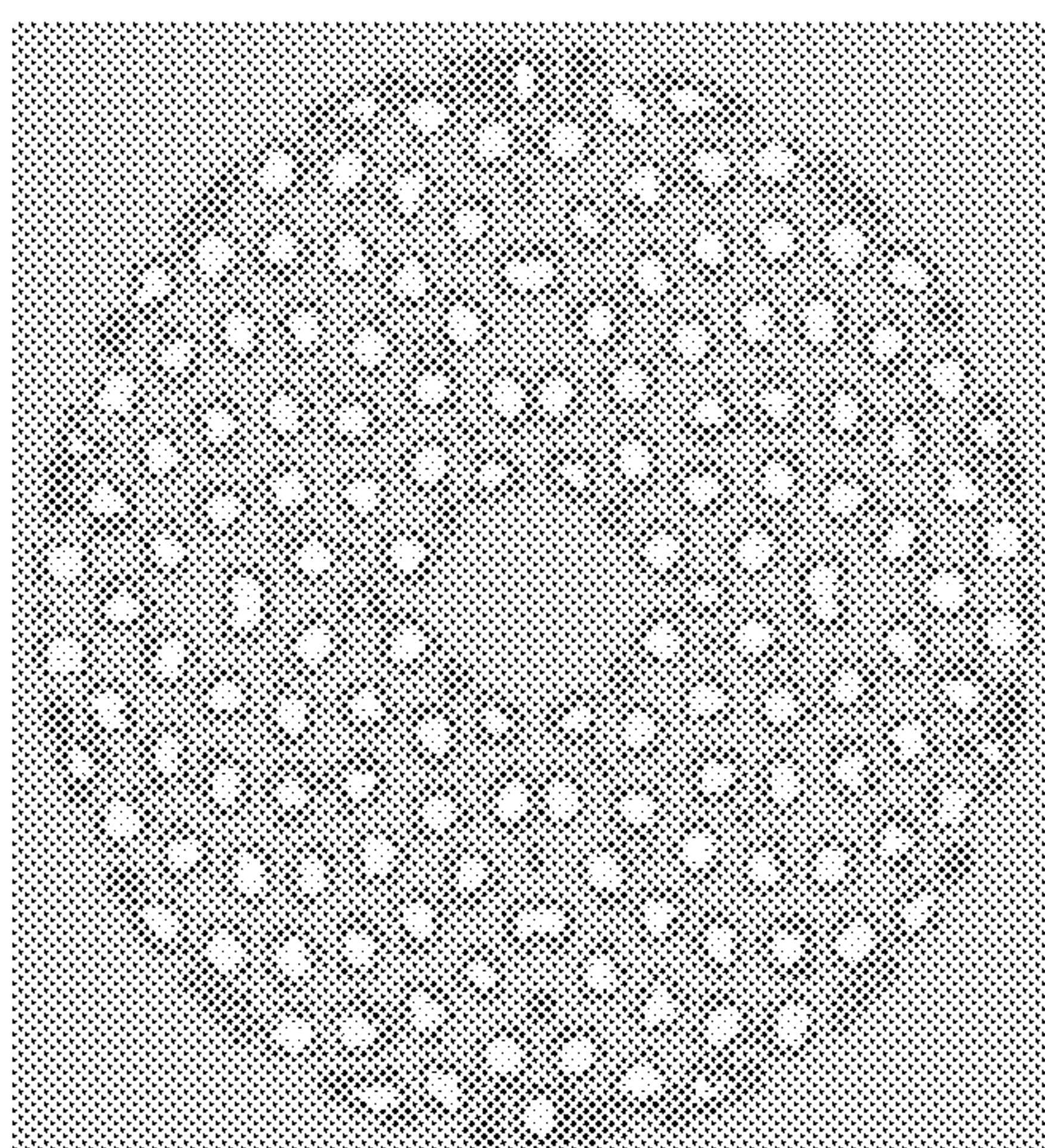
2.6 mm dia 148 holes 5" disc 7.8% removed area
