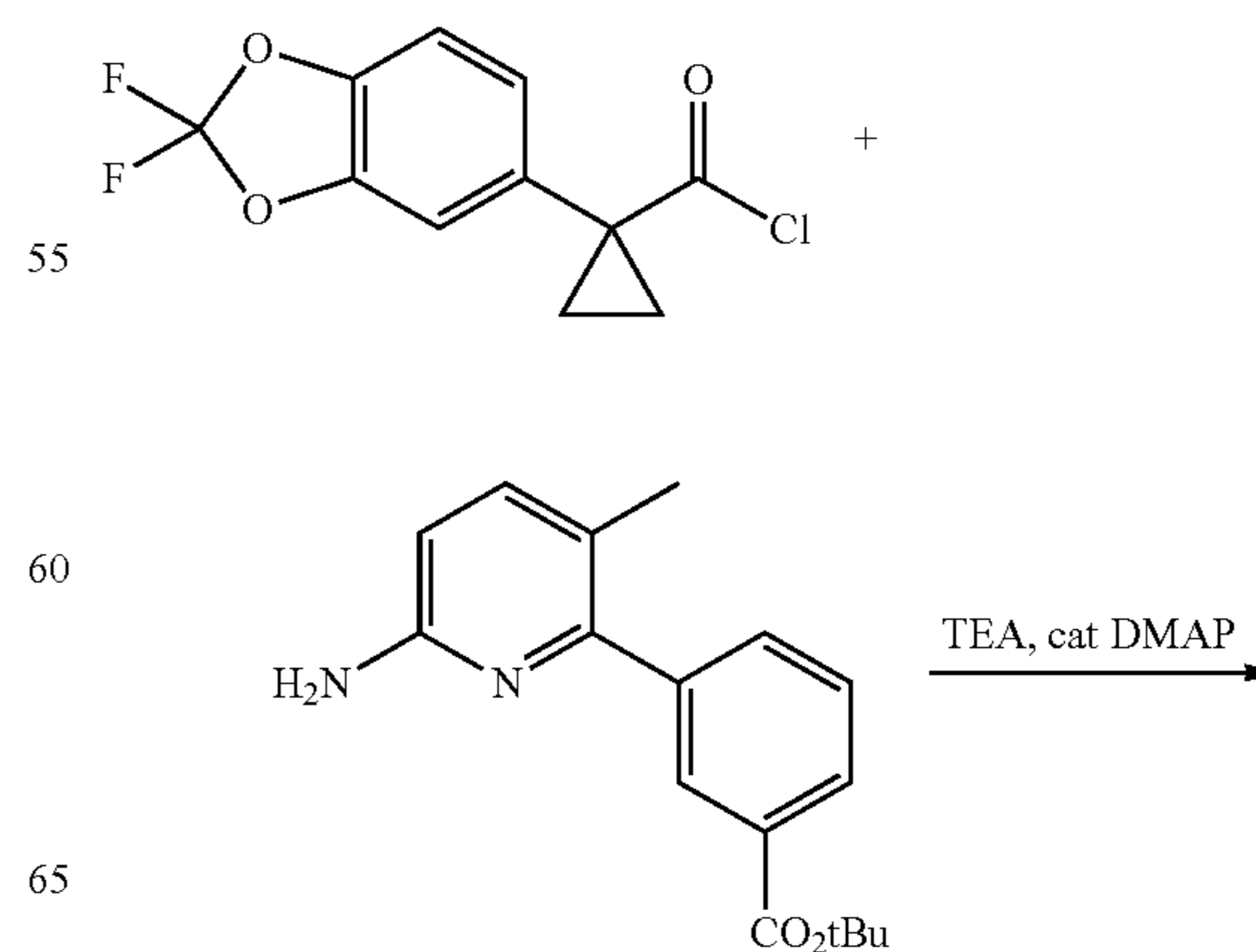
Scheme 4. Formation of an acid salt of 3-(6-(1-(2,2-difluorobenzo[d][1,3]dioxol-5-yl)cyclopropanecarbonyl)-3-methylpyridin-2-yl)benzoic acid.
