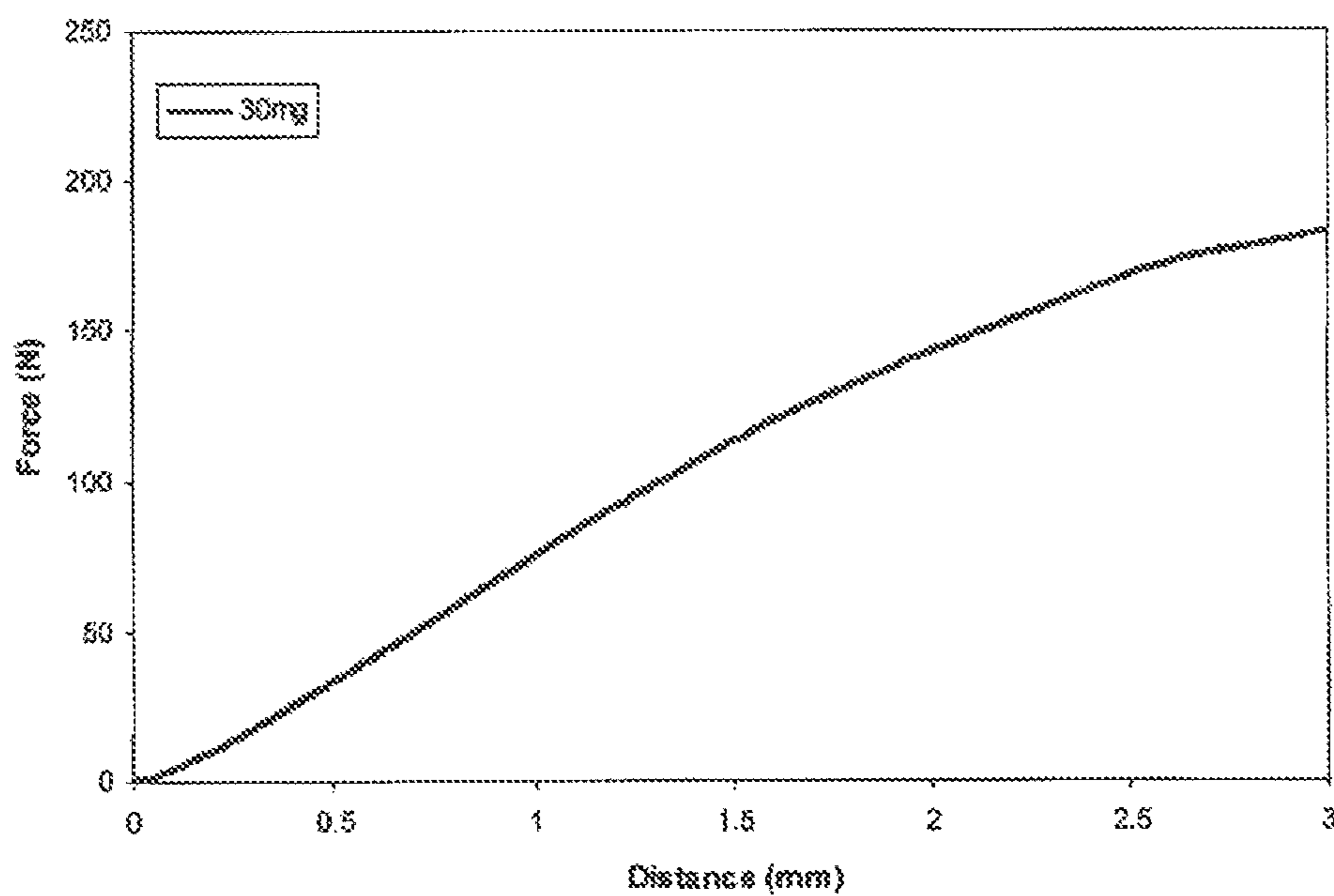
Example 20 Indentation Test of Example 13.4 tablet
