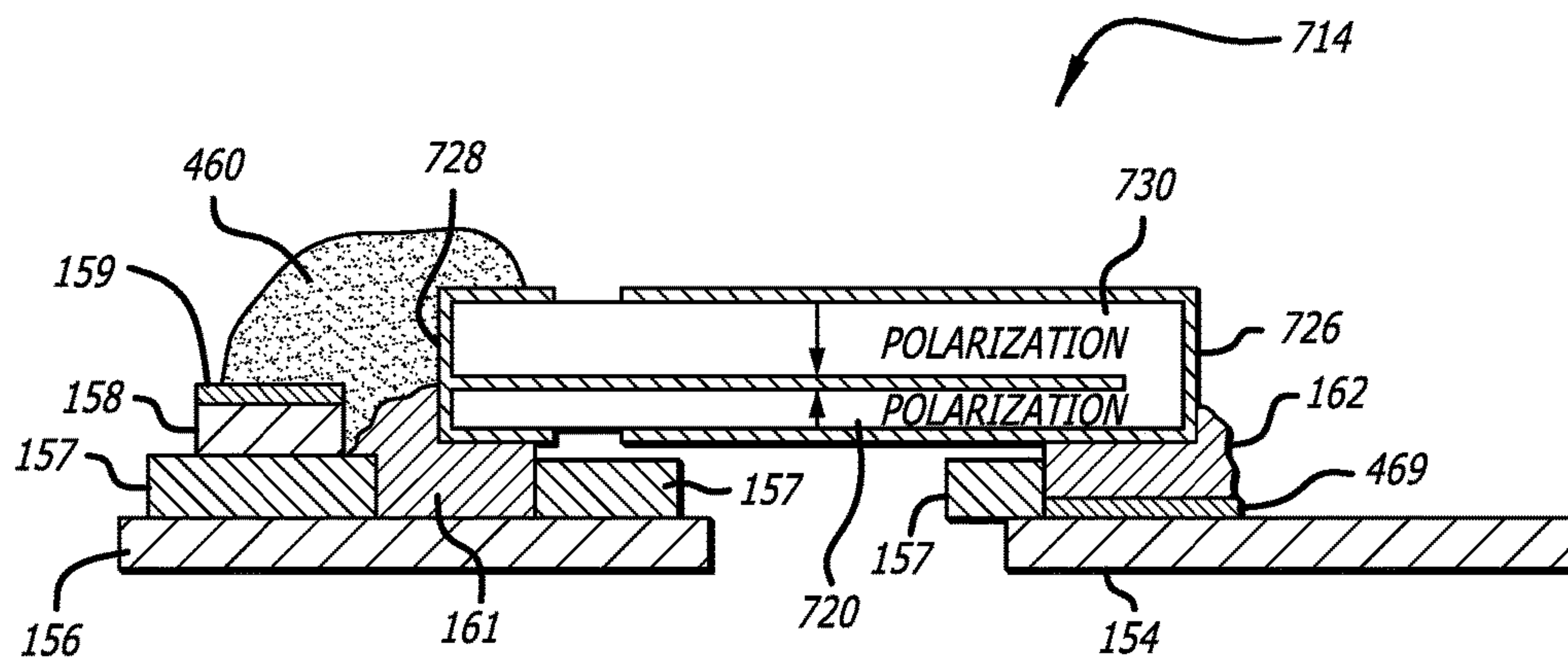
FIG. 41 COMMONLY POLED
