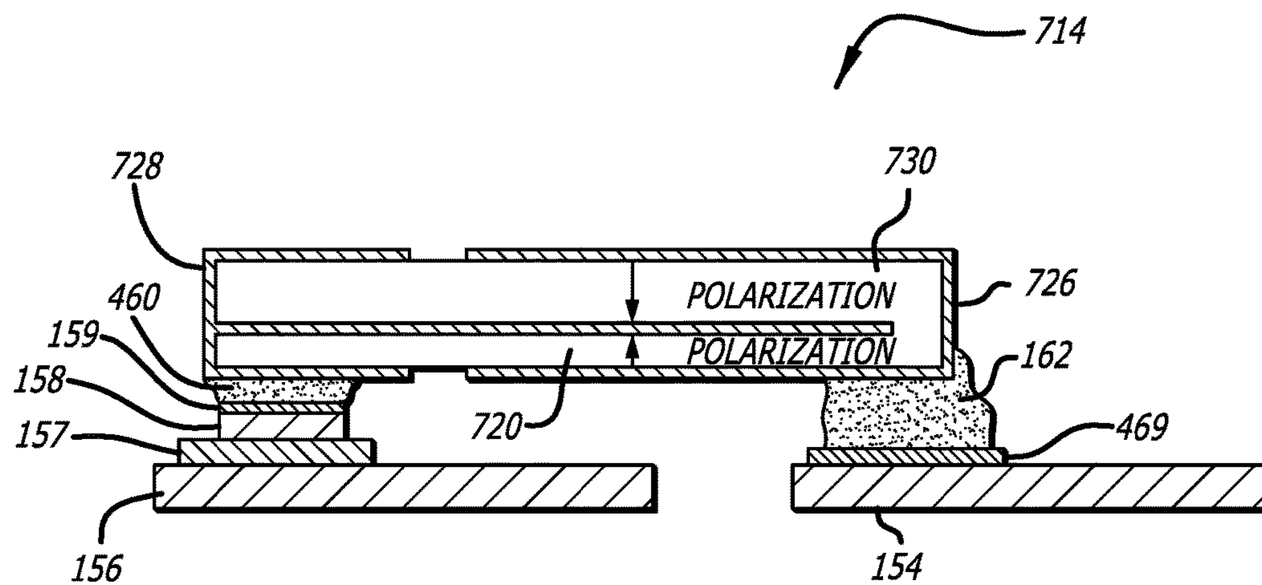
FIG. 37 COMMONLY POLED
