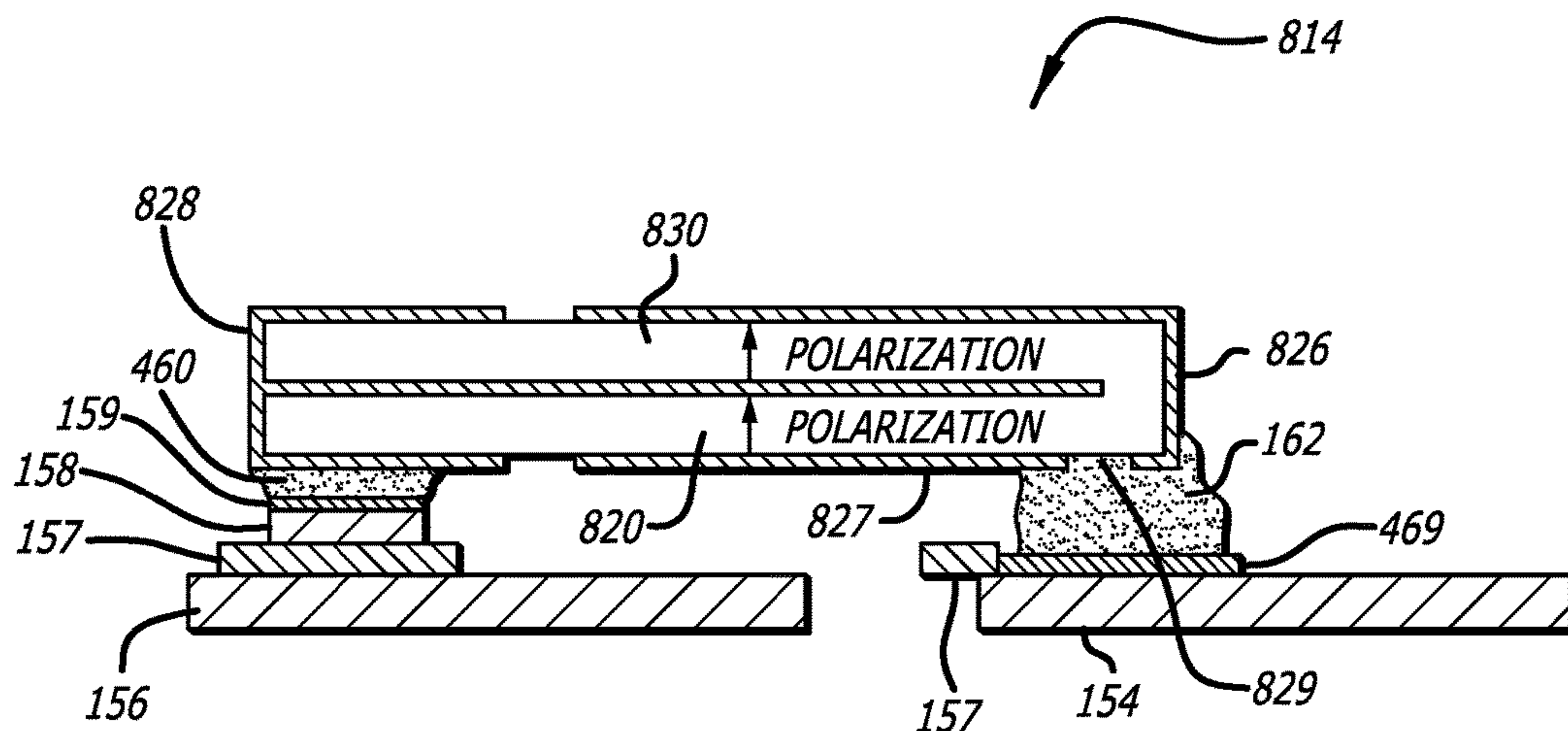
FIG. 39 OPPOSITELY POLED
