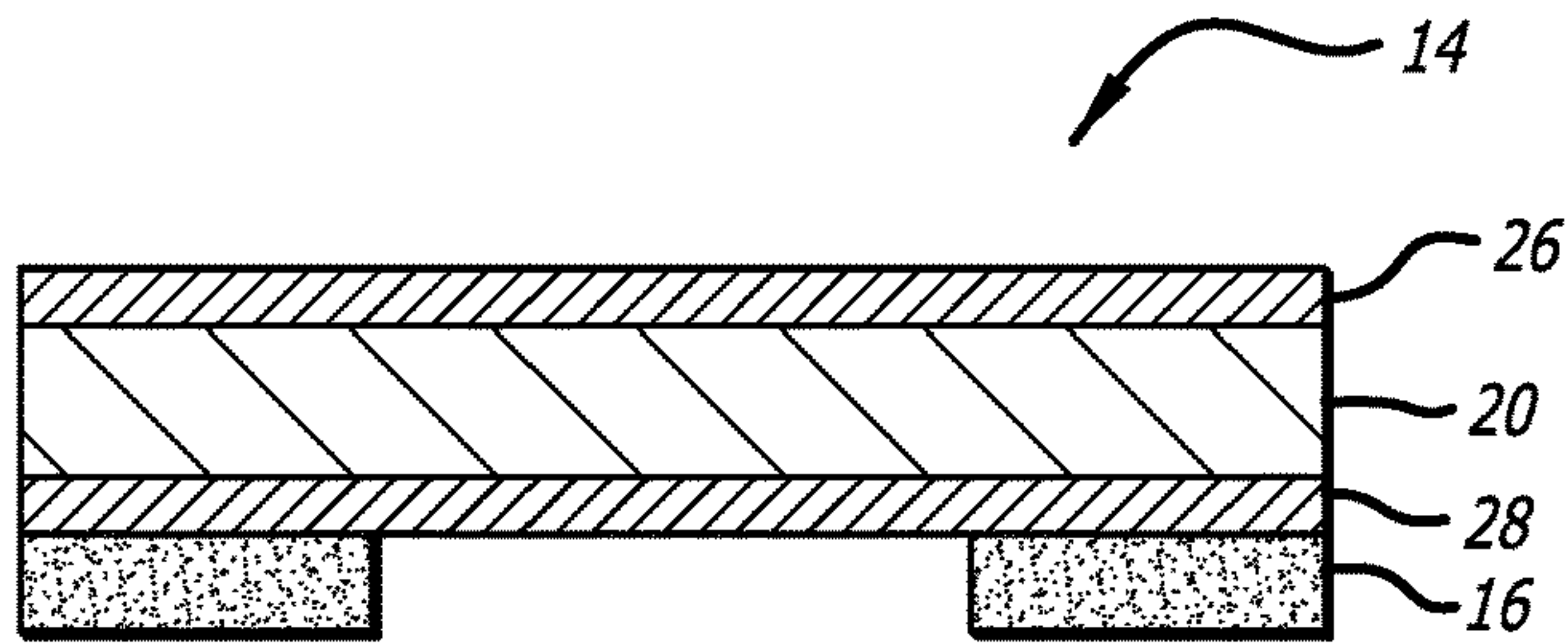
FIG. 3 (Prior Art)
