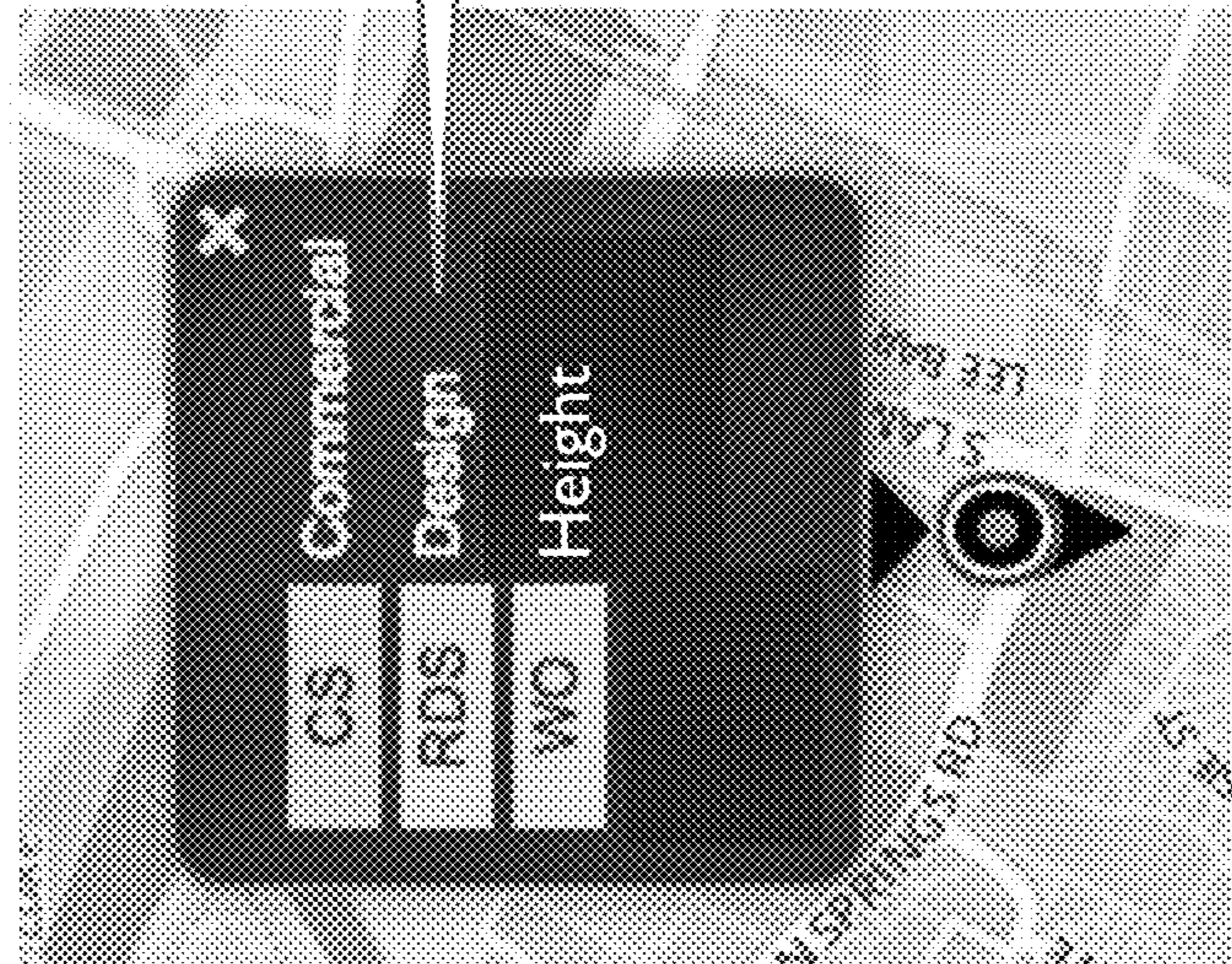
Fig 32 - Data Output
