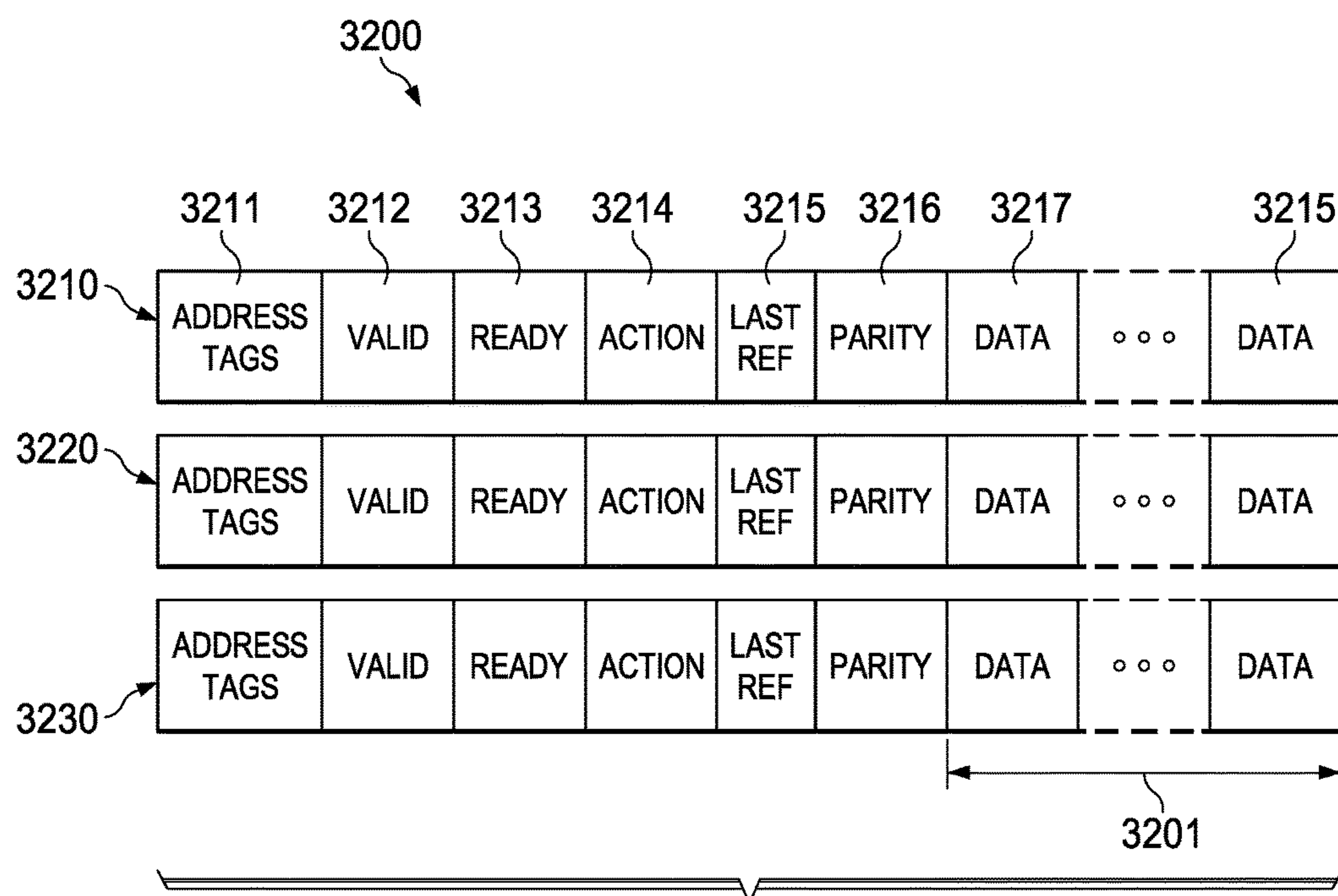
FIG. 32 (PRIOR ART)
