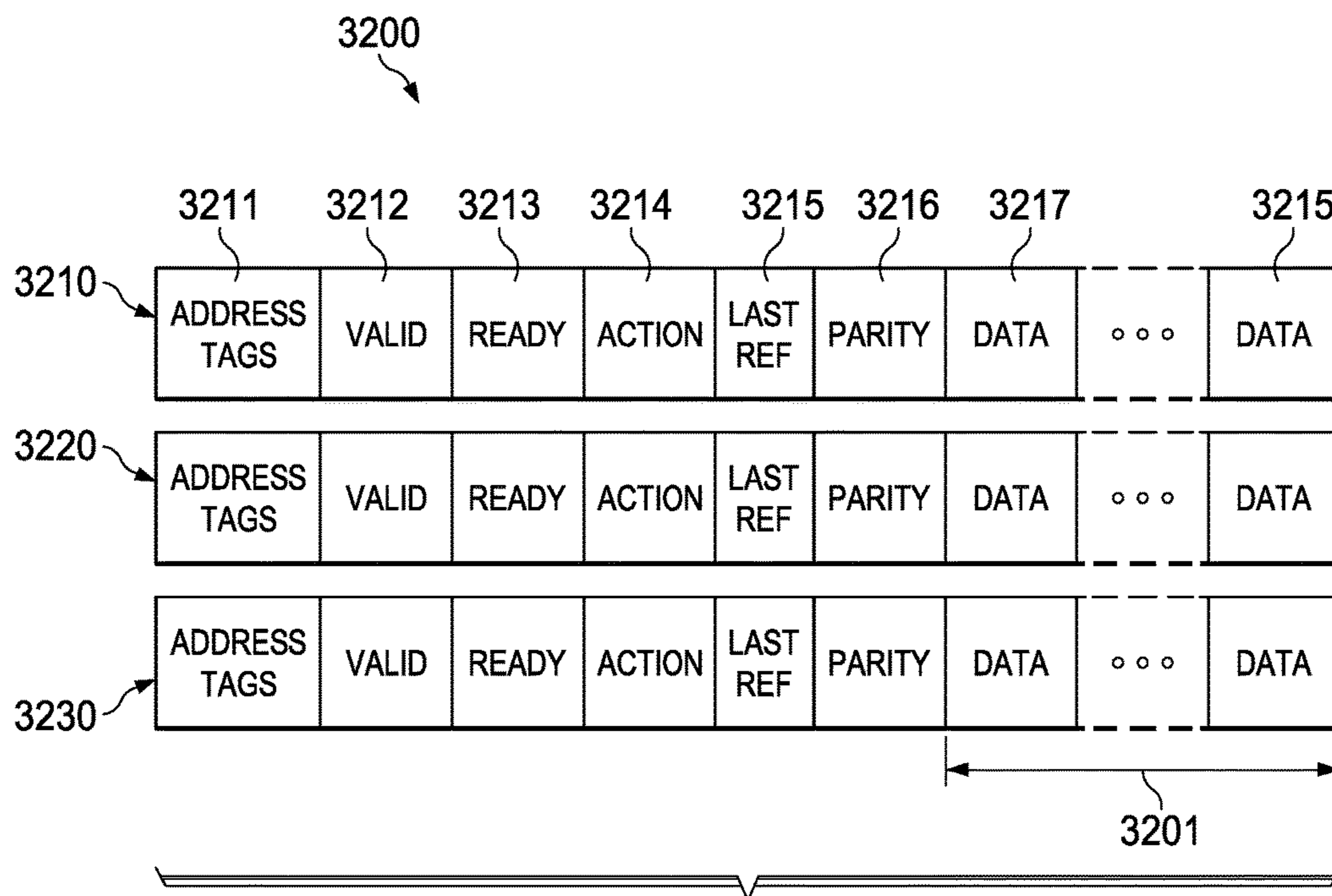
FIG. 32 (PRIOR ART)
